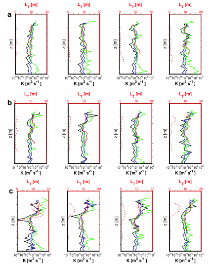
Figure 5. Panel a L_T (red dotted line), K_G (black line), K_{PP} (blue line) K_T (green line) and K_v (red line) for stations 9, 11, 14 and 18; panel b for stations 43, 45, 46 and 48 and panel c for stations 78, 82, 87 and 92
