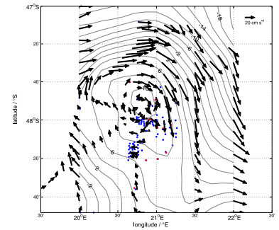
Figure 2. ADCP velocity vectors averaged between 150 and 200 m and 10 km along track and streamfunction [ 1000 \text{ m}^2 \text{ s}^{-1} ] showing a closed cyclonic circulation centered at 47.85°S, 20.75°E, which extends over roughly 100 to 150 km diameter. Probably detached from a northeast protruding meander, location of CTD (blue circles) and MST stations (red circles)
