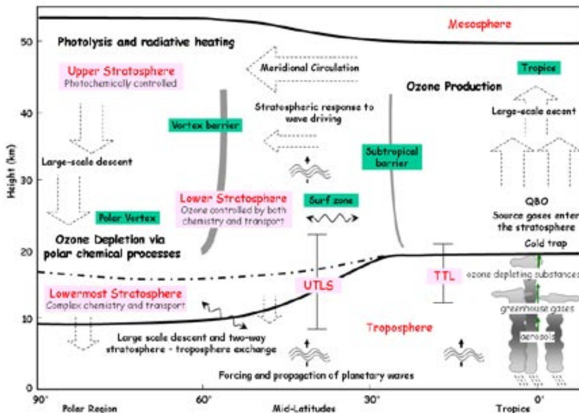
FIG. 1. Schematic diagram of the principal regions and processes in the winter hemispheric stratosphere. Broad arrows denote diabatic circulation and wavy arrows denote transport along isentropic surfaces. The average position of the tropopause is shown by the lower thick-black line, the average position of the stratopause by the upper thick-black line, and the 380-K isentropic surface by the thick-black dashed line. The vertical bars denote the range of the UTLS and TTL.
