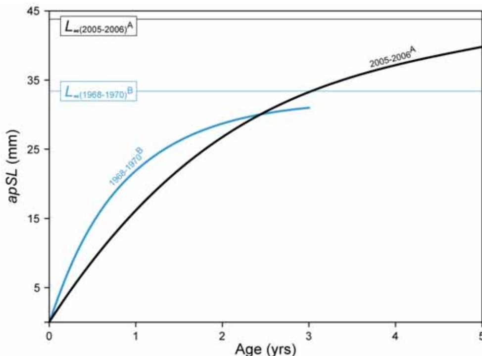
Fig. 23: VBGFs of D. hanleyanus with the parameters L_{\infty} = 44 mm and K = 0.47 yr -1 at Mar de las Pampas during 2005-2006 ( A : present study) in comparison with estimated growth parameters L_{\infty} = 33.5 mm and K = 1.18 yr -1 at Villa Gesell during 1968-1970 ( B : Penchaszadeh and Olivier 1975).
