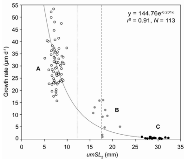
Fig. 4: D. hanleyanus . Relationship between umSL_2 (mm) and growth rate ( \mu\text{m d}^{-1} ) within the three groups, defined following Herrmann et al. (under review-e): O recruits (A: < 11 mm iapSL ), ● juveniles (B: 11-22 mm iapSL ) and ● adults (C: > 22 mm iapSL ). Dotted line indicate size at first maturity (13 mm) and dashed line indicate size of 50 % population maturity (17 mm) (Herrmann et al. under review-e).
