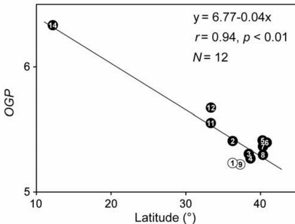
Fig. 7: OGP estimated from length-frequency data and obtained from ELEFAN by several populations of M. mactroides (1-12) and M. donacium (14) located at different latitudes. Comparing values (see Table 2) from this study (①) and from Olivier et al. (1971) (⑨).
