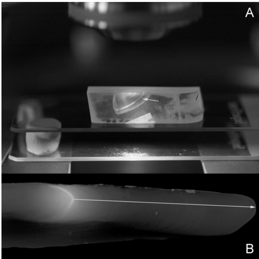
Fig. 3: D. hanleyanus ( umSL_2 = 7.31 mm) under a fluorescent microscope equipped with blue light, sampled and embedded in Epoxicure resin after 45 days experimental time ( A ). Thin section ( B ) along the major growth axis indicates a growth increment of 1.48 mm and the direction of growth ( arrow ).
