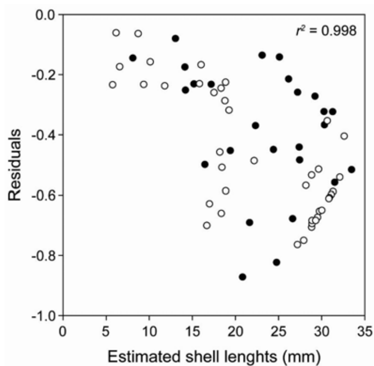
Fig. 5: D. hanleyanus . Residuals of estimated shell lengths of (●) SAD converted from LFD and of (O) SID from IFM, showing no significant difference (ANOVA, F_{1,64} = 2.153 , p > 0.05 ).
