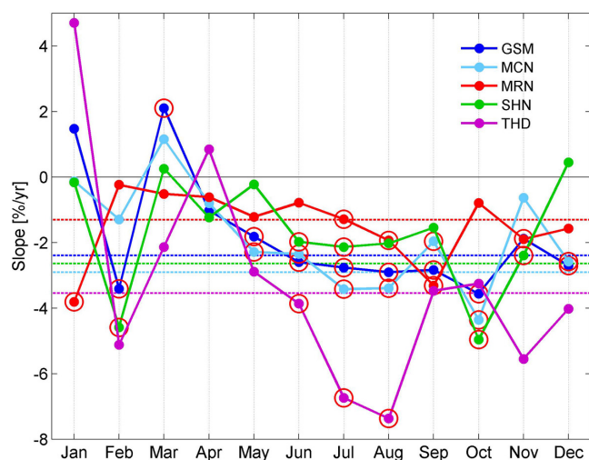
Fig. 5. Seasonal Mann-Kendall trend analysis (red circles correspond to 90% confidence levels) associated with Sen's slopes (colored dots) for the scattering coefficients of eastern and northwestern stations. The dotted lines correspond to the annual trend.
