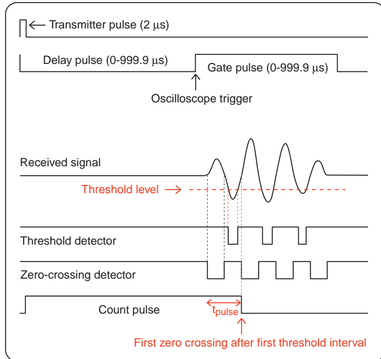
Figure 6—1 Schematic diagram of pulse timing and threshold peak detection (modified after GEOTEK manual).
