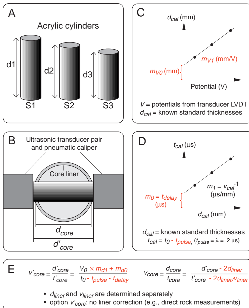
Figure 6—2 Schematic of PWL calibration. A. Physical standard used. B. Measurement geometry. C. and D. Calibration principle. E. Application of calibration to core measurement.
