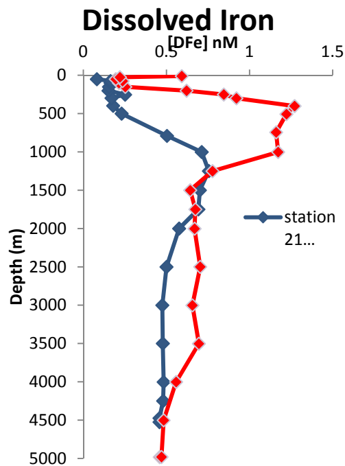
Figure 7: Profiles of dissolved iron versus depth.
