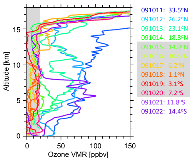
Fig. 1. Western Pacific tropospheric ozone mixing ratios from balloon sondes as a function of altitude. The legend shows date and latitude of each sounding. Gray shading indicates detection limit (left) and soundings with ozone abundances mostly below the detection limit (right).
