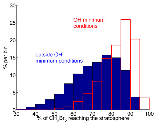
Fig. 9. Distribution of the fraction of boundary layer \text{CH}_2\text{Br}_2 surviving the transport through the troposphere for “outside minimum” conditions (filled blue) and “OH minimum” conditions (outlined red).
