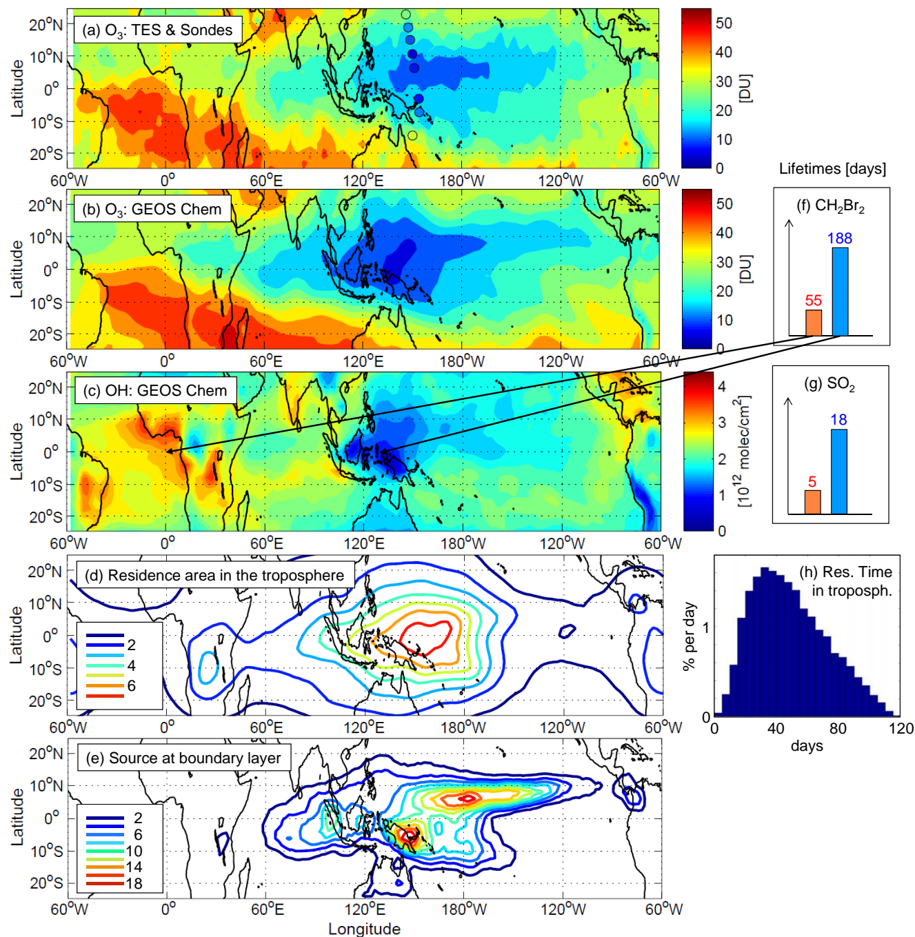
Fig. 4. Tropospheric ozone columns from (a) TES for October 2009 (results for 2005–2009 are similar, see Fig. 5), the sondes (open circles, dates see Fig. 1), and (b) GEOS Chem (mean 1–15 October 2009). (c) OH columns from GEOS-Chem (mean 1–15 October 2009). (d, e, h) show ATLAS 4-months backtrajectory runs for air entering the stratosphere (1 October–31 January). Average conditions for 2002–2011, individual results for 2009 in Figs. 7 and 8. (d) Density distribution function of the horizontal positions of the trajectories between the boundary layer and the LCPs. (e) Density distribution function of the horizontal positions of the last contact with the boundary layer. The values in (d) and (e) are normalized such that a horizontally uniform distribution corresponds to a value of 1 at every grid point. (f–g) Examples of gas-phase lifetimes of relevant species in the mid-troposphere (500 hPa) at the equator for typical conditions over the Atlantic ( 0^\circ E, orange) and for conditions in the OH minimum ( 130^\circ E, blue). (h) Distribution of residence times between last contact with the boundary layer and the LCP for trajectories ascending into the stratosphere.
