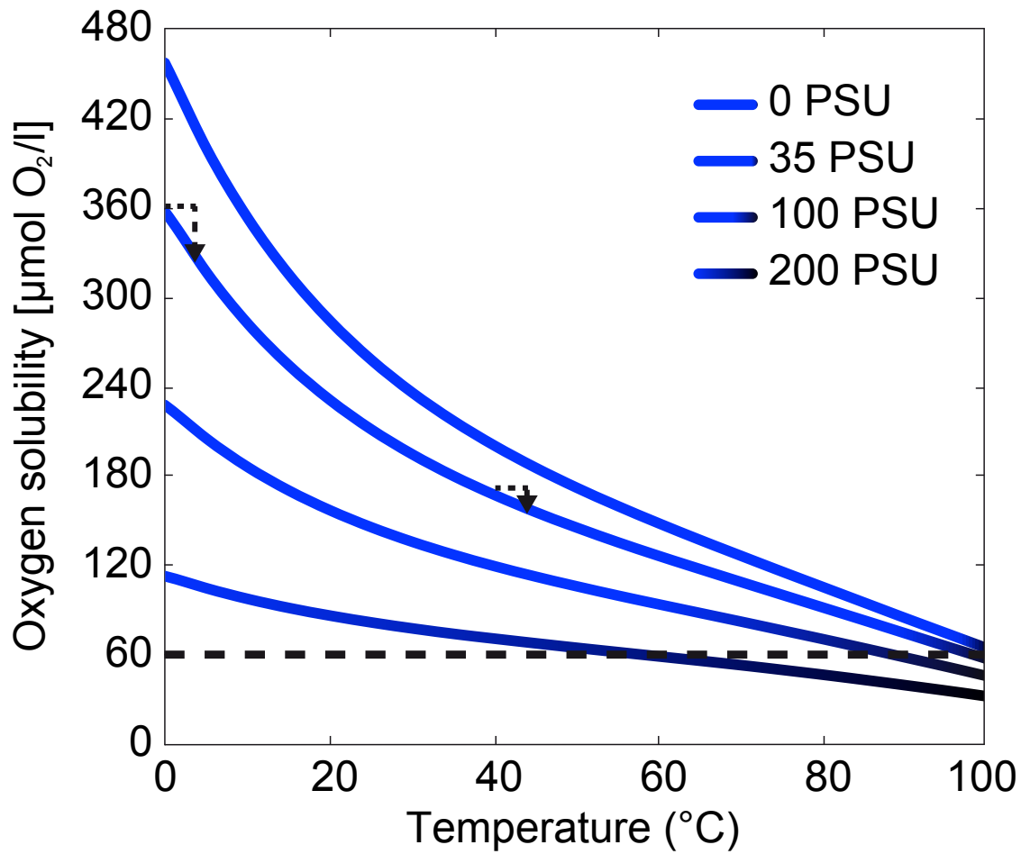
fig. S1 Oxygen solubility in air-saturated water of different salinities. The black dotted line indicates the transition to hypoxia adapted communities found below oxygen concentrations of \approx 60 \mu\text{mol O}_2/\text{l} or < 2\text{mg O}_2/\text{l} . Black dotted arrows exemplify the decrease in oxygen solubility in 0^\circ\text{C} and 40^\circ\text{C} seawater (35 PSU) upon warming according to the RCP scenario 8.5 predicted for 2100.
