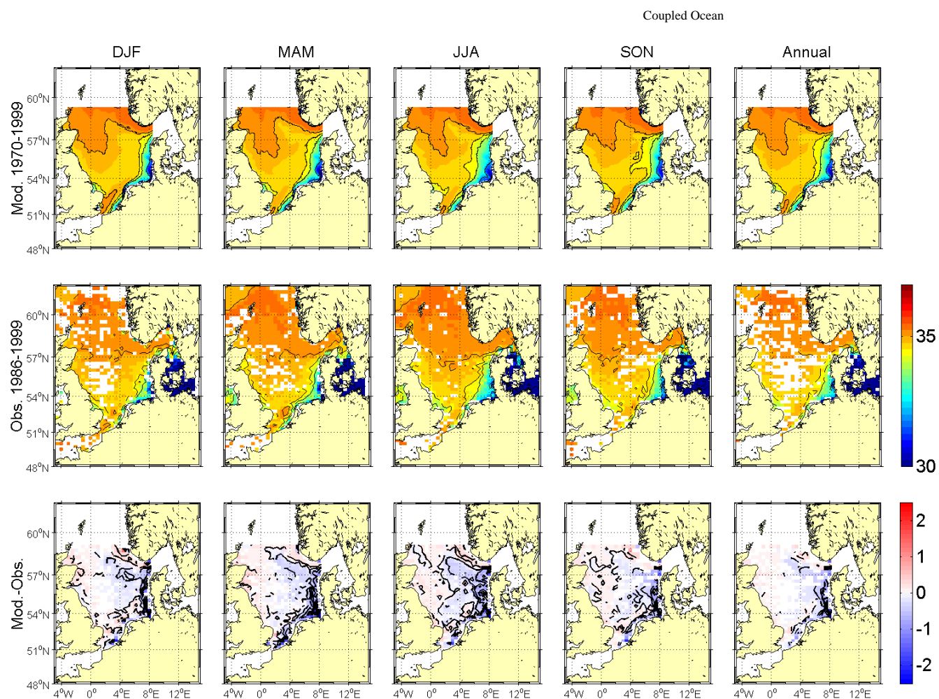
Figure 5.3.18A: Comparison of seasonal and annual means of bottom salinity [psu] for NEMO-Nordic run 470 for the base period 1970-1999 with KNSC means. The upper row shows average model results, the middle row observed climatological means and the lower row the difference between the model results and the climatology.
