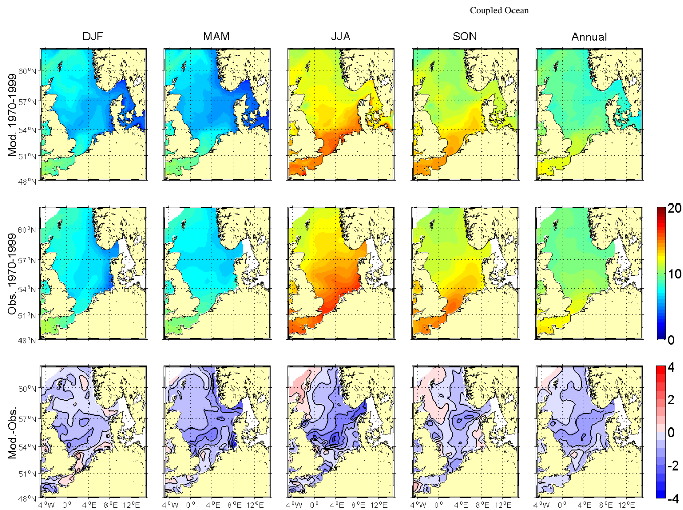
Figure 5.1.2A: Comparison of seasonal and annual means of sea surface temperature [°C] for MPIOM run 215 for the base period 1970-1999 with climatological means from the BHC. The upper row shows average model distributions, the middle row observed climatological means and the lower row difference between the model results and the climatology.
