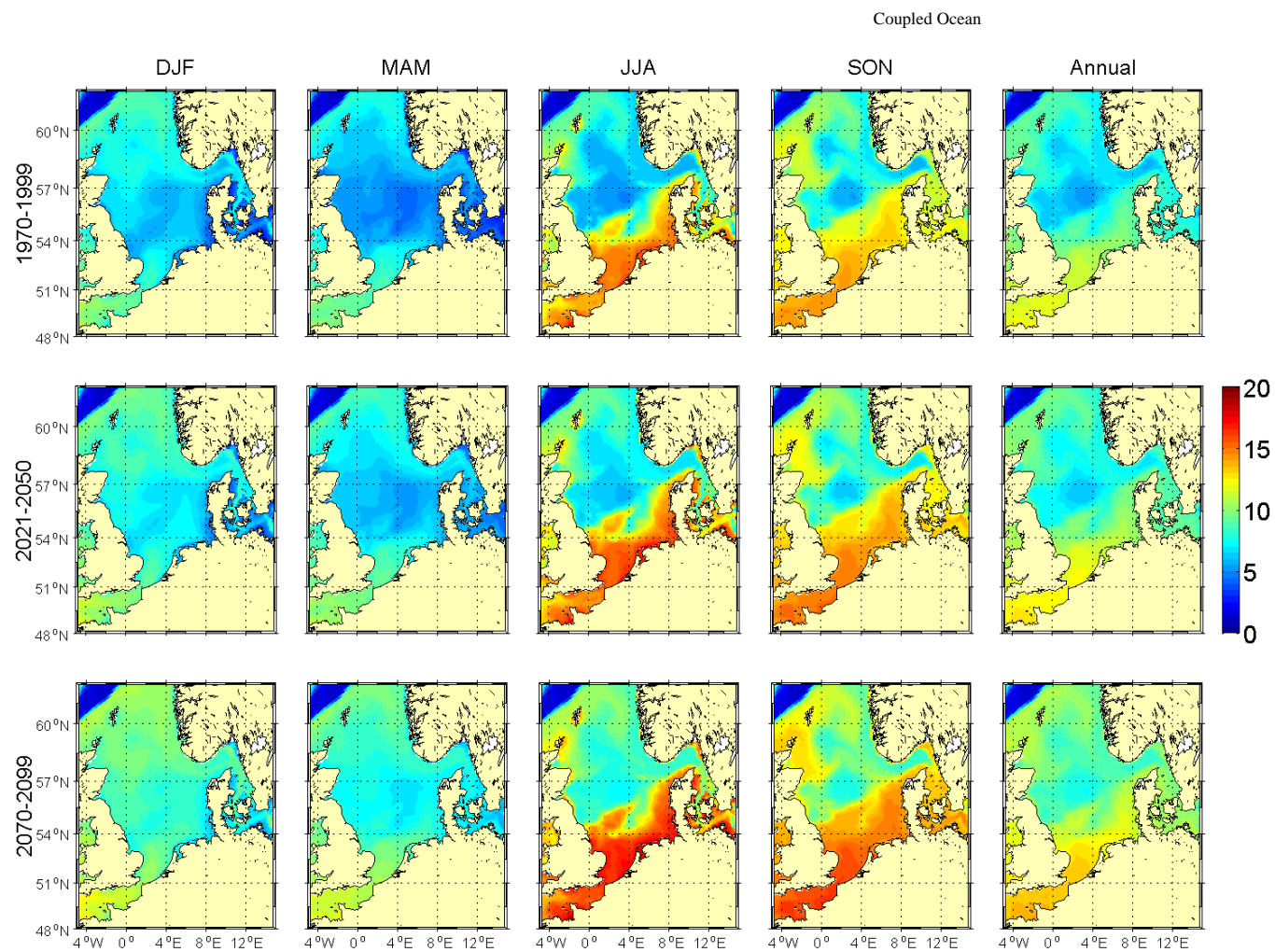
Figure 5.1.4A: Seasonal and annual means of bottom temperature [°C] for MPIOM run 215 (A1B scenario run). The upper row shows averages for the period 1970-1999, the middle row for 2021-2050 and the lower row for 2070-2099.
