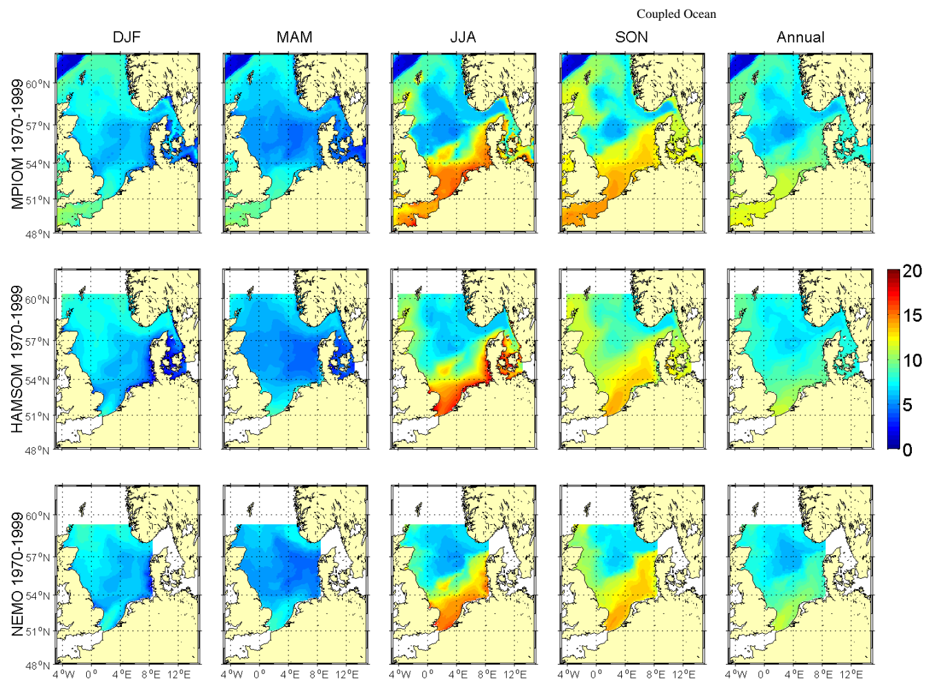
Figure 5.4.4A: Seasonal and annual means of bottom temperature [°C] for the period 1970-1999. Upper row MPIOM run 215, middle row HAMSOM run 202 and lower row NEMO-Nordic run 470 (all A1B scenario).
