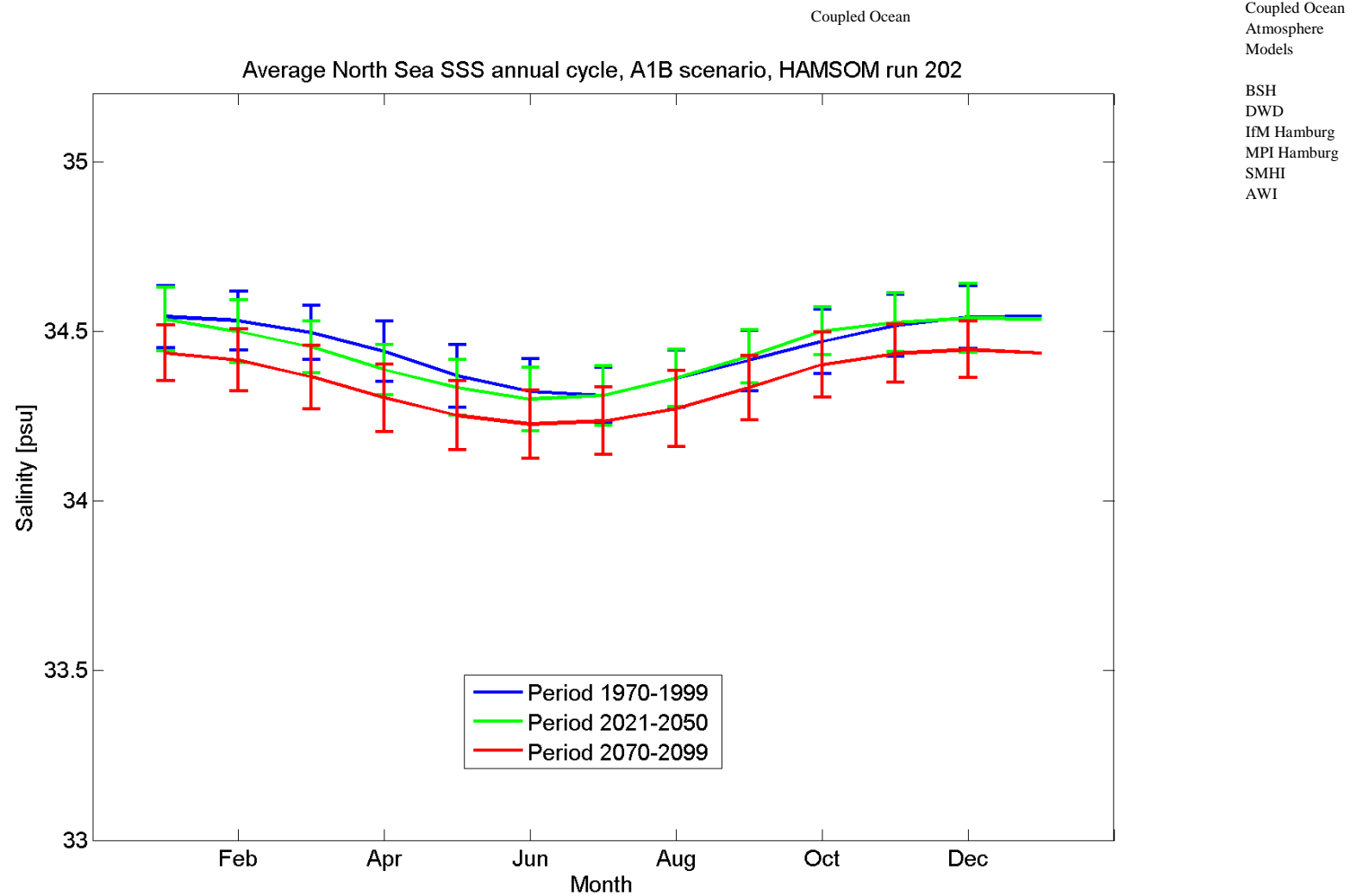
Figure 5.2.22A: The mean annual cycle of sea surface salinity [psu] for HAMSOM run 202 (A1B scenario run) for 1970-1999 (blue), 2021-2050 (green) and 2070-2099 (red). The means are representing averages over the North Sea area given in Figure 4.1. The error bars are indicating time variability.
