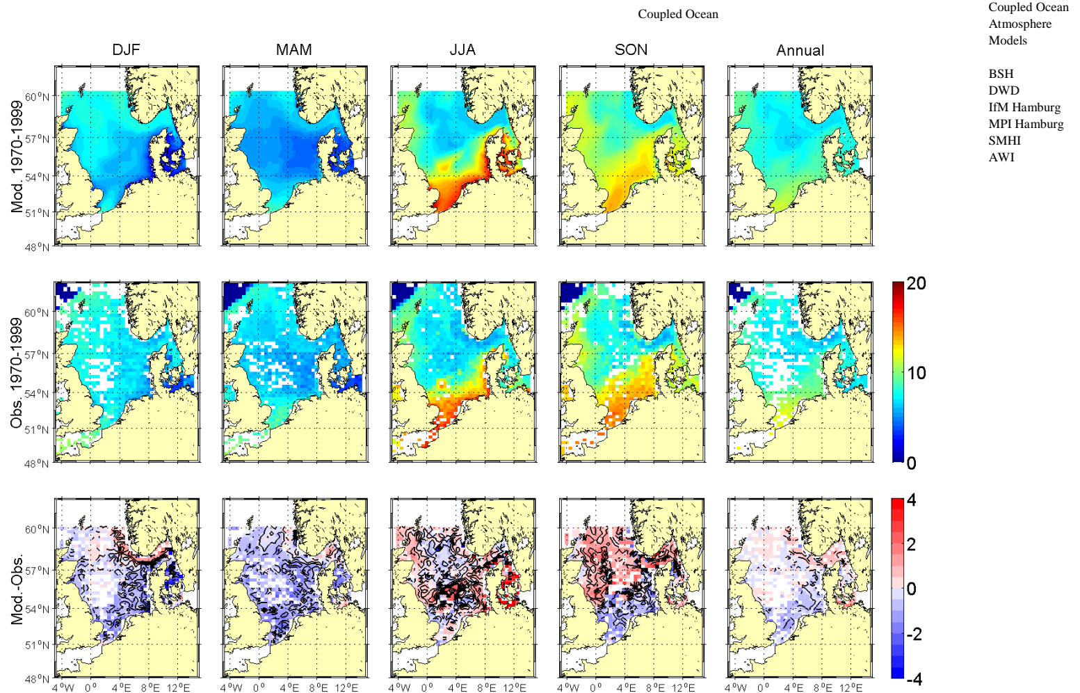
Figure 5.2.6A: Comparison of seasonal and annual means of bottom temperature [°C] for HAMSOM run 202 for the base period 1970-1999 with KNSC means. The upper row shows average model distributions, the middle row observed climatological means and the lower row the difference between the model results and the climatology.
