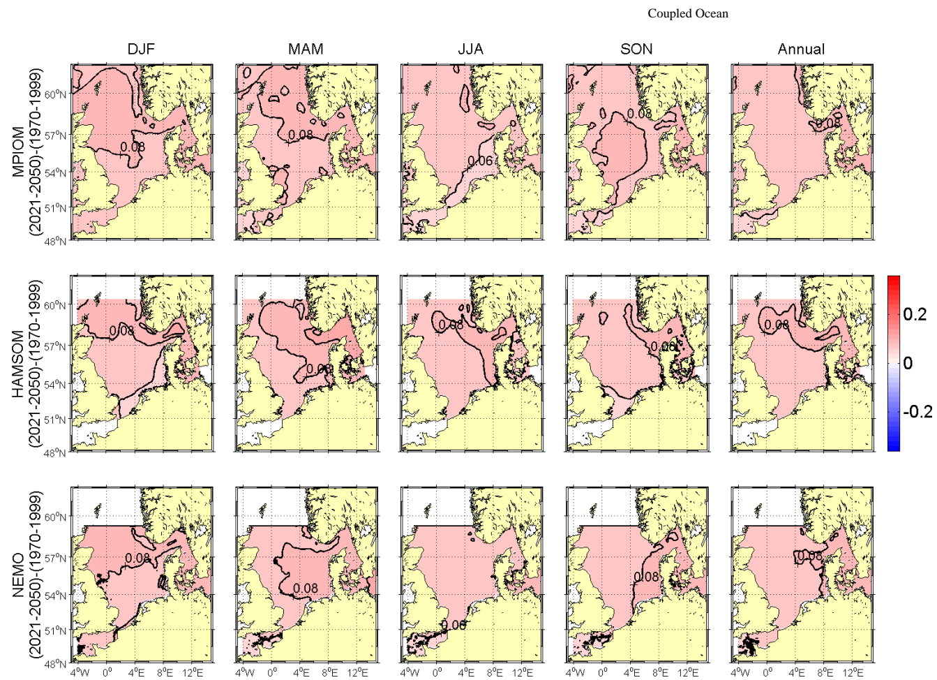
Figure 5.4.32A: Changes in seasonal and annual means of sea surface height [m] from (1970-1999) to (2021-2050). Upper row MPIOM run 215, middle row HAMSOM run 202 and lower row NEMO-Nordic run 470 (all A1B scenario). Selected isolines have been labelled for better orientation, contour interval is 0.02 m.
