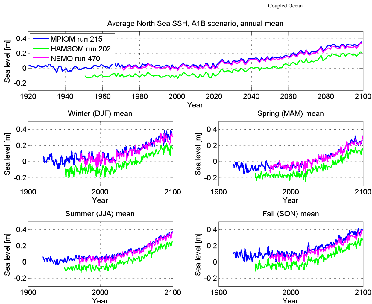
Figure 5.4.34A: Time series of seasonal and annual means of sea surface height [m] for MPIOM run 215 (blue), HAMSOM run 202 (green) and NEMO-Nordic run 470 (magenta). The sea surface heights represent averages over the North Sea area given in Figure 4.1. Upper row annual means, lower rows seasonal means.
