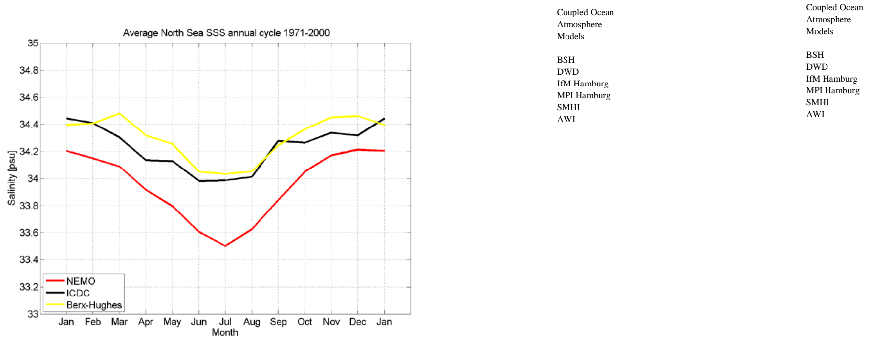
Figure 4.2.3A: The mean annual cycle of sea surface salinity [psu] for NEMO-Nordic run 477 (red), KNSC (black), BHC (yellow) over the time period 1971 till 2000. The means are representing averages over the North Sea area.
