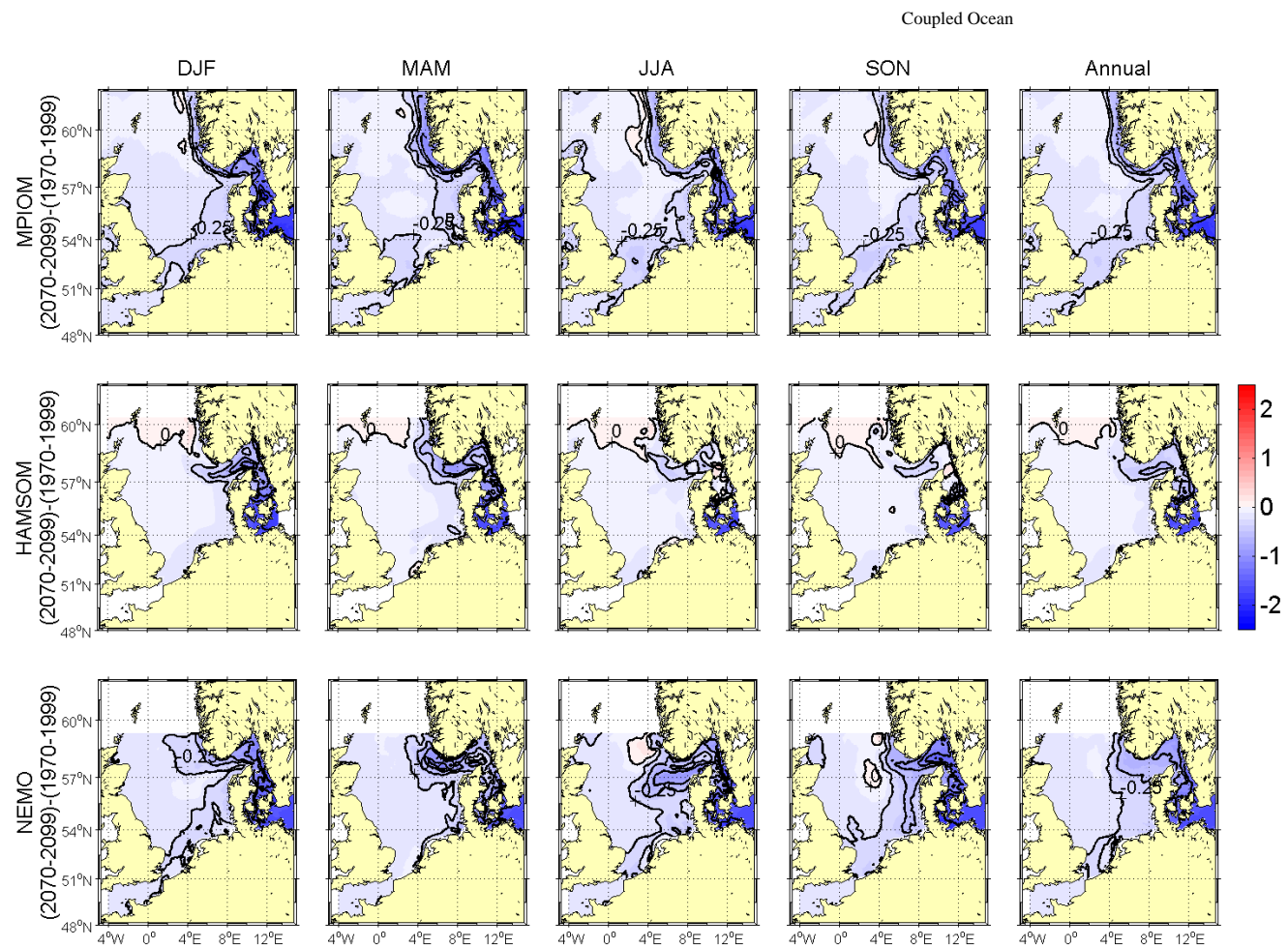
Figure 5.4.22A: Changes in seasonal and annual means of sea surface salinity [psu] from (1970-1999) to (2070-2099). Upper row MPIOM run 215, middle row HAMSOM run 202 and lower row NEMO-Nordic run 470 (all A1B scenario). Selected isolines have been labelled for better orientation, contour interval is 0.25 psu.
