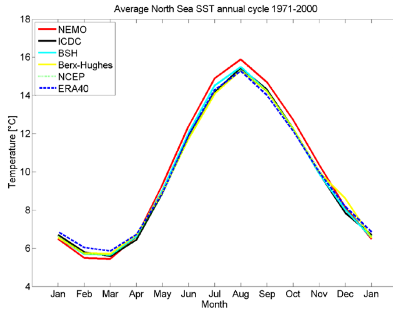
Figure 4.1.3A: The mean annual cycle of sea surface temperatures [°C] for NEMO-Nordic run 477 (red), KNCS (ICDC, black), BSH observations (cyan), BHC (yellow), NCEP (green) and ERA40 (blue) over the time period 1971 till 2000. The means are representing averages over the North Sea area.
