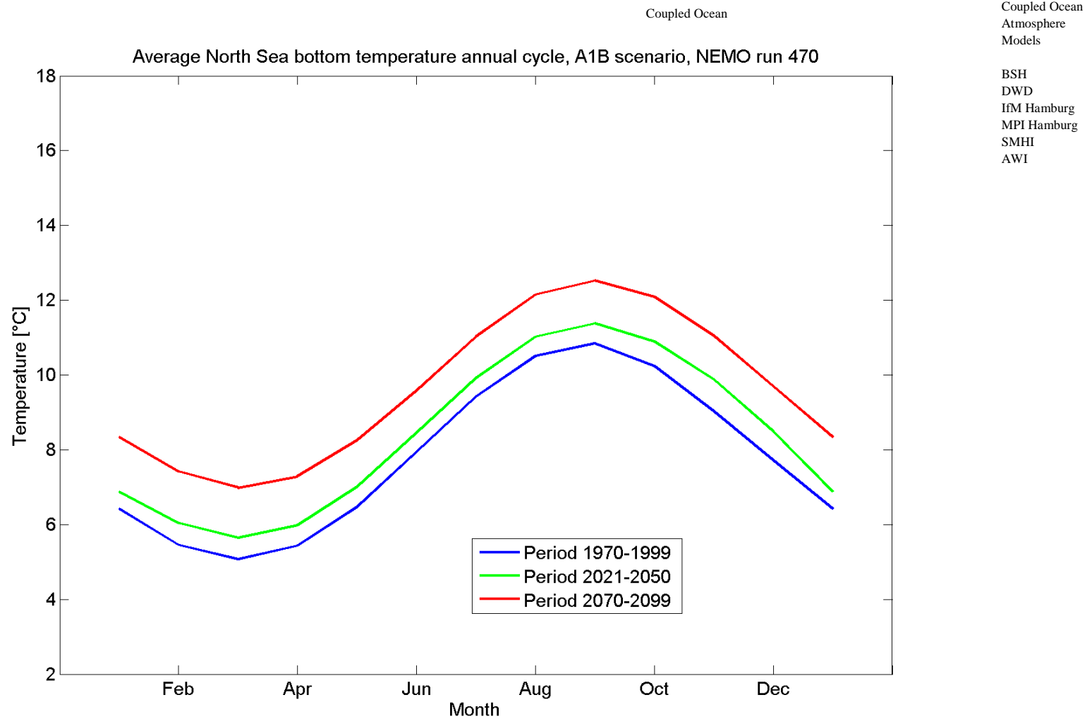
Figure 5.3.12A: The mean annual cycle of bottom temperatures [°C] for NEMO-Nordic run 470 (A1B scenario run) for 1970-1999 (blue), 2021-2050 (green) and 2070-2099 (red). The means are representing averages over the North Sea area given in Figure 4.1.
