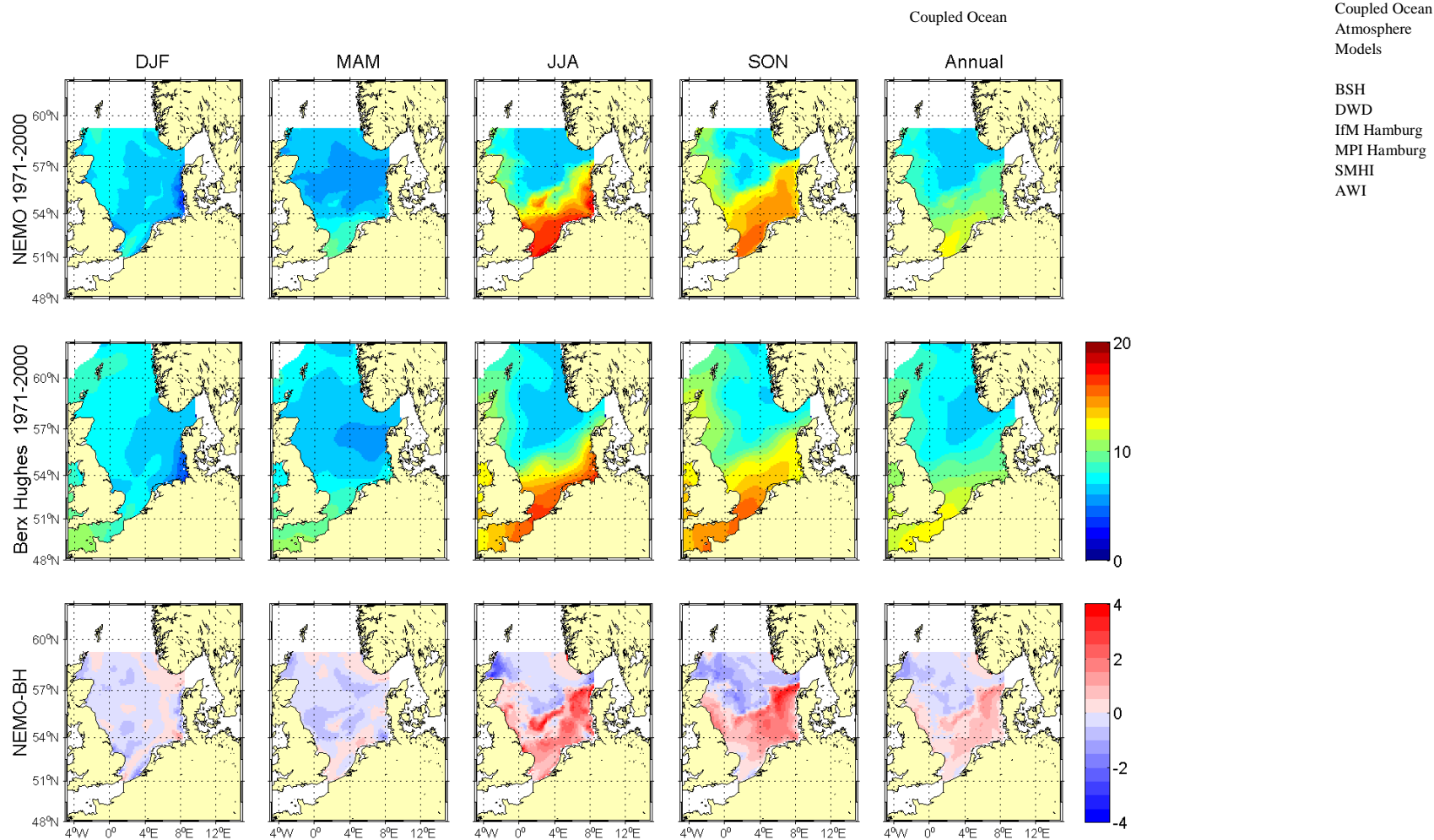
Figure 4.3.27A: Seasonal and annual means of bottom temperature [°C] averaged over the period 1971-2000: The mean bottom temperature results from NEMO-Nordic (run 477) are presented in the upper row, in the middle the bottom temperature from the BHC and in the lower row the difference between the model results and the climatology.
