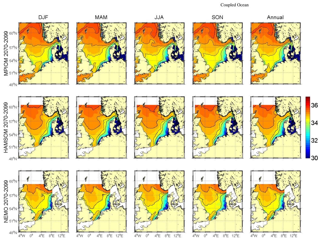
Figure 5.4.20A: Seasonal and annual means of bottom salinity [psu] for the period 2070-2099. Upper row MPIOM run 215, middle row HAMSOM run 202 and lower row NEMO-Nordic run 470 (all A1B scenario).
