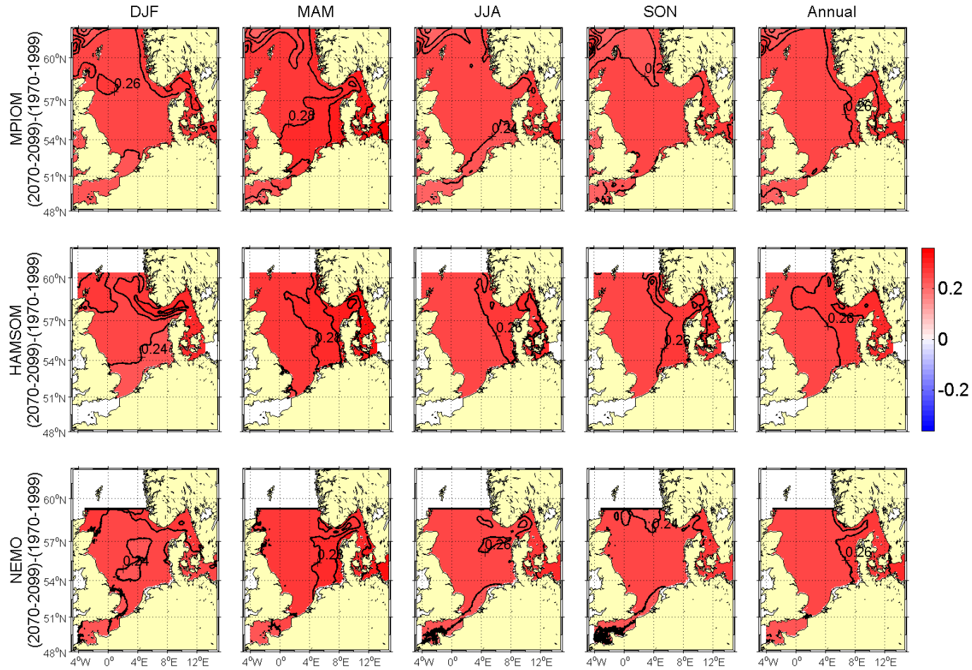
Figure 5.4.33A: Changes in seasonal and annual means of sea surface height [m] from (1970-1999) to (2070-2099). Upper row MPIOM run 215, middle row HAMSO run 202 and lower row NEMO-Nordic run 470 (all A1B scenario). Selected isolines have been labelled for better orientation, contour interval is 0.02 m.
