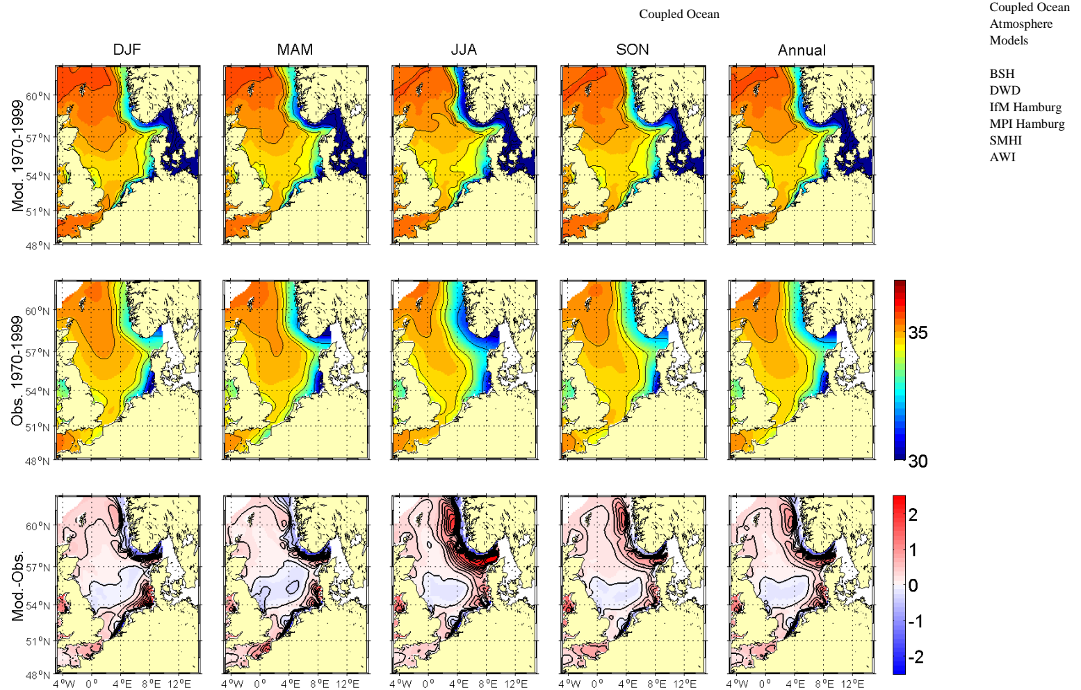
Figure 5.1.14A: Comparison of seasonal and annual means of sea surface salinity [psu] for MPIOM run 215 for the base period 1970-1999 with climatological means from the BHC. The upper row shows average model distributions, the middle row observed climatological means and the lower row the difference between the model results and the climatology.
