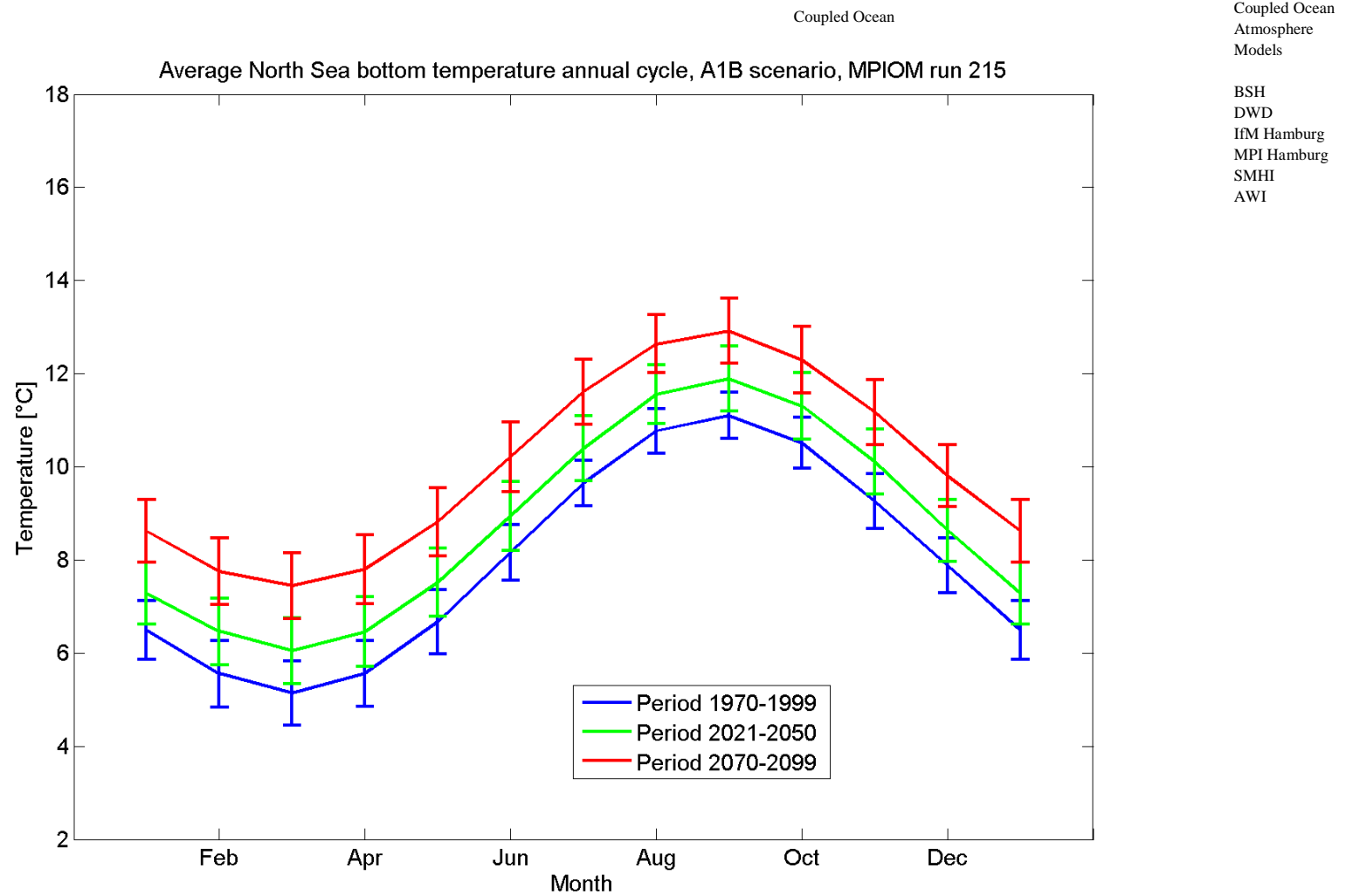
Figure 5.1.12A: The mean annual cycle of bottom temperatures [°C] for MPIOM run 215 (A1B scenario) 1970-1999 (blue), 2021-2050 (green) and 2070-2099 (red). The means are representing averages over the North Sea area given in Figure 4.1. The error bars are indicating time variability.
