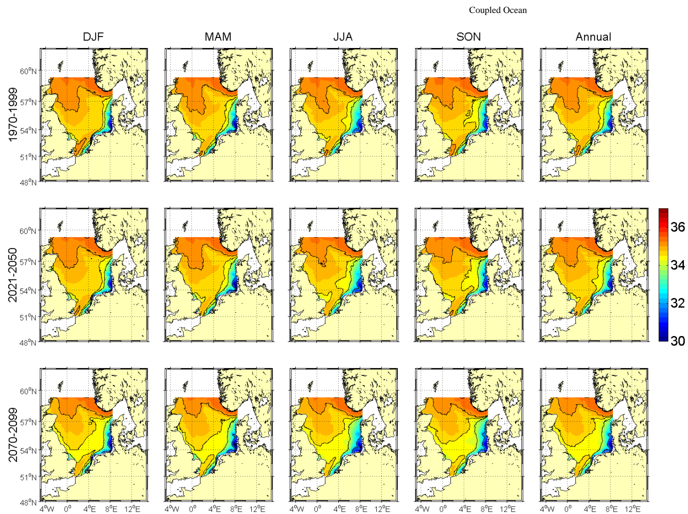
Figure 5.3.16A: Seasonal and annual means of bottom salinity [psu] for NEMO-Nordic run 470 (A1B scenario run). The upper row shows averages for the period 1970-1999, the middle row for 2021-2050 and the lower row for 2070-2099.
