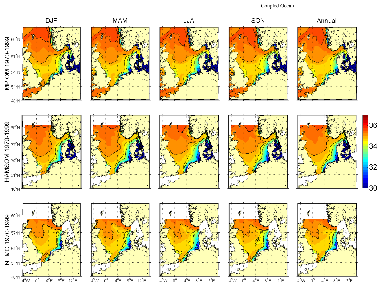
Figure 5.4.18A: Seasonal and annual means of bottom salinity [psu] for the period 1970-1999. Upper row MPIOM run 215, middle row HAMSOM run 202 and lower row NEMO-Nordic run 470 (all A1B scenario).
