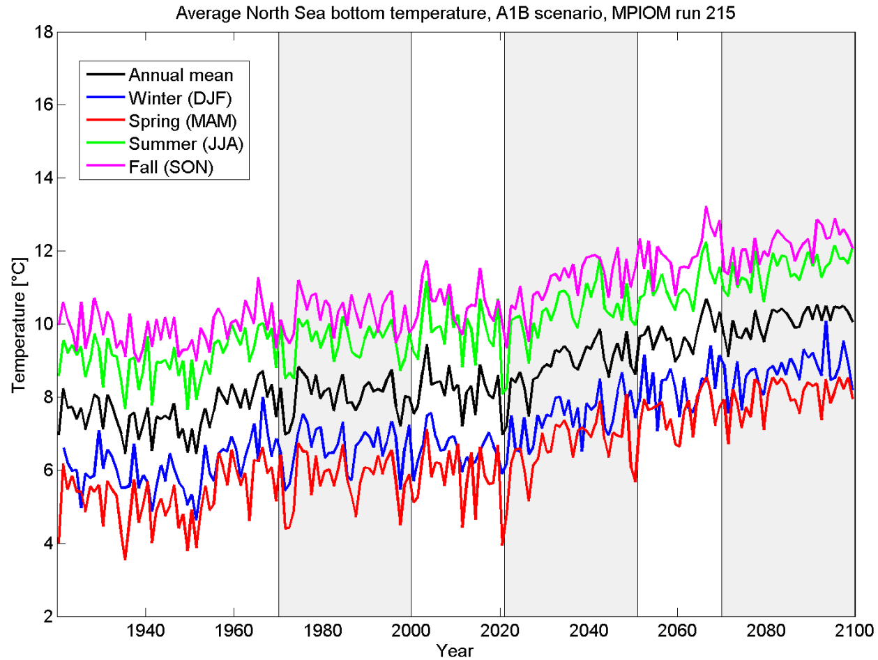
Figure 5.1.11A: Time series of seasonal and annual means of bottom temperature [°C] for MPIOM run 215 (A1B scenario run) from 1920-2099. The temperatures represent averages over the North Sea area given in Figure 4.1.
