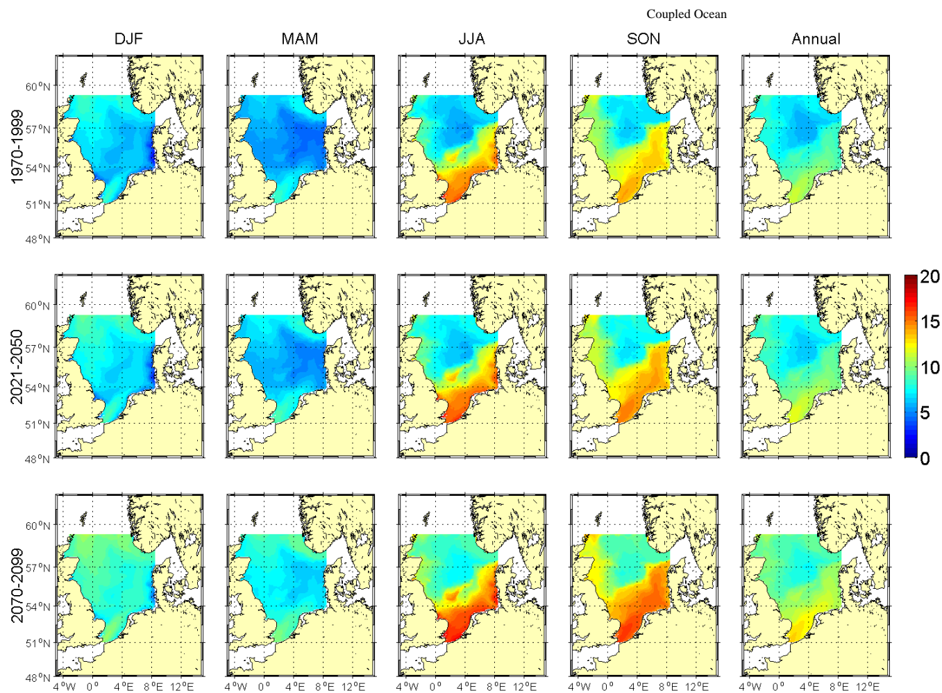
Figure 5.3.4A: Seasonal and annual means of bottom temperature [°C] for NEMO-Nordic run 470 (A1B scenario run). The upper row shows averages for the period 1970-1999, the middle row for 2021-2050 and the lower row for 2070-2099.
