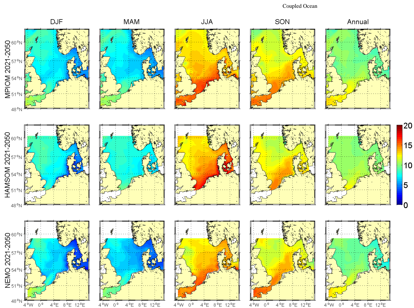
Figure 5.4.2A: Seasonal and annual means of sea surface temperature [°C] for the period 2021-2050. Upper row MPIOM run 215, middle row HAMSOM run 202 and lower row NEMO-Nordic run 470 (all A1B scenario).
