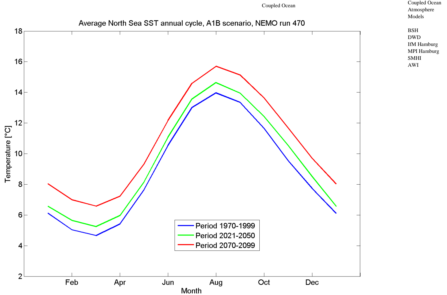
Figure 5.3.10A: The mean annual cycle of sea surface temperatures [°C] for NEMO-Nordic run 470 (A1B scenario run) for 1970-1999 (blue), 2021-2050 (green) and 2070-2099 (red). The means are representing averages over the North Sea area given in Figure 4.1.
