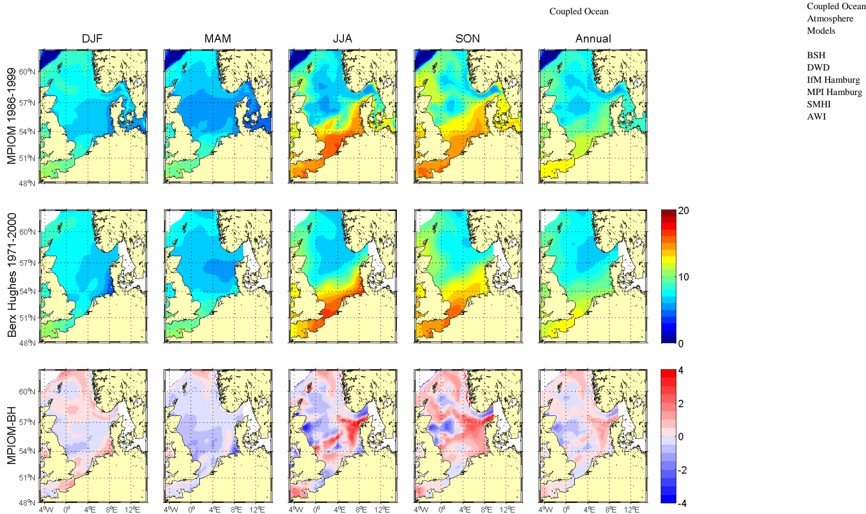
Figure 4.3.25A: Seasonal and annual means of bottom temperature [°C]: The mean bottom temperature results from MPIOM (run 253) averaged over the period 1986-1999 are presented in the upper row, in the middle the mean bottom temperature from the BHC averaged over the period 1971-2000 and in the lower row difference between the model results and the climatology.
