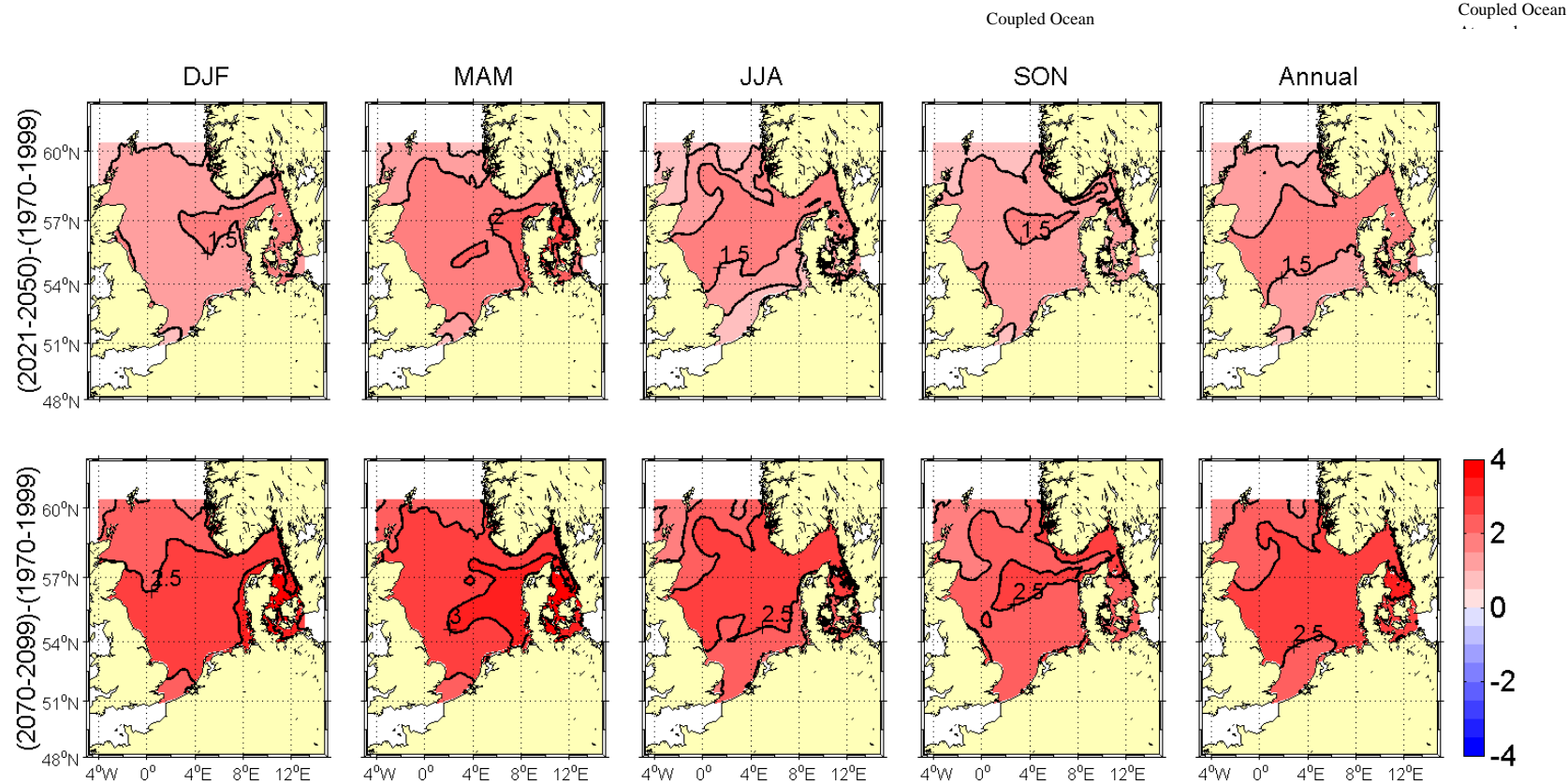
Figure 5.2.8A: Changes in seasonal and annual bottom temperature [°C] for HAMSOM run 202 (A1B scenario run). Upper panel from (1970-1999) to (2021-2050) and lower panel from (1970-1999) to (2070-2099). The contour interval is 0.5 °C. Selected isolines have been labelled for better orientation.
