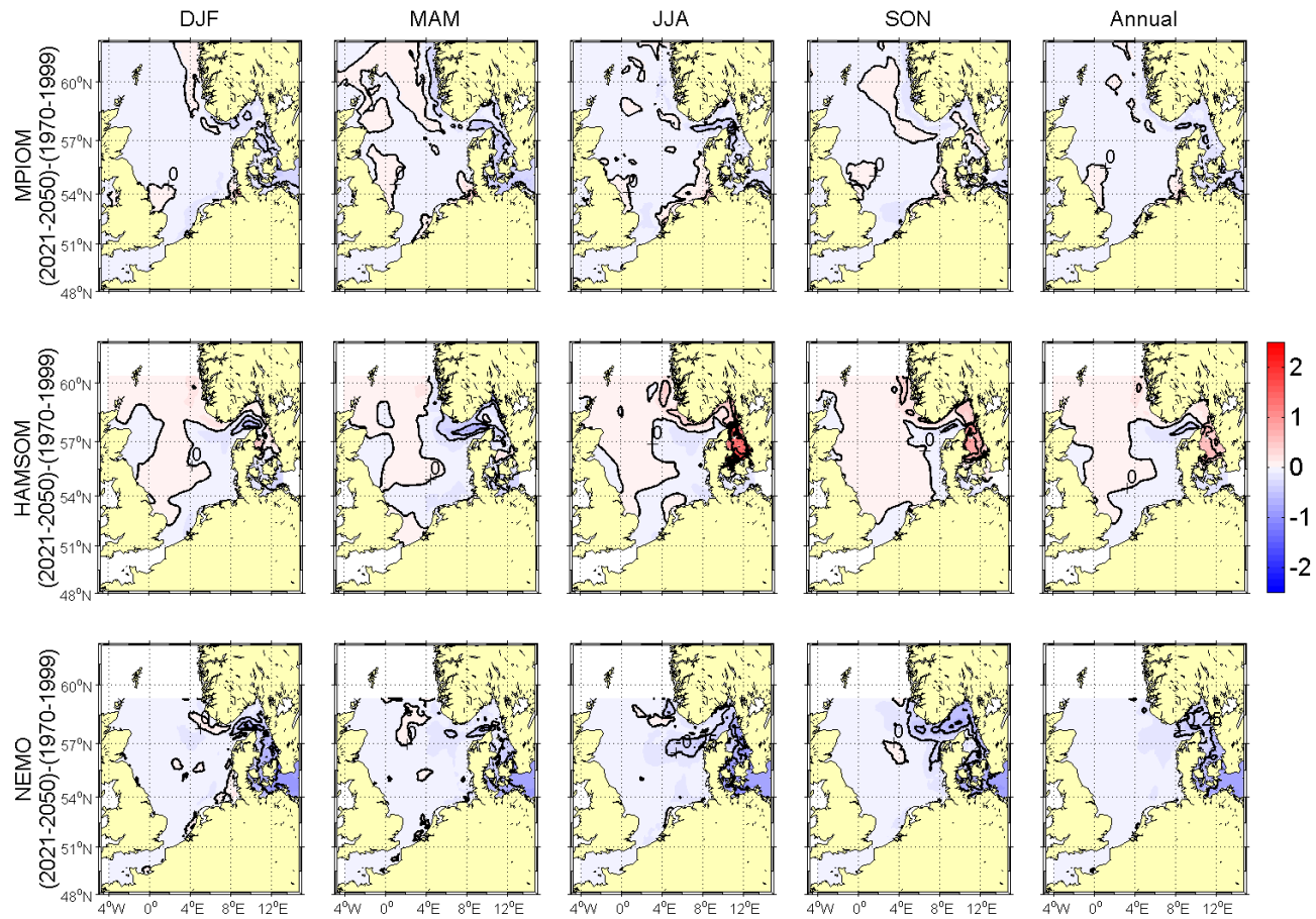
Figure 5.4.21A: Changes in seasonal and annual means of sea surface salinity [psu] from (1970-1999) to (2021-2050). Upper row MPIOM run 215, middle row HAMSOM run 202 and lower row NEMO-Nordic run 470 (all A1B scenario). Selected isolines have been labelled for better orientation, contour interval is 0.25 psu.
