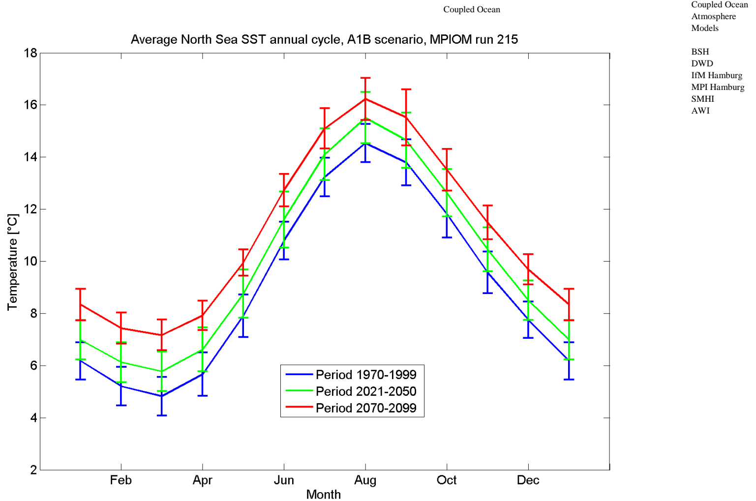
Figure 5.1.10A: The mean annual cycle of sea surface temperatures [°C] for MPIOM run 215 (A1B scenario run) for 1970-1999 (blue), 2021-2050 (green) and 2070-2099 (red). The means are representing averages over the North Sea area given in Figure 4.1. The error bars are indicating time variability.
