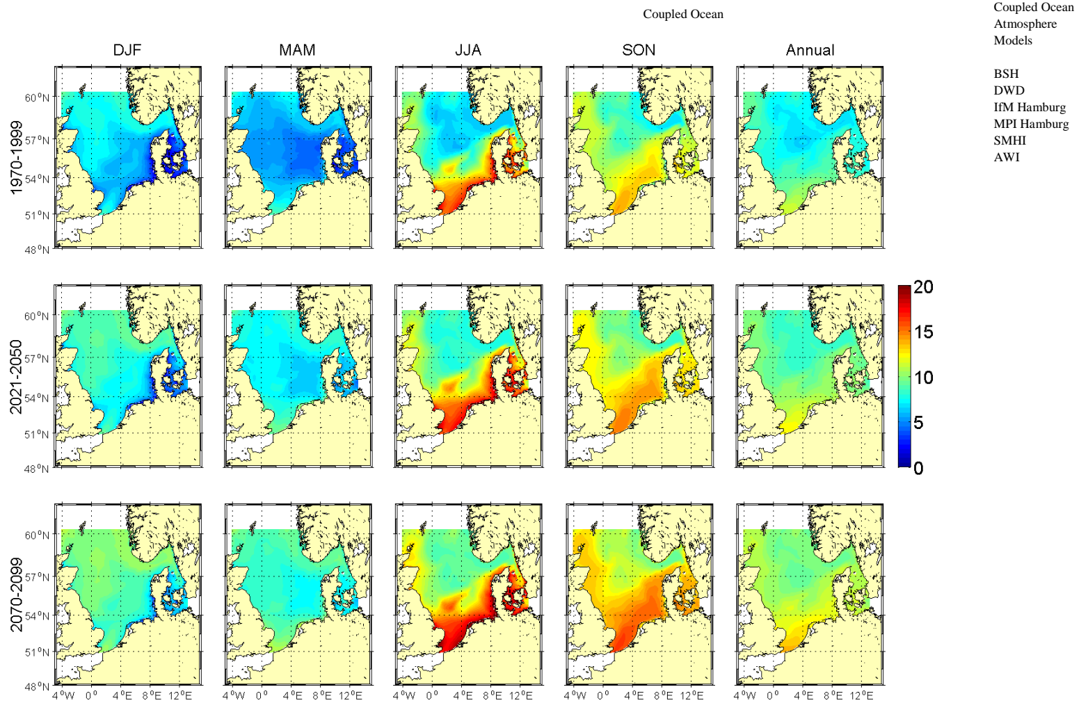
Figure 5.2.4A: Seasonal and annual means of bottom temperature [°C] for HAMSOM run 202 (A1B scenario run). The upper row shows averages for the period 1970-1999, the middle row for 2021-2050 and the lower row for 2070-2099.
