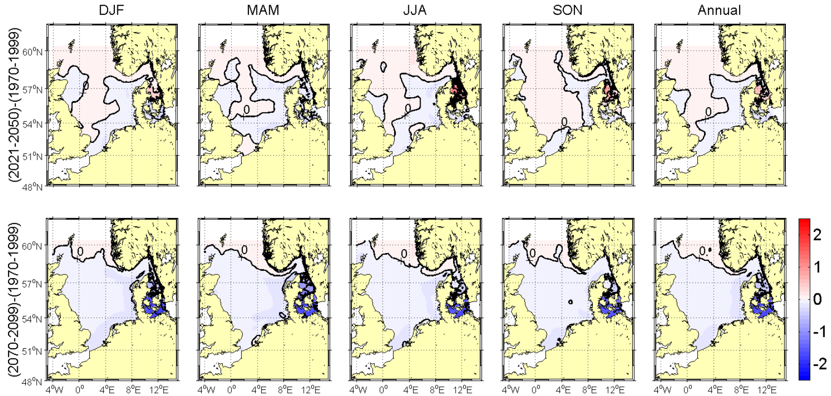
Figure 5.2.20A: Changes in seasonal and annual bottom salinity [psu] for HAMSOM run 202 (A1B scenario run). Upper panel from (1970-1999) to (2021-2050) and lower panel from (1970-1999) to (2070-2099). The contour interval is 0.5 °C. Selected isolines have been labelled for better orientation.
