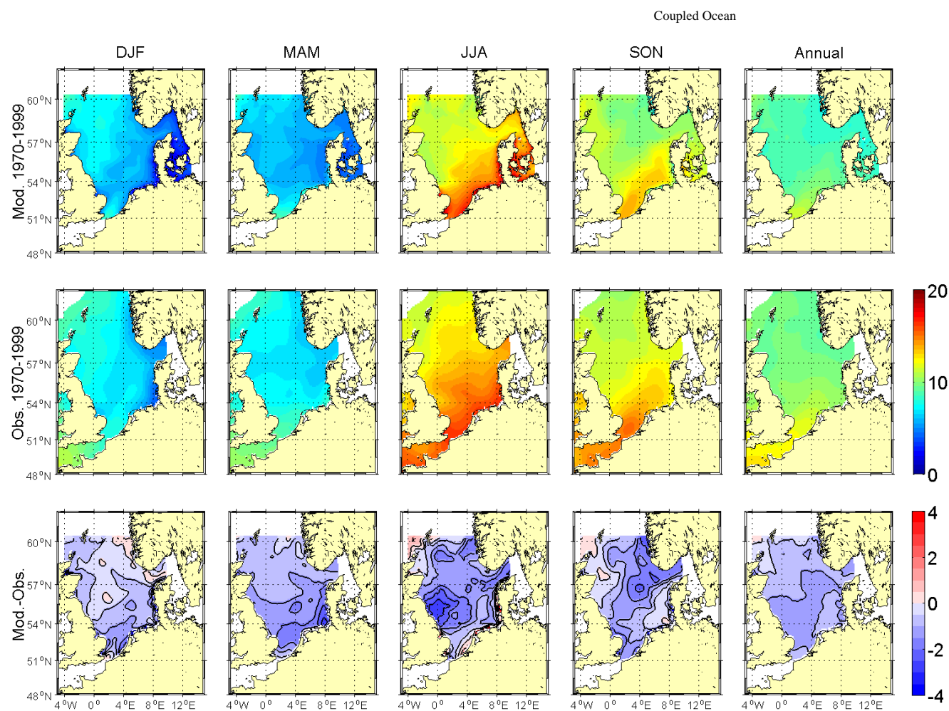
Figure 5.2.2A: Comparison of seasonal and annual means of sea surface temperature [°C] for HAMSOM run 202 for the base period 1970-1999 with BHC means. The upper row shows average model distributions, the middle row observed climatological means and the lower row the difference between the model results and the climatology.
