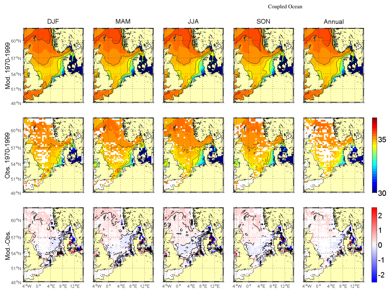
Figure 5.1.18A: Comparison of seasonal and annual means of bottom salinity [psu] for MPIOM run 215 for the base period 1970-1999 with KNSC means. The upper row shows average model distributions, the middle row observed climatological means and the lower row the difference between the model results and the climatology.
