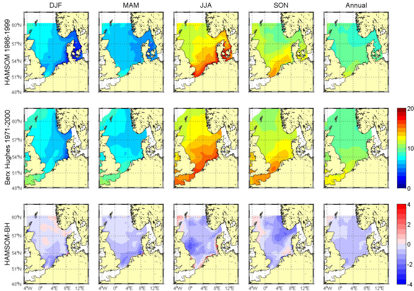
Figure 4.3.12A: Seasonal and annual means of sea surface temperature [°C]: The mean sea surface temperatures from HAM SOM (run 201) averaged over the period 1986-1999 are presented in the upper row, in the middle the mean surface temperatures from the BHC averaged over the period 1971-2000 and in the lower row the difference between the model results and the climatology.
