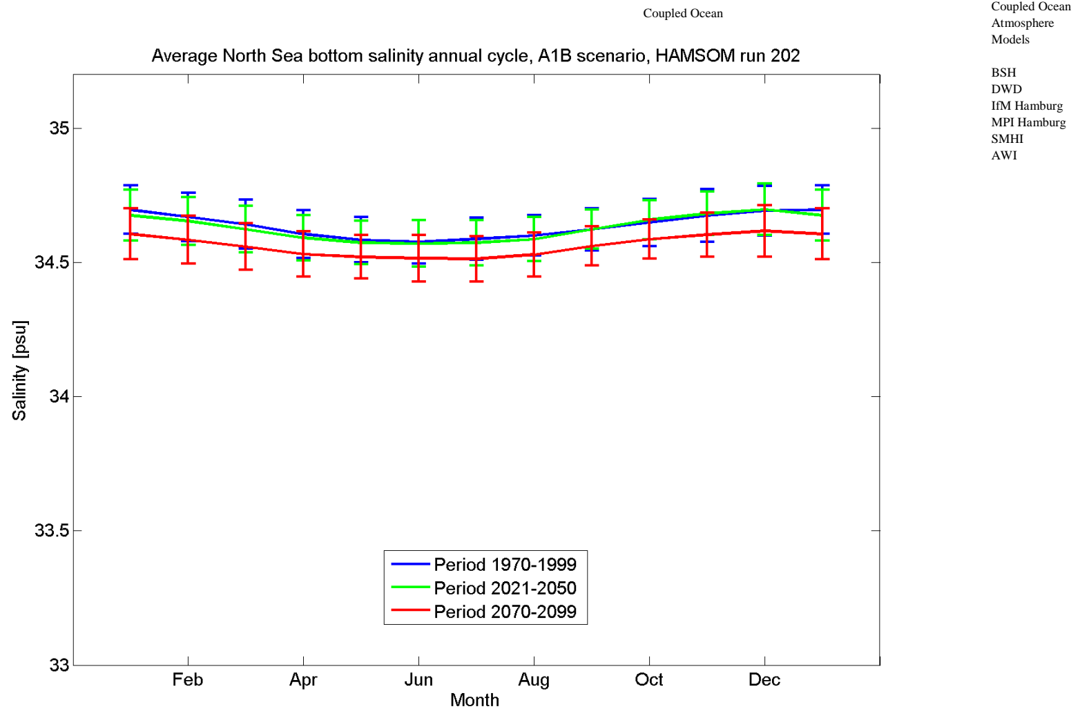
Figure 5.2.24A: The mean annual cycle of bottom salinity [psu] for HAMSOM run 202 (A1B scenario run) for 1970-1999 (blue), 2021-2050 (green) and 2070-2099 (red). The means are representing averages over the North Sea area given in Figure 4.1. The error bars are indicating time variability.
