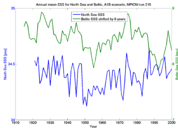
Figure 5.1.5: Comparison of sea surface salinity time series from the North Sea (blue) and Baltic (green). The record from the Baltic is leading by 6 years and has been shifted accordingly in the figure.
