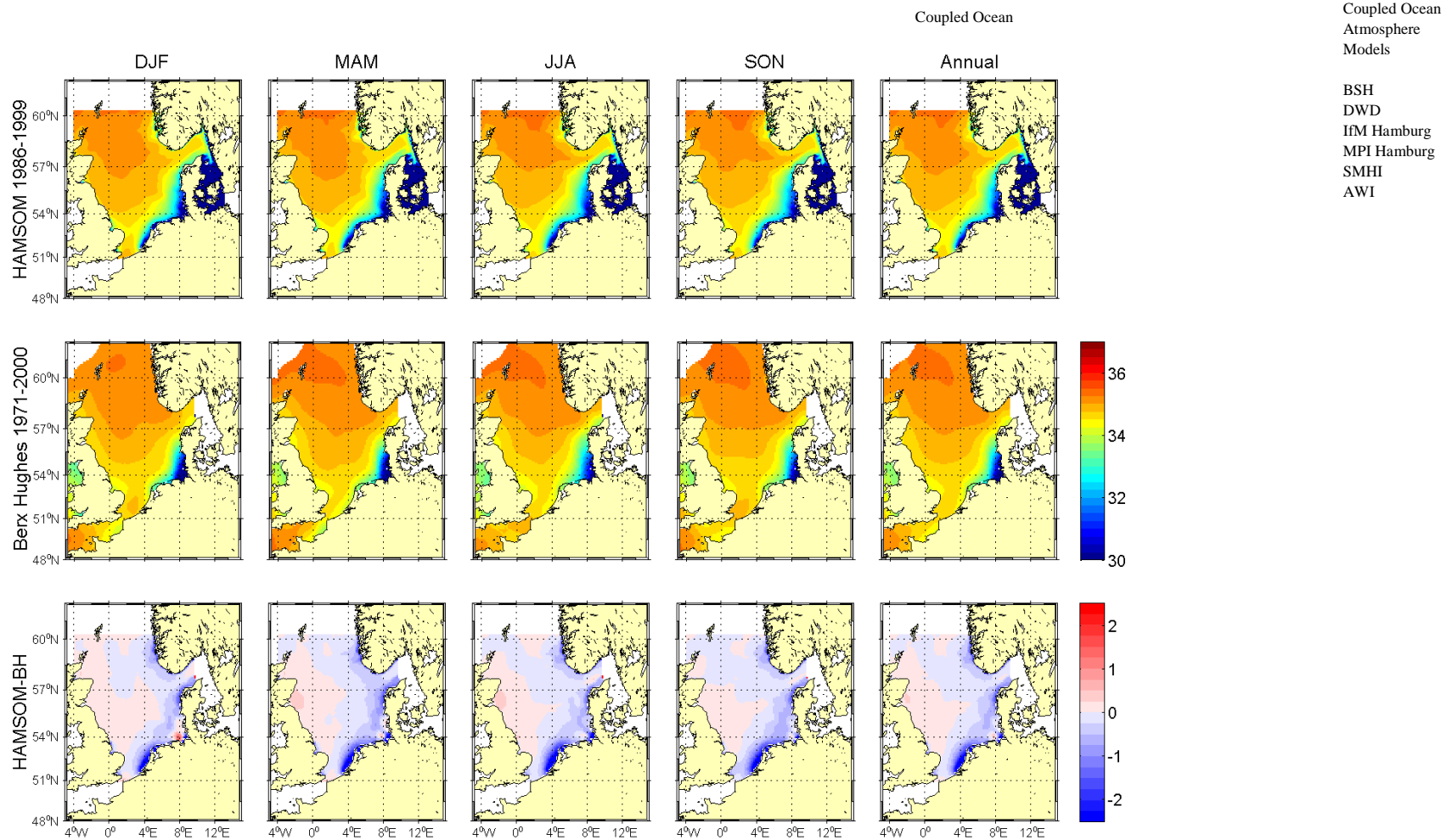
Figure 4.3.29A: Seasonal and annual means of bottom salinity [psu]: The mean bottom salinity results from HAM SOM (run 201) averaged over the period 1986-1999 are presented in the upper row, in the middle row the mean bottom salinity from the BHC averaged over the period 1971-2000 and in the lower row the difference between the model results and the climatology.
