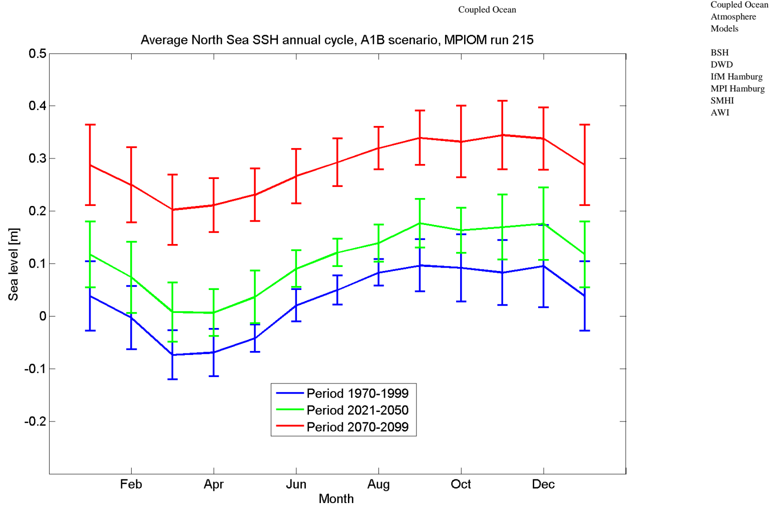
Figure 5.1.28A: The mean annual cycle of sea surface height [m] for MPIOM run 215 (A1B scenario run) 1970-1999 (blue), 2021-2050 (green) and 2070-2099 (red). The means are representing averages over the North Sea area given in Figure 4.1. The error bars are indicating time variability.
