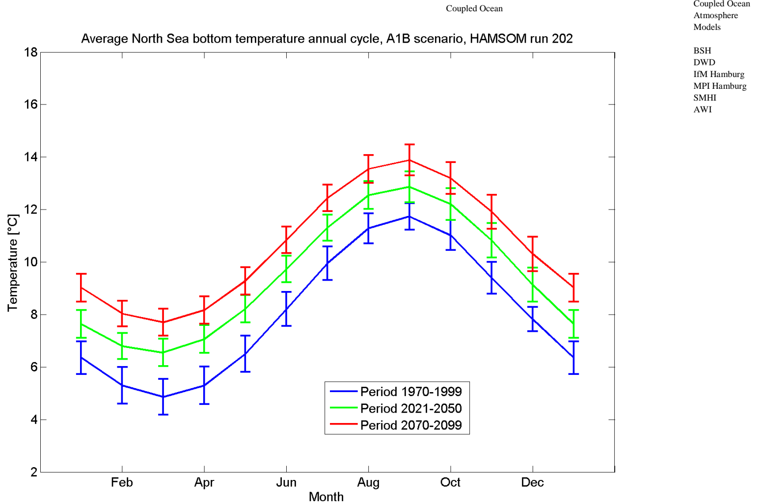
Figure 5.2.12A: The mean annual cycle of bottom temperatures [°C] for HAMSOM run 202 (A1B scenario run) for 1970-1999 (blue), 2021-2050 (green) and 2070-2099 (red). The means are representing averages over the North Sea area given in Figure 4.1. The error bars are indicating time variability.
