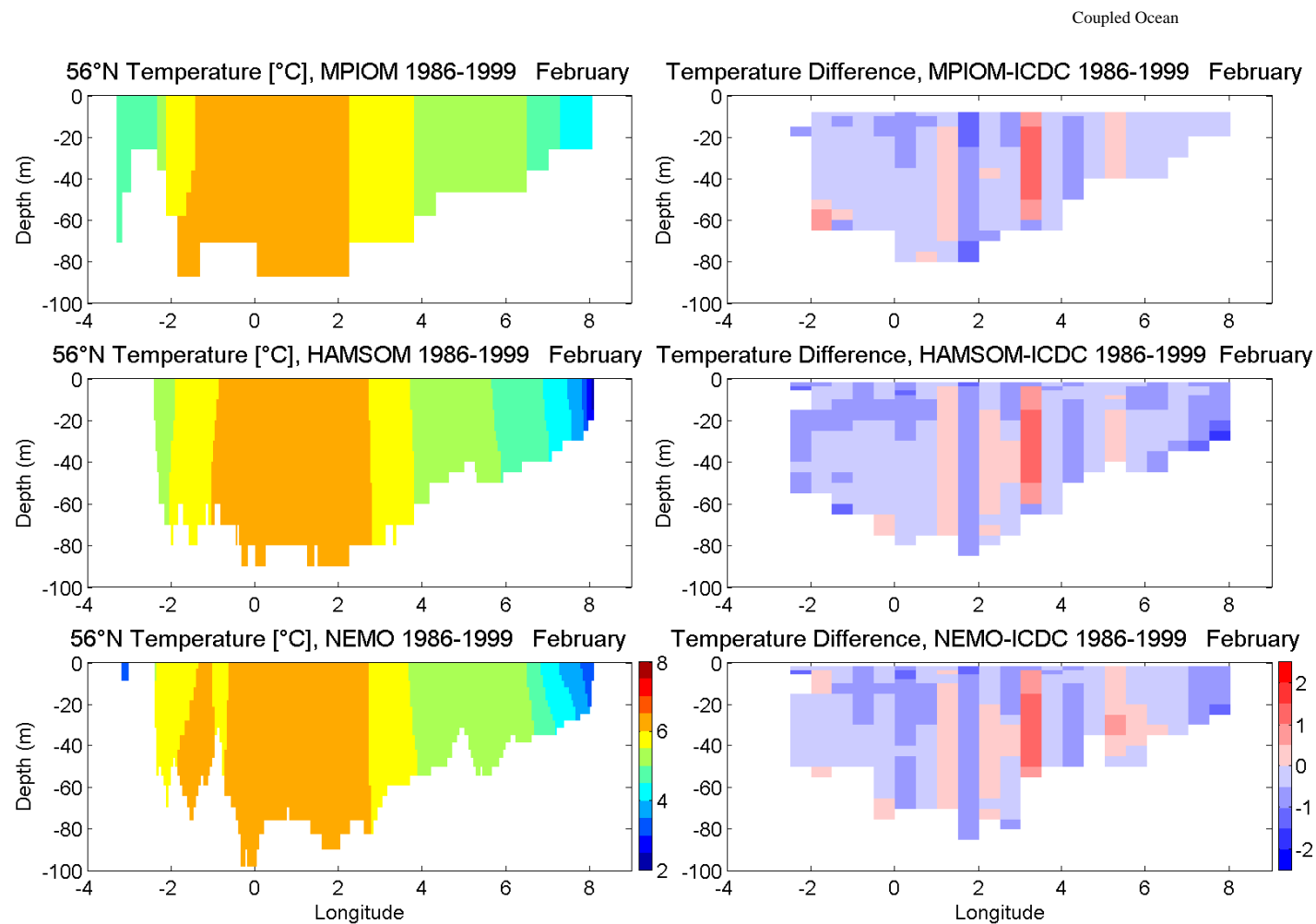
Figure 4.4.5A: The mean February temperature [°C] for the time period 1986-1999 is presented for transect along 56°N. Mean simulated temperature by MPIOM, HAMSOM and NEMO-Nordic (from top to bottom) is presented on the left hand side and on the right hand side the difference between each model result and the temperature from the KNCS climatology.
