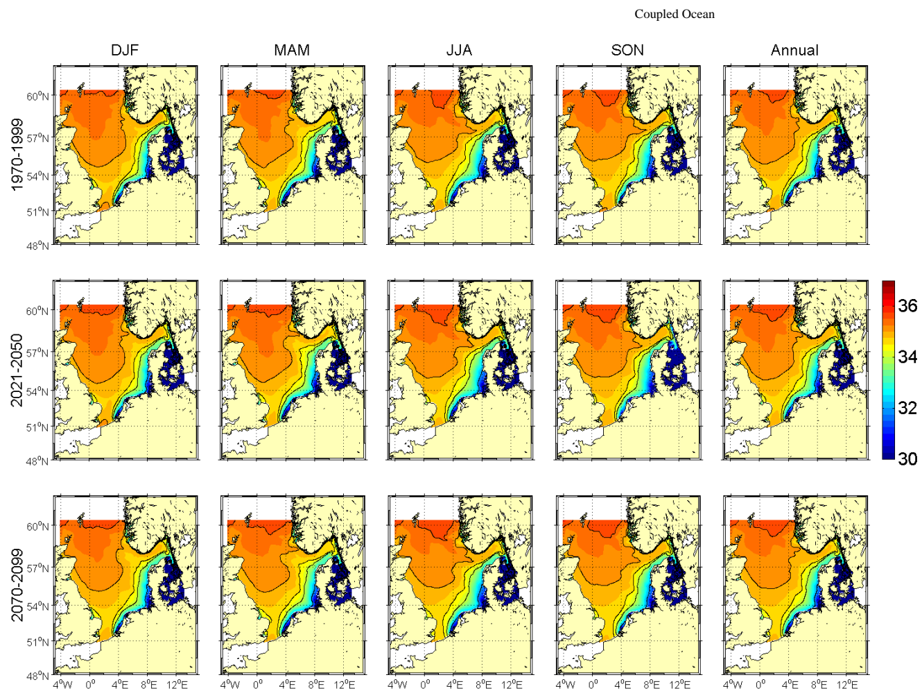
Figure 5.2.16A: Seasonal and annual means of bottom salinity [psu] for HAMSOM run 202 (A1B scenario run). The upper row shows averages for the period 1970-1999, the middle row for 2021-2050 and the lower row for 2070-2099.
