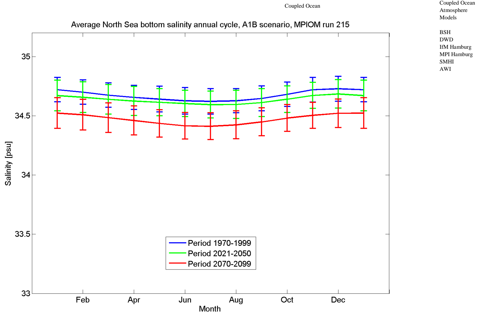
Figure 5.1.24A: The mean annual cycle of bottom salinity [psu] for MPIOM run 215 (A1B scenario run) for 1970-1999 (blue), 2021-2050 (green) and 2070-2099 (red). The means are representing averages over the North Sea area given in Figure 4.1. The error bars are indicating time variability.
