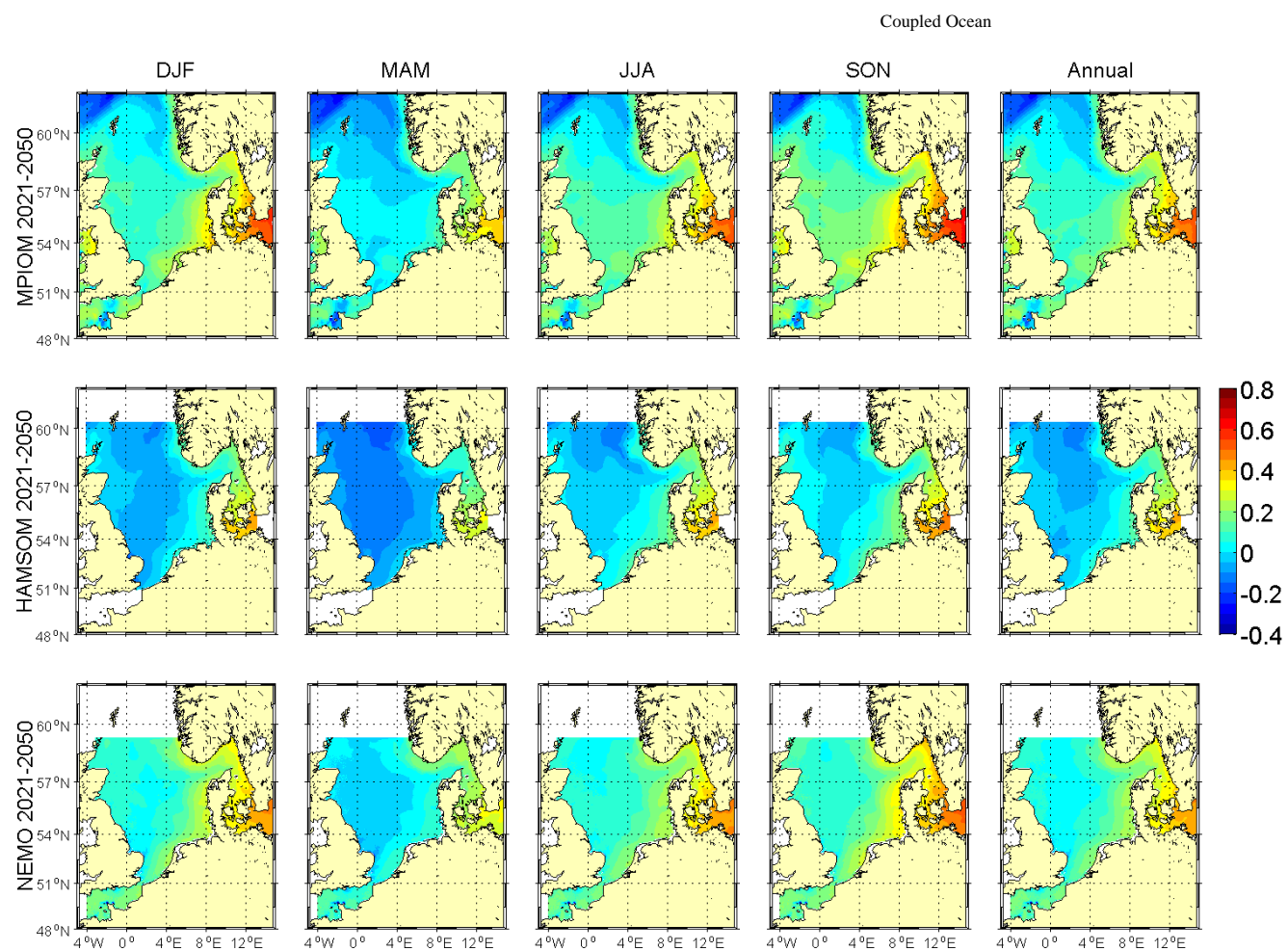
Figure 5.4.30A: Seasonal and annual means of sea surface height [m] for the period 2021-2050. Upper row MPIOM run 215, middle row HAMSOM run 202 and lower row NEMO-Nordic run 470 (all A1B scenario).
