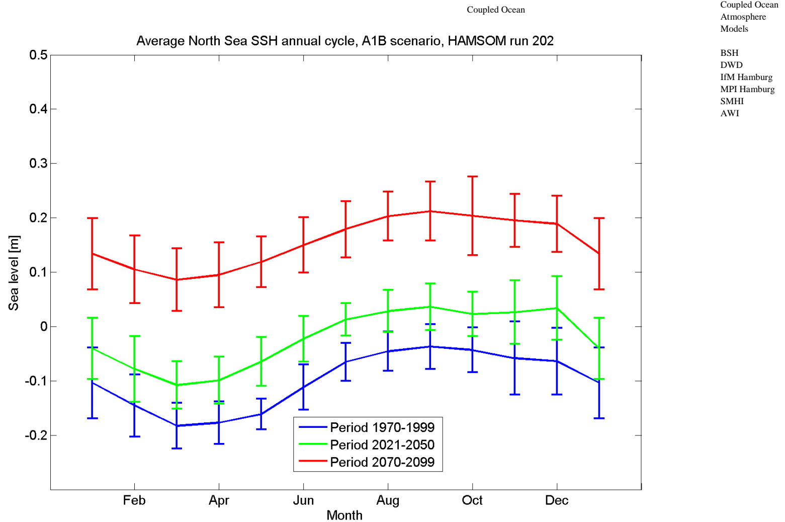
Figure 5.2.28A: The mean annual cycle of sea surface height [m] for HAMSOM run 202 (A1B scenario run) 1970-1999 (blue), 2021-2050 (green) and 2070-2099 (red). The means are representing averages over the North Sea area given in Figure 4.1. The error bars are indicating time variability.
