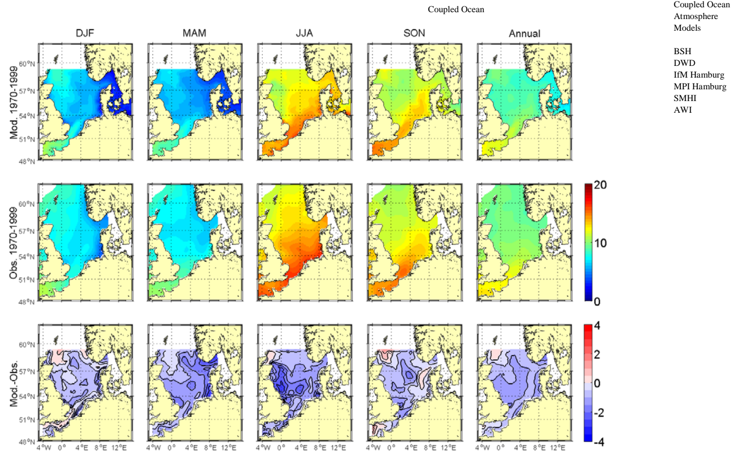
Figure 5.3.2A: Comparison of seasonal and annual means of sea surface temperature [°C] for NEMO-Nordic run 470 for the base period 1970-1999 with BHC means. The upper row shows average model distributions, the middle row observed climatological means and in the lower row the difference between the model results and the climatology.
