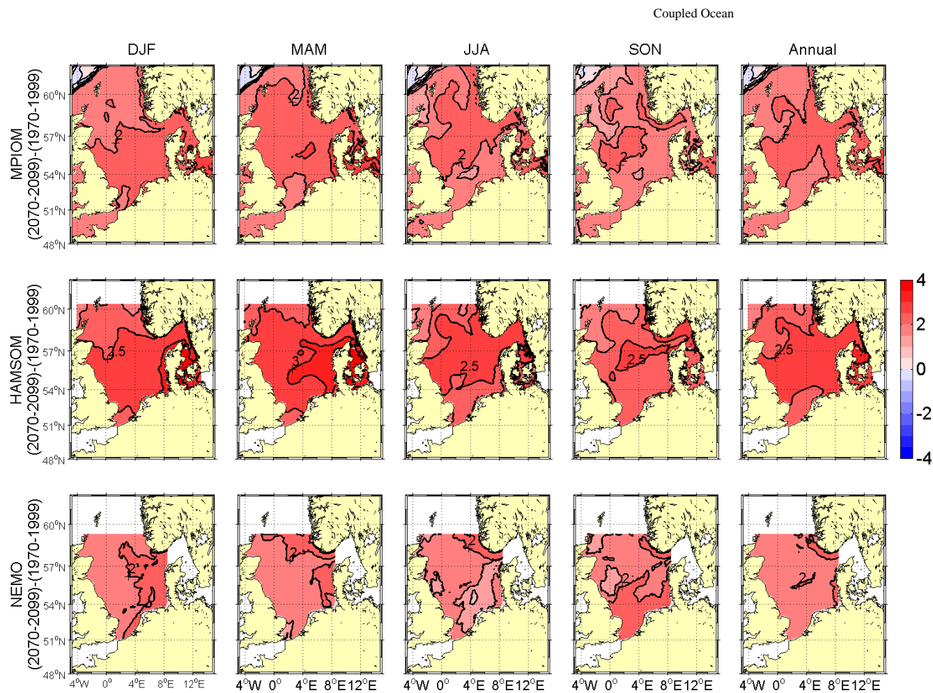
Figure 5.4.10A: Changes in seasonal and annual means of bottom temperature [°C] from (1970-1999) to (2070-2099). Upper row MPIOM run 215, middle row HAMSUM run 202 and lower row NEMO-Nordic run 470 (all A1B scenario). Selected isolines have been labelled for better orientation, contour interval is 0.5 °C.
