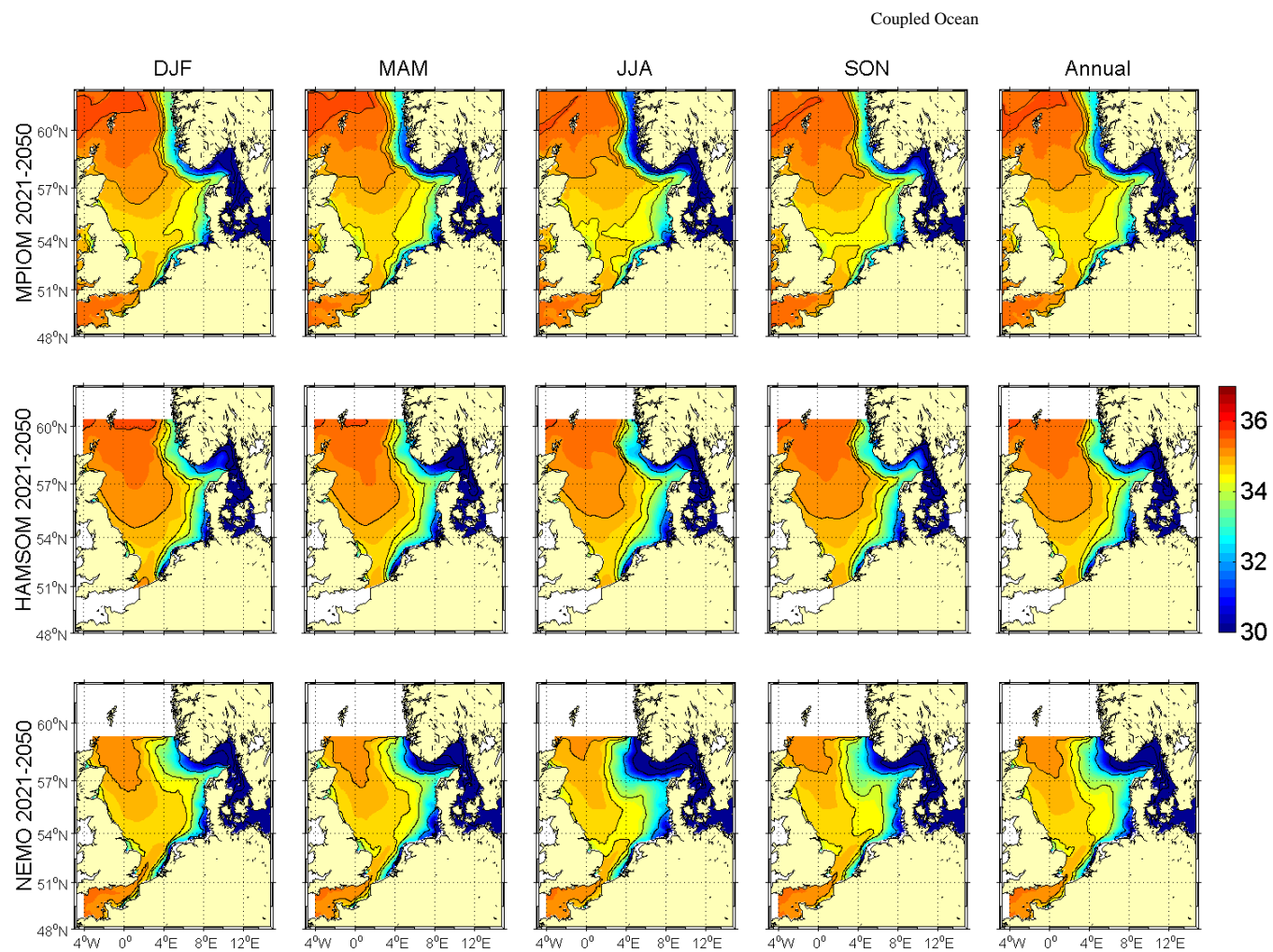
Figure 5.4.16A: Seasonal and annual means of sea surface salinity [psu] for the period 2021-2050. Upper row MPIOM run 215, middle row HAMSOM run 202 and lower row NEMO-Nordic run 470 (all A1B scenario).
