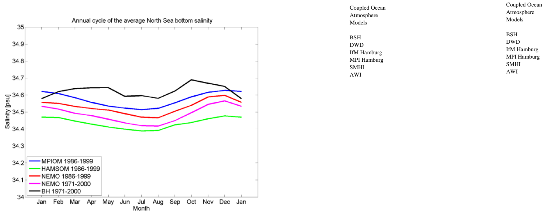
Figure 4.2.5A: The mean annual cycle of bottom salinity [psu] for MPIOM run 253 1986-1999 (blue), HAMSOM 1986-1999 (green), NEMO-Nordic run 477 1986-1999 (red), NEMO-Nordic run 477 1971-2000 (magenta), BHC (black). The means are representing averages over the North Sea area.
