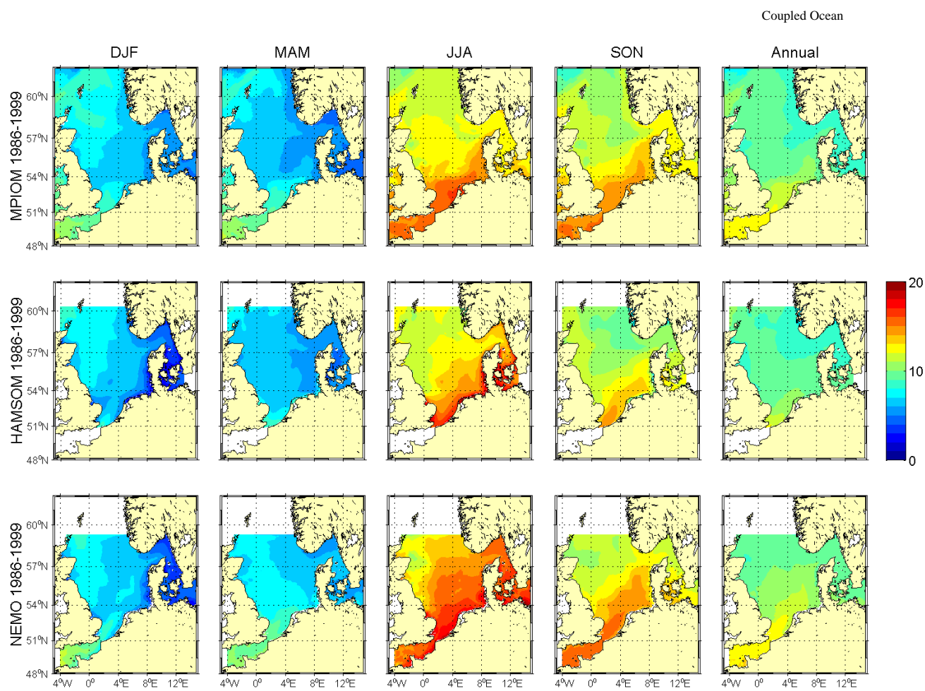
Figure 4.3.3A: Seasonal and annual means of sea surface temperature [ ^{\circ}\text{C} ] averaged over the period 1986-1999. The mean SST results from MPIOM (run 253) are presented in the upper row, in the middle row from HAMSOM (run 201) and in the lower row from NEMO-Nordic (run 477).
