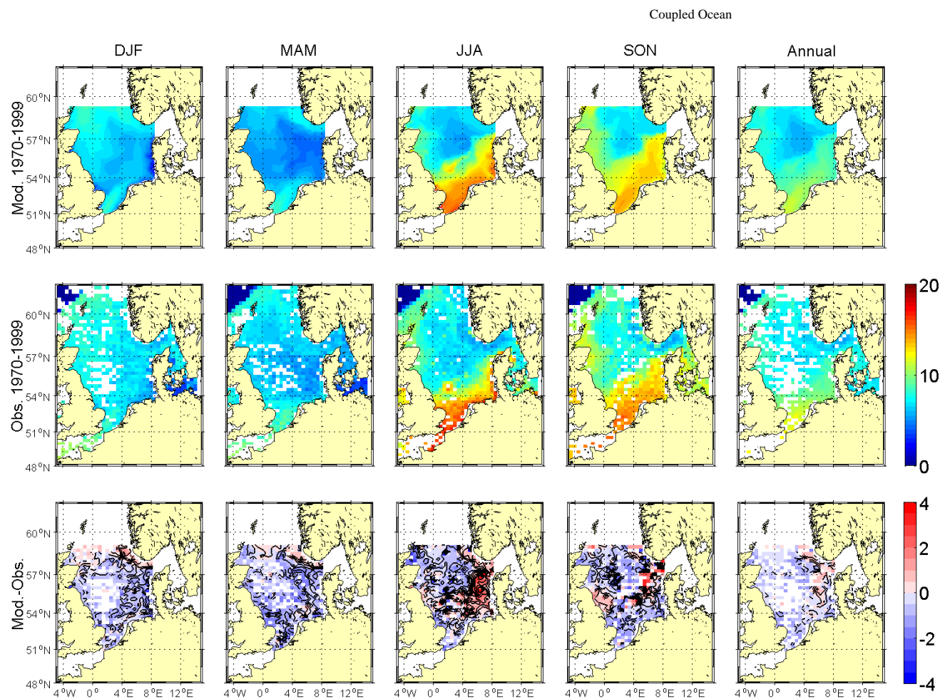
Figure 5.3.6A: Comparison of seasonal and annual means of bottom temperature [°C] for NEMO-Nordic run 470 for the base period 1970-1999 with KNCS means. The upper row shows average model results, the middle row observed climatological means and the lower row the difference between the model results and the climatology.
