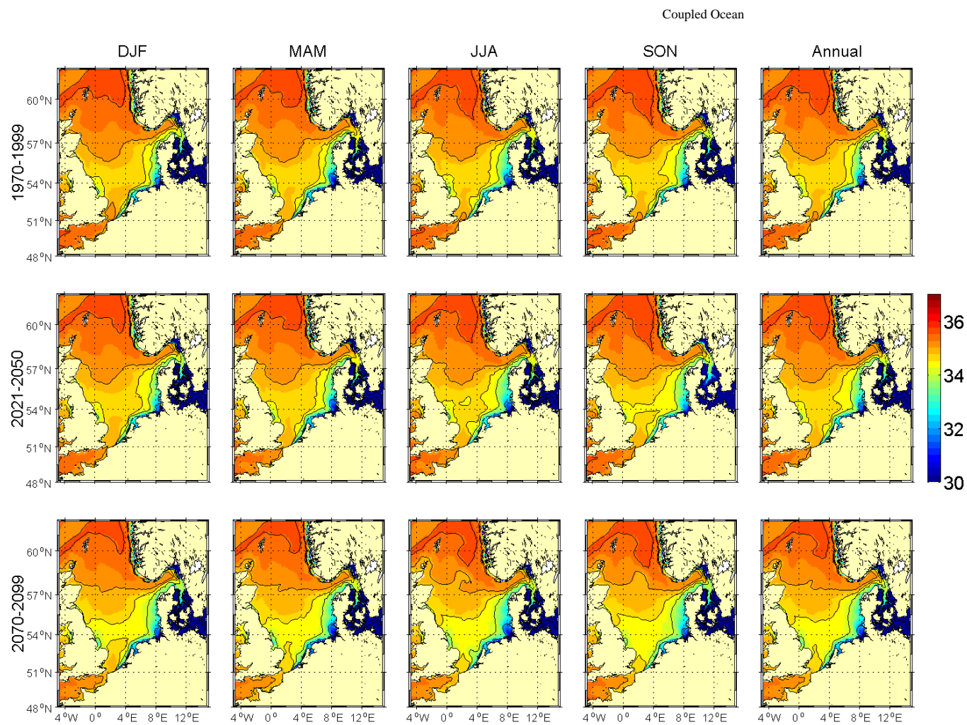
Figure 5.1.16A: Seasonal and annual means of bottom salinity [psu] for MPIOM run 215 (A1B scenario run). The upper row shows averages for the period 1970-1999, the middle row for 2021-2050 and the lower row for 2070-2099.
