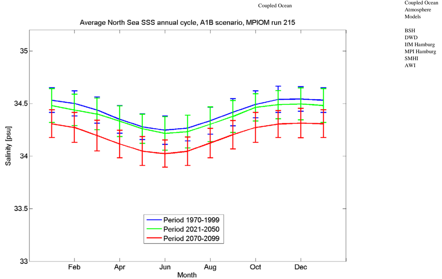
Figure 5.1.22A: The mean annual cycle of sea surface salinity [psu] for MPIOM run 215 (A1B scenario run) for 1970-1999 (blue), 2021-2050 (green) and 2070-2099 (red). The means are representing averages over the North Sea area given in Figure 4.1. The error bars are indicating time variability.
