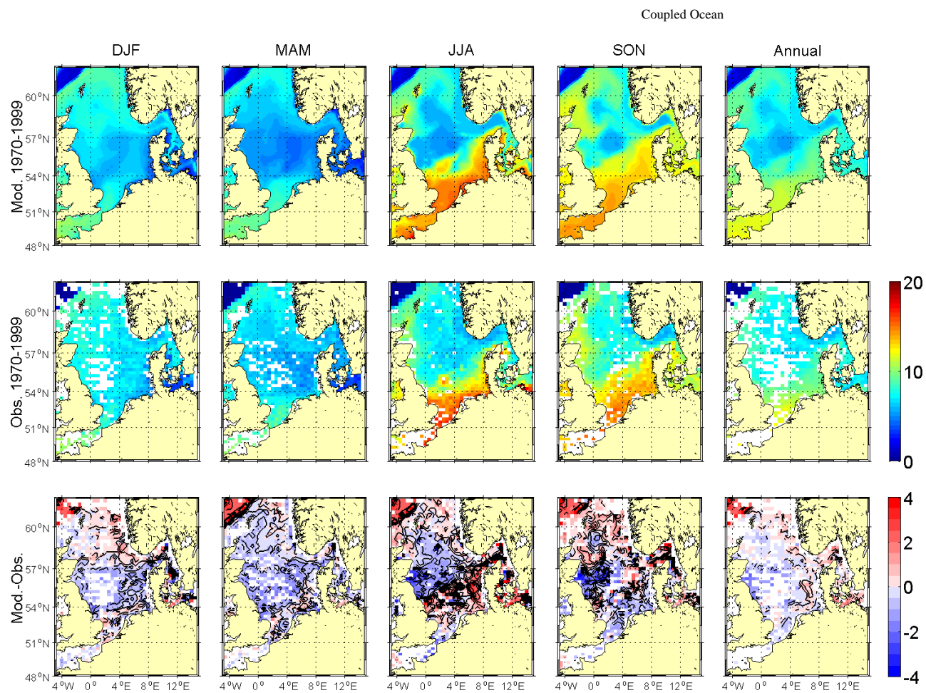
Figure 5.1.6A: Comparison of seasonal and annual means of bottom temperature [°C] for MPIOM run 215 for the base period 1970-1999 with KNSC means. The upper row shows average model distributions, the middle row observed climatological means and the lower row the difference between the model results and the climatology.
