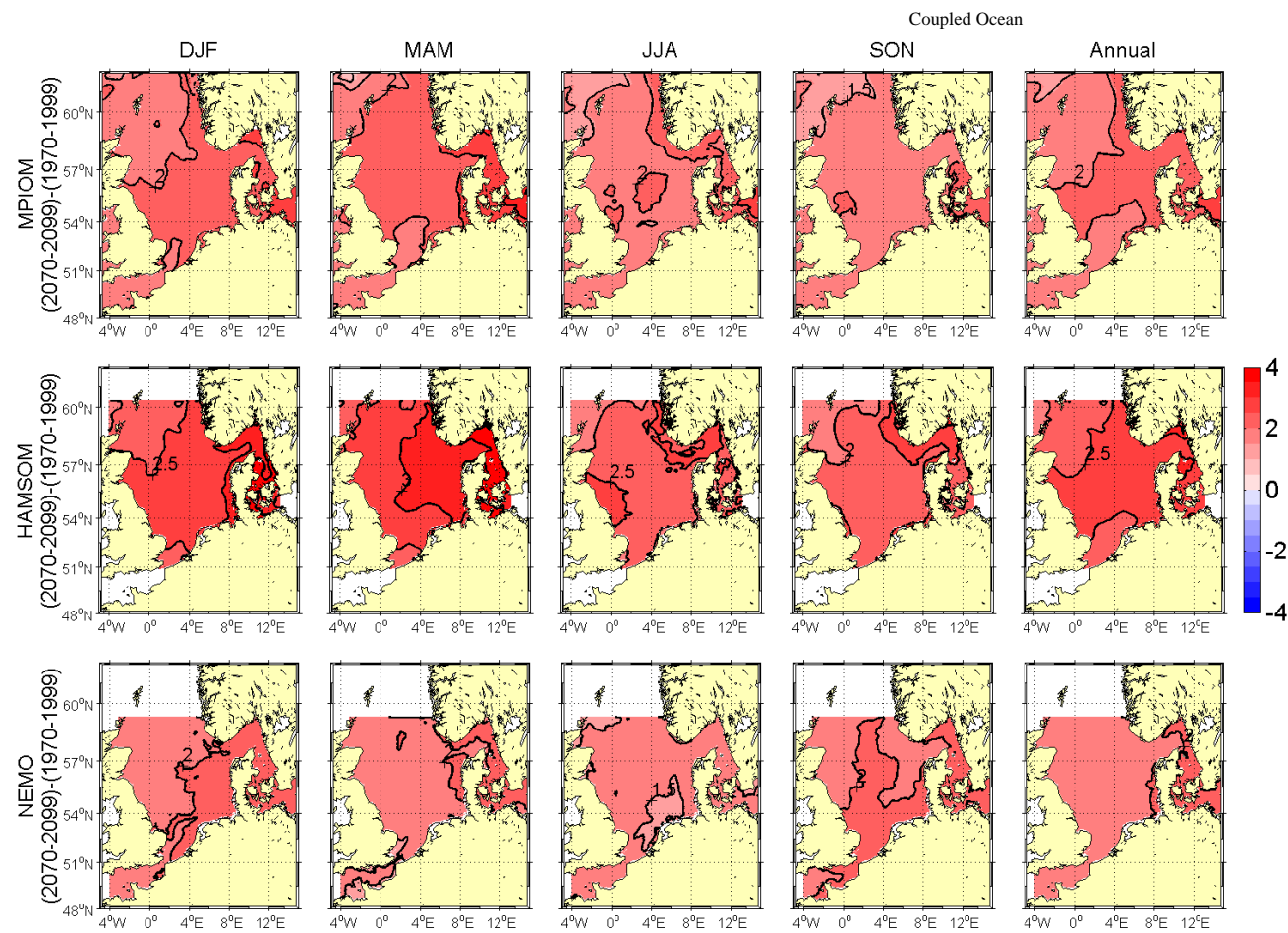
Figure 5.4.8A: Changes in seasonal and annual means of sea surface temperature [°C] from (1970-1999) to (2070-2099). Upper row MPIOM run 215, middle row HAMSOM run 202 and lower row NEMO-Nordic run 470 (all A1B scenario). Selected isolines have been labelled for better orientation, contour interval is 0.5 °C.
