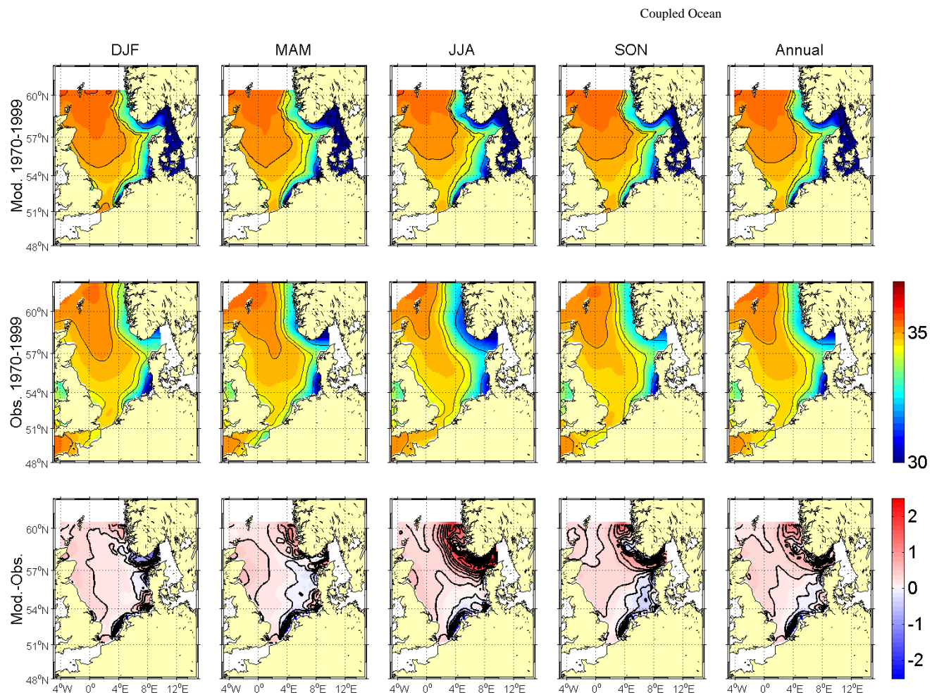
Figure 5.2.14A: Comparison of seasonal and annual means of sea surface salinity [psu] for HAMSOM run 202 for the base period 1970-1999 with BHC means. The upper row shows average model distributions, the middle row observed climatological means and the lower row the difference between the model results and the climatology.
