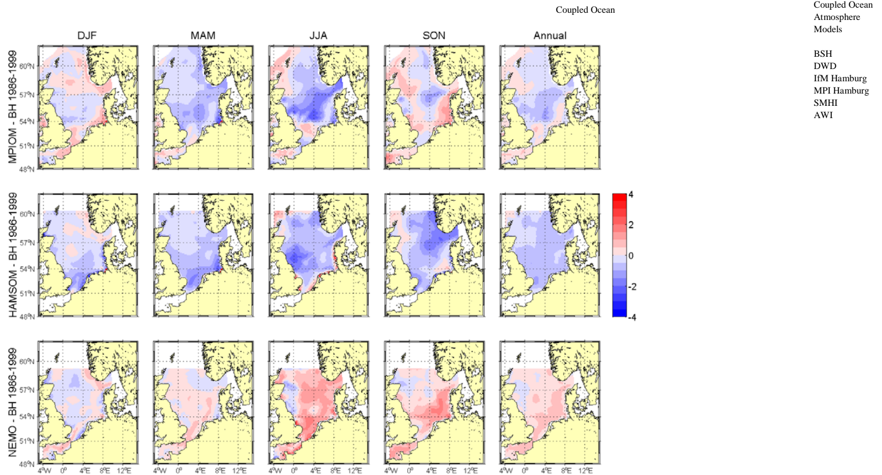
Figure 4.3.5A: Differences of modelled seasonal and annual means of sea surface temperature [°C] averaged over the period 1986-1999 to the BHC (1971-2000): MPIOM (run 253, upper row), HAMSOM (run 201, middle row) and from NEMO-Nordic (run 477, lower row).
