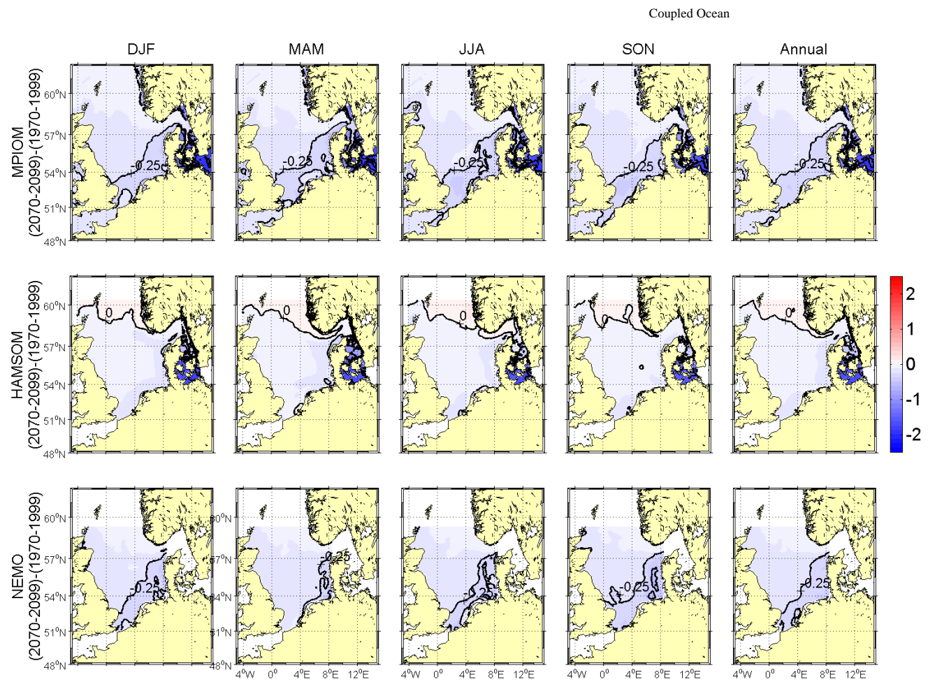
Figure 5.4.24A: Changes in seasonal and annual means of bottom salinity [psu] from (1970-1999) to (2070-2099). Upper row MPIOM run 215, middle row HAMSOM run 202 and lower row NEMO-Nordic run 470 (all A1B scenario). Selected isolines have been labelled for better orientation, contour interval is 0.25 psu.
