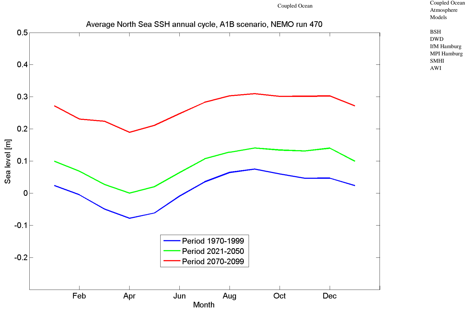
Figure 5.3.28A: The mean annual cycle of sea surface height [m] for NEMO-Nordic run 470 (A1B scenario run) for 1970-1999 (blue), 2021-2050 (green) and 2070-2099 (red). The means are representing averages over the North Sea area given in Figure 4.1.
