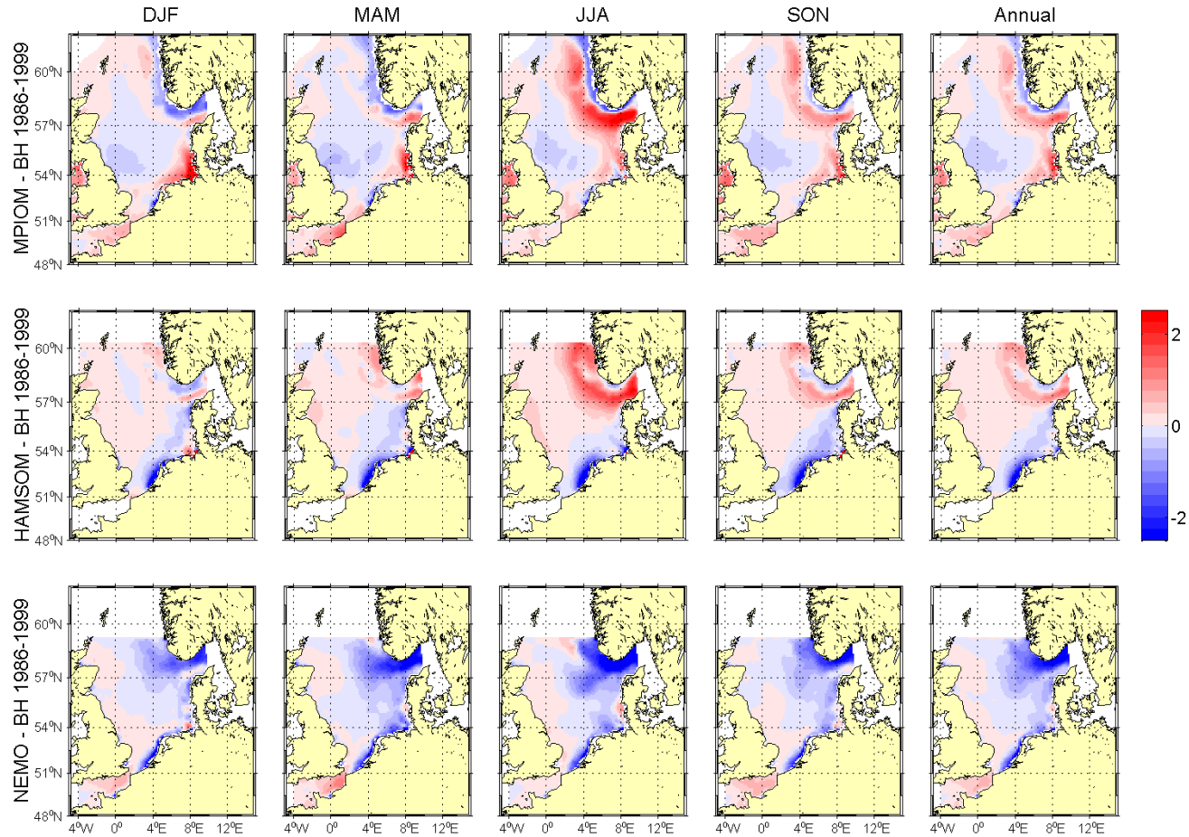
Figure 4.3.8A: Differences of modelled seasonal and annual means of sea surface salinity [psu] (1986-1999) to the BHC (1971-2000): MPIOM (run 253, upper row), HAMSOM (run 201, middle row) and from NEMO-Nordic (run 477, lower row).
