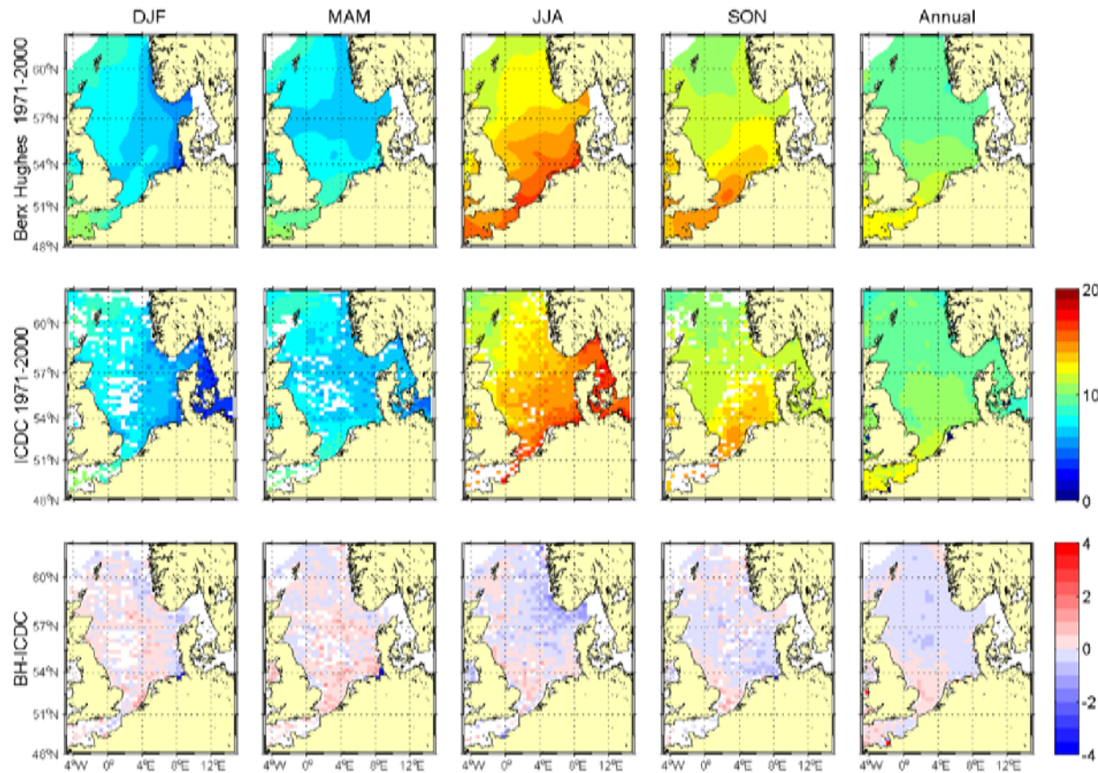
Figure 4.3.1A: Seasonal and annual means of sea surface temperature [°C] from BHC (upper row) and KNSC (ICDC, middle row) for the period 1971-2000 and their differences (lower row).
