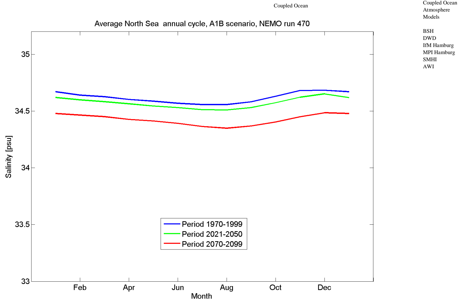
Figure 5.3.24A: The mean annual cycle of bottom salinity [psu] for NEMO-Nordic run 470 (A1B scenario run) for 1970-1999 (blue), 2021-2050 (green) and 2070-2099 (red). The means are representing averages over the North Sea area given in Figure 4.1.
