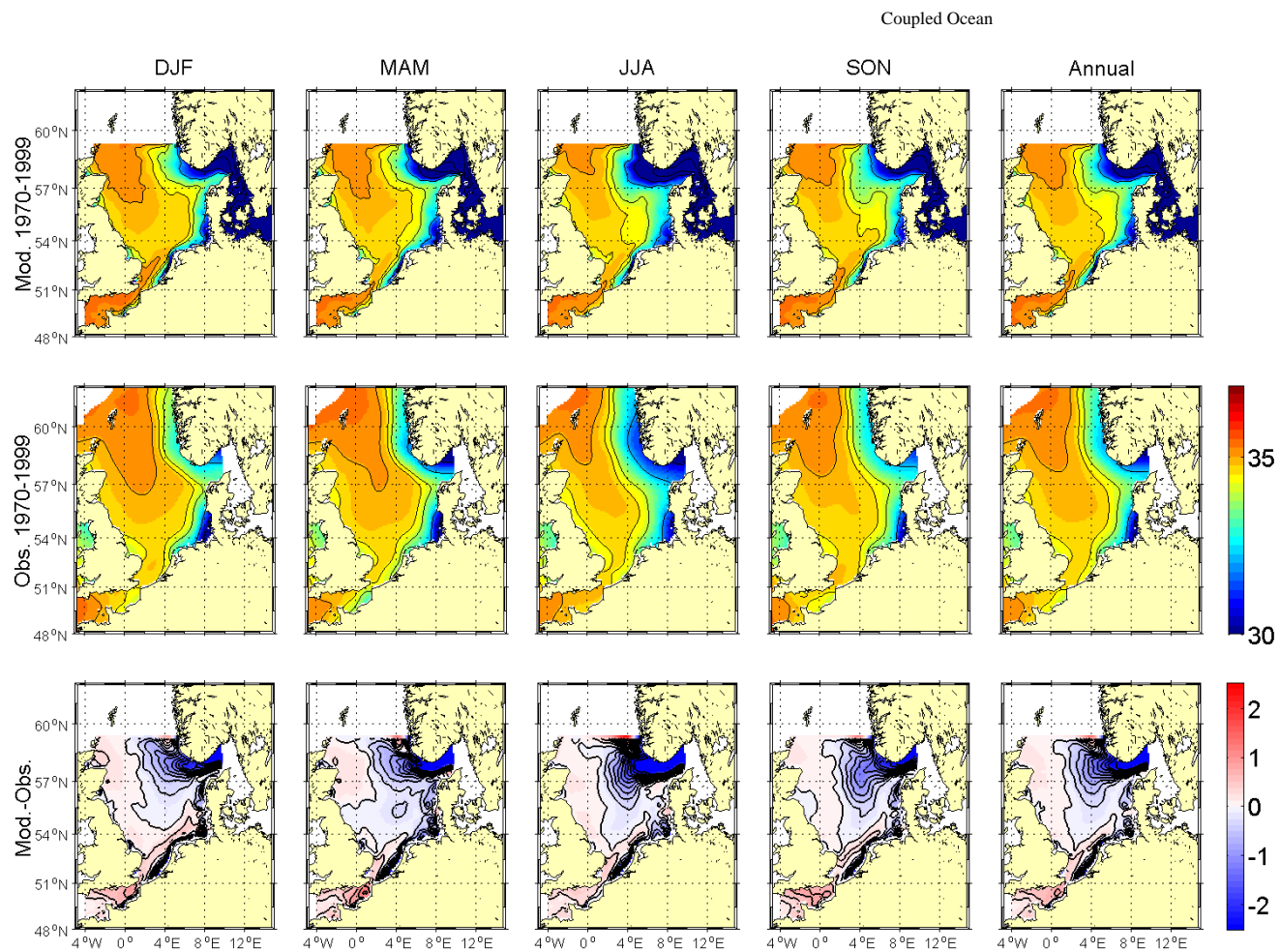
Figure 5.3.14A: Comparison of seasonal and annual means of sea surface salinity [psu] for NEMO-Nordic run 470 for the base period 1970-1999 with BHC means. The upper row shows average model distributions, the middle row observed climatological means and the lower row the difference between the model results and the climatology.
