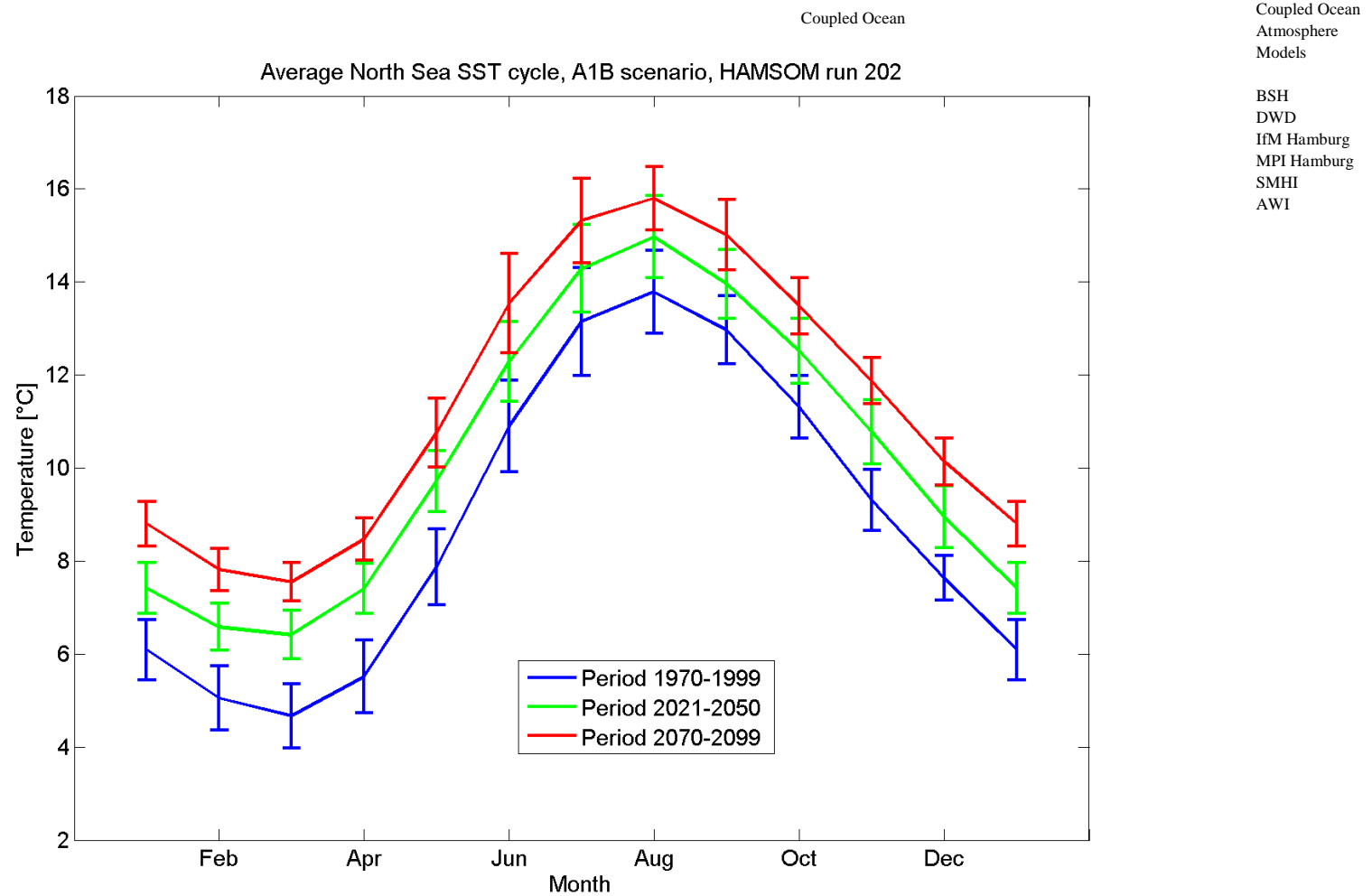
Figure 5.2.10A: The mean annual cycle of sea surface temperatures [°C] for HAMSOM run 202 (A1B scenario run) for 1970-1999 (blue), 2021-2050 (green) and 2070-2099 (red). The means are representing averages over the North Sea area given in Figure 4.1. The error bars are indicating time variability.
