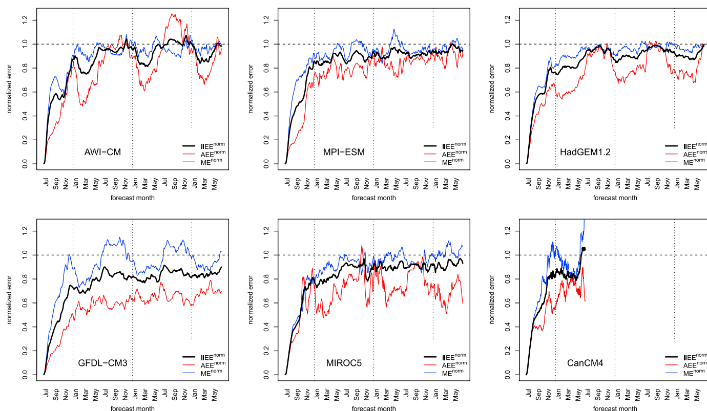
Figure 3. Normalized integrated ice-edge error (IIEE norm ; black), absolute extent error (AEE norm ; red), and misplacement error (ME norm ; blue) for each model. The (negative) deviation from 1 can be interpreted as predictable fraction. The CanCM4 forecast ensembles were integrated only for 1 year. Note that AEE norm and ME norm do not sum to IIEE norm because they have been normalized separately.
