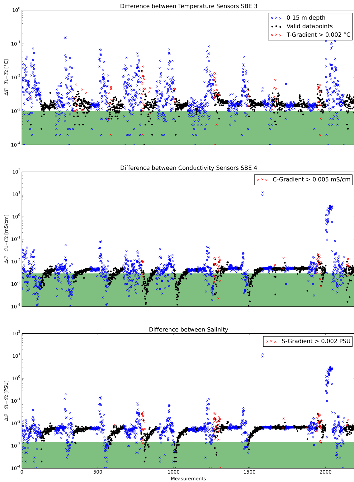
Figure 2: Data accuracy of sensor pairs HE420
