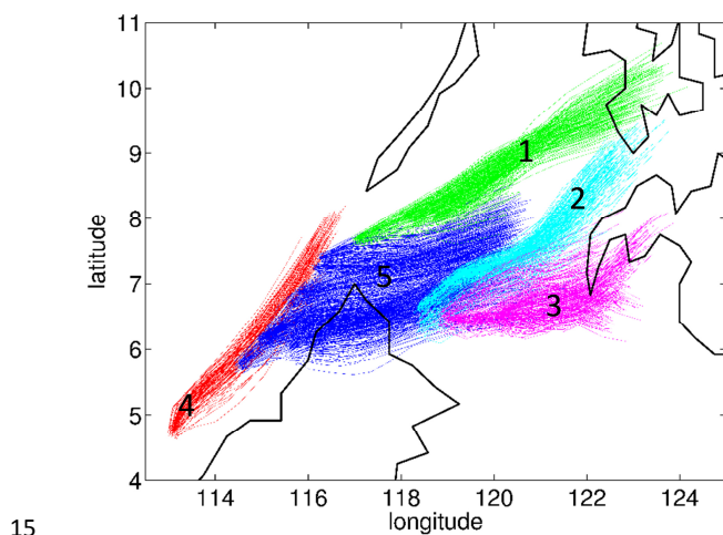
15 Figure 8: Backward trajectories over 24 hours from all OVOC measurement locations are shown. The trajectories are color-coded according to the atmospheric transport regime.
