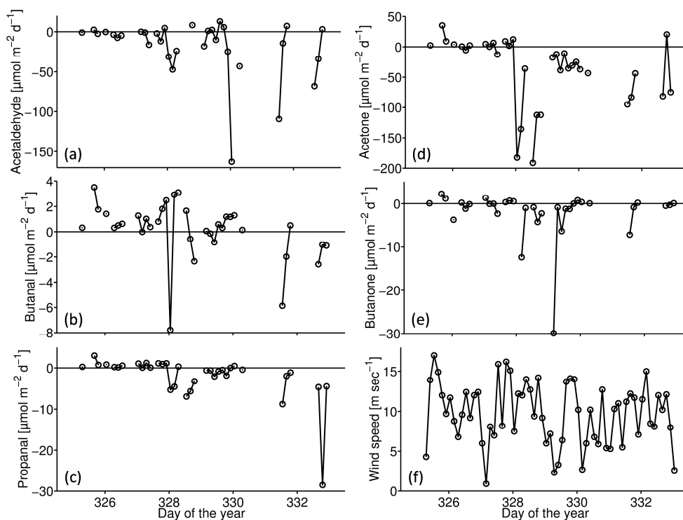
Figure 5: Calculated fluxes of the OVOCs (panel a-e). Fluxes above the zero line indicate fluxes out of the ocean, fluxes below the zero line indicate fluxes into the ocean. Panel f shows the wind speed plotted against the day of the year (DOY).
