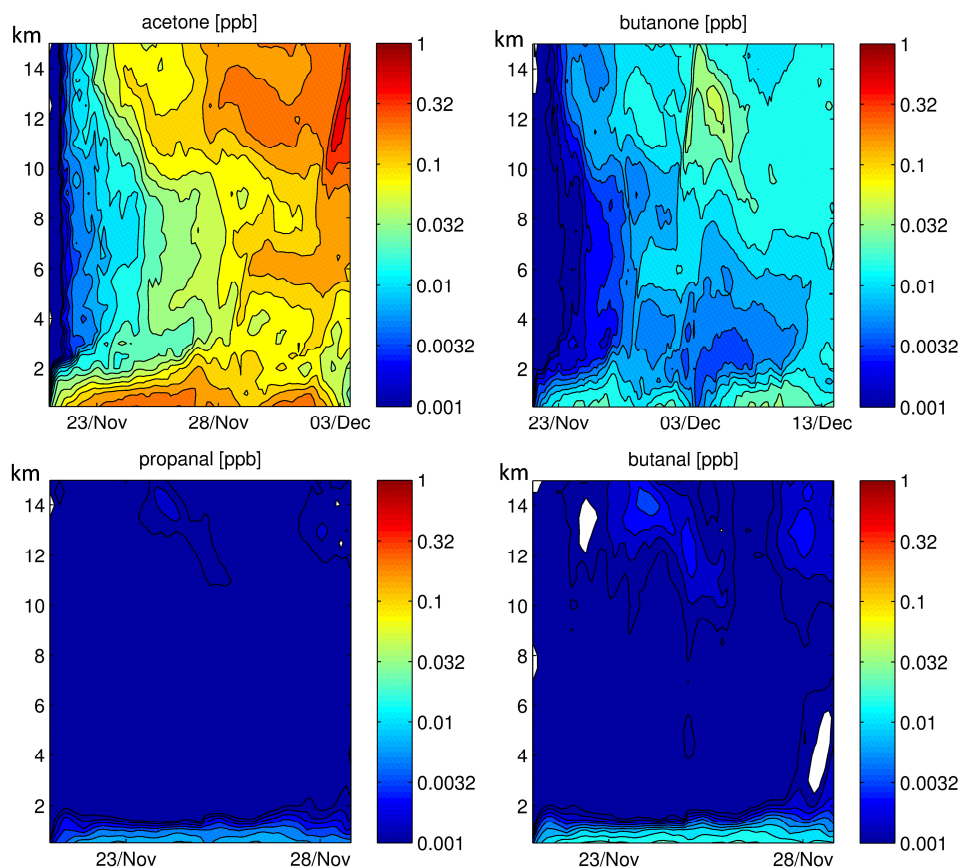
Figure 9: Vertical distribution of the OVOCs derived from FLEXPART model simulations. OVOCs are released from the measurement locations over the time period of the cruise according to the respective ocean-atmosphere flux.
