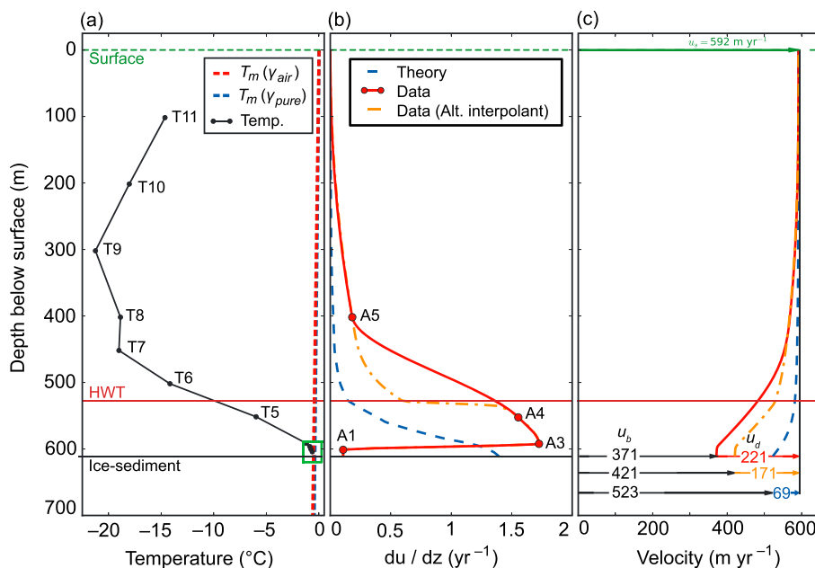
Figure 5. Depth profiles of (a) temperature, (b) internal deformation, and (c) velocity at site S30. The red dashed line on Figure 5a is the Clausius-Clapeyron gradient for pure ice and air-saturated water, and the green box around the ice-sediment interface shows the extent of Figure 6. An alternative interpolant is plotted on Figure 5b with an orange dashed line. Theoretical horizontal velocity gradients du/dz and deformational velocities (blue dashed lines) plotted on Figures 5b and 5c were calculated using Glen’s flow law and the surface slope. See text for details.
