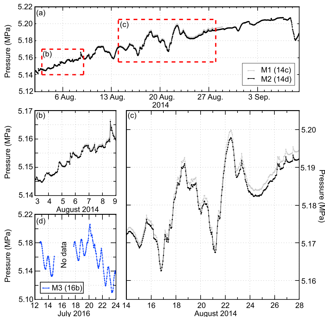
Figure 8. Pressure time series from (a–c) BH14c, BH14d and (d) BH16b. Figures 8b and 8c show enlarged sections of Figure 8a. Data are plotted at an hourly interval.
