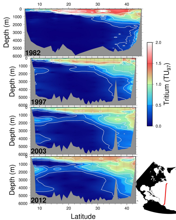
Figure 5. Four meridional tritium sections along roughly 52^{\circ} W in the North Atlantic taken in 1982, 1997, 2003, and 2012. The tritium concentrations have been decay-corrected to a common time (1 January 1997) for comparison. Contour intervals are 0.2 \text{ TU}_{97} , and measurement uncertainties are of order 0.01 \text{ TU}_{97} or better. Due to differences in cruise tracks, the topography for the 1982 occupation differs from the others.
