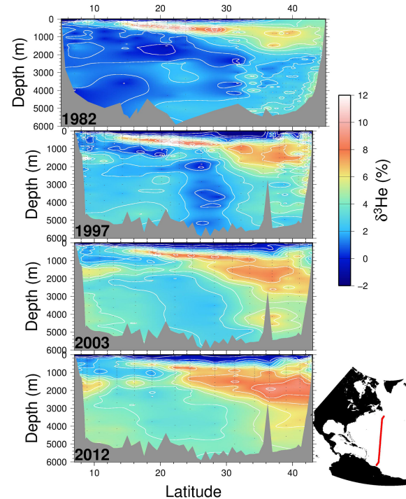
Figure 6. Four meridional \delta^3\text{He} sections along roughly 52^{\circ} W in the North Atlantic taken in 1982, 1997, 2003, and 2012. Contour intervals are 1 \% , and measurement uncertainties are 0.15 \% . Due to differences in cruise tracks, the topography for the 1982 occupation differs from the others.
