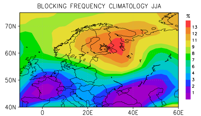
FIGURE 4 Summer blocking frequency climatology. The period is 1950–2015. Units: percent of blocked days from total number of summer days
