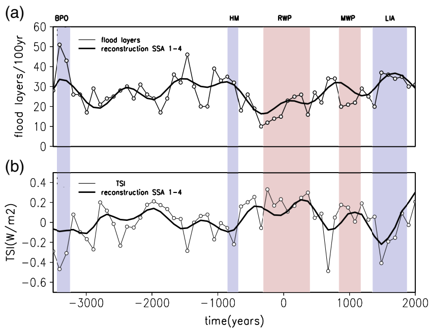
FIGURE 8 (a) Time series of the frequency of flood layer years in a 100-year window (thin) and its reconstruction from the first four SSA components (thick). (b) Time series of 100-year TSI anomaly averages (thin) and its reconstruction from the first four SSA components (thick) (see text for details)
