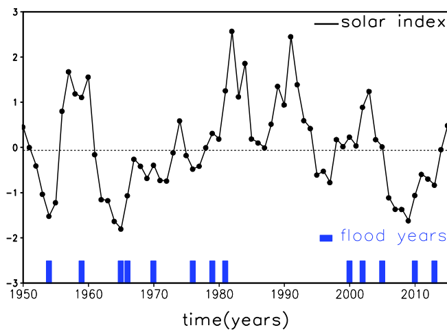
FIGURE 1 River Ammer summer flood years (vertical bars) and solar activity index (solid line) for 1950–2015 (see text for details)
