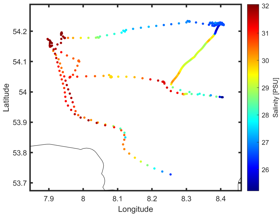
Figure 2: Cruisemap of HE547.
