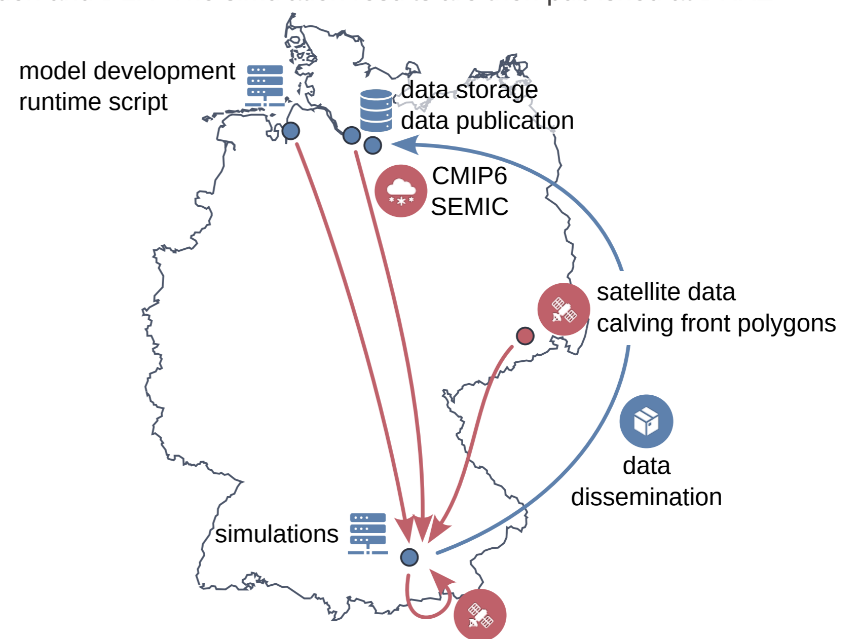
Fig. 4: Illustration of the planned workflow for the ice sheet modeling application. The workflow will be designed to be easily transferable to other applications.
