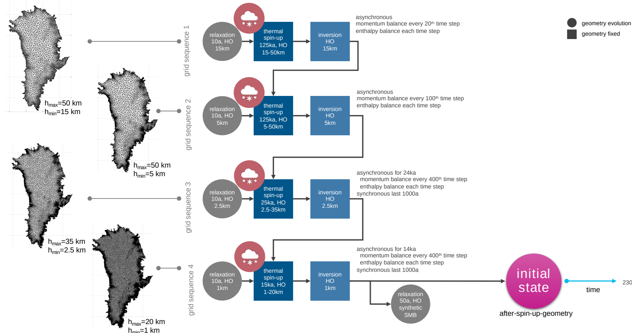
Fig. 3: Illustration of the spinup process used by Rückamp et al. (2018) to generate an initial state for the simulation of the Greenland Ice Sheet. To generate a model of the ice sheet that is consistent with the current geometry and temperature field, several similar simulations have to be run. Here, four different sequences with different grids and different coupling between the evolution of the geometry and the evolution of the temperature field are used.
