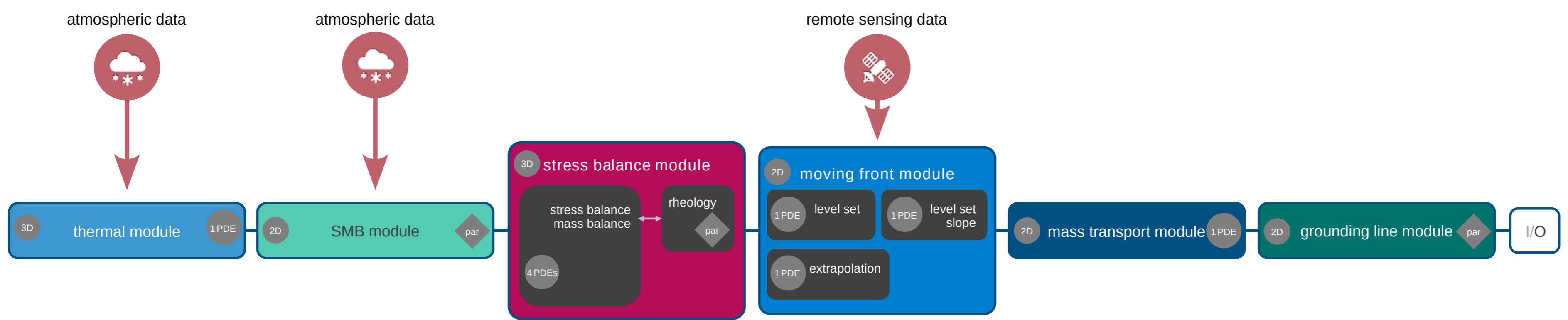
Fig. 1: Schematic showing one time step of a typical ice sheet model. The thermal module, which solves the enthalpy field, relies on atmospheric forcing data. The same is true for the surface mass balance module, which describes mass accumulation and ablation processes at the ice sheet surface. The stress balance module, solves the stress and mass balance of continuum mechanics to evaluate the velocity field. The moving front module, which describes the advance and retreat of the ice sheet's lateral margins, can benefit from additional data derived from satellite remote sensing. The mass transport module describes the evolution of the ice sheet geometry. The grounding line module tracks the position of the grounding line. At the end of the time step, the model output is written.
