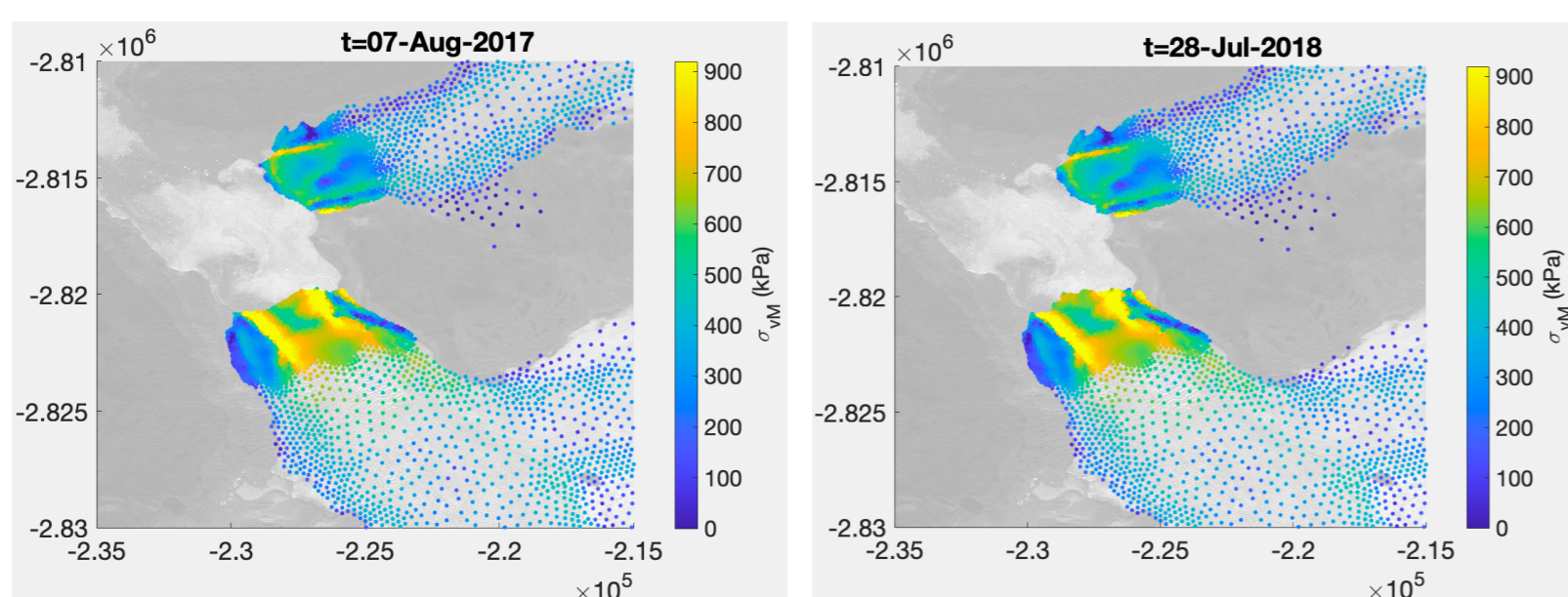
Fig. 2: Prescribing the geometry of floating glacier tongues in Greenland with calving front positions derived from satellite remote sensing allows the calculation of the equivalent von Mises stress, color coded in the figure. Equivalent von Mises stress values are consistent with corresponding calving laws.
