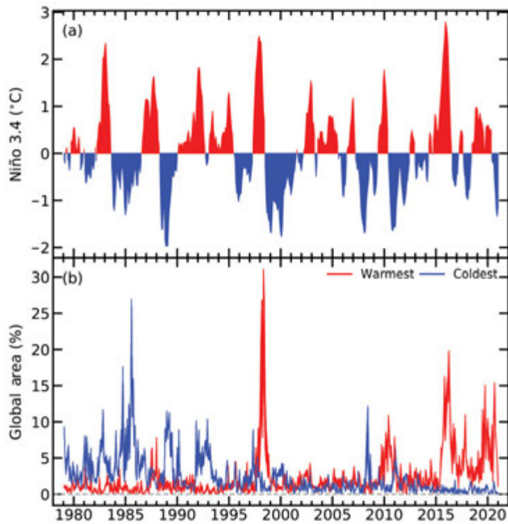
Fig. 2.7. (a) Sea surface temperature anomaly ( ^{\circ}\text{C} ) in the Niño 3.4 region in the central equatorial Pacific. (b) Fraction of Earth (%) with record warm (red) and cold (blue) monthly LTT values. The width of the line represents the difference between the UAH and RSS datasets.
