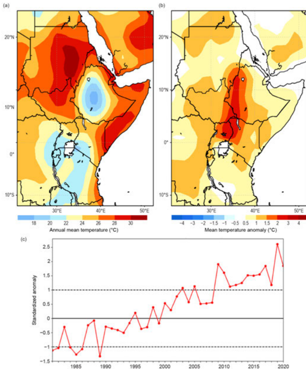
Fig. 7.26. Annual (a) mean temperature ( ^{\circ}\text{C} ) and (b) mean temperature anomalies ( ^{\circ}\text{C} ) for East Africa. 1981–2010 base period. (c) Annual standardized temperature anomaly time series for the period 1981–2020. (Sources: NOAA/NCEP and NOAA CPC.)
