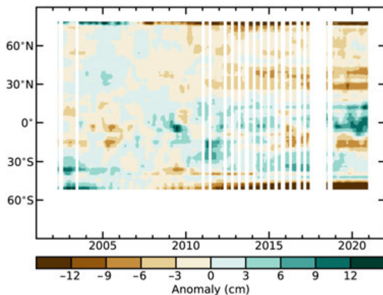
Fig. 2.31. Zonal means of terrestrial water storage anomalies, excluding those in Antarctica, Greenland, the Gulf Coast of Alaska, and polar islands, in cm equivalent height of water, based on gravity observations from GRACE and GRACE-FO. The anomalies are relative to a base period of 2004–09.
