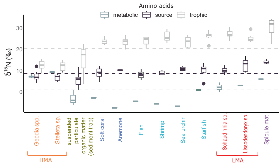
FIGURE 3 δ 15 N values for the different amino acid classes. Horizontal dotted lines indicate the average value of all individual samples for the respective classes.
