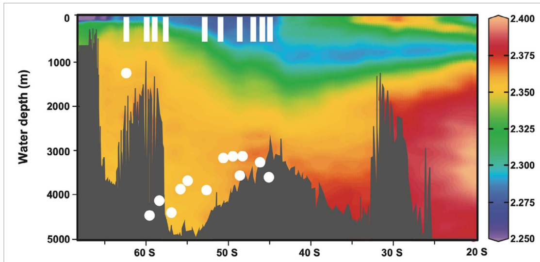
Fig. 5.23: Section along the cruise track on the EIOT, projected onto 100° E latitude. Shown are GLODAP 2.2-based atlas values of alkalinity in mmol/kg are shown, with locations of station sampling. White lines mark deployments of multi-net for plankton sampling. White dots show stations with MUC and core sampling. Note that dots were projected onto the plane of the transect and thus do not always show accurate bottom topography.
