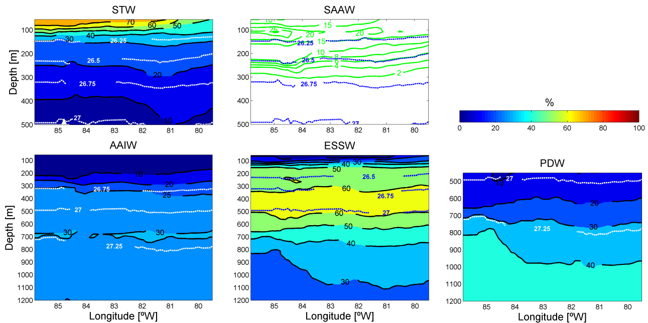
Fig. 3. Water mass distribution (%) along the 14° S section between 85°50' W and the continental shelf for the M77 cruise (February 2009), for subtropical water (STW), subantarctic water (SAAW), antarctic intermediate water (AAIW), equatorial subsurface water (ESSW) and pacific deep water (PDW) as defined in Table 1. Selected isopycnals are shown as dotted white/blue lines.
