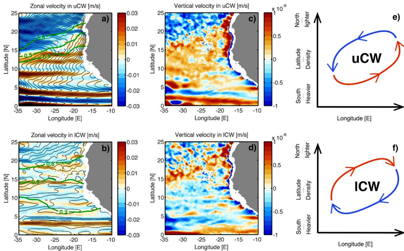
Figure 11. Flow patterns in the northeastern tropical Atlantic Ocean as deduced from the climatological ECCO2 annual-mean flow field. Vertically averaged zonal velocity (in color) for (a) the uCW and (b) the ICW strata; positive values denote eastward flow. Black contours denote the Eulerian stream function with 0.1 Sv increments; green contours represent the averaged NACW proportion within the corresponding layer. (c, d) Analogous plots but for the vertical velocity, with the positive values denoting upward flow. (e, f) Simplified schemes of the 3-D circulation in both layers.
