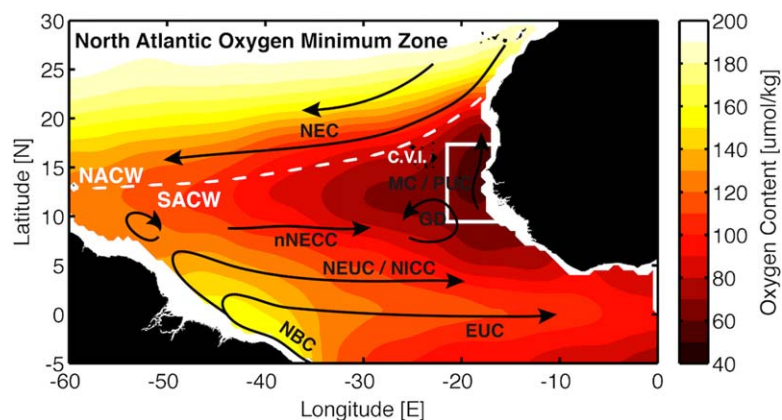
Figure 1. Schematic circulation pattern in the tropical Atlantic Ocean as derived from previous studies, overlaying the climatological oxygen content of the 200–500 m layer. The naOMZ box (Lagrangian particles release region) is indicated by a white box. The frontal zone between SACW and NACW is shown as a white-dashed line; C.V.I. refers to the Cape Verde Islands. Main currents: North Brazil Current (NBC), Equatorial Undercurrent (EUC), North Equatorial Undercurrent (NEUC), North Intermediate Counter Current (NICC), northern branch of the North Equatorial Counter Current (nNECC), Mauritanian Current (MC), Poleward Undercurrent (PUC), Guinea Dome (GD), and North Equatorial Current (NEC).
