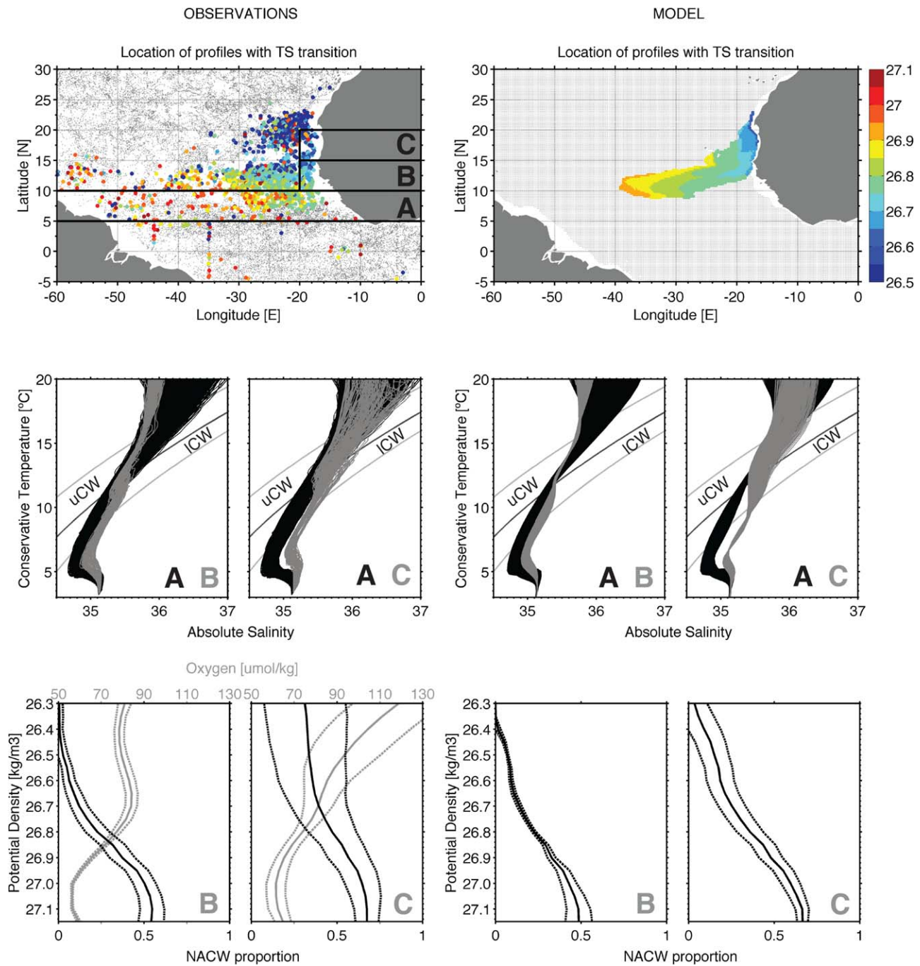
Figure 3. (top) The colored dots show the location of the T/S profiles with a marked thermohaline transition, defined as a change in the slope of the T/S profiles greater than 0.1°C per salinity unit with respect to the NACW and SACW predefined slopes. The color code indicates the density level where the transition is found. (middle) T/S diagrams of those profiles located in the A, B, and C regions shown in the top-left panel, plotted according to the black-gray code shown inside each box; regions B and C include 135 and 109 profiles, respectively. (bottom) Mean profiles of NACW proportion and oxygen content for regions B and C; the dashed lines denote one standard deviation. The left plots are for the observational data set, while the right plots are for the ECCO2 model output. Note that the ECCO2 model does not include the oxygen field.
