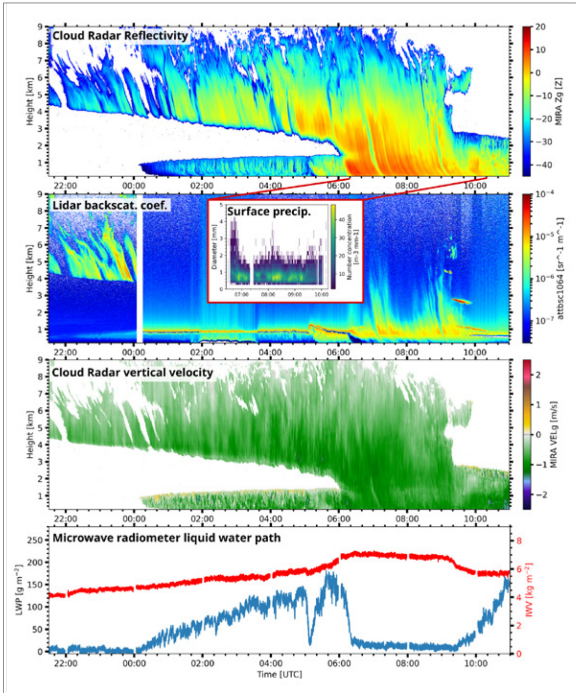
Fig. 4.20.2: An exemplary dataset from 18-19 April 2023: Shown are the cloud radar reflectivity, lidar backscatter, cloud particle vertical velocity, liquid water path and integrated water vapour. The inset shows precipitation data from the disdrometer.
