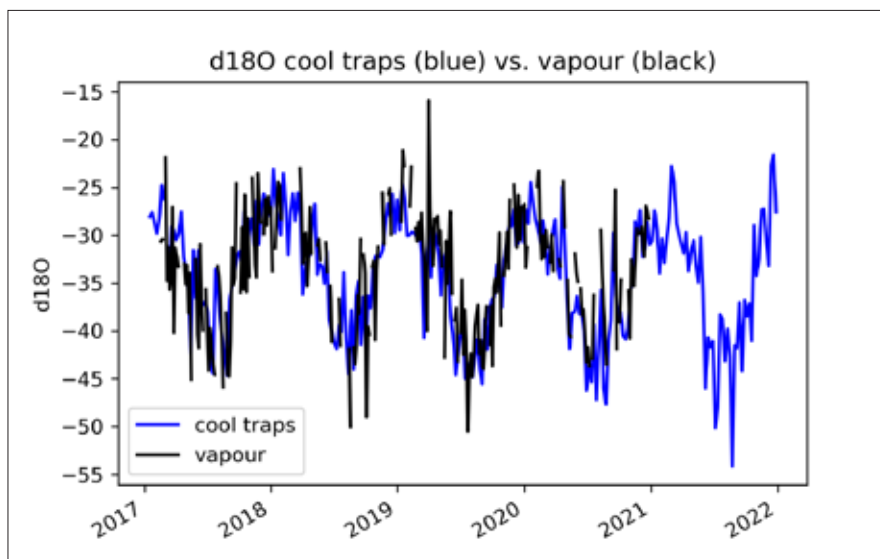
Fig. 4.29.2: Isotope \delta^{18}\text{O} variations measured at water samples collected from cold traps (blue line) and measured directly in vapour (black line) at Neumayer III Station during the years 2017-2022 (unpublished figure by M. Hoerhold and M. Behrends, AWI, 2023).
