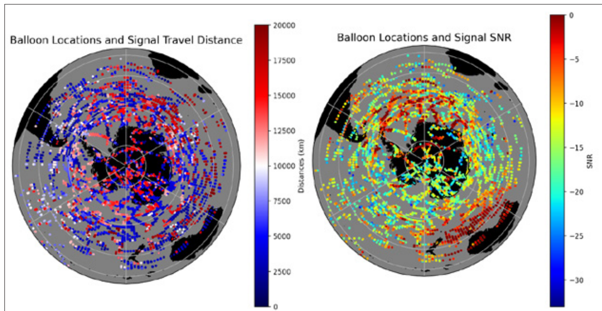
Fig. 4.21.4: Maps depicting the maximum distance and highest SNR obtained for each WSPR grid square, displaying data from all six long-duration WSPR flights. The distance scale features white to indicate the distance between the South Pole and the equator for reference purposes.
