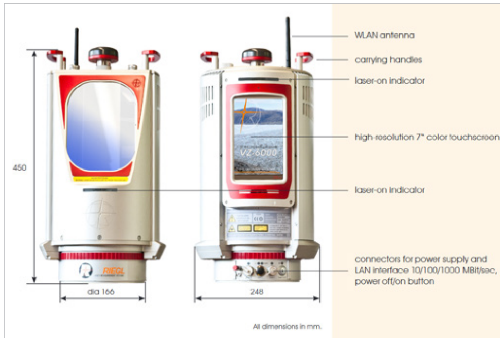
Fig. 4.22.1: RIEGL VZ® - 6000: operating elements and connectors (RIEGL, 2020)
