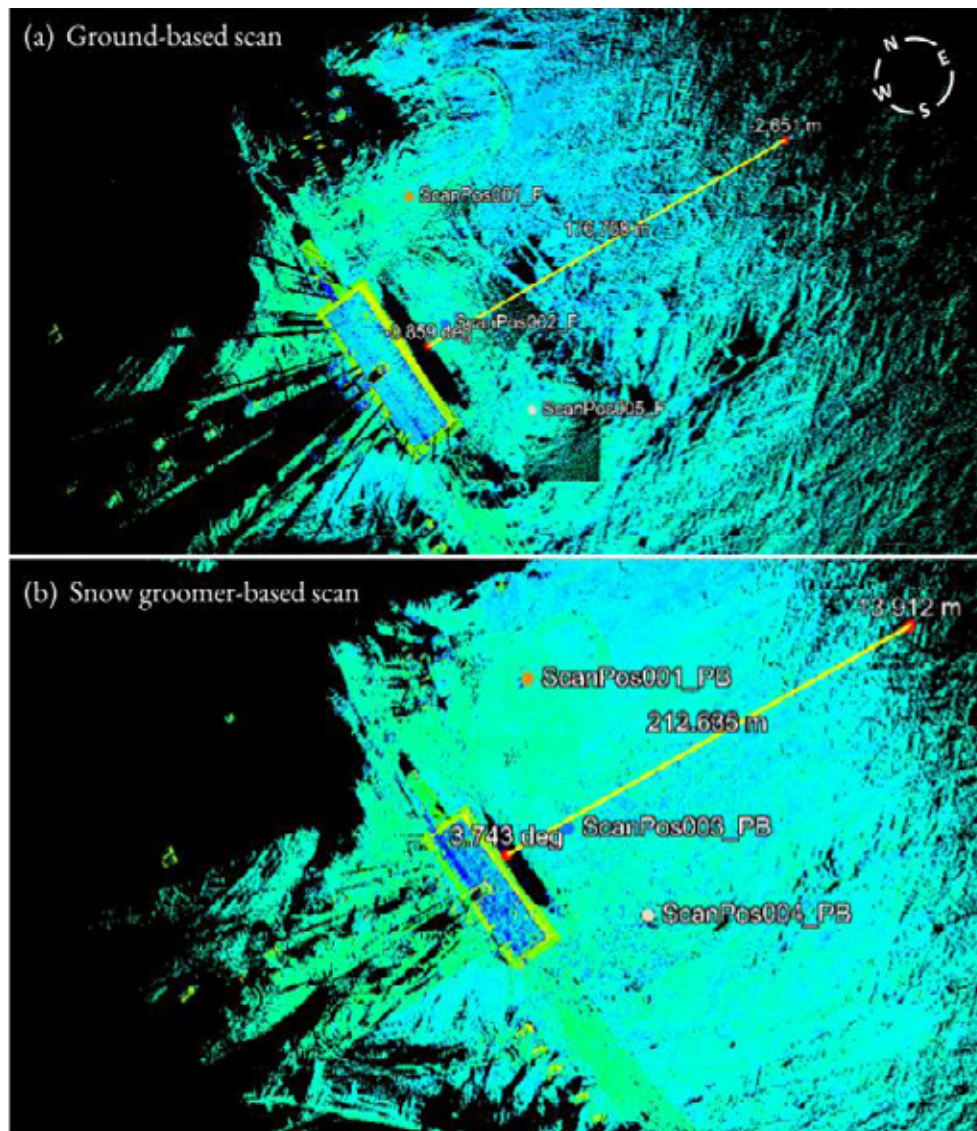
Fig. 4.22.3: Point clouds of the snow surface at the East side of Neumayer Station III. They result from scans taken from three different positions with the device placed (a) at ground height and (b) at snow groomer roof height.
