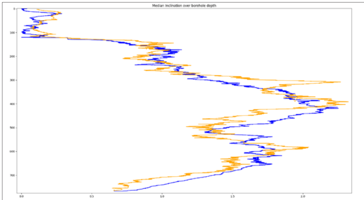
Fig. 5.1.4: Plot of the running median of the previous 200 samples @ 300ms interval over depth, blue marks the way down and orange the way up. X axis inclination in degree, Y axis depth in meter
