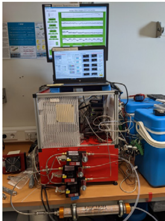
Fig. 4.29.1: Iso-Ant water vapour CRDS analyzer and instrumental setup before deinstallation in November 2022 (photo taken M. Behrens, AWI).
