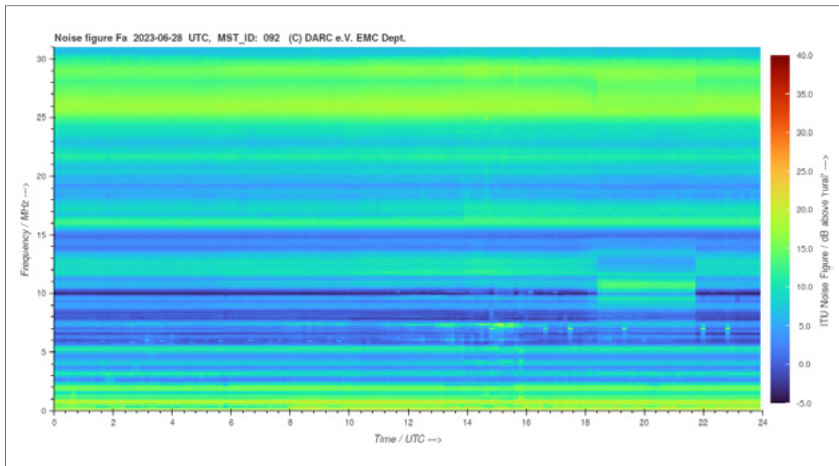
Fig. 4.23.13: Heatmap of the noise measurement at SPUSO based on the ITU class rural
