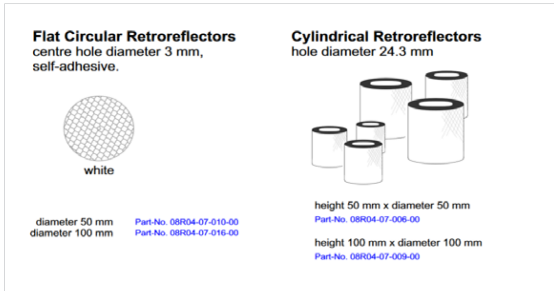
Fig. 4.22.2: Reflector targets used during field work at Neumayer Station III for local scan data registration (RIEGL, 2006). Both flat circular disk reflectors (left) and cylinder reflectors (right) were tested.
