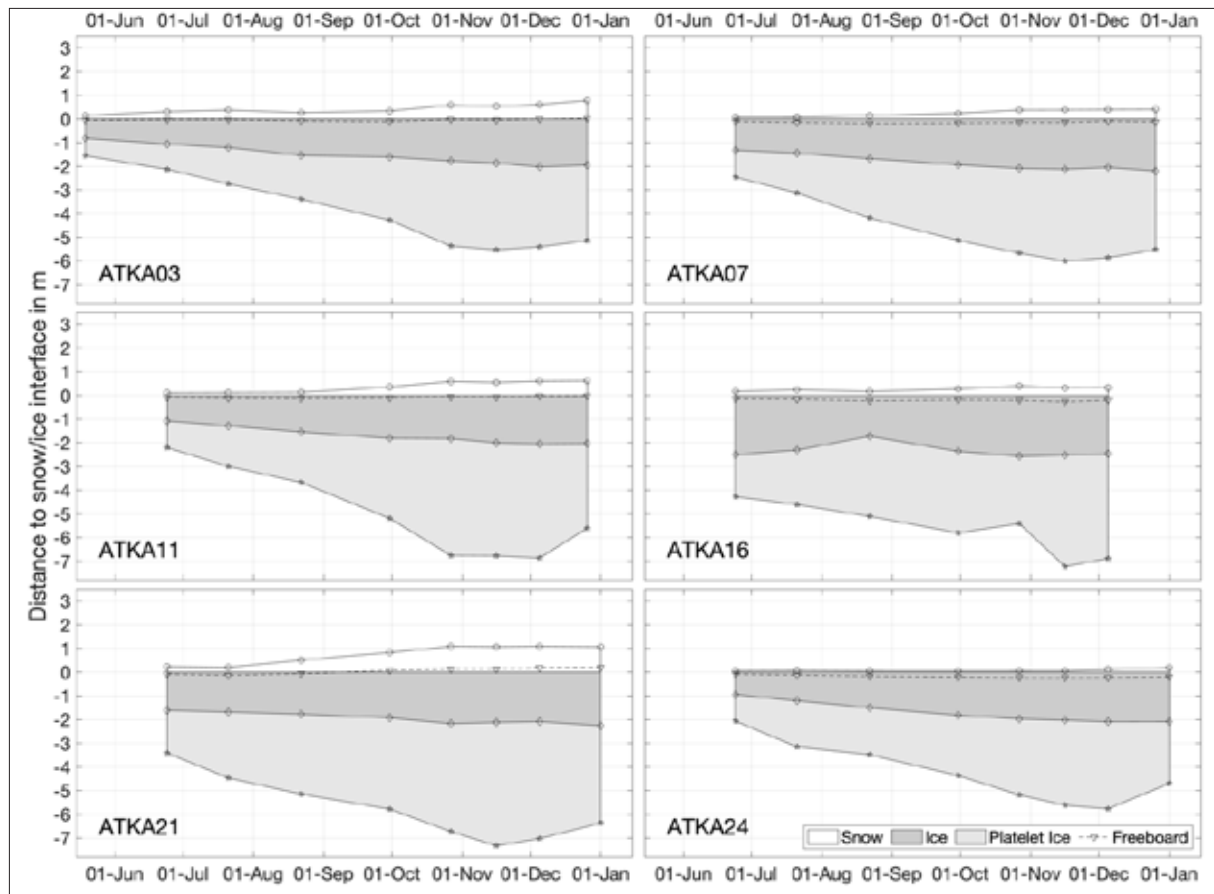
Fig. 4.6.2: Overview of all manual snow depth, sea ice and sub-ice platelet layer thickness as well as freeboard measurements for the six sampling sites along the standard AFIN transect (Fig. 4.6.1A) in 2022.
