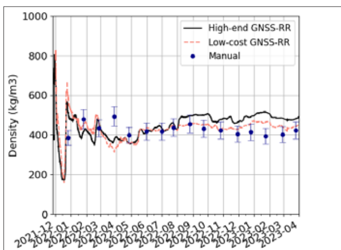
Fig. 4.13.2: GNSS-RR derived density time series from the high-end and low-cost system compared to manual observations.
