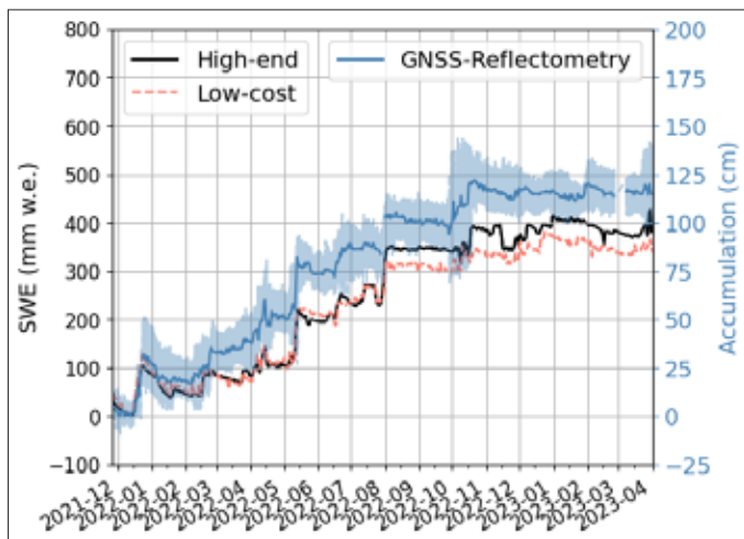
Fig. 4.13.1: Derived timeseries from GNSS reflectometry and refractometry for accumulation and SWE
