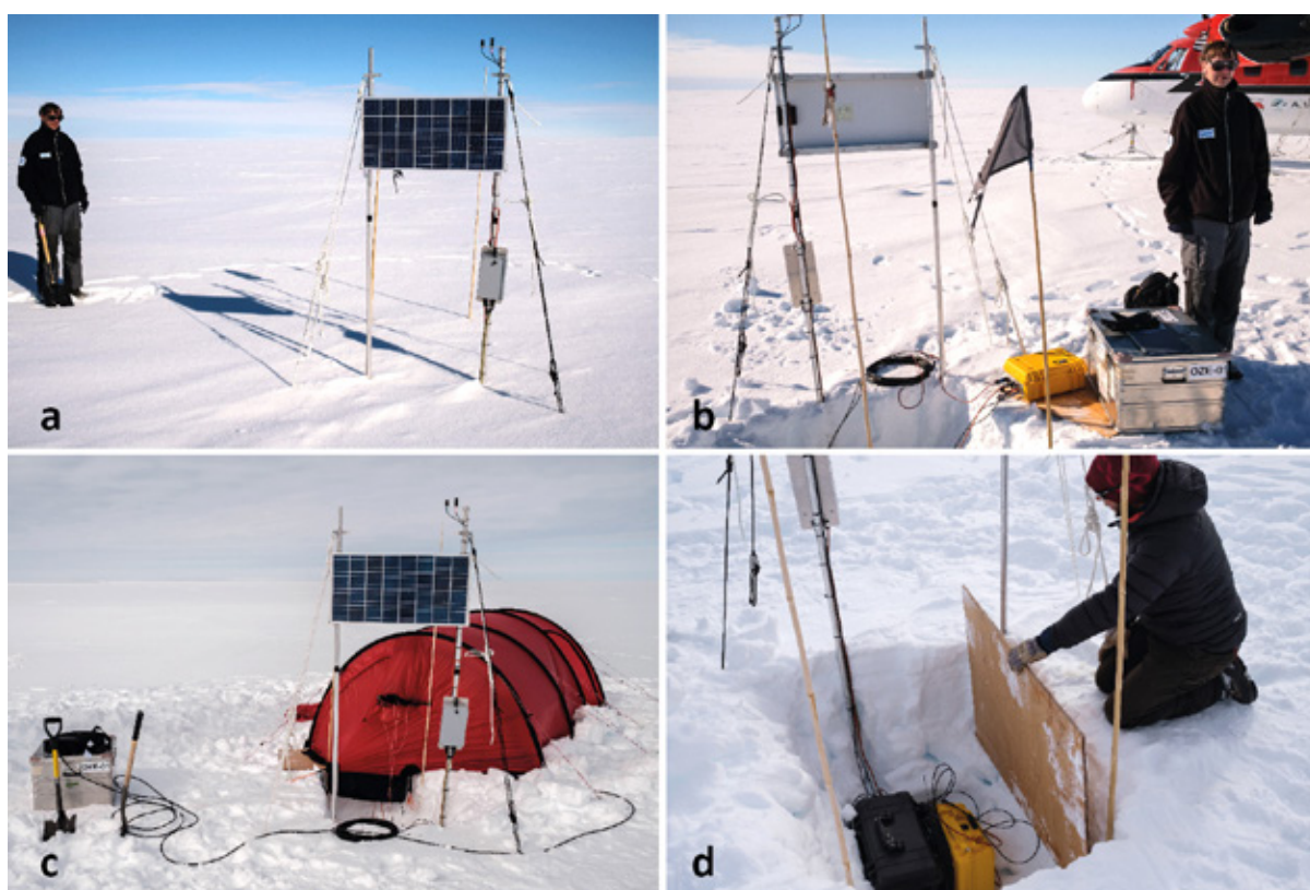
Fig. 5.3.3: Service of the oceanographic mooring at site FSE2. a) Condition at arrival; b) retrieval of the data logger to fix the firmware issue; c) data download of the SBE37IMP Microcats via the inductive modem link during an overnight stay. d) closing of lid within the snow pit after service was done.
