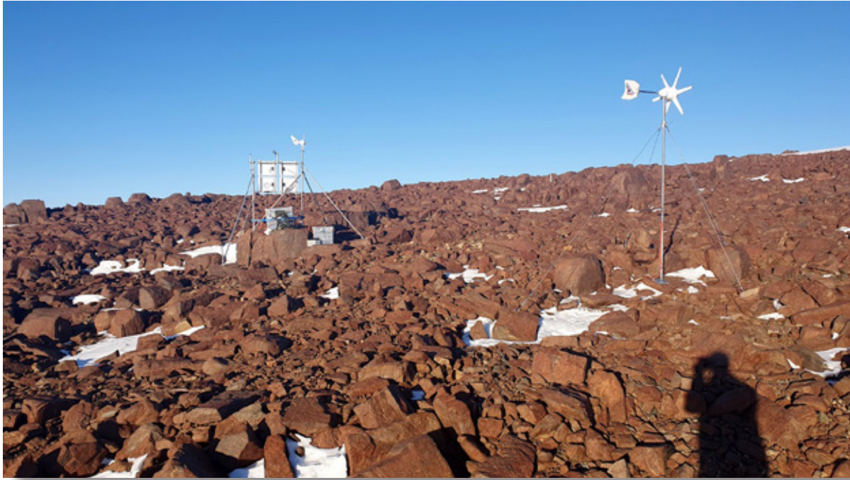
Fig. 4.25.2: Setup of the permanent GNSS station FOP1 at Forstefjell.
