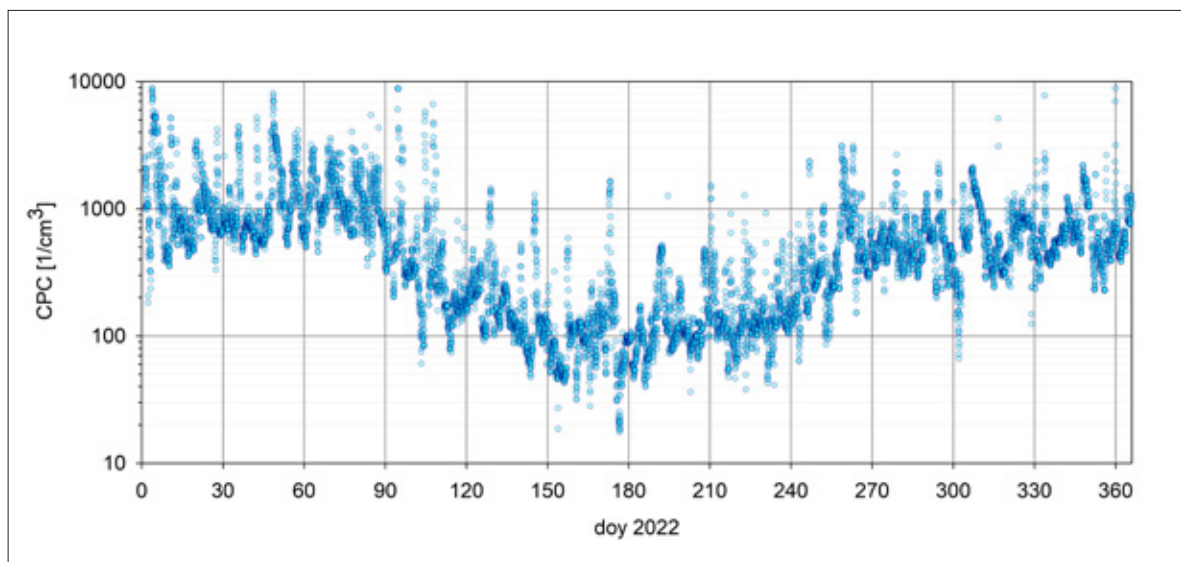
Fig. 4.2.1: Time series of the CP concentrations for the year 2022 measured with a TSI type CPC 3775 condensation particle counter. This instrument detects all particles above the lower 50 % cut-off diameter of 4 nm (day 2022 = day of the year 2022).
