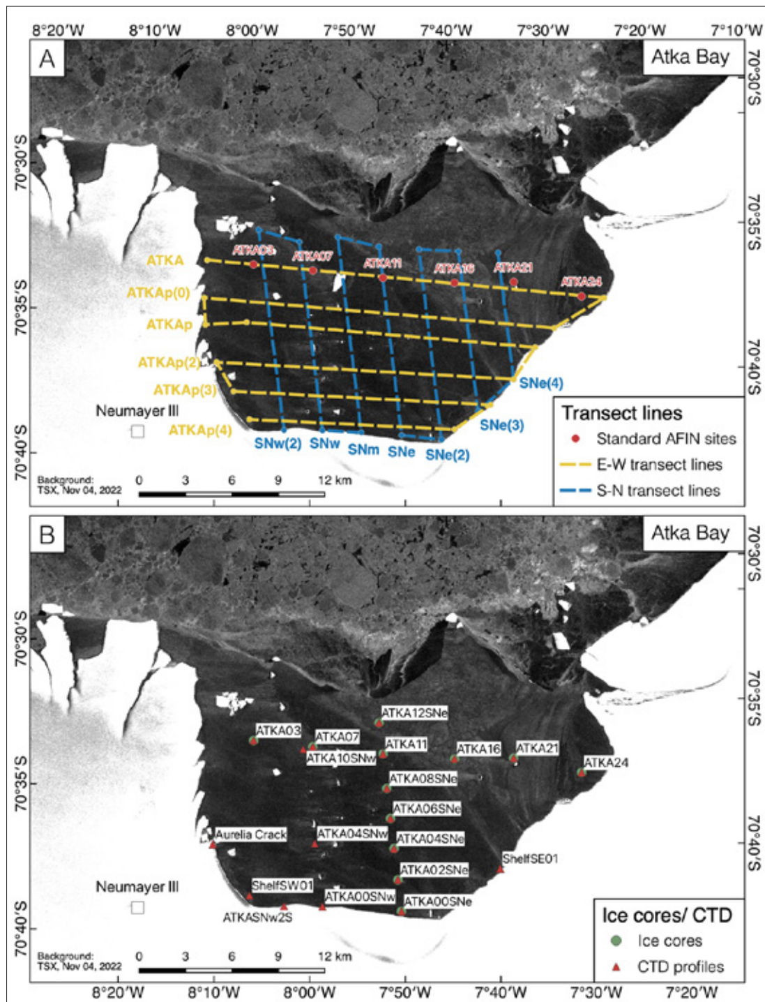
Fig. 4.6.1: Overview on all transects and measurement sites in Atka Bay for the season 2022. In panel (A), ATKA03-24 denote the routine measurement sites of AFIN. Numbers (03-24) state the distance to the western shelf ice edge. In addition, surveyed east-to-west (E-W, yellow) and south-to-north (S-N, blue) transect lines with the GEM-2 device are noted. Panel (B) shows all sampling sites for drilled ice cores (green circles) and CTD profiles (red triangles). Background: TerraSAR-X image recorded on 4 November 2022.
