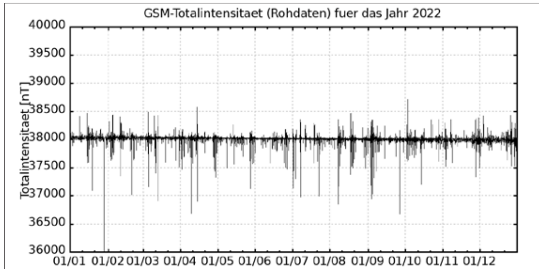
Fig. 4.3.3: Total Intensity of the geomagnetic field at Neumayer Station III, recorded by the Overhauser GSM-19.
