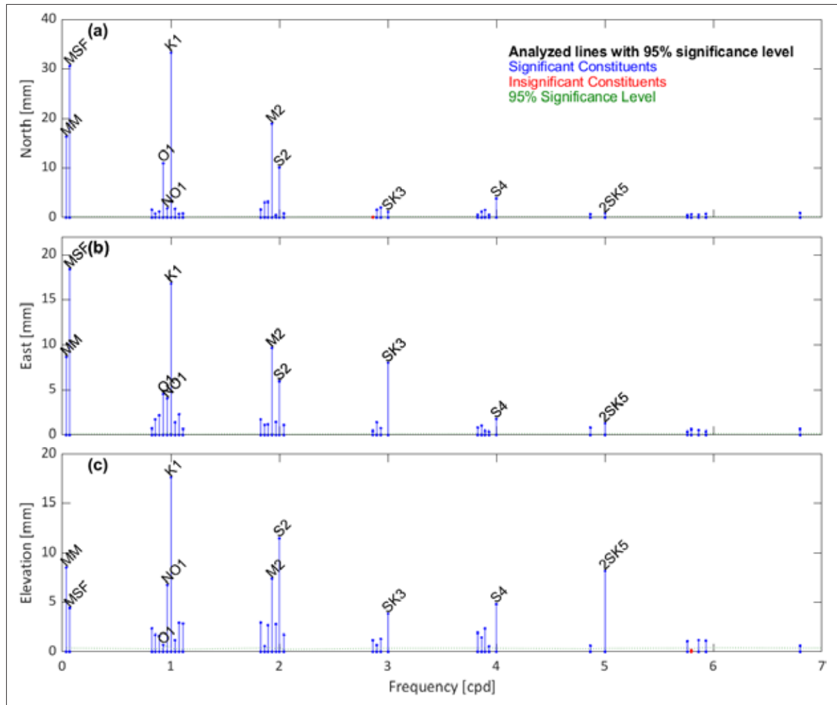
Fig. 4.14.3: Amplitudes of the tidal ice movement at GPS02 for (a) the north, (b) the east and (c) the high component
