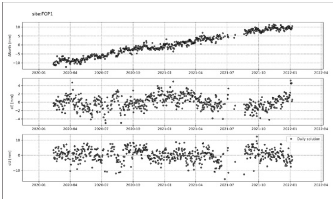
Fig. 4.25.6: Preliminary processing of the GNSS data observed at the permanent site Forstefjell (FOP1) from 02/2020 to 01/2022, resulting time series for the coordinate components north (top), east (middle) and up (bottom panel).
