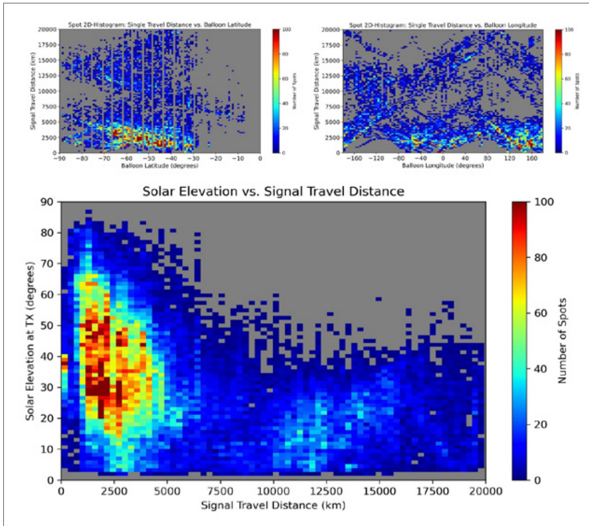
Fig. 4.21.5: Top: Spot 2D-Histogram of signal travel distance vs. balloon latitudes (left) and longitudes (right). Bottom: Spot 2D-Histogram of solar elevation during balloon transmission vs. signal travel distance. For each plot, reds indicate more spots.
