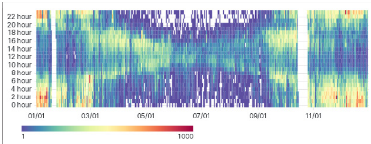
Fig. 4.23.8: Transmitted and world wide reported spots over the year 2022
