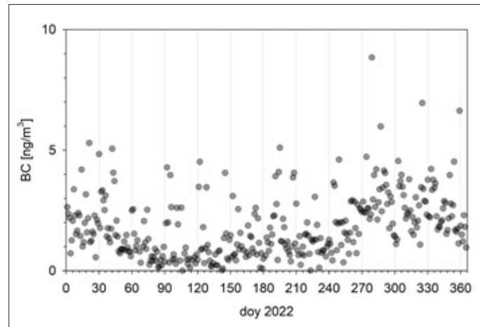
Fig. 4.2.3: Time series of BC concentrations measured at Neumayer Station III with a so-called Multi Angle Absorption Photometer (MAAP, Thermo). Note that the BC data shown were rigorously cleaned from local contamination, which is feasible considering wind direction and particle concentrations. Here, the presented data are daily medians based on the originally data taken in 1-minute intervals (see: https://doi.pangaea.de/10.1594/PANGAEA.956056 ).
