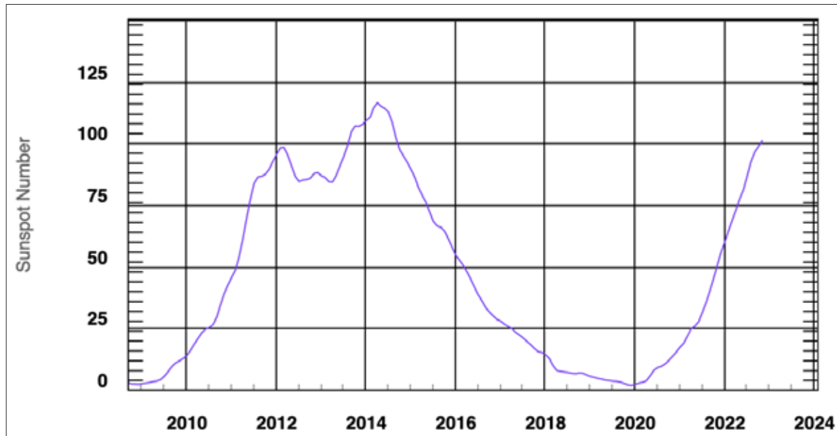
Figure 4.23.2: Development of solar activity for the previous and current cycle (source: NOAA SWPC https://www.swpc.noaa.gov ).
