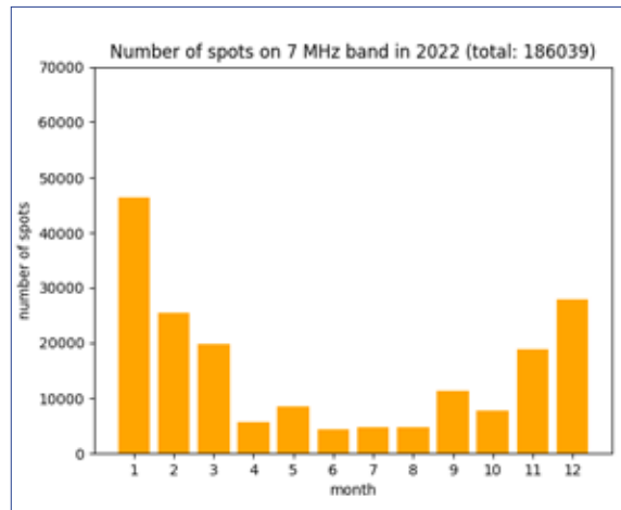
Fig. 4.23.6: Number of spots on 7 MHz throughout 2022 (October count reduced by a 10-day downtime of the transmitter)
