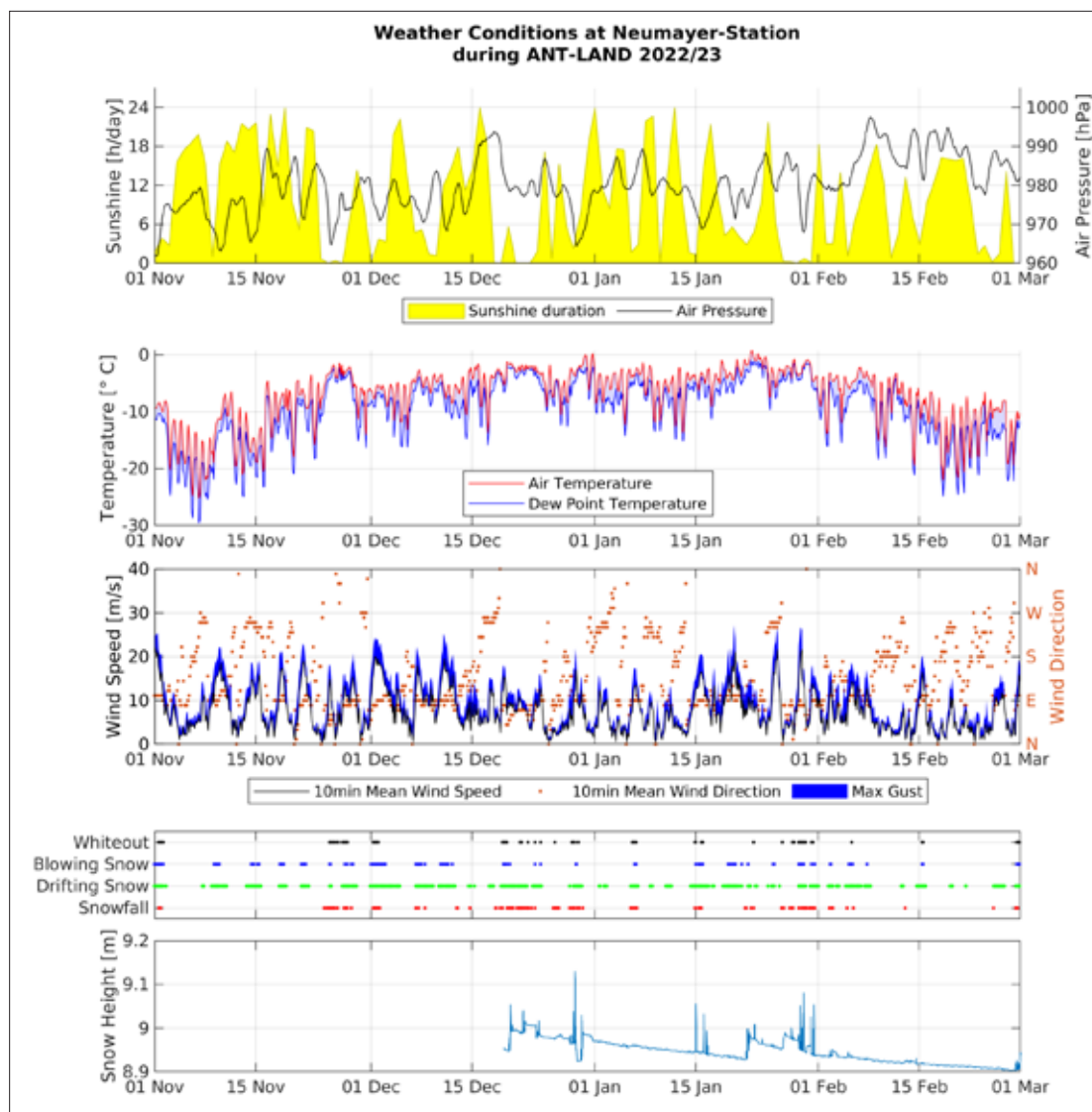
Fig. 2.1: Weather conditions at Neumayer Station III during ANT-Land 2022/23
