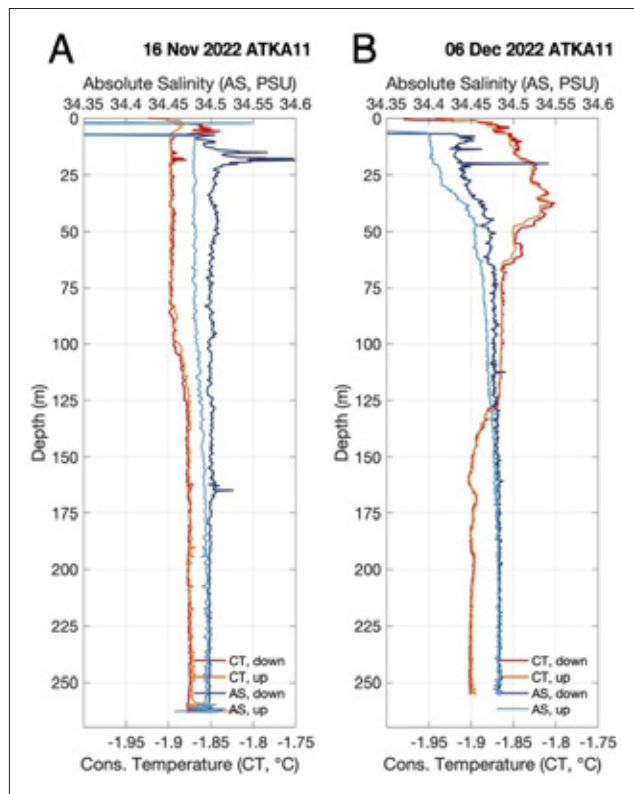
Fig. 4.6.6: Profiles of absolute salinity and conservative temperature for the down- and upcast respectively (dark/light blue, red/orange) at ATKA11 on (A) 16 November and (B) 6 December 2022.
