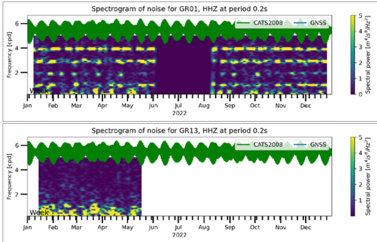
Fig. 4.14.2: Spectrograms of seismic noise levels calculated from probabilistic power spectral densities (PPSD, McNamara and Buland, 2004; Fromm et al., 2023) reveal tidal signals with 1-4 cpd (cycles per day) at station GR01 which is close to the grounding line, whereas station GR13, approximately 20 km away from the grounding line, is not affected by tidal forcing.
