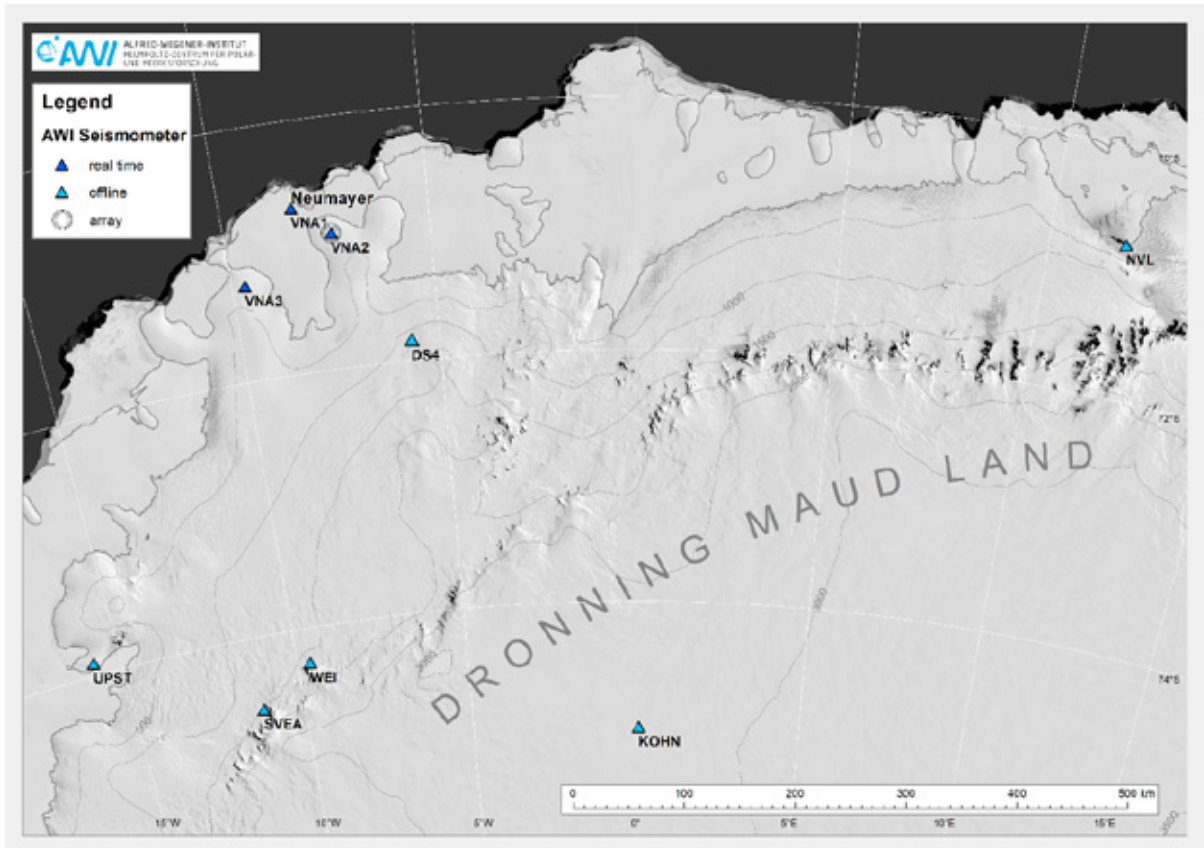
Fig. 4.3.1: Map showing the active seismometer stations in Dronning Maud Land of the AWI network during 2022
