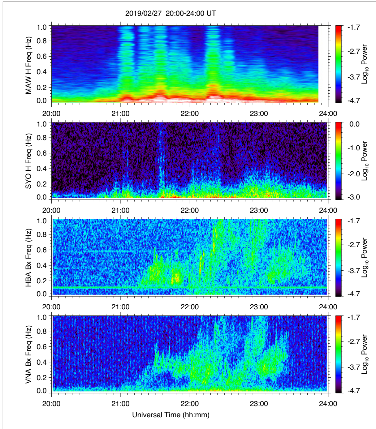
Fig. 4.16.1: Geomagnetic spectrograms on 27 February 2019 using data from Antarctic stations Mawson (MAW), Syowa (SYO), Halley Research Station (HBA), and Neumayer Station III (VNA). Intervals of Pulsations of Diminishing Periods (IPDPs), a subtype of EMIC waves, are observed at HBA and VNA (-62.2 and -60.6 CGM lat; Salzano et al, 2022). Near-simultaneous Pi1Bs are observed at MAW and SYO (-70.4 and -66.5 CGM lat).
