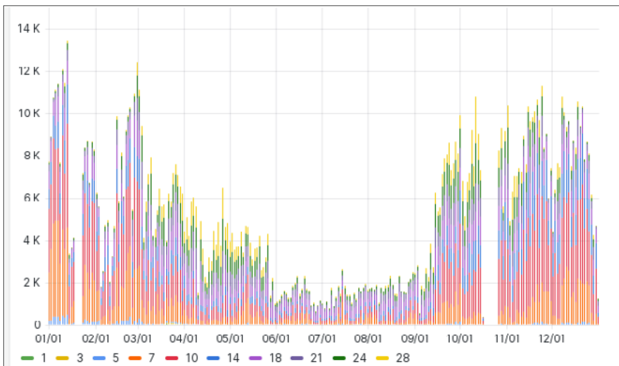
Fig. 4.23.1: Worldwide reported spots from the transmitter during 2022 per day and bands
