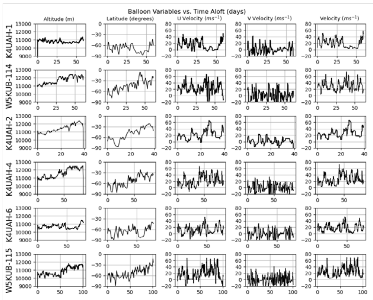
Fig. 4.21.3: Preliminary balloon data plotted vs. days after launch
