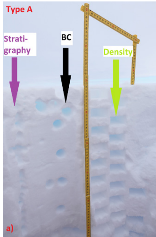
Fig. 4.19.2: Photographic documentation of a snow pit (Type A) with markers for BC sampling, density cutter and stratigraphy measurements
