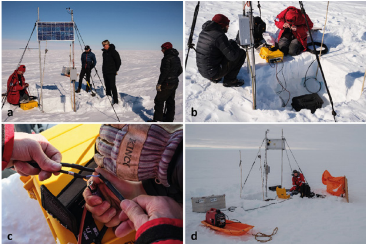
Fig. 5.3.1: Service of the oceanographic mooring at site FSW1. a-c) Retrieval of the data logger to fix the broken mooring cable; d) data download of the SBE37IMP Microcats via the inductive modem link.
