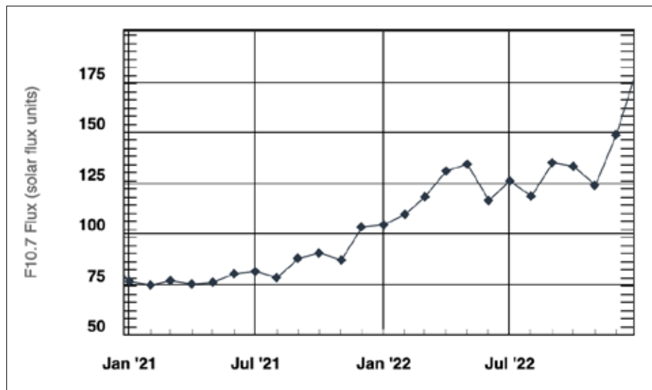
Fig. 4.23.7: Development of solar activity (as expressed by monthly averages of F10.7 cm flux) during 2021 and 2022 (source: NOAA SWPC https://www.swpc.noaa.gov )
