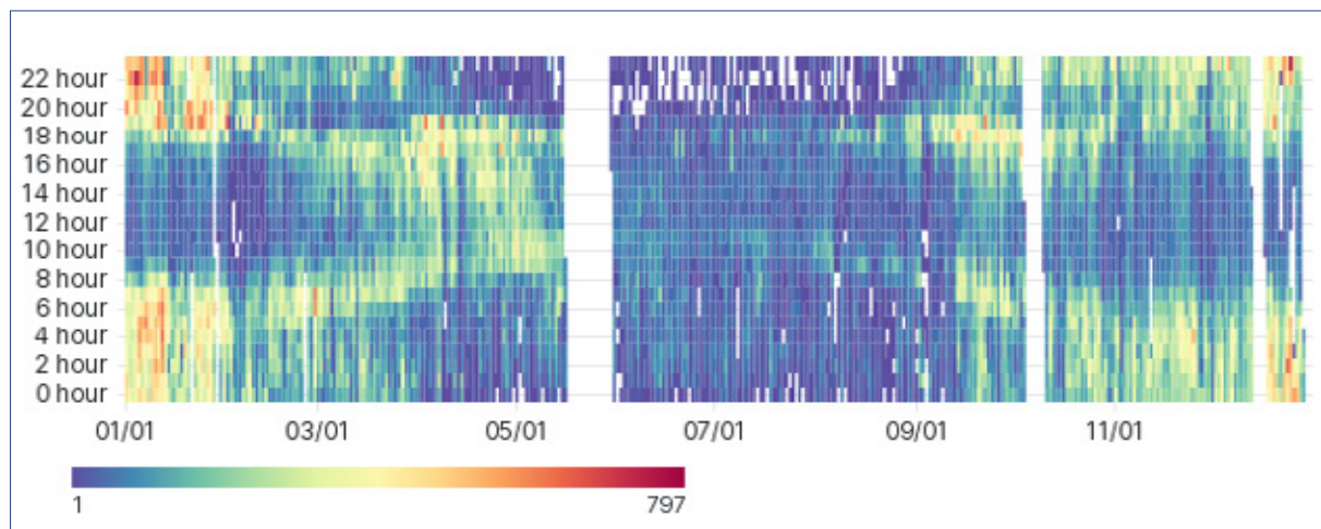
Fig. 4.23.10: At SPUSO received worldwide transmitted spots over the year 2022 on the smaller loop antenna.
