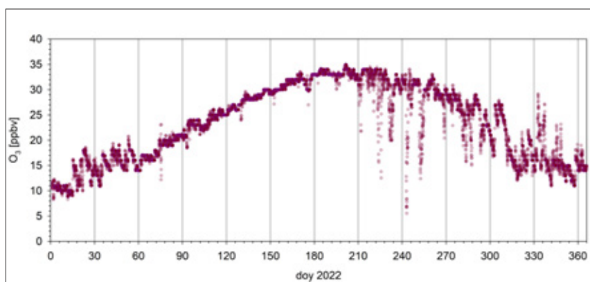
Fig. 4.2.5: Measured surface ozone time series (ppbv: parts per billion by volume) at Neumayer Station III for the year 2022 (measured with an UV photometer O3 41M, Environnement). Presented data are one-hour averages based on originally one-minute data.
