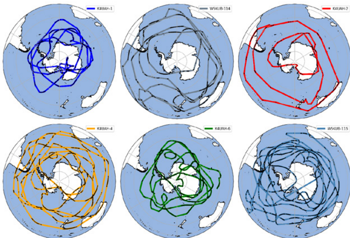
Fig. 4.21.2: Maps showing the trajectories of the six WSPR balloon flights. The black dots over the colored flight trajectories show points when the balloon transmitted a data point.
