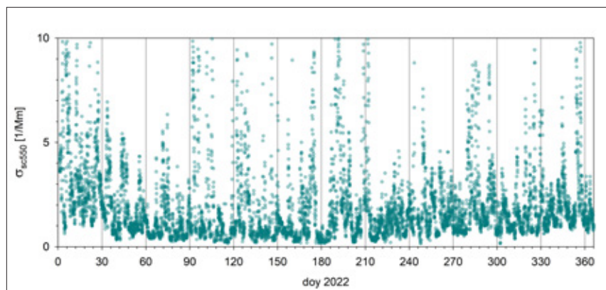
Fig. 4.2.4: Time series of aerosol scattering coefficient at 550 nm, s_{sp}(550) , measured with an integrating nephelometer (TSI Model 3563). Presented data are one-hour averages based on originally one-minute data.
