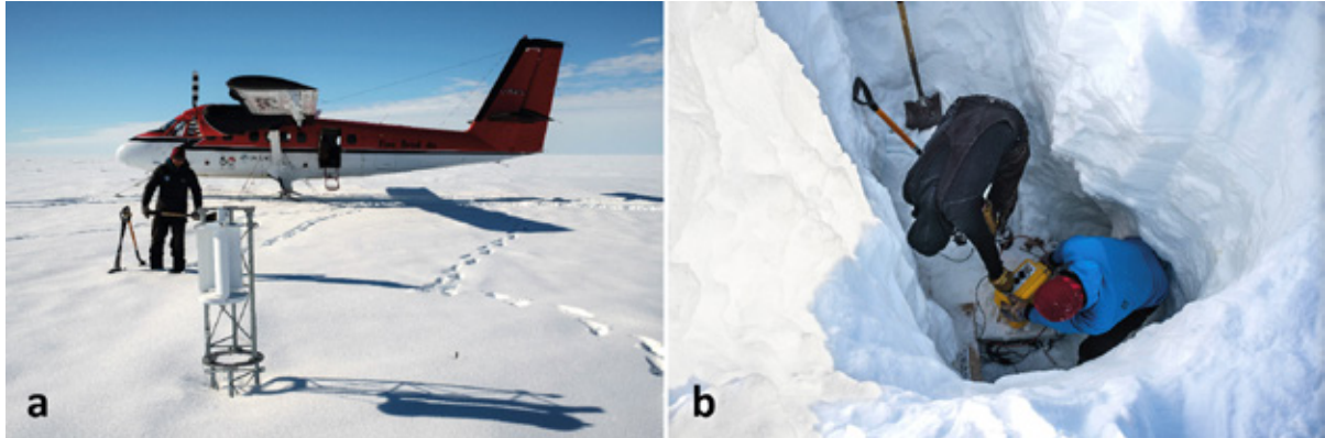
Fig. 5.3.4: Retrieval of equipment at site SFG_East. a) The wind generator still sticking out; b) the equipment was buried beneath 3-4 m snow, was dug out manually.
