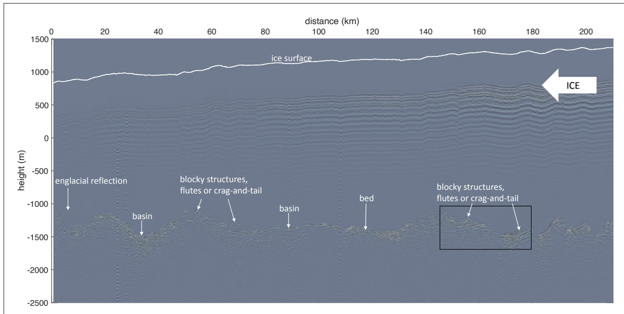
Fig. 5.2.3: Throughout the 208 km profile we see blocky structures identified elsewhere as flutes or ‘crag-and-tail’ features. We see englacial reflections some 200 m above the bed on the far-left side, fading out and reappearing at km 160–180. We see several basins, a large one, 20 km long, 110 m deep, at km 90. The inset box, also showing these blocky structures, has been surveyed before by Muto et al. (2019).
