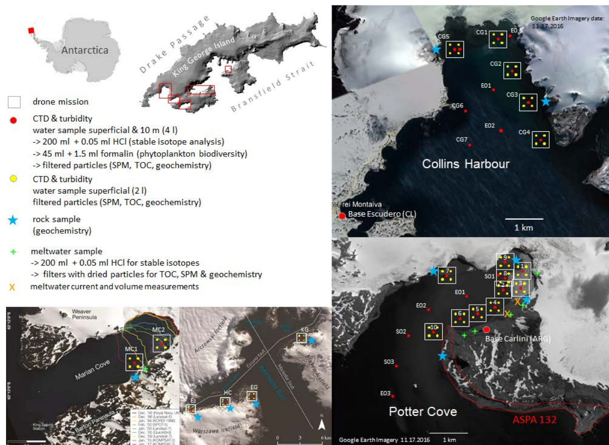
Fig. 5.5.1: ANT-Land-SIGMA-I study areas in Maxwell and Admiralty Bay, King George Island. Exemplary data collection in front of Polar Friendship Glacier at Collins Harbour and Fourcade Glacier at Potter Cove.
