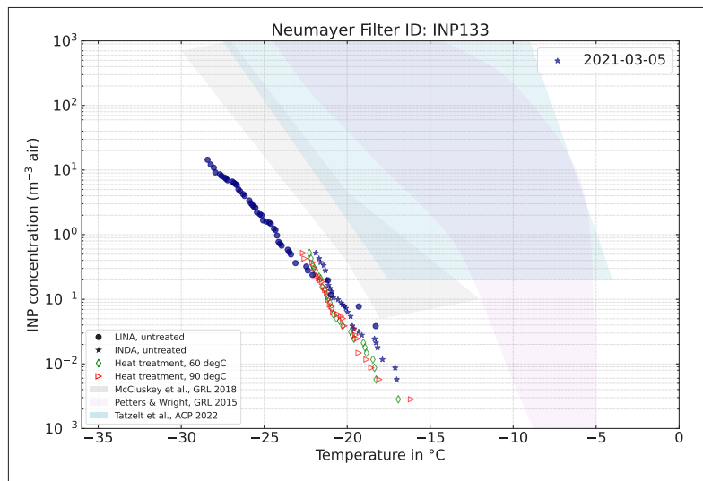
Fig. 4.18.1: Example of INP freezing spectra (blue area: Tatzelt et al., 2022, grey area: McCluskey et al., 2018); sample period was two weeks, the date gives the start day of the sampling period. Each filter is analysed with two different freezing arrays covering by this a wider freezing range. Besides the samples are heated to 60°C and 90°C to gain information on the fraction of heat-labile ice active protein.
