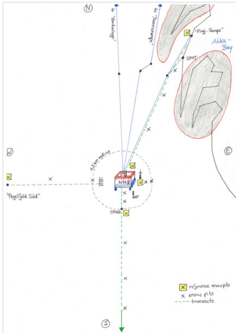
Fig. 4.19.1: Sketch of the BC transects around Neumayer Station III
