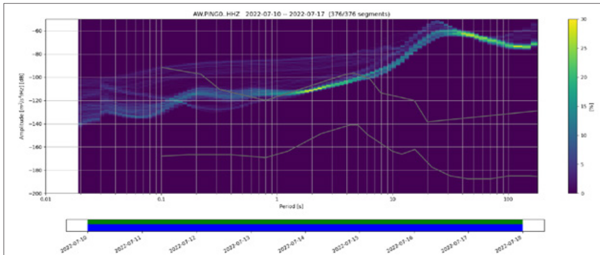
Fig. 4.17.2: Periodogram of two components of the seismometer.
