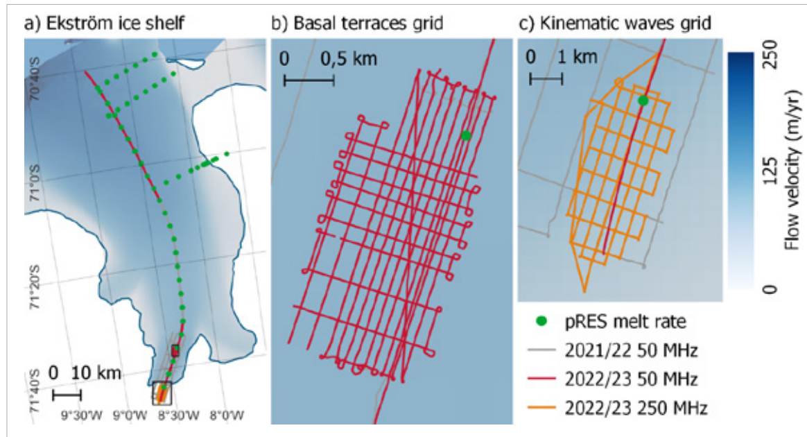
Fig. 4.15.1: Location of ground-penetrating radar transects (lines) and static radar measurement points (circles). Transects from 2021/22 (grey) were revisited with the 50 MHz radar to map temporal changes (red). 250 MHz data were collected to map kinematic waves in the firm (orange).
