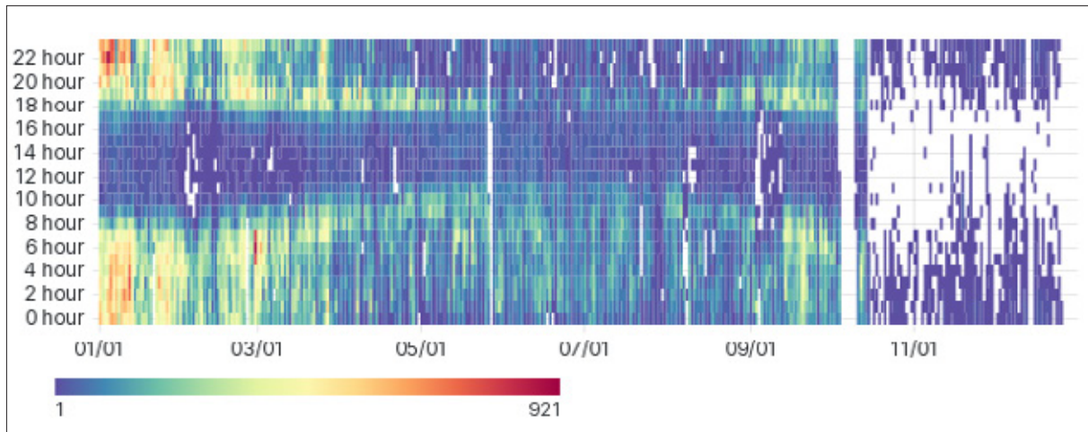
Fig. 4.23.9: At SPUSO received worldwide transmitted spots over the year 2022 on the larger loop antenna.
