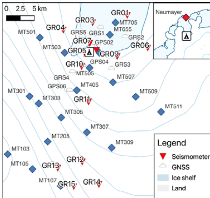
Fig. 4.14.1: Positions of seismological stations (GR01-GR15), GNSS Stations (GPS1-GPS7, GRS0-5) and MT stations (MT103-MT705)
