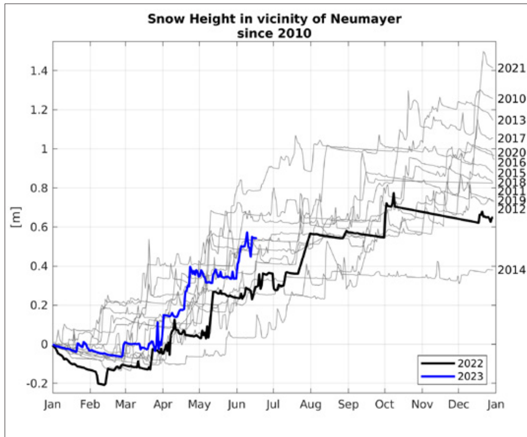
Fig. 2.2: Snow height measured in the vicinity of Neumayer Station III with sensor Jenoptik SHM30 from 2010 until December 2022, and with its successor Lufft SHM31 from December 2022 until June 2023. Most recent data is shown in blue, accumulation of 2022 in black, earlier years in grey.
