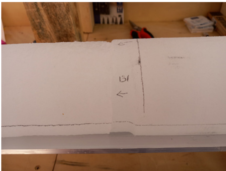
Fig. 5.1.2: Smooth fit of the core from the pilot hole to the deep core
