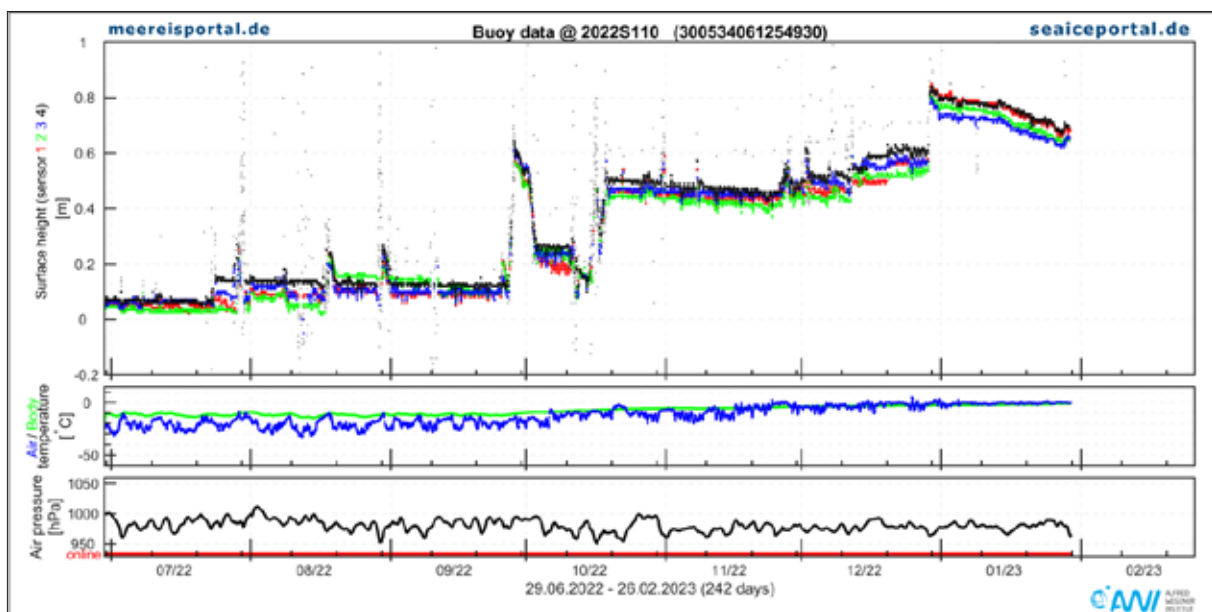
Fig. 4.6.4: Time series of snow accumulation along with the respective meteorological conditions for Snow Buoy 2022S110, deployed on 29 June 2022 at ATKA11 (Fig. 4.6.1, data.meereisportal.de).
