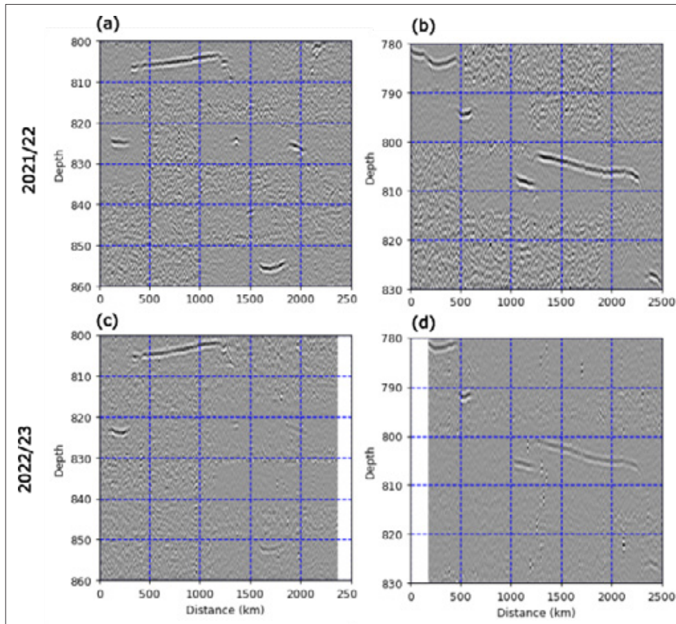
Fig. 4.15.3: Snapshots for basal terracing observed at the ice-ocean interface at Ekström Ice Shelf. Profiles (a,b) were collected in 2021/22 whereas profiles (c,d) stem from repeat visits in 2022/23. The signal stability is remarkable, and such time series can be used to decipher ocean-induced melting on small spatial scales.
