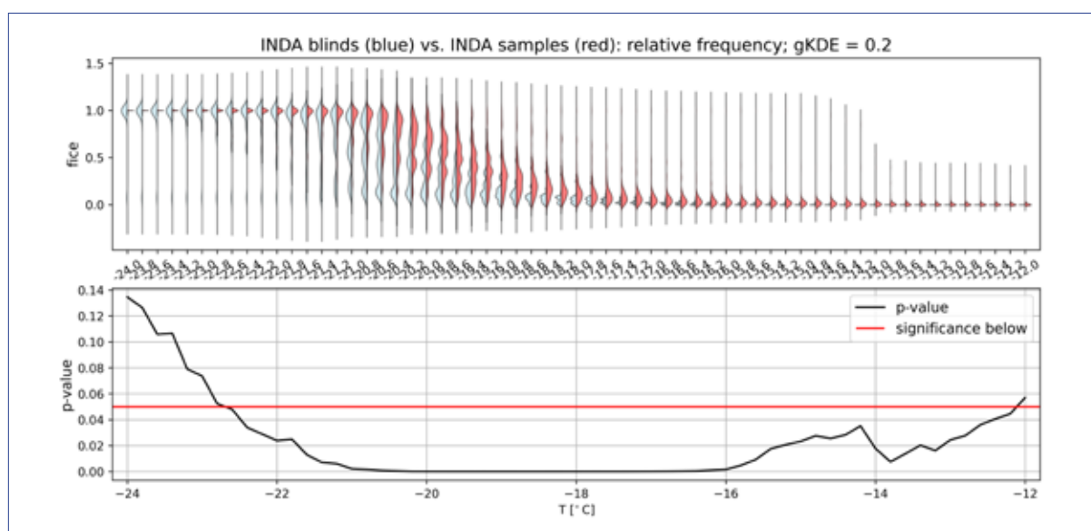
Fig. 4.18.2: Violin plot of ice fraction spectra including all currently analysed samples (red: samples, blue: field blanks). The sampling period ranges from February 2019 until December 2021 with weekly to biweekly resolution.
