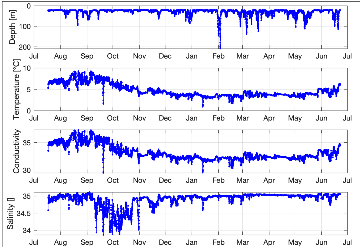
Fig. 4.4: Timeseries at 22m depth at mooring F4-S-8 over the deployment period, showing (top to bottom) depth (m), temperature ( ^{\circ}\text{C} ), conductivity, and salinity.
