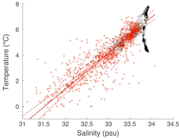
Figure 4. Underway surface ocean salinity versus temperature. Values for the inner core correspond to the red circles. The regression (based only on inner core data) of T on S and S on T are indicated by the dashed red lines. The geometric mean of these two regressions is shown by the red solid line. Values from the transitional domain are indicated by the grey symbols (asterisks: 18 January 3h00 to 16h00; crosses: 19 January 12h00 to 22h30). Values for unperturbed water masses are shown by the black symbols (asterisks: 17 January 12h00 to 18 January 3h00; crosses: 19 January 22h30 to 20 January 12h00).
