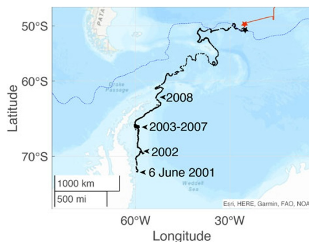
Figure 2. Track of iceberg A43f (black line) determined by satellite scatterometer, from 6 June 2001 to 21 January 2009 (data source: Budge and Long (2018), and https://www.scp.byu.edu/data/iceberg/ ). The black star indicates the last recorded position for A43f on 21 January 2009. The red line shows the track of Polarstern until station 102 on 18 January 2009 (indicated by the red star). The dashed blue line marks the (climatological) position of the APF (Orsi and others, 1995). Black arrows show relevant positions and periods of A43f drift trajectory.
