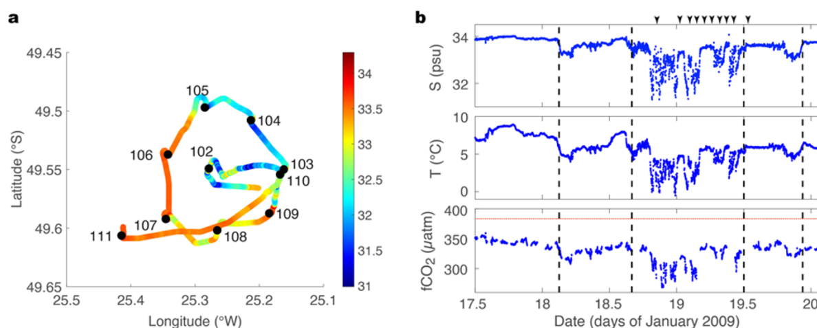
Figure 3. a, Location of CTD stations (102–111) between 18 and 19 January 2009 (black circles) and underway salinity (colored dots) from the bow thermosalinograph of Polarstern . b, Time series (blue lines) of salinity S (upper panel), temperature T (middle panel) and surface ocean f\text{CO}_2 (lower panel) from the ship's intake at \sim 11 m depth. The atmospheric f\text{CO}_2 is also indicated by the red dotted line in the lower panel. The position of CTD-rosette deployments (stations) is indicated by the black arrows in the upper panel (from left to right stations 102–111). Boundaries of the domains (see text for further details) are indicated by black vertical dotted lines.
