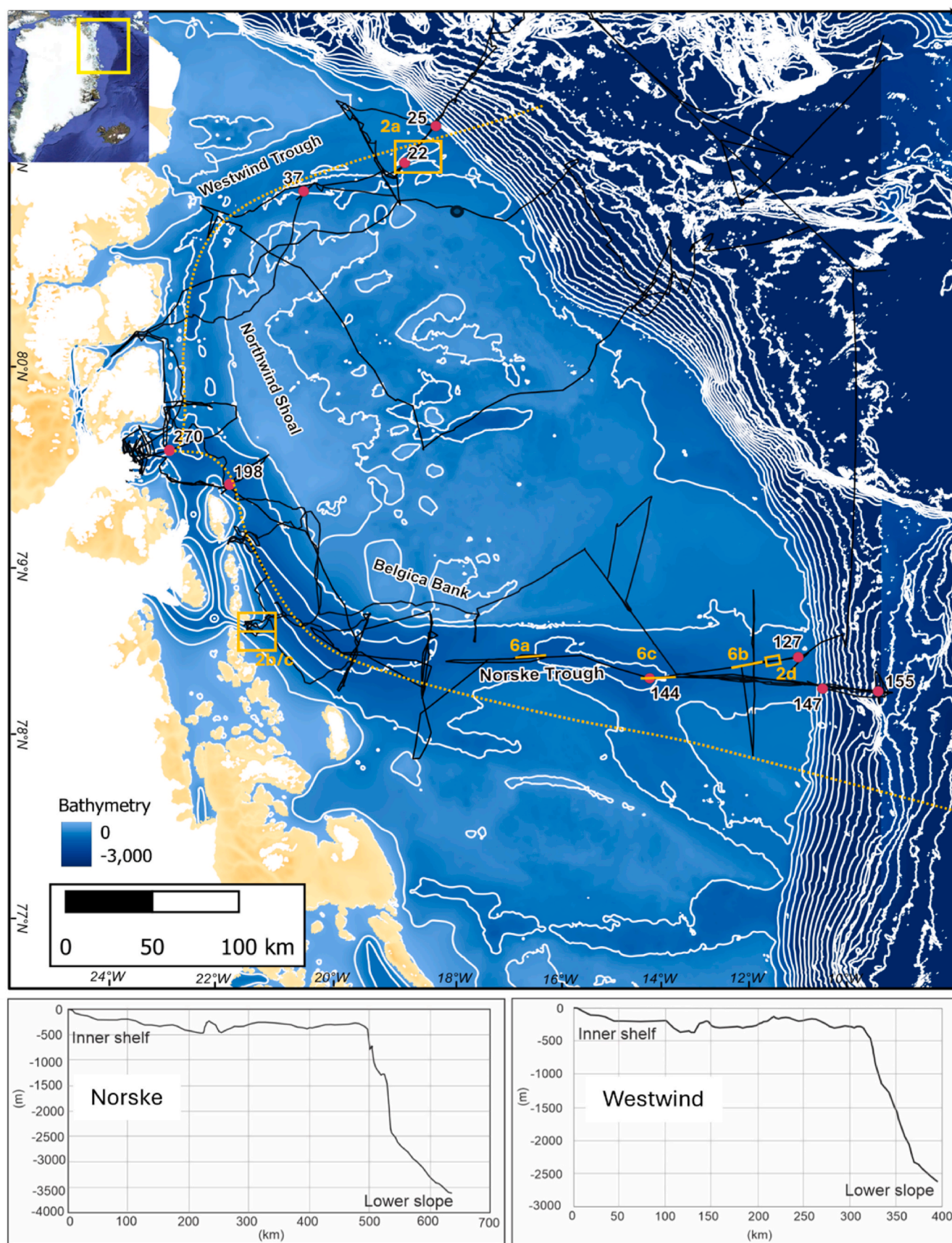
Fig. 1. Bathymetry of the continental margin adjoining NE Greenland, ship tracks along which geophysical data were collected (black lines) and locations of cores and figures referred to in text. Note Westwind Trough and Norske Trough are separated by the shallow areas of Belgica Bank and Northwind Shoal. Also shown in lower panels are topographic profiles along Norske and Westwind troughs extending from the continental slope to the inner shelf (marked as orange dotted lines in plan view). (For interpretation of the references to colour in this figure legend, the reader is referred to the Web version of this article.)
