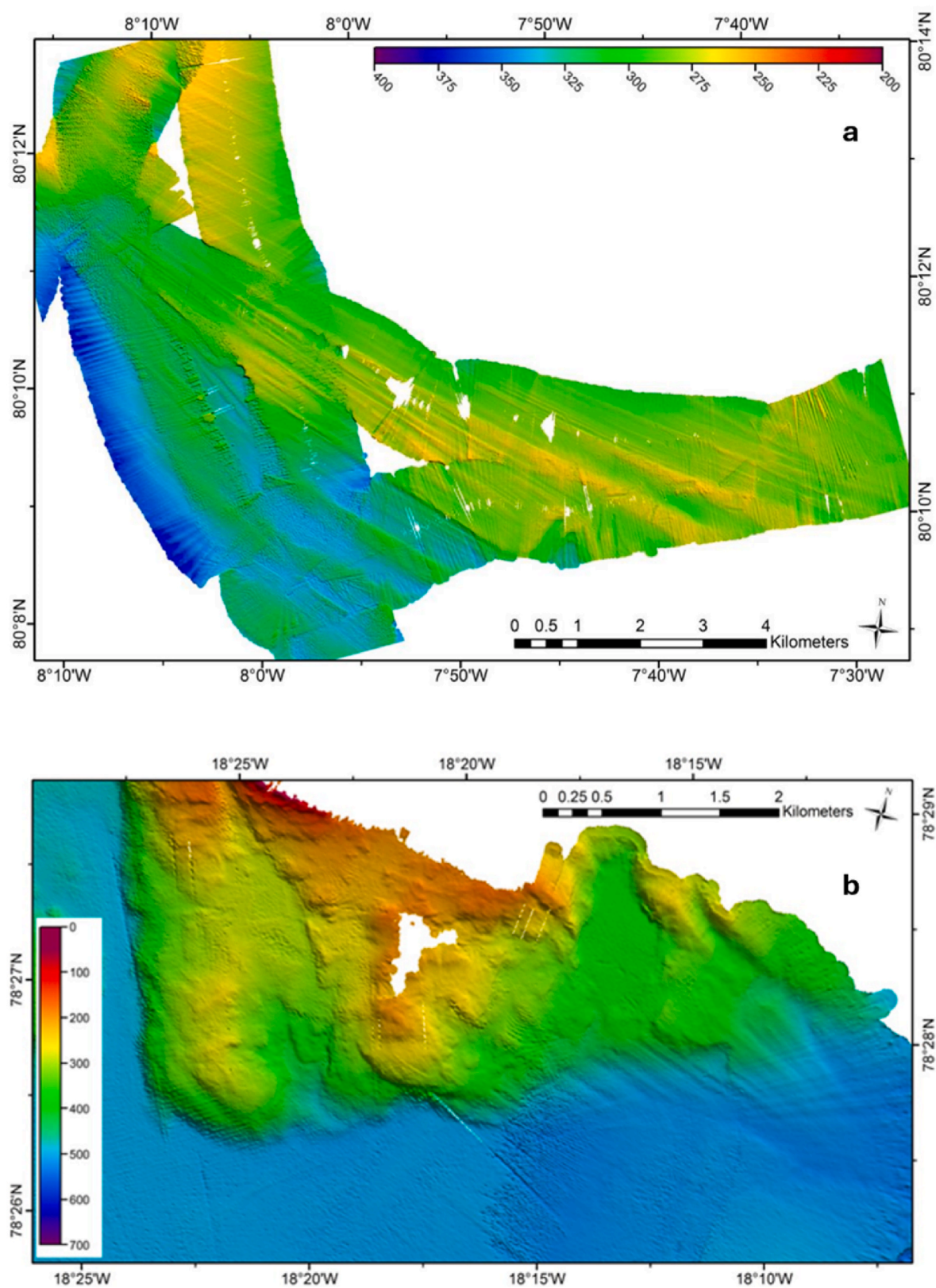
Fig. 2. Multibeam swath bathymetric images of streamlined landforms and ploughmarks on the sea floor of Westwind and Norske troughs. (a) Mega-scale glacial lineations from outer Westwind Trough; (b) and (c) Examples of streamlined seafloor bedforms Norske Trough; (d) Elongate rectilinear scours and ploughmarks incised into the seafloor of outer Norske Trough.
