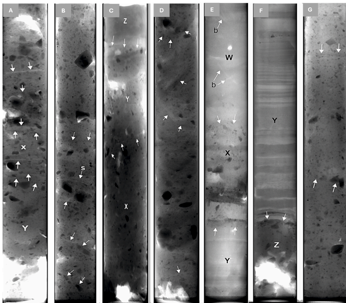
Fig. 5. X-radiographs of core lithofacies from Westwind and Norske troughs. (A) Core PS109-25, 168.5–268 cm depth. The lowermost 42 cm of the core comprises a massive, matrix-supported, clast-rich diamicton ('Y'). This is overlain gradationally by stratified, clast-rich, matrix-supported diamicton. Stratification (arrowed) is imparted by textural variations in the matrix and by the presence of laminations of mud and sandy mud. Contacts with the surrounding diamicton range from sharp to diffuse. (B) Core PS109-22, 65–160 cm depth. The x-radiograph shows massive, matrix-supported and clast-rich diamicton with subrounded to angular clasts dispersed in a silty clay matrix. In places there are inclined clast alignments and lineaments (arrowed) as well as very subtle stratification ('s'). (C) Core PS109-37, 56–106 cm depth. The lower 31 cm of the core comprises a massive, matrix-supported, muddy diamicton with dispersed clasts in a silty matrix ('X'). This is overlain by 12 cm of crudely stratified pebbly mud with relatively abrupt upper and lower contacts (arrowed). Note the gently inclined stratification. This stratified mud is overlain by 6 cm of clast-free massive silty and silty clay muds from 56 to 62 cm depth ('Z'). (D) Core PS100-127, 91–183 cm depth. Massive, matrix-supported diamicton with dispersed clasts. Occasional discontinuities and clast lineaments (arrowed) impart a locally developed 'swirled appearance to the sediment. (E) Core PS100-144, 46–116 cm depth. The lowermost ~118 cm of the x-radiograph shows laminated to stratified silty-clay muds with horizontal to sub-horizontal, planar parallel lamination ('Y'). These are overlain by c. 20 cm of more gritty, massive to crudely stratified muds with abundant granules, sand and occasional pebbles ('X'). The base and top (arrowed) of this more clast-rich facies are respectively sharp and gradational. The upper 29 cm of the x-radiograph is characterised by massive, silty clay ('W') with occasional zoophycos burrows ('b'). (F) Core PS100-144, 116–216 cm depth. The lowermost 26 cm of the x-radiograph comprises a massive, matrix-supported diamicton ('Z') which is overlain sharply (contact is arrowed) by 74 cm of laminated silty clay with planar, parallel, horizontal to sub-horizontal laminae. (G) Core PS109-147, 96–196 cm depth. Massive matrix-supported diamicton with dispersed clasts in a silty clay matrix. The diamicton appears largely structureless with only occasional discontinuities and clast alignments (arrowed).
