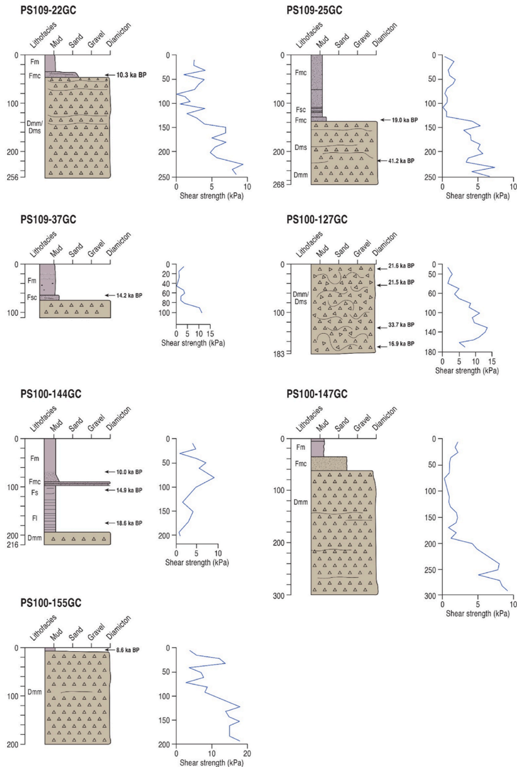
Fig. 4. Lithofacies logs, shear strength plots and radiocarbon dates of cores from Westwind Trough and Norske Trough as discussed in this paper.
