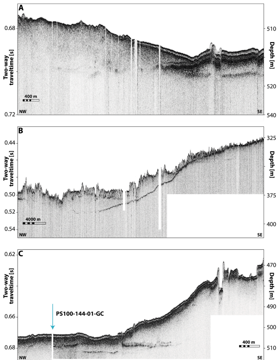
Fig. 6. Parasound records of subseafloor acoustic stratigraphy mid-outer Norske Trough. (a) GZW middle Norkse Trough. Ice flow was from left to right in the image. Note the prominent wedge shape and acoustically transparent layer which stratigraphically overlies the wedge. (b) Iceberg ploughed seafloor outer Norske Trough. (c) Parasound record of core site PS100-144.
