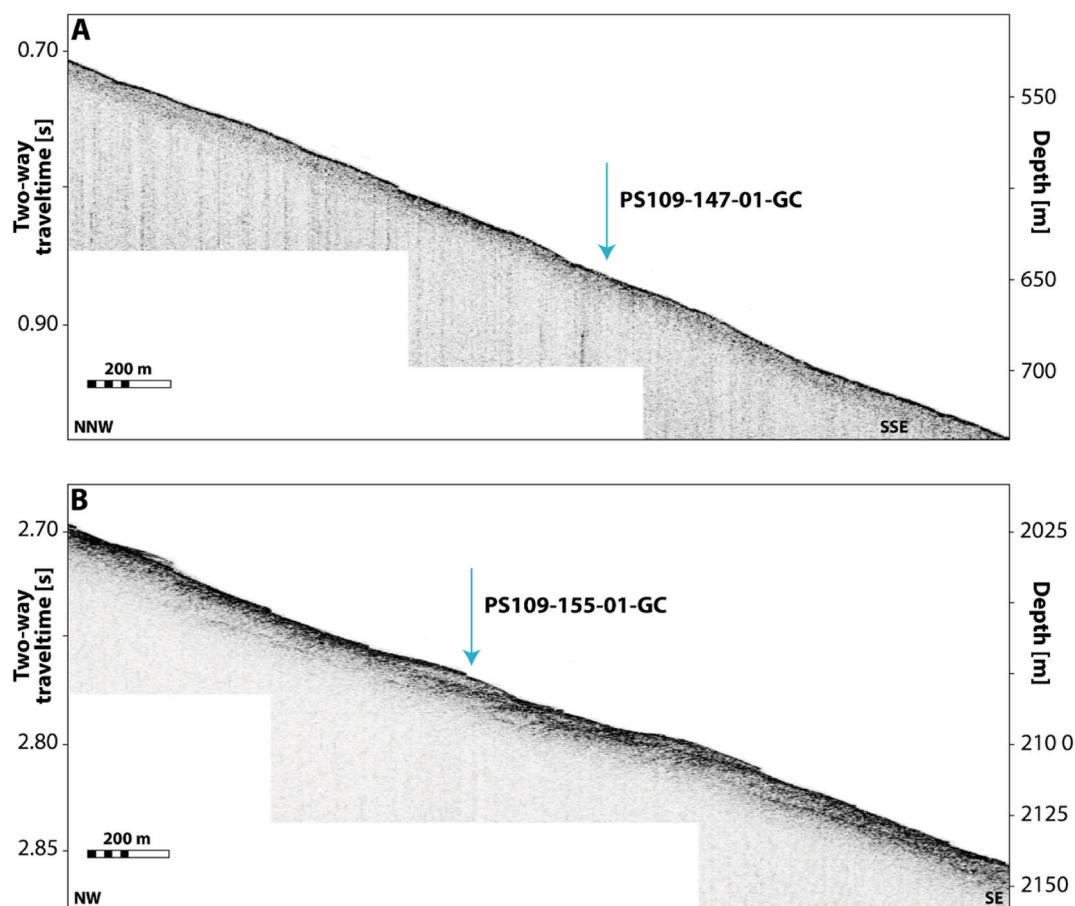
Fig. 7. Parasound records from continental slope adjoining Norske Trough. (a) Location of core PS109-147-01-GC. (b) Location of core PS109-155-01-GC. Note lenticular acoustic units interpreted as glacigenic debris flows (see text).
