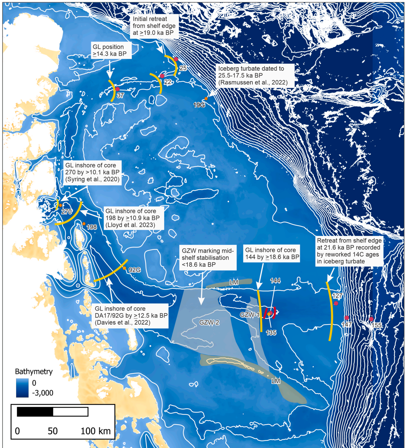
Fig. 8. Reconstruction of ice sheet extent at the LGM offshore NE Greenland and isochrones showing position of grounding line within Norske and Westwind troughs during deglaciation. ‘GZW-1’ and ‘GZW-2’ represent the positions and extents of grounding-zone wedges from the shelf and ‘LM’ represents the position of lateral moraines adjacent to Norske Trough (after Arndt et al., 2015; López-Quirós et al., 2024). The location of additional cores is also shown: core 135 (López-Quirós et al., 2024), core 198 (Lloyd et al., 2023) and core 270 (Syring et al., 2020).
