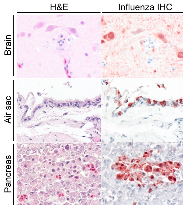
Fig. 4. Serial sections of hematoxylin and eosin staining (H&E) and influenza IHC in tissues of skuas found dead. Brain and pancreas belong to SK07, air sac belongs to SK09. Cells positive for virus antigen by immunohistochemistry (IHC) stain red in the nucleus and cytoplasm. Brain and pancreas: the center of the H&E picture contains necrotic debris (loss of architecture, hyper eosinophilia, karyorrhexis and pyknosis) close to neuronal cells and exocrine pancreatic cells that express virus antigen (visible in IHC). Air sac: virus-antigen-positive cells largely have their normal morphology, with no associated lesions.
