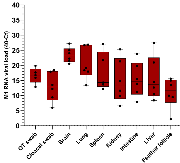
Fig. 3. Influenza A RNA viral loads in different organs of skuas. Boxplot of the relative expression of M1 viral RNA loads (40 – Cq) in different organs and tissue swabs (OT swab: oropharyngeal or tracheal swab) of skuas diagnosed with HPAI as cause of death and tested positive for M1, H5, N1 and HPAI RT-qPCRs (SK07-12). Each black dot represents a single detection.
