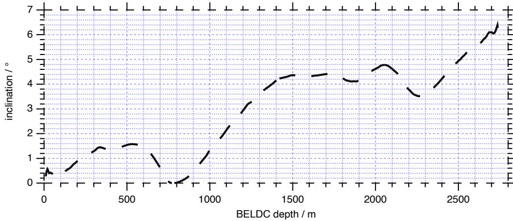
Fig. 5.1.9: Inclination of the hole recorded during the final filter run on 1 January 2025.
