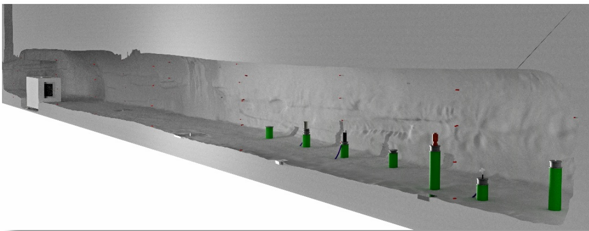
Fig. 4.3.3: 3D model of the new observatory
