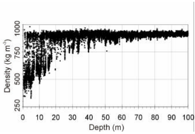
Fig. 3. Density-depth profile of the core (5 mm resolution)
