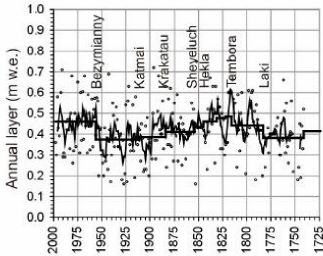
Fig. 6. The annual layer thickness AD 1725–1999 derived from d^{18}O and d oscillations and from interpolation between volcanic time-markers. Dots symbolise thickness of a single year, black curve – 5 year running mean and step line – mean annual layer thickness between presumed volcanic eruptions.
