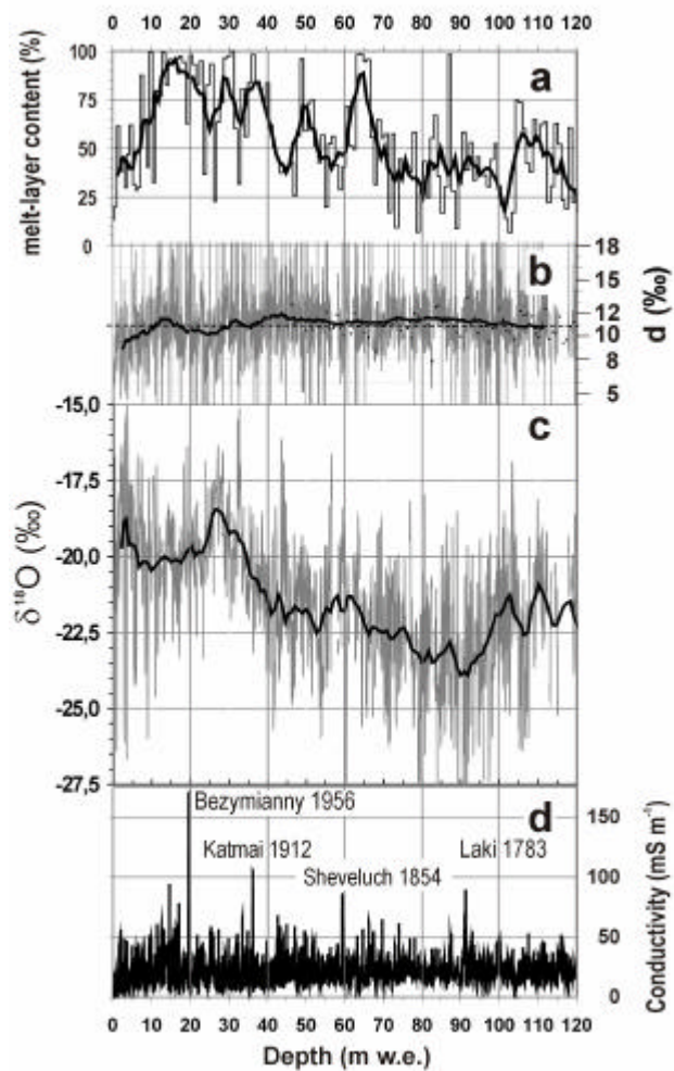
Fig. 4. Profiles from the upper 120 m w.e. (136 m depth) of the main core from Akademii Nauk ice cap. (a) melt-layer content - step function 1 m values, black curve 5 m running mean (b) D excess d, (c) \delta^{18}O – in (b) and (c): grey 25 mm data, black curve 5 m running mean (d) electrical conductivity (DEP) – 5mm resolution
