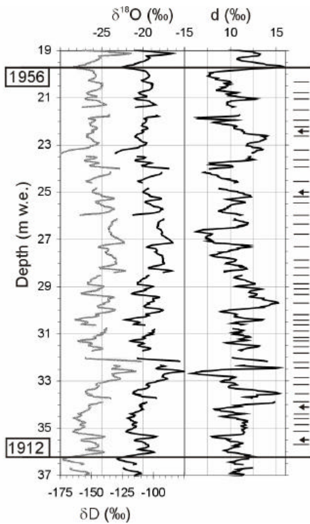
Fig. 5. Stable isotope variations between the 1956 Bezymianny event and the layer with high electrical conductivity assumed to be originating from the eruption of Katmai in 1912. Tags on right-hand side indicate our interpretation of annual cycles. Arrows mark peaks which can be interpreted as additional years.
