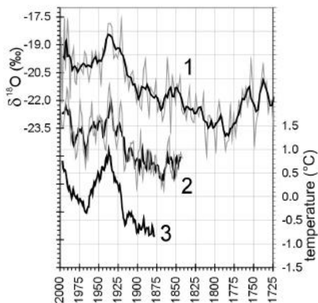
Fig. 7. Dated \delta^{18}\text{O} curve (1) for the segment of ice core shown in Fig. 4 – 1 m mean values and 5 m running means (approx. 2.3 respectively 12 years) – compared with air temperature (2) measured at Vardø/North Norway – 5 and 10 years running mean values – and trend of composite surface air temperature in the Arctic (3) – 6 years running mean – deviation from mean temperature 1961–2000 (data from Polyakov and others, 2003).
