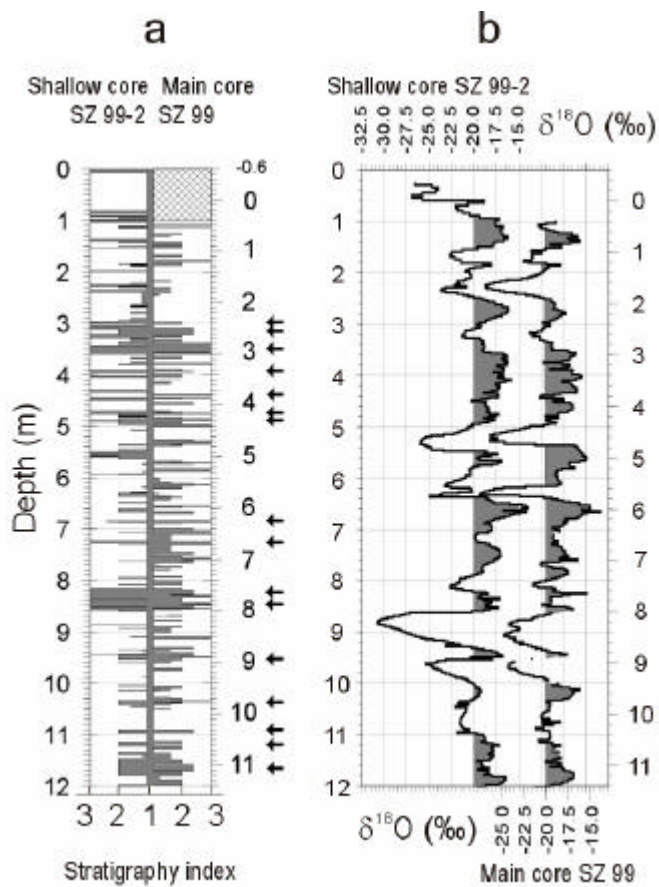
Fig. 2. Comparison of visible stratigraphy (a) and \delta^{18}O (b) in the upper part of the main core SZ 99 and the shallow core SZ 99-2 drilled some 200 m apart:
