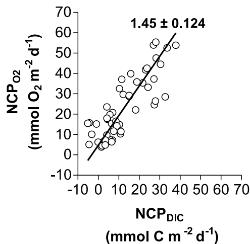
Figure 4. Net community production computed from oxygen incubation ( \text{NCP}_{\text{O}_2} ) versus NCP computed from DIC and TA ( \text{NCP}_{\text{DIC}} ) with a model II regression line.
