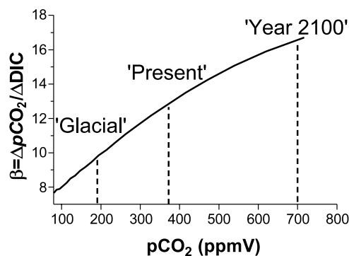
Figure 8. Buffer factor of the carbonate system for increasing partial pressure of \text{CO}_2 at the initial conditions of the experiment (salinity, 31.3; temperature, 10.0°C; \text{TA} , 2150 \mu\text{mol kg}^{-1} ).
