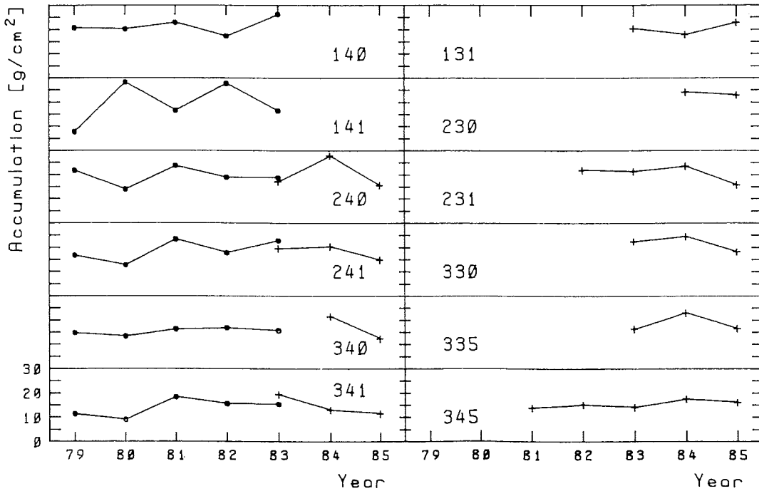
Fig. 4. Amount of annual accumulation at the measuring points of the Filchner I and Filchner II field programmes. (o) snow-pit 1984; (+) snow-pit 1986.
