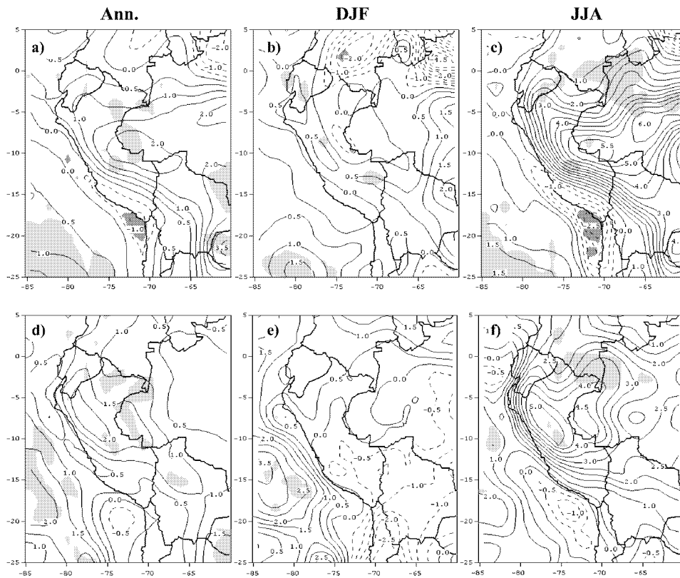
Figure 10. Trend in relative humidity (in % decade -1 , top row) between 1979 and 1995 and total cloud cover (in % decade -1 , bottom row) between 1979 and 1998 based on ECHAM-4 T106 simulation. Trends are shown for annual mean (left column), DJF (middle column) and JJA (right column). Contour interval is 0.5%, negative contours are dashed and regions where humidity or total cloud cover has significantly increased (decreased) at the 95% confidence level are shaded in light (dark) gray. Figures have been smoothed with a 3 \times 3 averaging filter.
