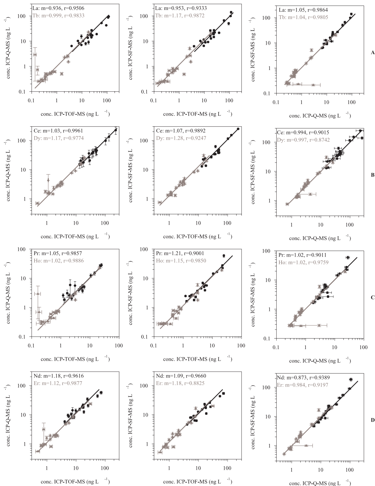
Figure 1: REE concentrations with SD in \text{ng L}^{-1} in Antarctic ice core samples plotted as ICP-Q-MS concentrations vs. ICP-TOF-MS concentrations, ICP-SF-MS concentrations vs. ICP-TOF-MS concentrations and ICP-SF-MS concentrations vs. ICP-Q-MS concentrations with associated parameters for a linear fit ( y = m \cdot x , Assumption: intercept=0). Errors of each measurement were taken as weighting parameters ( \text{error} = \text{SD} / \sqrt{n} , n = \text{replicate analysis} ).
