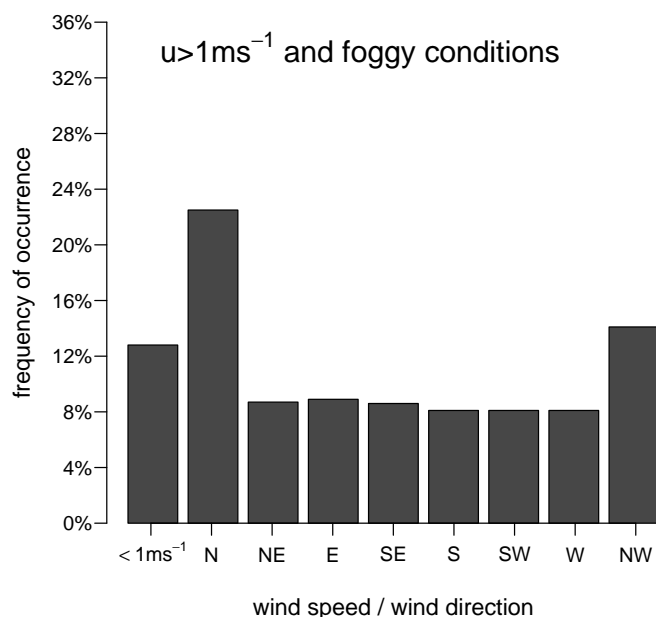
Figure 3.3: Frequency of occurrence of windspeed >1 \text{ m s}^{-1} with respect to wind direction during foggy weather conditions. The wind directions during low windspeeds <1 \text{ m s}^{-1} were not taken into consideration.
