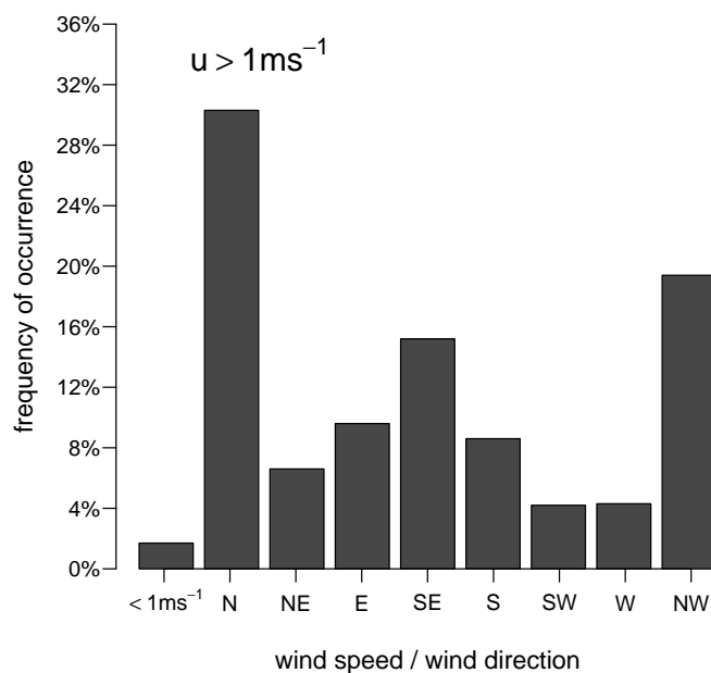
Figure 3.2: Frequency of occurrence of windspeed >1 \text{ m s}^{-1} with respect to wind direction during the entire campaign. The wind directions during low windspeeds <1 \text{ m s}^{-1} were not taken into consideration.
