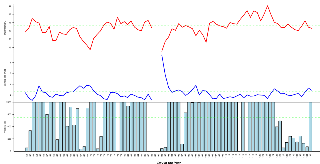
Figure 3.1: Meteorological conditions during the entire field campaign in Costa Rica. Daily median temperature (upper panel), median daily windspeed and median daily visibility in the lower panel. The dashed green lines represent the mean value of the shown parameter during the entire campaign. During the four days (Day 87-90), all the devices were switched off due to lack of fog.
