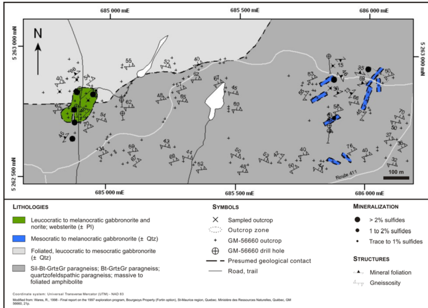
FIG. S2 Geology of the Rochette West prospect area
