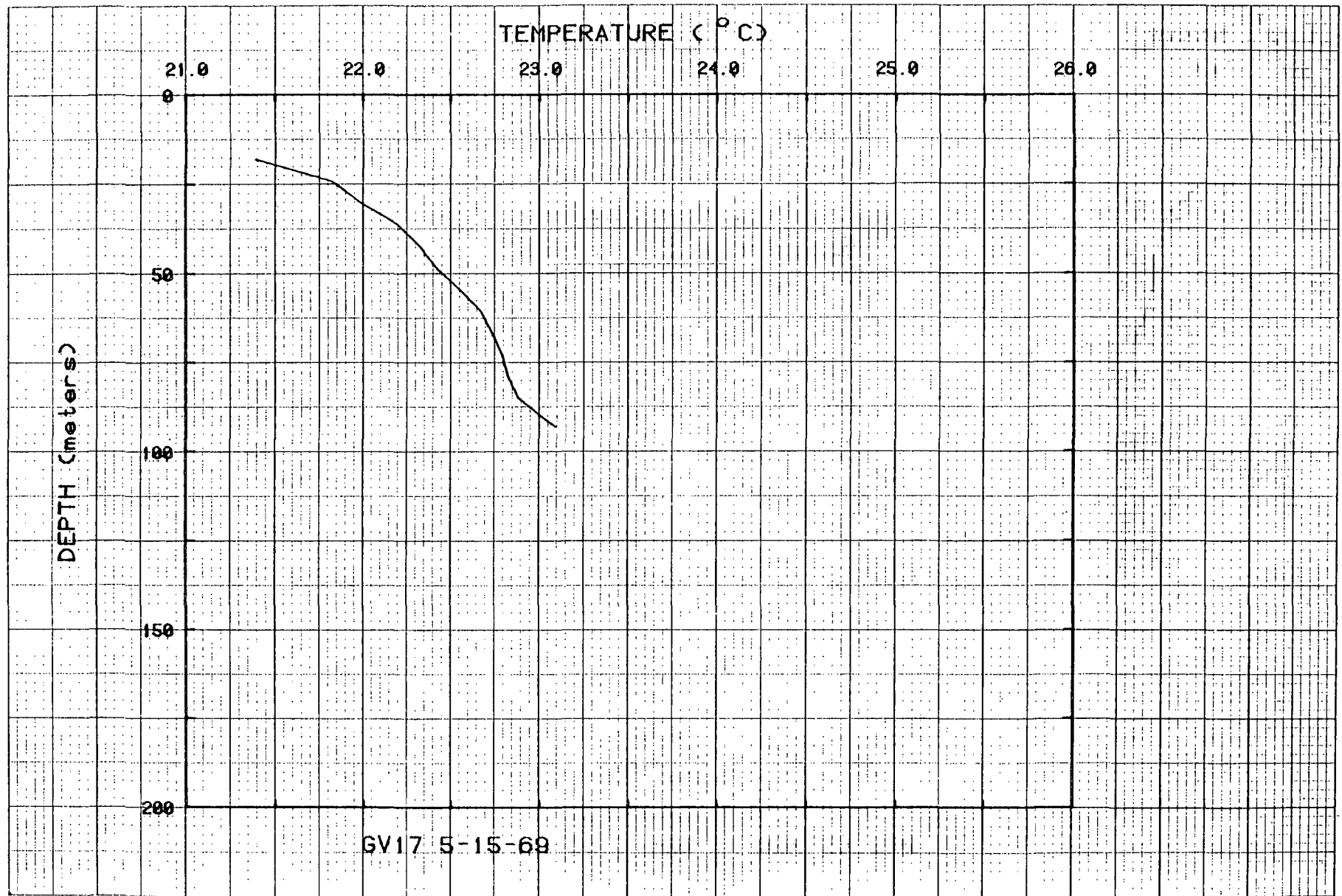
Figure 25. Temperatures for hole GV17.
