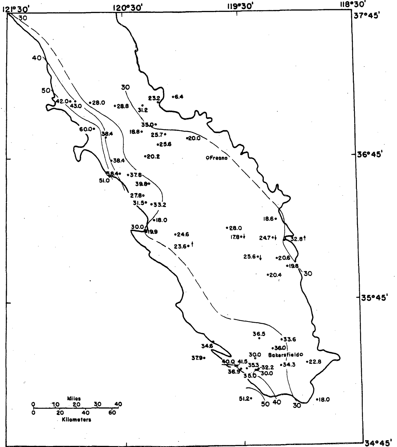
Figure 8. Gradient map of the southern portion of the Great Valley, California. Contour interval = 10°C/km.
