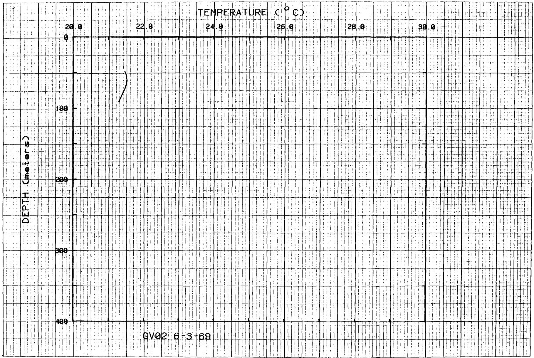
Figure 11. Temperatures for hole GV02.
