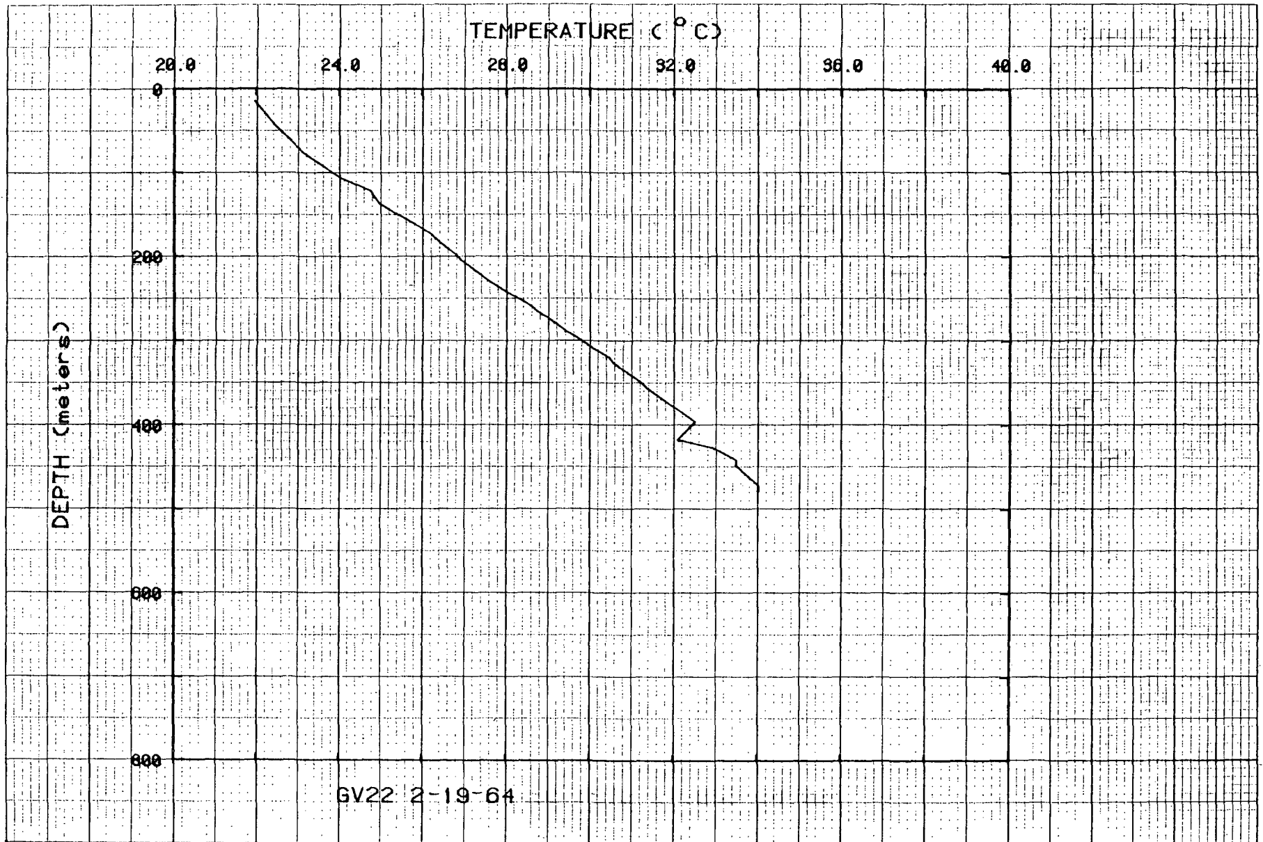
Figure 30. Temperatures for hole GV22.
