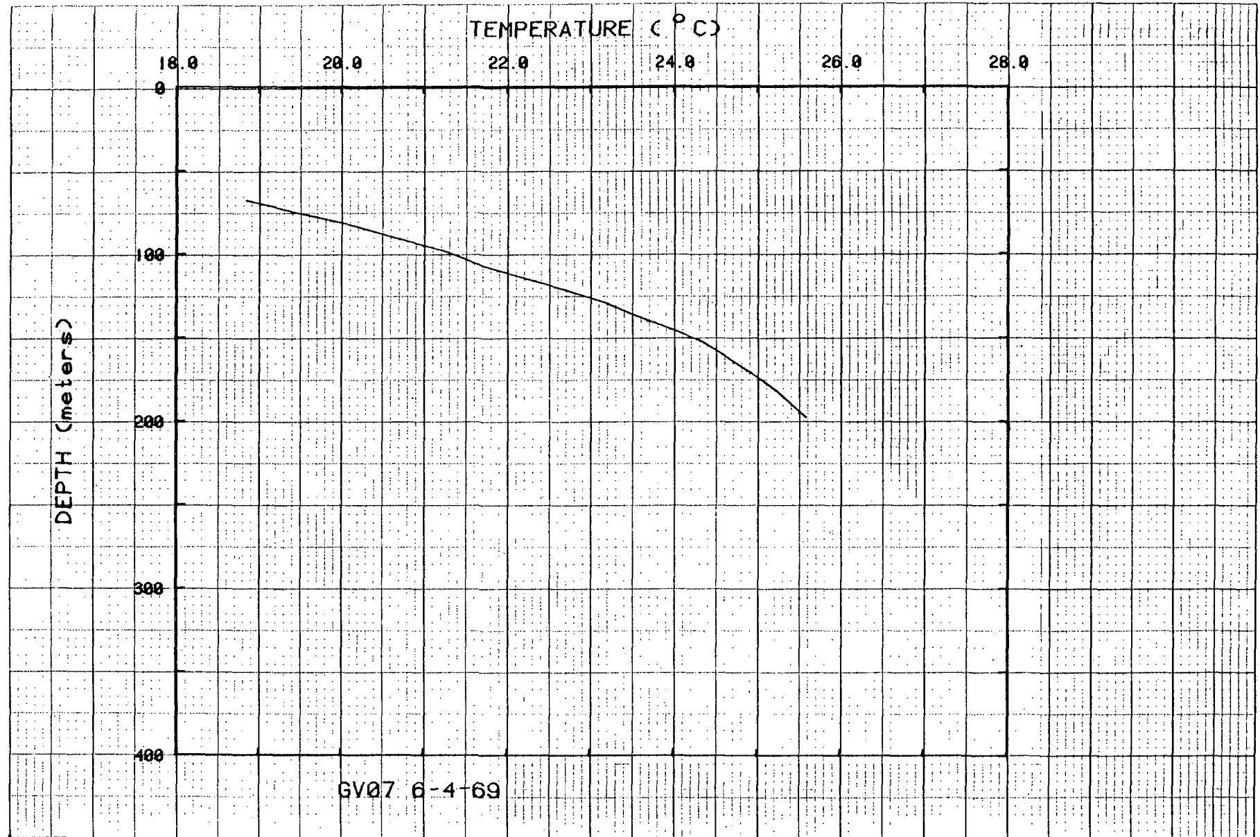
Figure 16. Temperatures for hole GV07.
