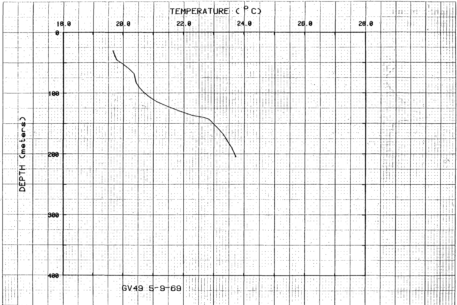
Figure 56. Temperatures for hole GV49.
