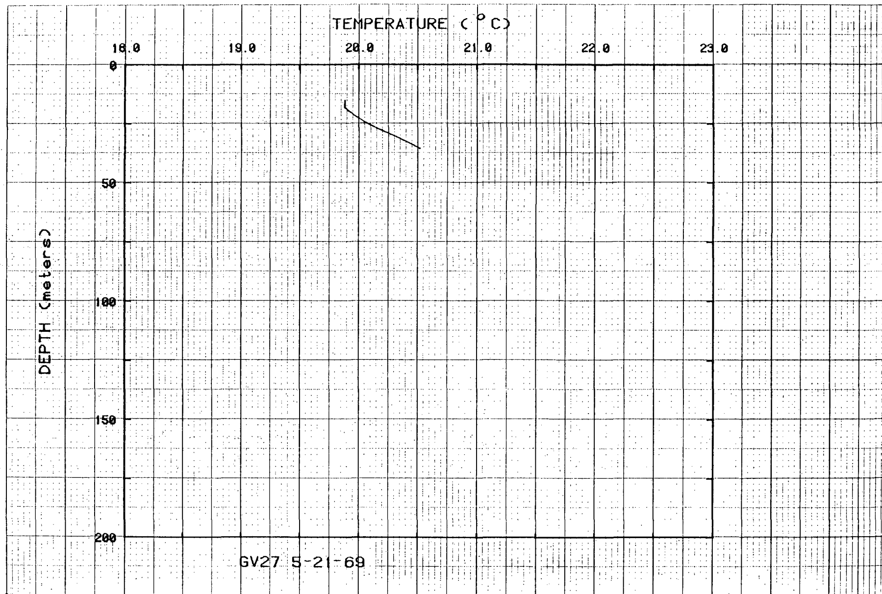
Figure 34. Temperatures for hole GV27.
