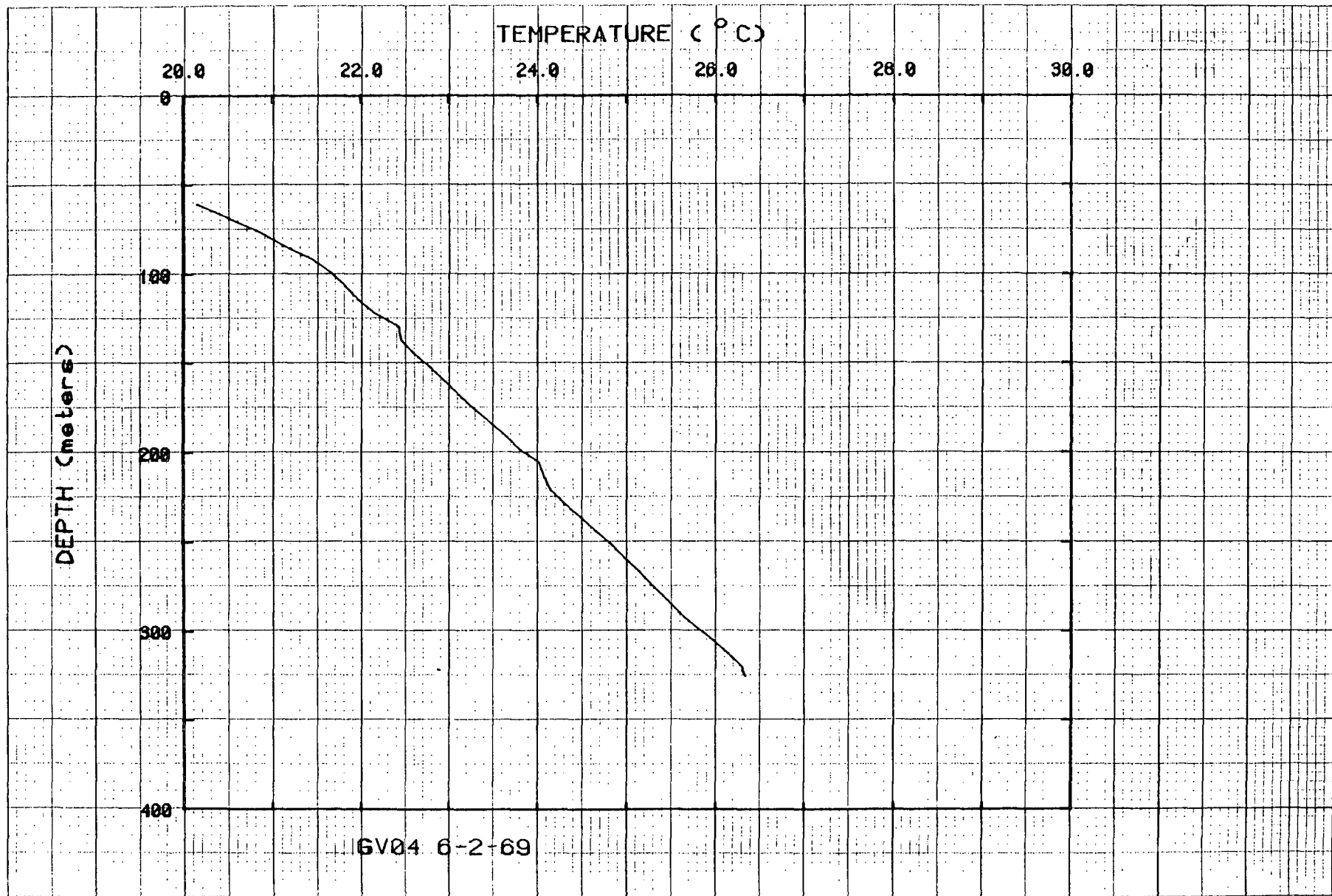
Figure 13. Temperatures for hole GV04.
