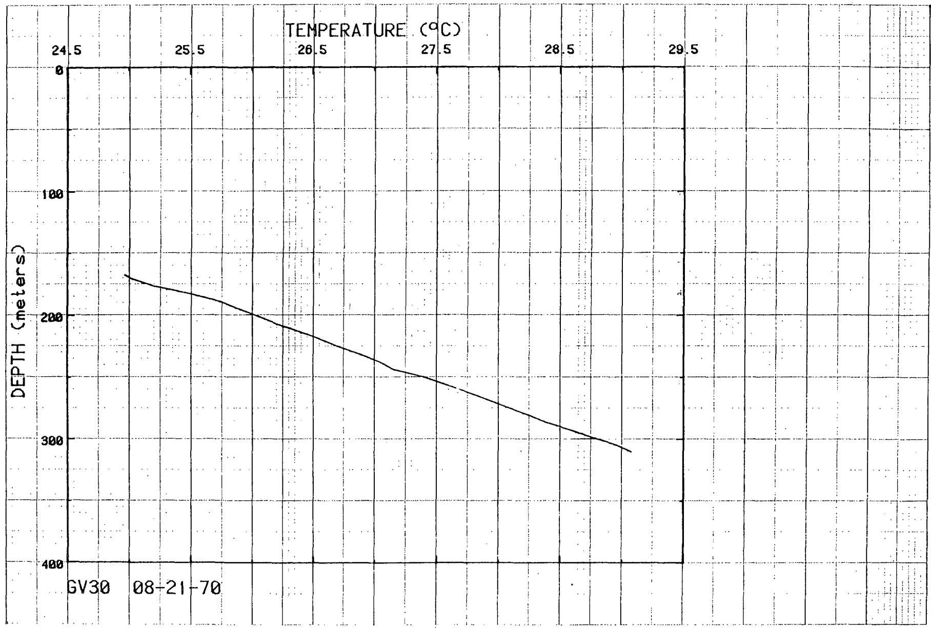
Figure 37. Temperatures for hole GV30.
