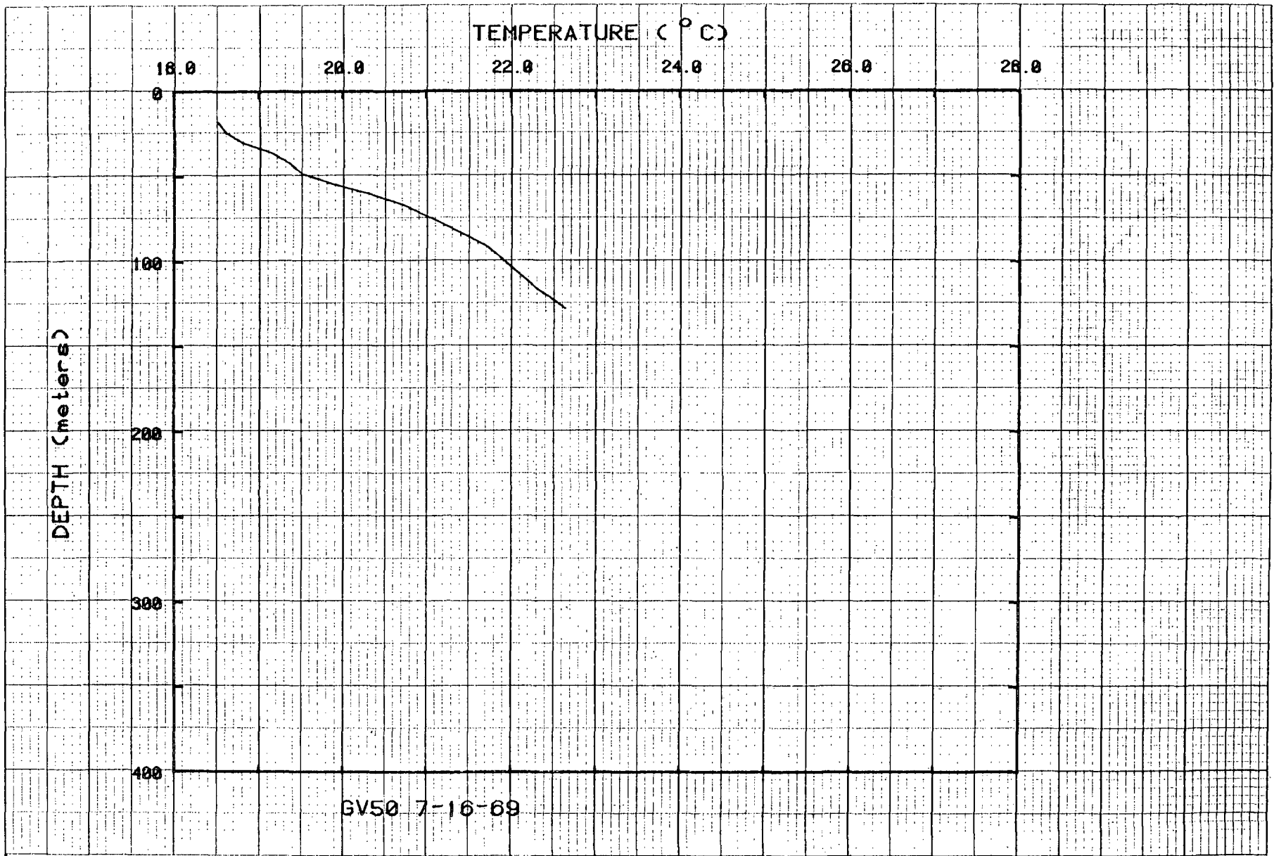
Figure 57. Temperatures for hole GV50.
