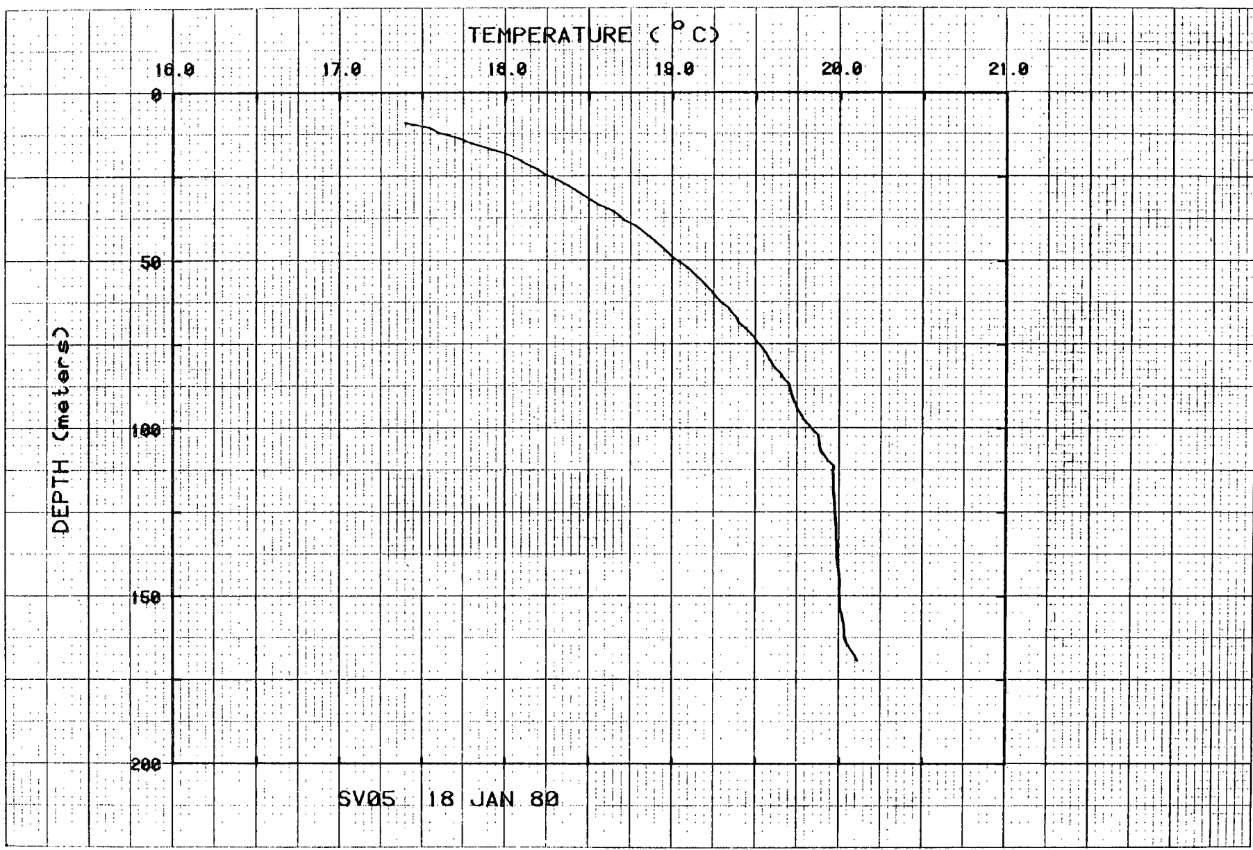
Figure 67. Temperatures for hole SV05.
