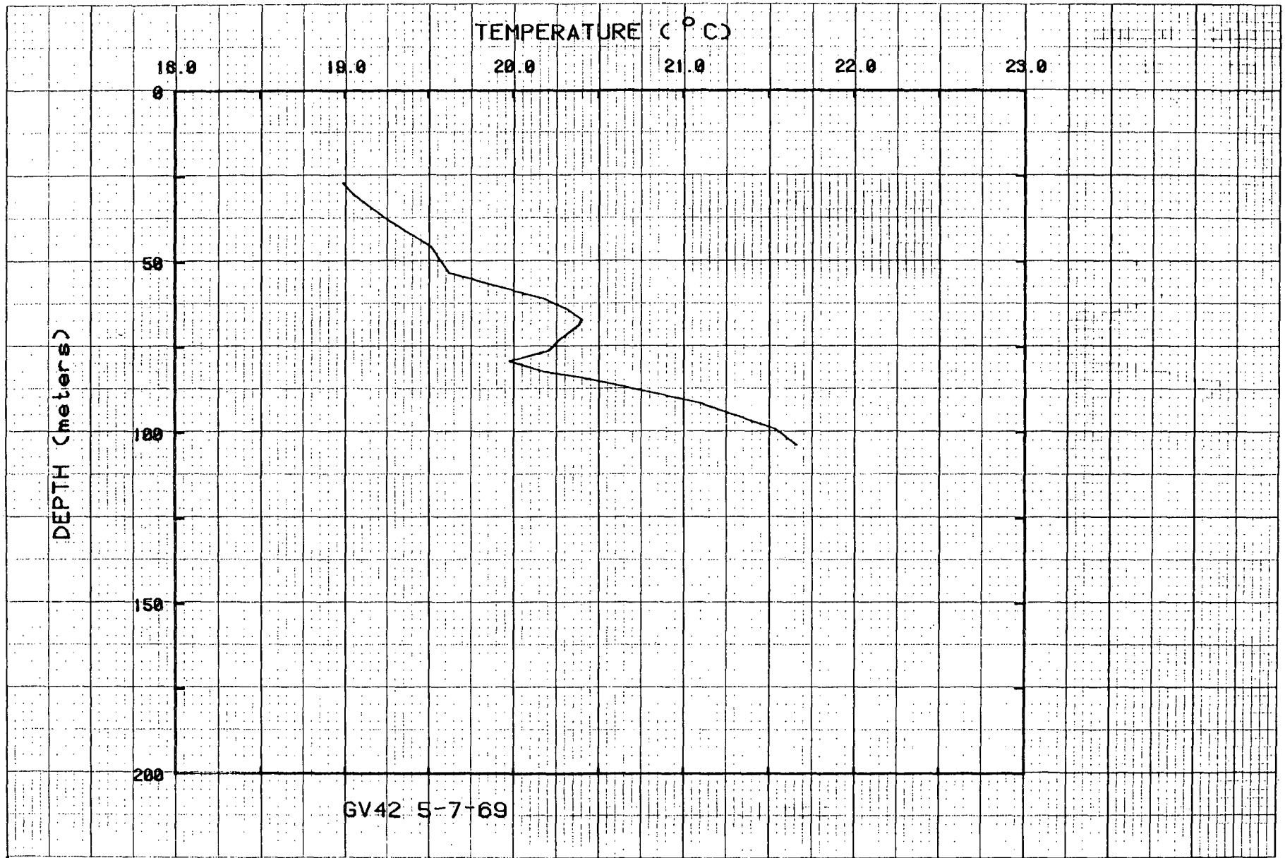
Figure 49. Temperatures for hole GV42.
