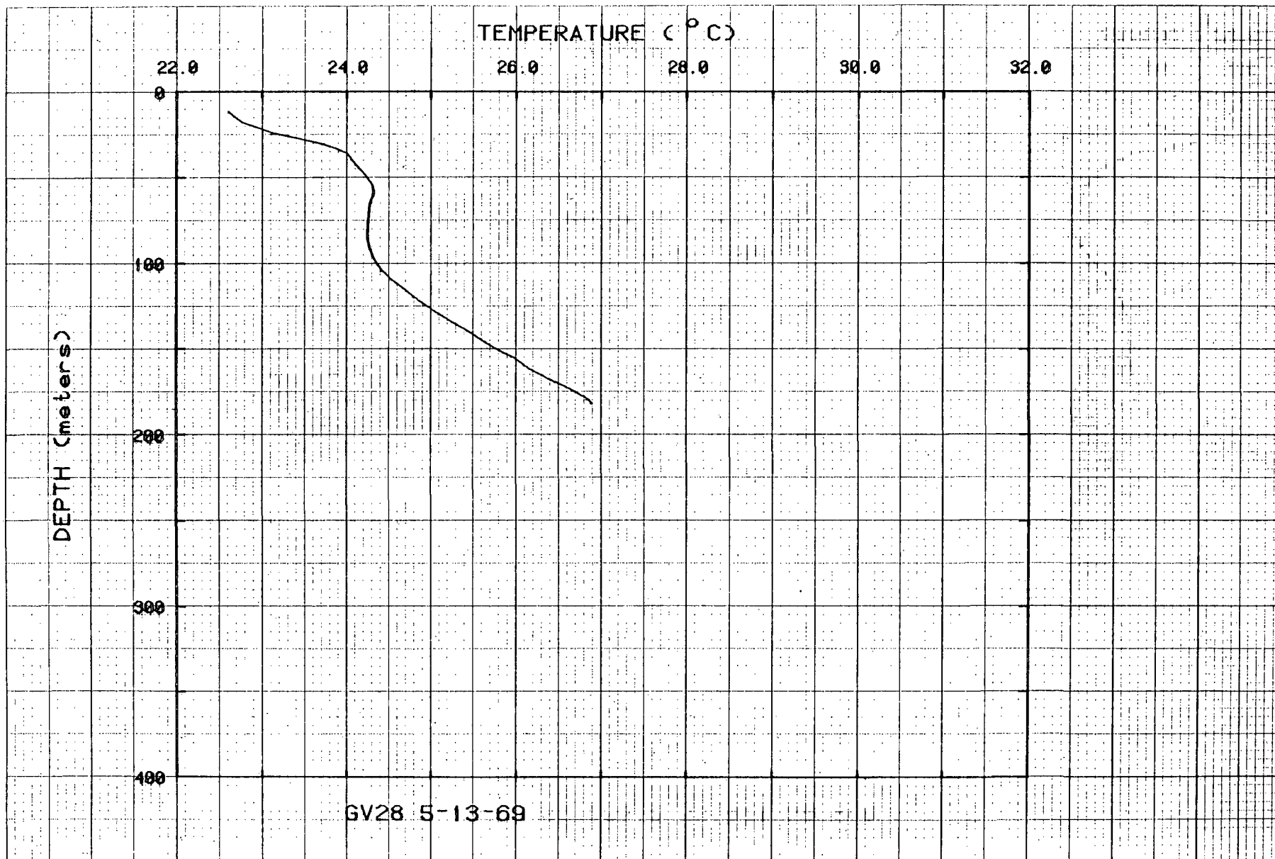
Figure 35. Temperatures for hole GV28.
