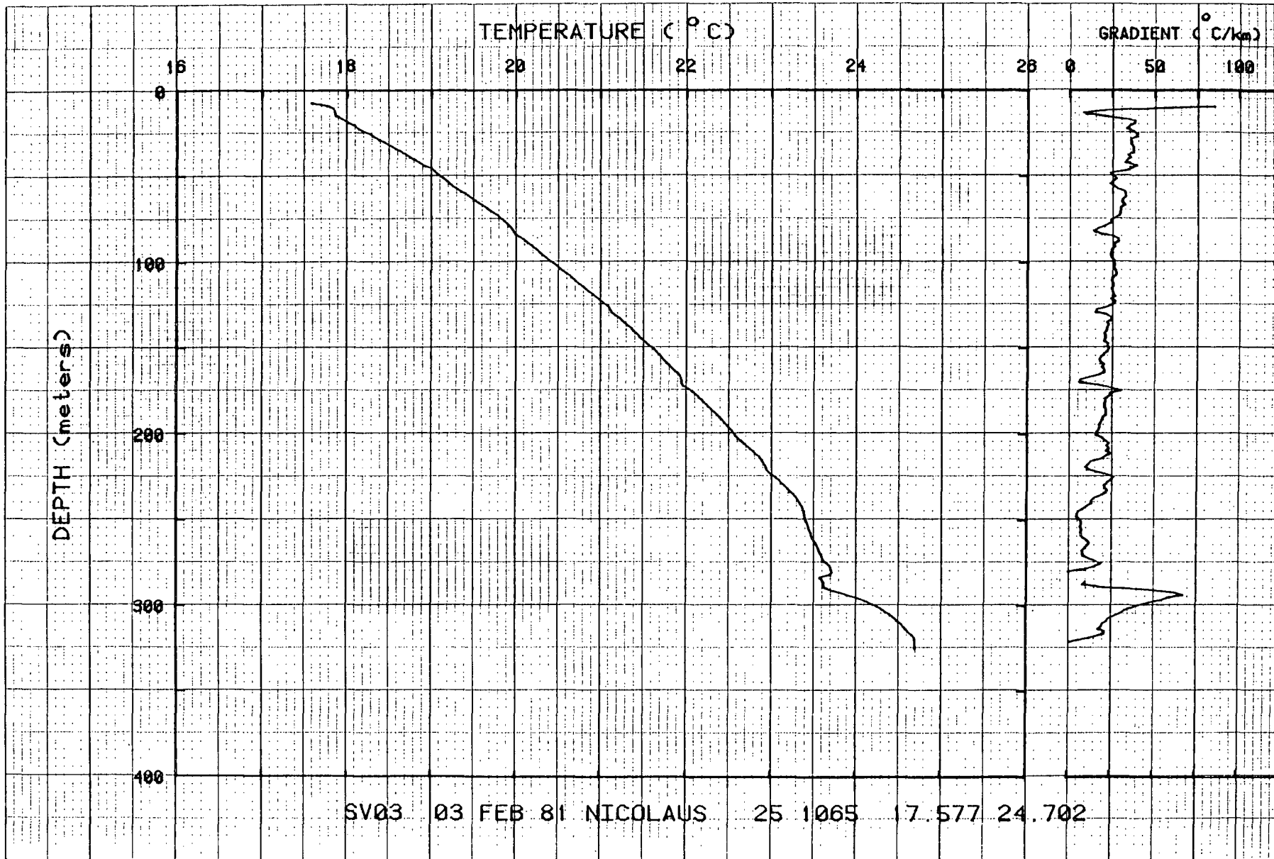
Figure 5. Temperatures and gradients for hole SV03.
