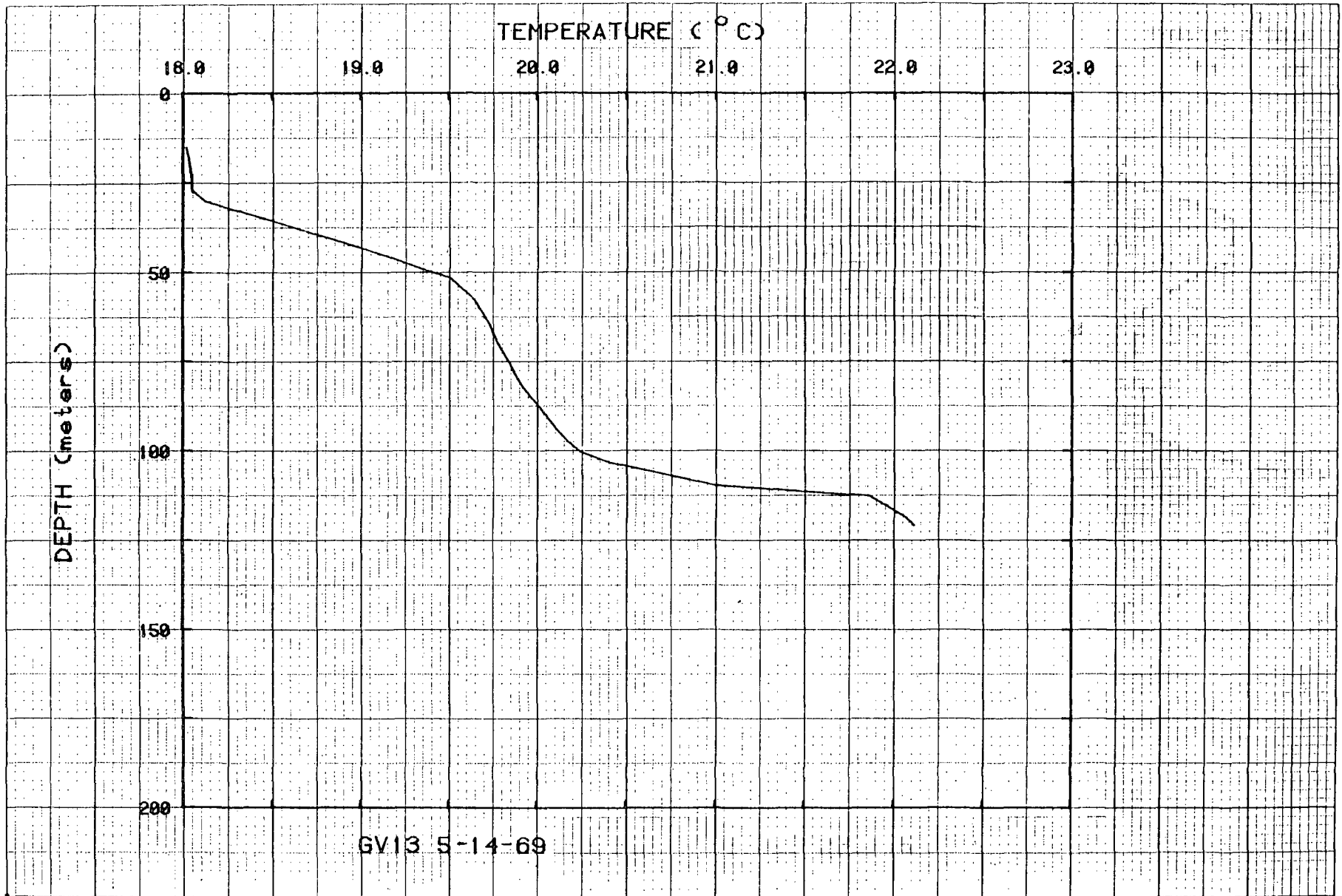
Figure 21. Temperatures for hole GV13.
