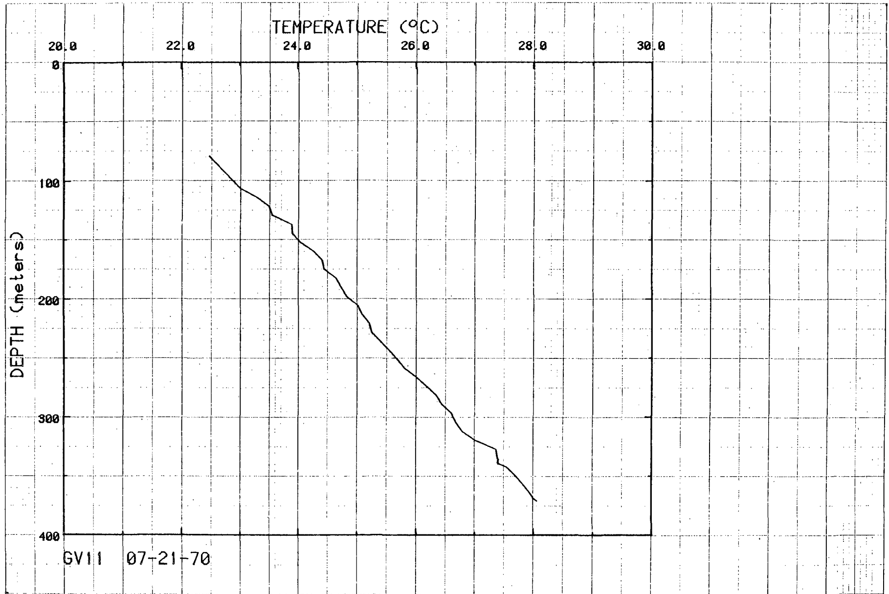
Figure 19. Temperatures for hole GV11.
