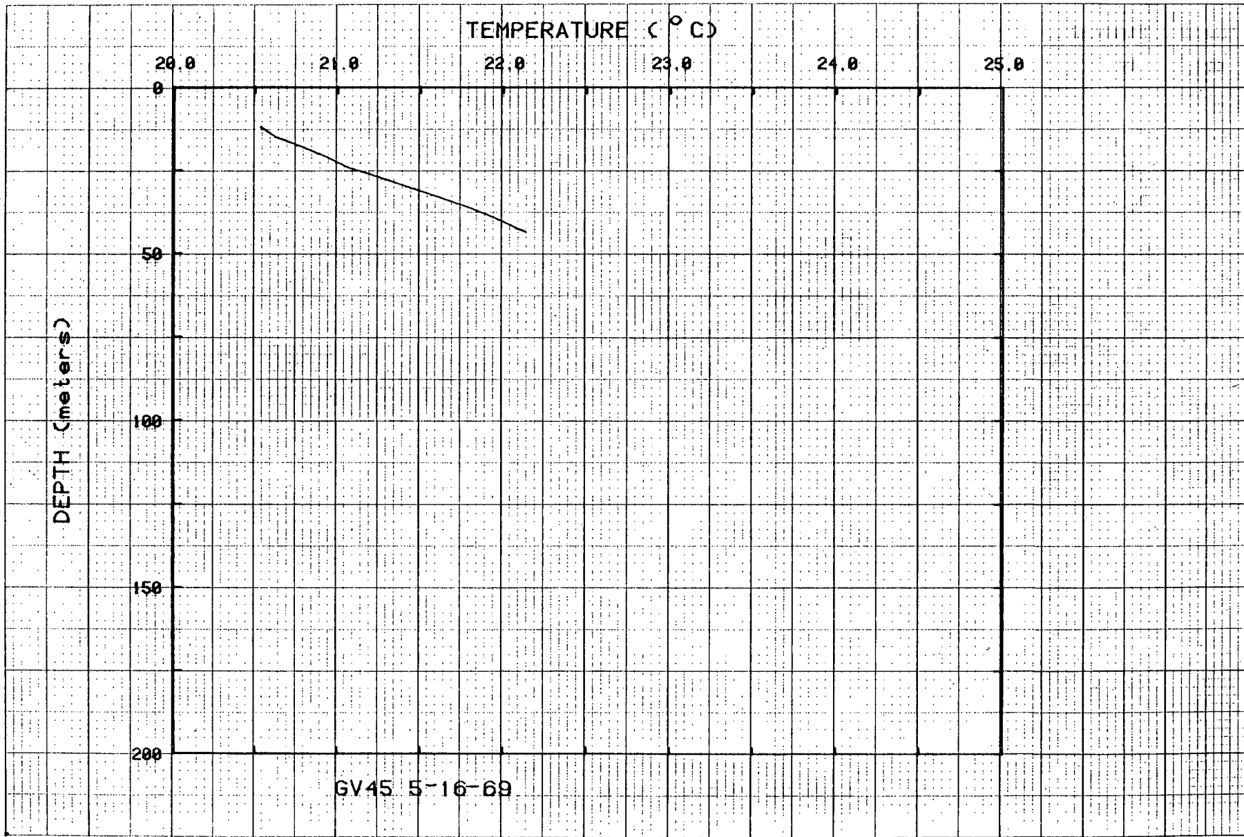
Figure 52. Temperatures for hole GV45.
