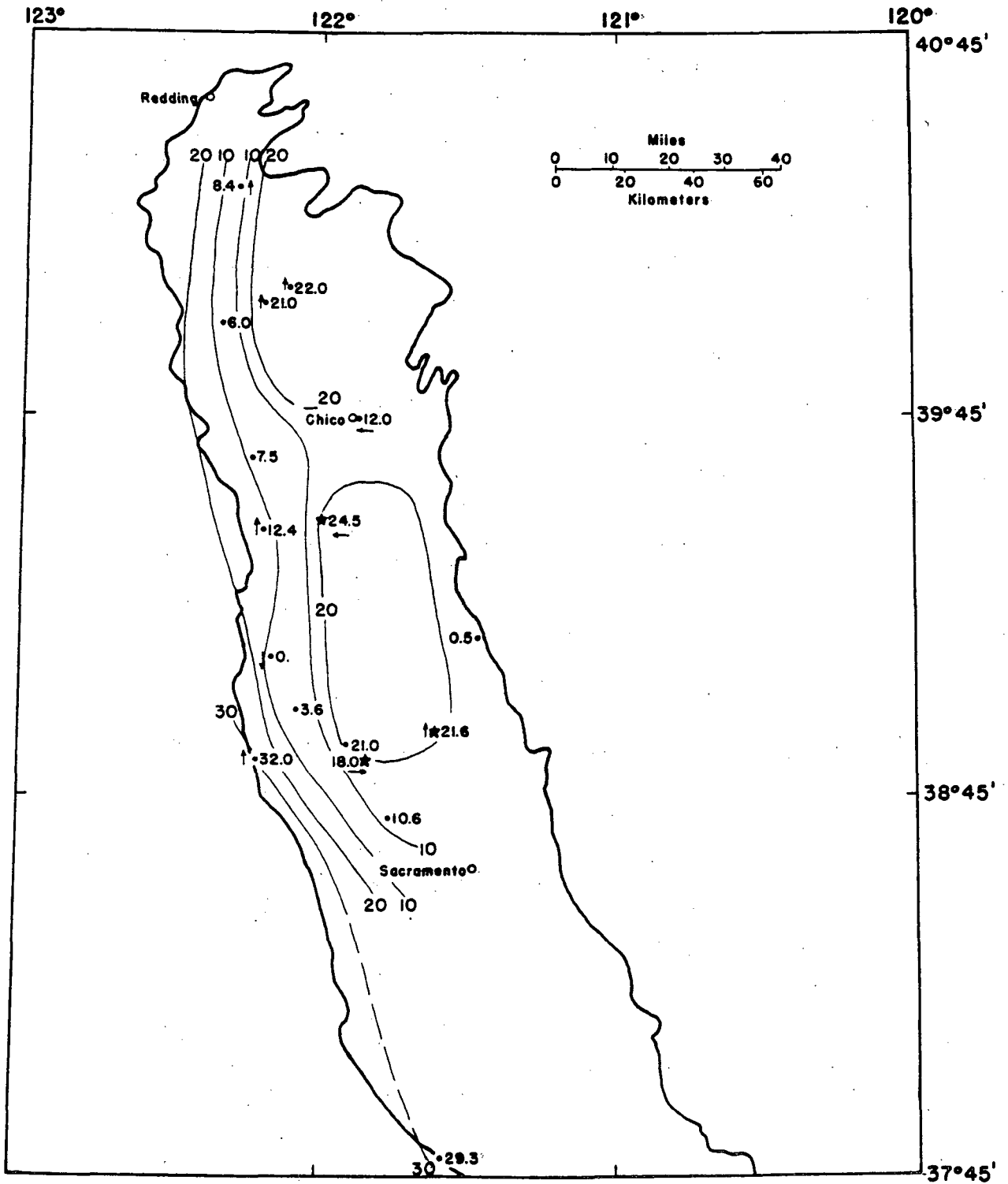
Figure 9. Gradient map of the northern portion of the Great Valley, California. Contour interval = 10^{\circ}\text{C}/\text{km} . New heat-flow sites are indicated by stars.
