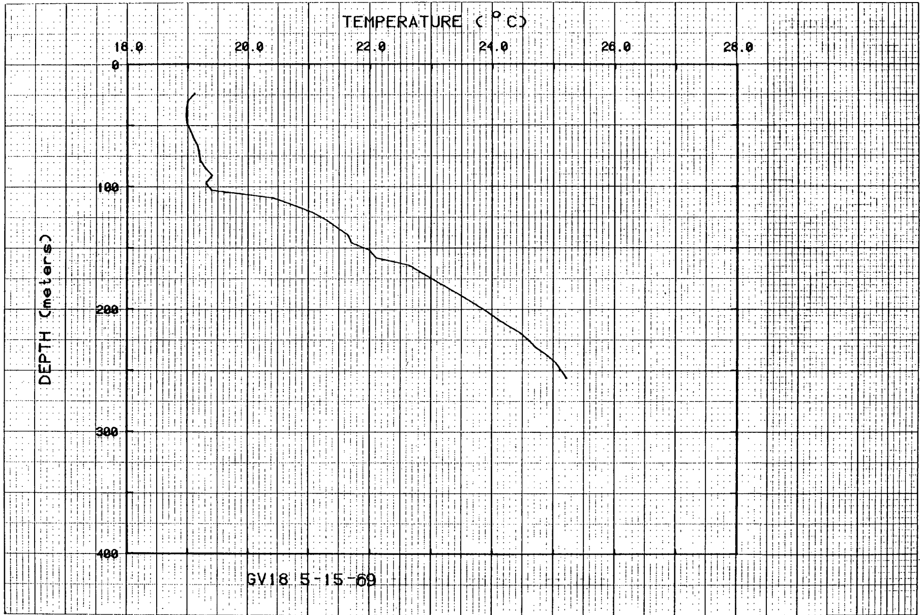
Figure 26. Temperatures for hole GV18.
