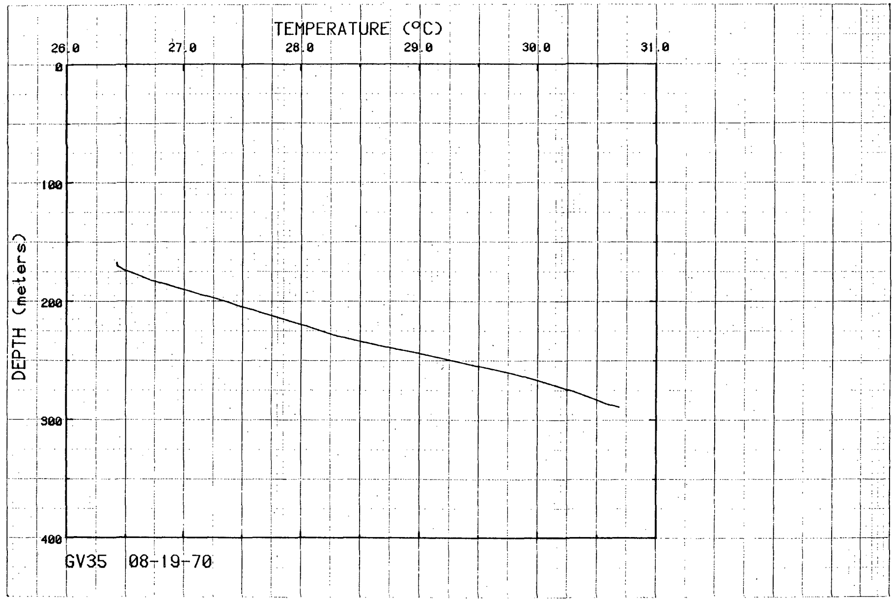
Figure 42. Temperatures for hole GV35.
