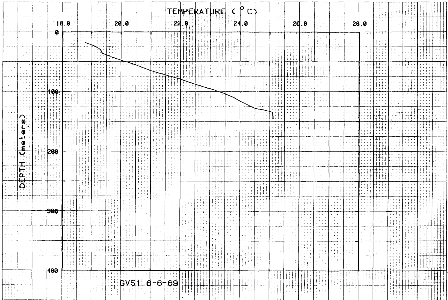
Figure 58. Temperatures for hole GV51.
