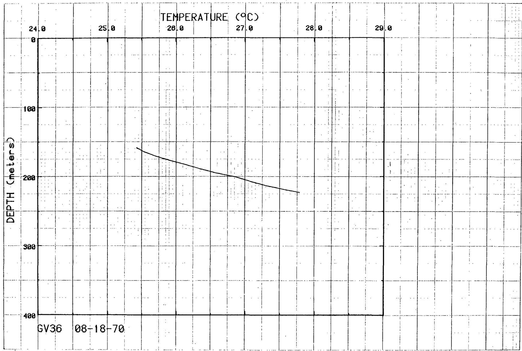
Figure 43. Temperatures for hole GV36.
