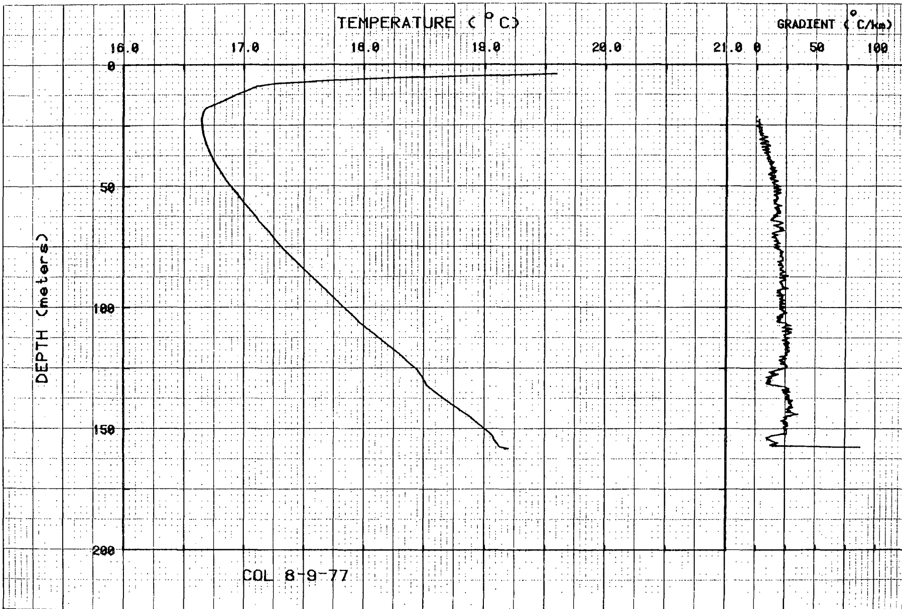
Figure 63. Temperatures and gradients for hole COL.
