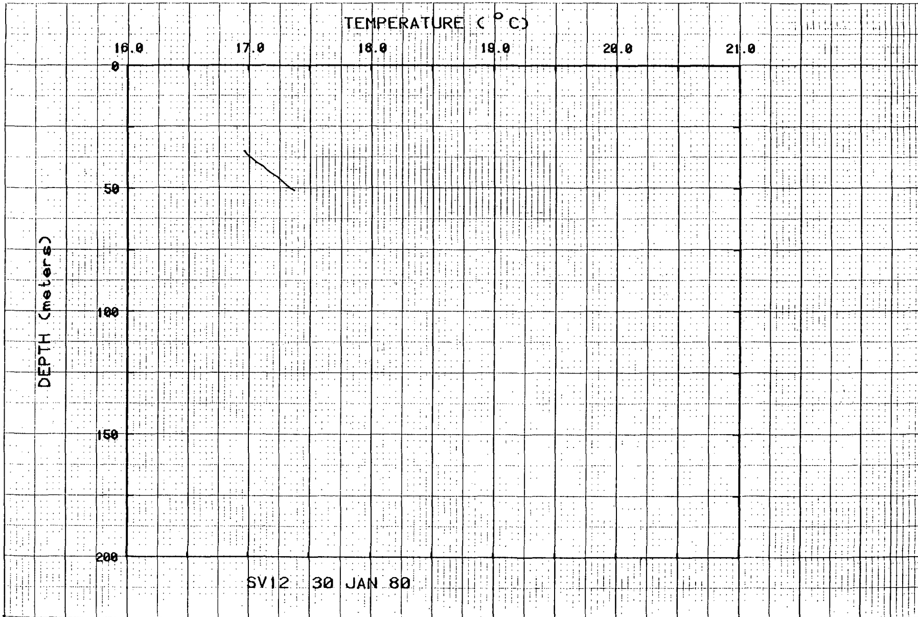
Figure 68. Temperatures for hole SV12.
