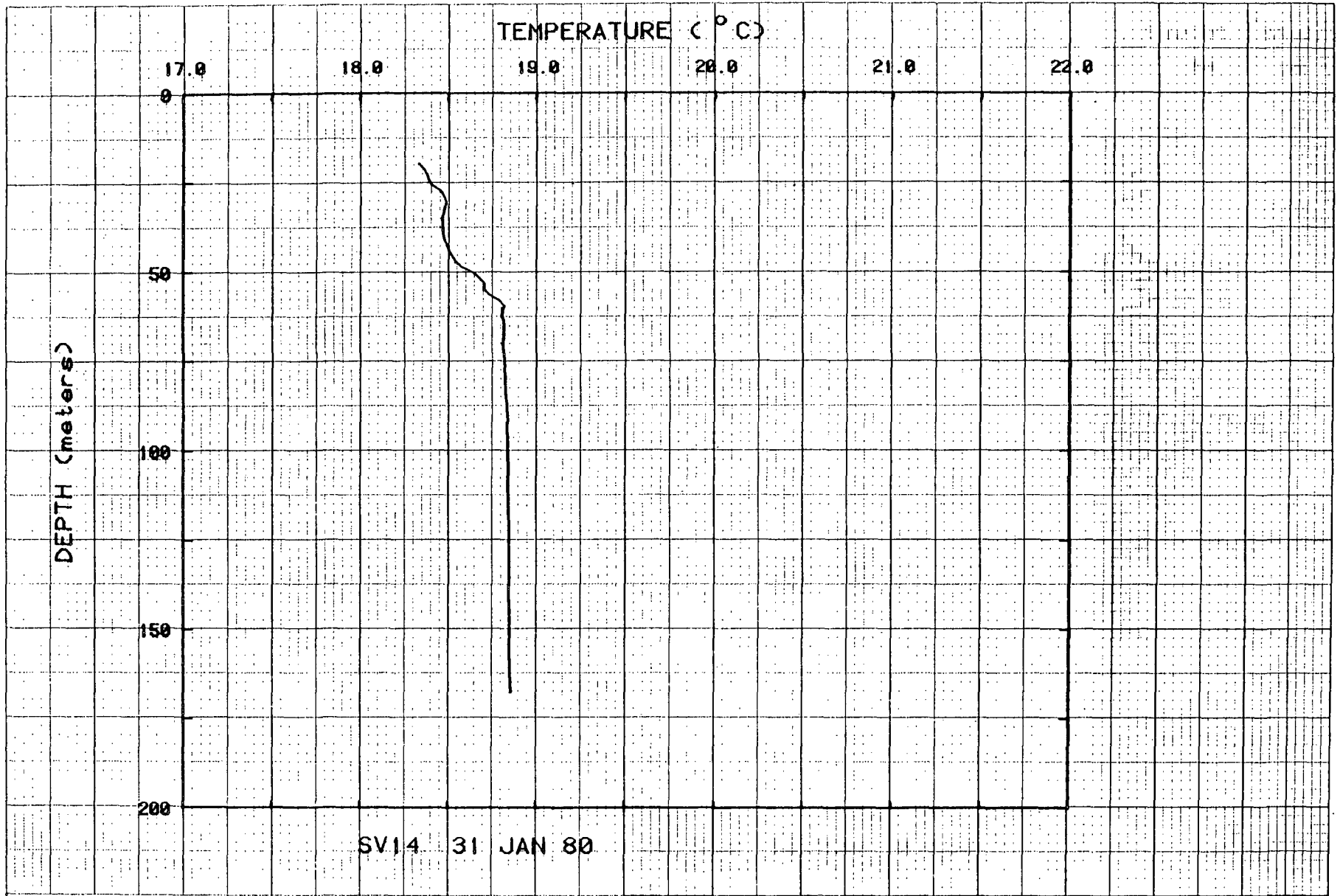
Figure 65. Temperatures for hole SV14.
