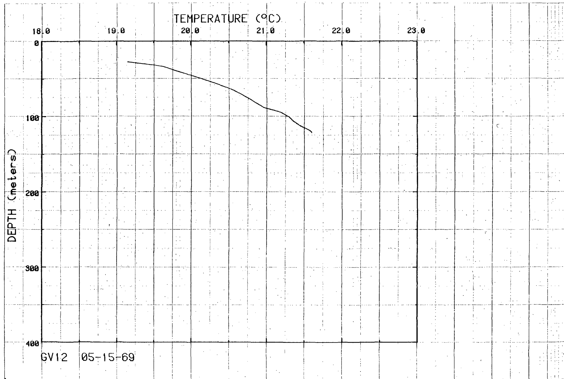
Figure 20. Temperatures for hole GV12.
