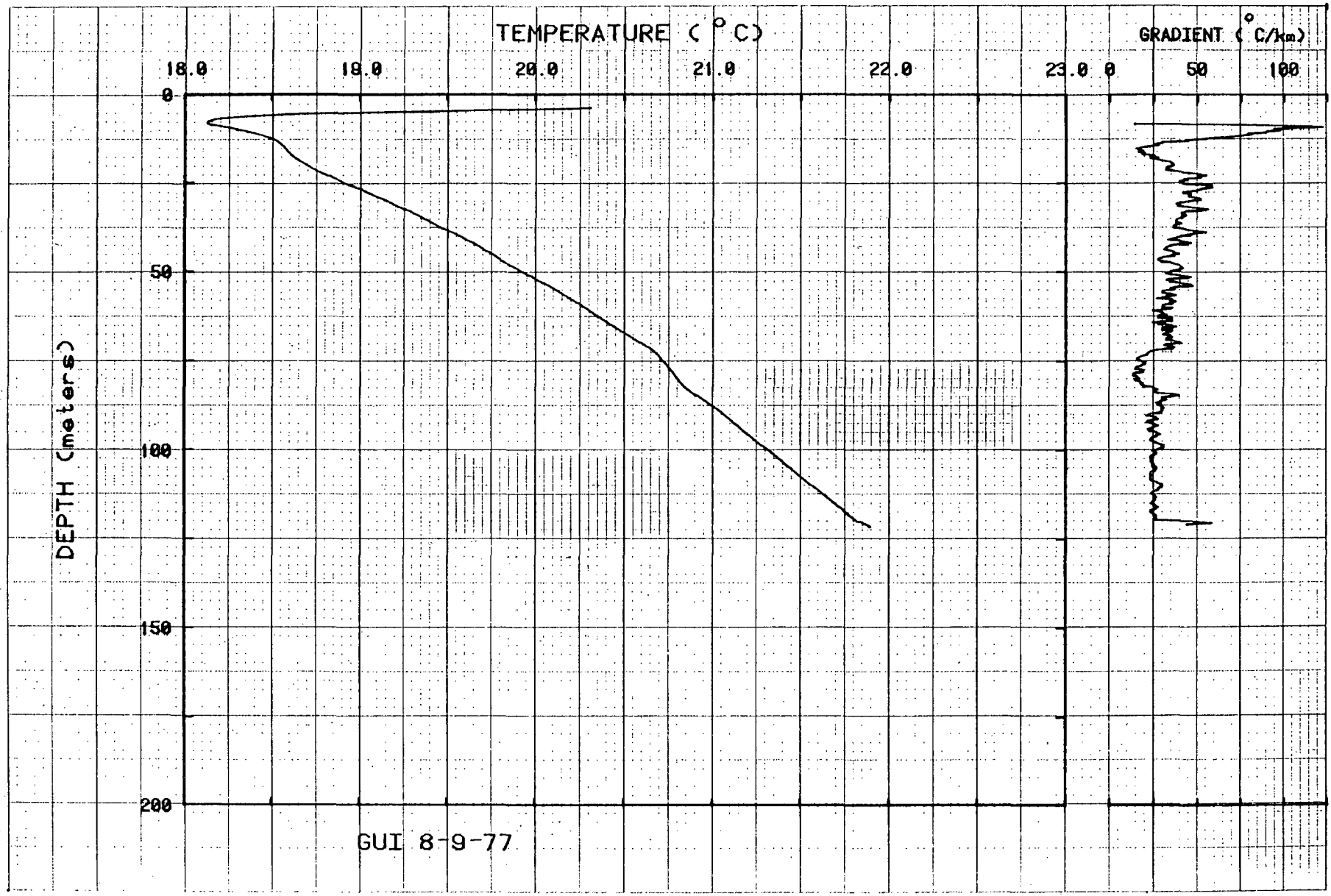
Figure 62. Temperatures and gradients for hole GUI.
