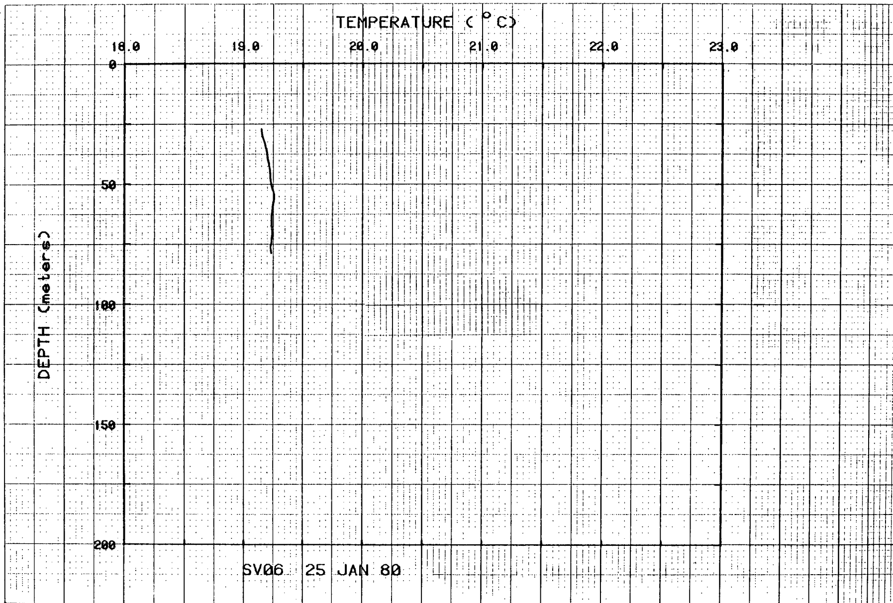
Figure 71. Temperatures for hole SV06.
