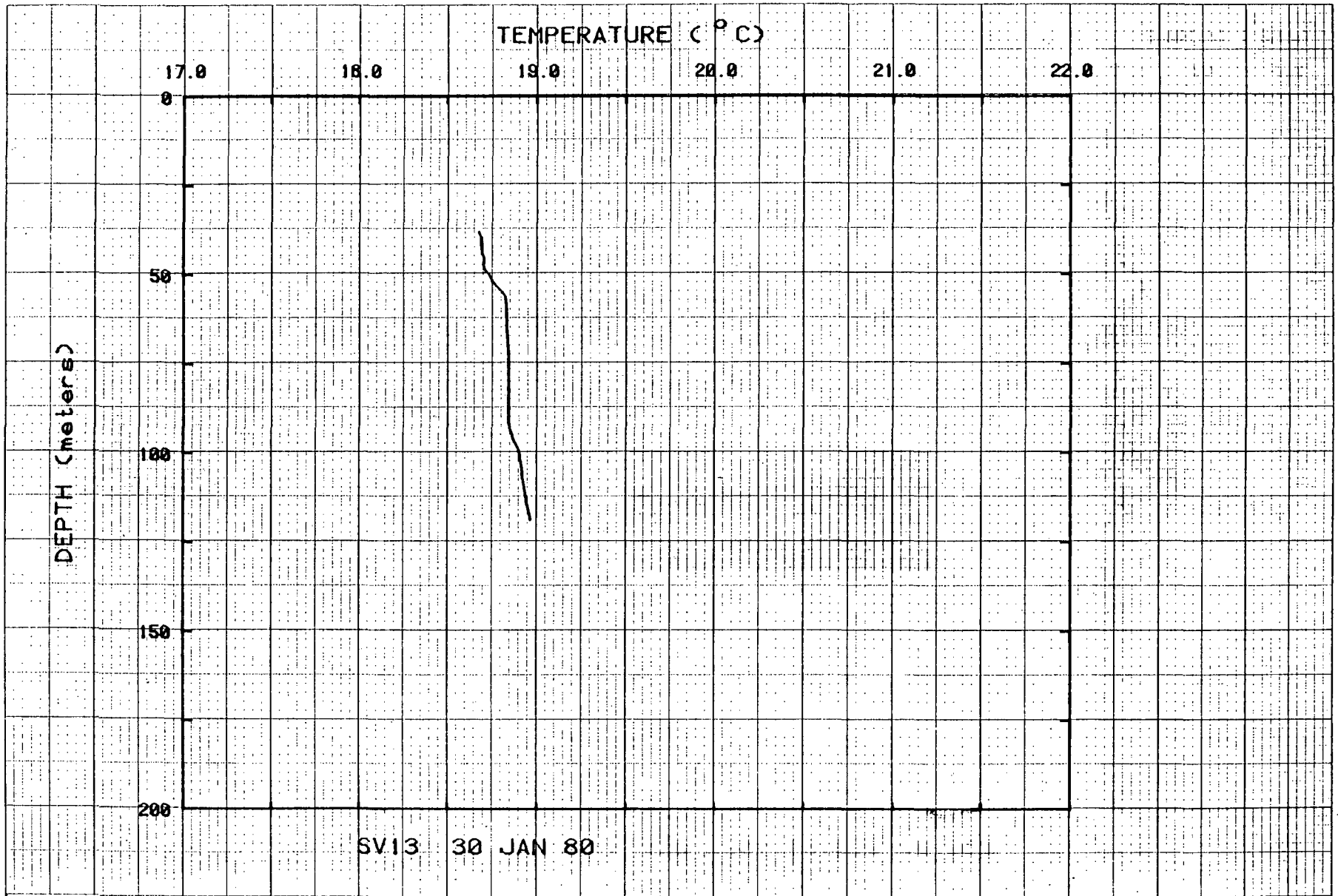
Figure 64. Temperatures for hole SV13.
