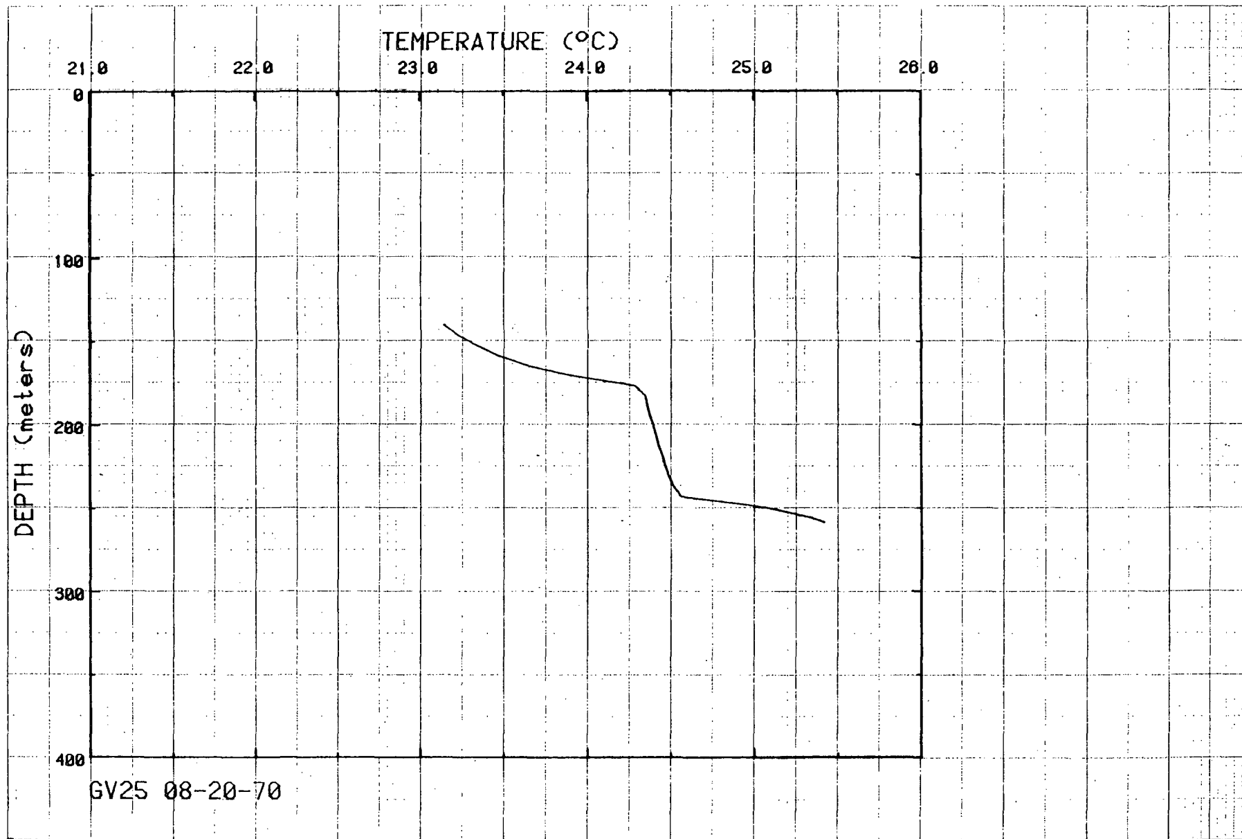
Figure 32. Temperatures for hole GV25.
