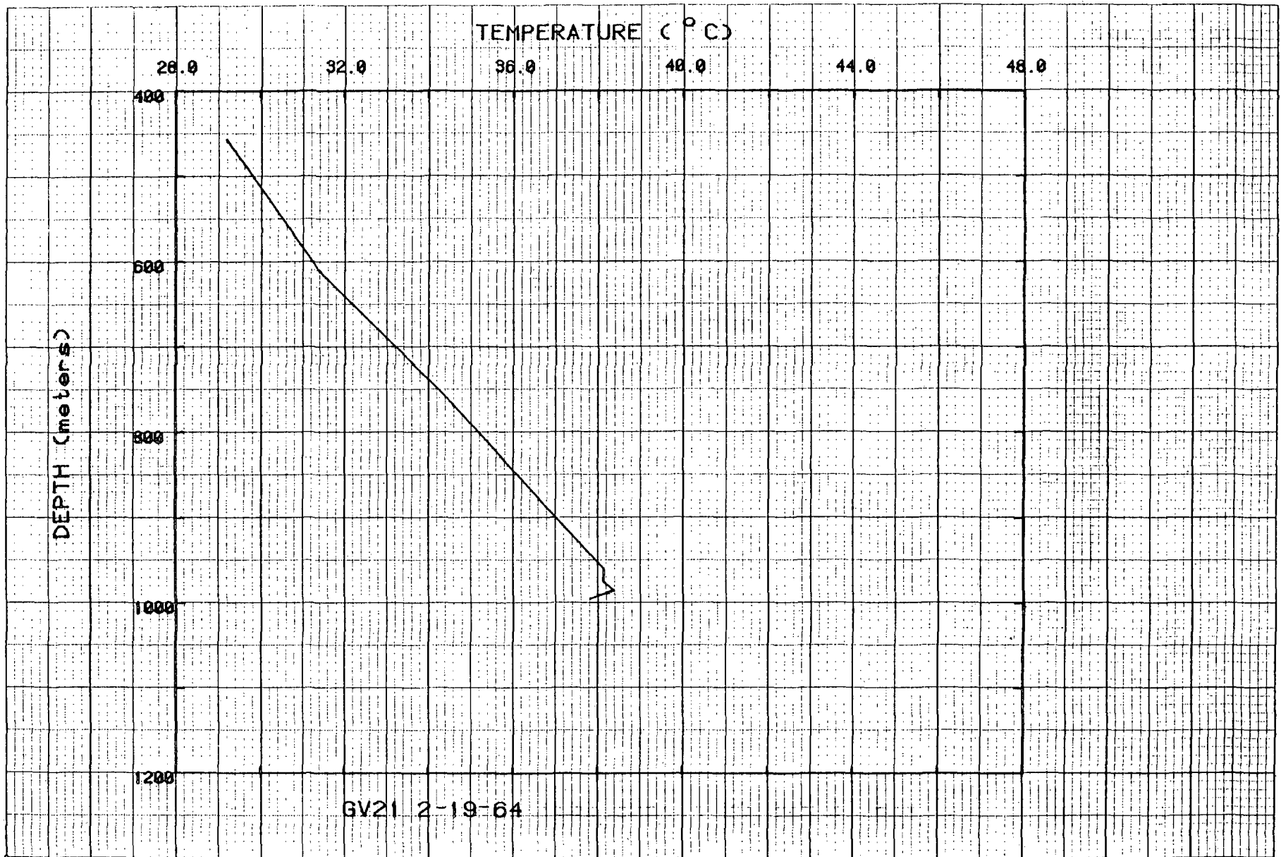
Figure 29. Temperatures for hole GV21.
