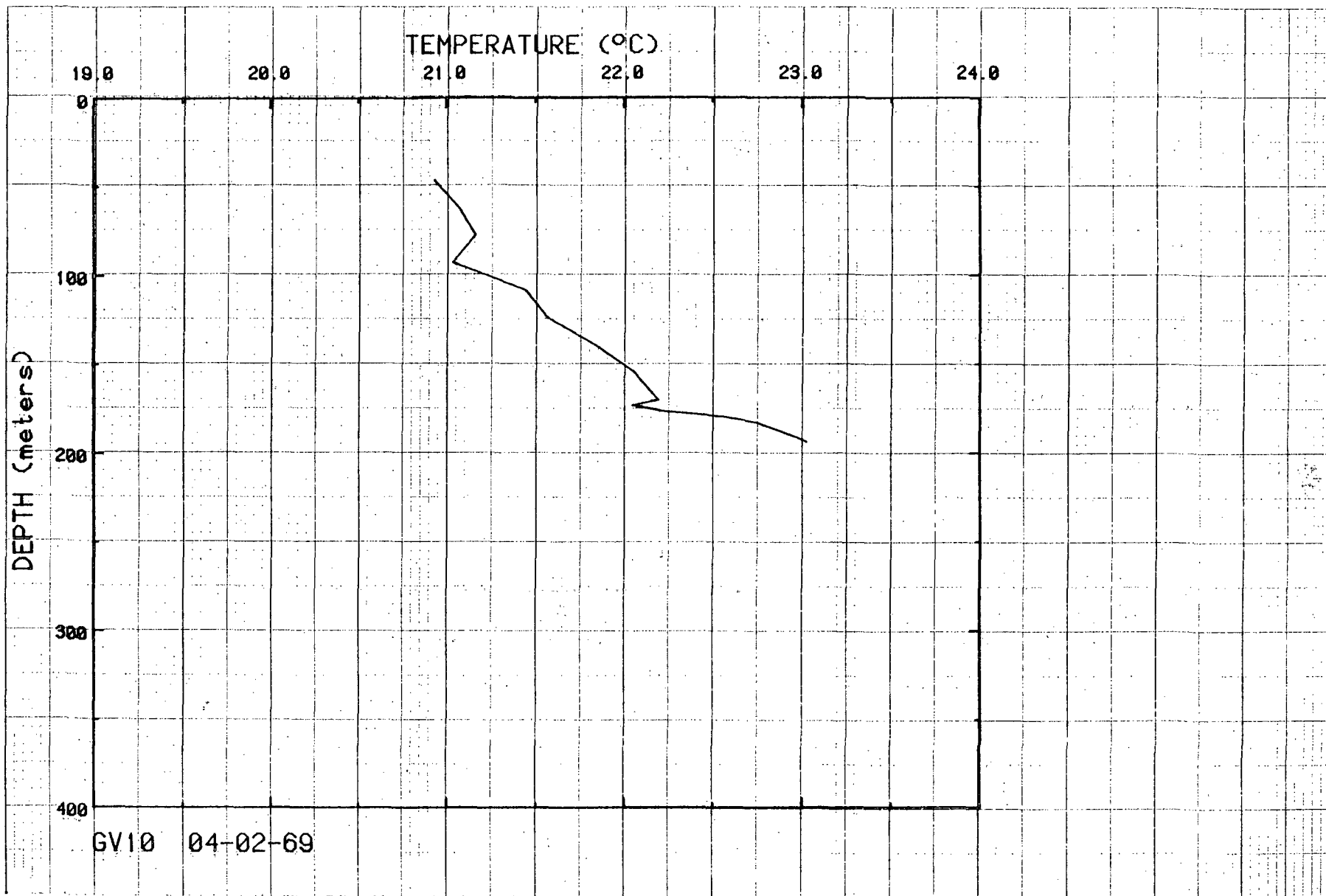
Figure 18. Temperatures for hole GV10.
