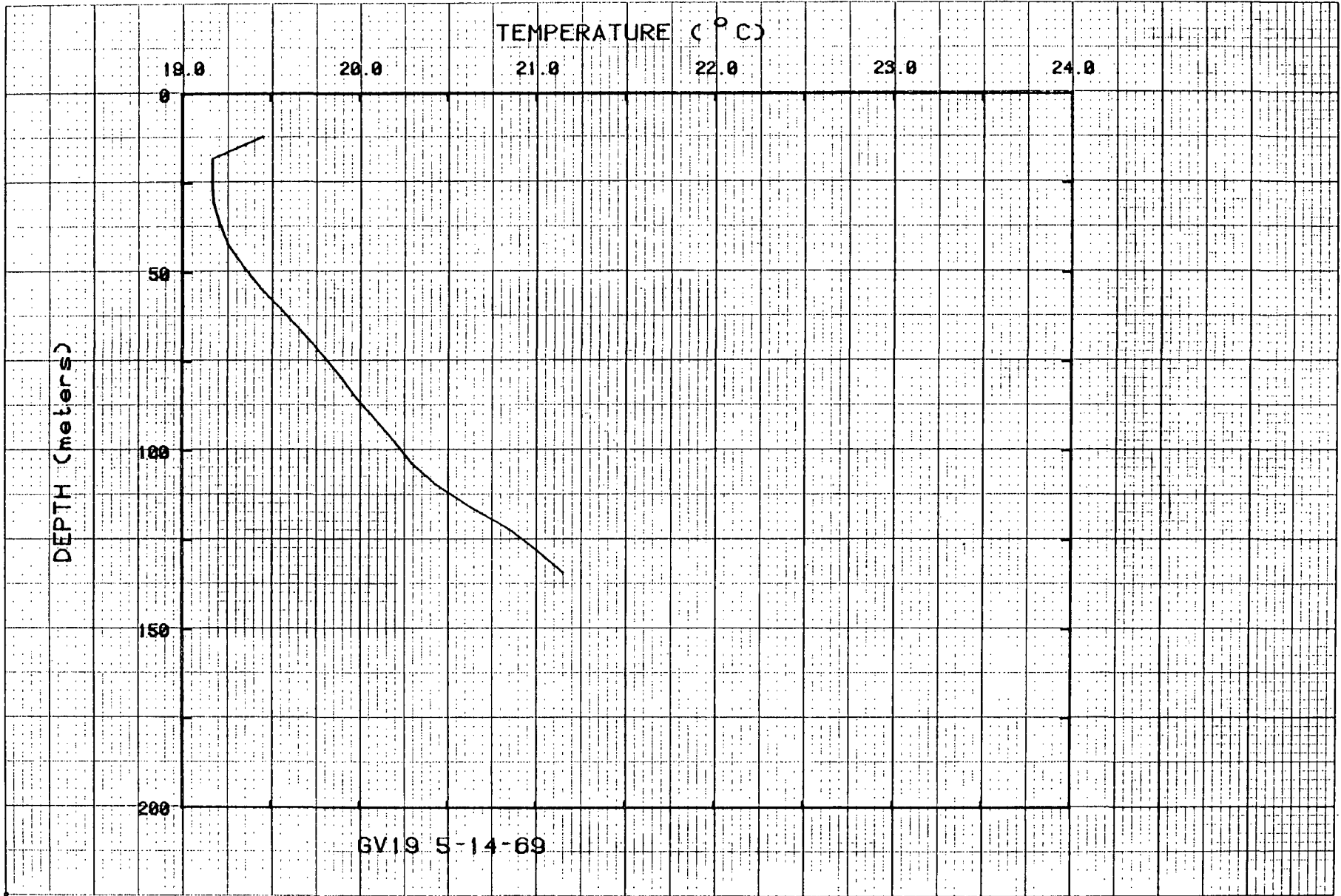
Figure 27. Temperatures for hole GV19.
