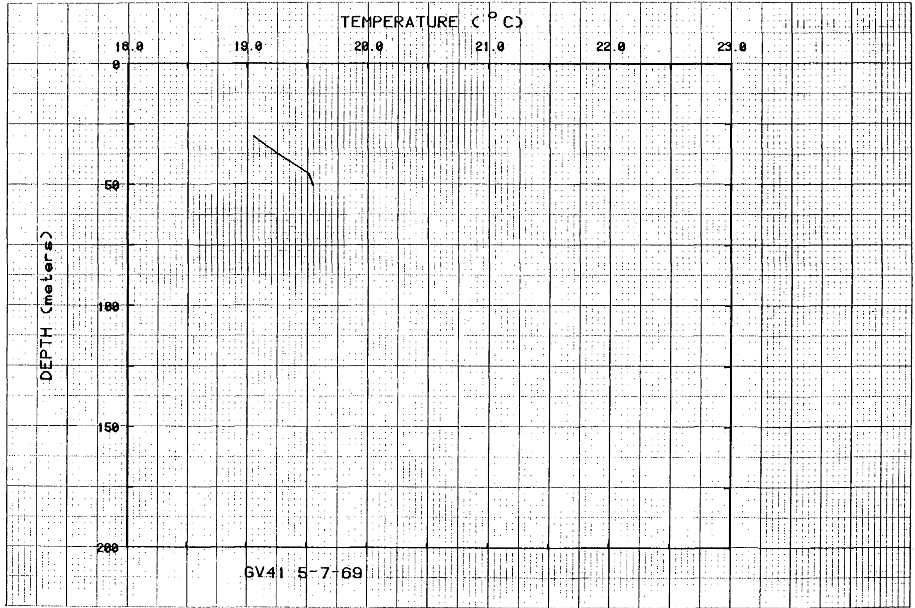
Figure 48. Temperatures in hole GV41.
