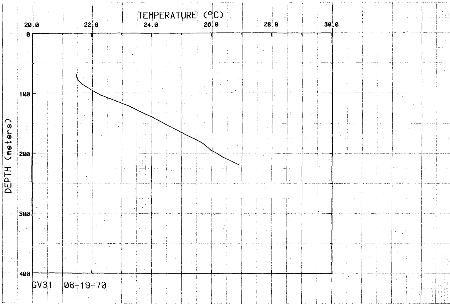
Figure 38. Temperatures for hole GV31.
