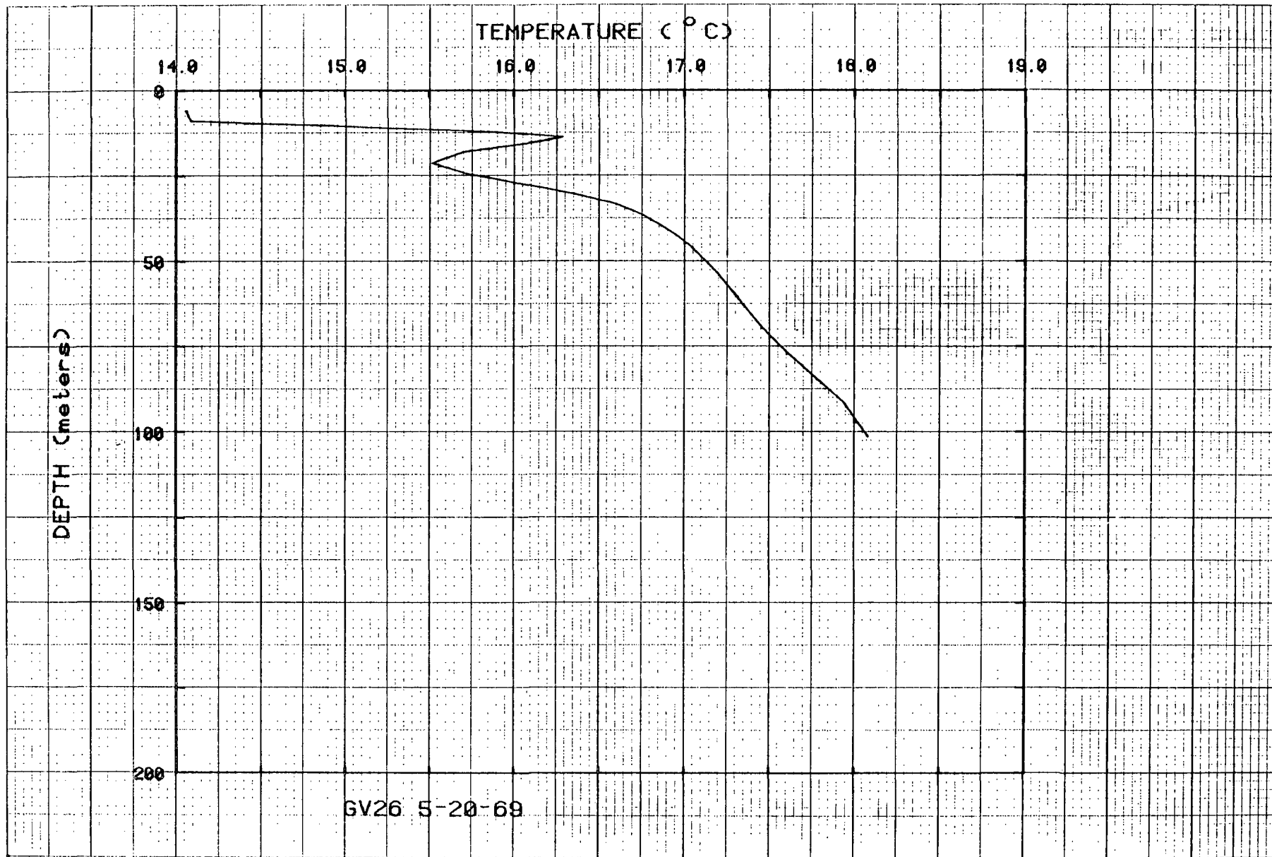
Figure 33. Temperatures for hole GV26.
