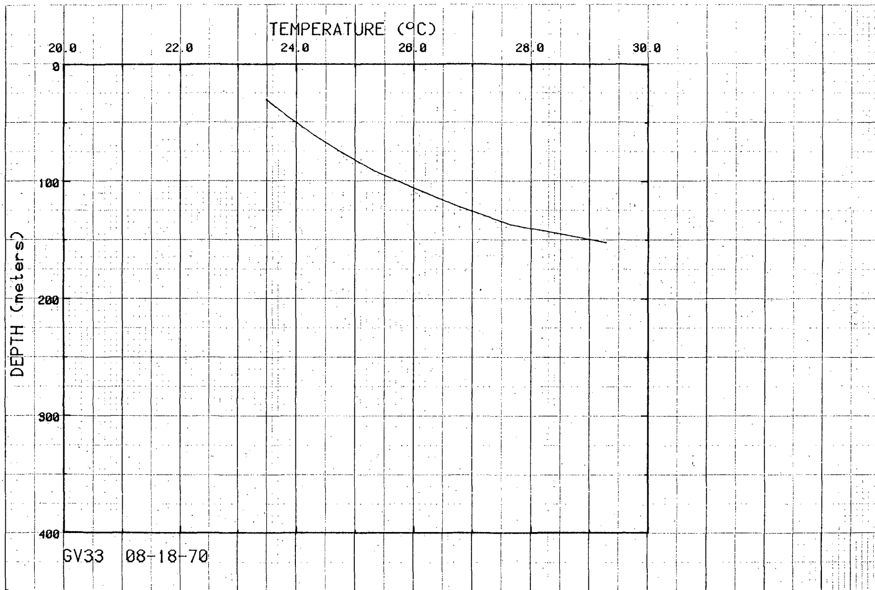
Figure 40. Temperatures for hole GV33.
