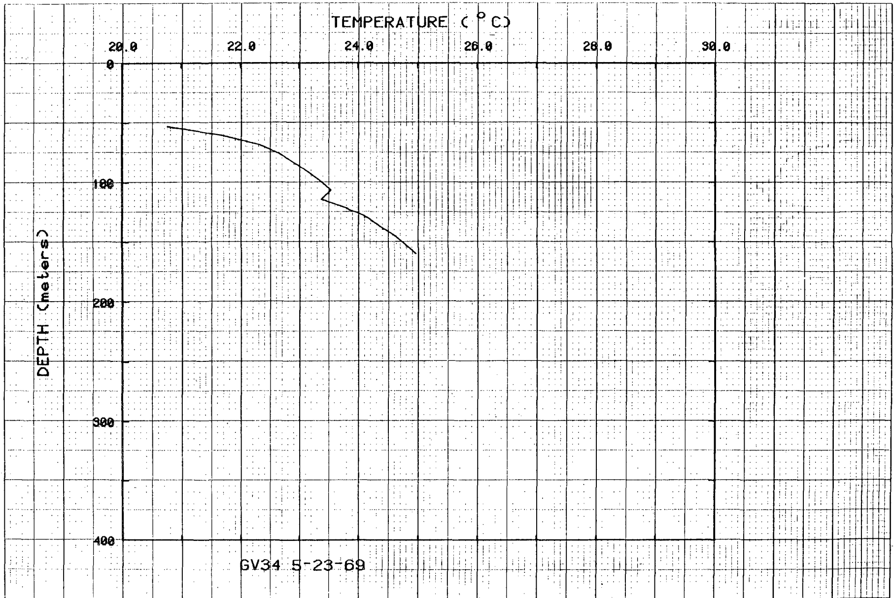
Figure 41. Temperatures for hole GV34.
