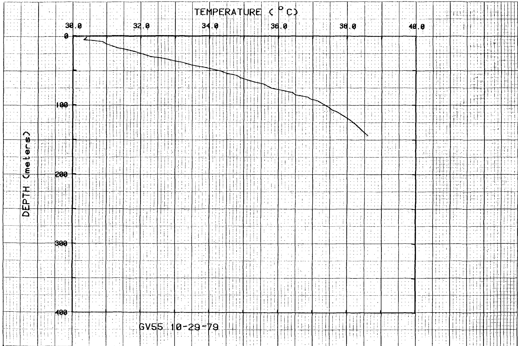
Figure 60. Temperatures for hole GV55.
