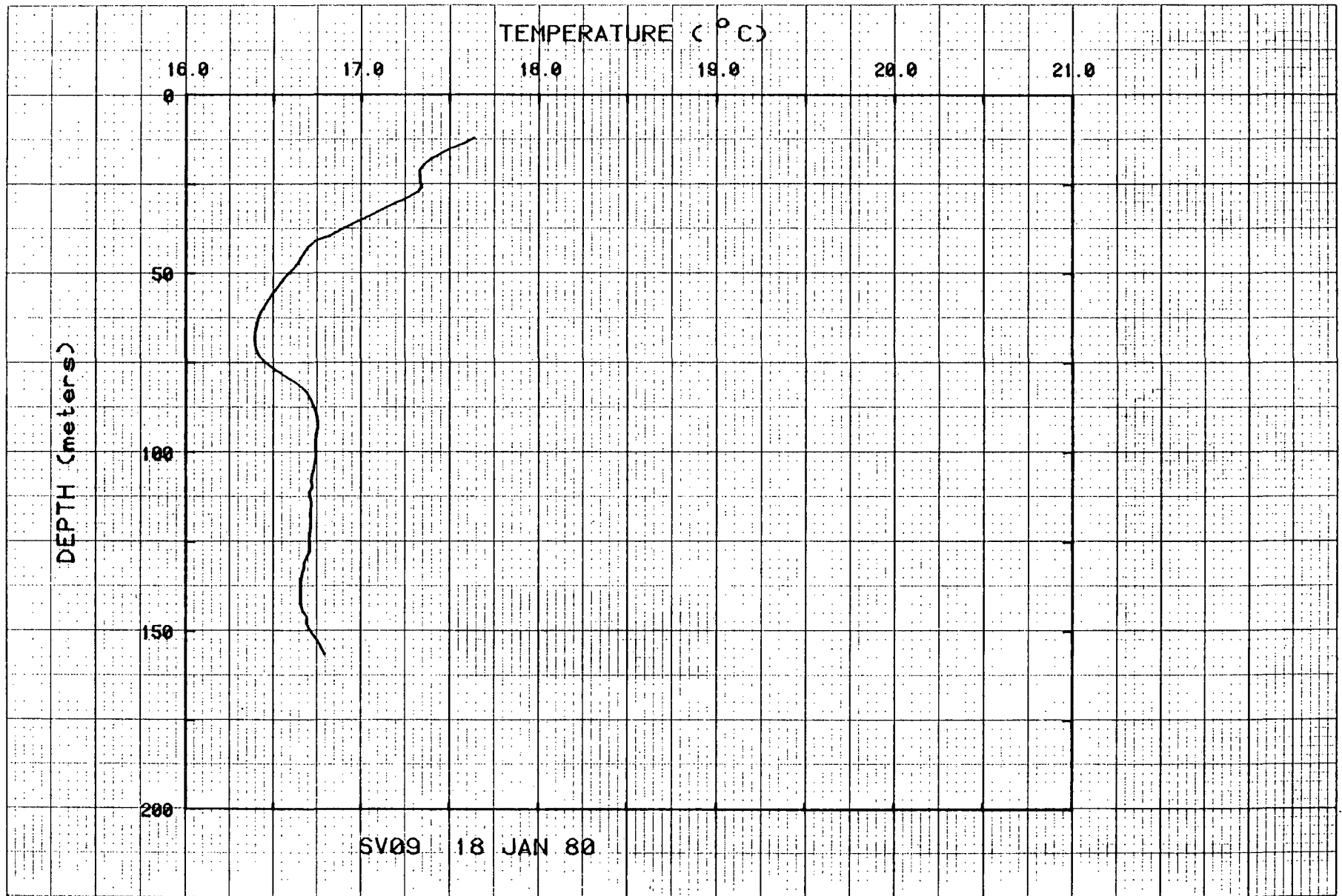
Figure 70. Temperatures for hole SV09.
