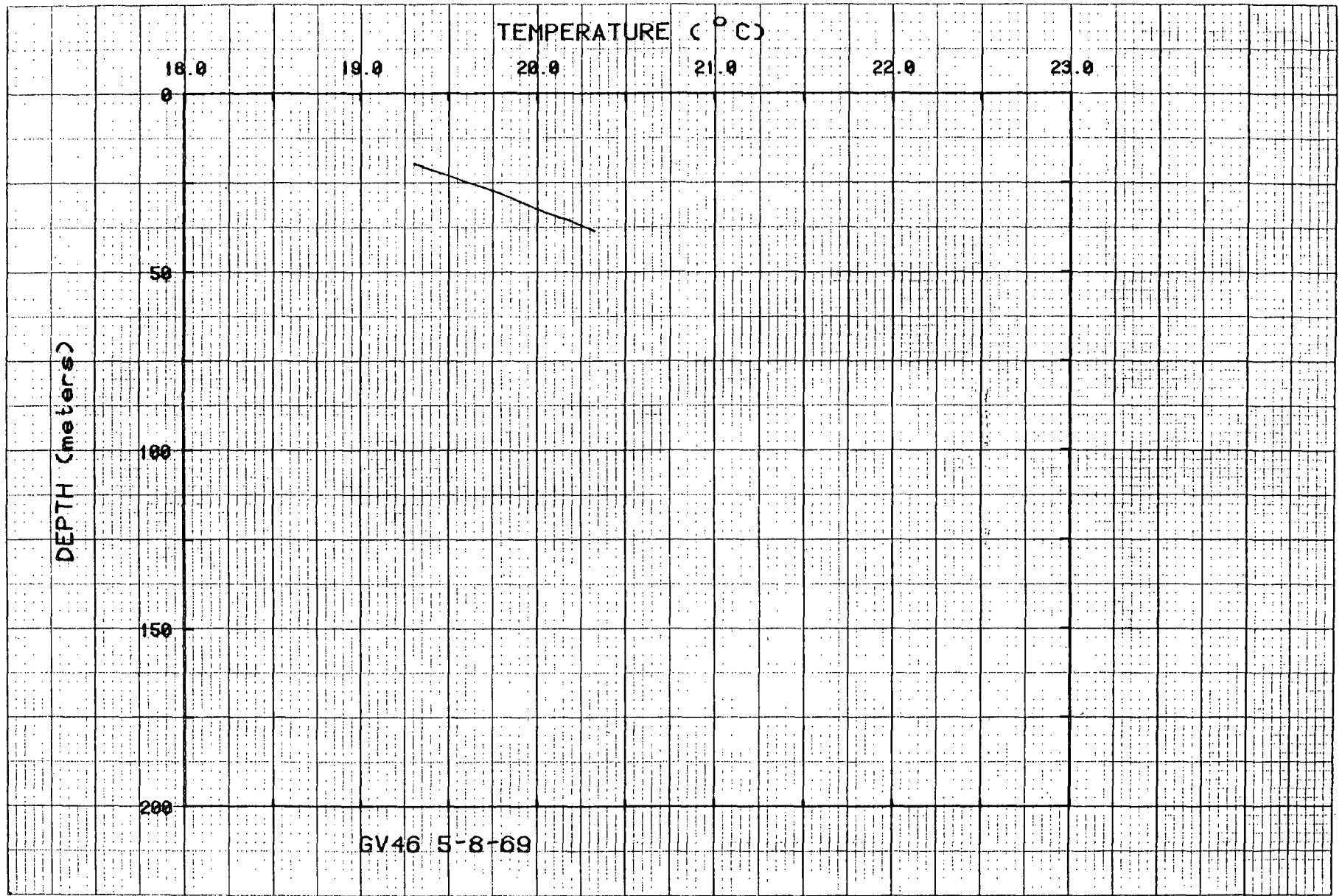
Figure 53. Temperatures for hole GV46.
