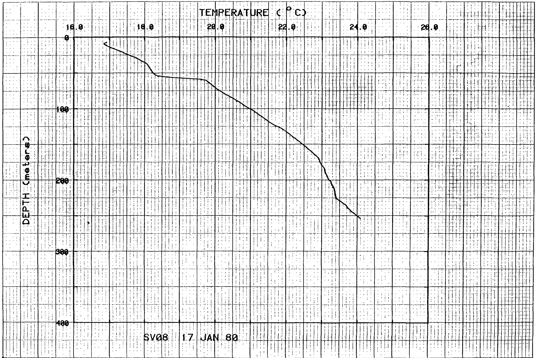
Figure 73. Temperatures for hole SV08.
