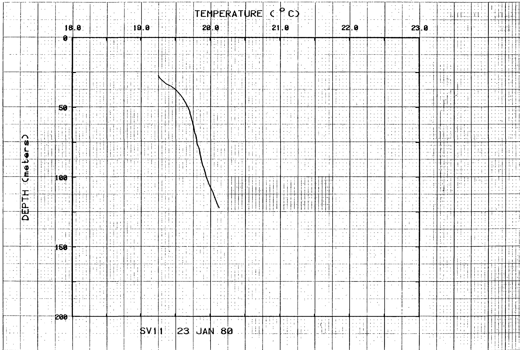
Figure 74. Temperatures for hole SV11.
