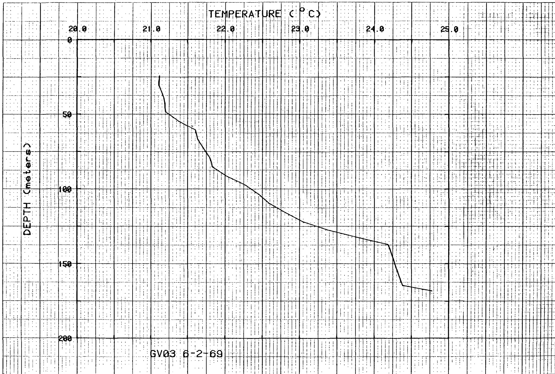
Figure 12. Temperatures for hole GV03.
