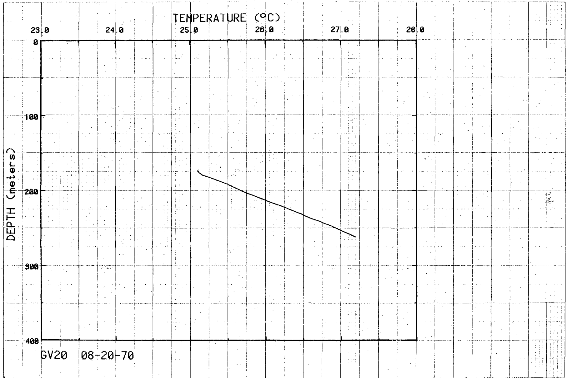
Figure 28. Temperatures for hole GV20.
