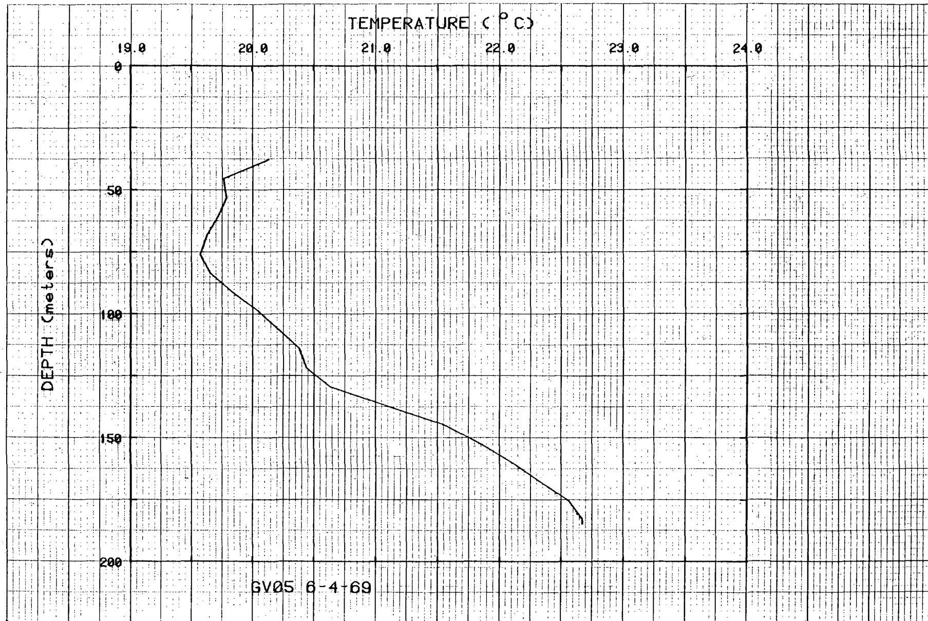
Figure 14. Temperatures for hole GV05.
