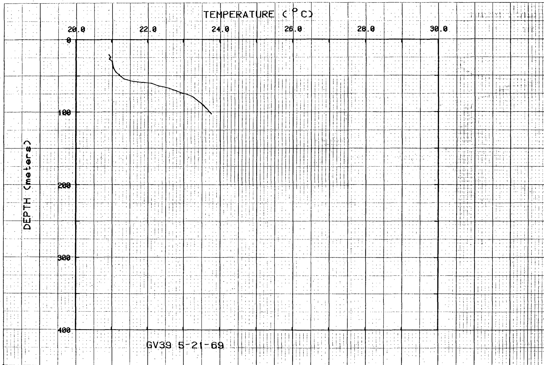
Figure 46. Temperatures for hole GV39.
