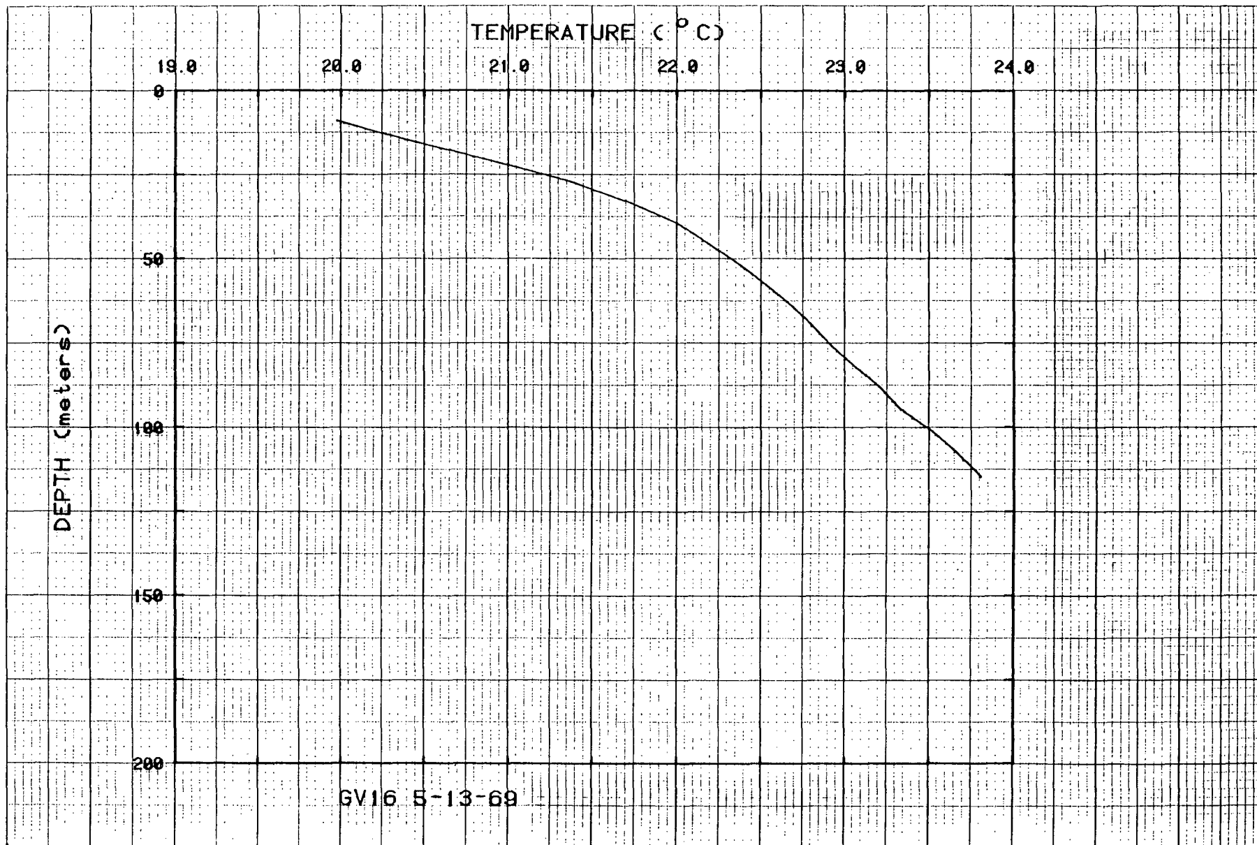
Figure 24. Temperatures for hole GV16.
