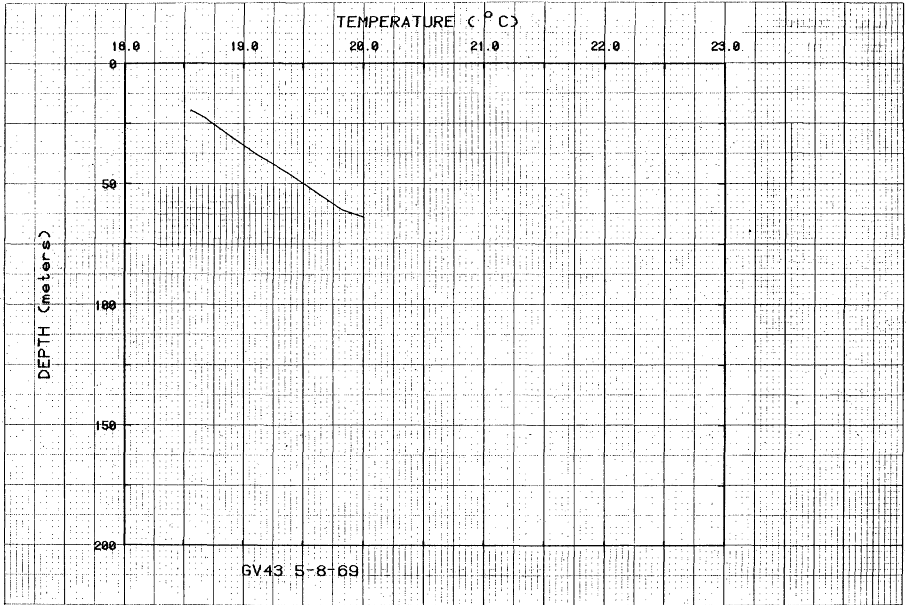
Figure 50. Temperatures for hole GV43.
