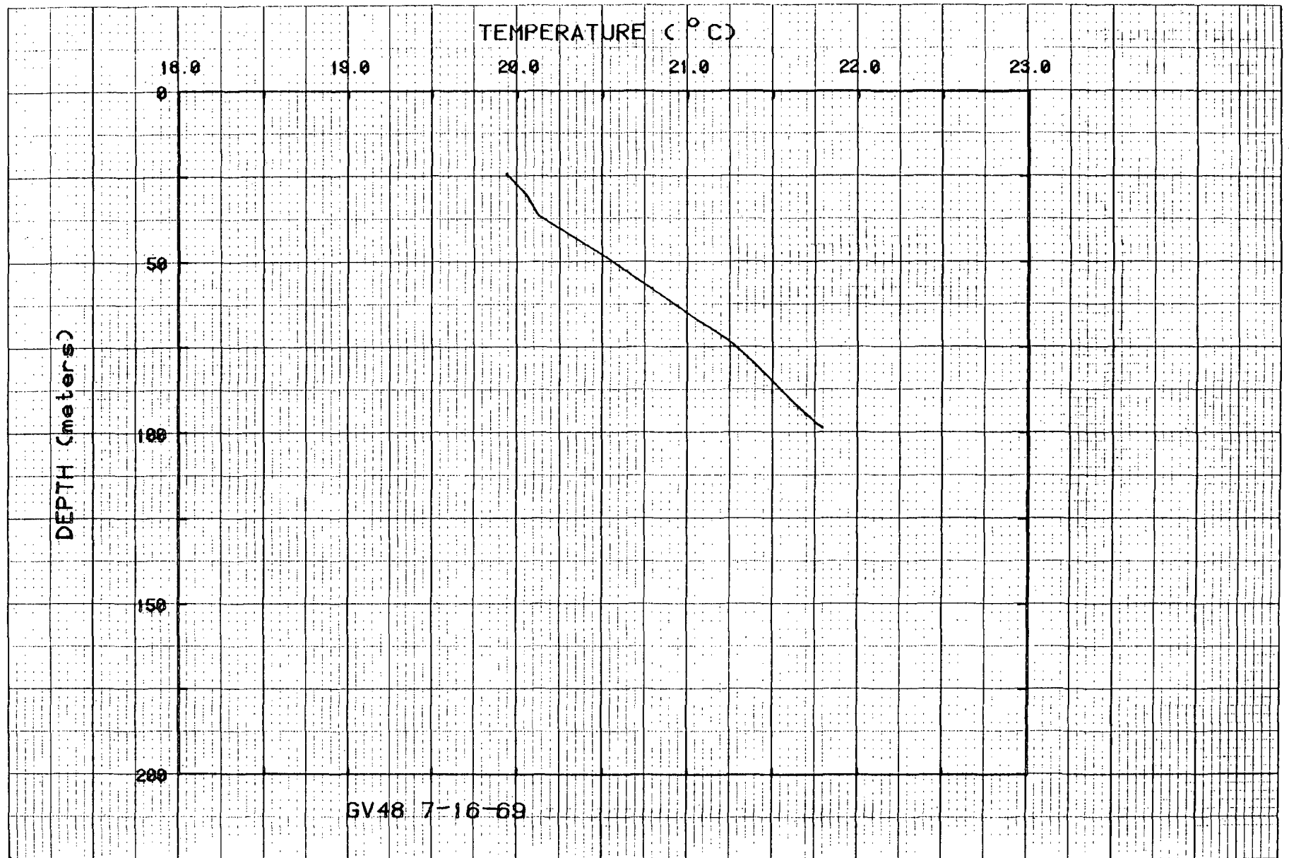
Figure 55. Temperatures for hole GV48.
