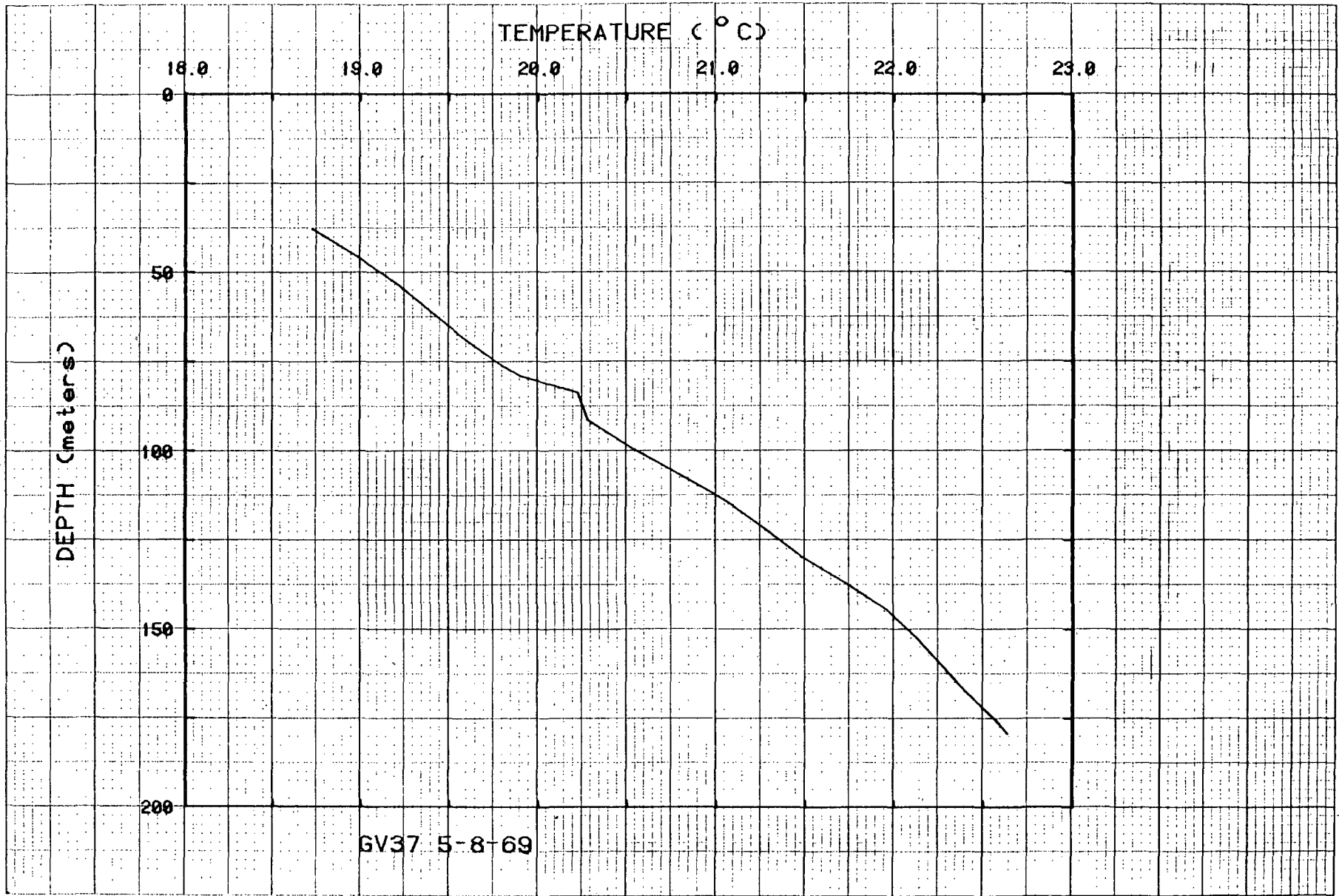
Figure 44. Temperatures for hole GV37.
