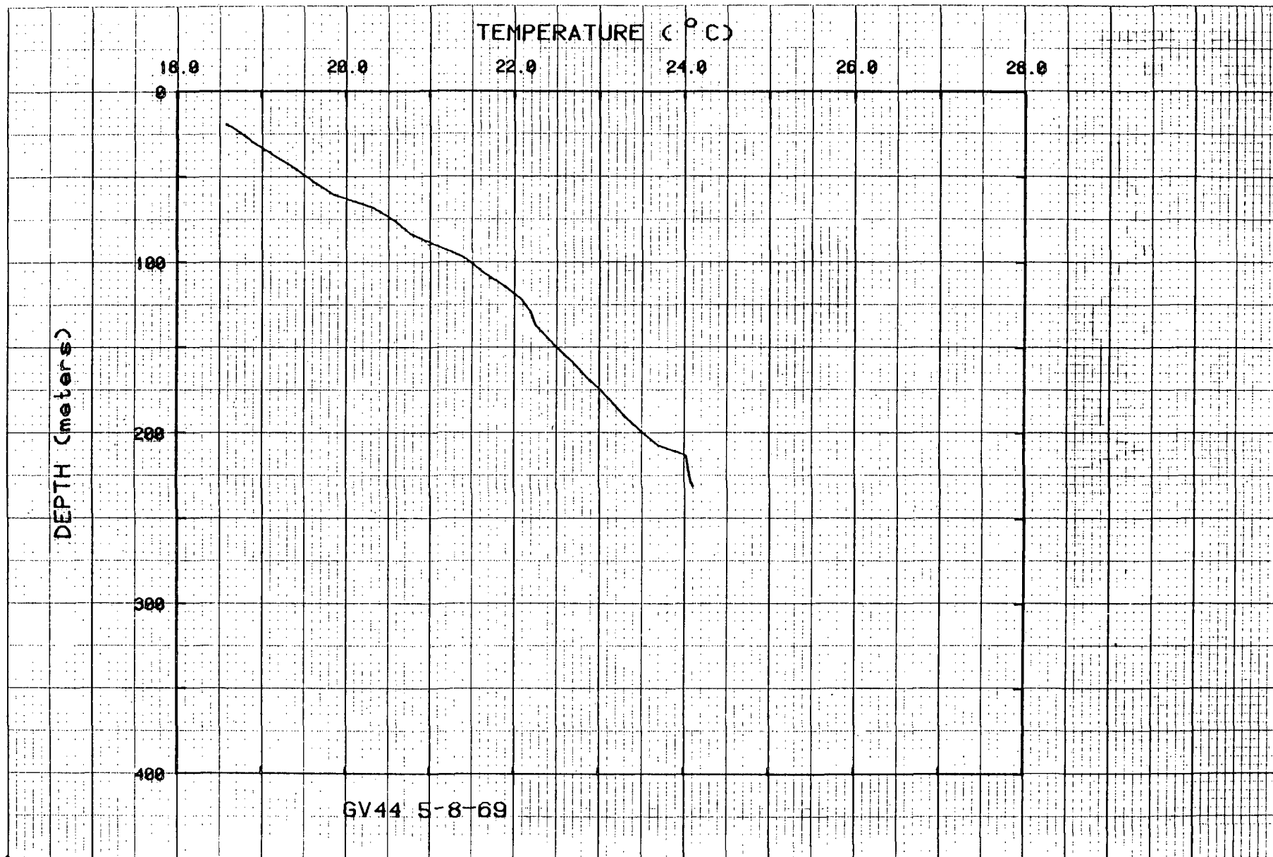
Figure 51. Temperatures for hole GV44.
