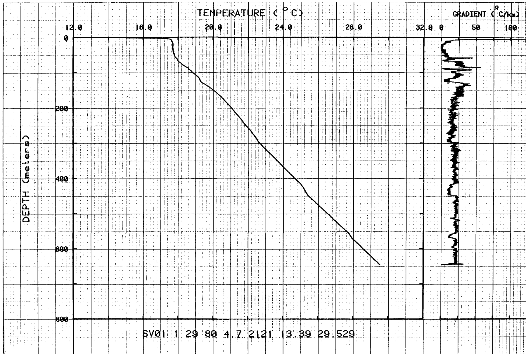
Figure 3. Temperatures and gradients for hole SV01.
