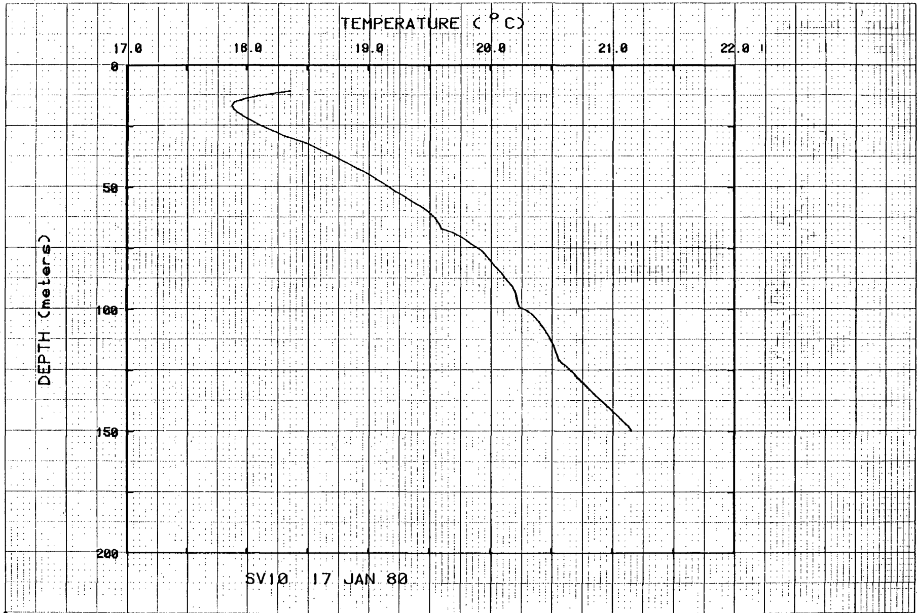
Figure 72. Temperatures for hole SV10.
