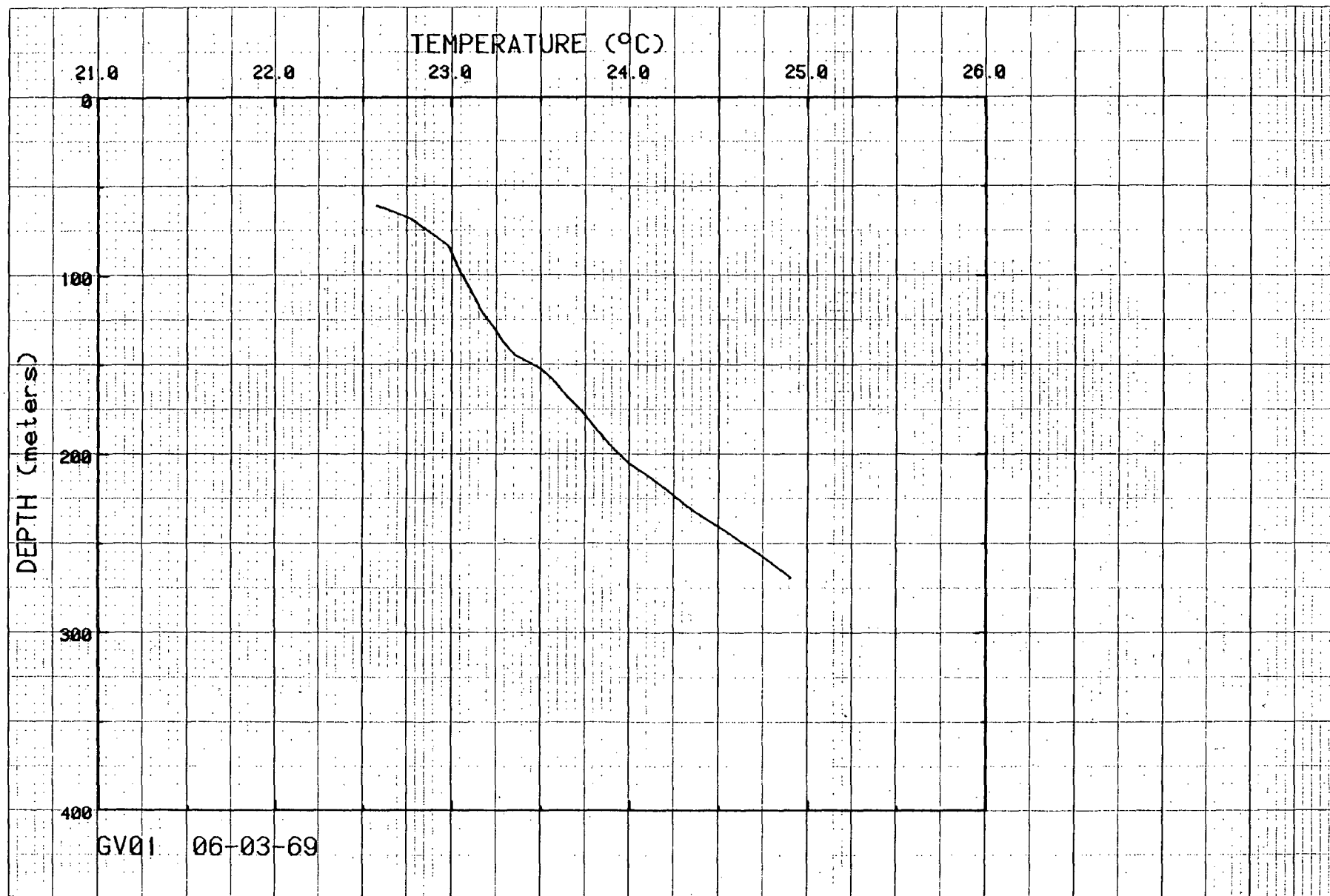
Figure 10. Temperatures for hole GV01.
