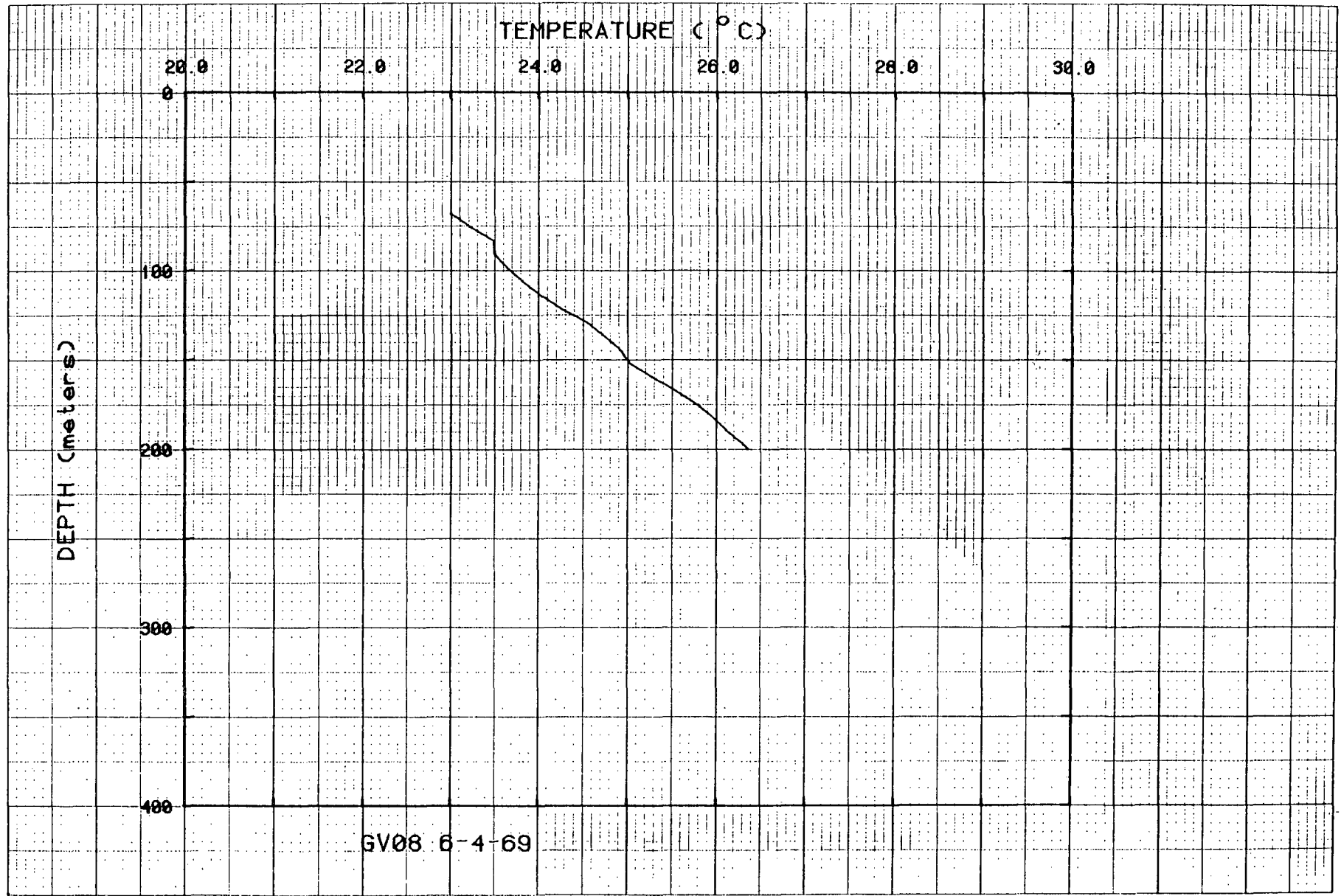
Figure 17. Temperatures for hole GV08.
