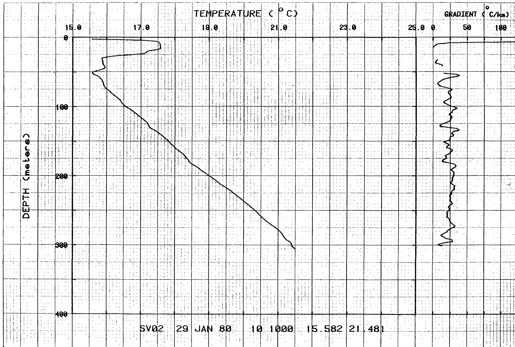
Figure 4. Temperatures and gradients for hole SV02.
