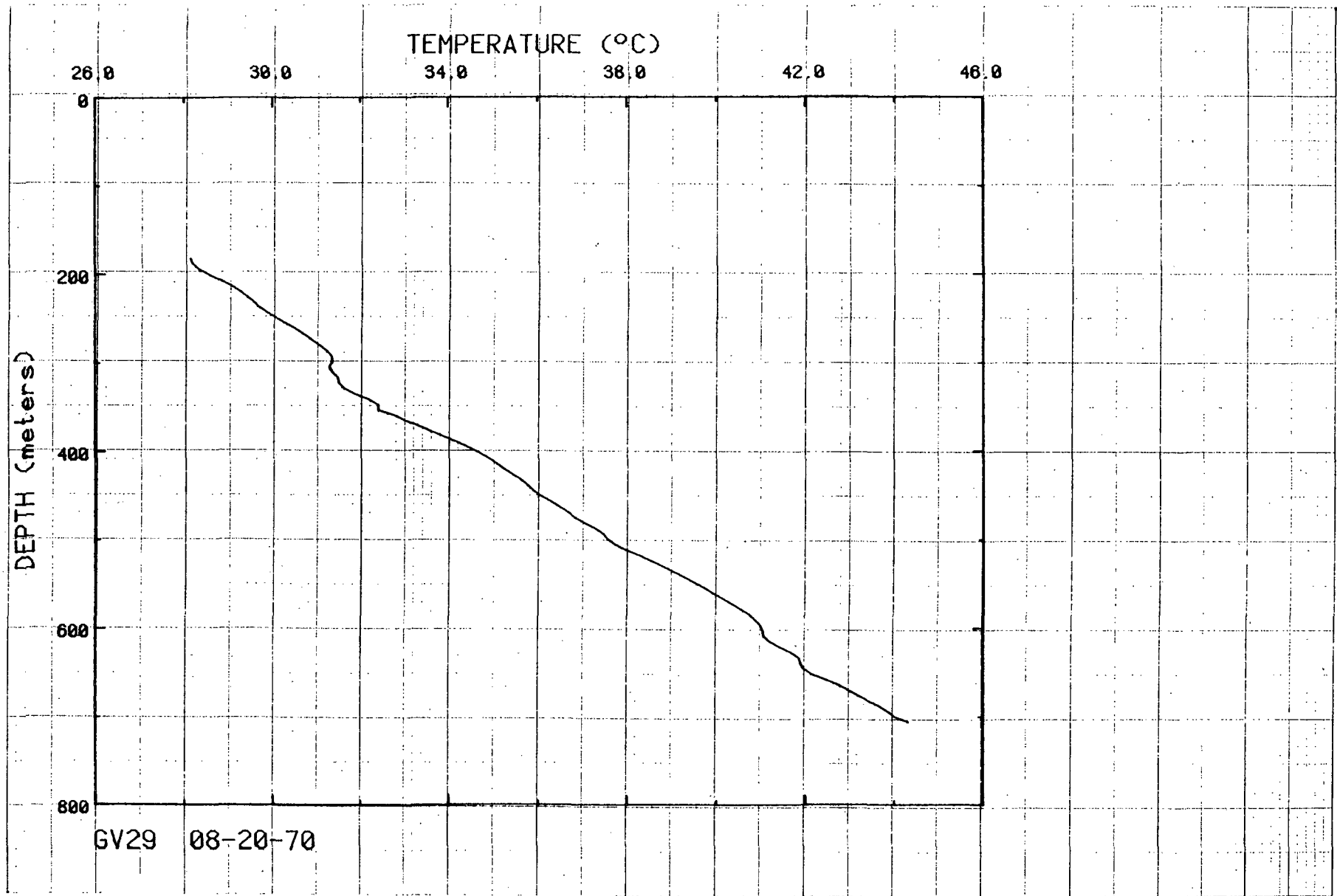
Figure 36. Temperatures for hole GV29.
