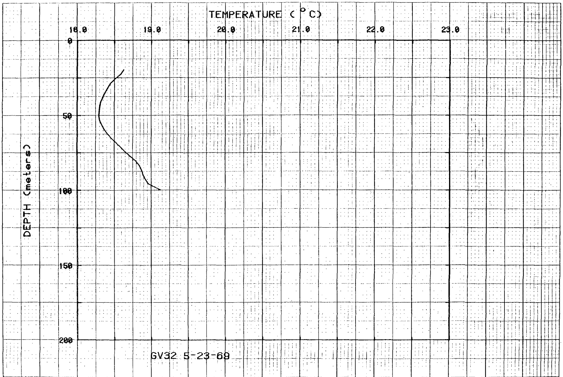
Figure 39. Temperatures for hole GV32.
