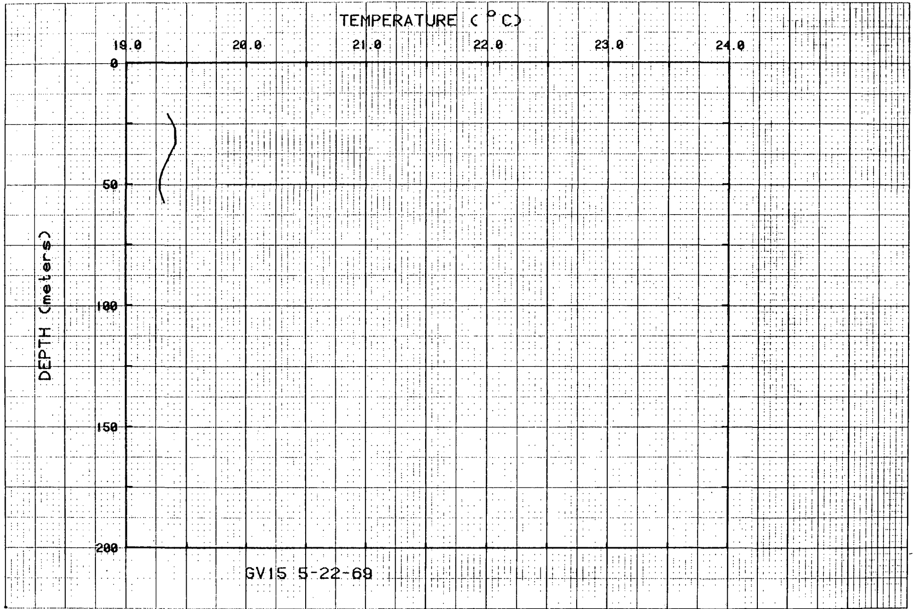
Figure 23. Temperatures for hole GV15.
