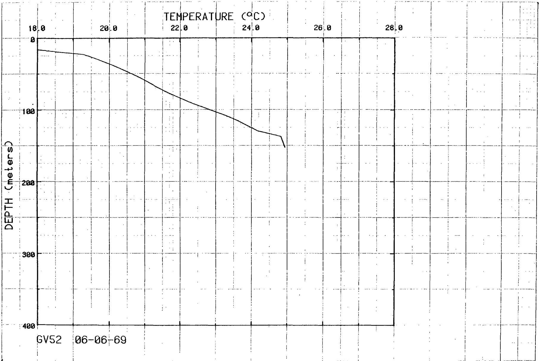
Figure 59. Temperatures for hole GV52.
