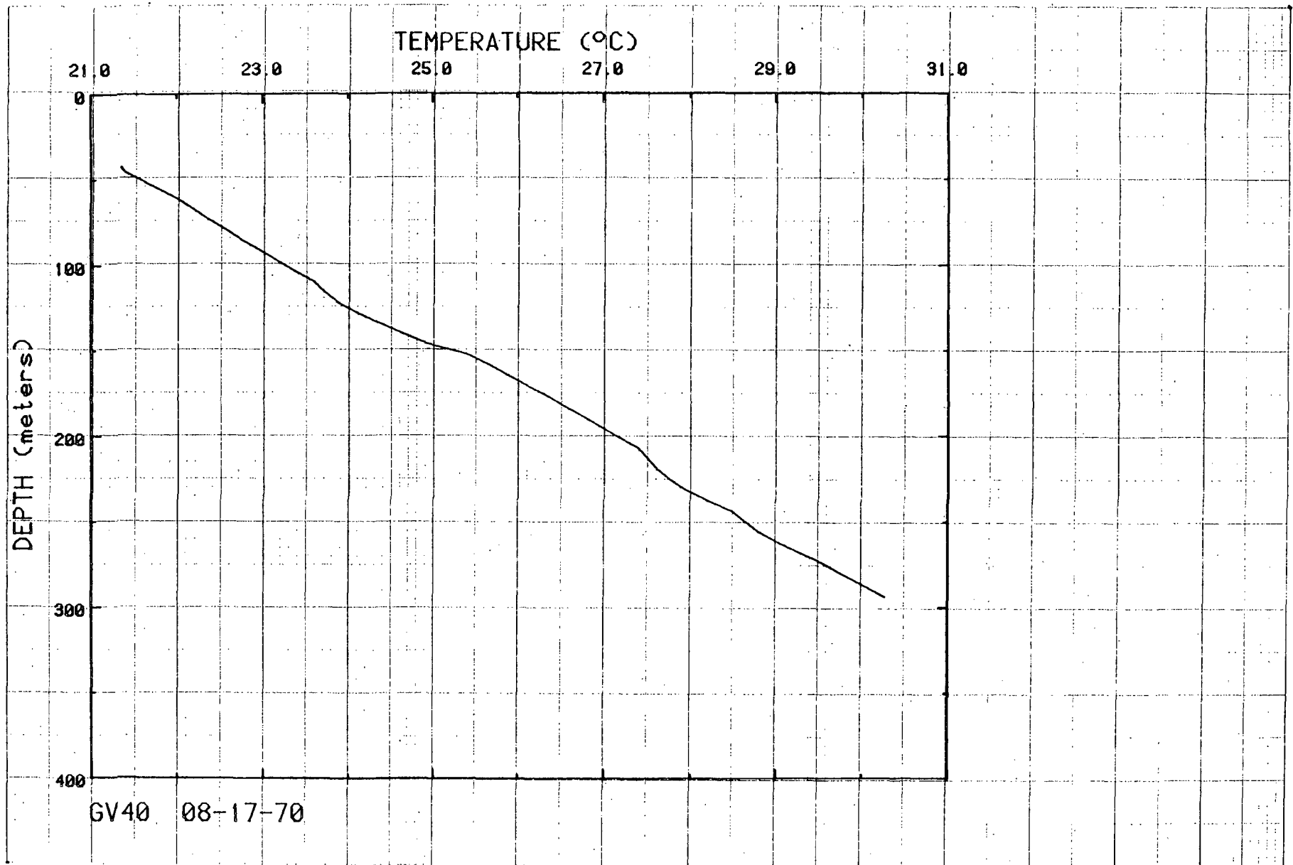
Figure 47. Temperatures for hole GV40.
