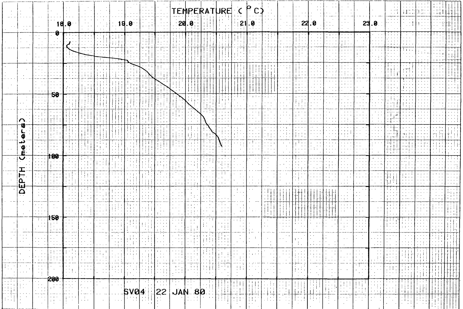
Figure 69. Temperatures for hole SV04.
