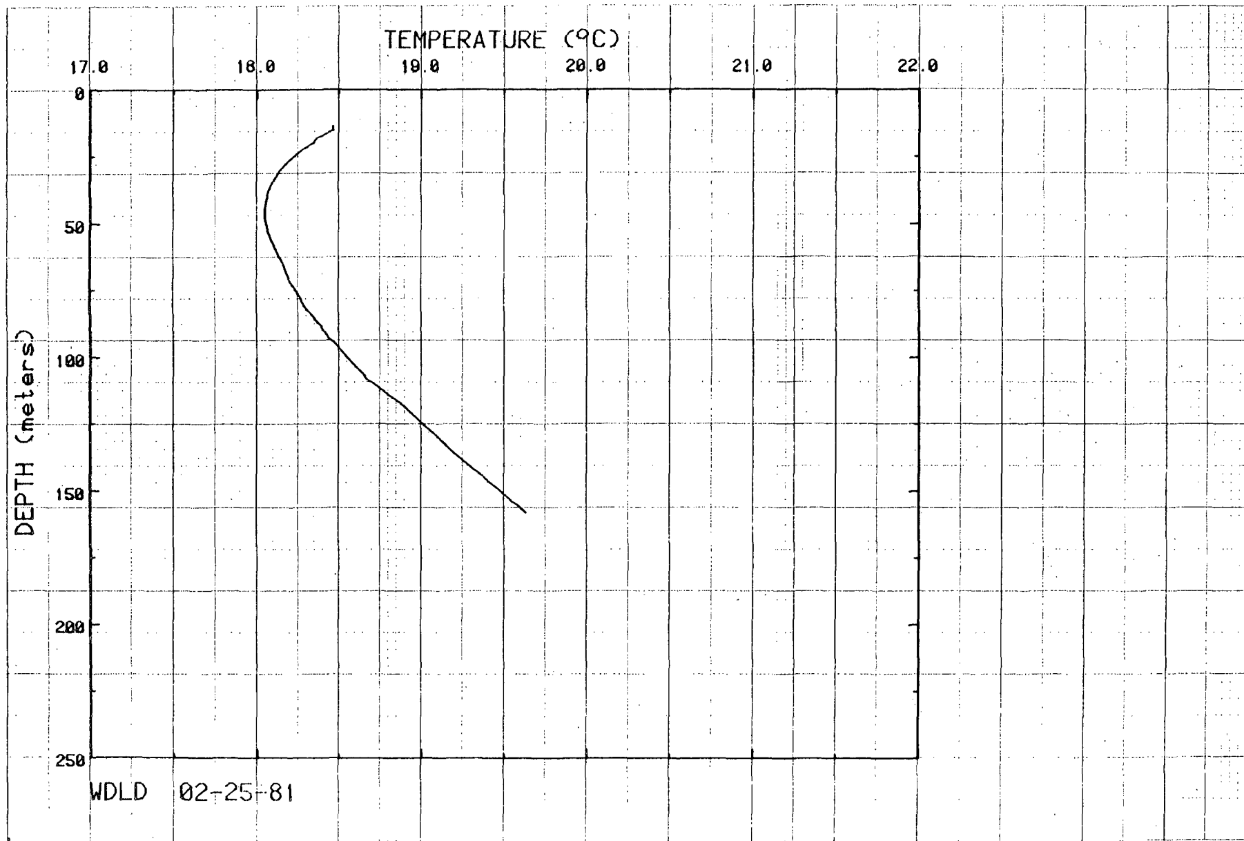
Figure 61. Temperatures for hole WDL D.
