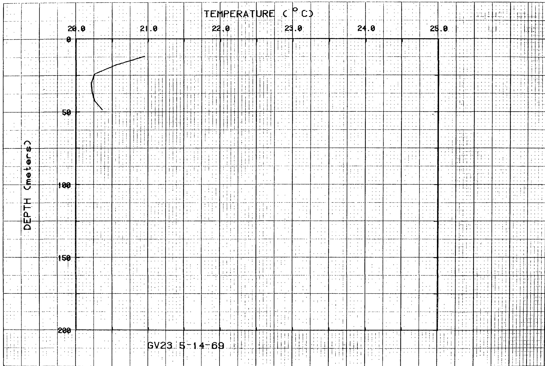
Figure 31. Temperatures for hole GV23.
