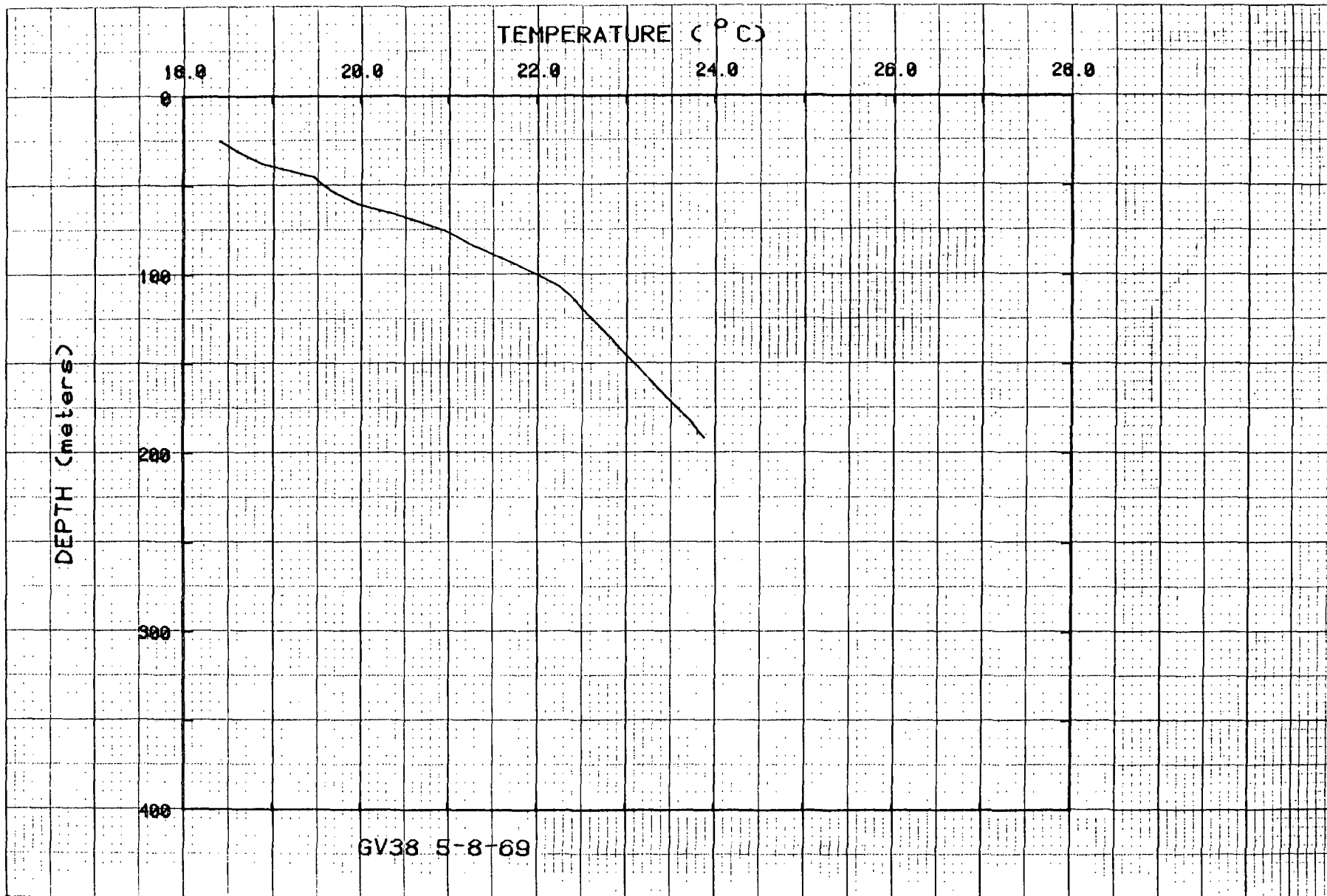
Figure 45. Temperatures for hole GV38.
