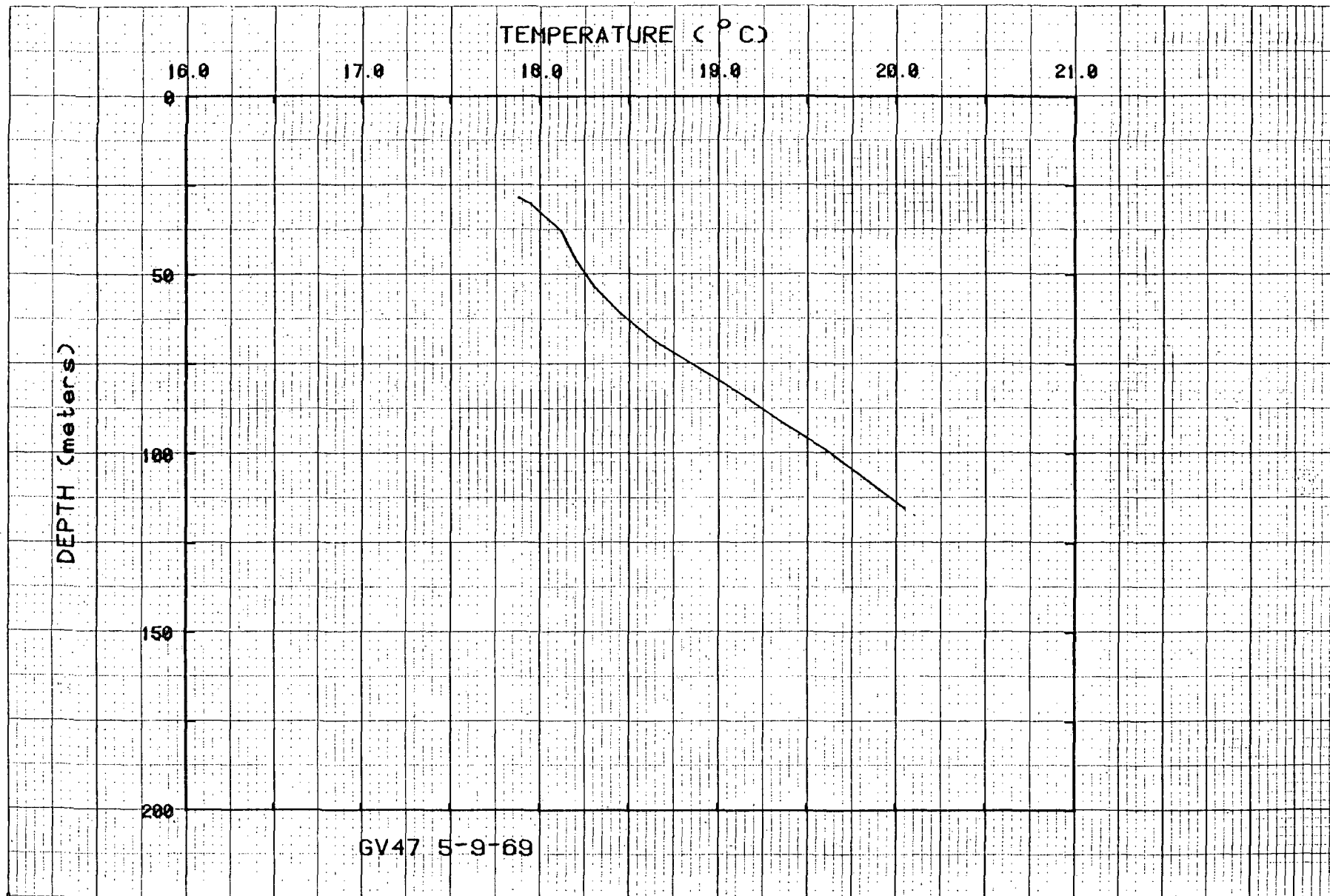
Figure 54. Temperatures for hole GV47.
