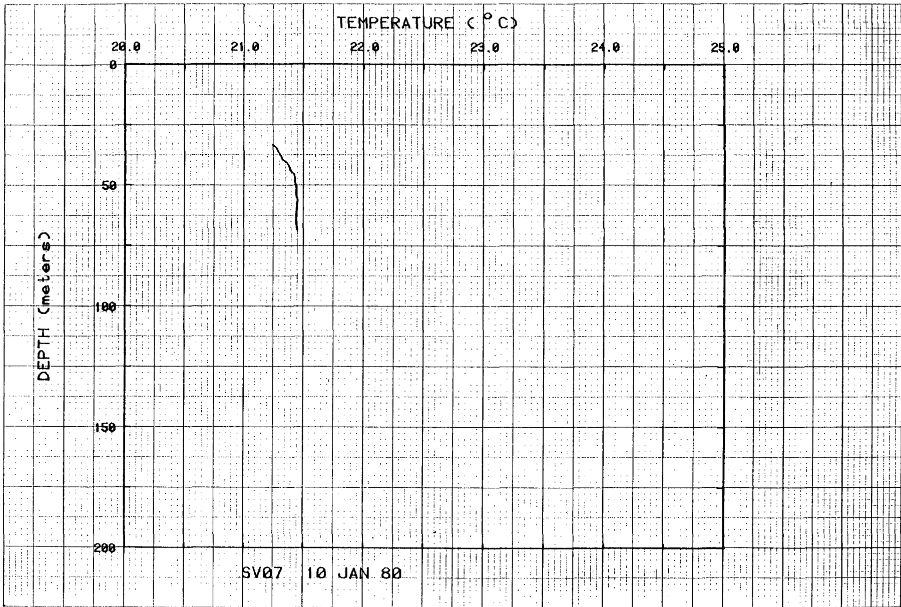
Figure 66. Temperatures for hole SV07.
