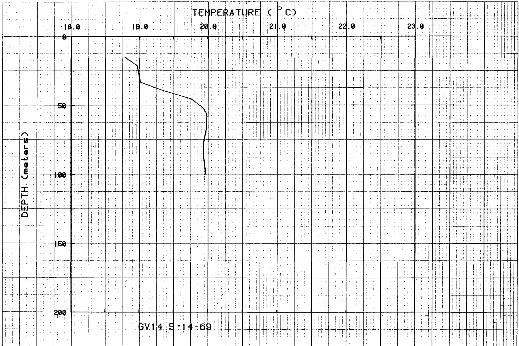
Figure 22. Temperatures for hole GV14.
