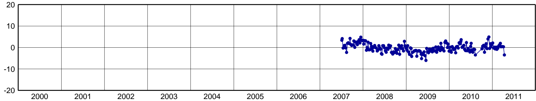
GRE0-North Component [mm]
