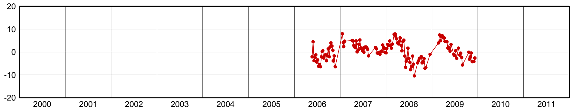
BANS-Up Component [mm]
