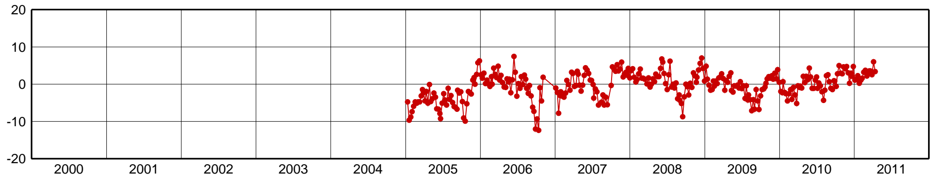
CHIH-Up Component [mm]
