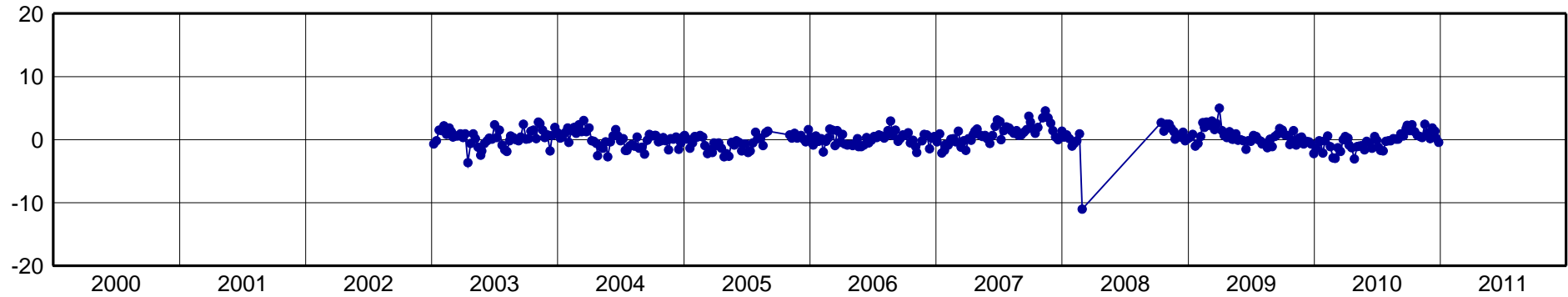
GLPS-North Component [mm]
