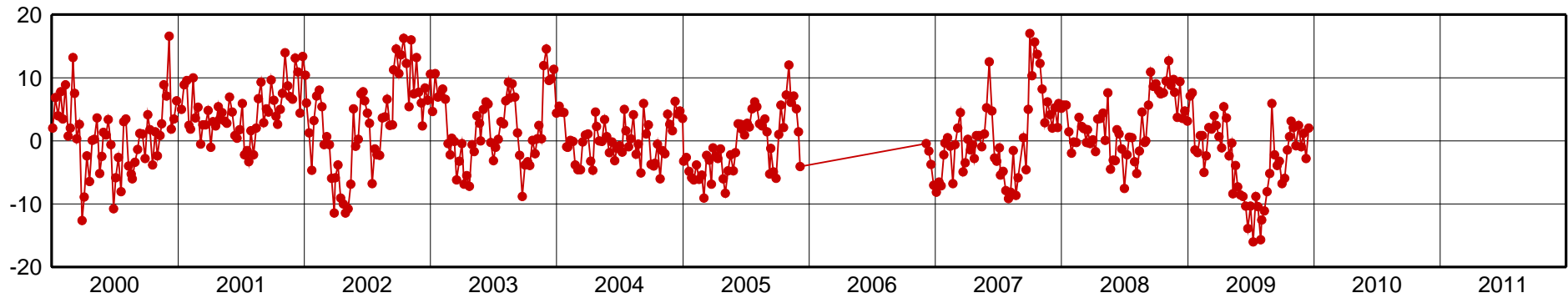
CIC1-Up Component [mm]
