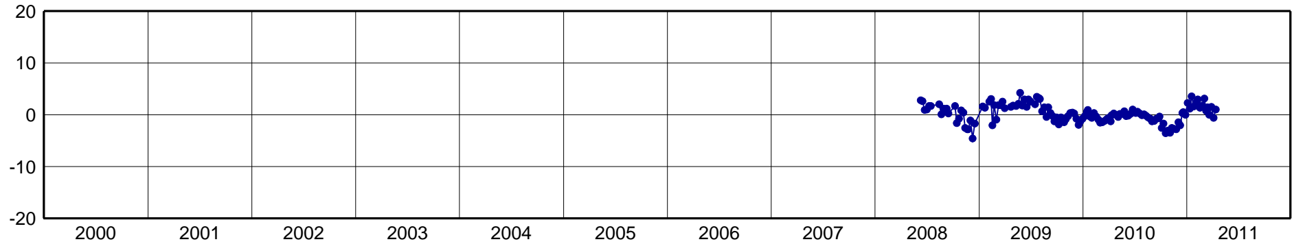
GOJA-North Component [mm]
