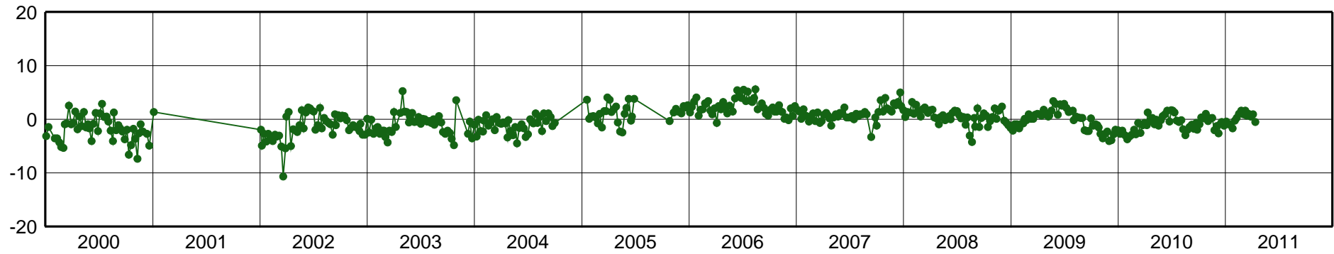
SCUB-East Component [mm]
