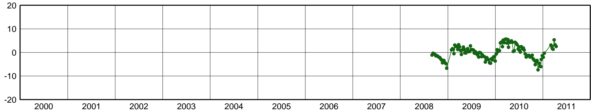
GYEC-East Component [mm]
