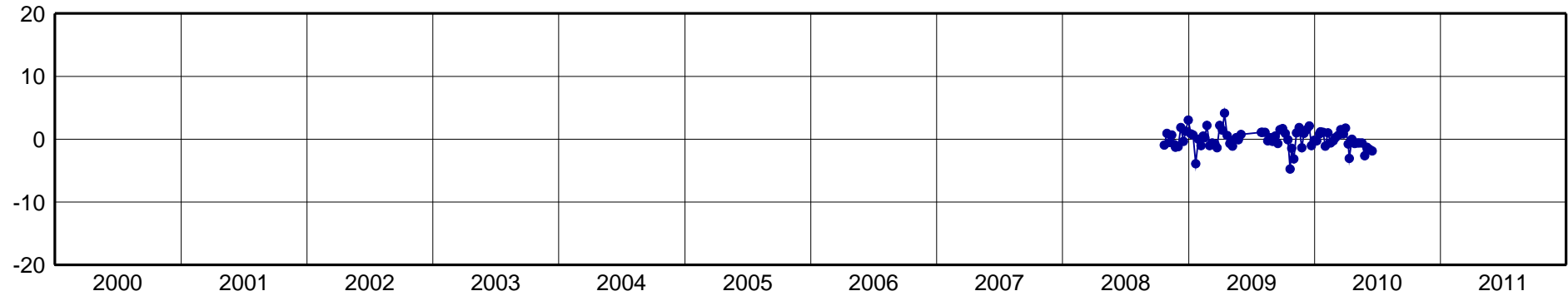
AZUE-North Component [mm]
