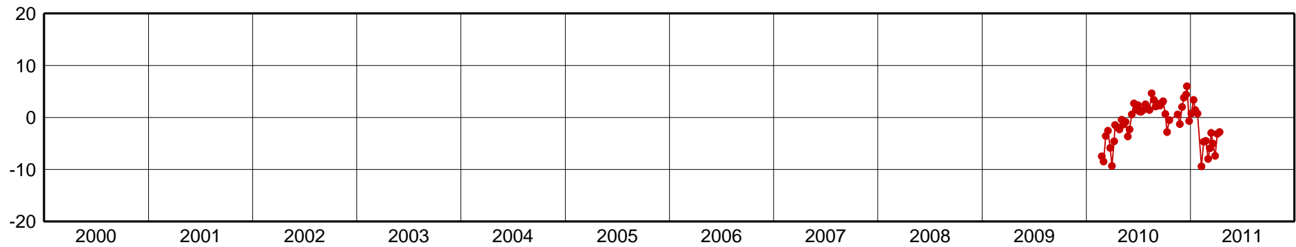
URUS-Up Component [mm]
