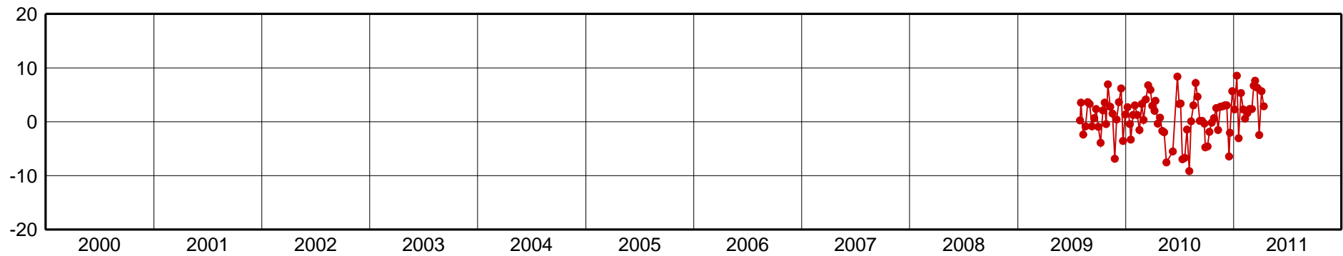
SVIC-Up Component [mm]
