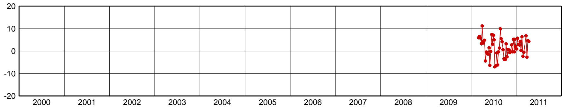
EBYP-Up Component [mm]
