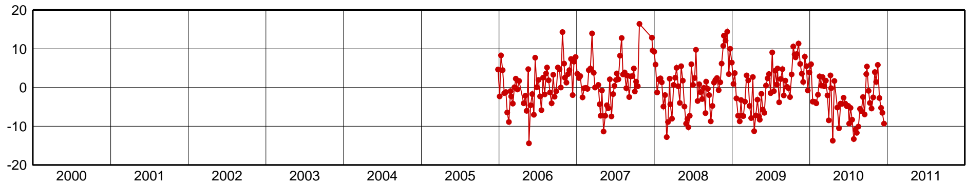
PMB1-Up Component [mm]
