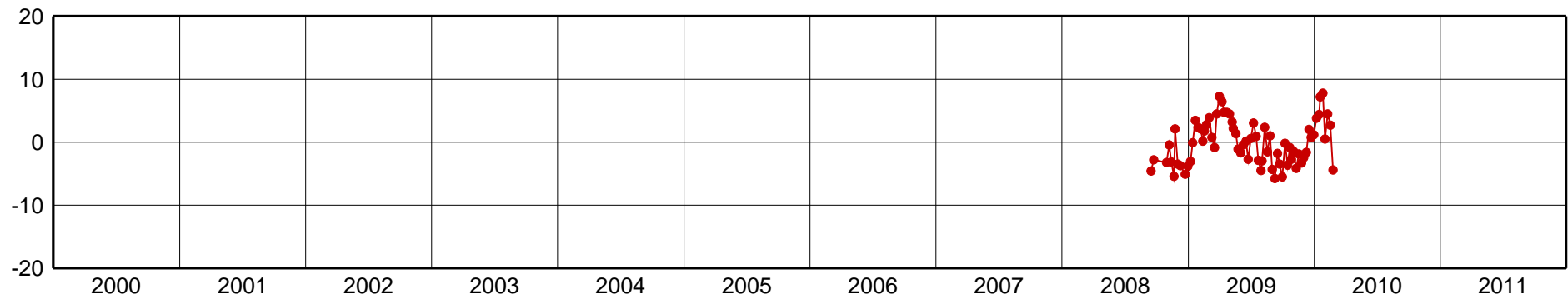
SRLP-Up Component [mm]
