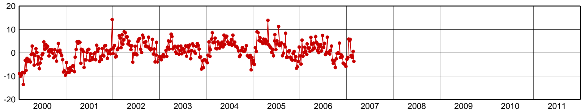
RI OG-Up Component [mm]
