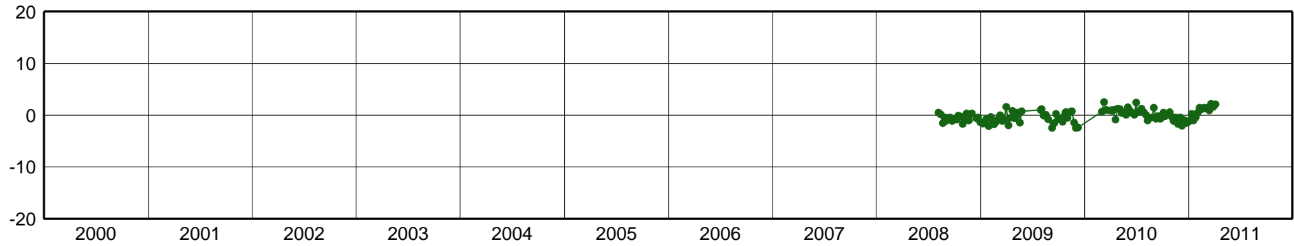
ARCA-East Component [mm]
