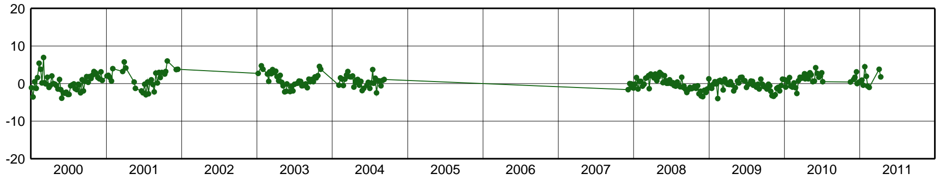
COYQ-East Component [mm]
