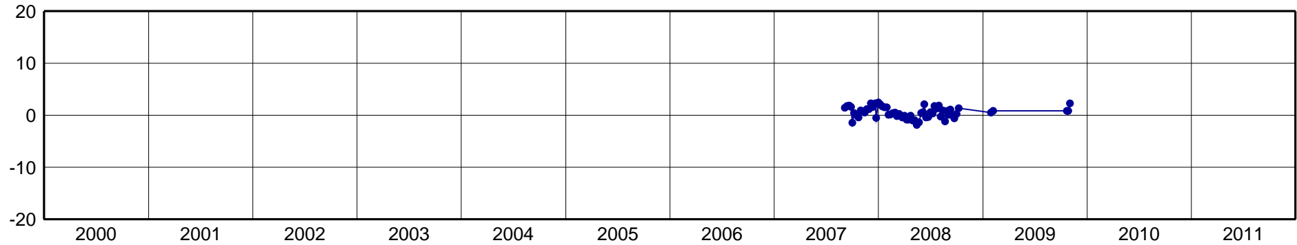
CRUZ-North Component [mm]
