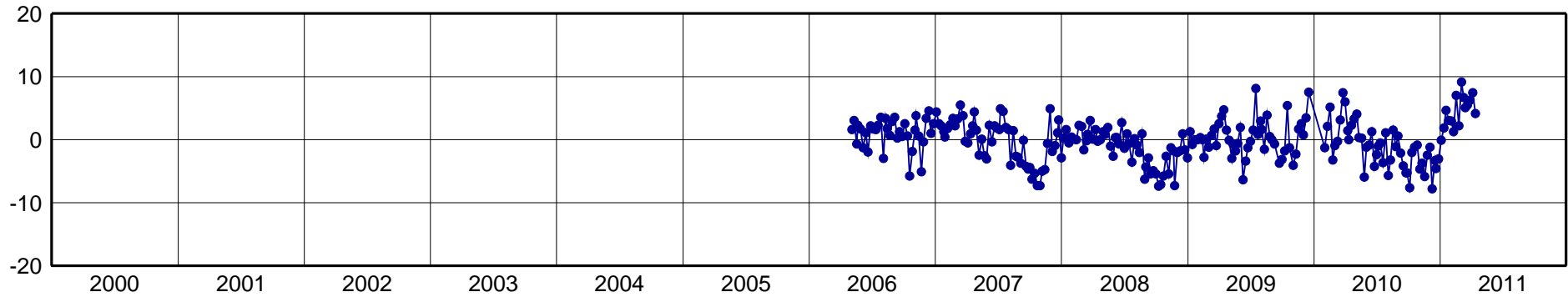
SAMA-North Component [mm]
