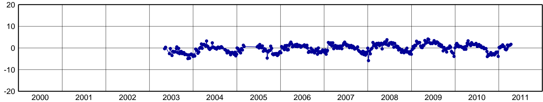
CHPI-North Component [mm]
