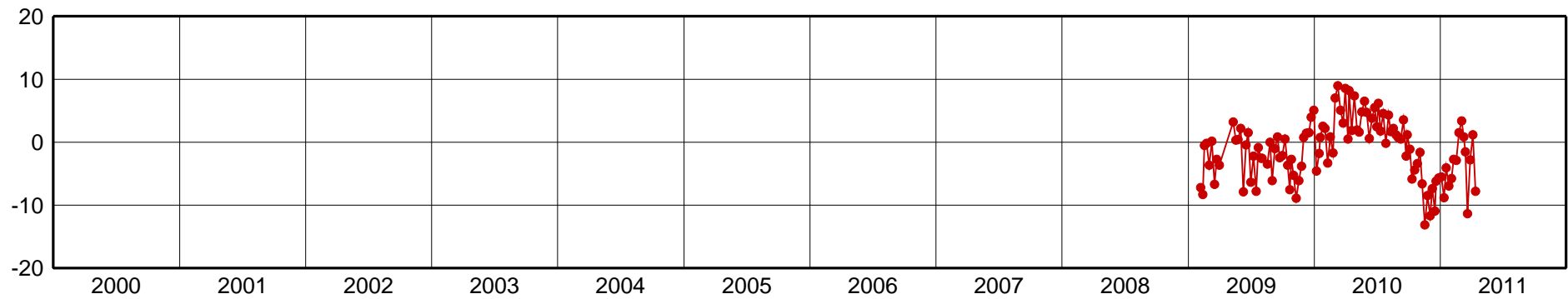
BATF-Up Component [mm]
