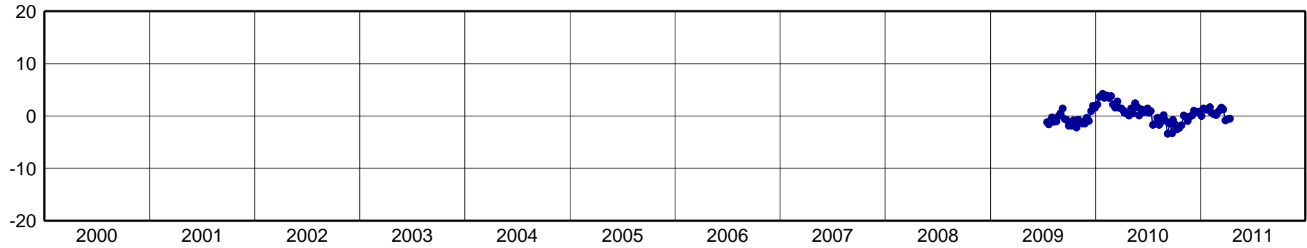
ICEP-North Component [mm]
