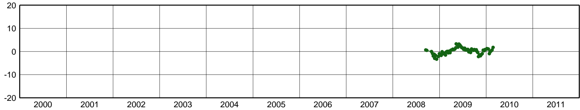
SRLP-East Component [mm]
