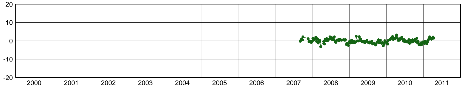
BOAV-East Component [mm]
