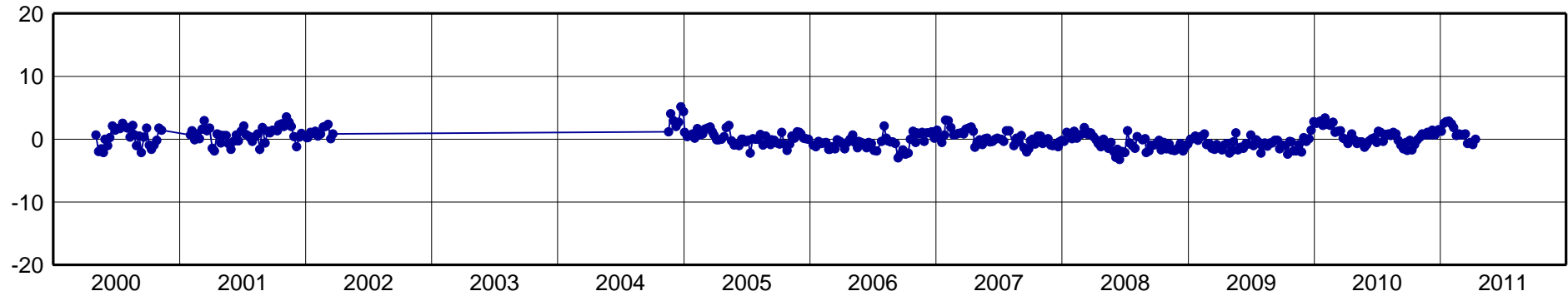
INEG-North Component [mm]
