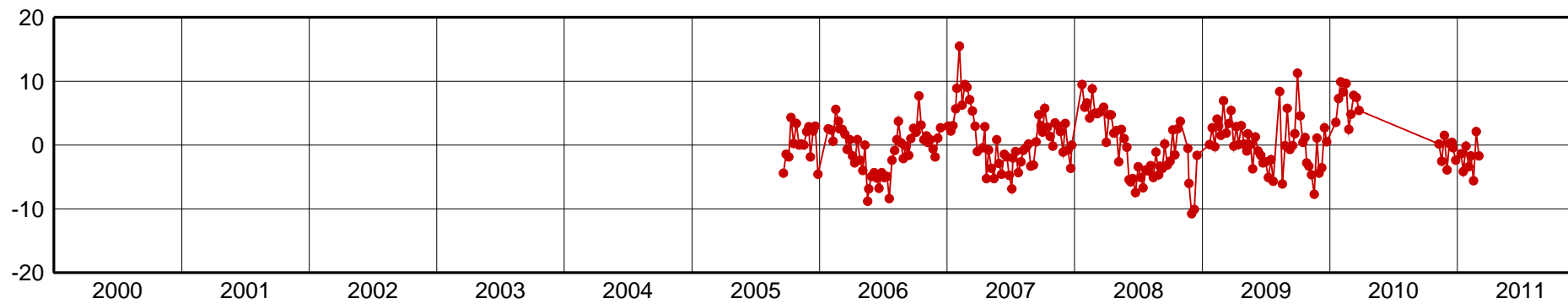
VIVI-Up Component [mm]
