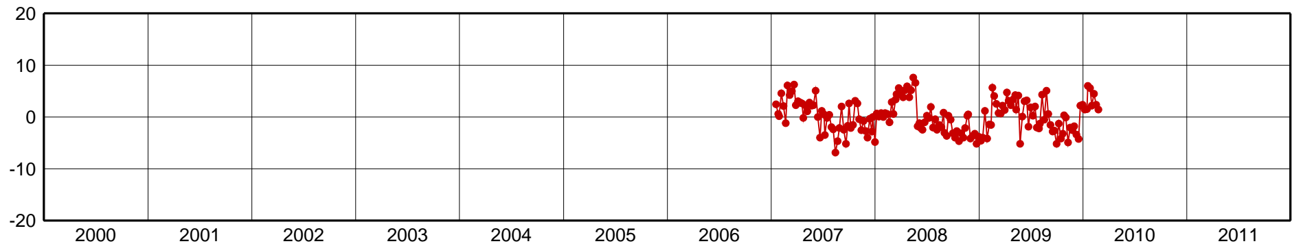
MZAS-Up Component [mm]
