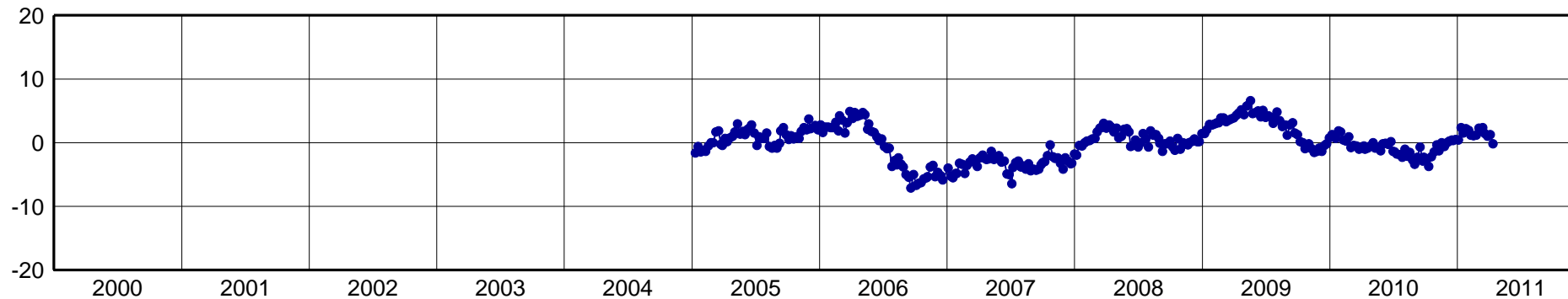
TOL2-North Component [mm]
