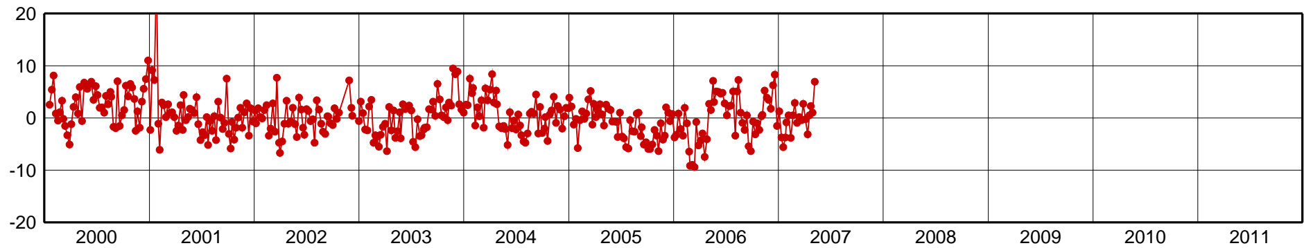
PARA-Up Component [mm]
