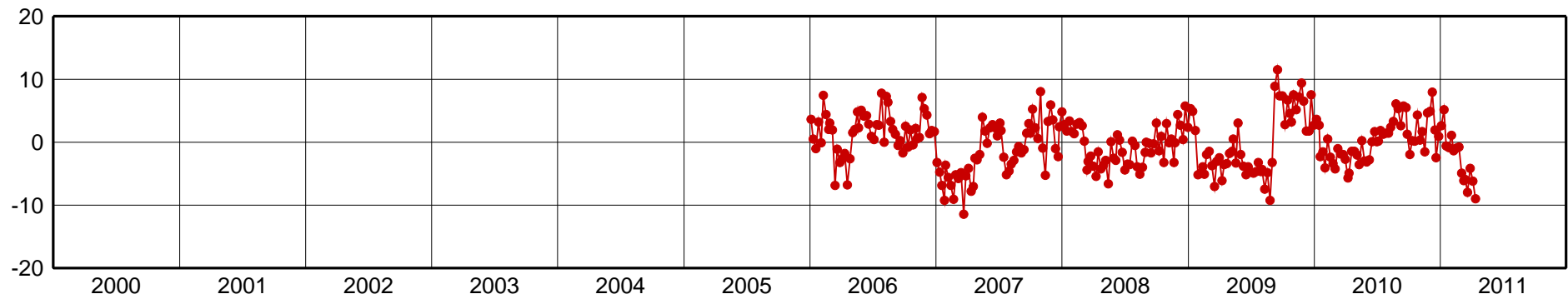
PPTE-Up Component [mm]
