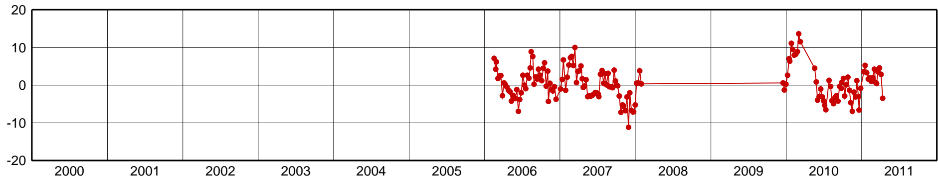
DORA-Up Component [mm]
