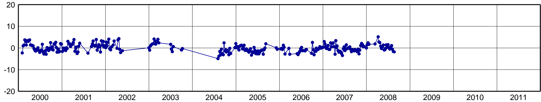
CART-North Component [mm]
