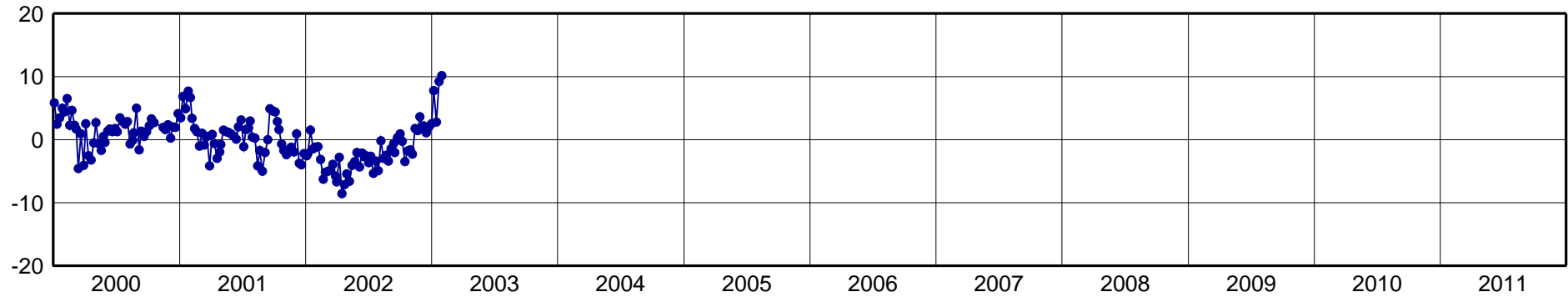
EISL-North Component [mm]
