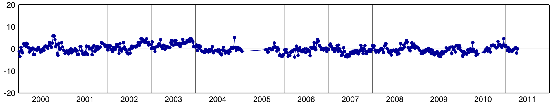
CRO1-North Component [mm]
