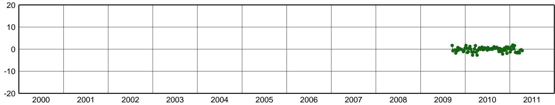
SJRP-East Component [mm]
