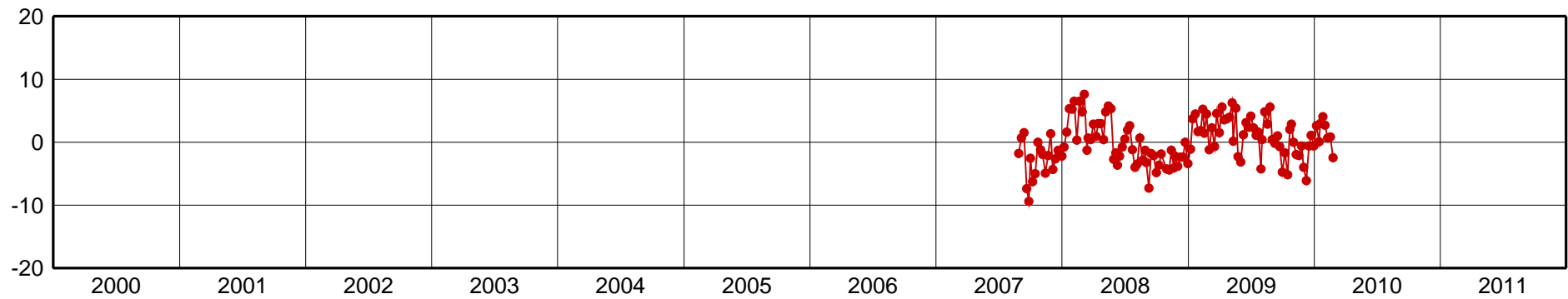
AZUL-Up Component [mm]
