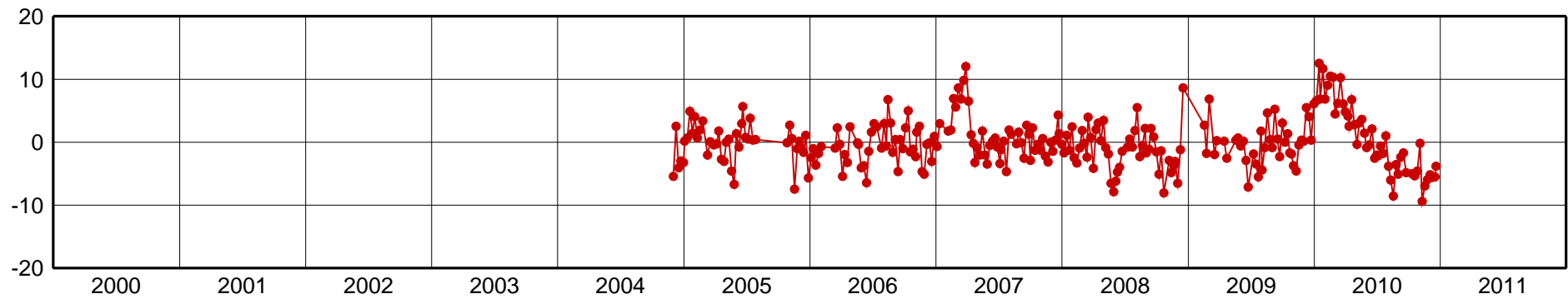
PERA-Up Component [mm]
