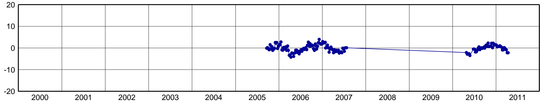
MEDE-North Component [mm]
