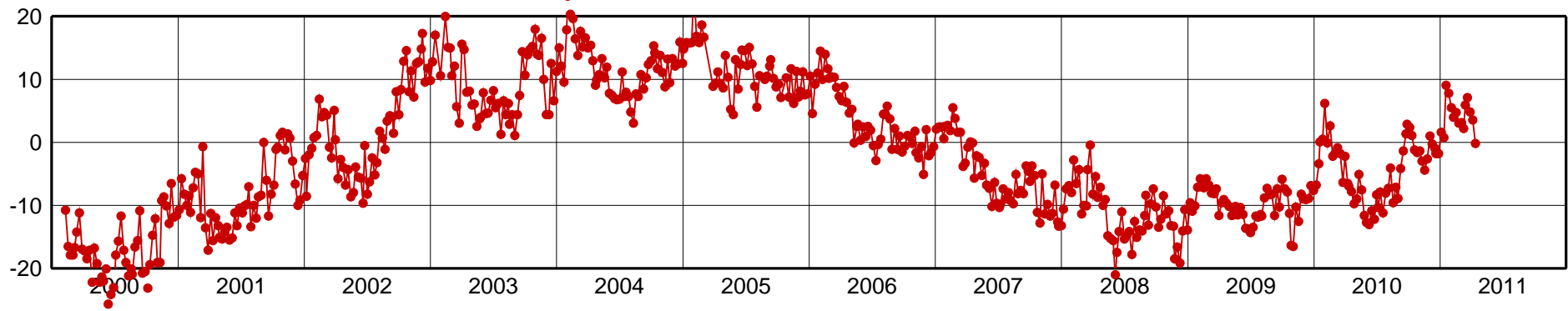
BOGA-Up Component [mm]
