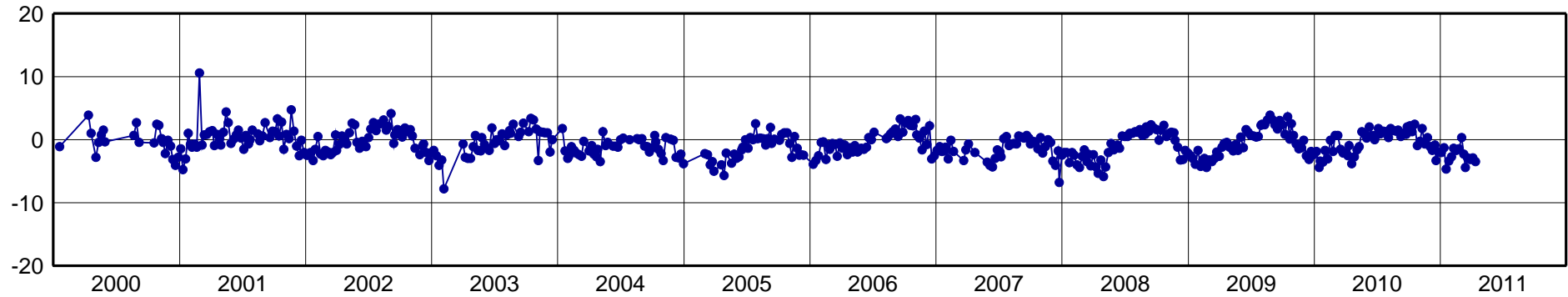
IMPZ-North Component [mm]
