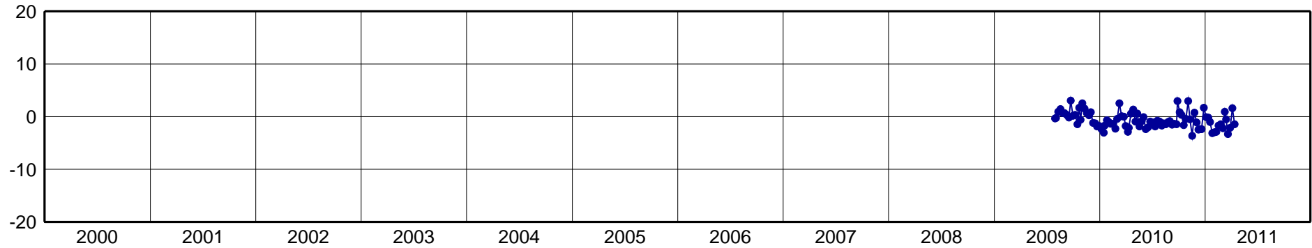
BAVC-North Component [mm]
