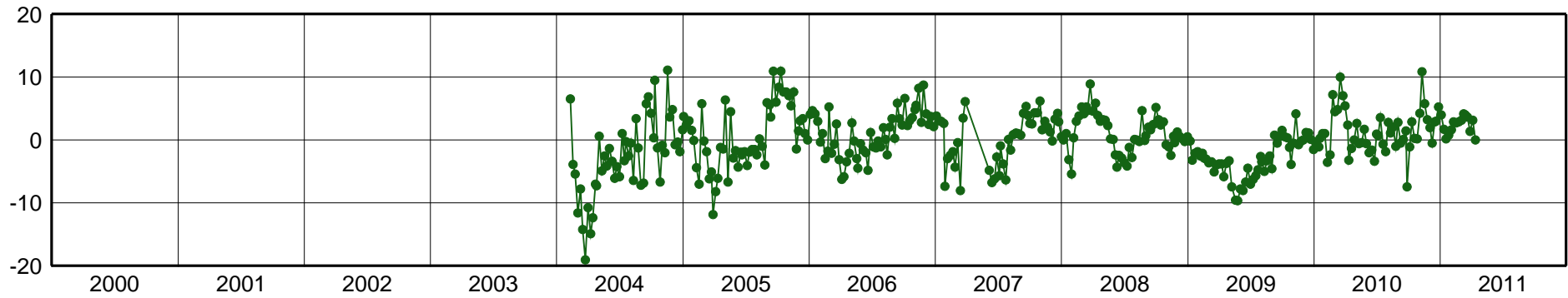
ISPA-East Component [mm]
