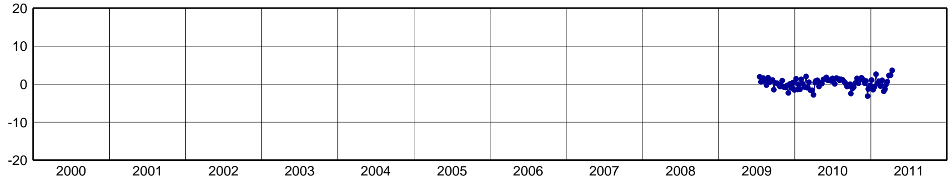
PRMA-North Component [mm]
