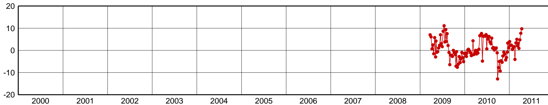
ICAM-Up Component [mm]
