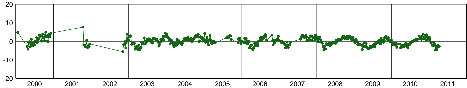
BOMJ-East Component [mm]
