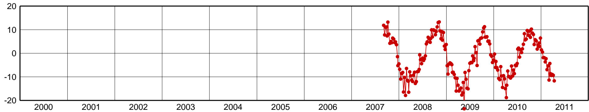
RIOB-Up Component [mm]
