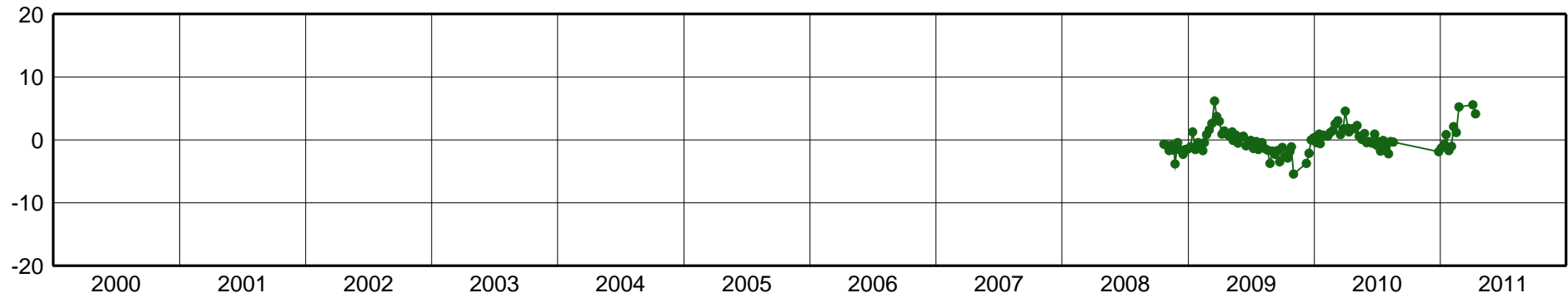
DAVI-East Component [mm]
