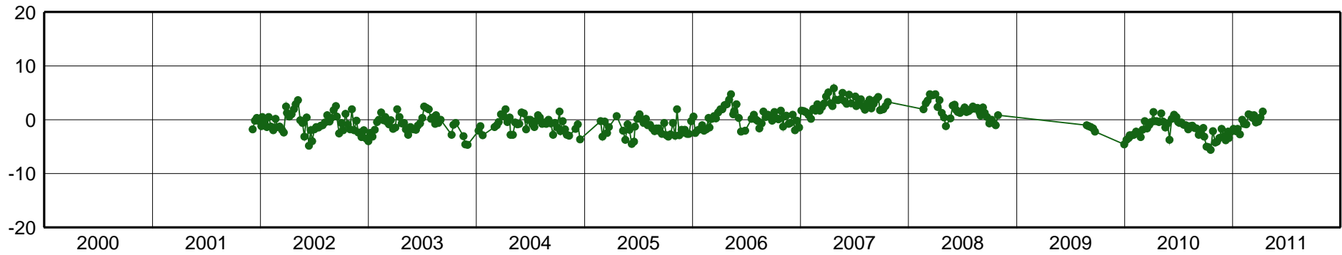
ELEN-East Component [mm]
