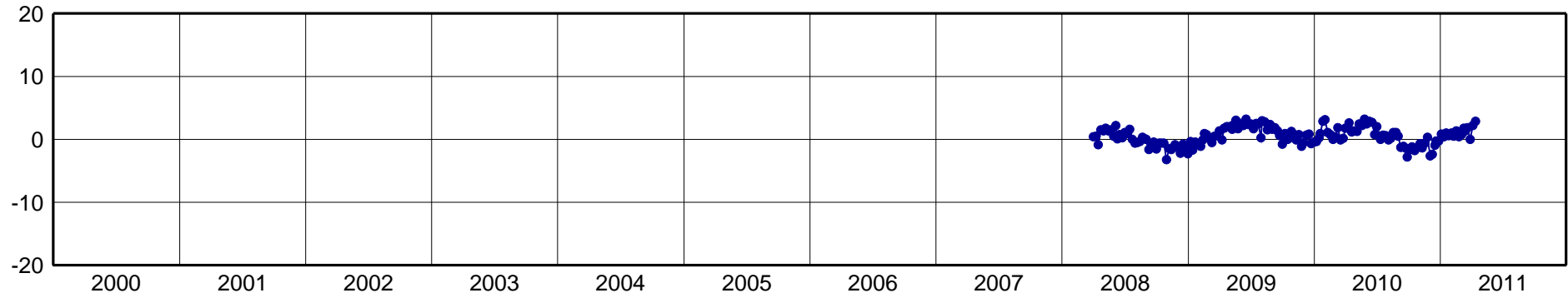
SCLA-North Component [mm]
