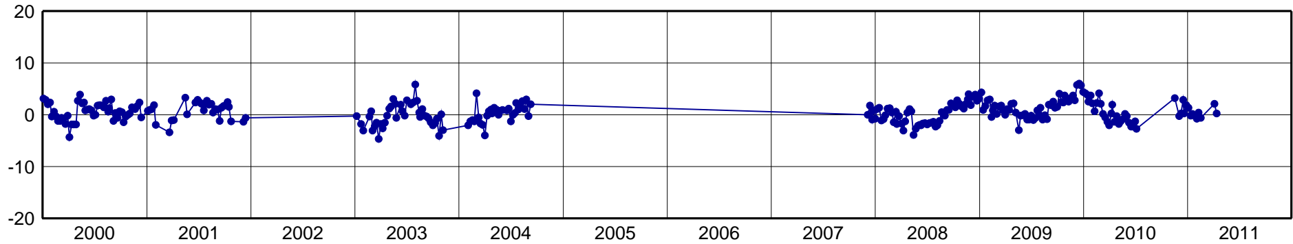
COYQ-North Component [mm]
