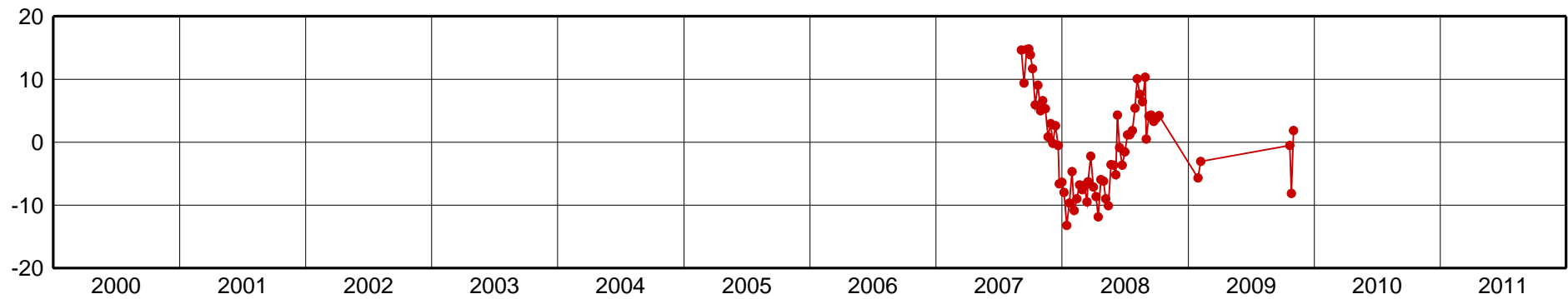
CRUZ-Up Component [mm]
