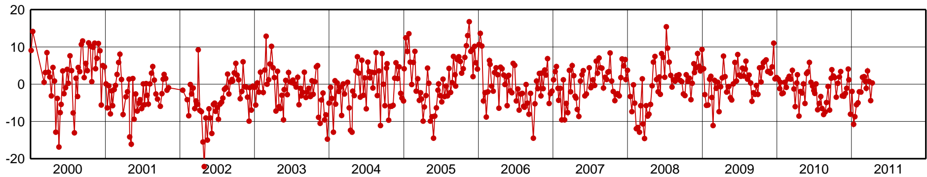
KOUR-Up Component [mm]
