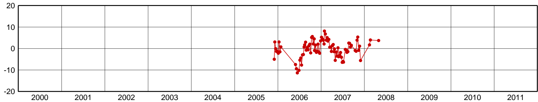
YOPA-Up Component [mm]
