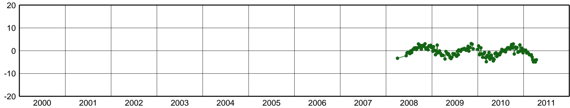
MGMC-East Component [mm]
