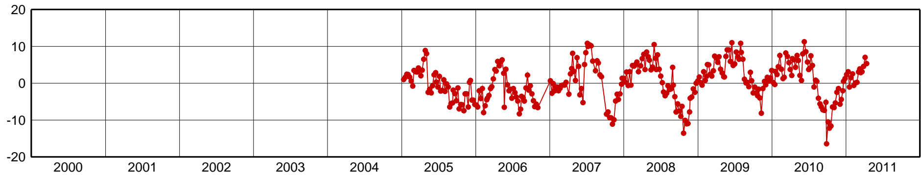
VIL2-Up Component [mm]
