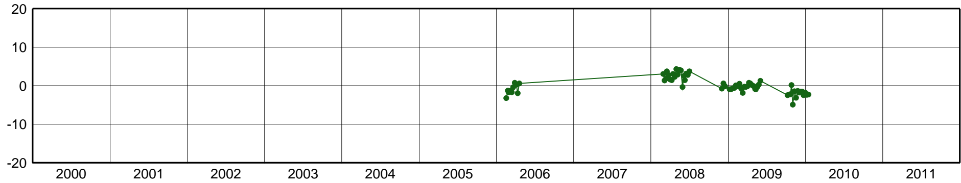
IBAG-East Component [mm]
