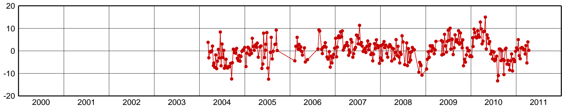
CUCU-Up Component [mm]
