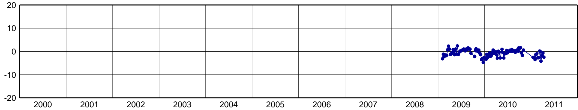
BAIR-North Component [mm]
