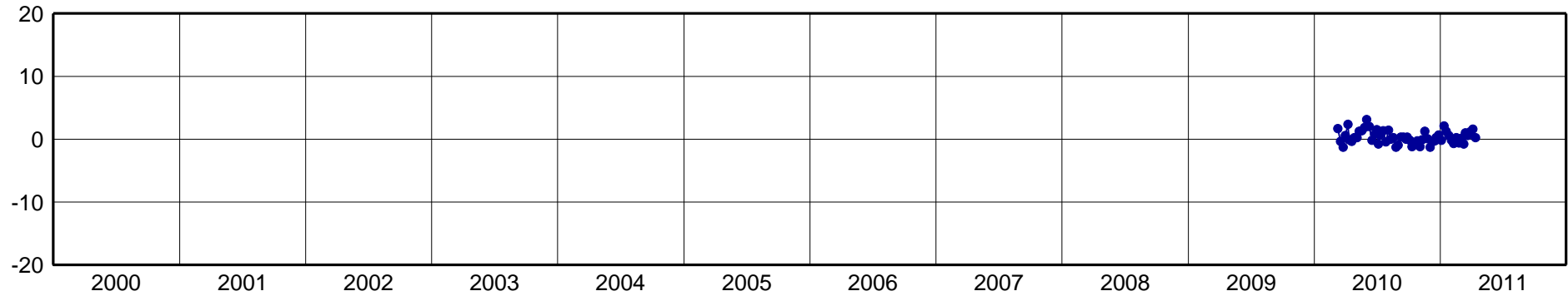
MPL2-North Component [mm]
