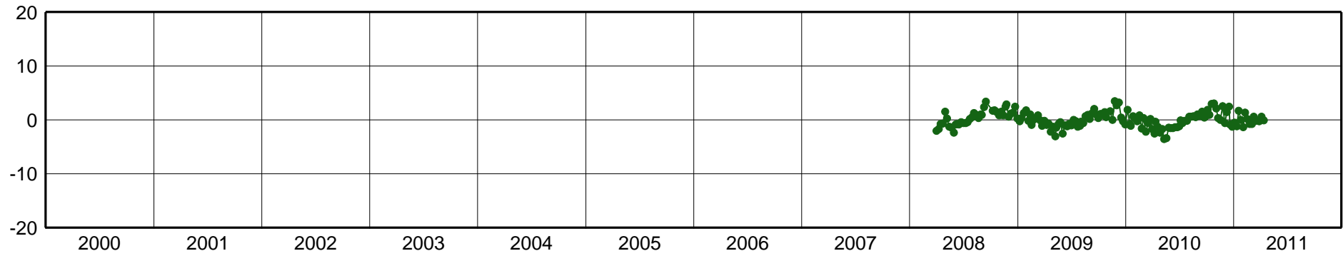
MTSF-East Component [mm]
