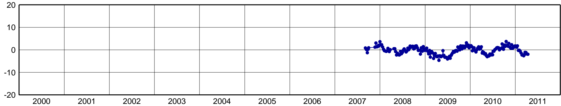
BOAV-North Component [mm]
