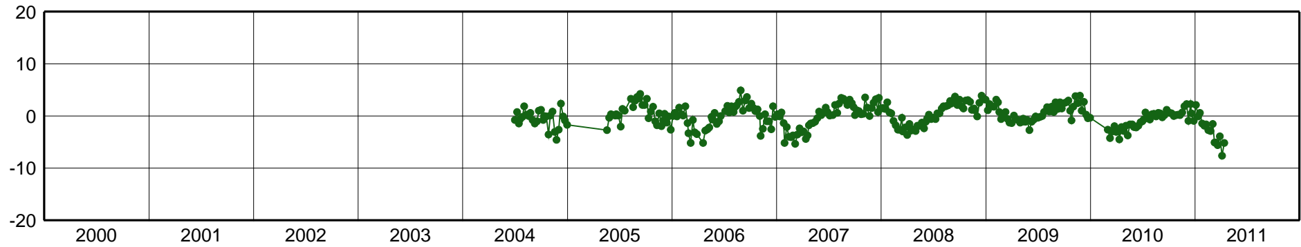
GVAL-East Component [mm]
