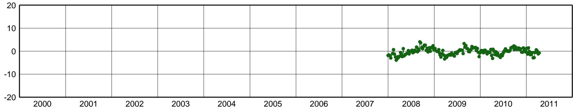
TOPL-East Component [mm]
