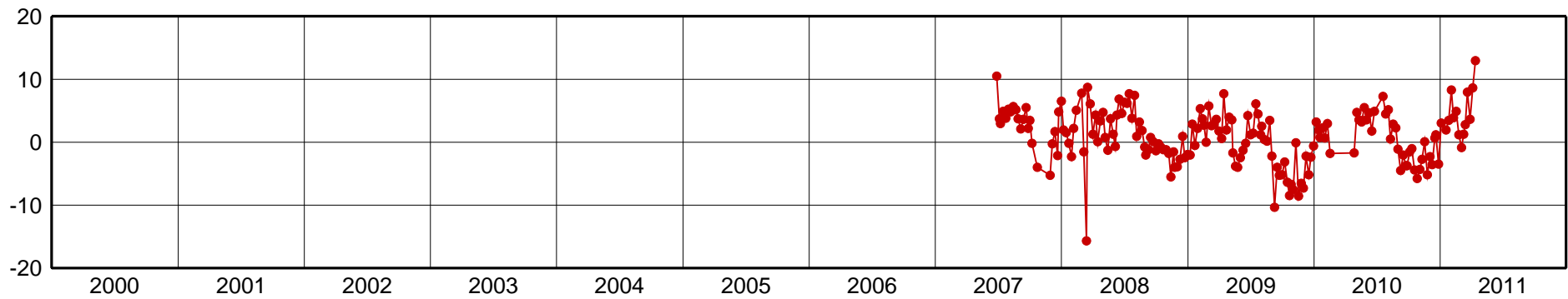
BRFT-Up Component [mm]
