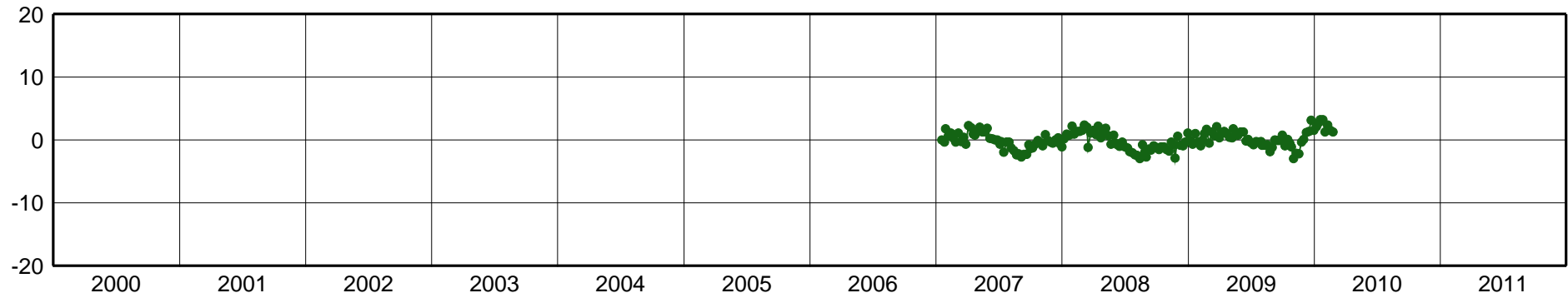
MZAS-East Component [mm]
