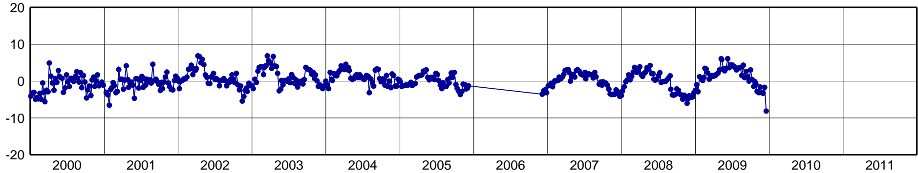
CIC1-North Component [mm]
