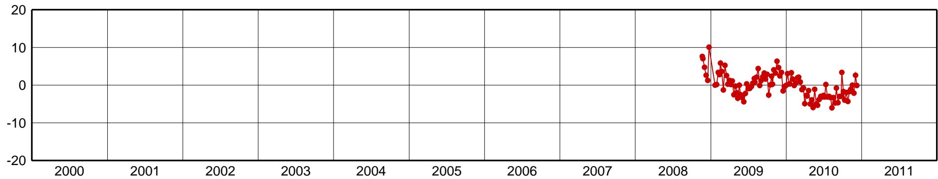
CUEC-Up Component [mm]
