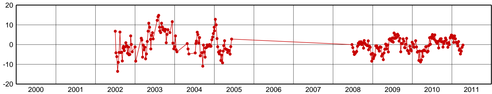
IQQE-Up Component [mm]
