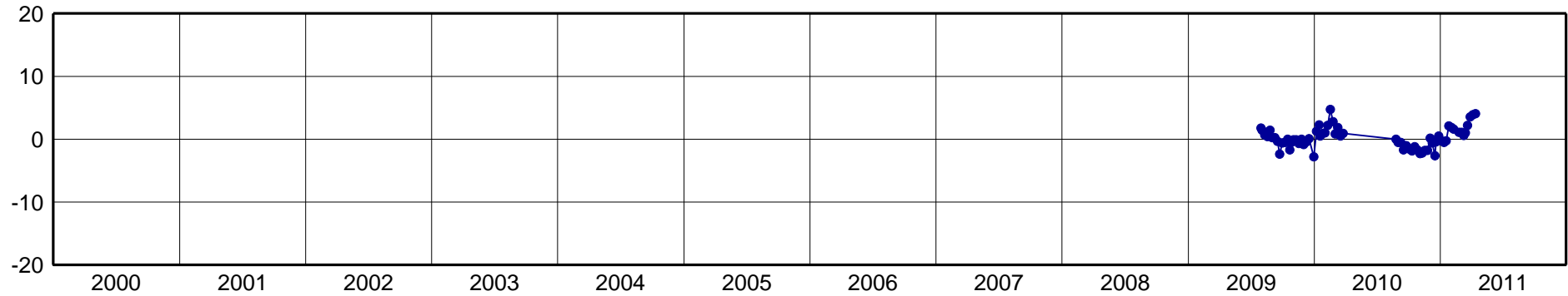
MSDO-North Component [mm]
