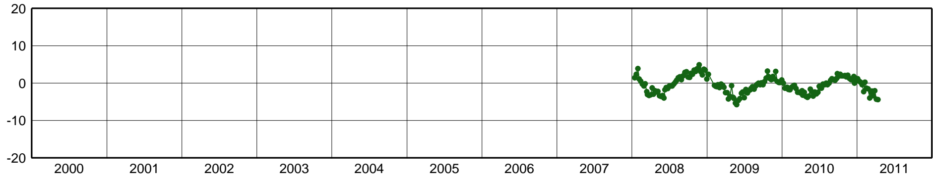
PEPE-East Component [mm]
