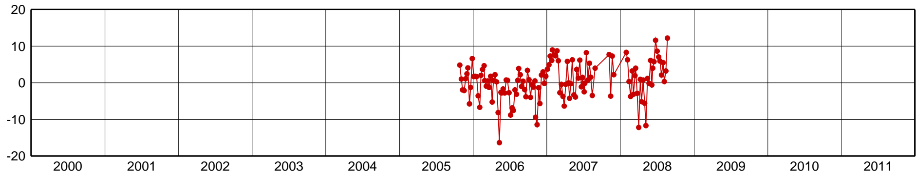
RIOH-Up Component [mm]
