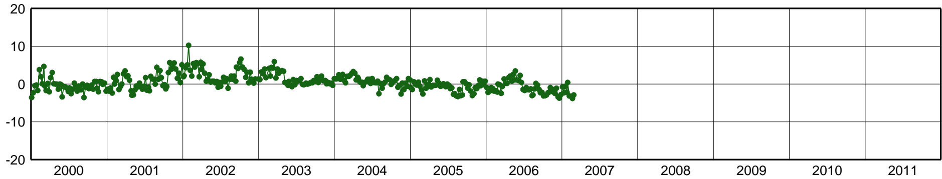
RI OG-East Component [mm]
