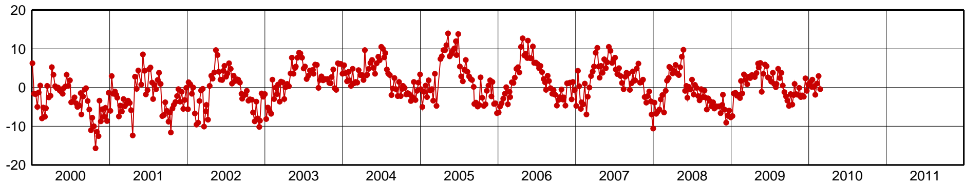
SANT-Up Component [mm]
