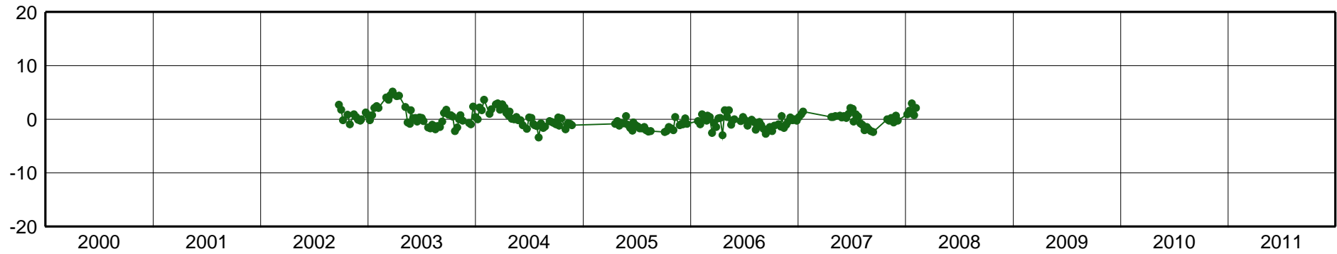
MPLA-East Component [mm]
