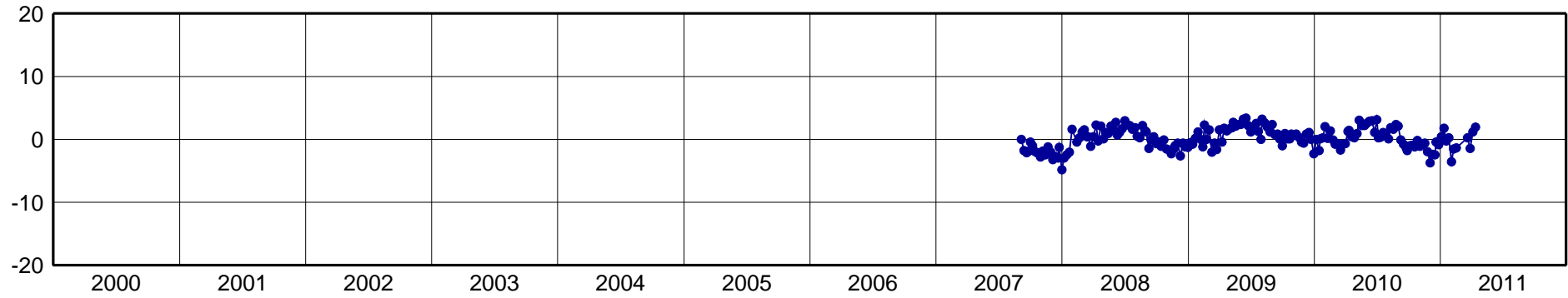
IMBT-North Component [mm]
