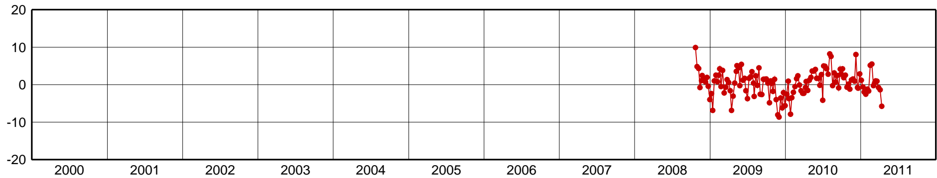
IGN1-Up Component [mm]
