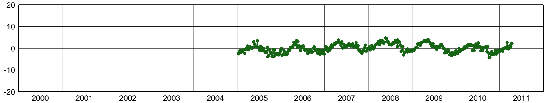
CHET-East Component [mm]
