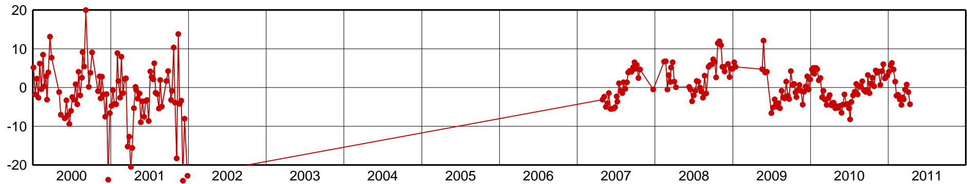
RIOP-Up Component [mm]
