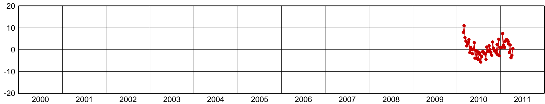
ABPD-Up Component [mm]
