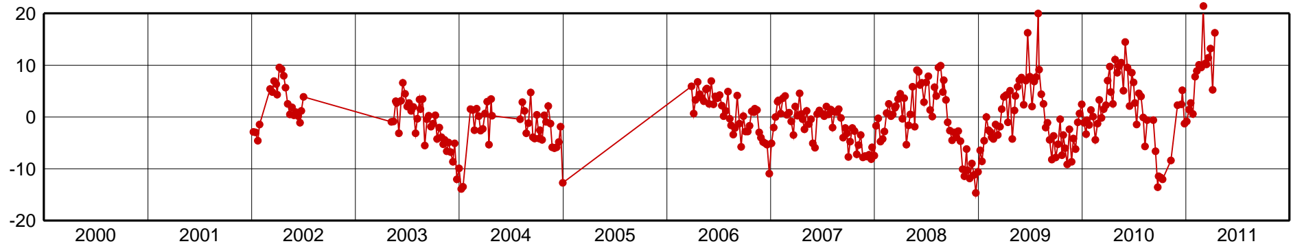
AUTF-Up Component [mm]
