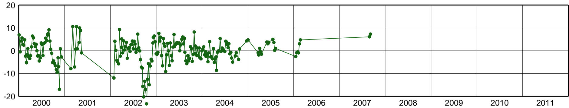
ASC1-East Component [mm]
