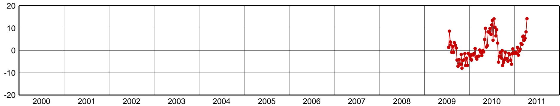
ICEP-Up Component [mm]
