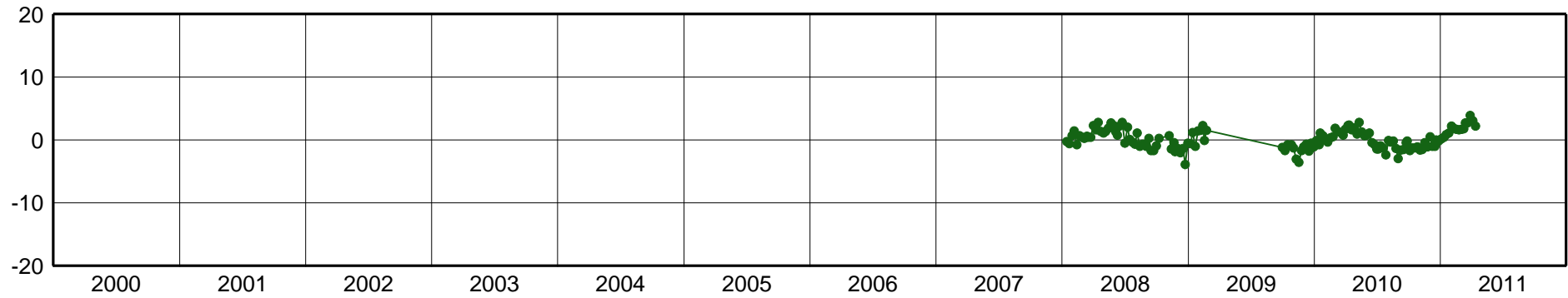
ROGM-East Component [mm]
