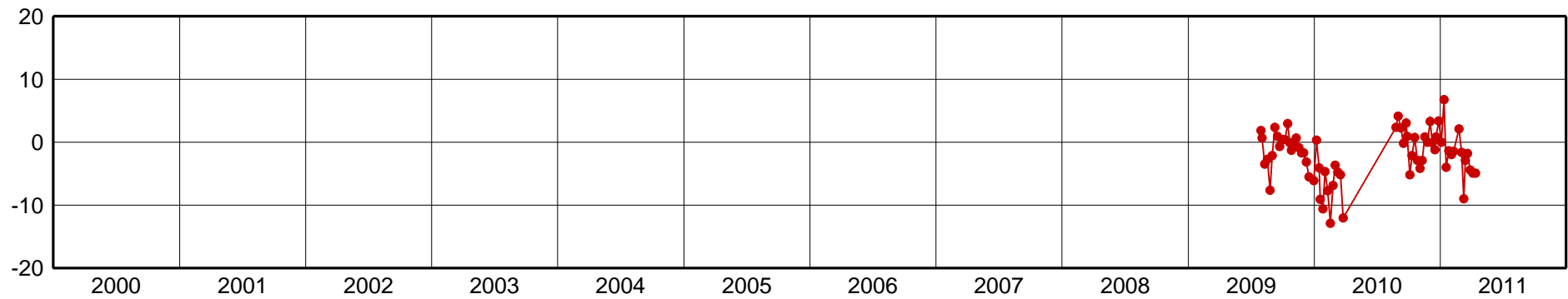
MSDO-Up Component [mm]
