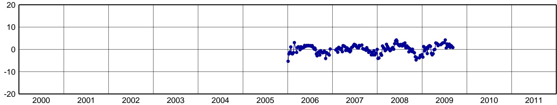
UBAT-North Component [mm]
