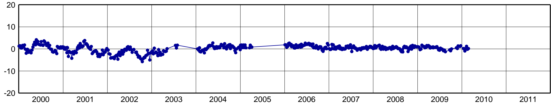
CFAG-North Component [mm]
