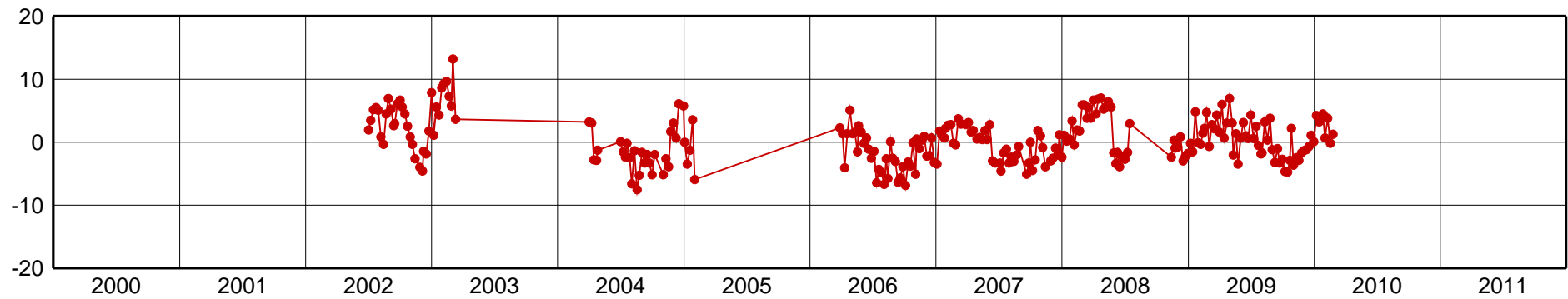
LHCL-Up Component [mm]
