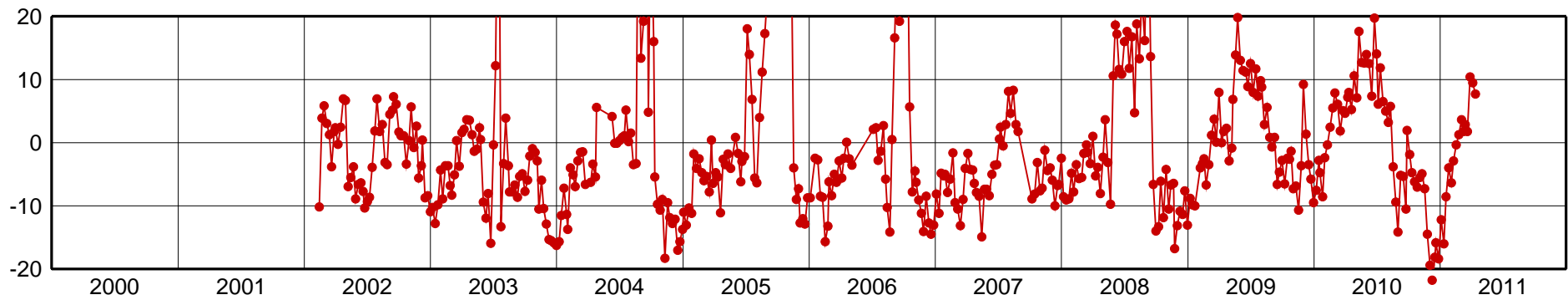
OH2-Up Component [mm]
