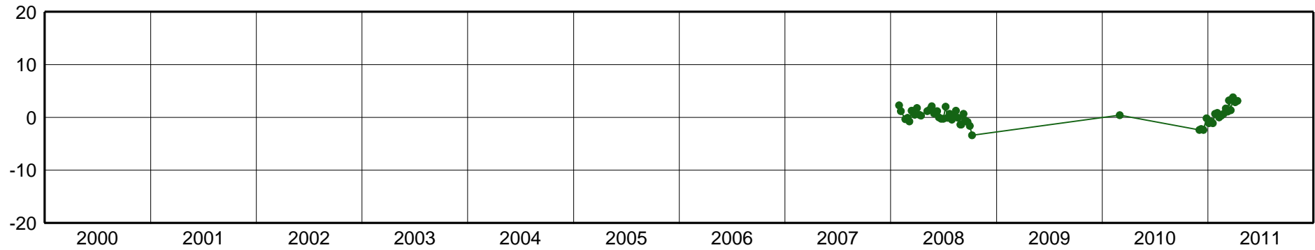
AMHU-East Component [mm]
