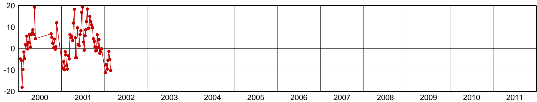
OHIG-Up Component [mm]
