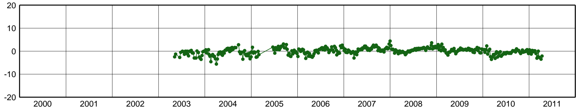
CHPI-East Component [mm]
