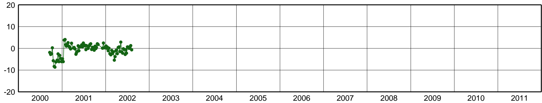
SLOR-East Component [mm]
