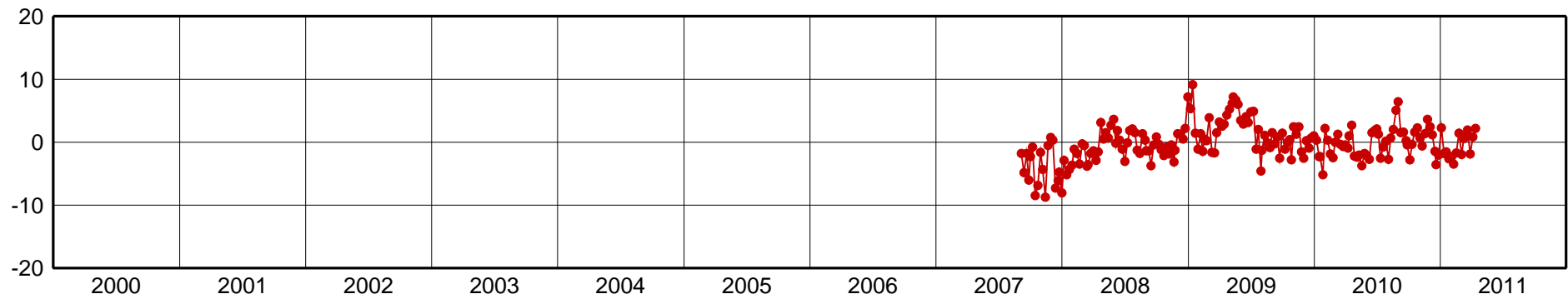
UFPR-Up Component [mm]
