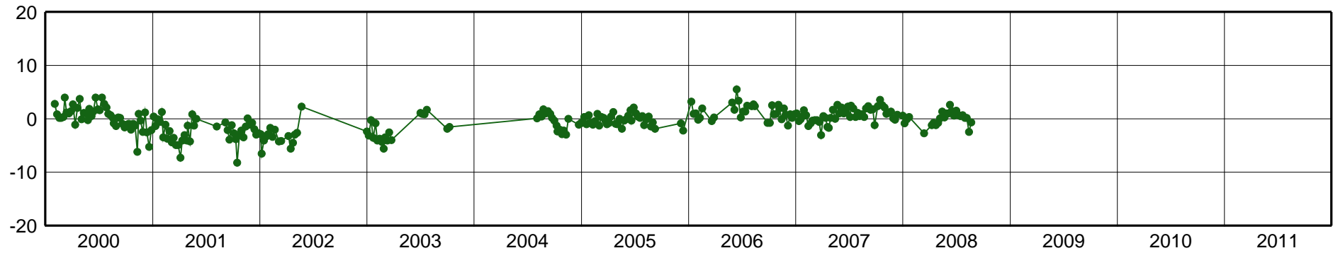
CART-East Component [mm]
