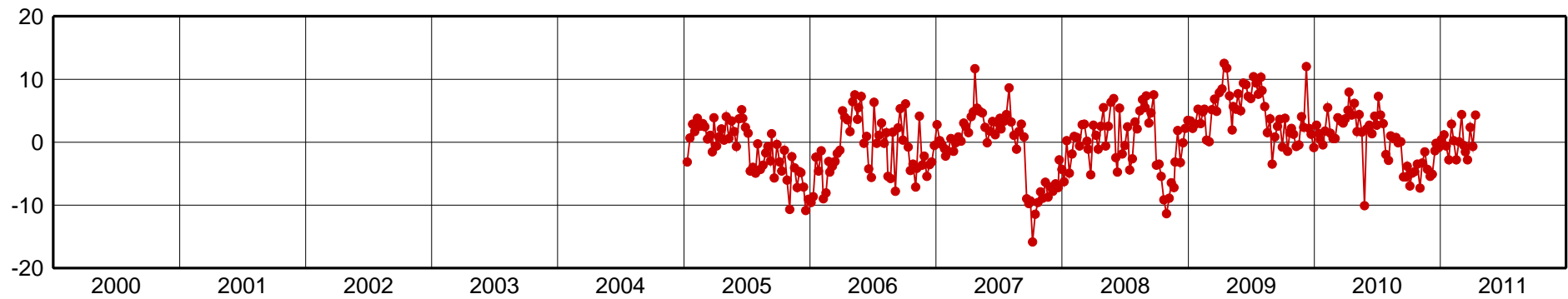
CHET-Up Component [mm]
