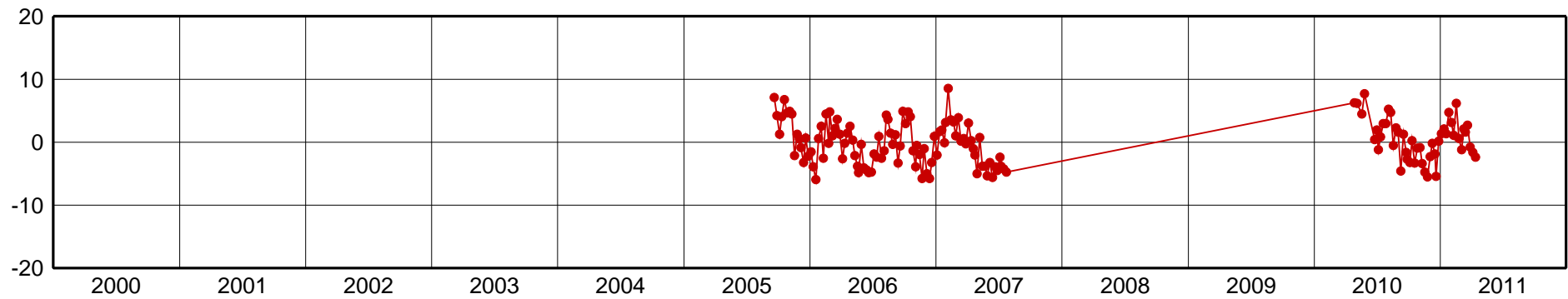
MEDE-Up Component [mm]
