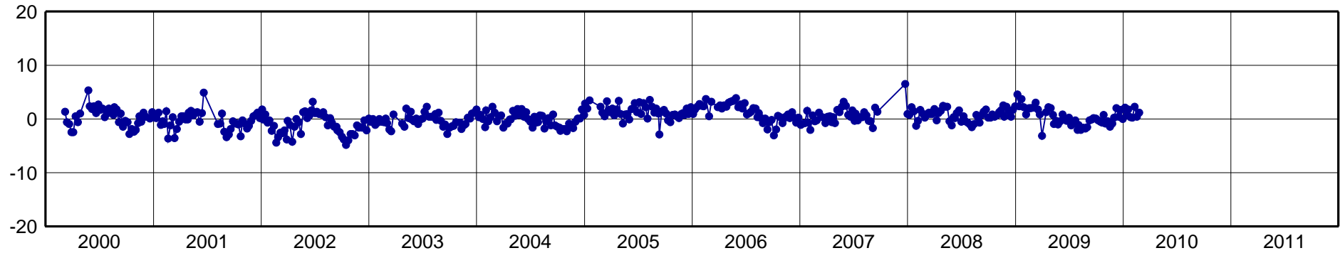
VBCA-North Component [mm]
