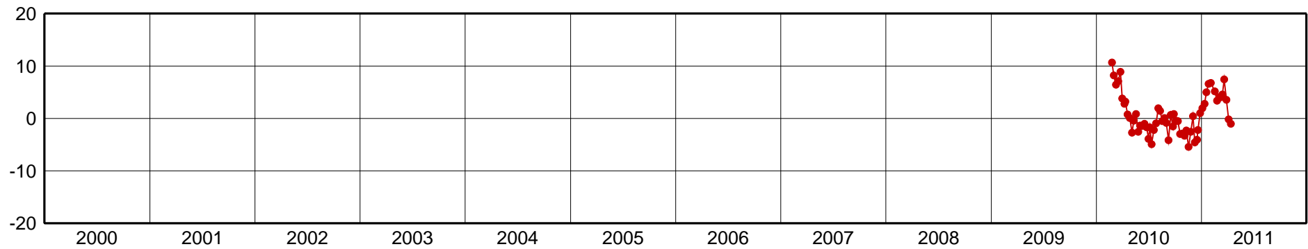
ABCC-Up Component [mm]
