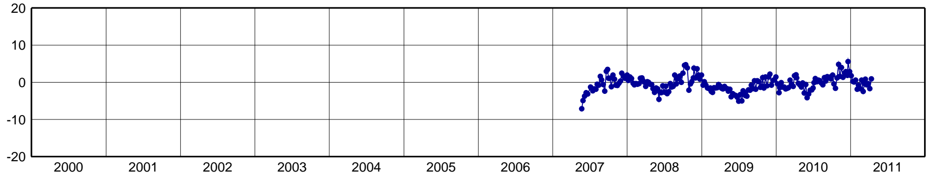
SMRT-North Component [mm]
