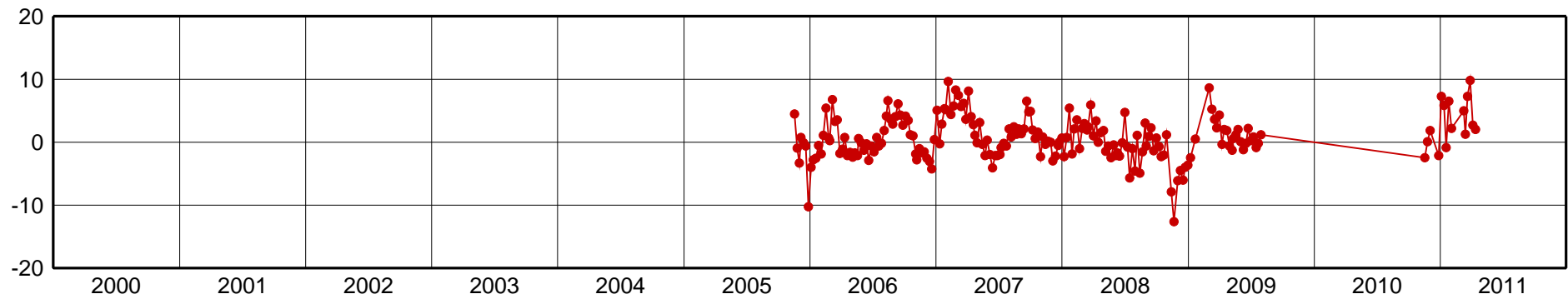
NEVA-Up Component [mm]
