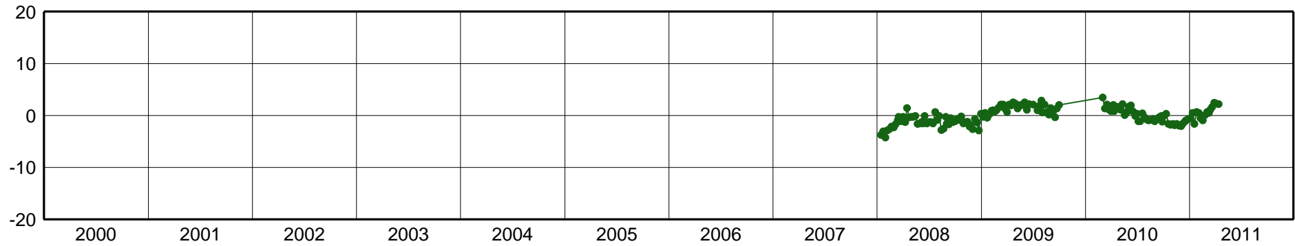
PSTO-East Component [mm]
