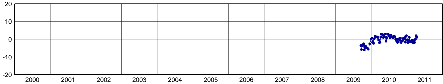
ROSA-North Component [mm]
