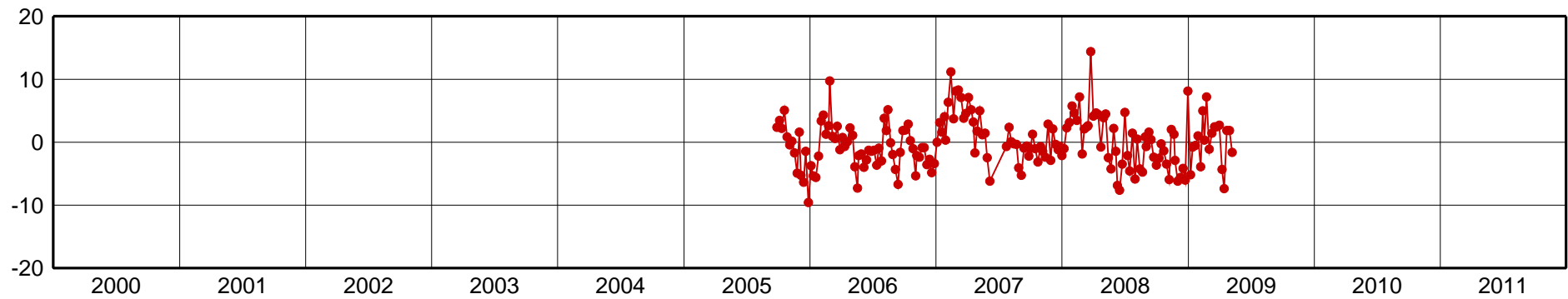
BUCA-Up Component [mm]
