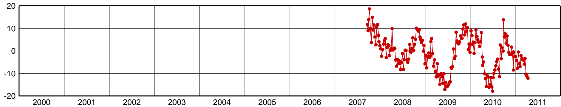
SAGA-Up Component [mm]
