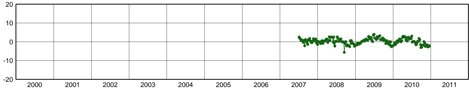
NAS0-East Component [mm]
