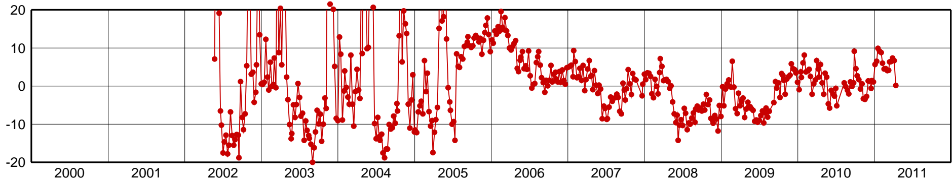
BOGT-Up Component [mm]
