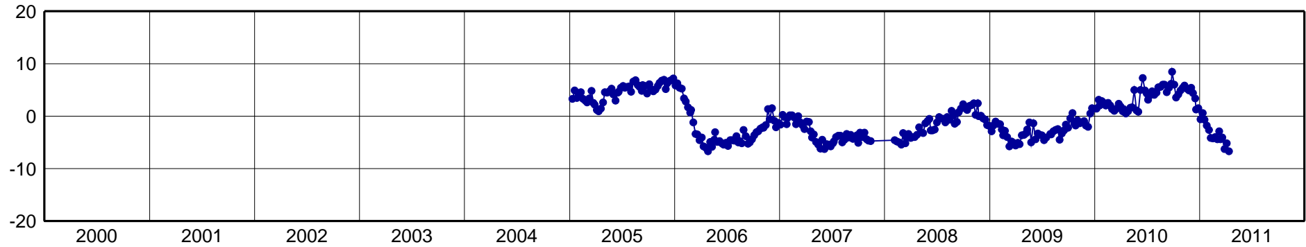
OAX2-North Component [mm]
