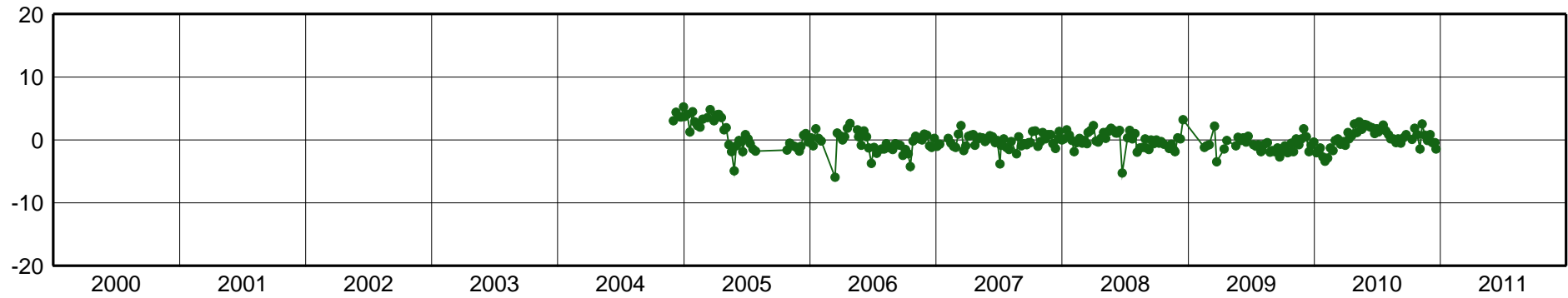
PERA-East Component [mm]
