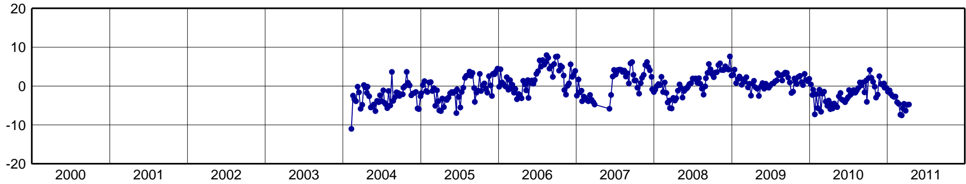
ISPA-North Component [mm]
