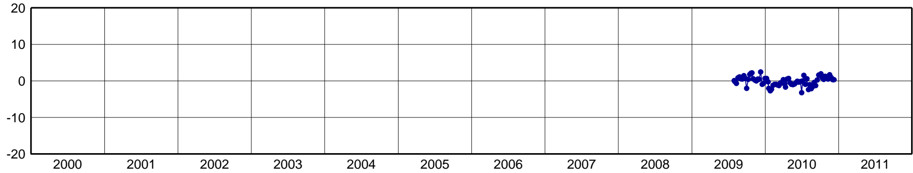
IQUI-North Component [mm]
