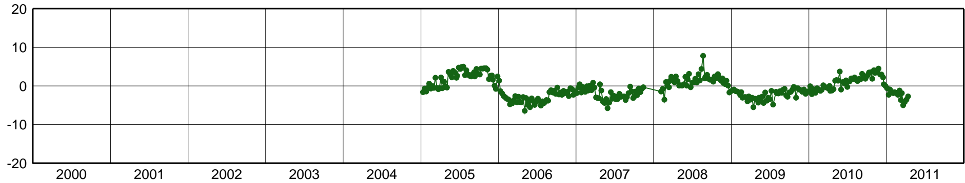
OAX2-East Component [mm]
