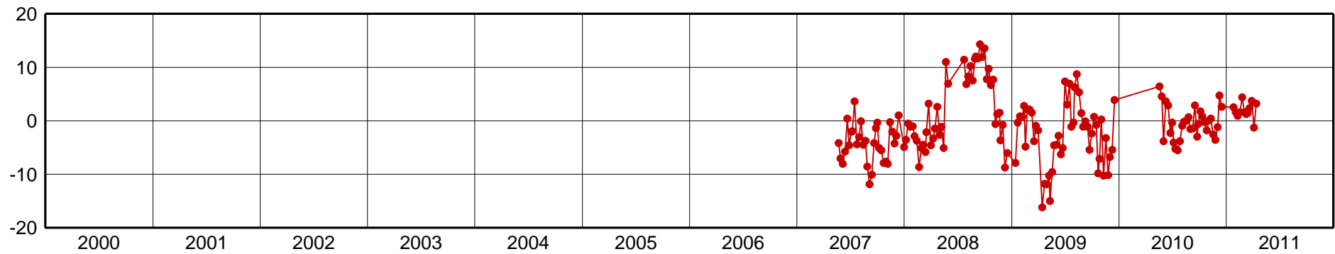
BERR-Up Component [mm]
