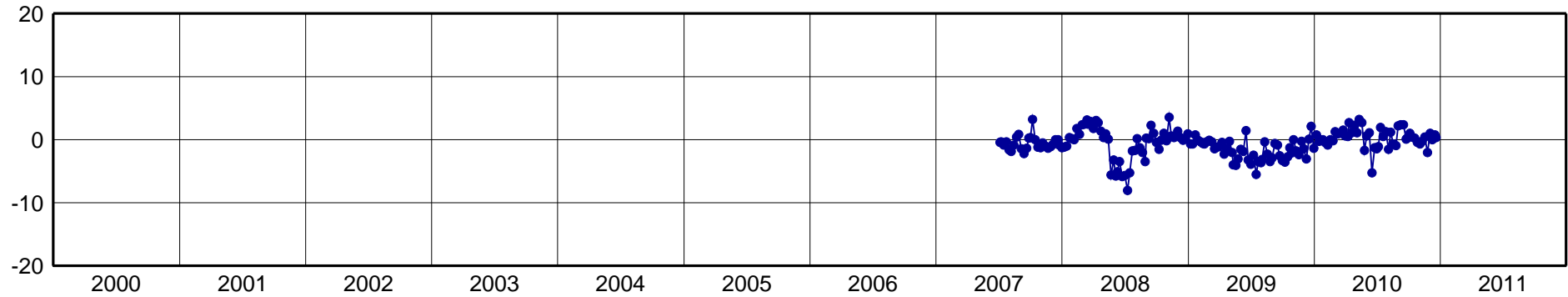
NAS0-North Component [mm]
