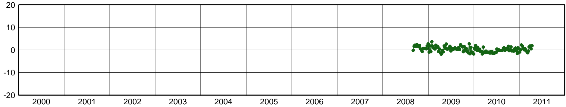
MTBA-East Component [mm]
