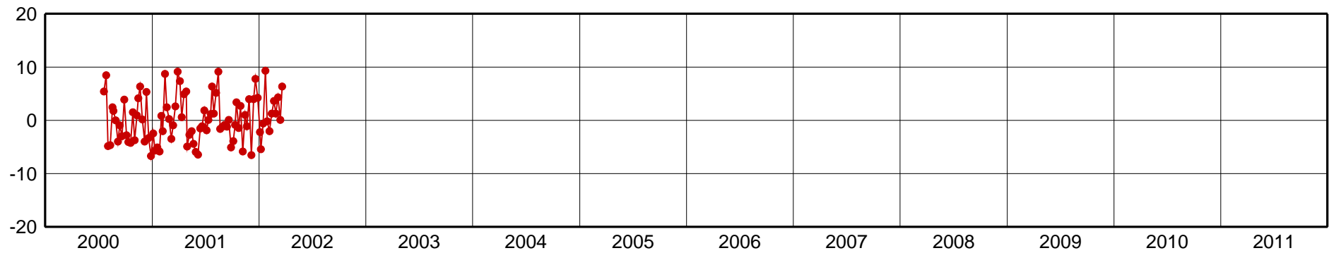
TEGU-Up Component [mm]
