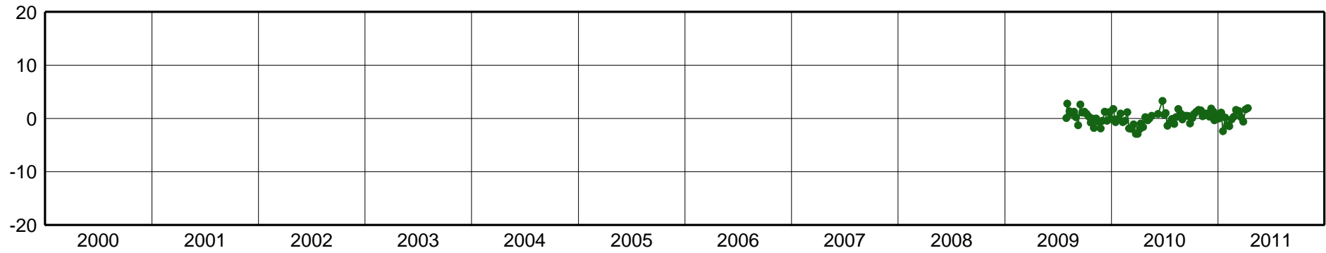
SVIC-East Component [mm]
