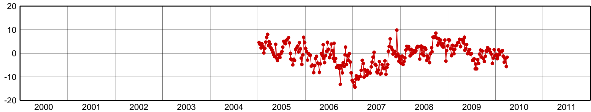
MEXI-Up Component [mm]
