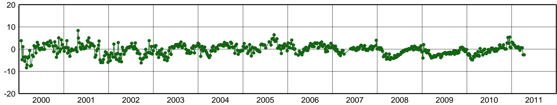
VICO-East Component [mm]
