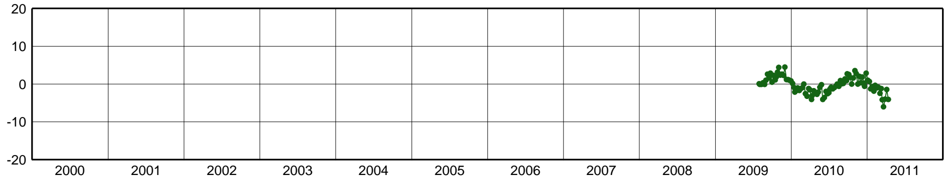
BAVC-East Component [mm]
