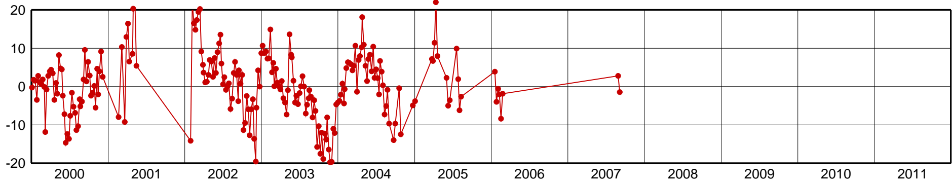
ASC1-Up Component [mm]
