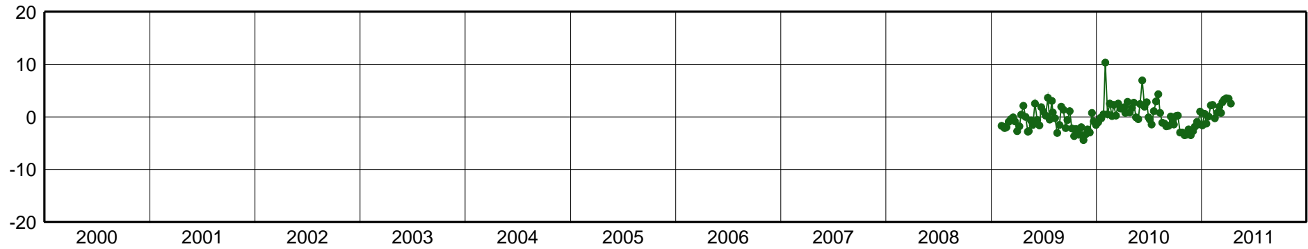
LJEC-East Component [mm]
