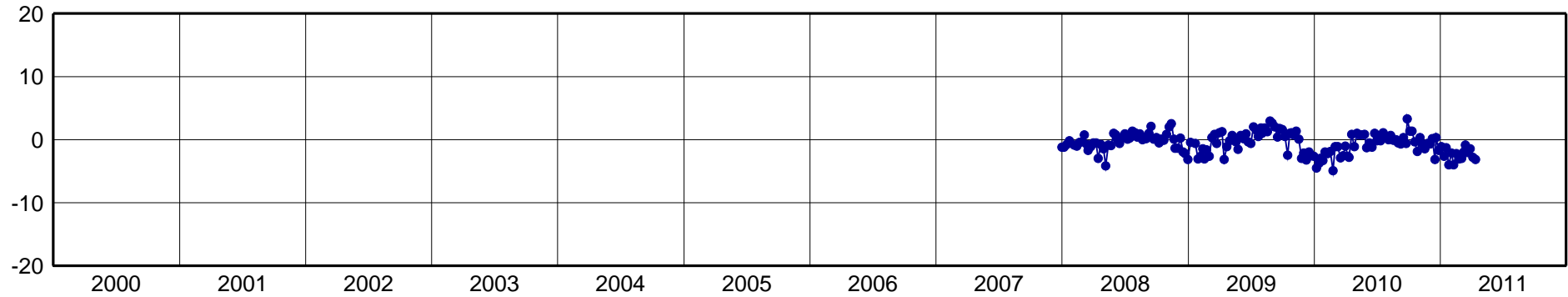
TOPL-North Component [mm]
