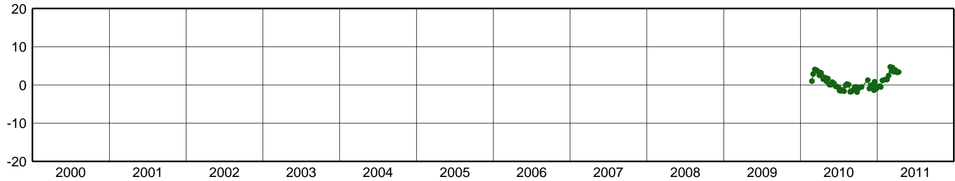
URUS-East Component [mm]
