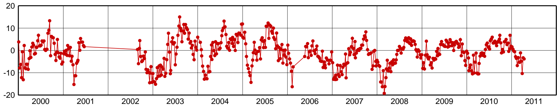
AREQ-Up Component [mm]
