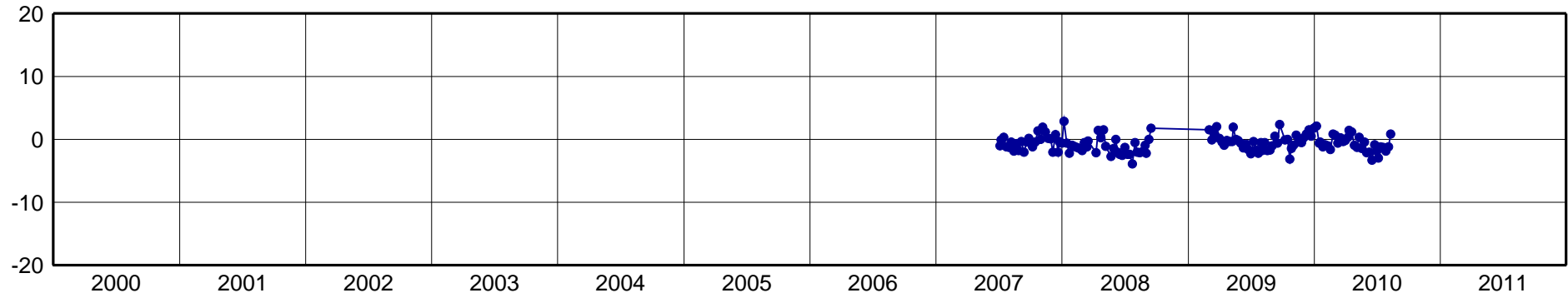
GTK0-North Component [mm]
