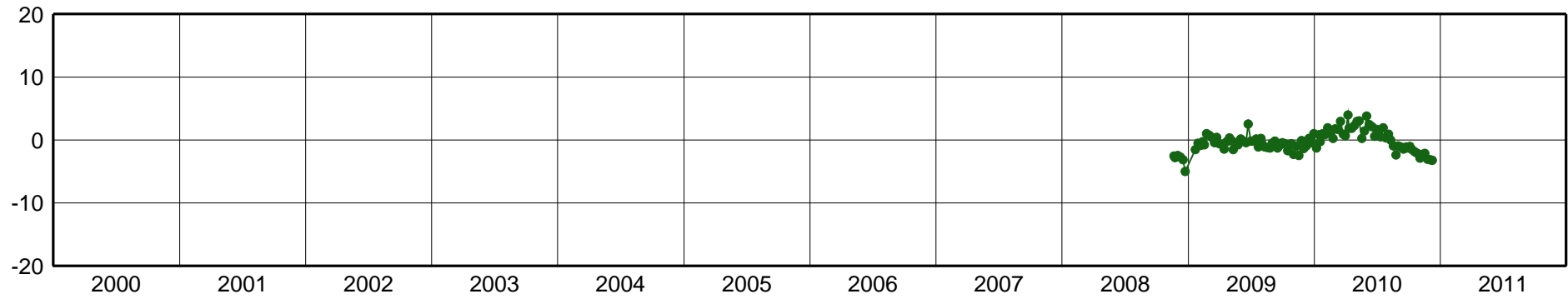
CUEC-East Component [mm]
