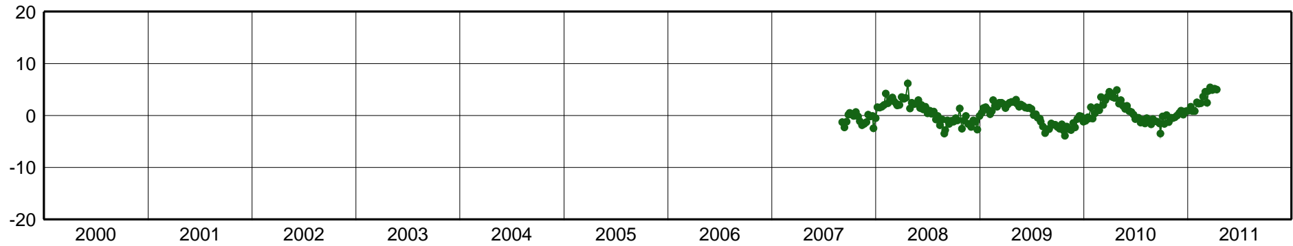
RIOB-East Component [mm]
