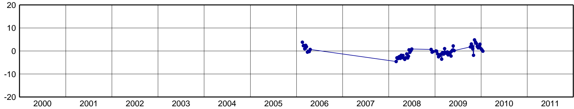
IBAG-North Component [mm]
