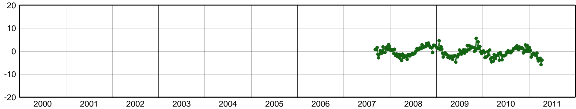
CEFE-East Component [mm]
