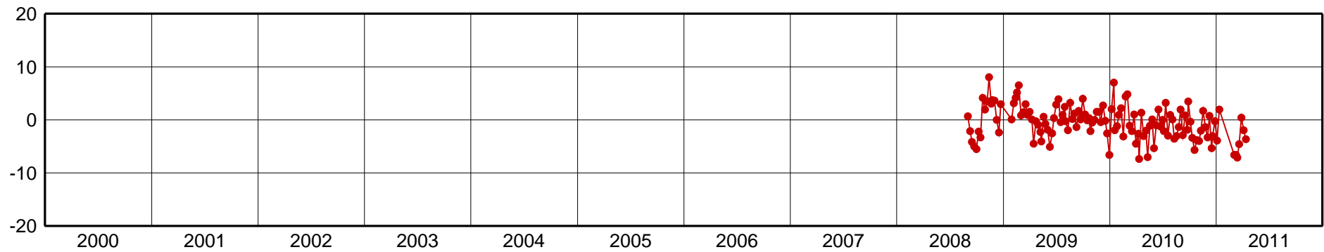
GYEC-Up Component [mm]
