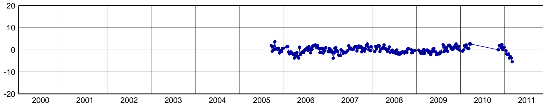
VIVI-North Component [mm]
