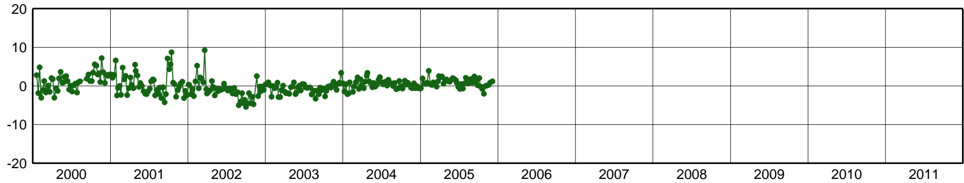
UEPP-East Component [mm]
