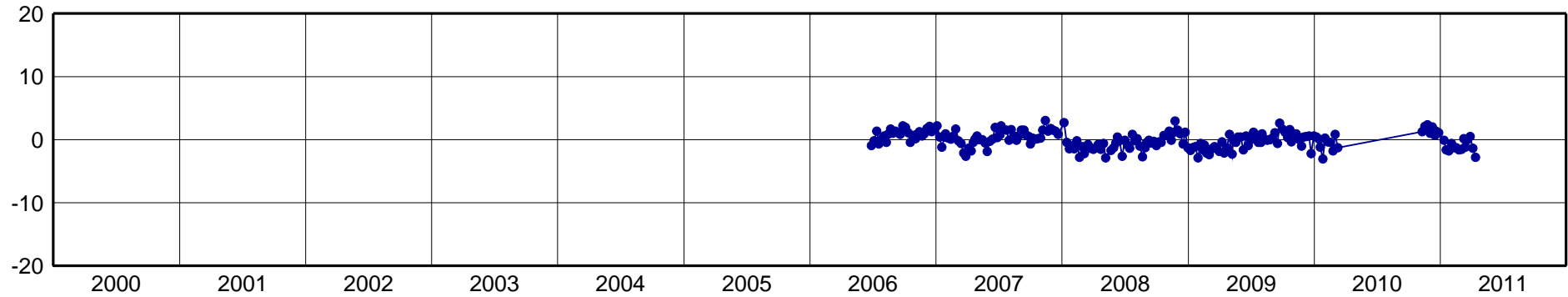
POPA-North Component [mm]
