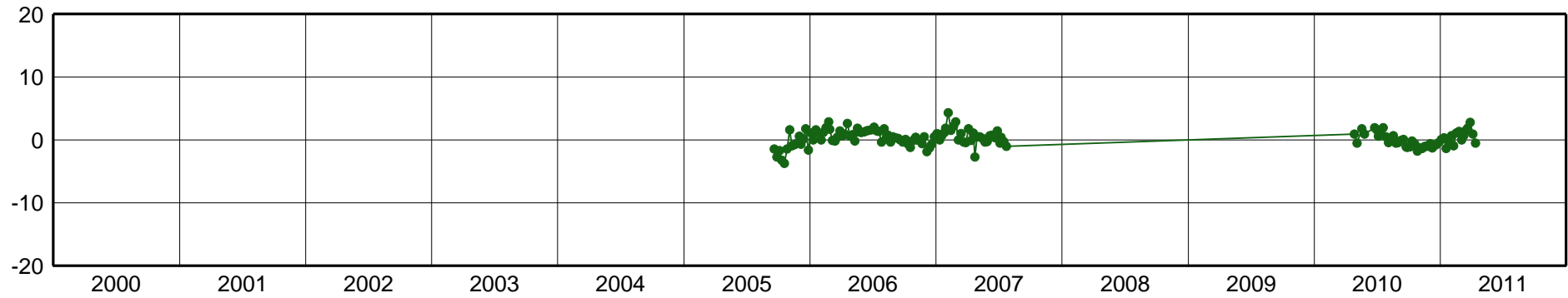
MEDE-East Component [mm]
