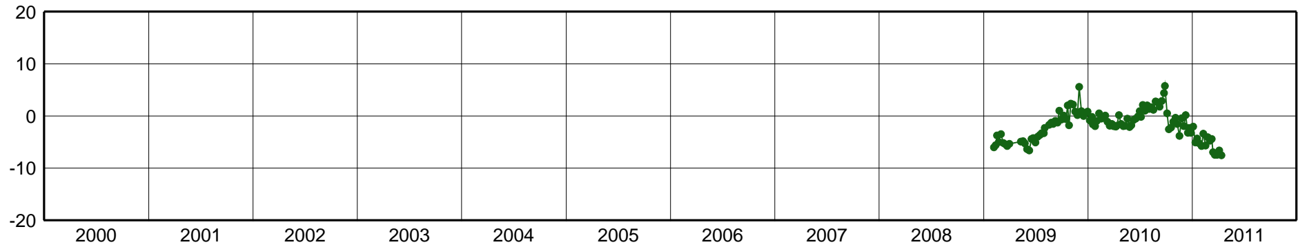
BATF-East Component [mm]
