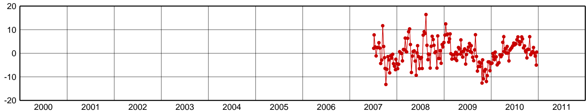
NAS0-Up Component [mm]
