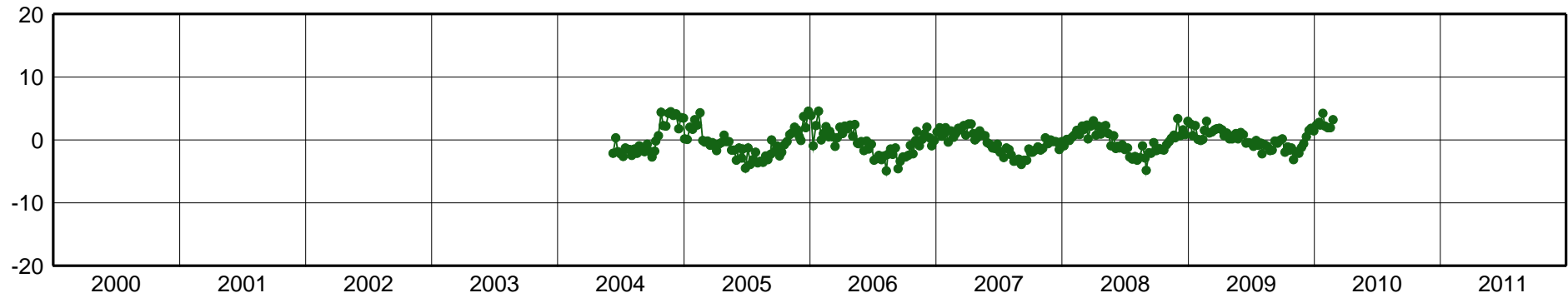
MZAC-East Component [mm]
