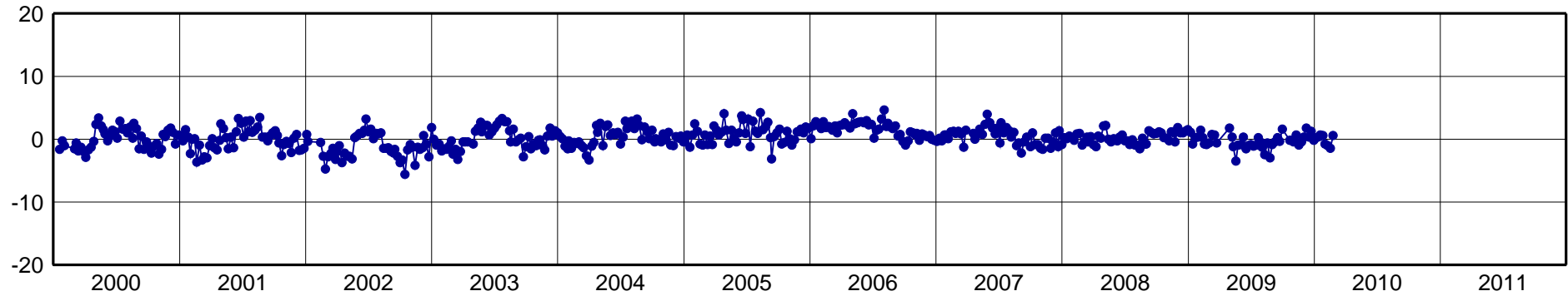
RWSN-North Component [mm]
