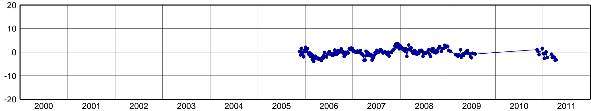
NEVA-North Component [mm]
