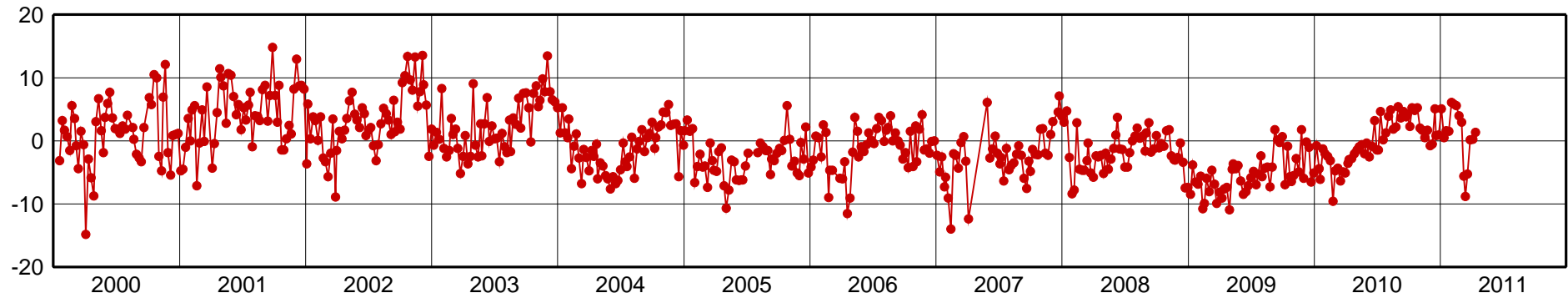
VICO-Up Component [mm]
