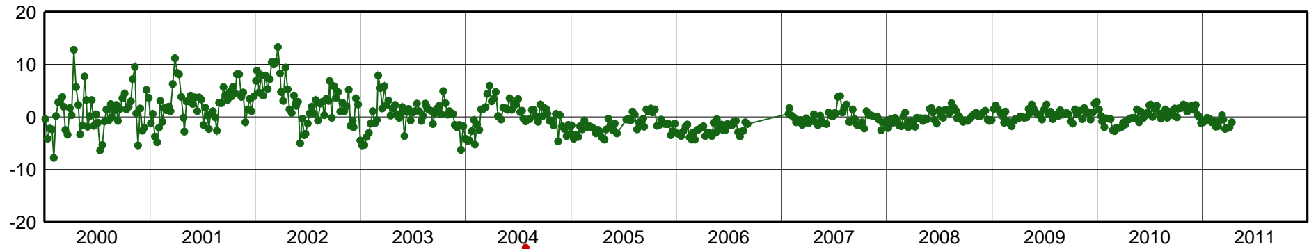
PIE1-East Component [mm]
