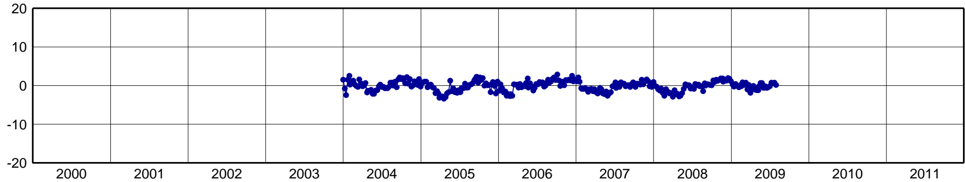
QUI1-North Component [mm]
