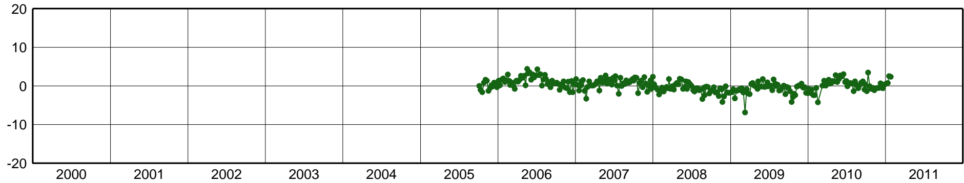
BUEN-East Component [mm]
