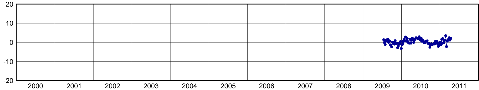
PRGU-North Component [mm]
