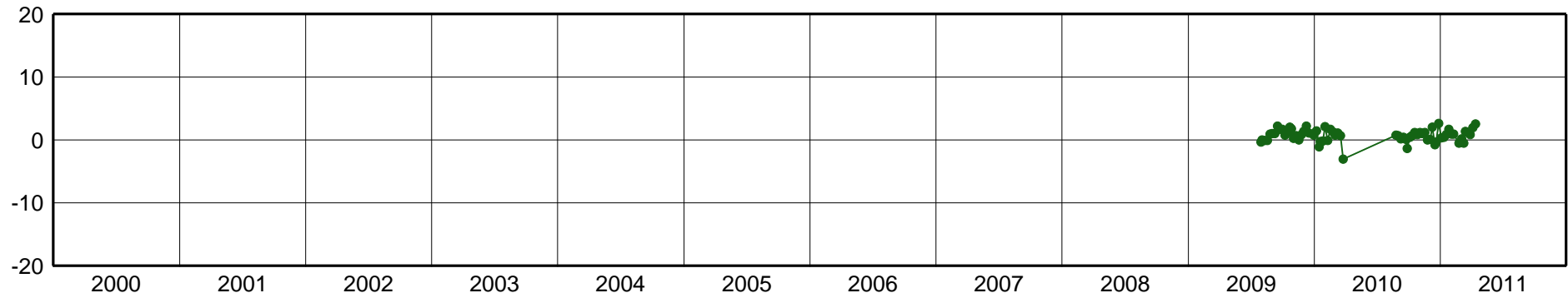
MSDO-East Component [mm]
