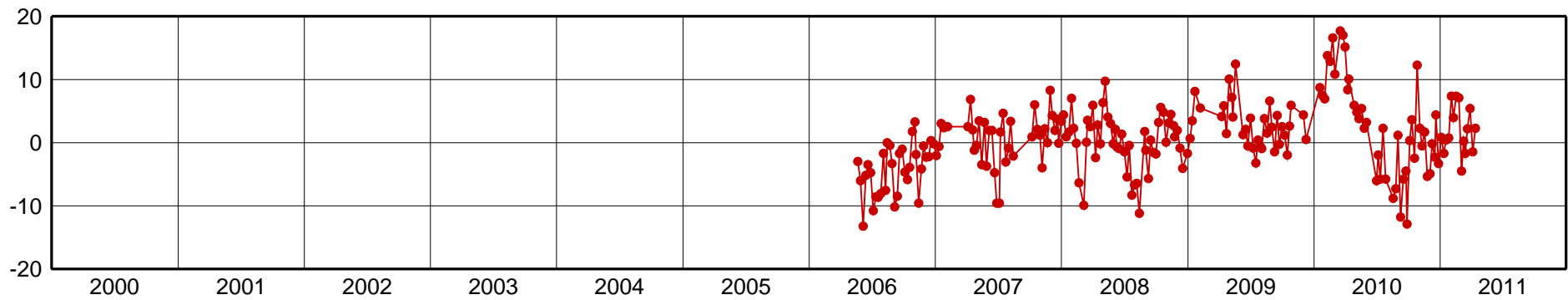
CRCS-Up Component [mm]
