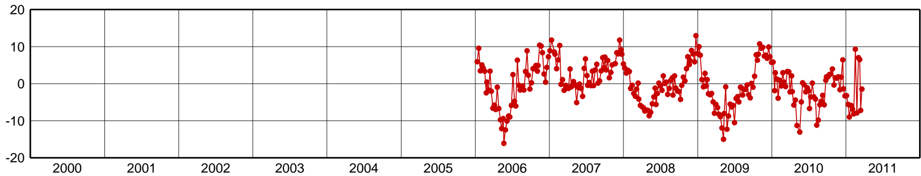
MAPA-Up Component [mm]
