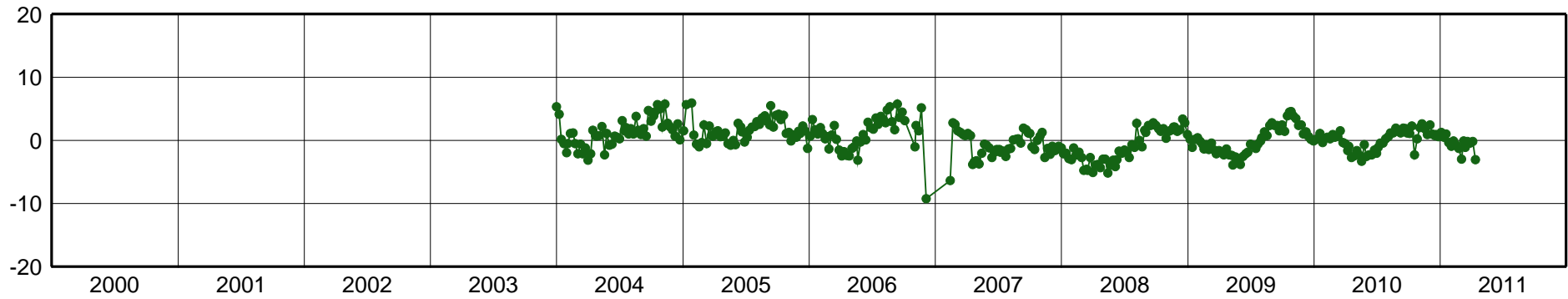
BELE-East Component [mm]
