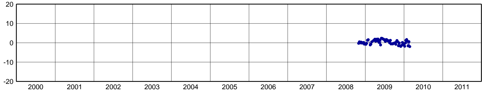
UYTA-North Component [mm]
