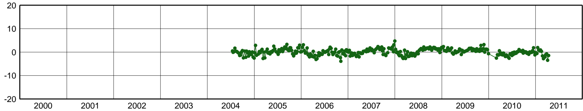
UBER-East Component [mm]
