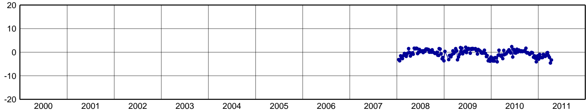
PEPE-North Component [mm]
