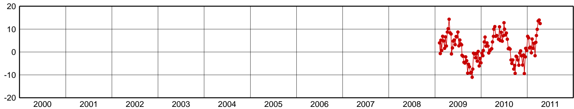
RNNA-Up Component [mm]
