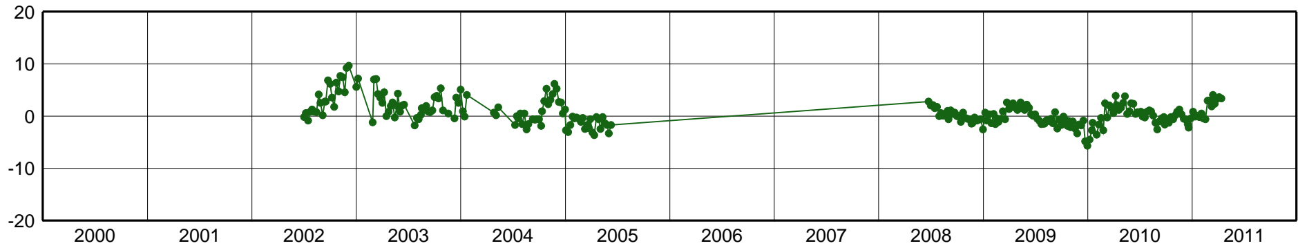
IQQE-East Component [mm]
