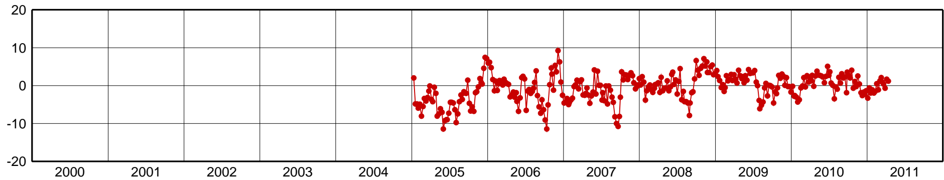
LPAZ-Up Component [mm]
