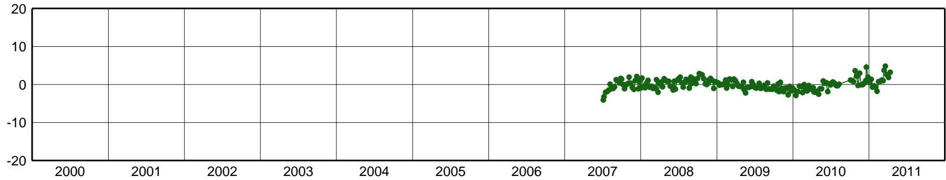
GRE0-East Component [mm]
