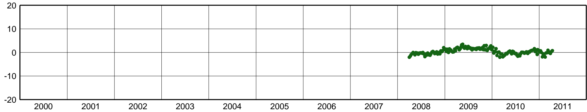
SCLA-East Component [mm]
