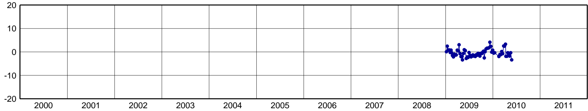
CASI-North Component [mm]
