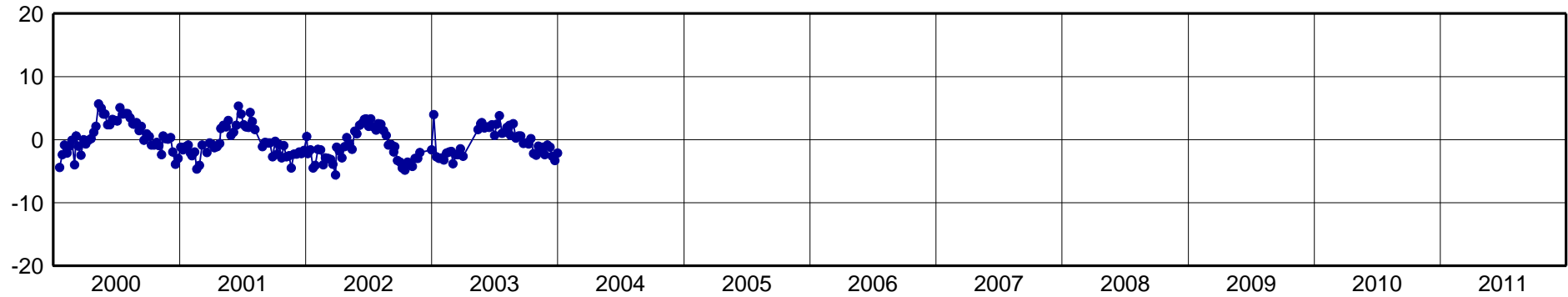
IGM0-North Component [mm]
