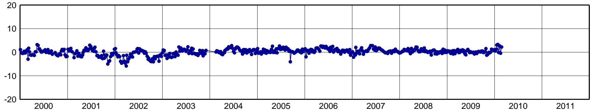
LPGS-North Component [mm]
