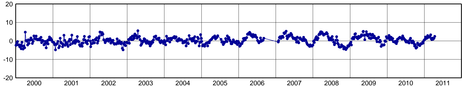
PIE1-North Component [mm]
