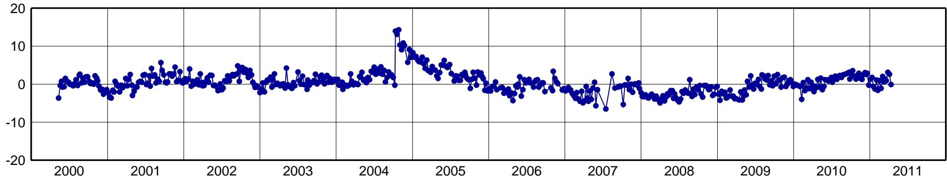
MANA-North Component [mm]
