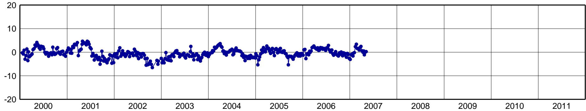
PARA-North Component [mm]
