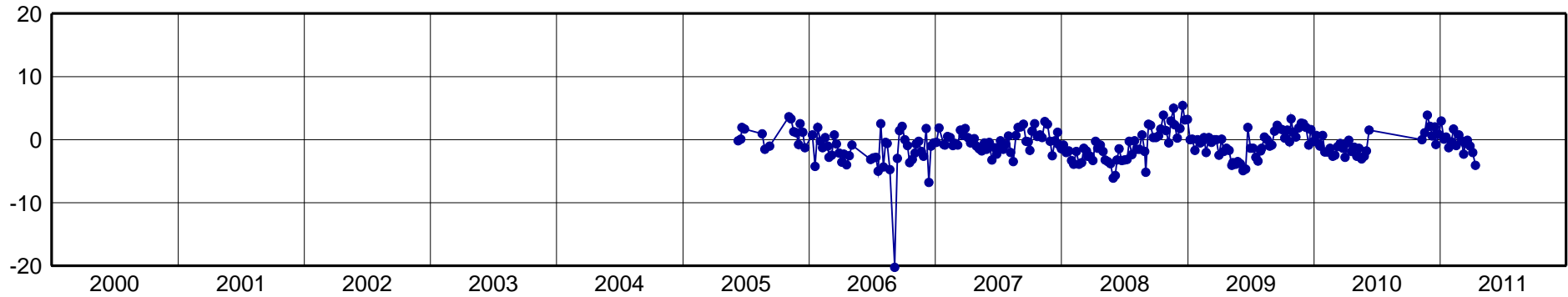
BDOS-North Component [mm]
