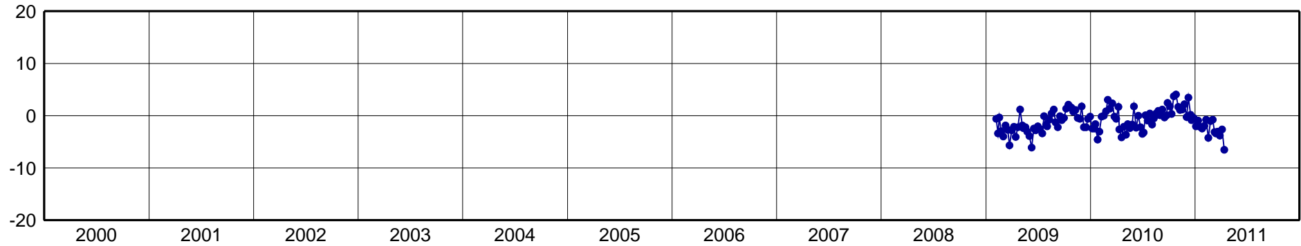
RNMO-North Component [mm]
