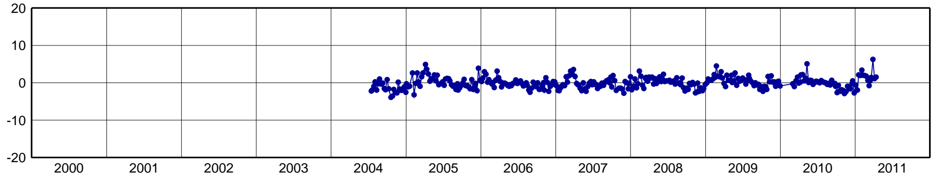
UBER-North Component [mm]
