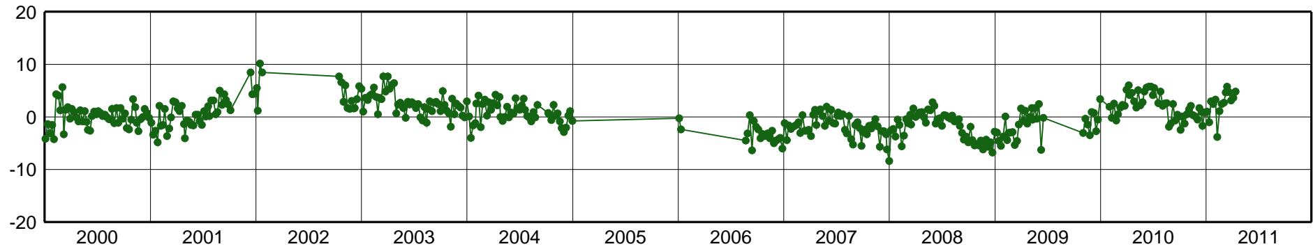
PARC-East Component [mm]
