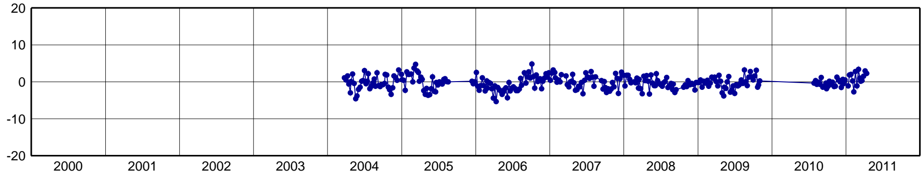
VALL-North Component [mm]
