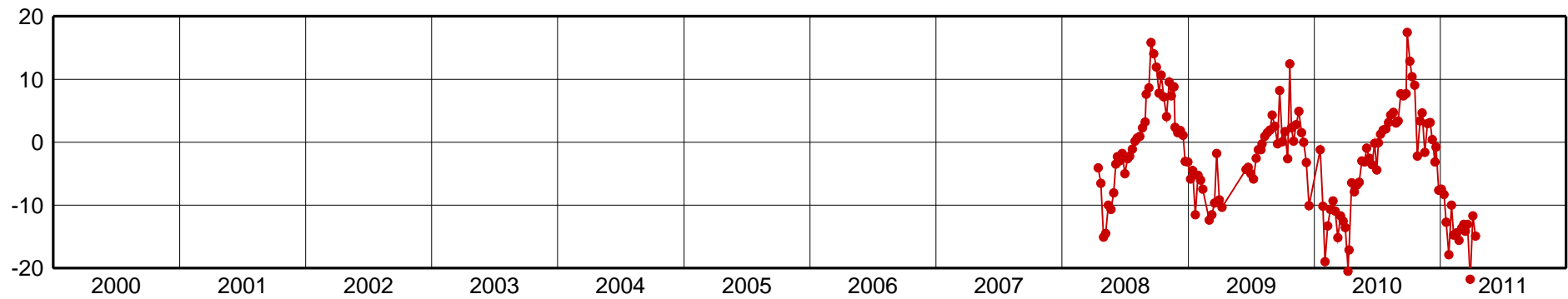
TOGU-Up Component [mm]
