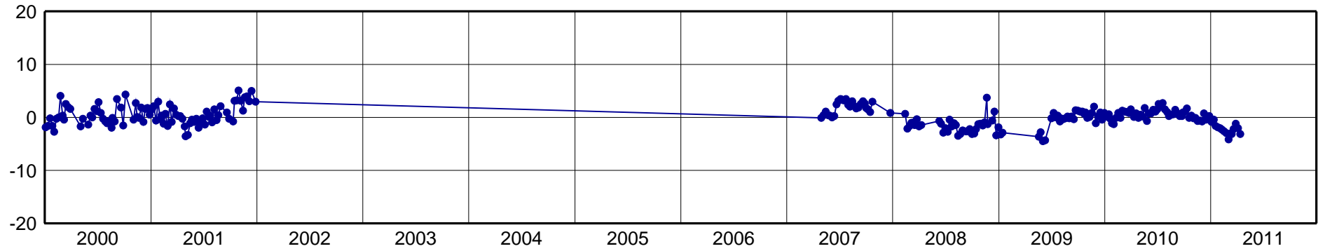
RIOP-North Component [mm]
