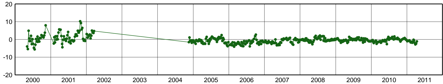
INEG-East Component [mm]
