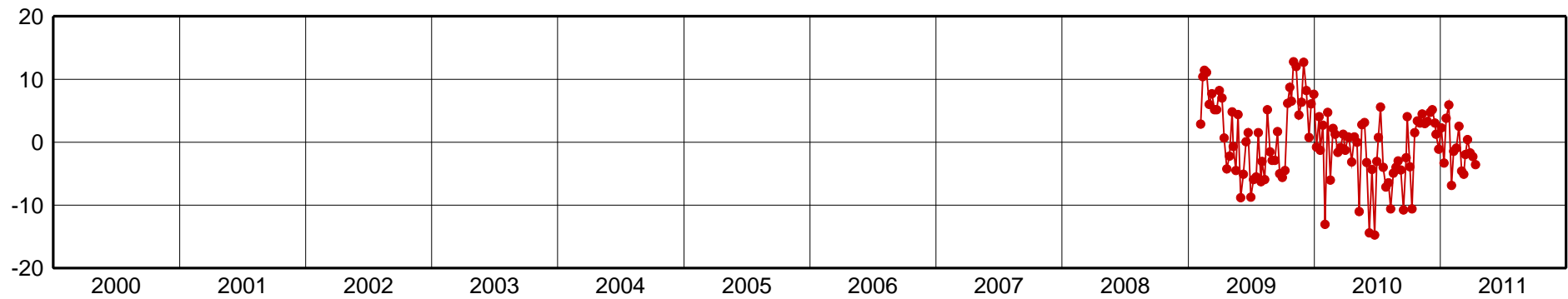
LJEC-Up Component [mm]
