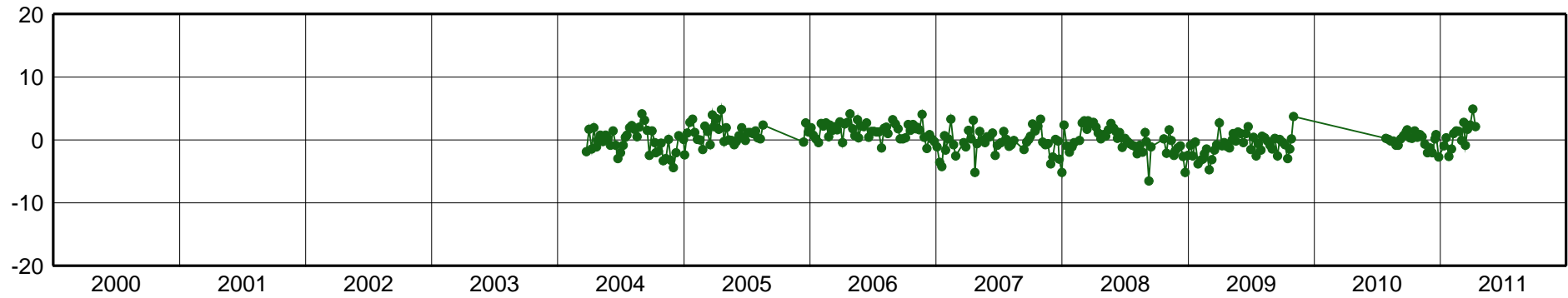
VALL-East Component [mm]
