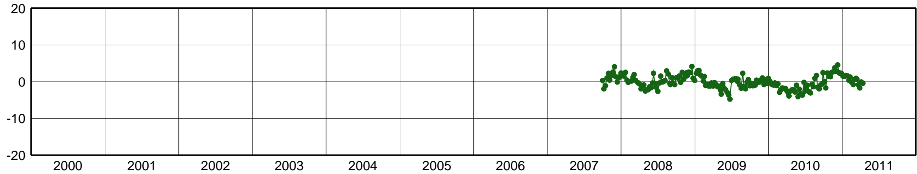
CULC-East Component [mm]
