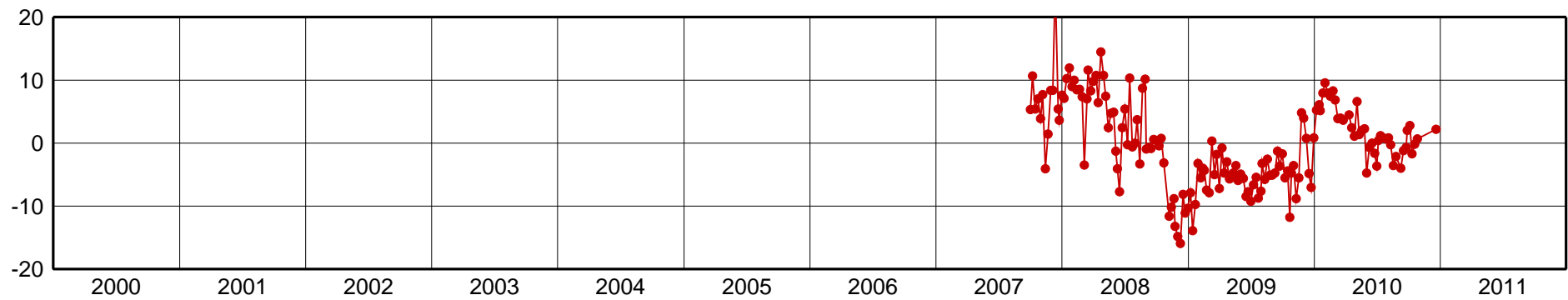
FQNE-Up Component [mm]
