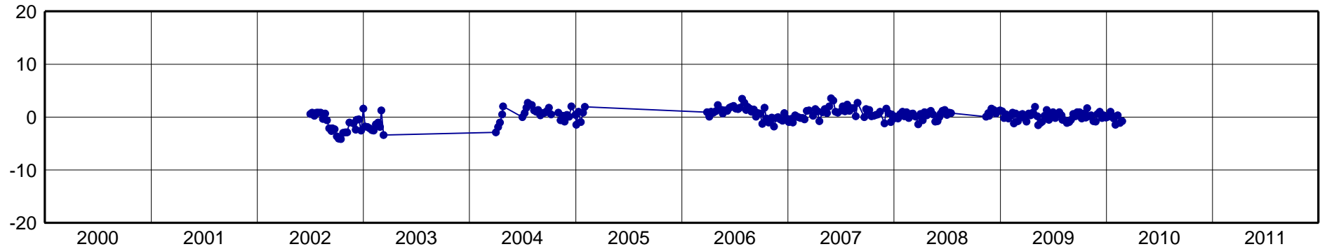
LHCL-North Component [mm]
