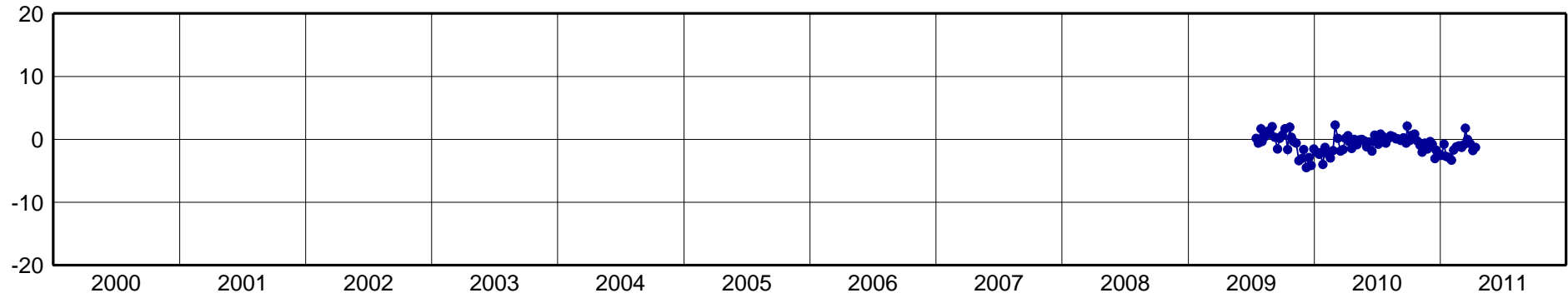
PISR-North Component [mm]
