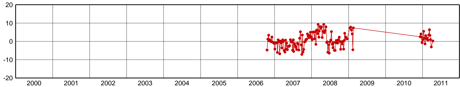
MECO-Up Component [mm]
