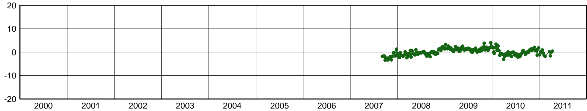
IMBT-East Component [mm]
