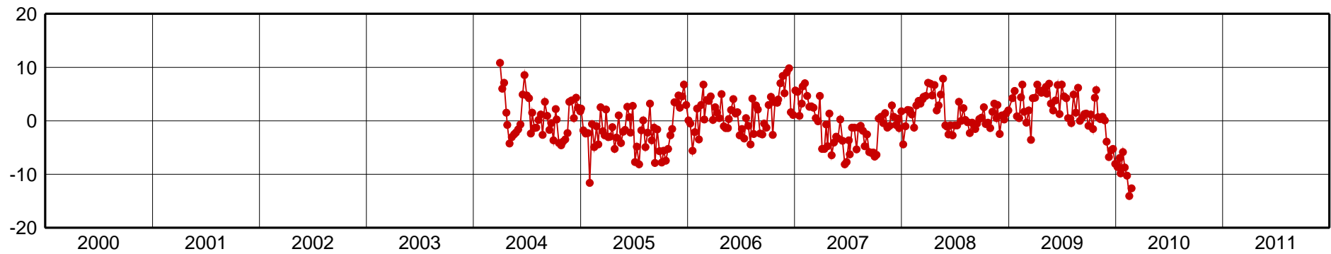
UNRO-Up Component [mm]
