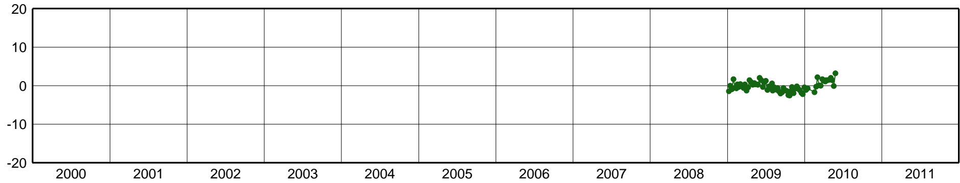
CASI-East Component [mm]
