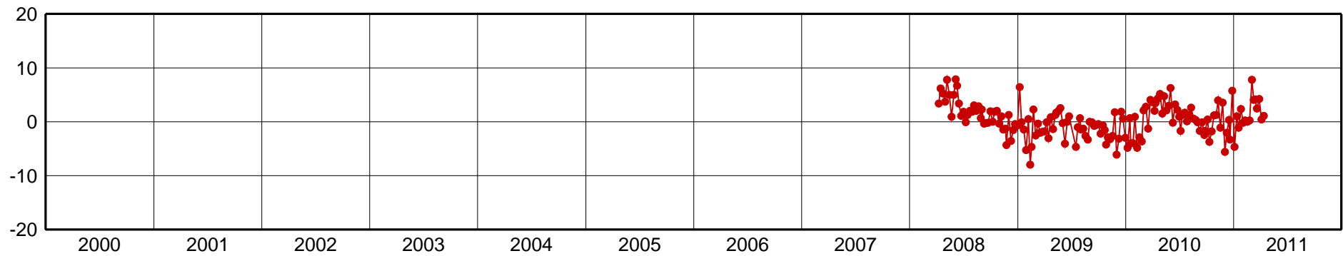
RJCG-Up Component [mm]
