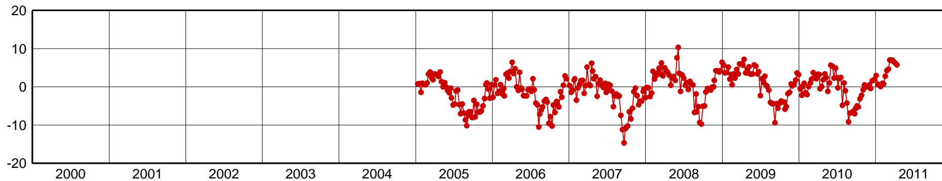
TOL2-Up Component [mm]
