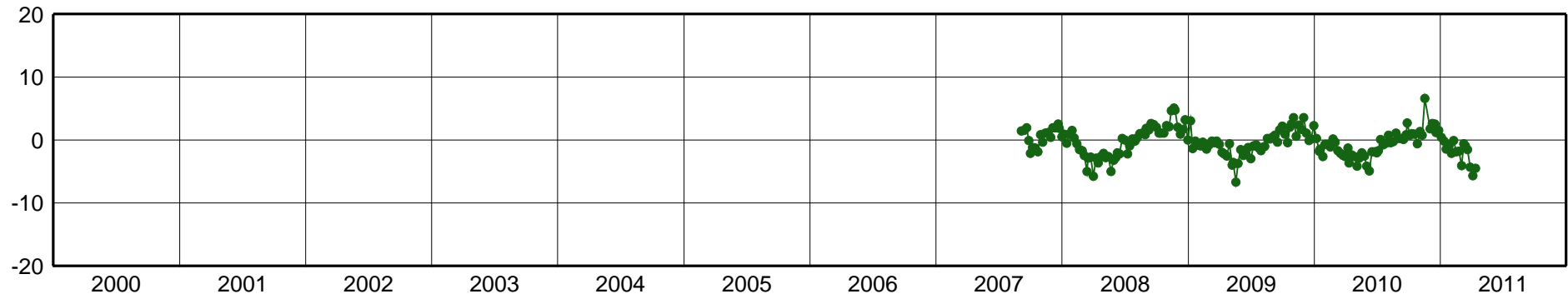
SAVO-East Component [mm]
