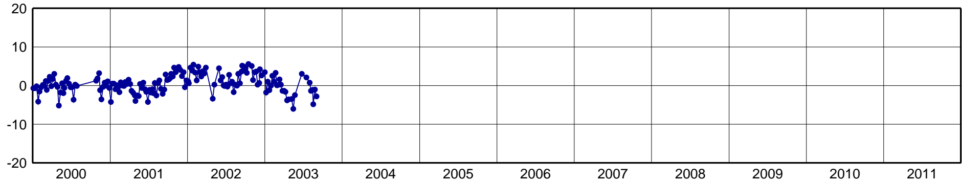
JAMA-North Component [mm]
