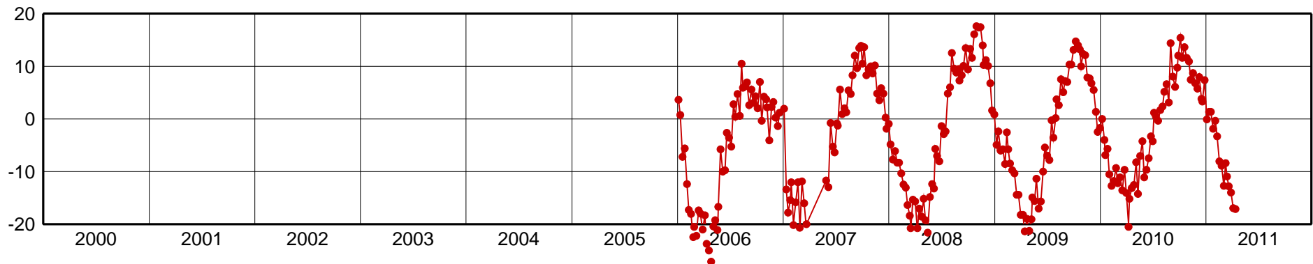
POVE-Up Component [mm]
