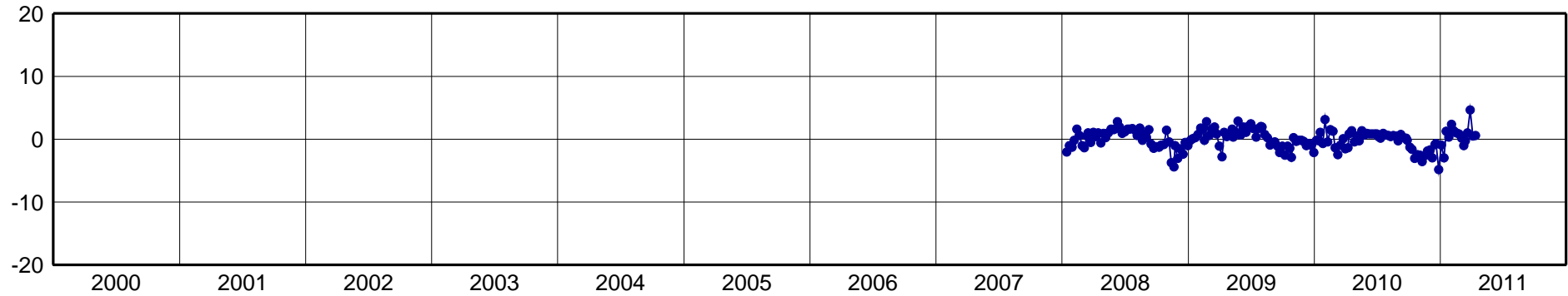
MGUB-North Component [mm]
