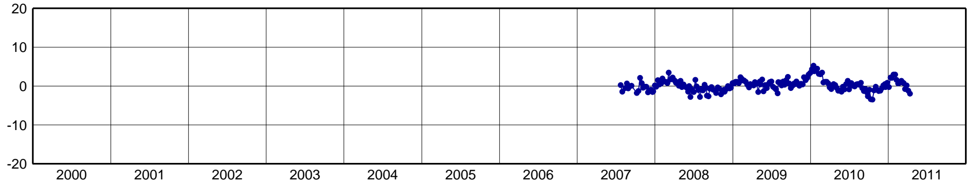
UGTO-North Component [mm]
