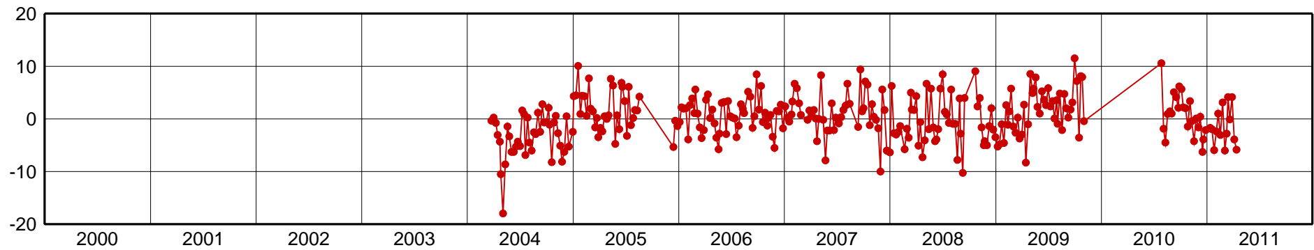
VALL-Up Component [mm]
