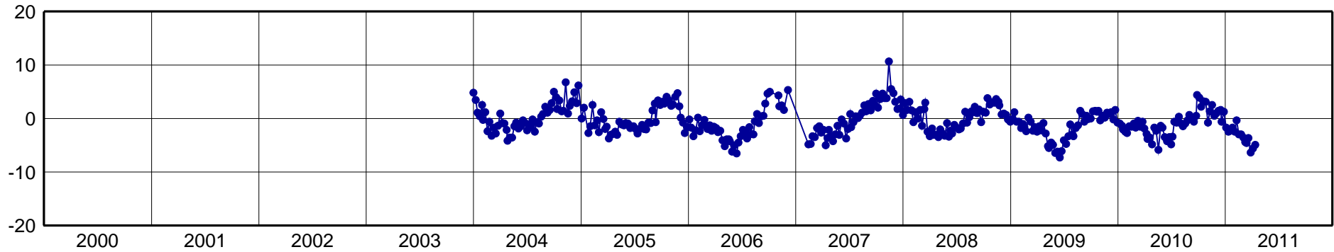
BELE-North Component [mm]
