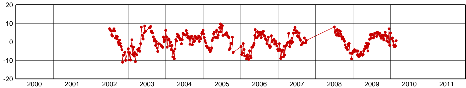
COPO-Up Component [mm]
