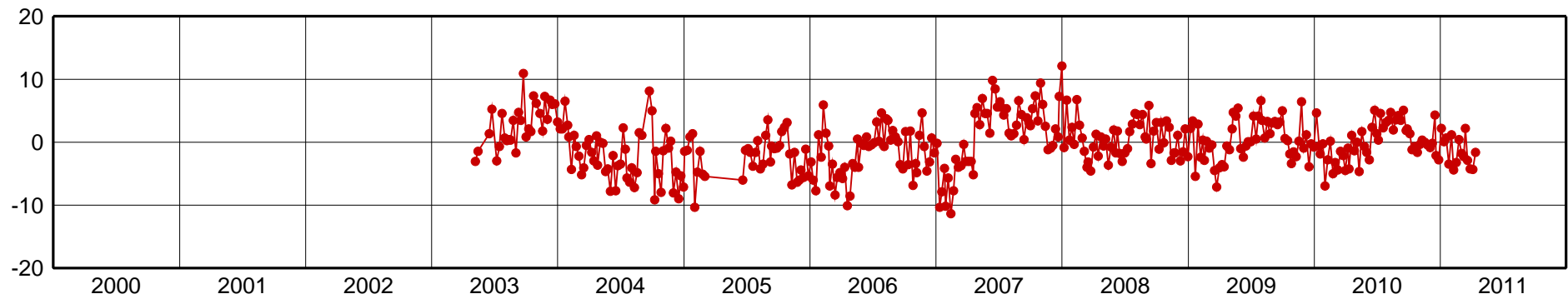
CHPI-Up Component [mm]
