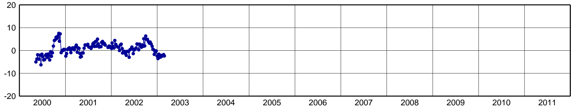
ESTI-North Component [mm]
