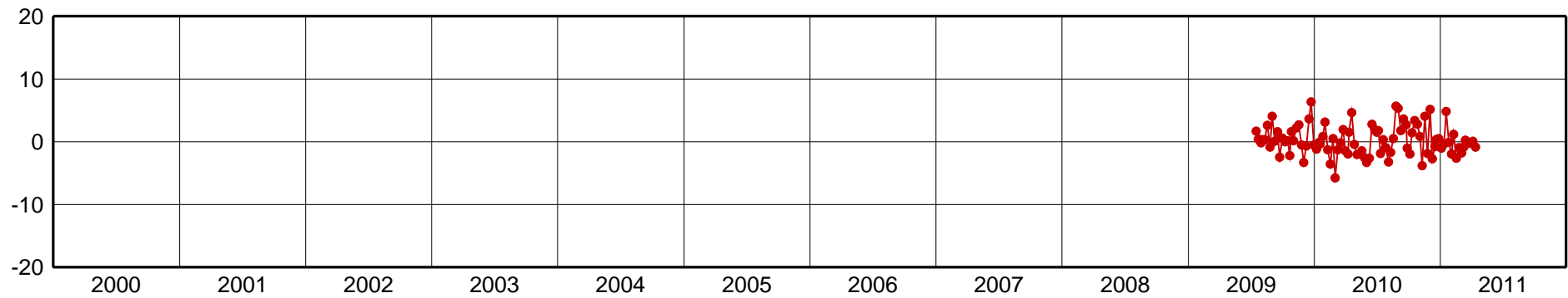
PRGU-Up Component [mm]
