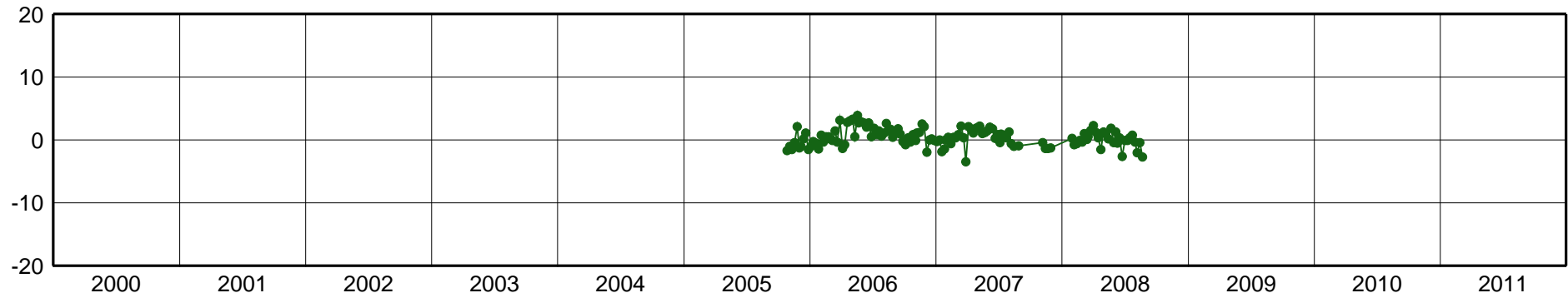
RIOH-East Component [mm]
