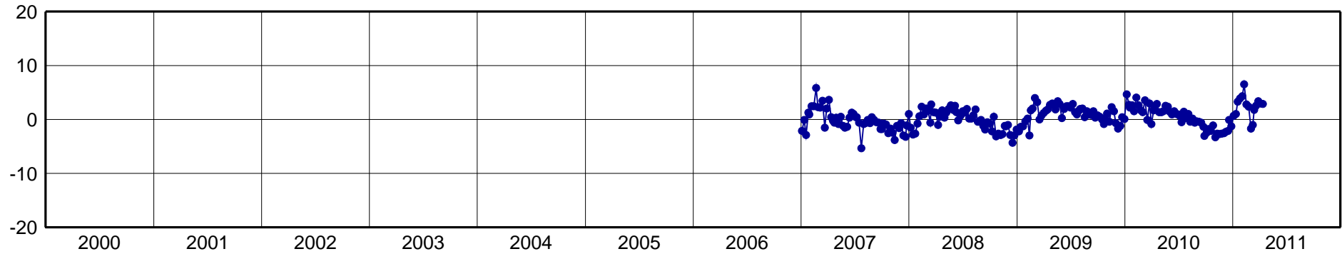
POLI-North Component [mm]
