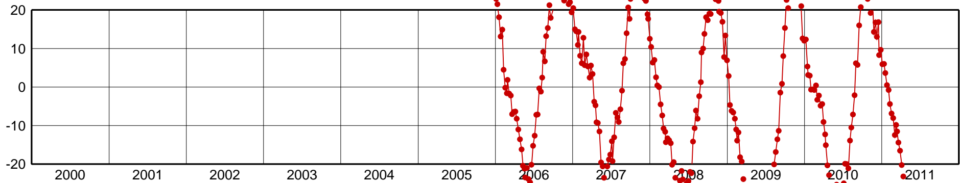
NAUS-Up Component [mm]
