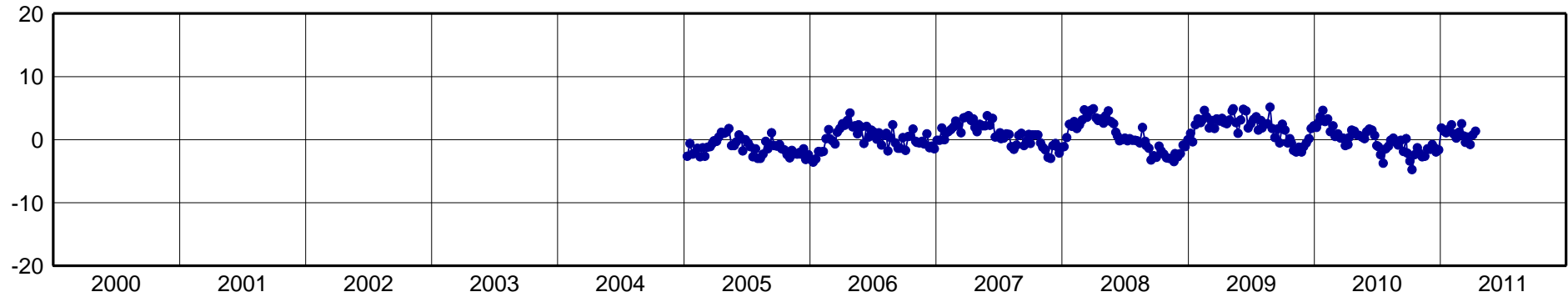
HER2-North Component [mm]
