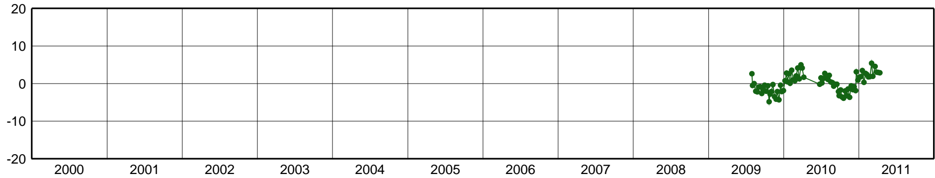
CALL-East Component [mm]
