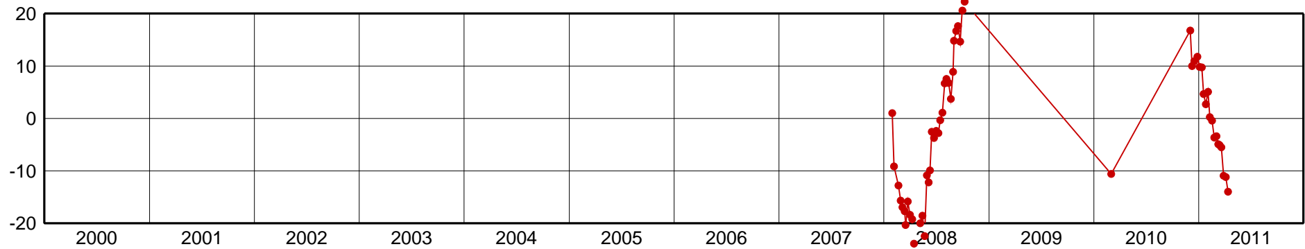
AMHU-Up Component [mm]
