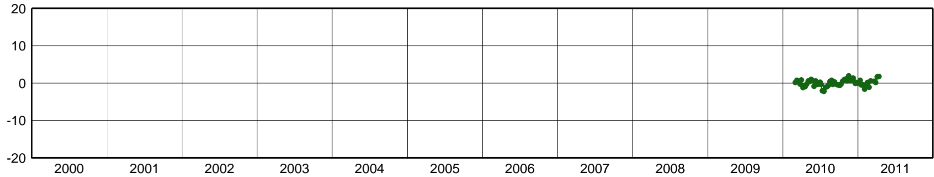
EBYP-East Component [mm]
