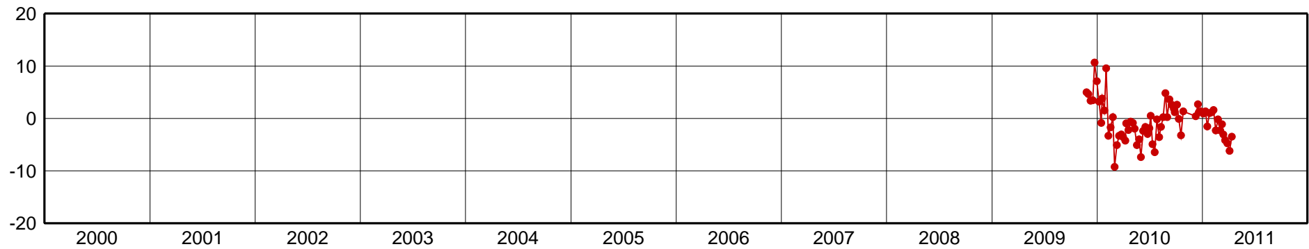
JBAL-Up Component [mm]
