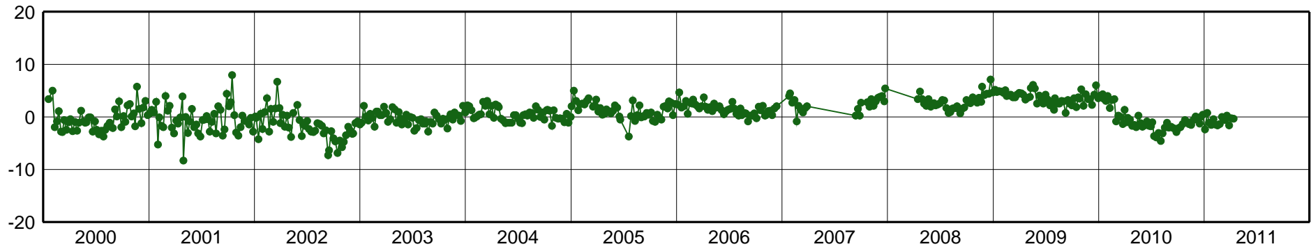
POAL-East Component [mm]
