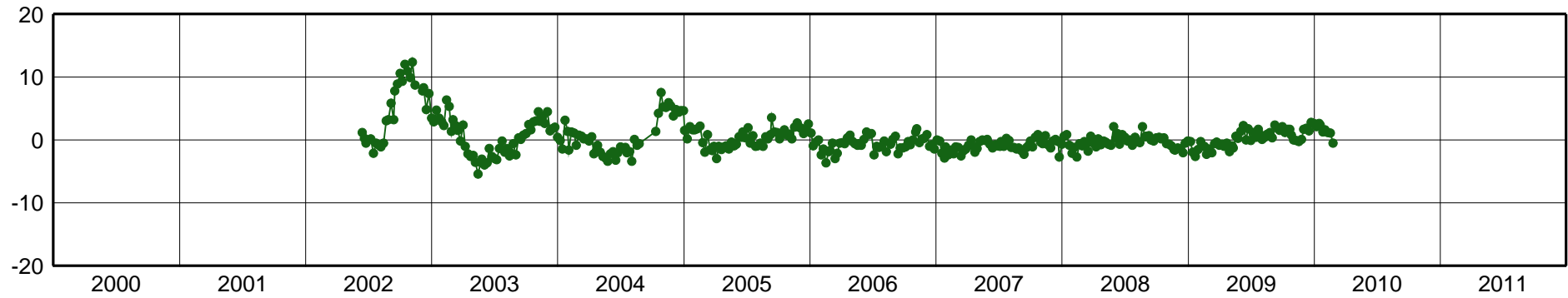
CONZ-East Component [mm]
