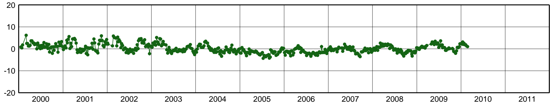
RWSN-East Component [mm]
