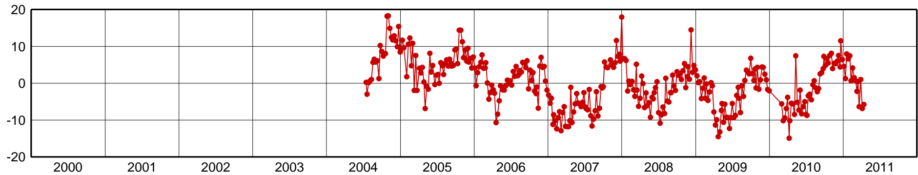
UBER-Up Component [mm]
