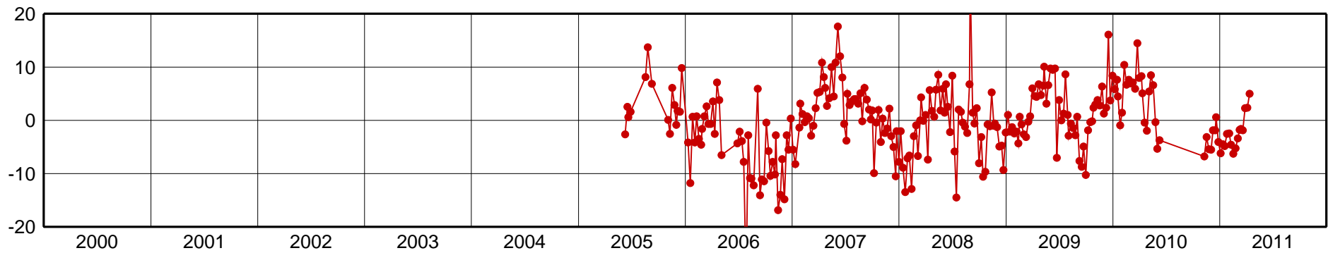
BDOS-Up Component [mm]
