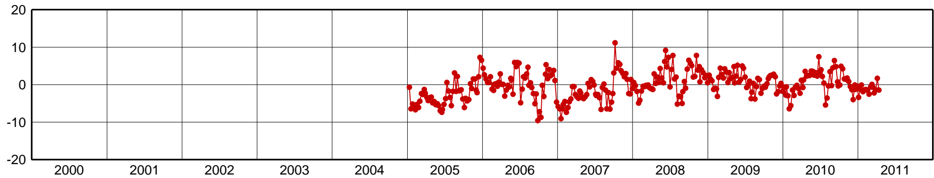
HER2-Up Component [mm]
