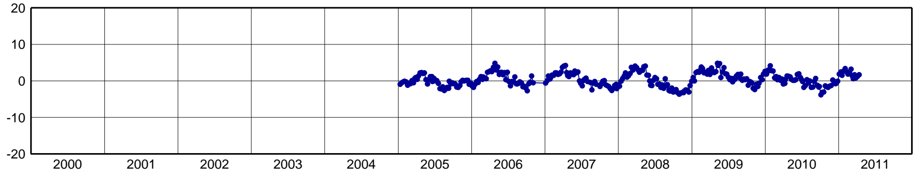
CHIH-North Component [mm]
