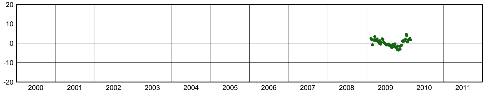
CATA-East Component [mm]
