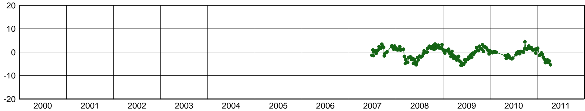
BRFT-East Component [mm]
