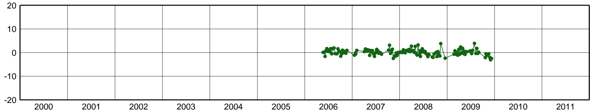
BANS-East Component [mm]
