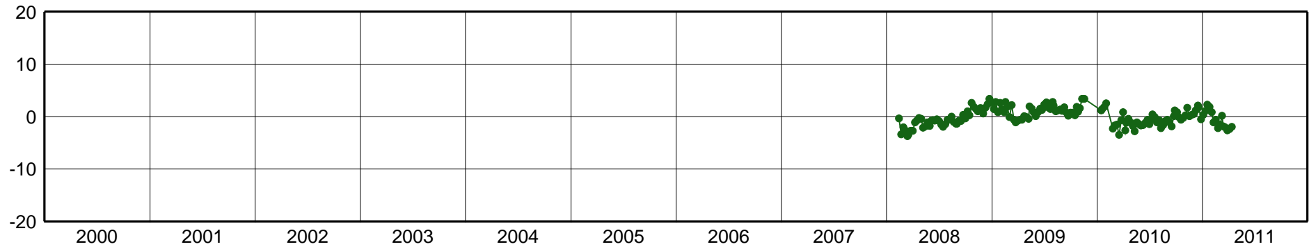
MGIN-East Component [mm]
