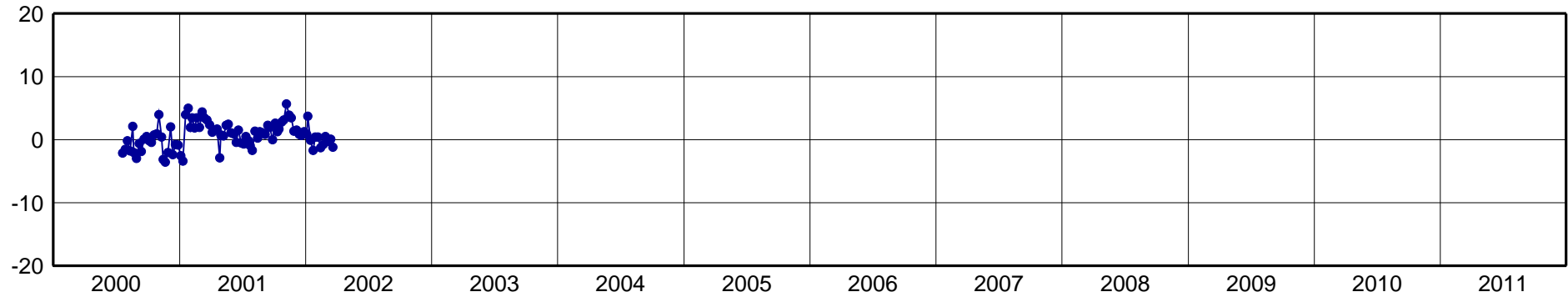
TEGU-North Component [mm]
