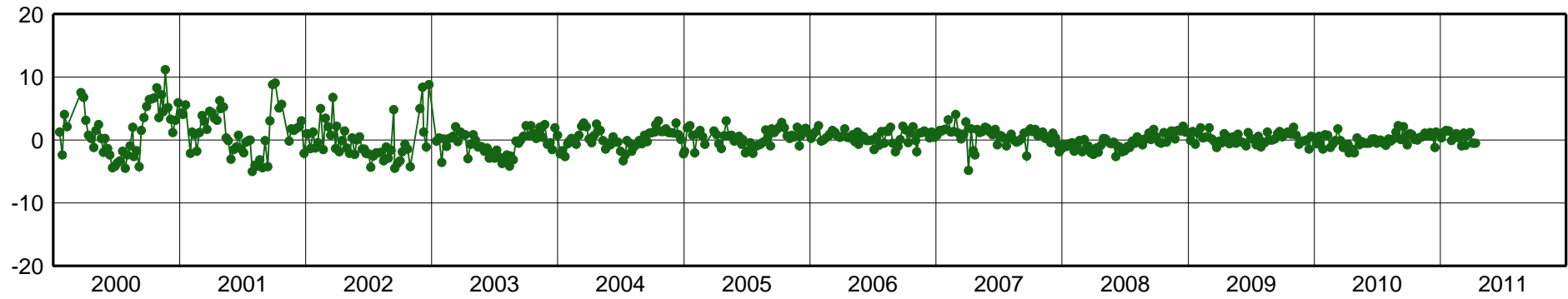
CUIB-East Component [mm]
