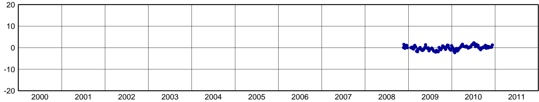
CUEC-North Component [mm]
