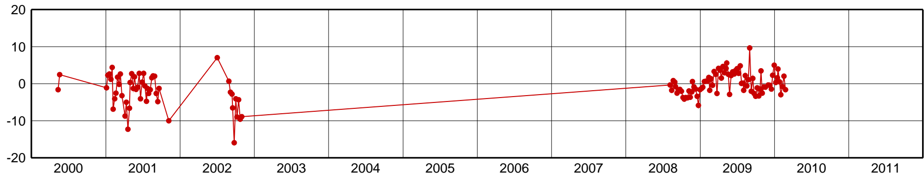
VALP-Up Component [mm]
