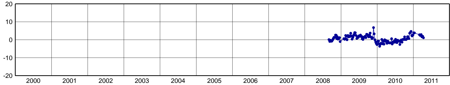
GYEC-North Component [mm]
