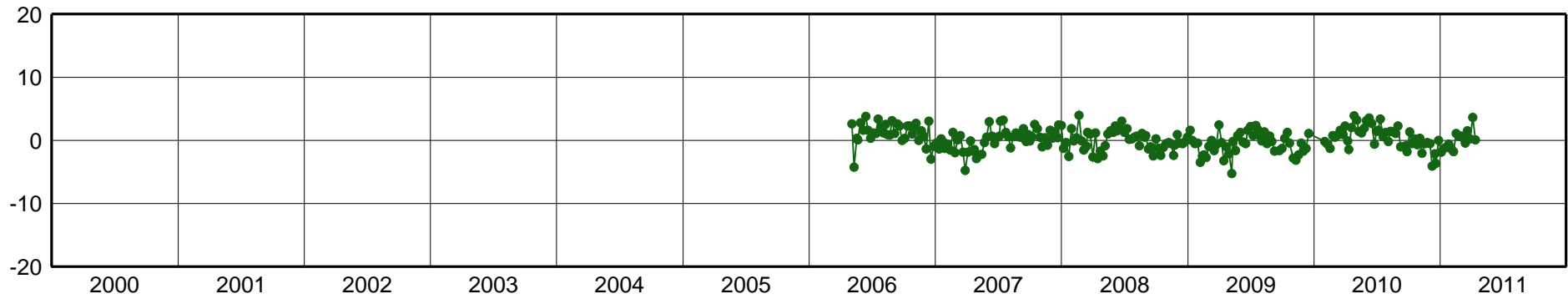
SAMA-East Component [mm]
