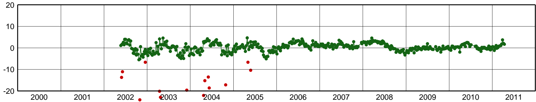
BOGT-East Component [mm]
