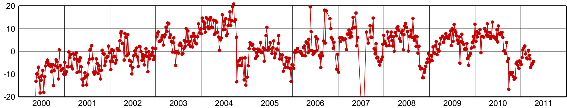
MANA-Up Component [mm]
