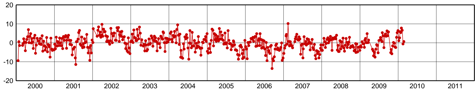
RWSN-Up Component [mm]
