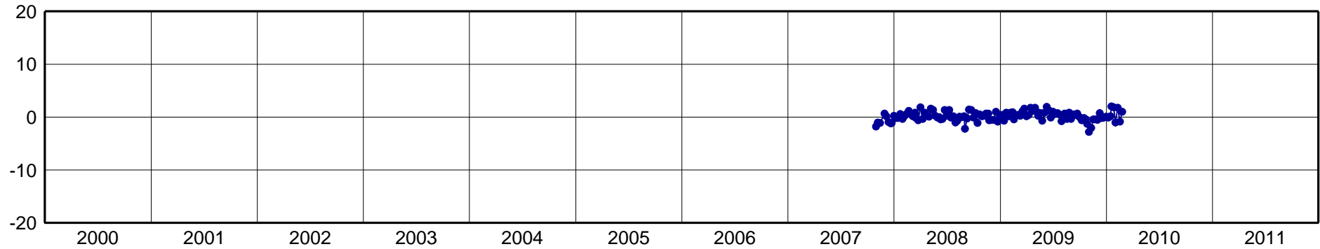
UYMO-North Component [mm]
