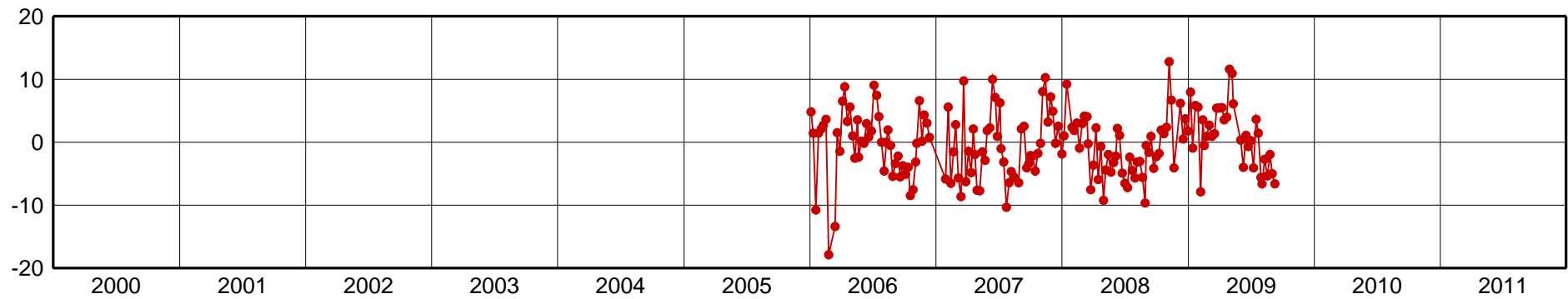
UBAT-Up Component [mm]
