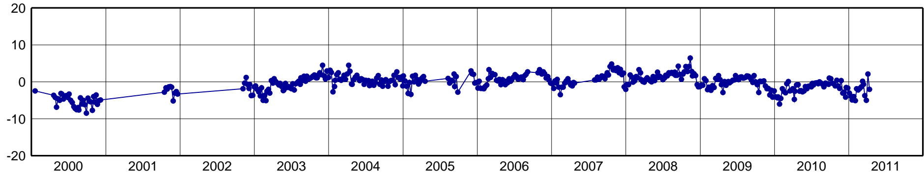
BOMJ-North Component [mm]
