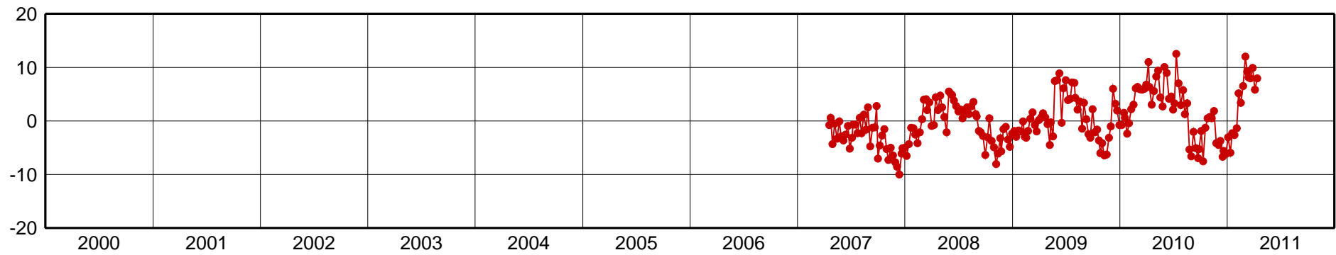
RIO2-Up Component [mm]
