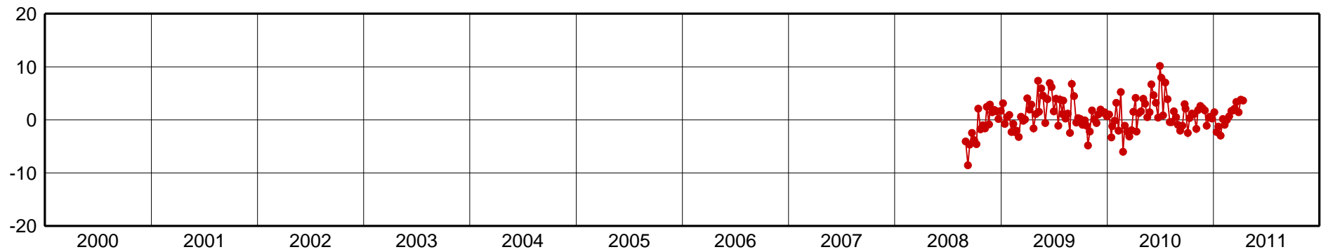
USLP-Up Component [mm]
