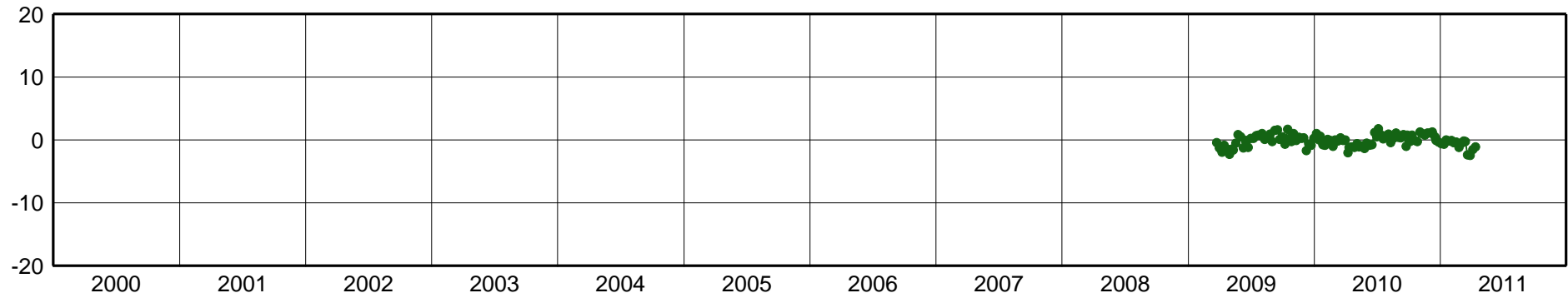
IDGO-East Component [mm]
