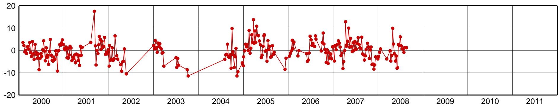
CART-Up Component [mm]
