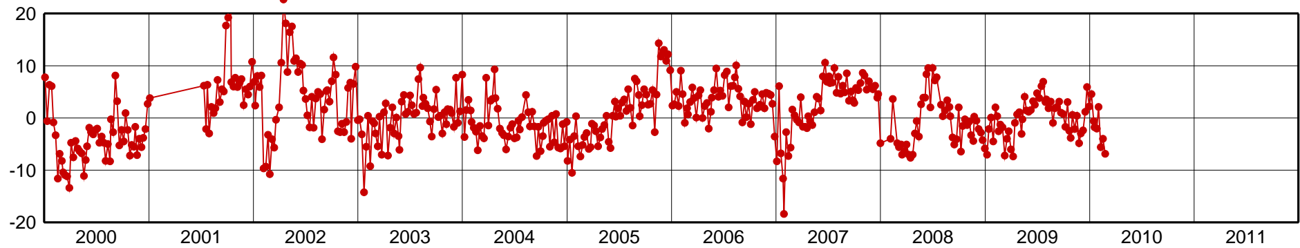
UNSA-Up Component [mm]
