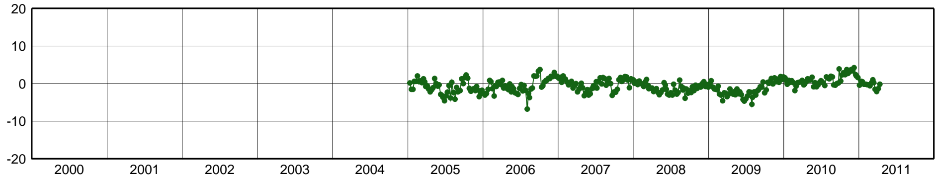
HER2-East Component [mm]
