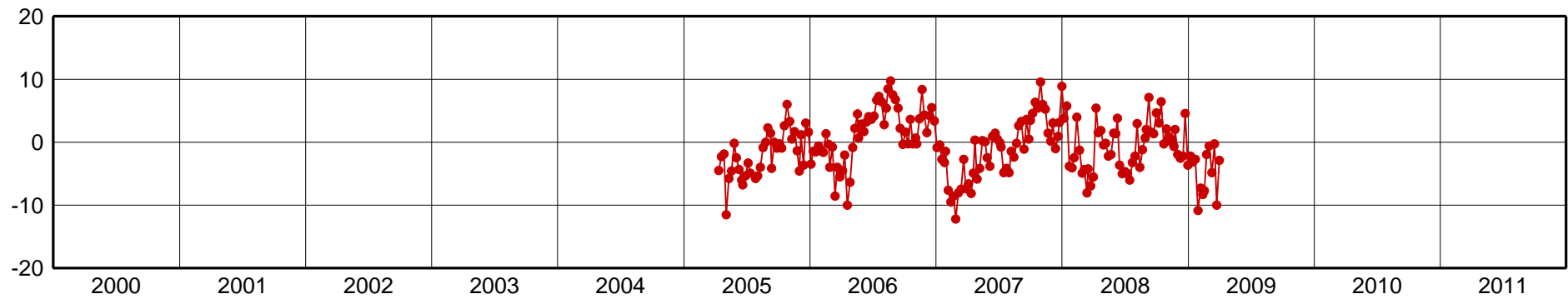
VARG-Up Component [mm]
