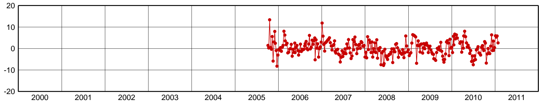
BUEN-Up Component [mm]
