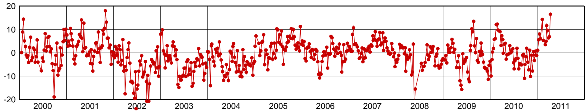
MARA-Up Component [mm]
