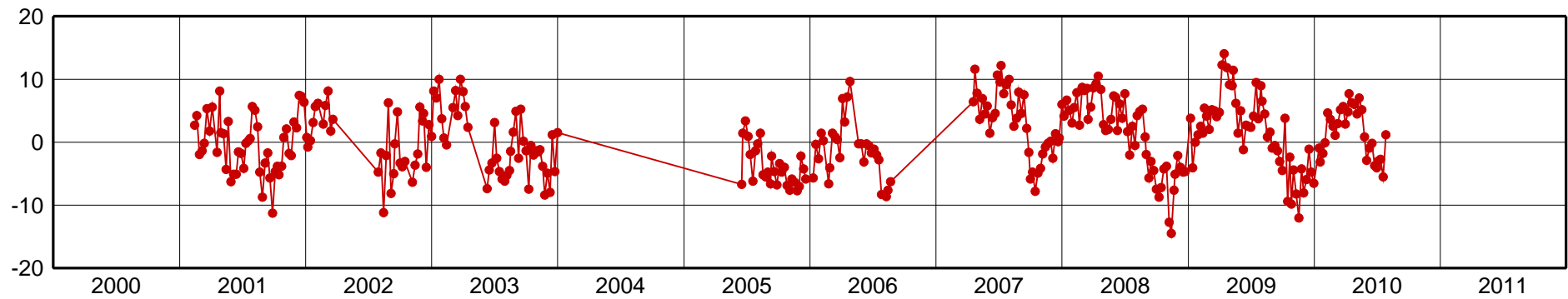
SSIA-Up Component [mm]
