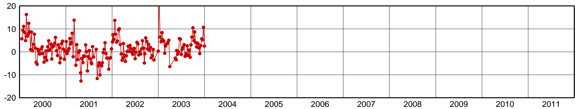
IGM0-Up Component [mm]
