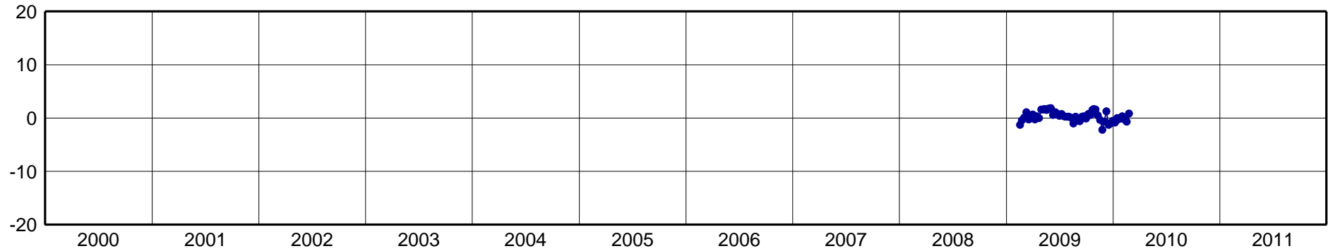
ALUM-North Component [mm]
