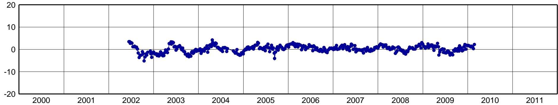
CONZ-North Component [mm]
