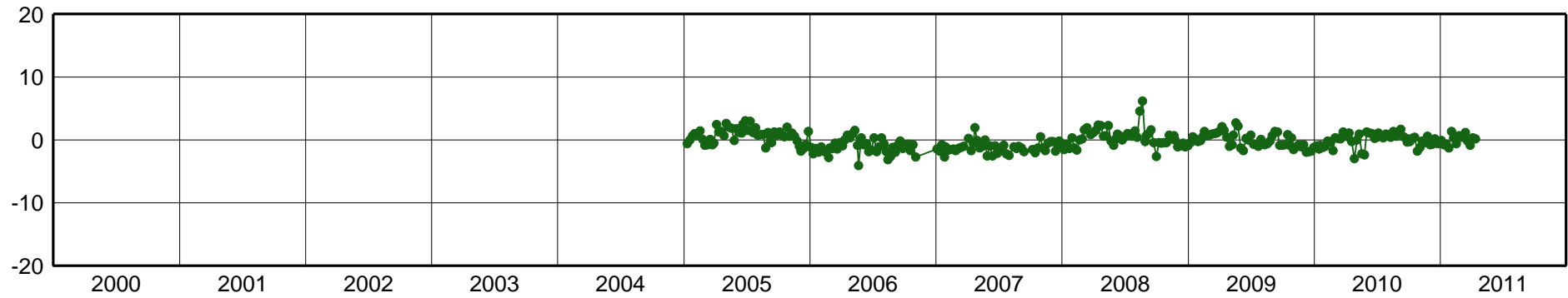
VIL2-East Component [mm]
