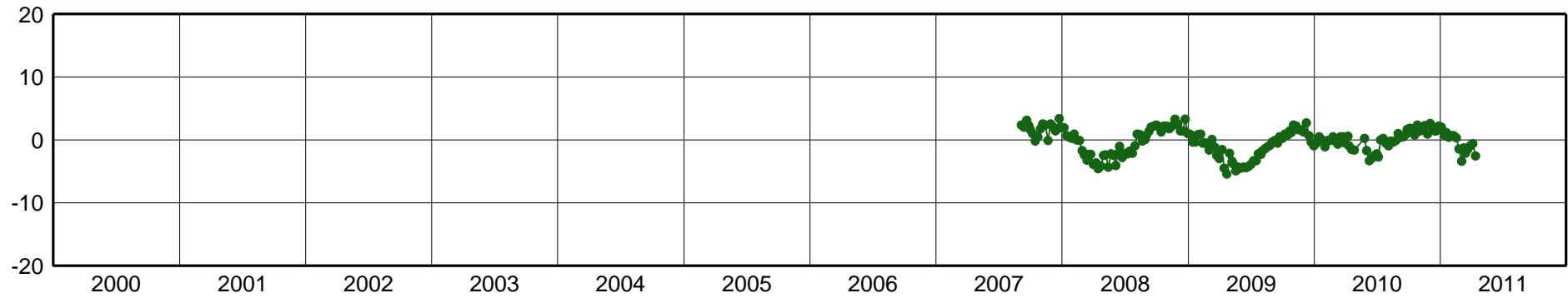
SALU-East Component [mm]
