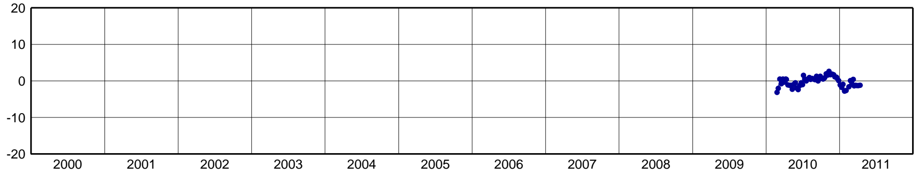
ABCC-North Component [mm]
