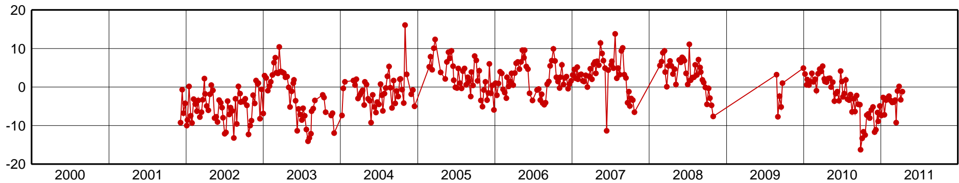
ELEN-Up Component [mm]
