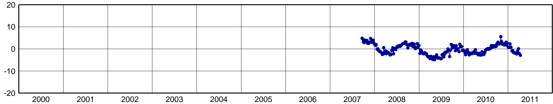
SAGA-North Component [mm]
