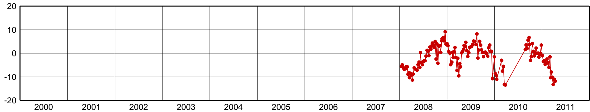
MSCG-Up Component [mm]
