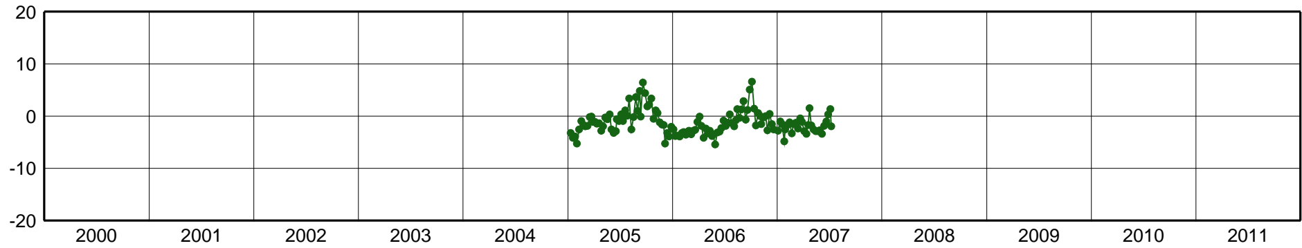
CULI-East Component [mm]
