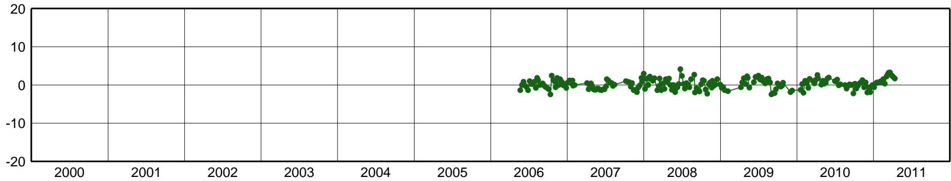
CRCS-East Component [mm]
