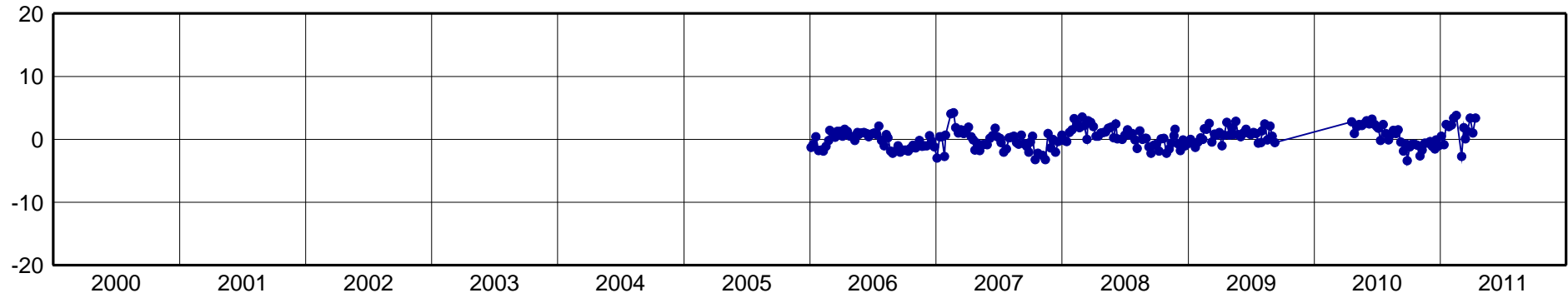
NEIA-North Component [mm]
