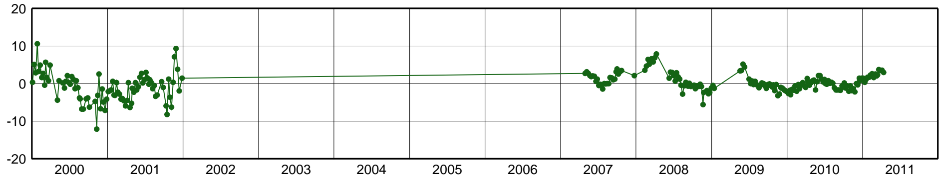
RIOP-East Component [mm]
