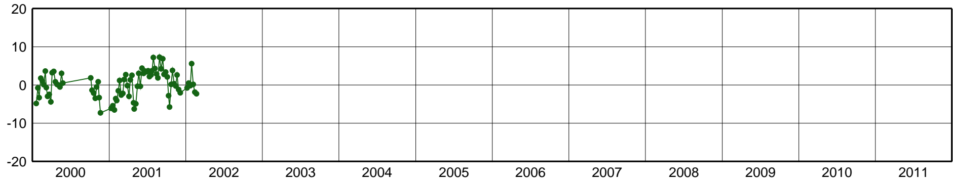
OHIG-East Component [mm]
