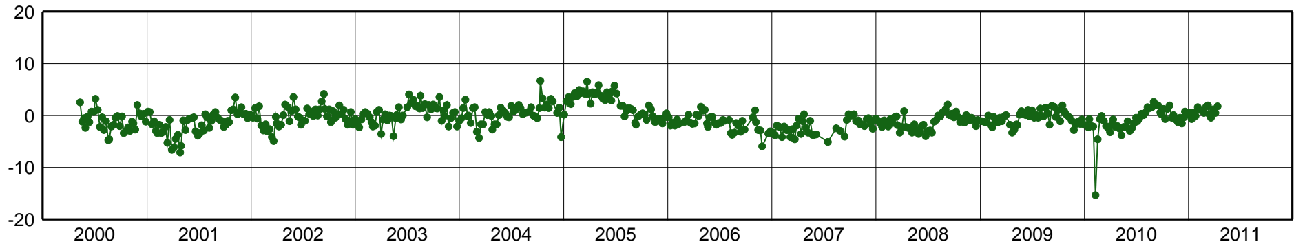
MANA-East Component [mm]
