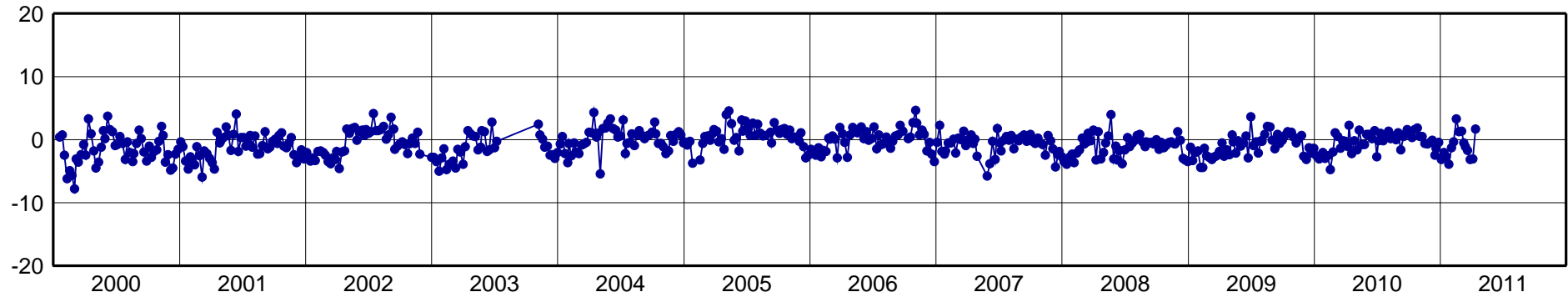
RECF-North Component [mm]
