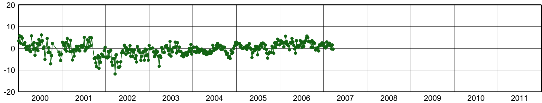
PUR3-East Component [mm]
