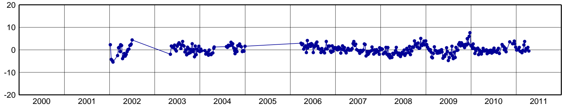
AUTF-North Component [mm]
