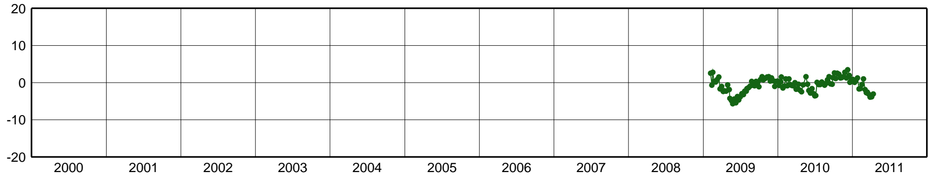
RNNA-East Component [mm]
