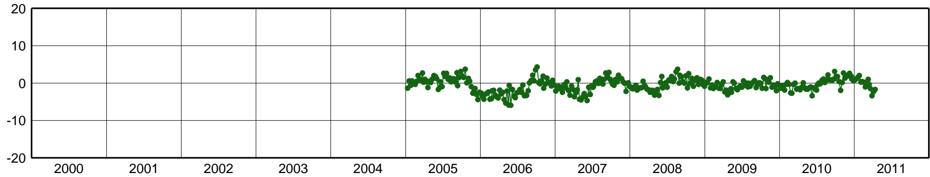
COL2-East Component [mm]
