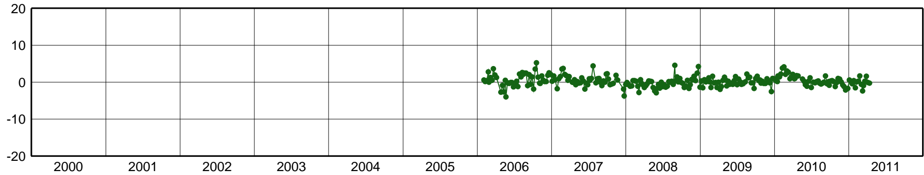
SRZN-East Component [mm]
