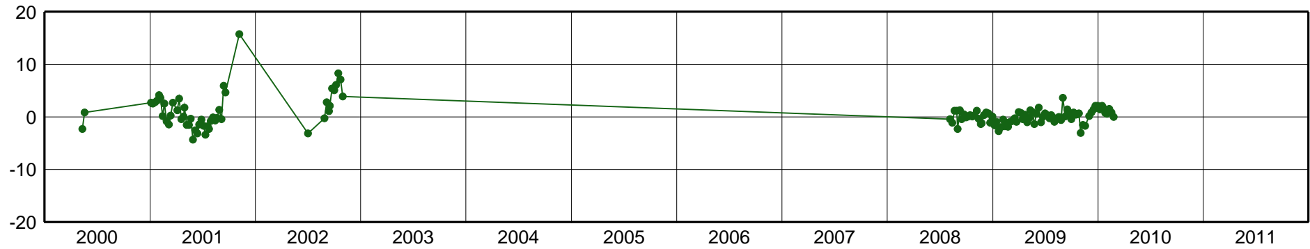
VALP-East Component [mm]
