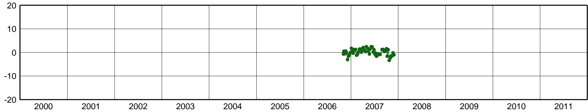
TUMA-East Component [mm]
