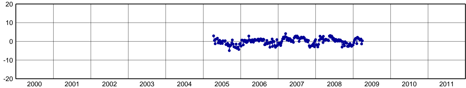
VARG-North Component [mm]
