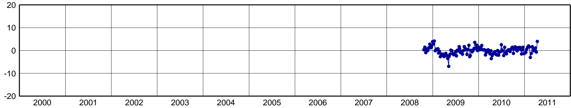
IGN1-North Component [mm]
