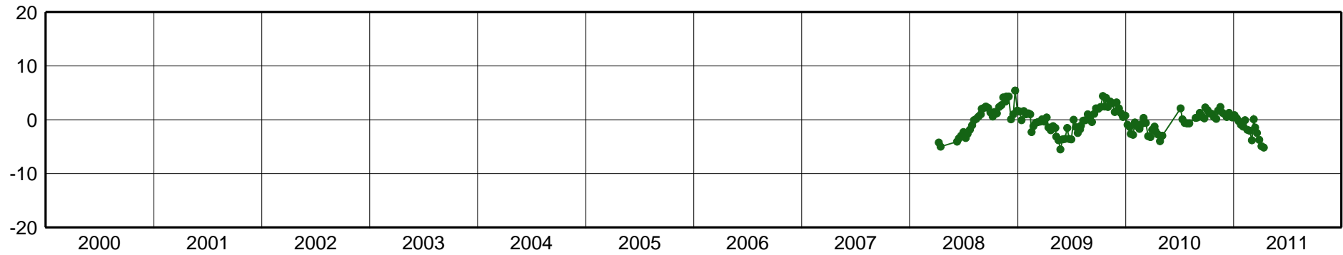
ALAR-East Component [mm]
