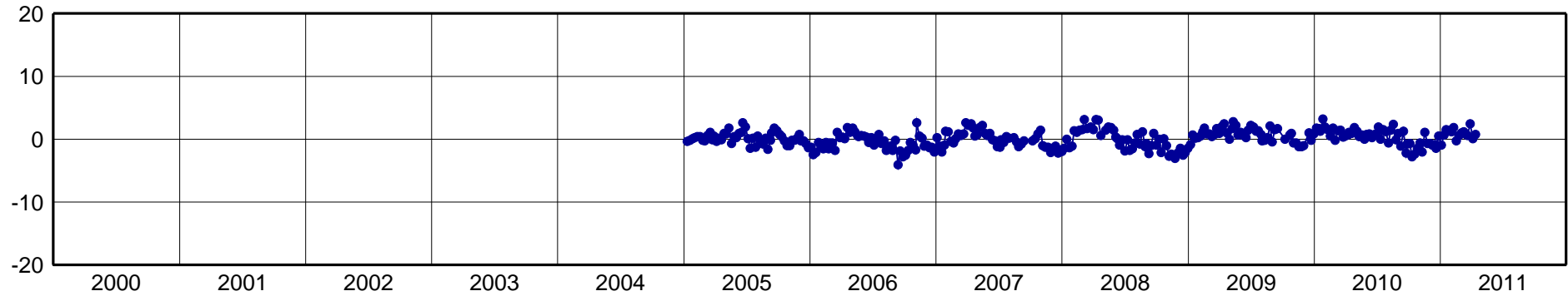
TAMP-North Component [mm]
