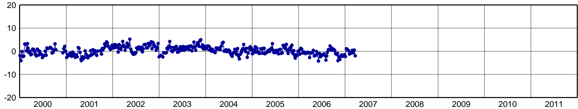
PUR3-North Component [mm]
