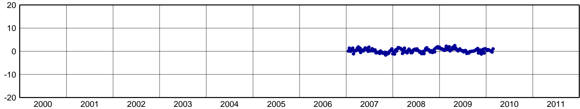
MZAS-North Component [mm]
