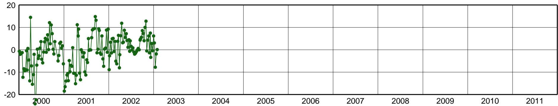
EISL-East Component [mm]
