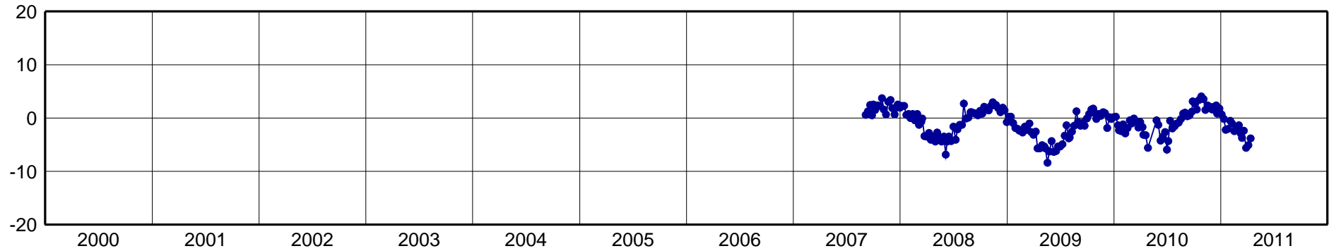
SALU-North Component [mm]
