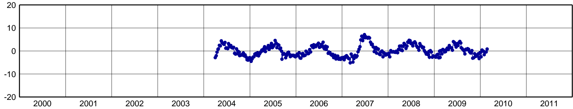
UNRO-North Component [mm]
