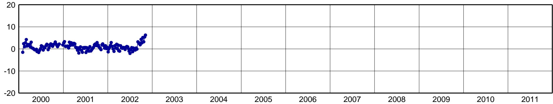
GALA-North Component [mm]
