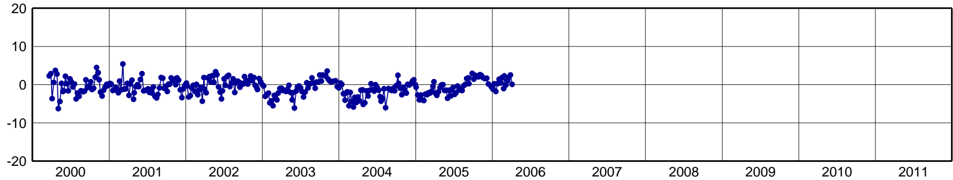
FORT-North Component [mm]
