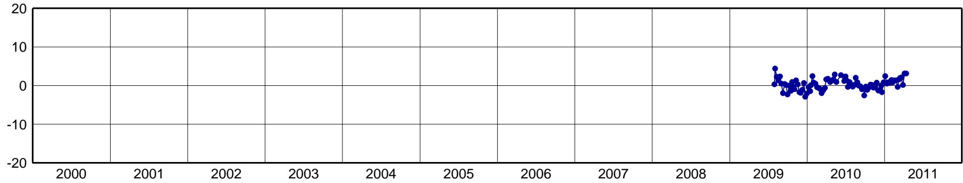
SVIC-North Component [mm]
