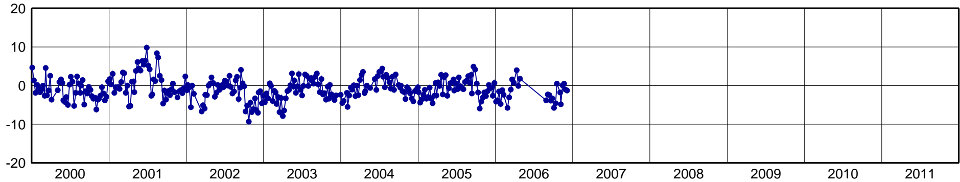
Goug-North Component [mm]
