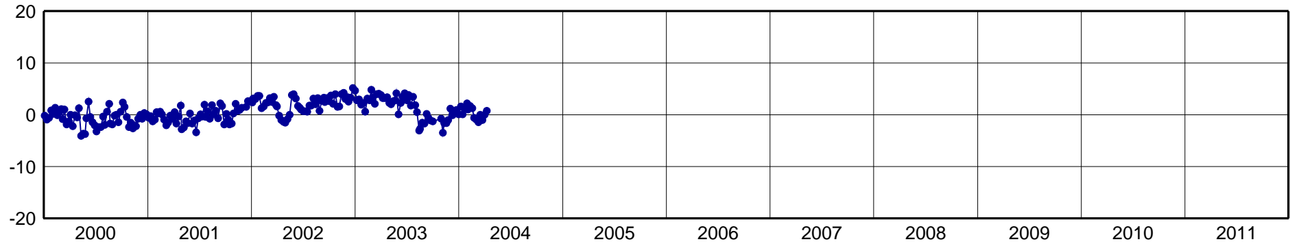
AOML-North Component [mm]
