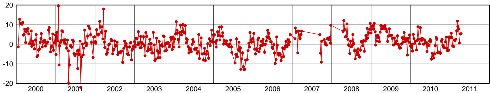
POAL-Up Component [mm]
