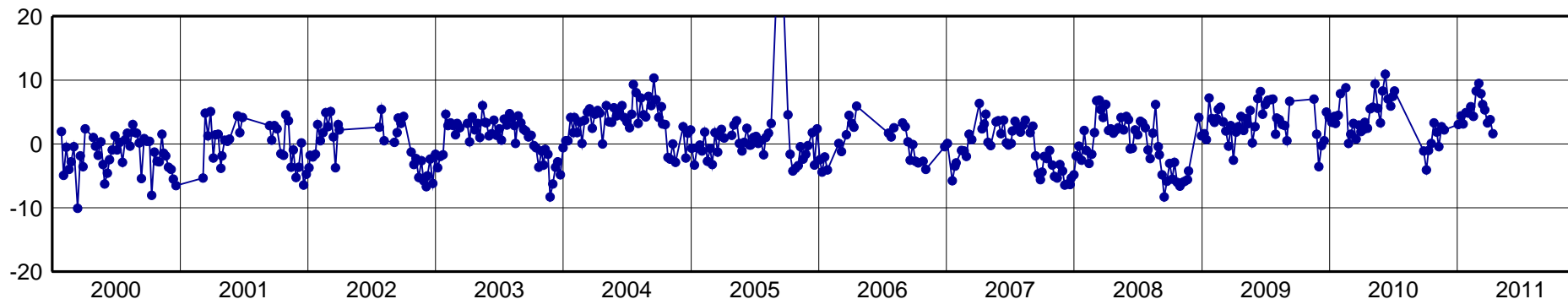
VESL-North Component [mm]
