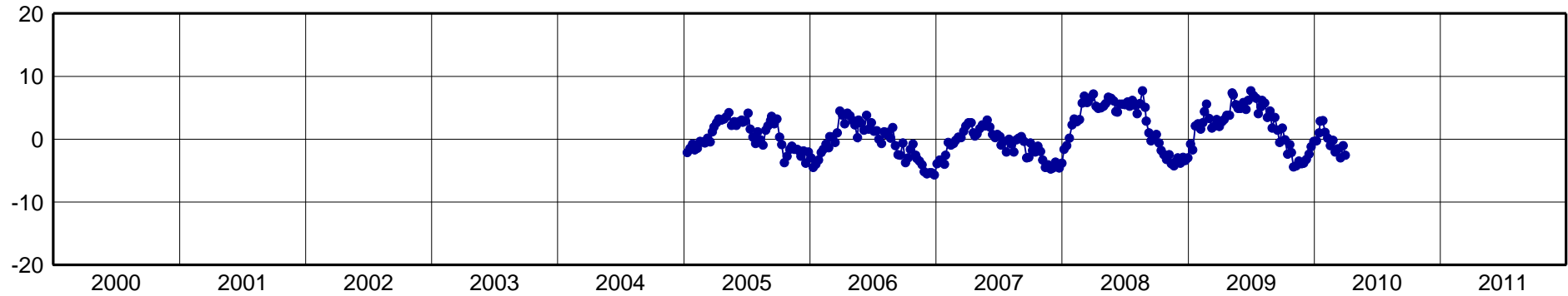
MEXI-North Component [mm]
