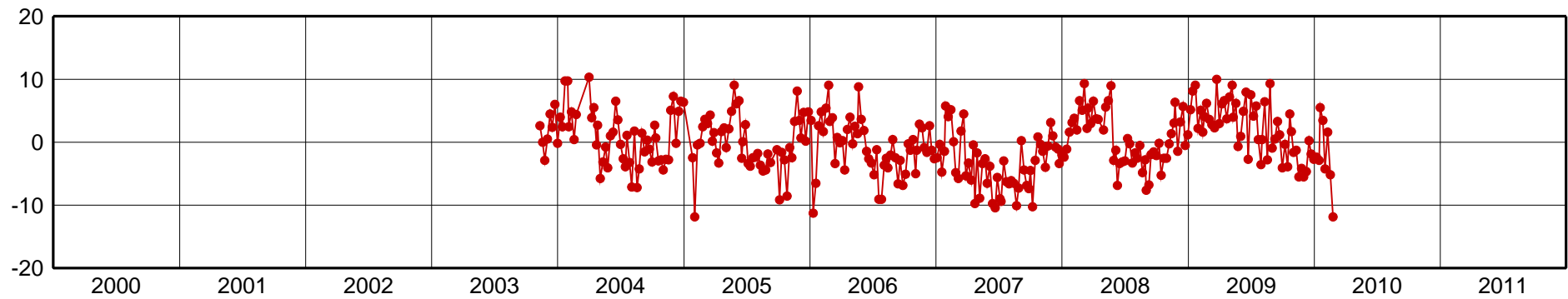
IGM1-Up Component [mm]
