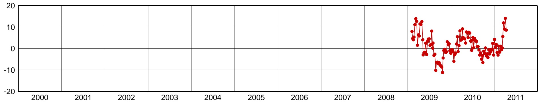
RNMO-Up Component [mm]
