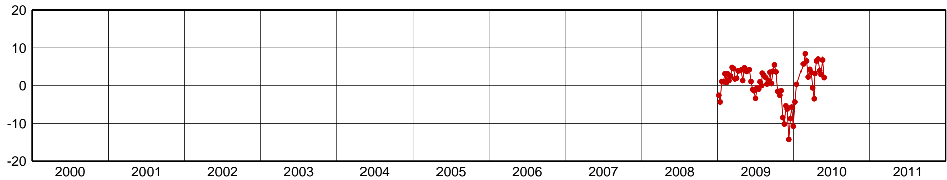
CASI-Up Component [mm]
