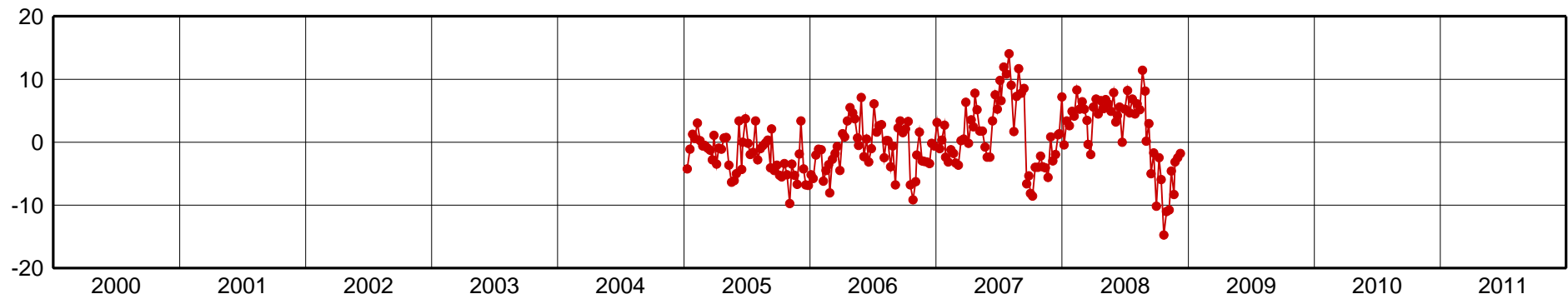
CAM2-Up Component [mm]
