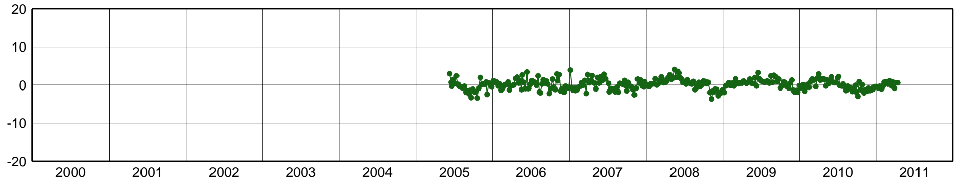
GCGT-East Component [mm]
