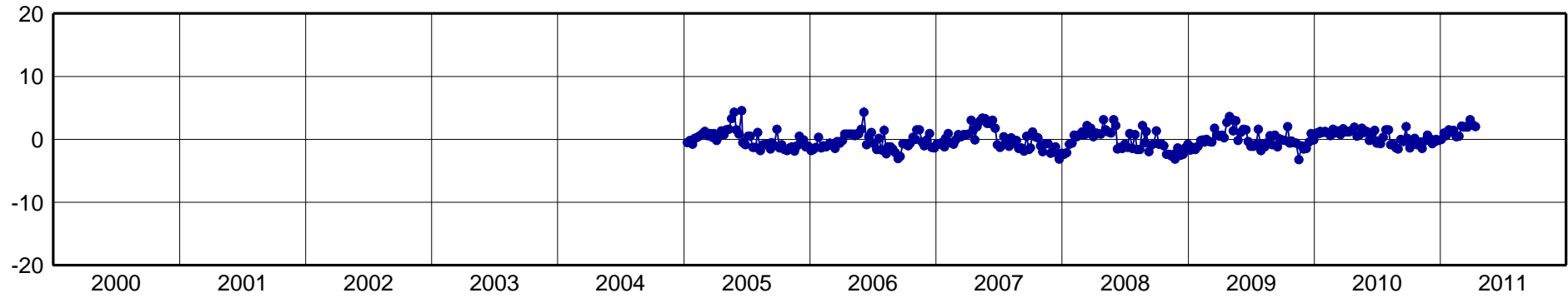
MERI-North Component [mm]
