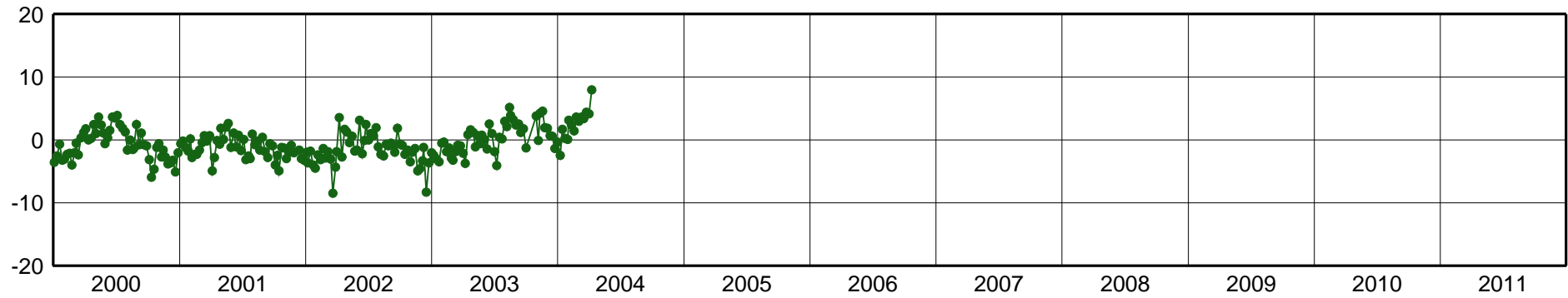
AOML-East Component [mm]
