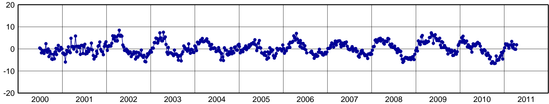
GOLD-North Component [mm]
