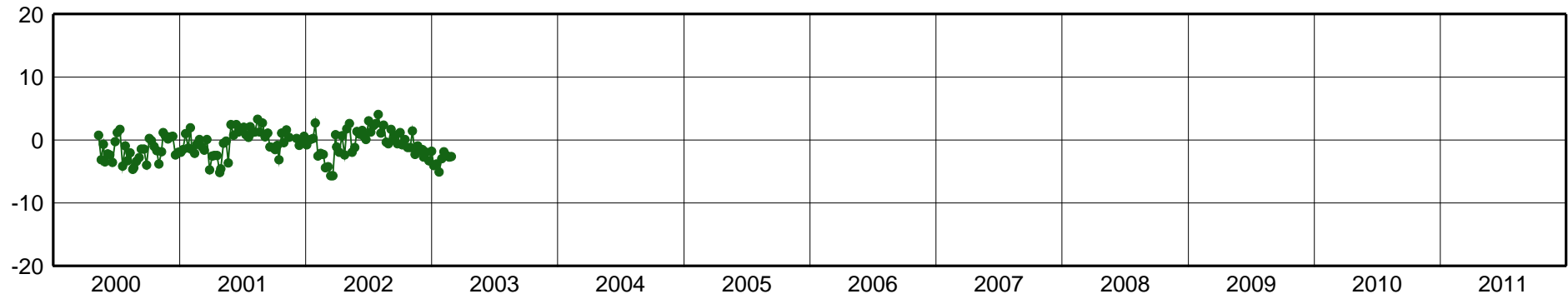
ESTI-East Component [mm]
