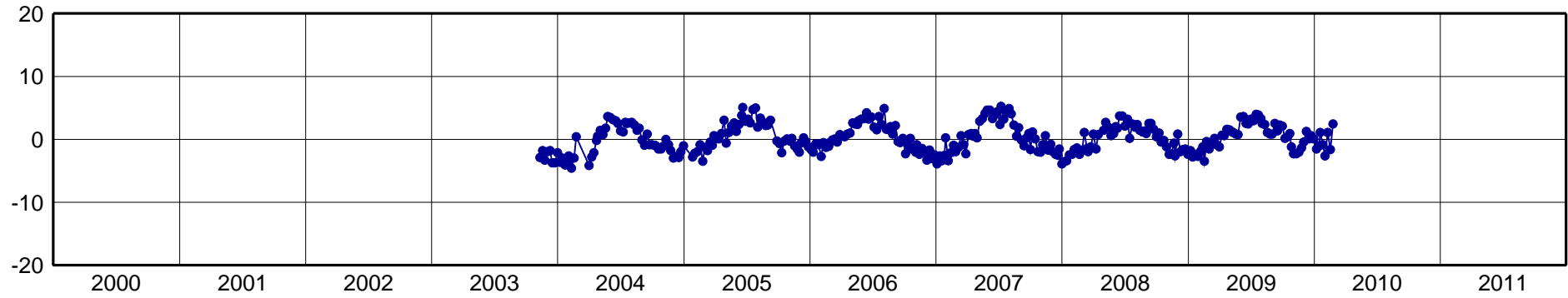
IGM1-North Component [mm]
