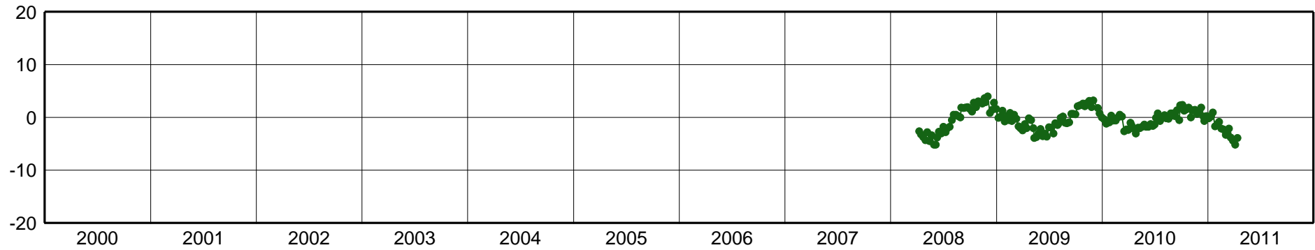
PBCG-East Component [mm]
