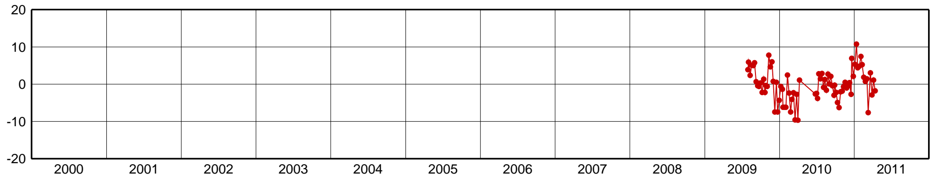
CALL-Up Component [mm]
