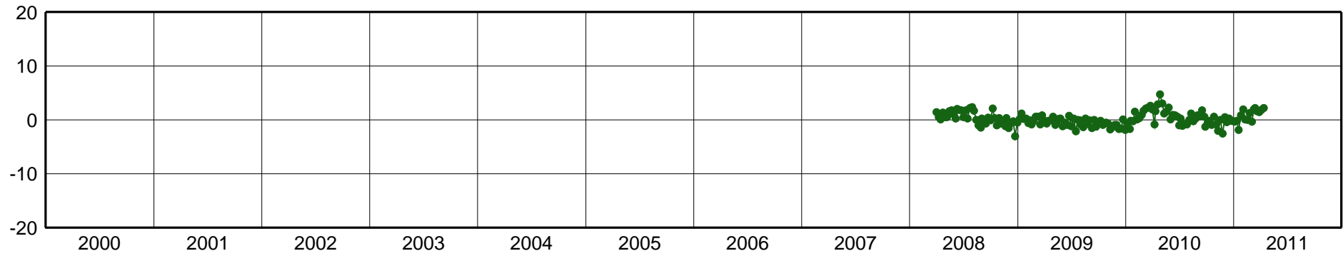
ROJI-East Component [mm]
