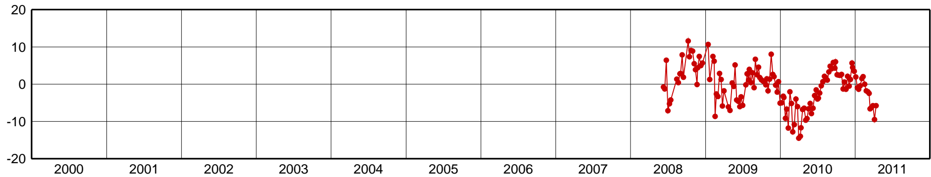
GOJA-Up Component [mm]
