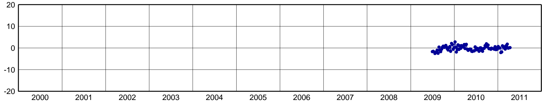
ESMR-North Component [mm]
