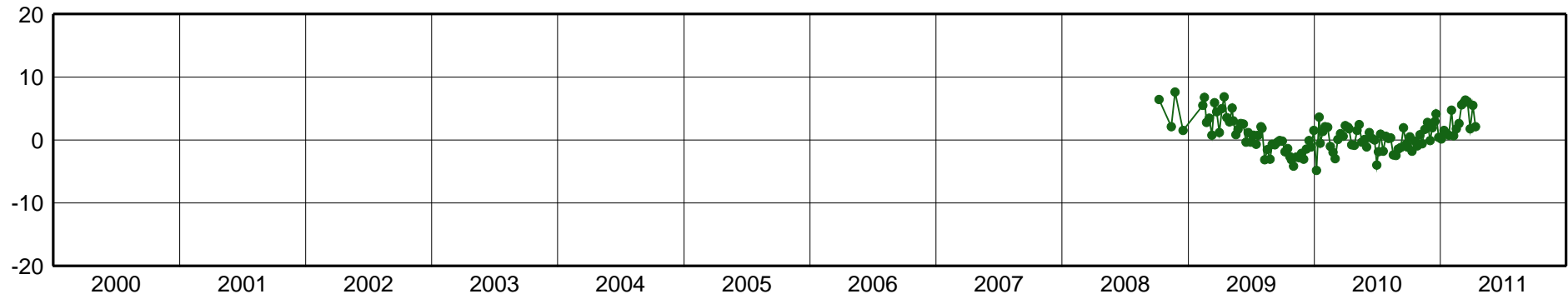
ESQU-East Component [mm]
