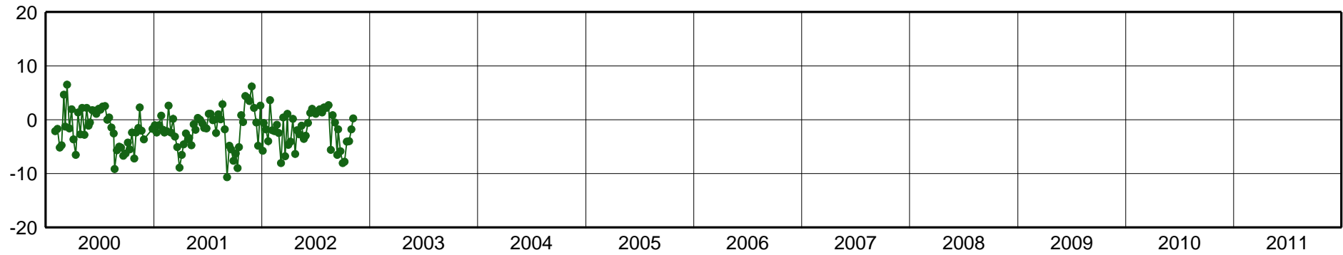
GALA-East Component [mm]
