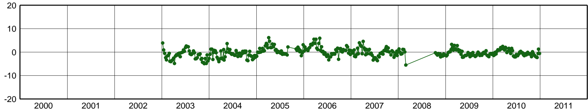
GLPS-East Component [mm]
