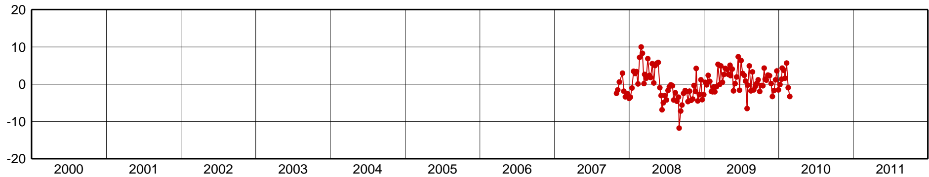
UYMO-Up Component [mm]
