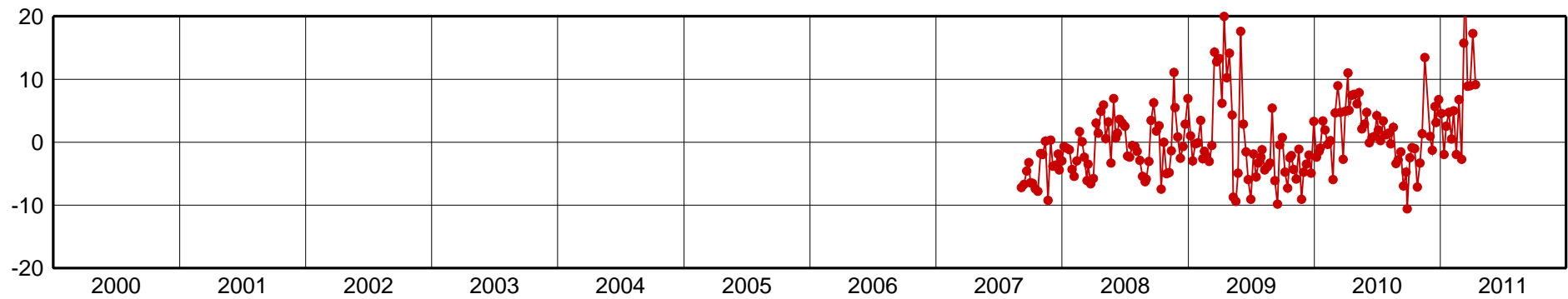
SAVO-Up Component [mm]
