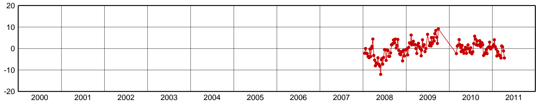
PSTO-Up Component [mm]
