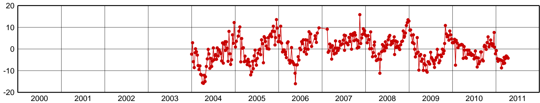
BELE-Up Component [mm]
