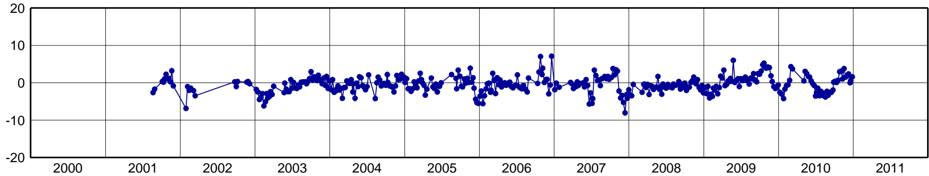
CRAT-North Component [mm]
