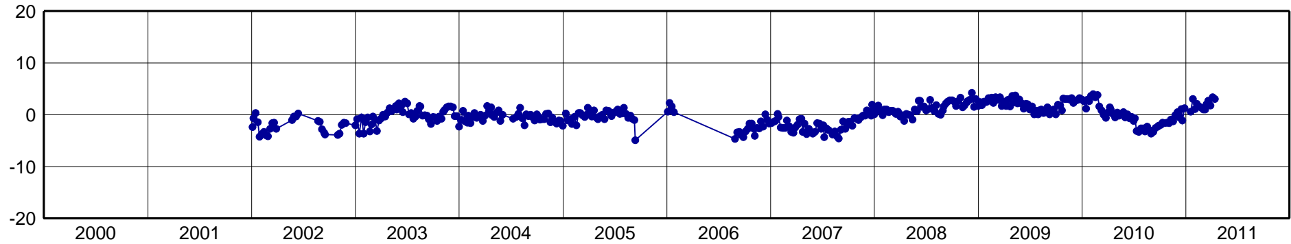
TUCU-North Component [mm]
