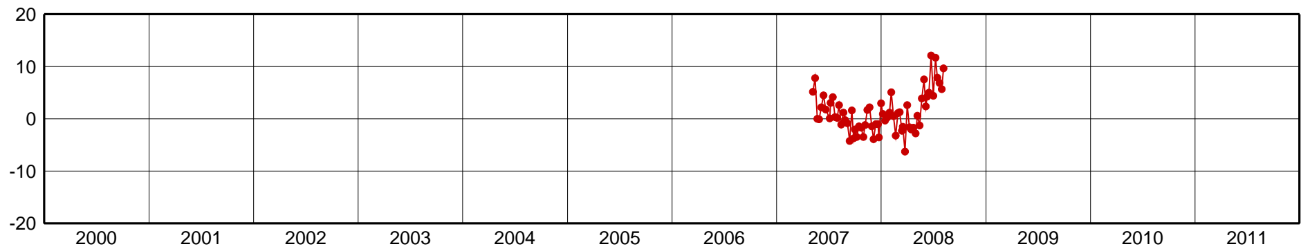
ANDS-Up Component [mm]
