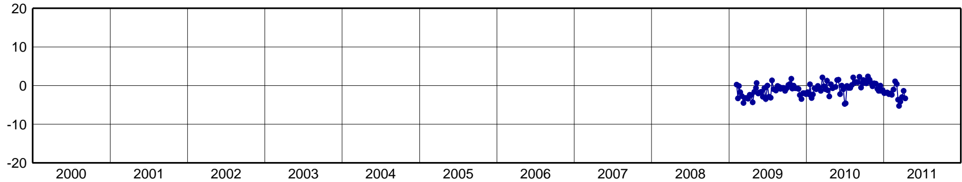
RNNA-North Component [mm]
