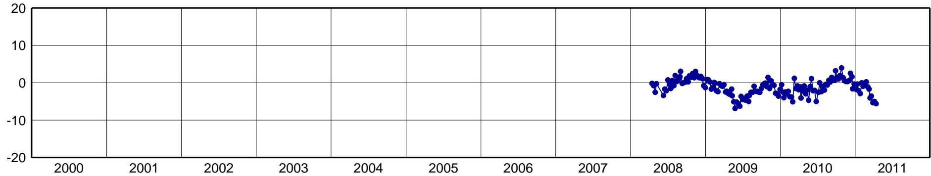
CEEU-North Component [mm]
