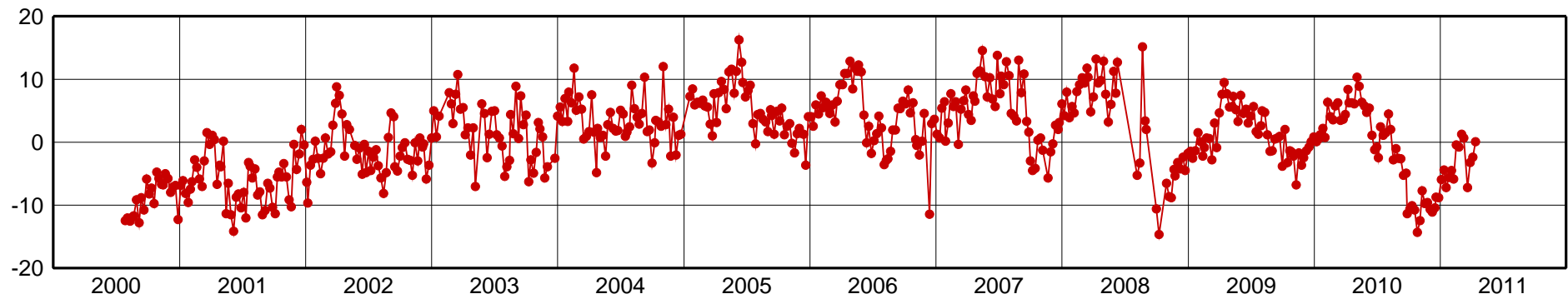
GUAT-Up Component [mm]
