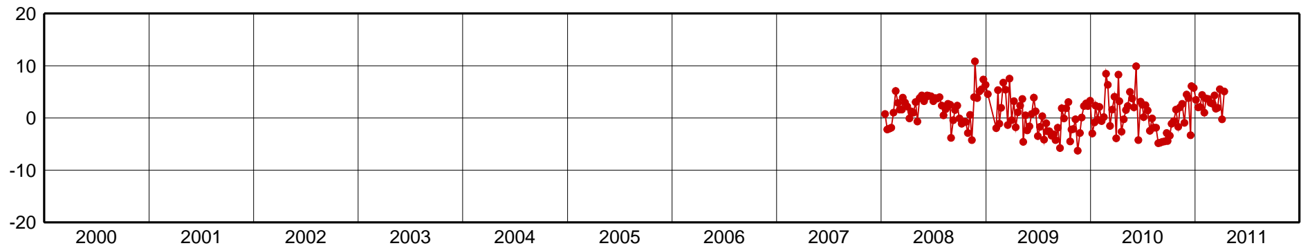
PEPE-Up Component [mm]
