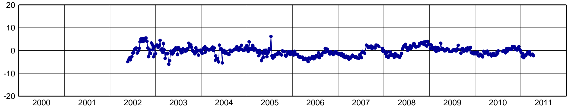
BOGT-North Component [mm]
