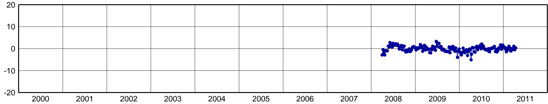
ROJI-North Component [mm]
