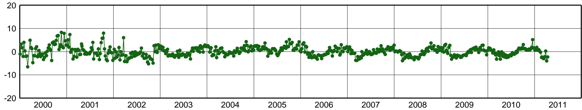
BRAZ-East Component [mm]
