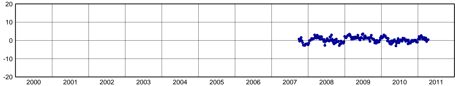
CULC-North Component [mm]
