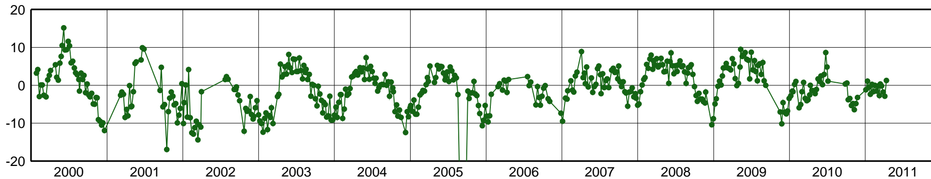
VESL-East Component [mm]
