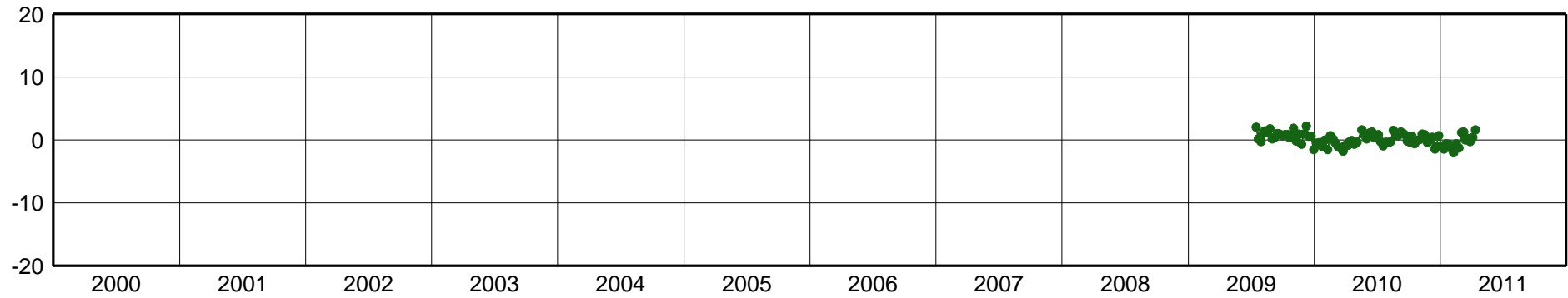
PRGU-East Component [mm]
