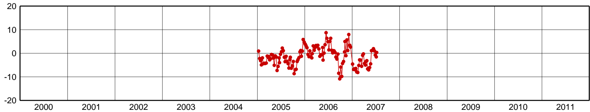
CULI-Up Component [mm]
