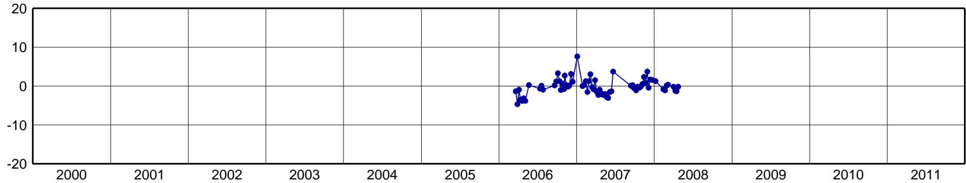
MOTE-North Component [mm]
