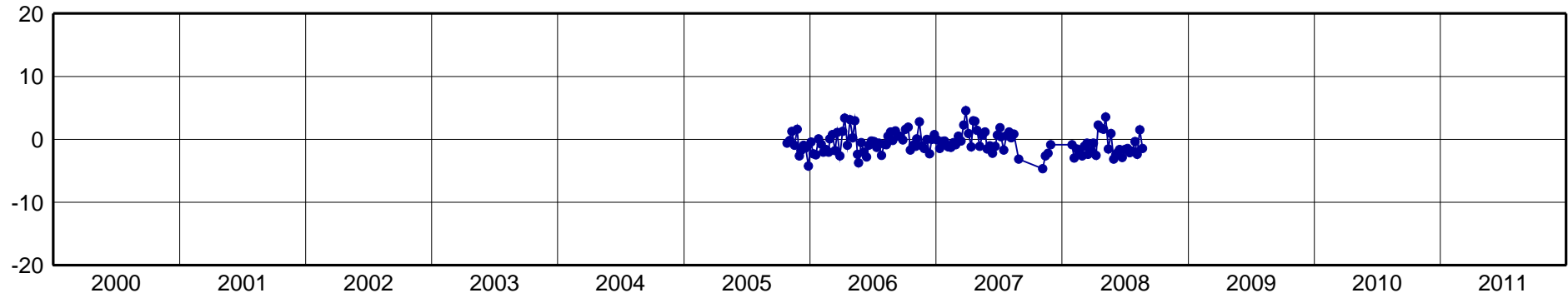
RIOH-North Component [mm]
