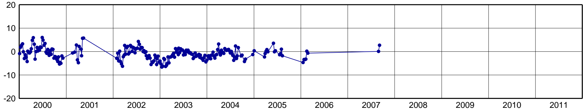
ASC1-North Component [mm]
