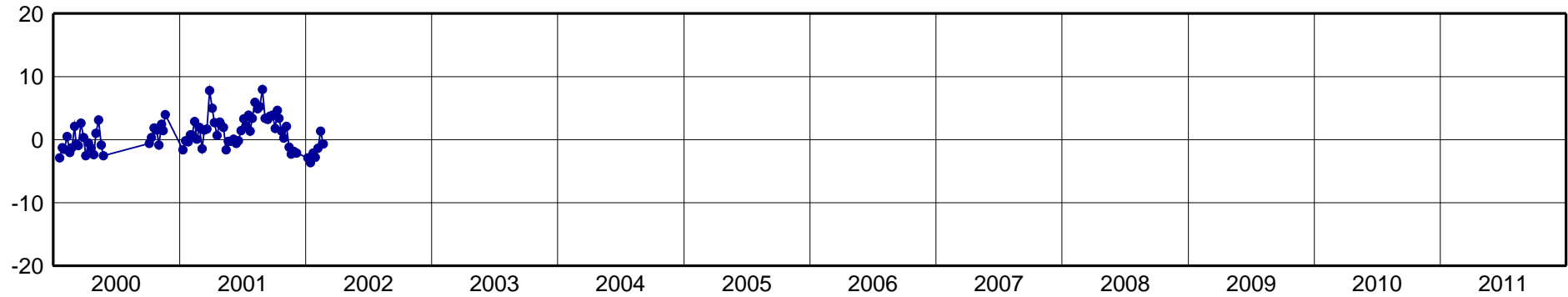
OHIG-North Component [mm]
