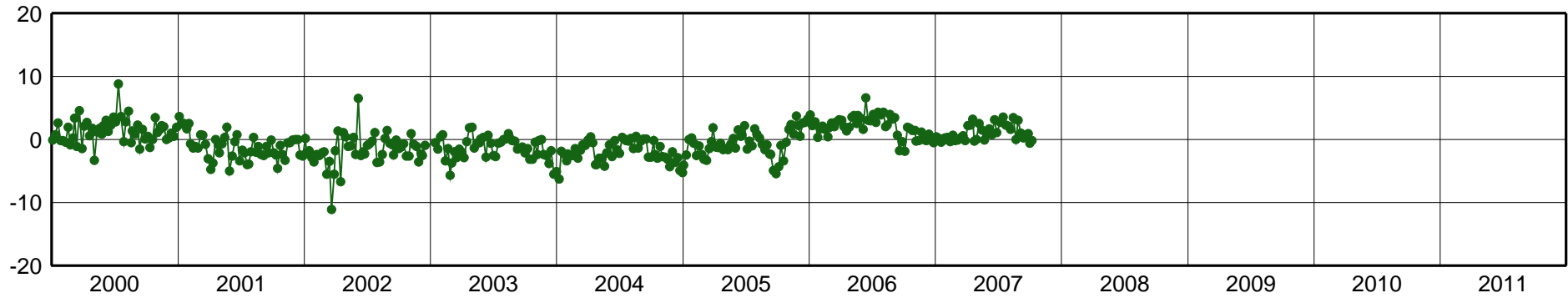
KYW1-East Component [mm]
