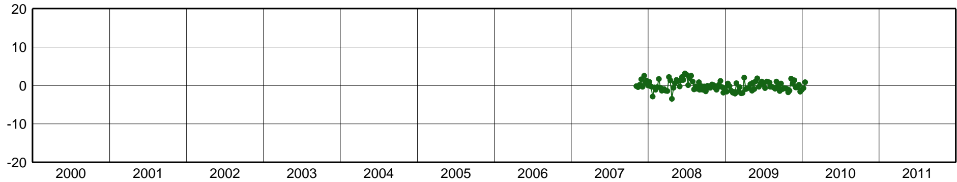
APTO-East Component [mm]
