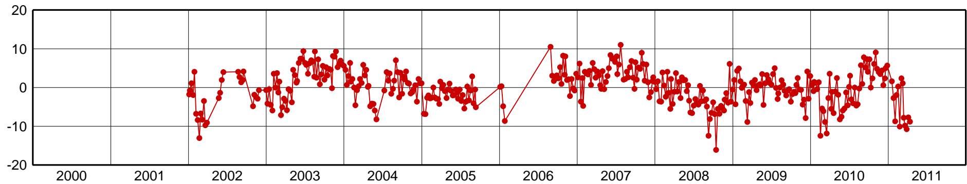
TUCU-Up Component [mm]
