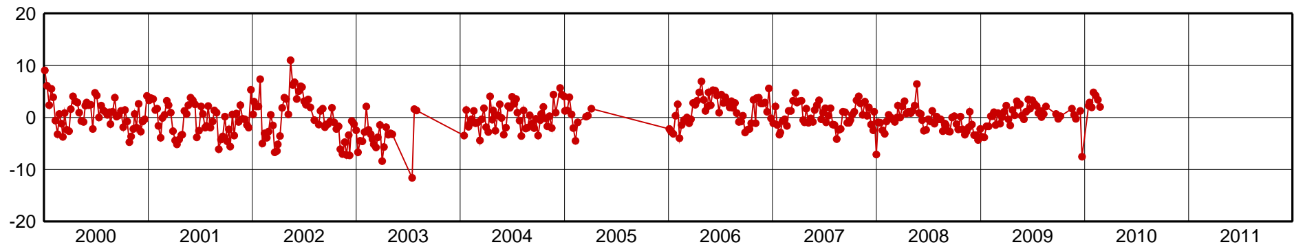
CFAG-Up Component [mm]
