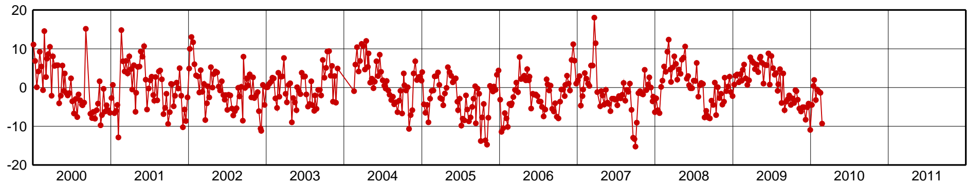
LPGS-Up Component [mm]
