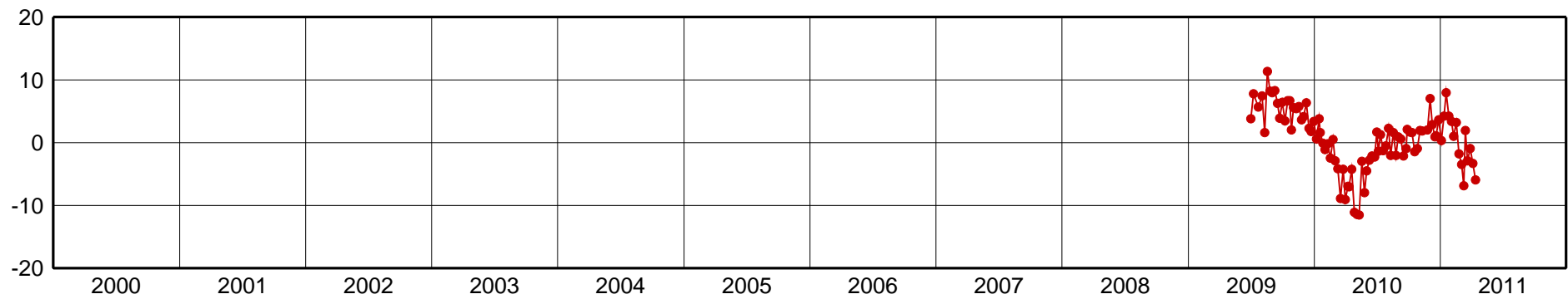
ESMR-Up Component [mm]
