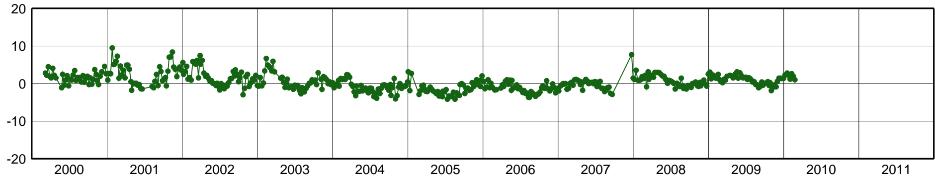
VBCA-East Component [mm]
