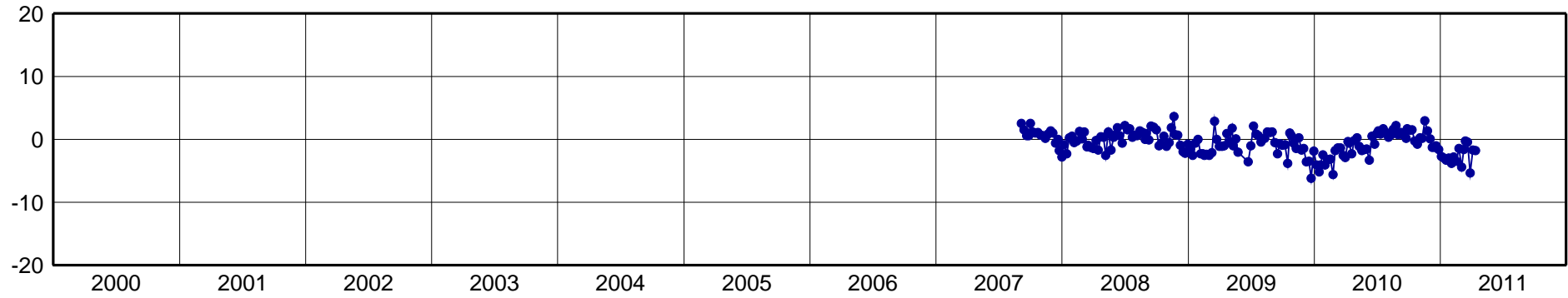
SSA1-North Component [mm]
