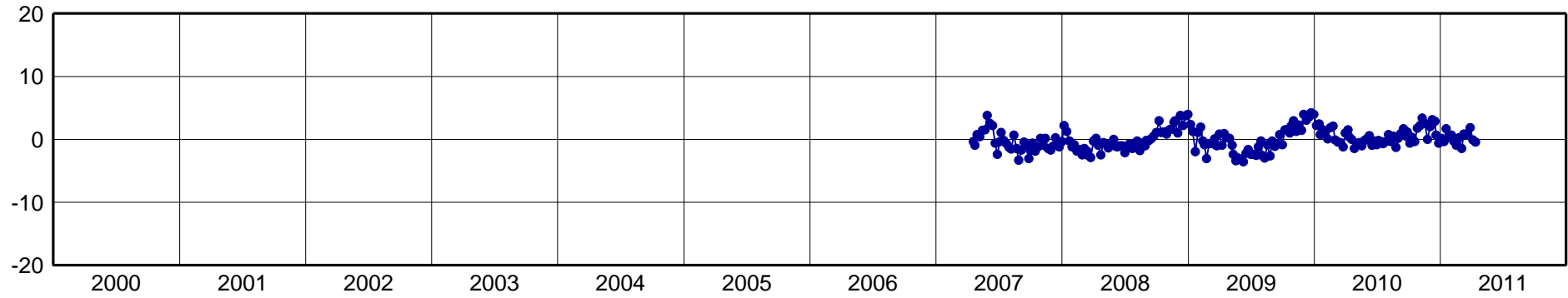
RIO2-North Component [mm]
