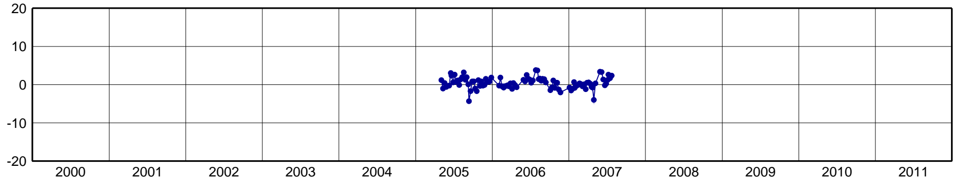
PDES-North Component [mm]
