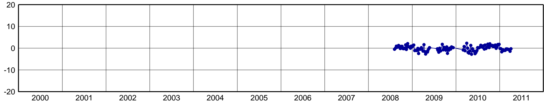
ARCA-North Component [mm]
