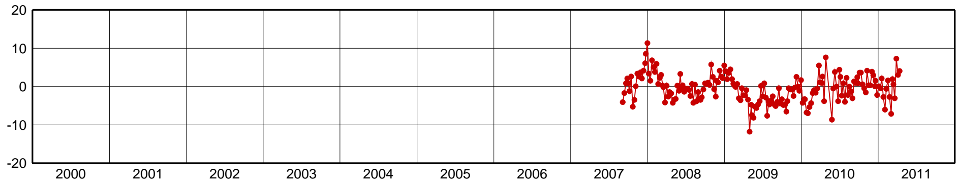
SALU-Up Component [mm]
