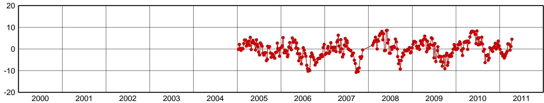
OAX2-Up Component [mm]
