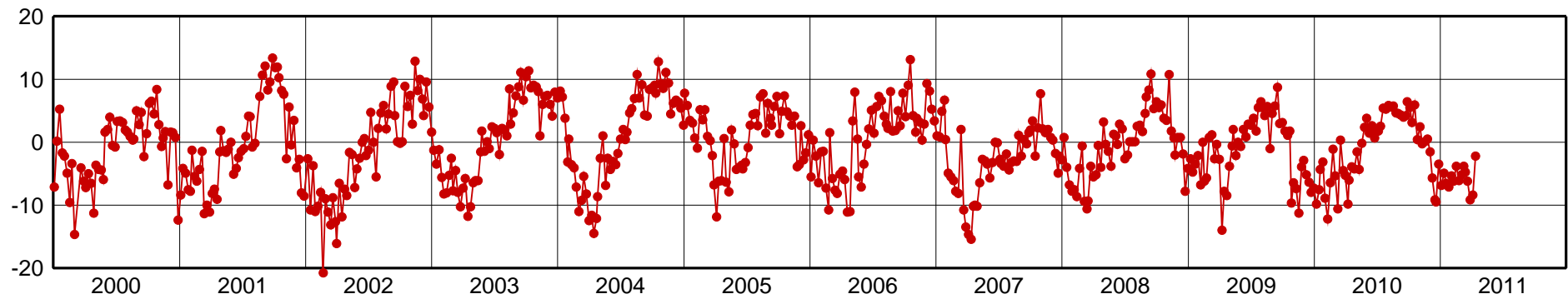
BRAZ-Up Component [mm]
