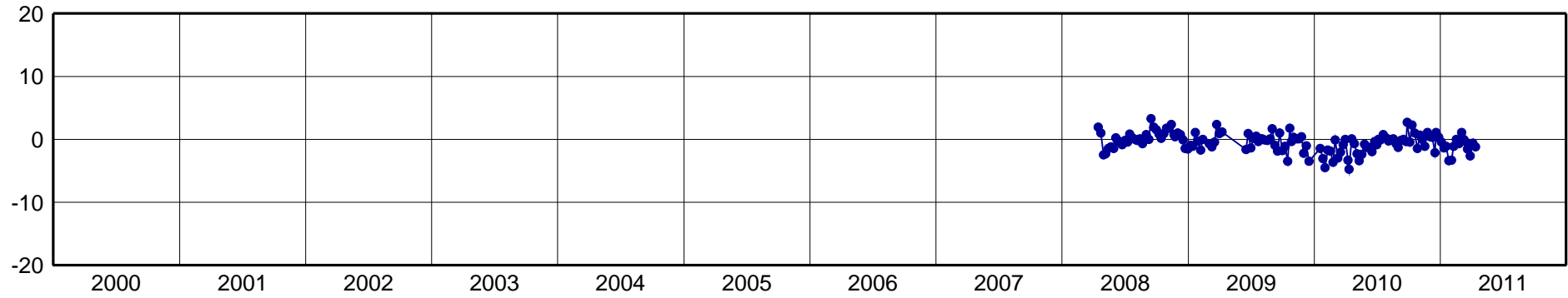
TOGU-North Component [mm]
