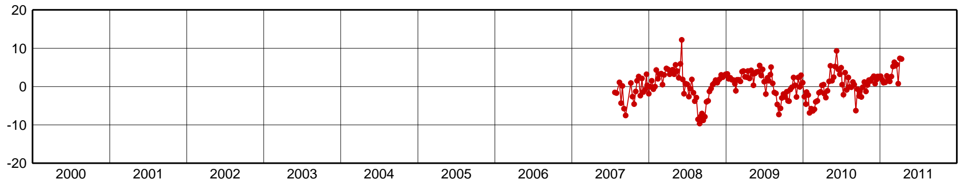
UGTO-Up Component [mm]
