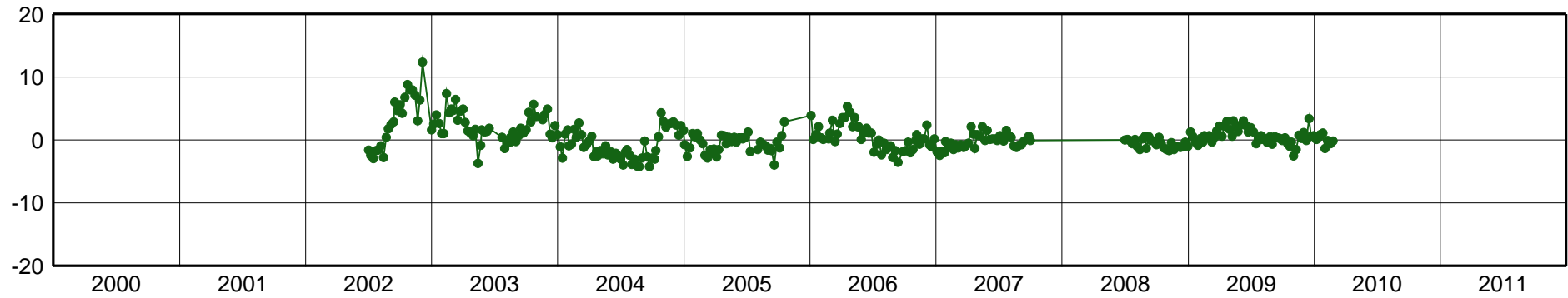
COPO-East Component [mm]
