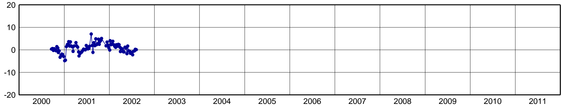
SLOR-North Component [mm]
