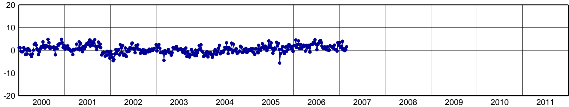
RIOG-North Component [mm]
