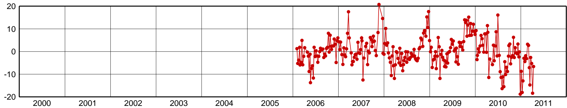
SRZN-Up Component [mm]
