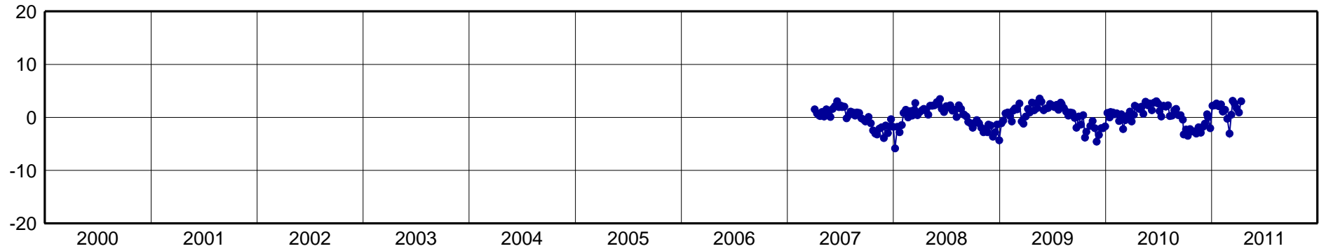
ONRJ-North Component [mm]
