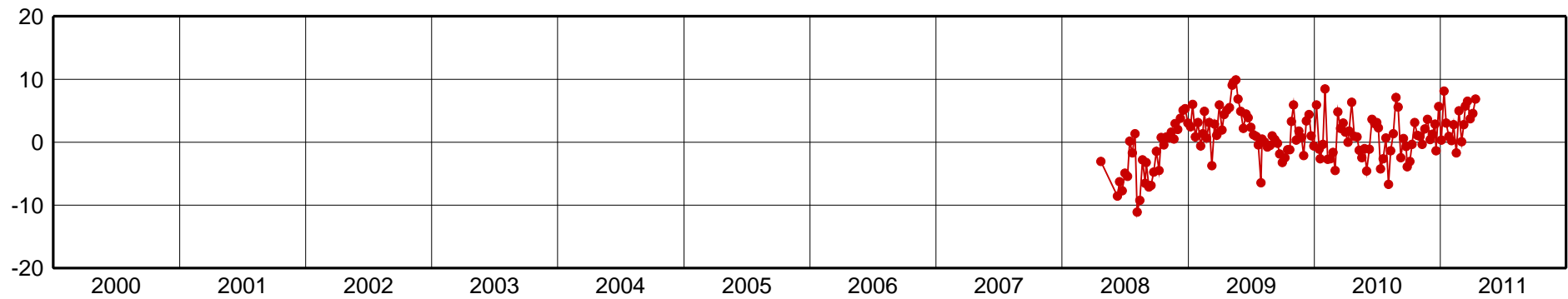
SCCH-Up Component [mm]
