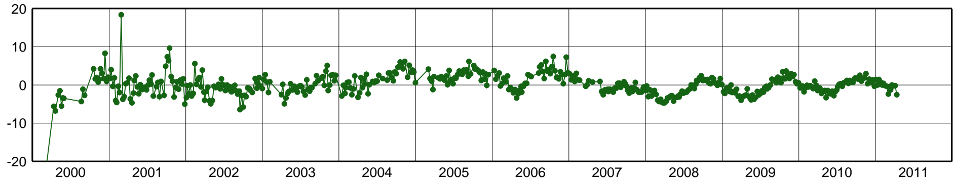
IMPZ-East Component [mm]
