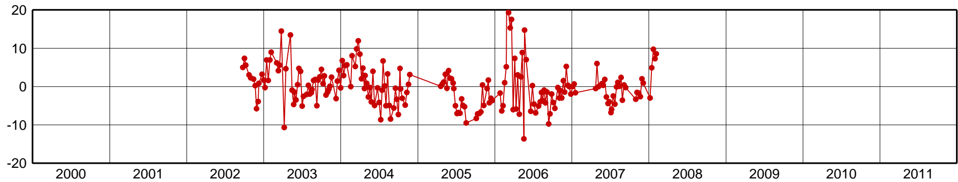
MPLA-Up Component [mm]
