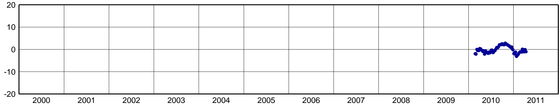
ABPW-North Component [mm]
