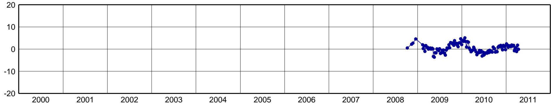
ESQU-North Component [mm]
