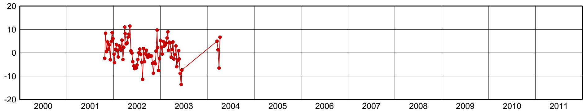
TEG1-Up Component [mm]
