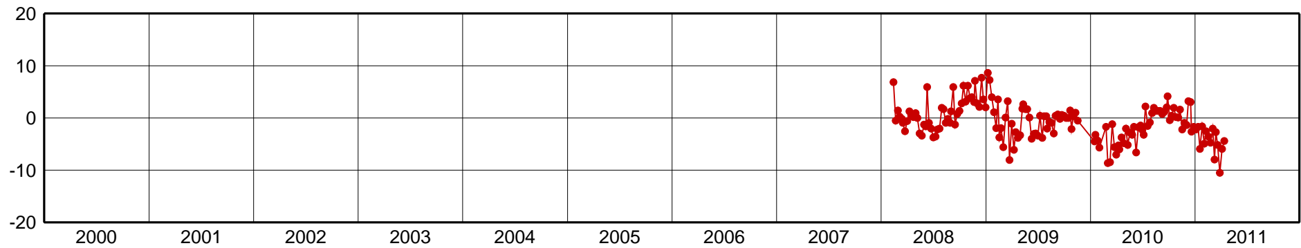
MGIN-Up Component [mm]
