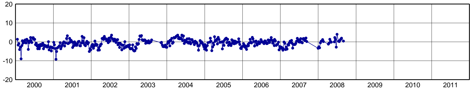
SALV-North Component [mm]
