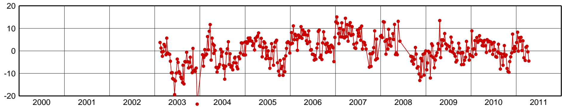
ETCG-Up Component [mm]
