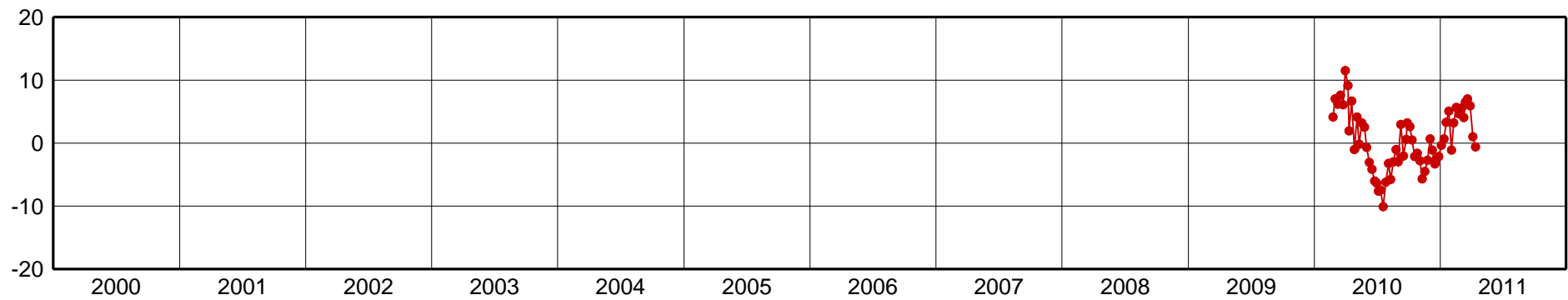
ABPW-Up Component [mm]
