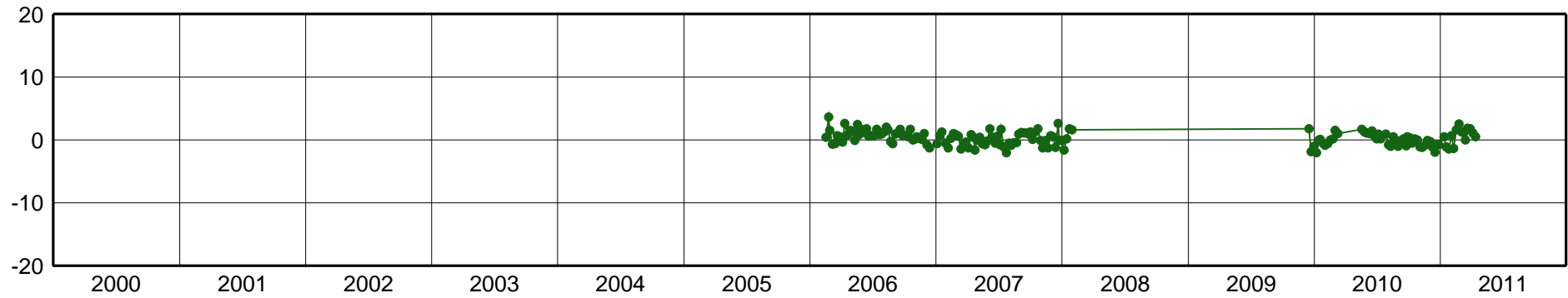
DORA-East Component [mm]
