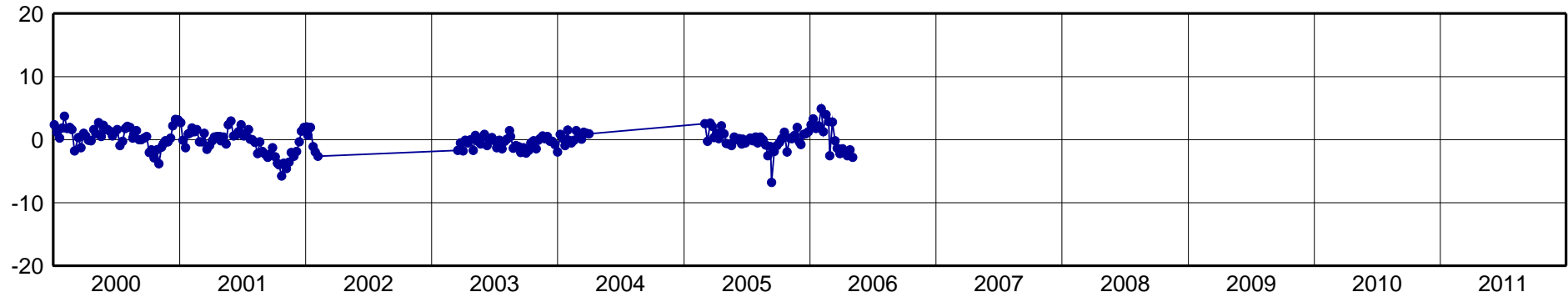
CORD-North Component [mm]
