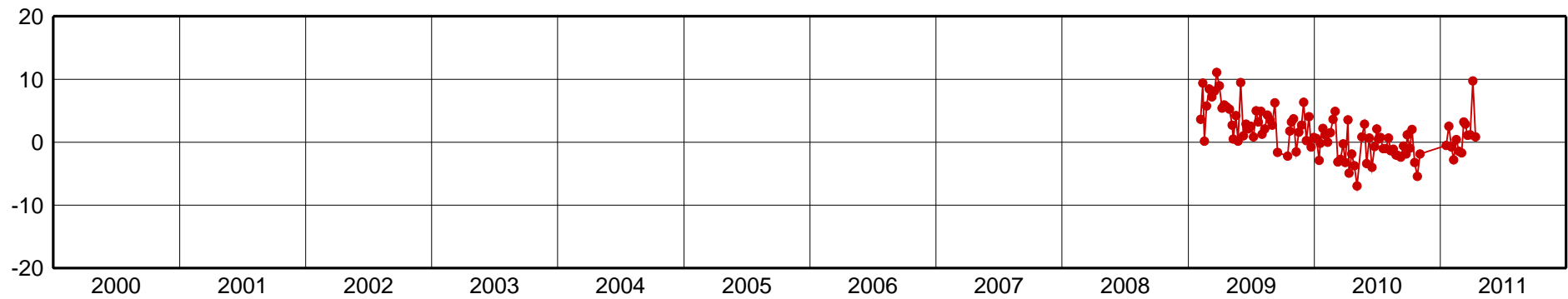
BAIR-Up Component [mm]
