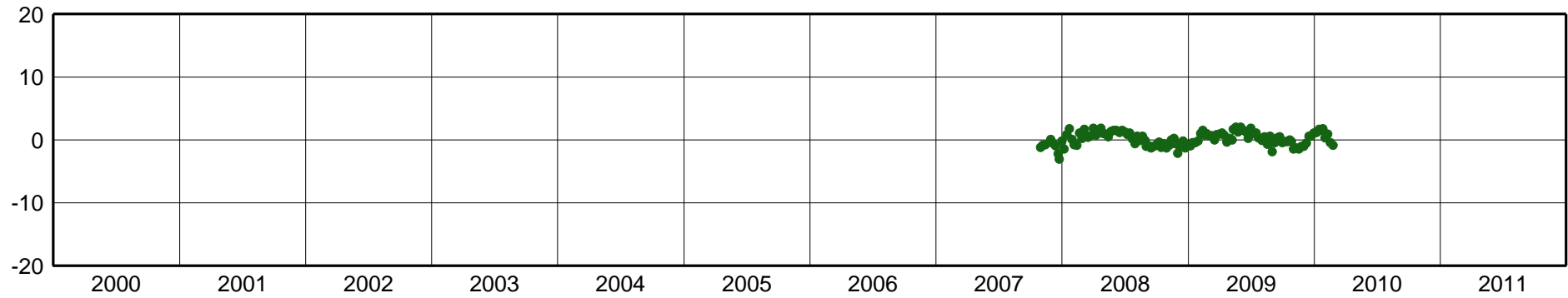
UYMO-East Component [mm]
