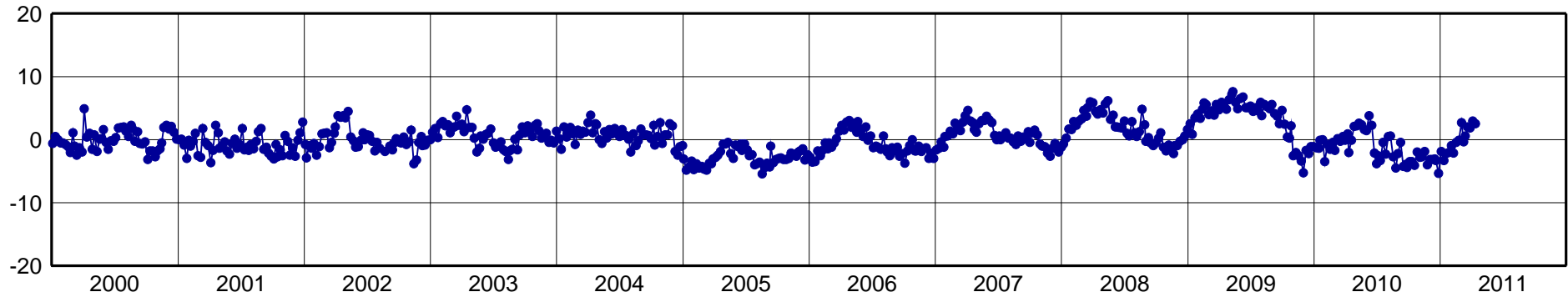
MDO1-North Component [mm]
