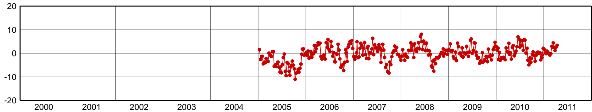
COL2-Up Component [mm]
