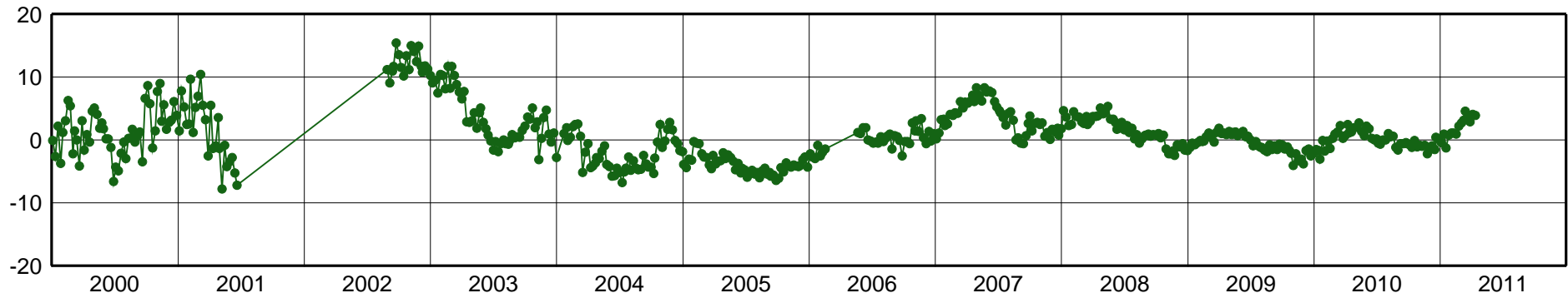
AREQ-East Component [mm]
