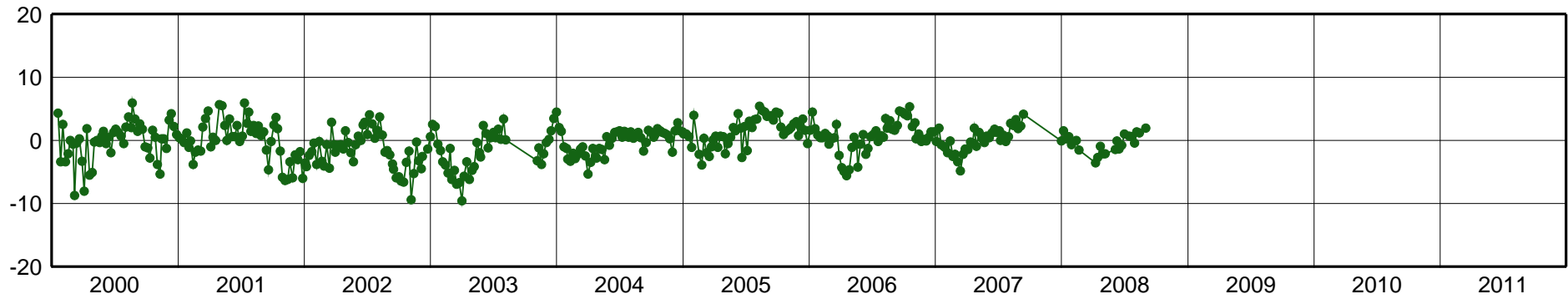
SALV-East Component [mm]
