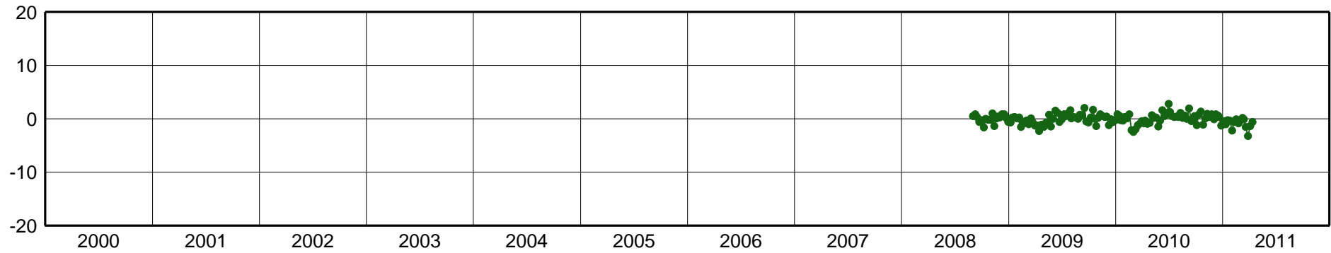
USLP-East Component [mm]
