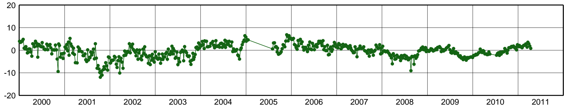
CRO1-East Component [mm]
