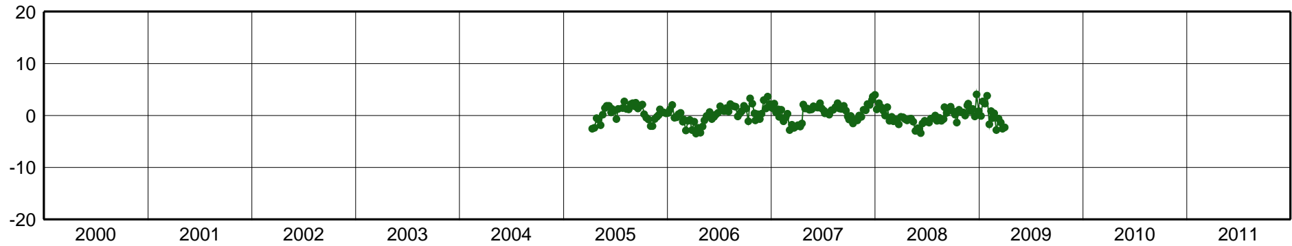
VARG-East Component [mm]
