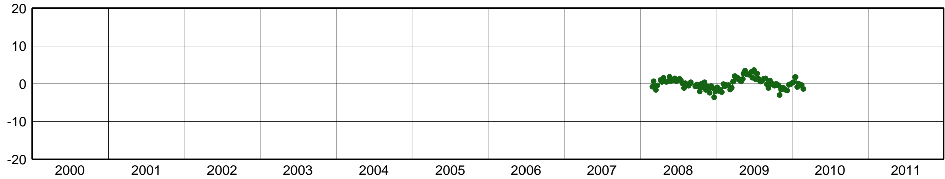
UYRO-East Component [mm]
