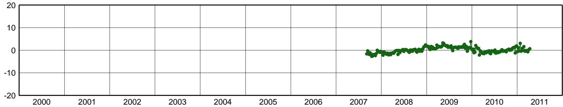
UFPR-East Component [mm]
