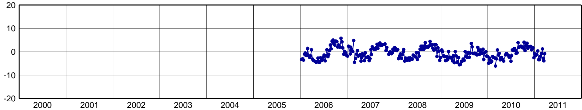
MAPA-North Component [mm]
