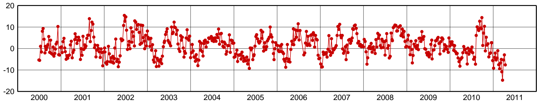
GOLD-Up Component [mm]
