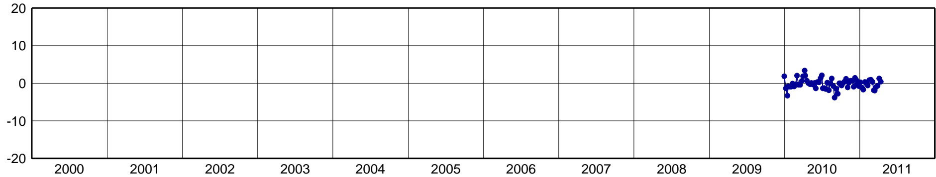
SCRZ-North Component [mm]
