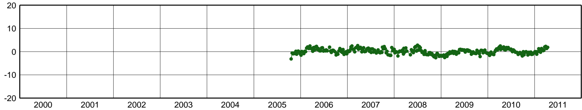
TUNA-East Component [mm]
