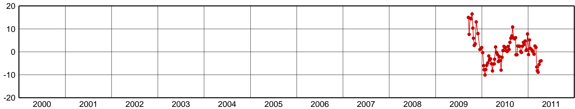
ROSA-Up Component [mm]
