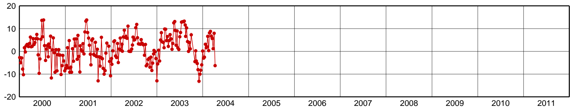
AOML-Up Component [mm]
