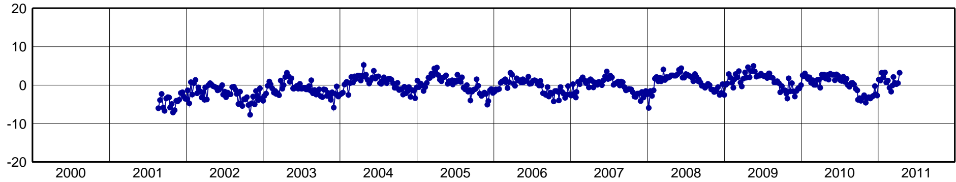
RIOD-North Component [mm]
