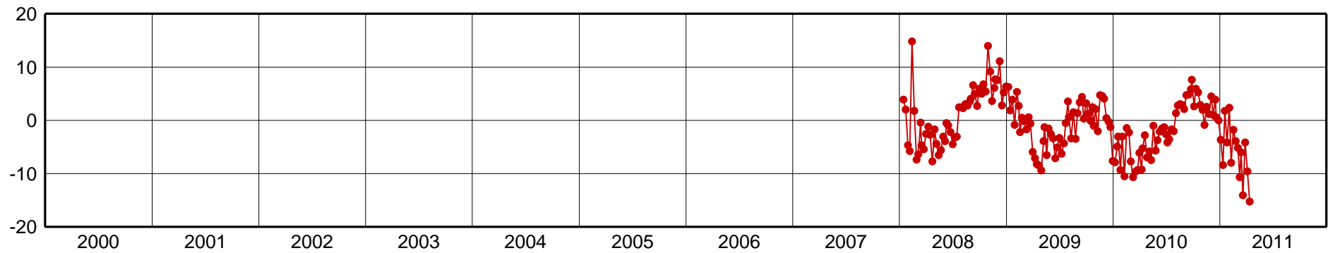
MGUB-Up Component [mm]
