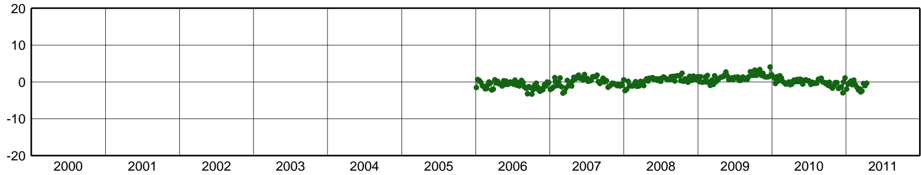
PPTE-East Component [mm]
