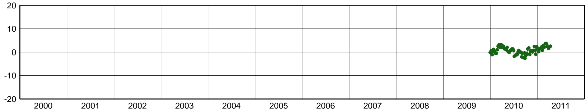
SCRZ-East Component [mm]
