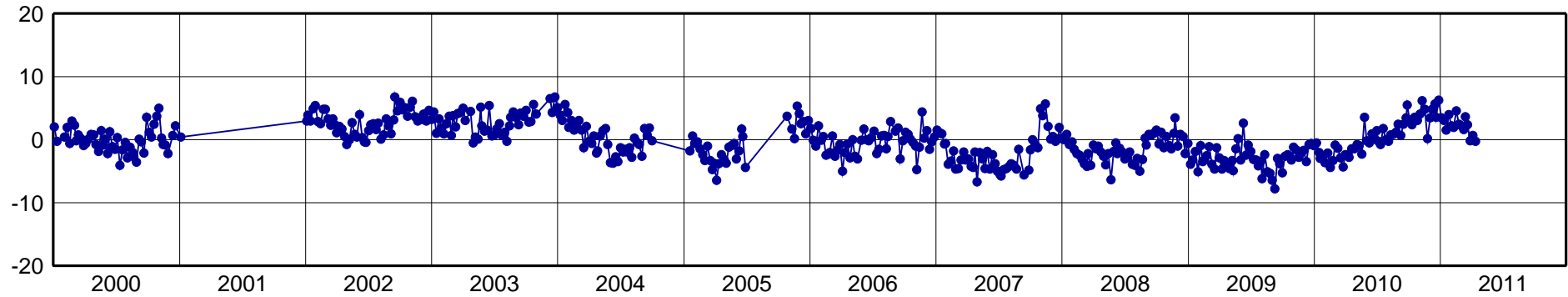
SCUB-North Component [mm]
