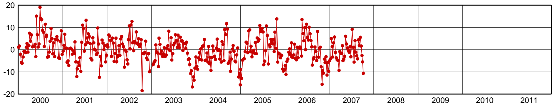
KYW1-Up Component [mm]
