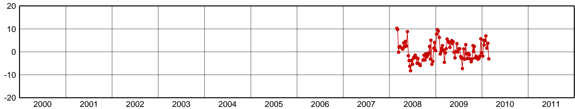
UYRO-Up Component [mm]
