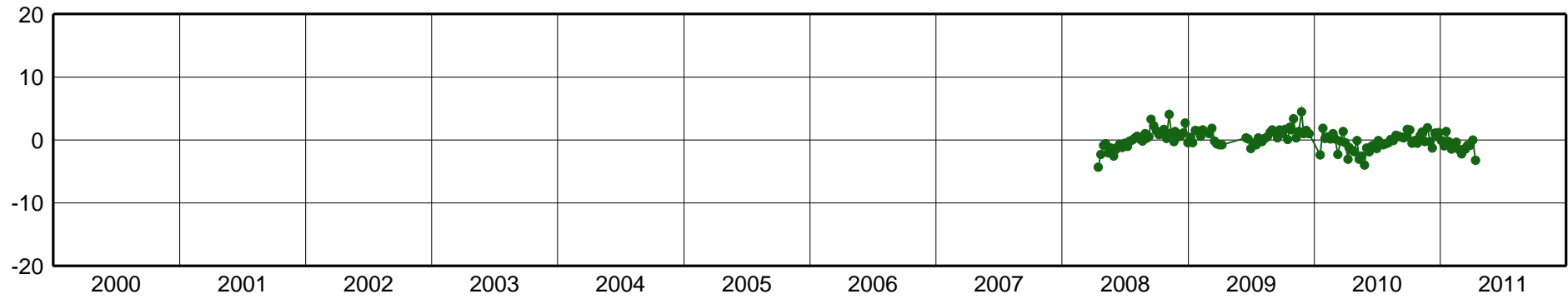
TOGU-East Component [mm]
