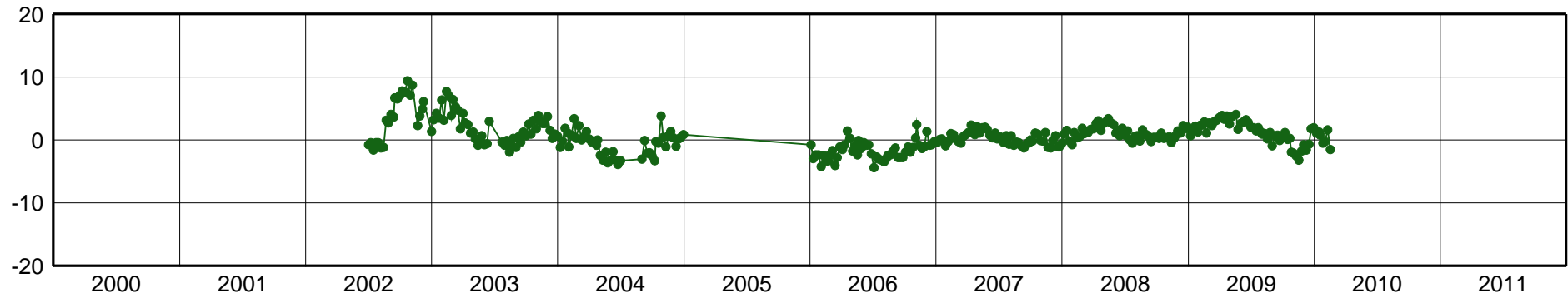
ANTC-East Component [mm]
