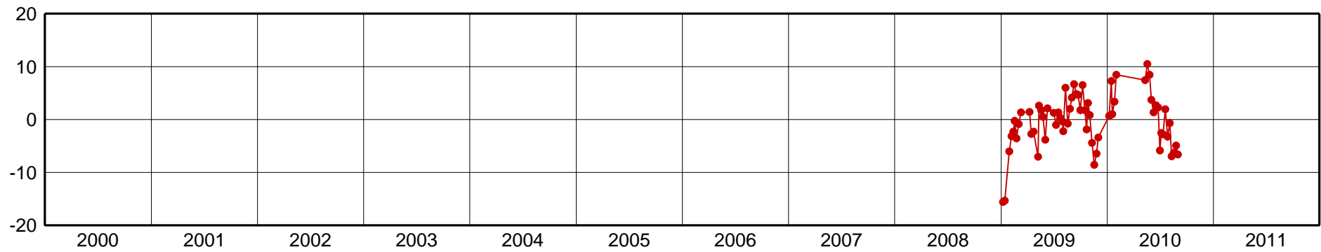
MAGA-Up Component [mm]
