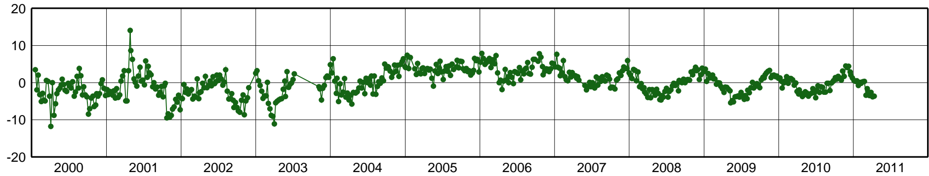
RECF-East Component [mm]
