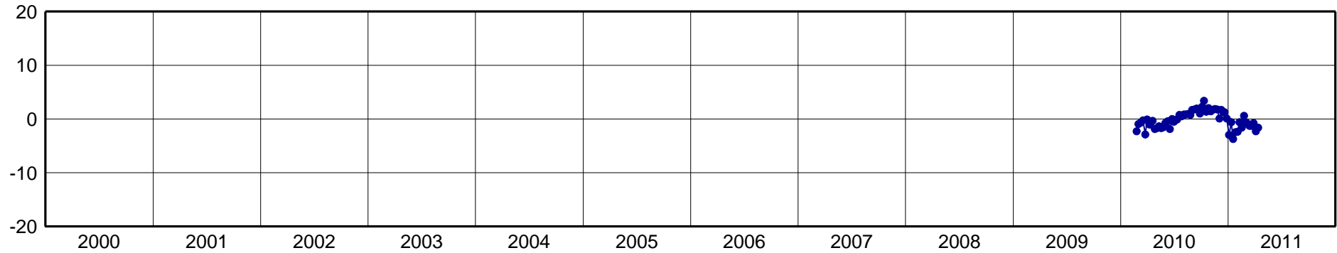
ABPD-North Component [mm]
