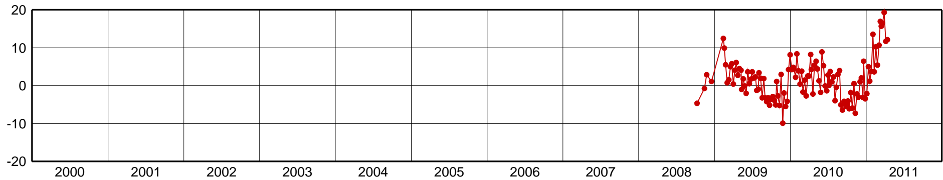
ESQU-Up Component [mm]
