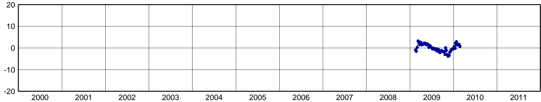
TERO-North Component [mm]
