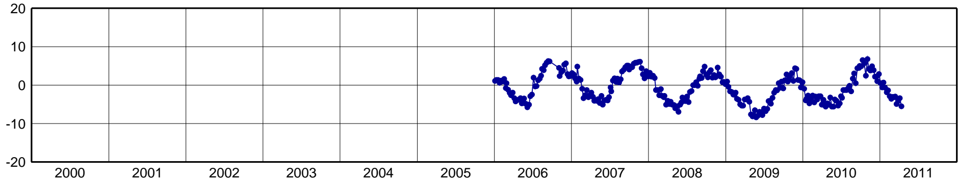
NAUS-North Component [mm]
