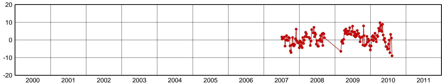
GTK0-Up Component [mm]
