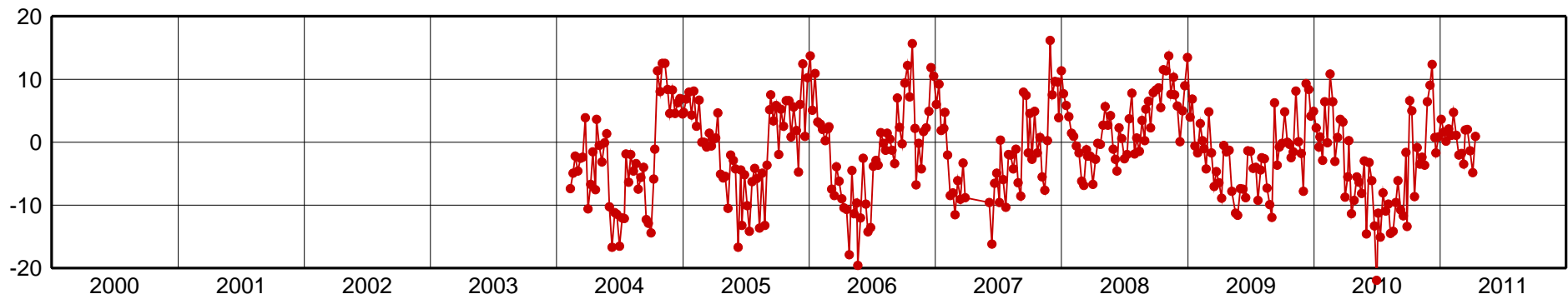
ISPA-Up Component [mm]
