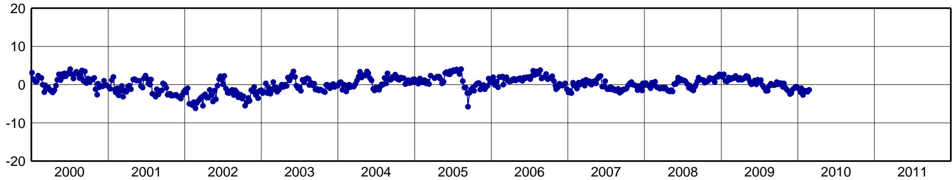
SANT-North Component [mm]
