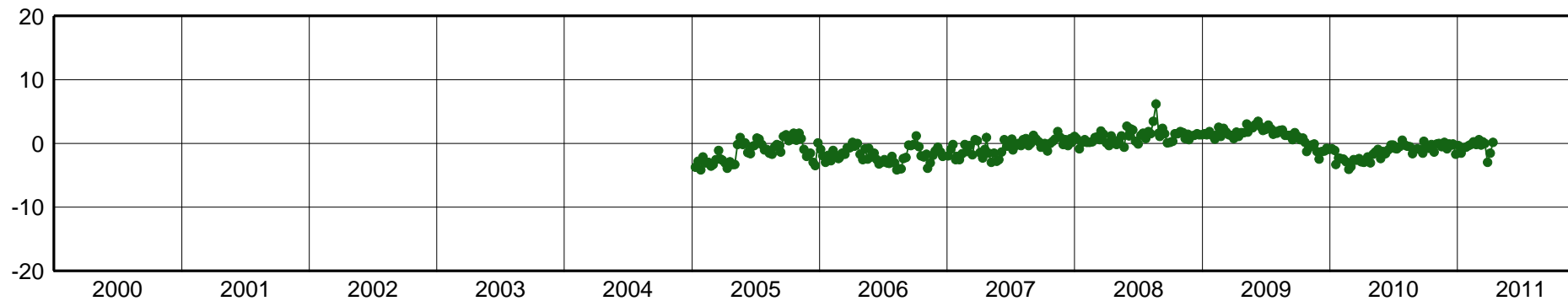
TOL2-East Component [mm]
