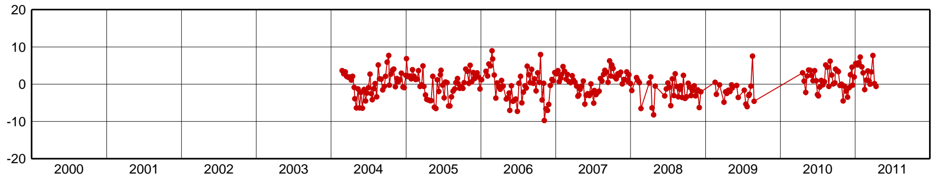
CALI-Up Component [mm]
