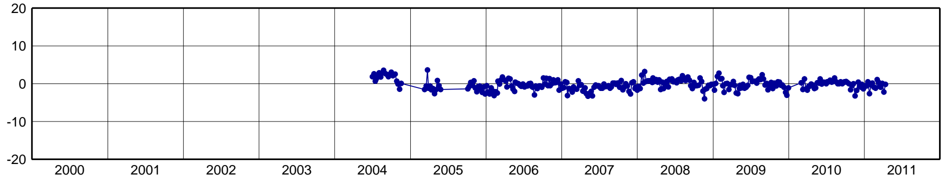
MCLA-North Component [mm]
