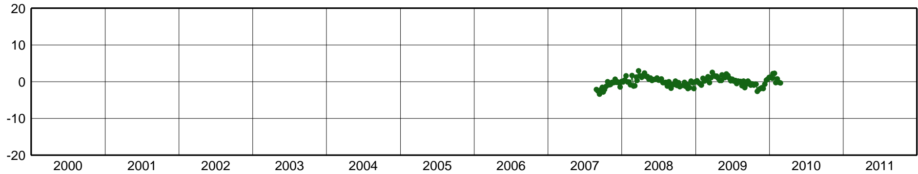
AZUL-East Component [mm]
