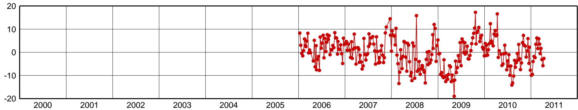
SRNW-Up Component [mm]
