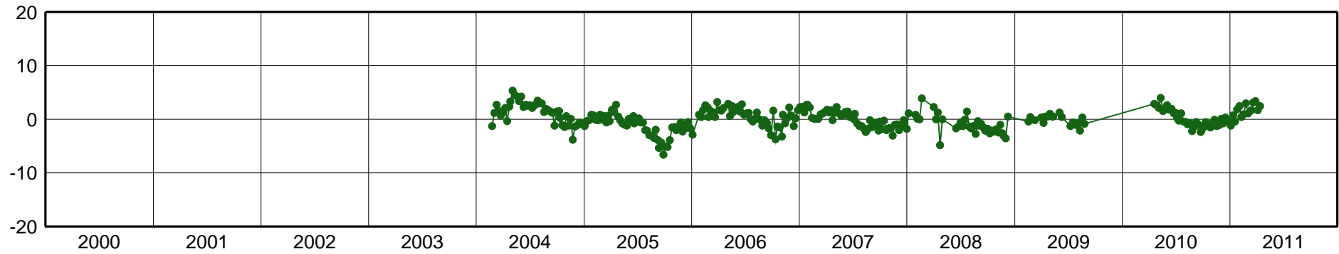
CALI-East Component [mm]
