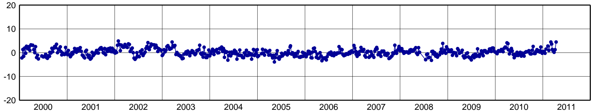
MARA-North Component [mm]
