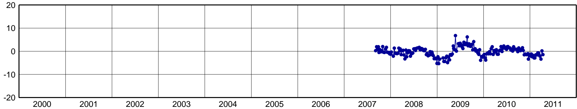
MABA-North Component [mm]
