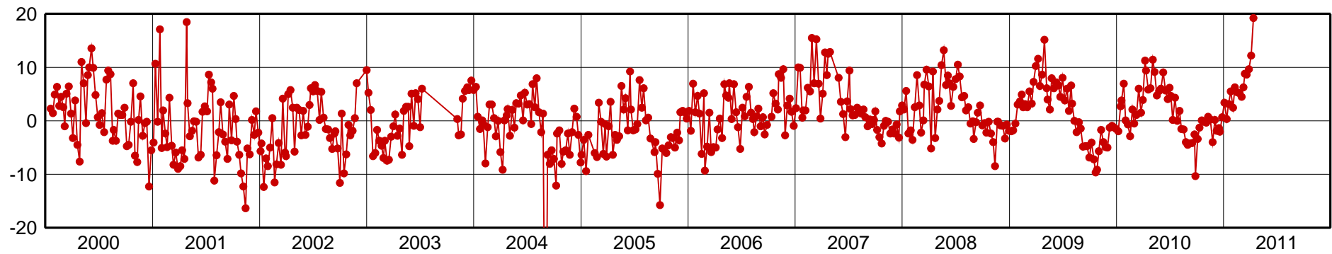
RECF-Up Component [mm]
