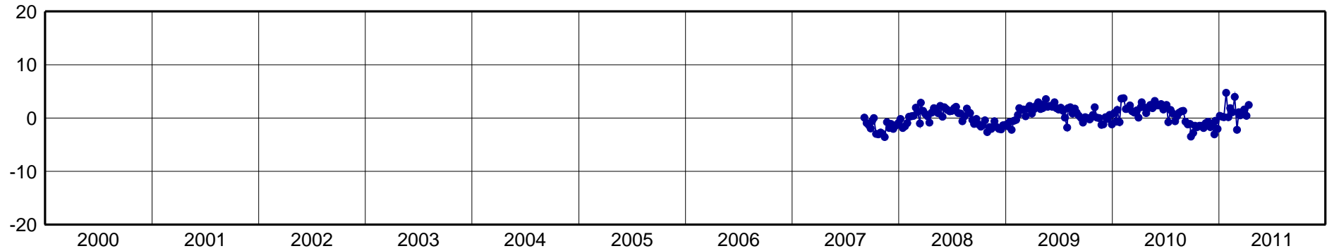
UFPR-North Component [mm]
