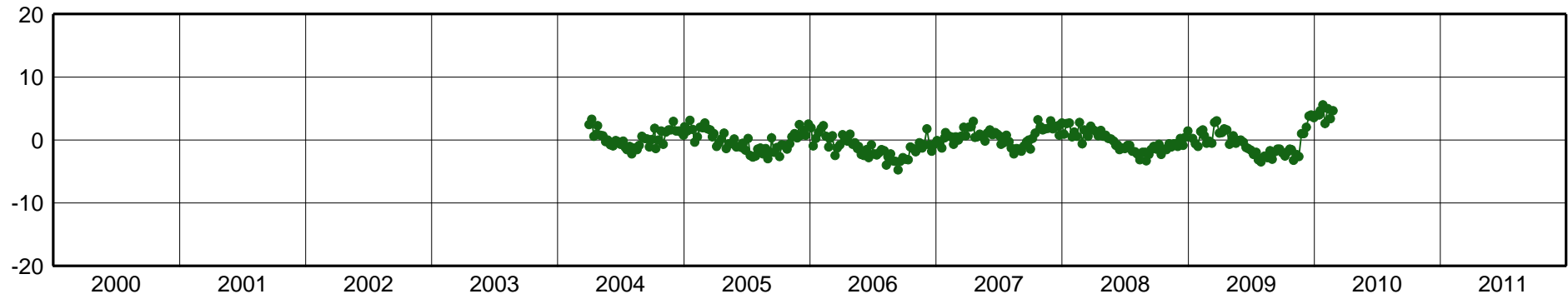
UNRO-East Component [mm]
