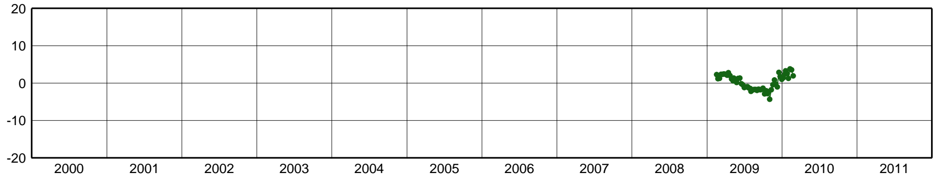
ALUM-East Component [mm]
