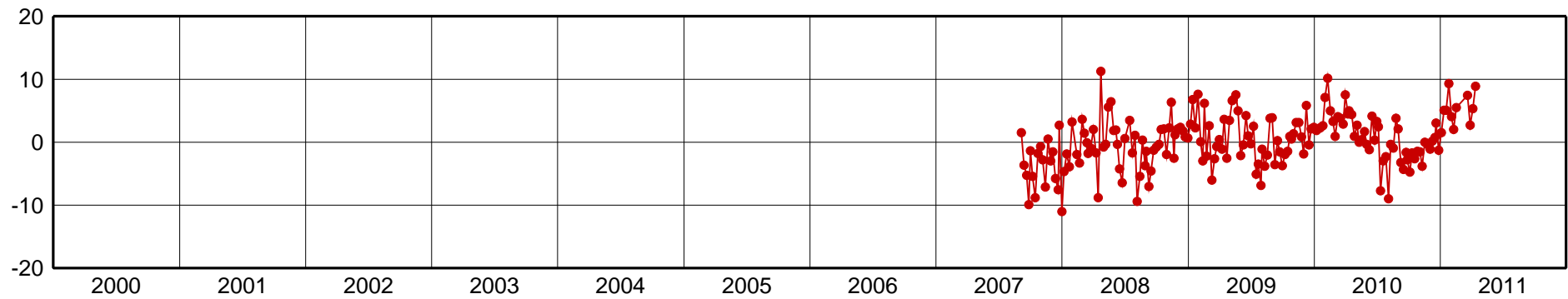
IMBT-Up Component [mm]
