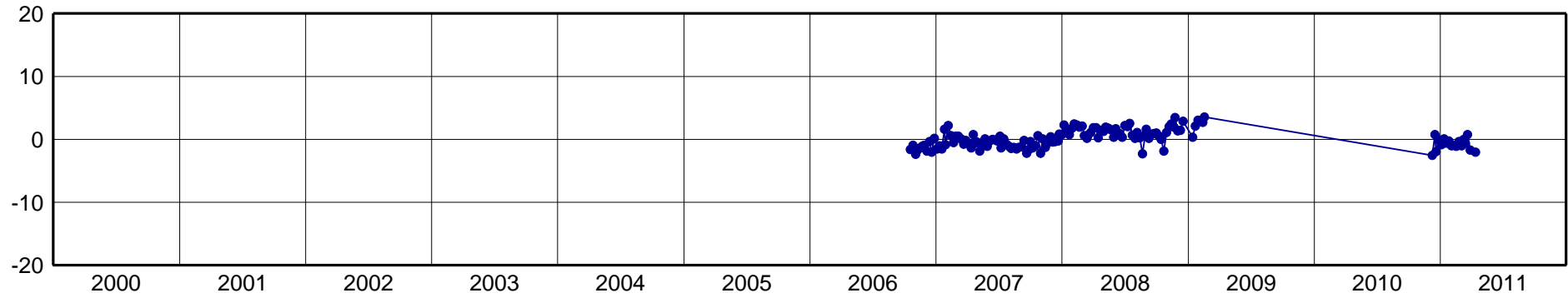
MECO-North Component [mm]
