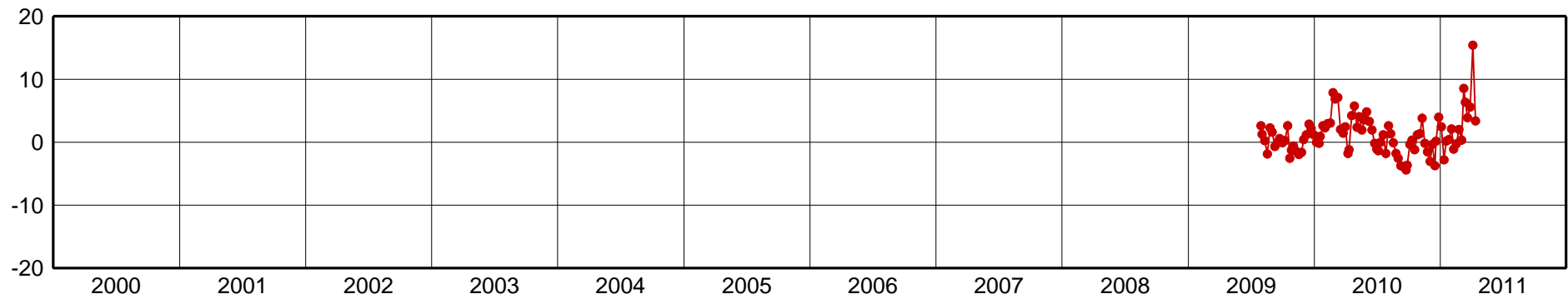
BAVC-Up Component [mm]
