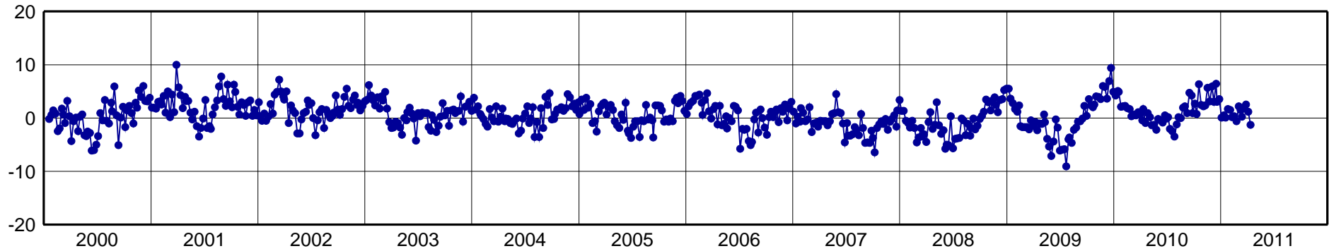
PALM-North Component [mm]
