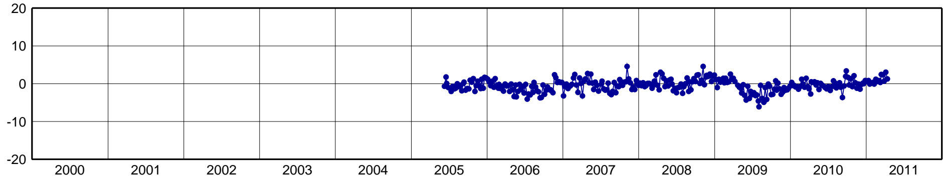
GCGT-North Component [mm]
