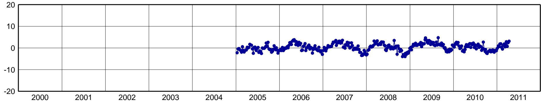
LPAZ-North Component [mm]
