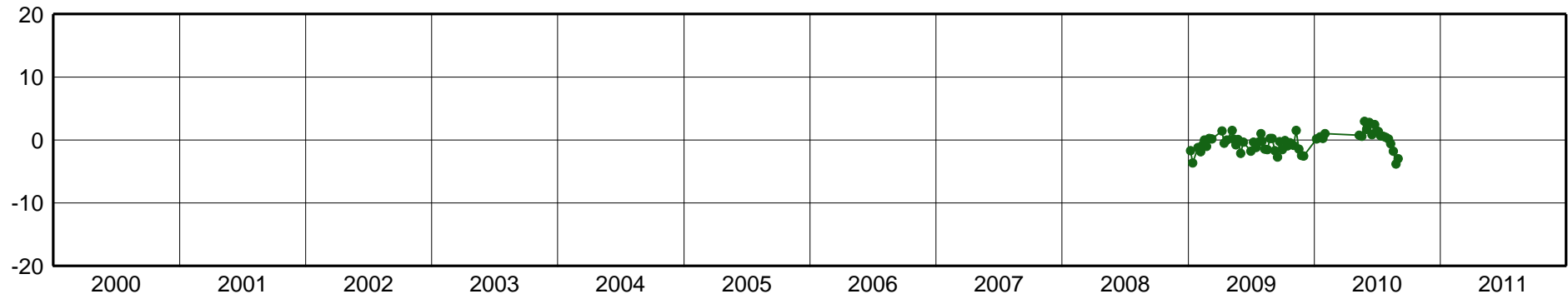
MAGA-East Component [mm]
