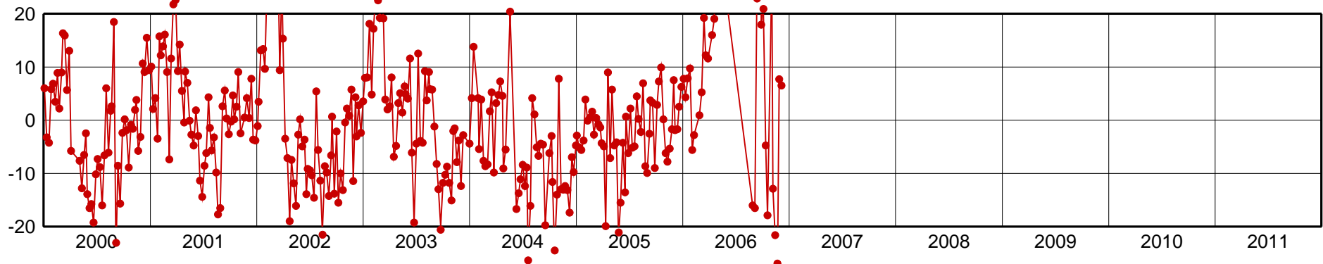
Goug-Up Component [mm]
