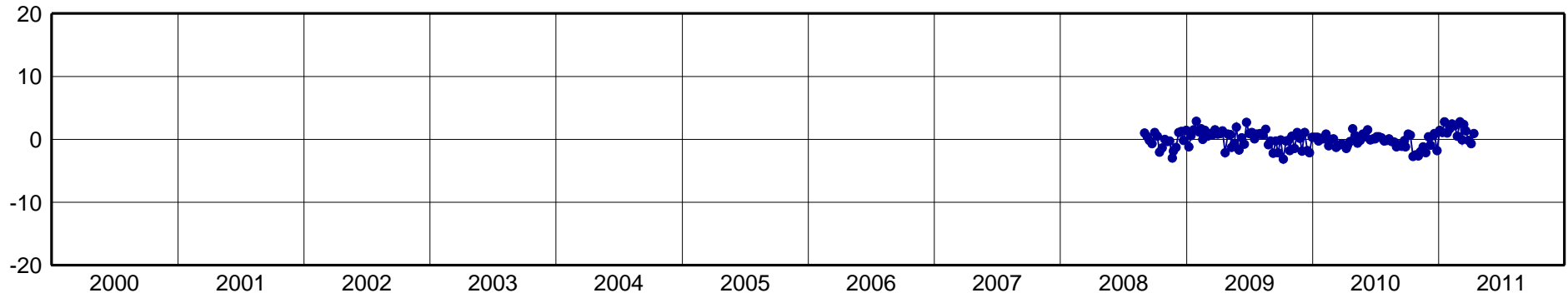
MTBA-North Component [mm]
