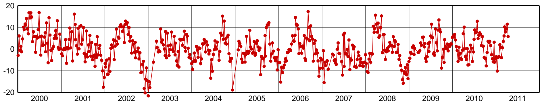
BRMU-Up Component [mm]
