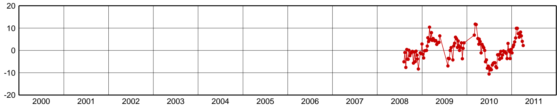
ARCA-Up Component [mm]
