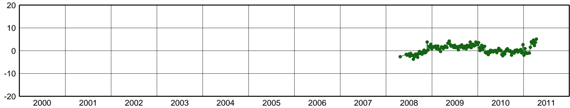
SCCH-East Component [mm]
