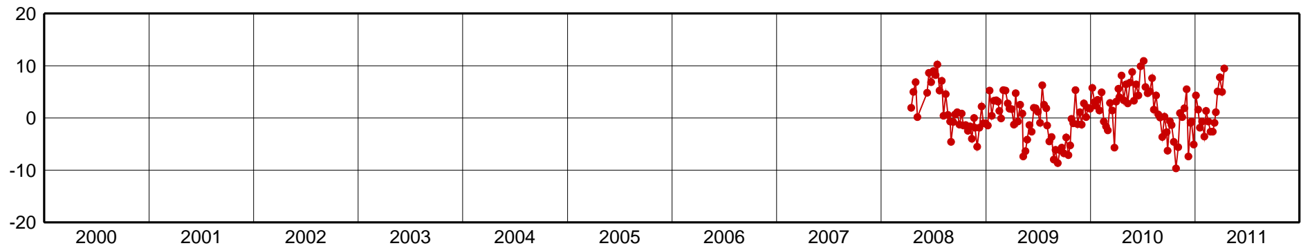
CEEU-Up Component [mm]
