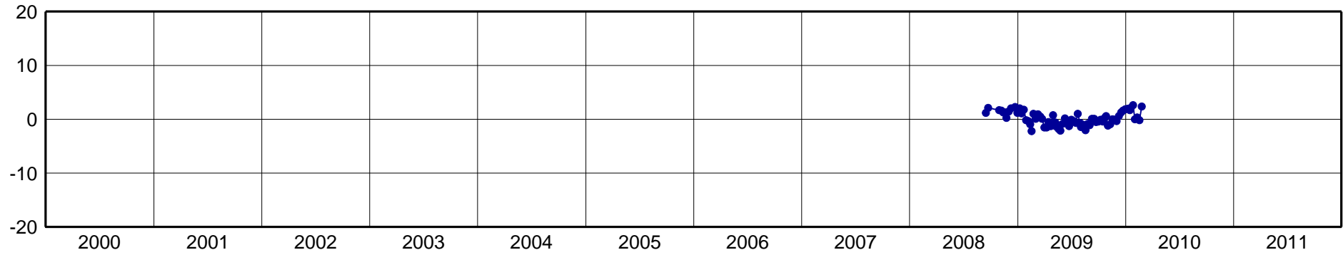
SRLP-North Component [mm]
