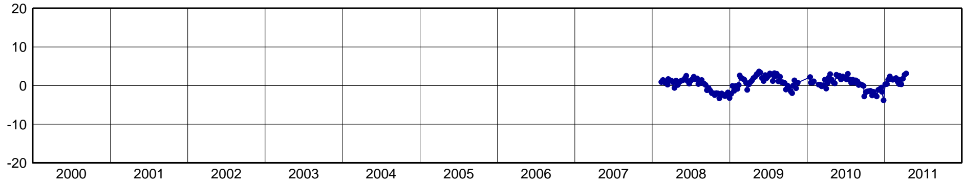
MGIN-North Component [mm]
