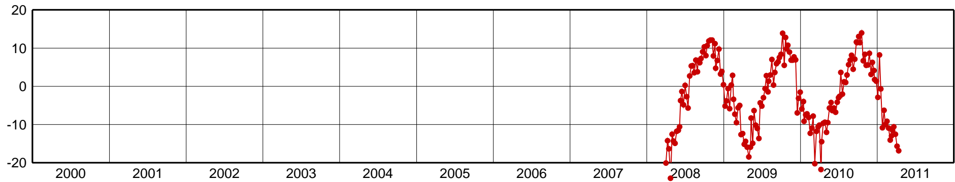
ROJI-Up Component [mm]
