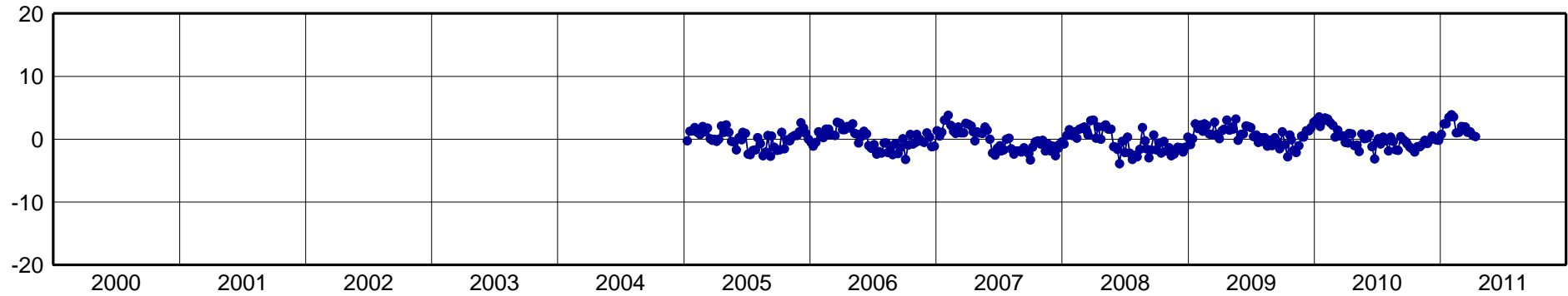
MTY2-North Component [mm]
