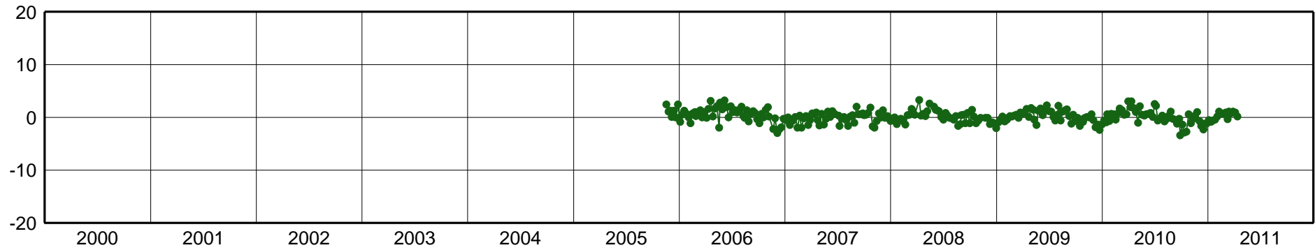
CBSB-East Component [mm]
