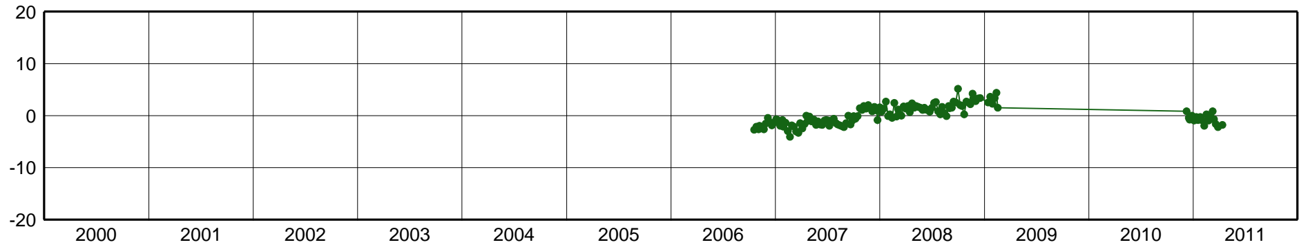
MECO-East Component [mm]
