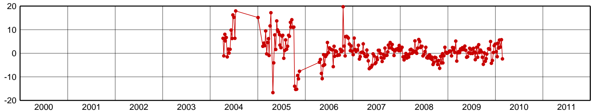
UCOR-Up Component [mm]
