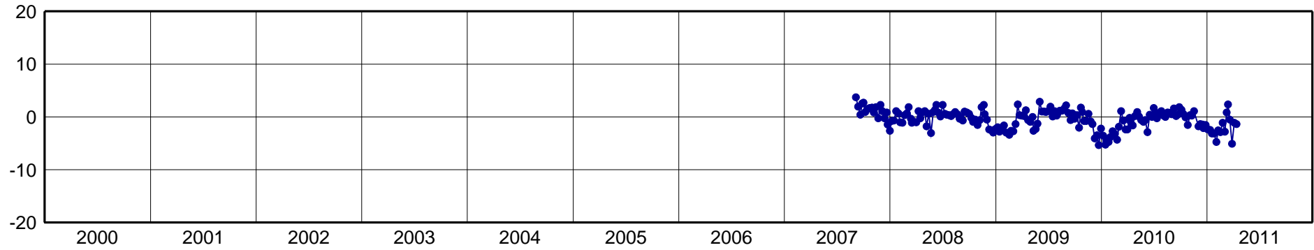
SAVO-North Component [mm]
