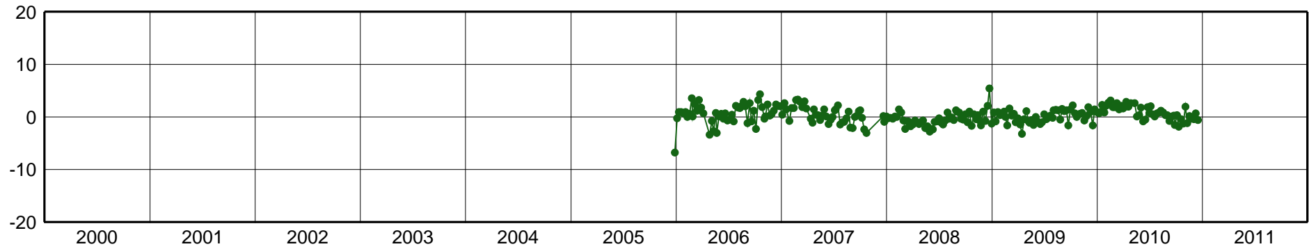
PMB1-East Component [mm]
