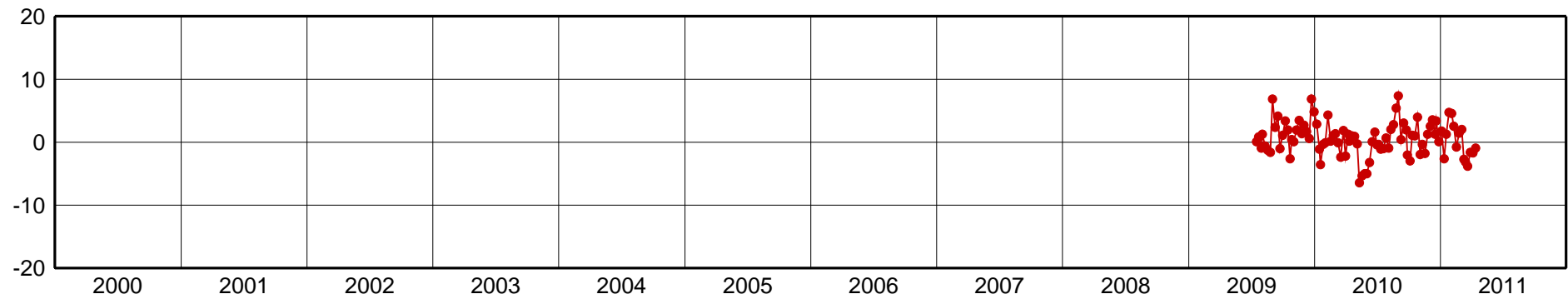
PRMA-Up Component [mm]
