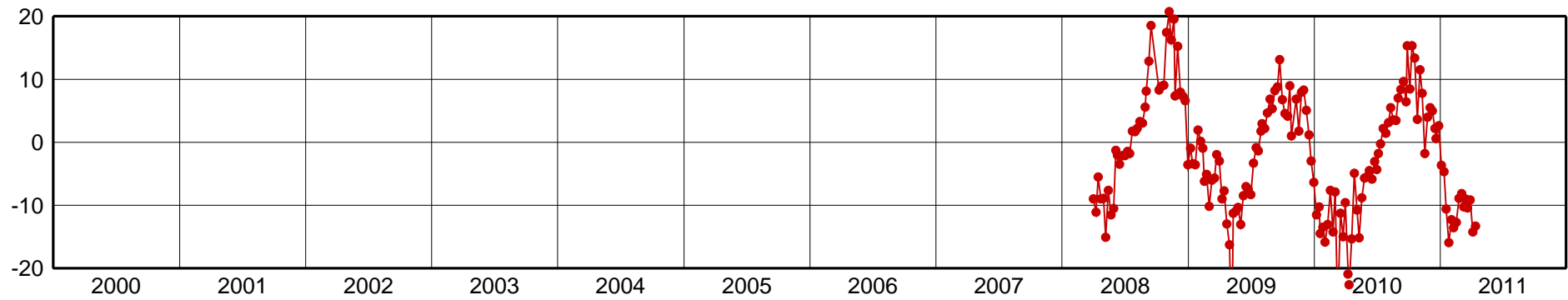
MTSF-Up Component [mm]
