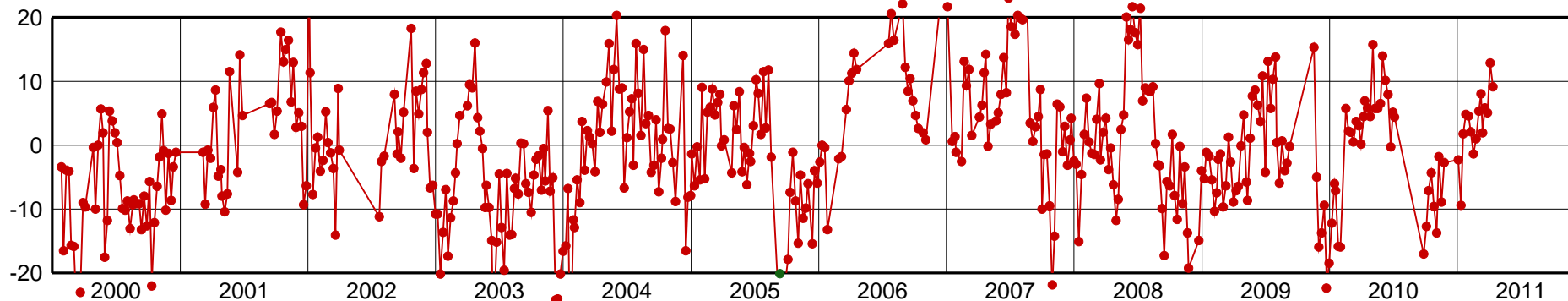
VESL-Up Component [mm]
