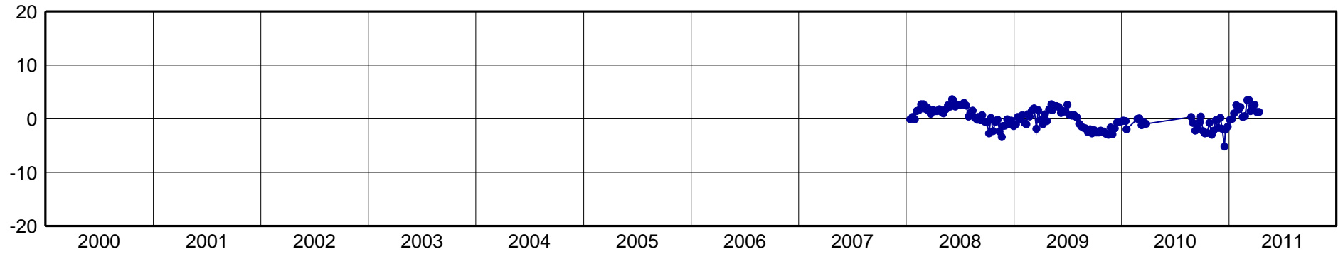
MSCG-North Component [mm]
