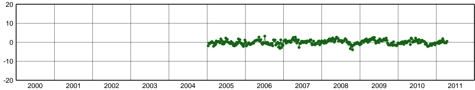
MERI-East Component [mm]
