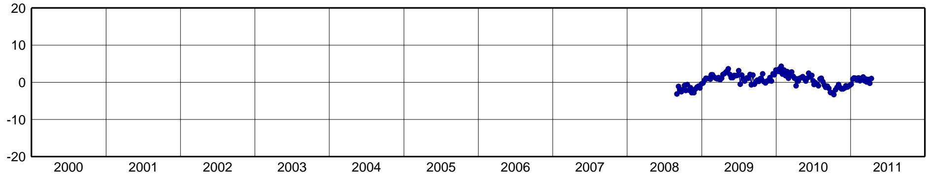
USLP-North Component [mm]
