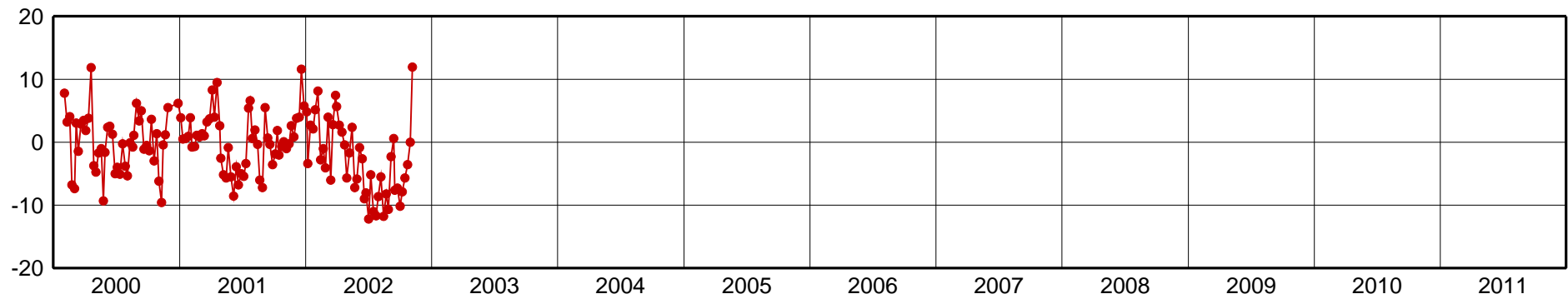
GALA-Up Component [mm]
