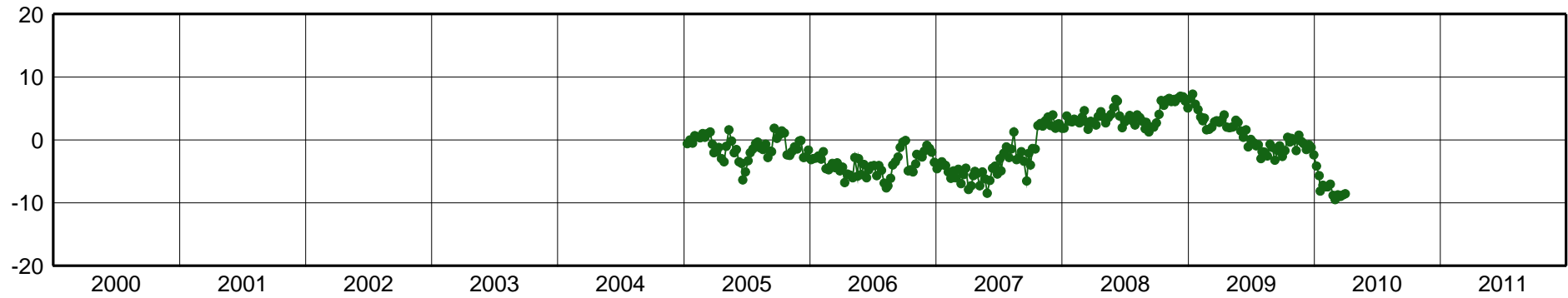
MEXI-East Component [mm]
