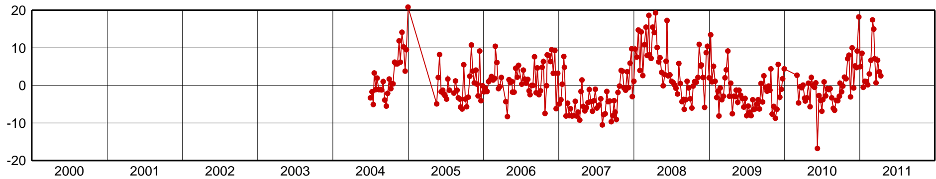
GVAL-Up Component [mm]
