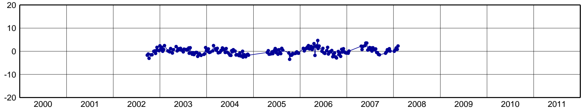
MPLA-North Component [mm]
