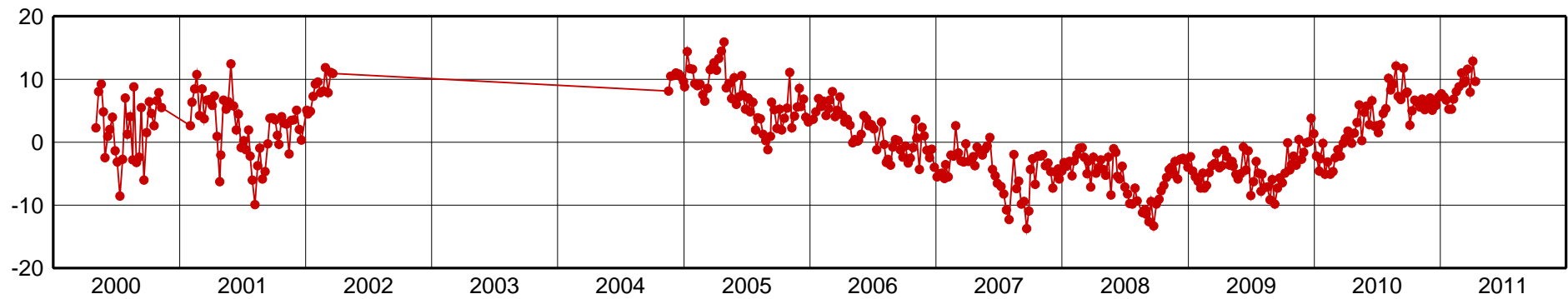
INEG-Up Component [mm]
