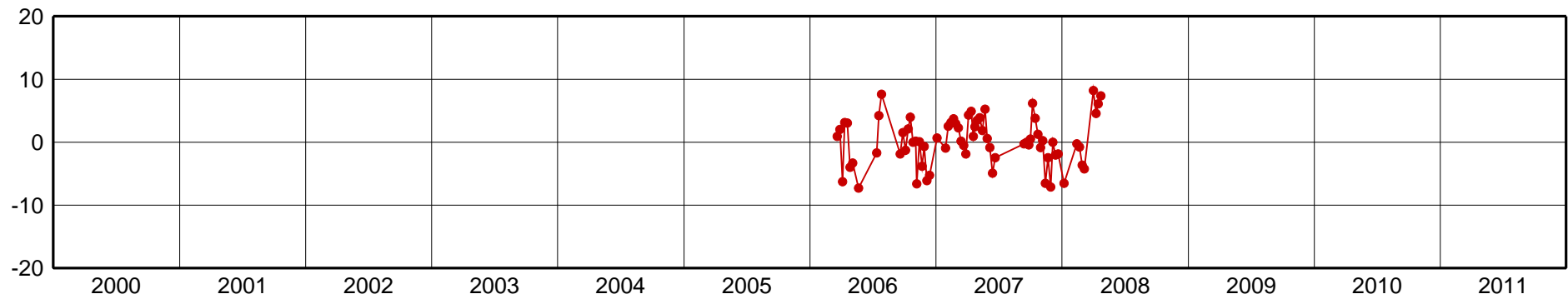
MOTE-Up Component [mm]
