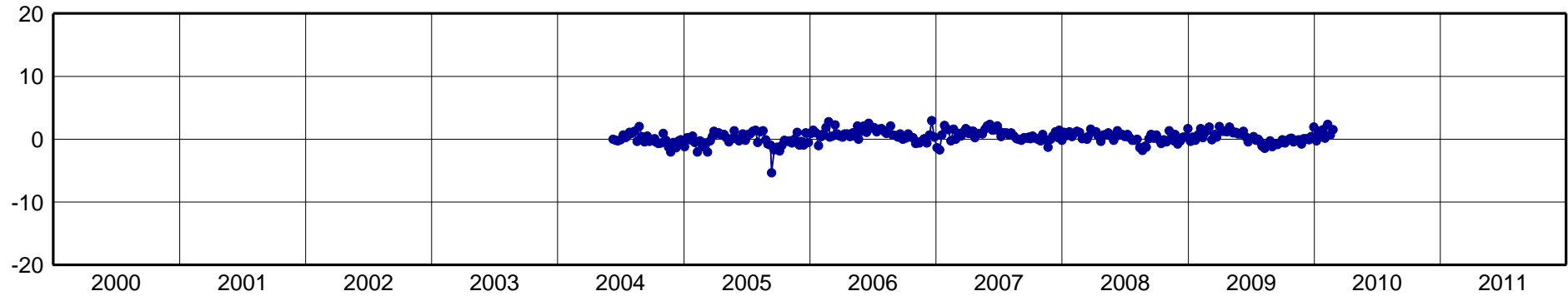
MZAC-North Component [mm]
