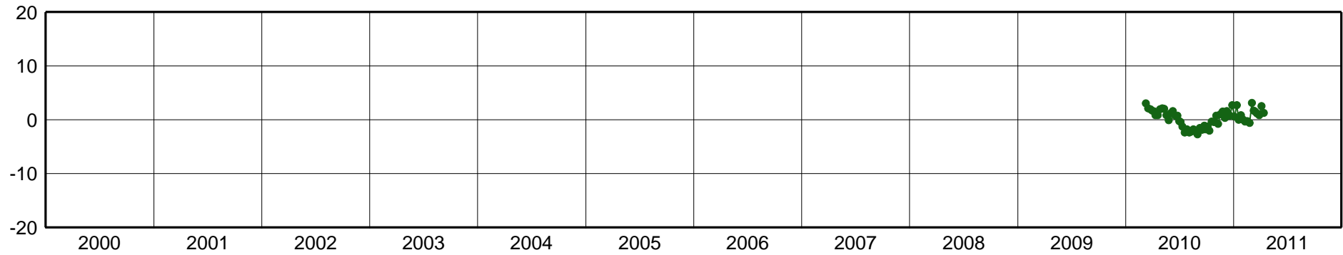
MPL2-East Component [mm]
