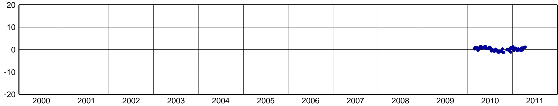
URUS-North Component [mm]
