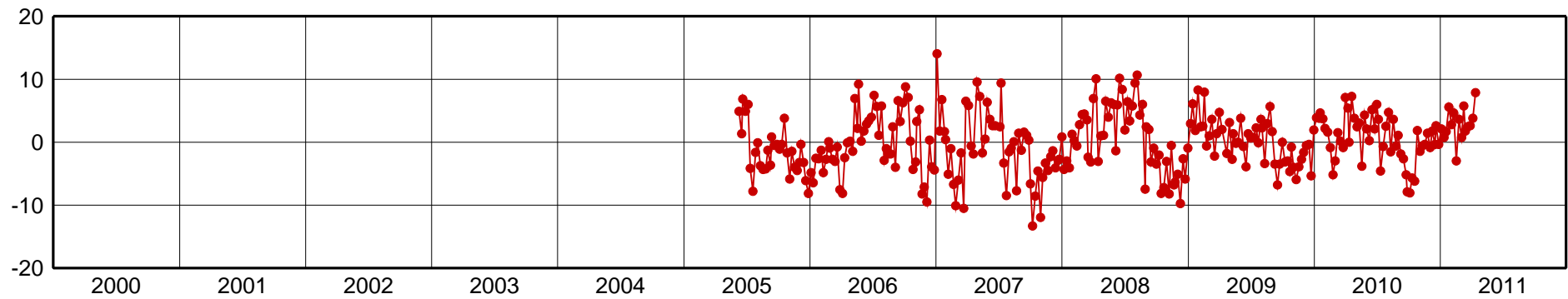
GCGT-Up Component [mm]
