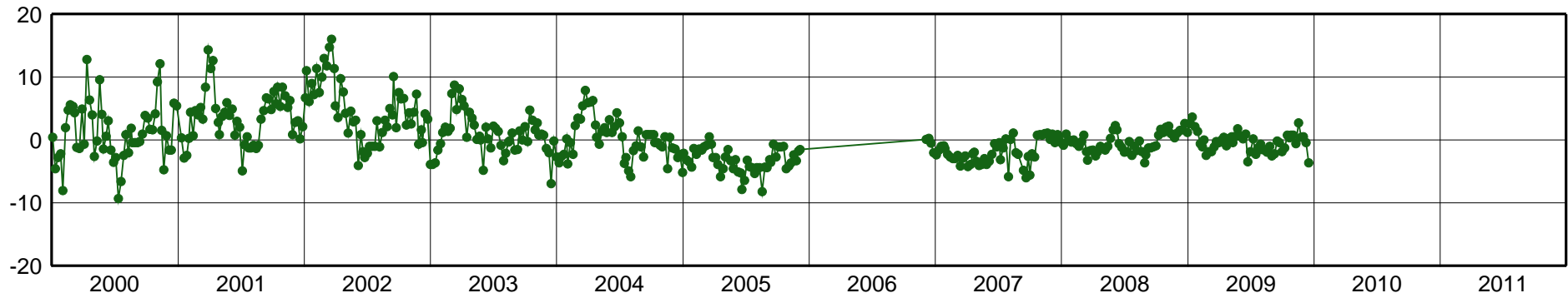
CIC1-East Component [mm]
