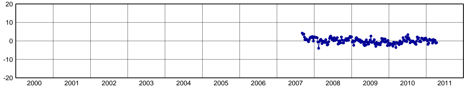
RIOB-North Component [mm]
