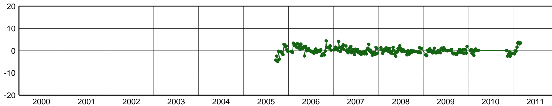
VIVI-East Component [mm]
