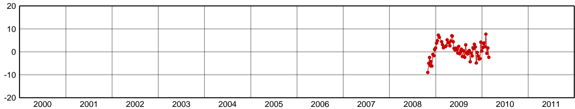
UYTA-Up Component [mm]
