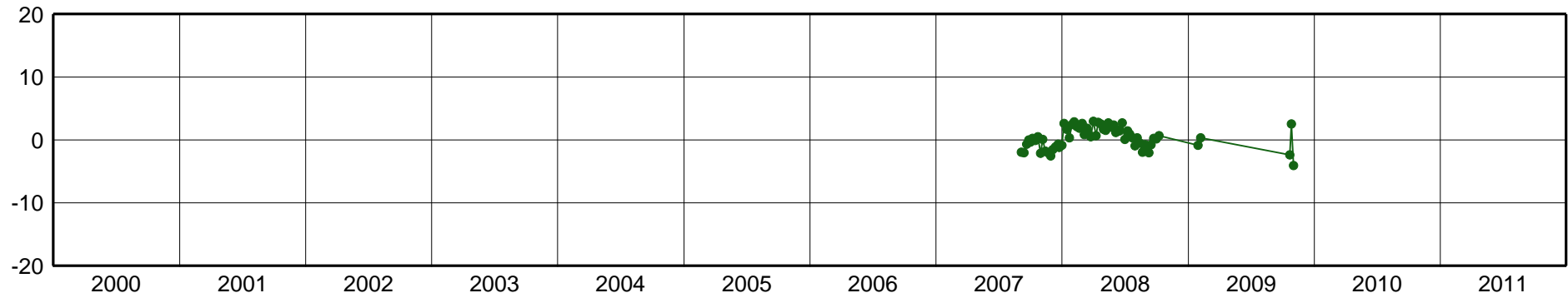
CRUZ-East Component [mm]
