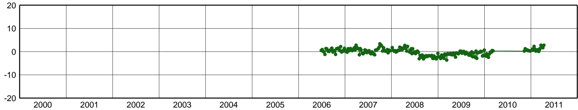
POPA-East Component [mm]
