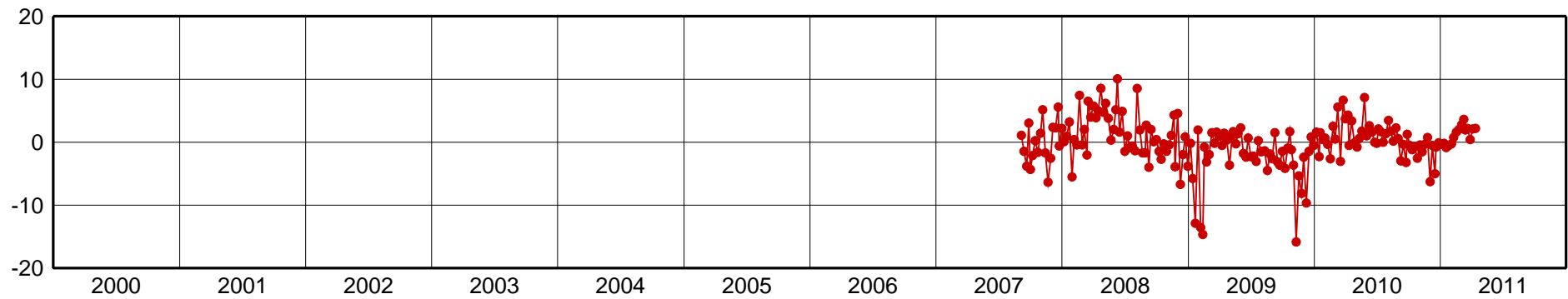
CEFE-Up Component [mm]
