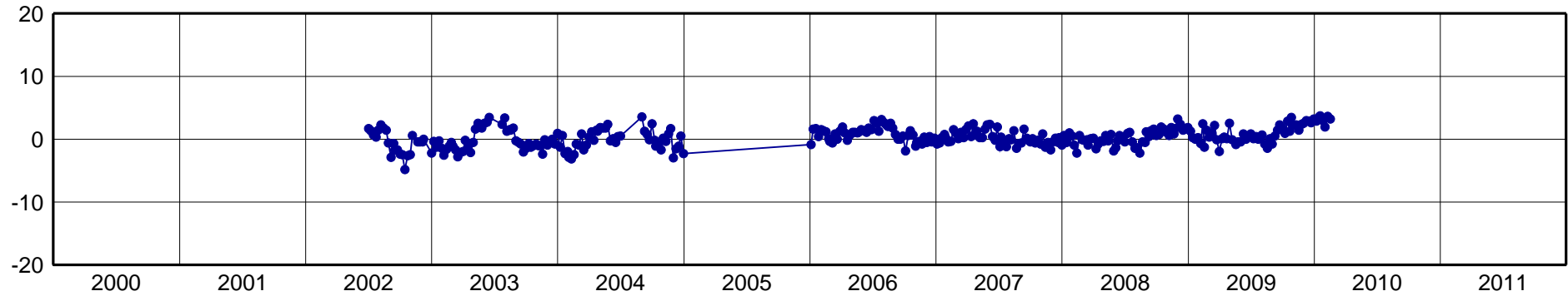
ANTC-North Component [mm]
