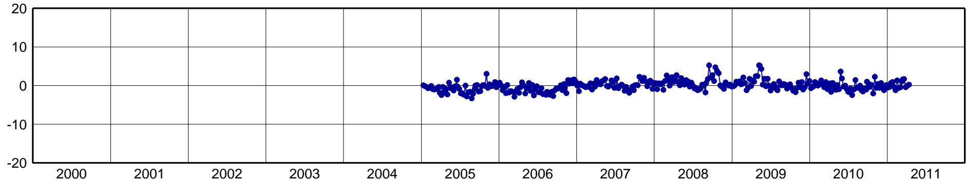
CHET-North Component [mm]
