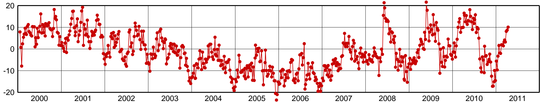
PALM-Up Component [mm]
