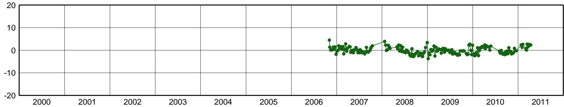
FLOR-East Component [mm]
