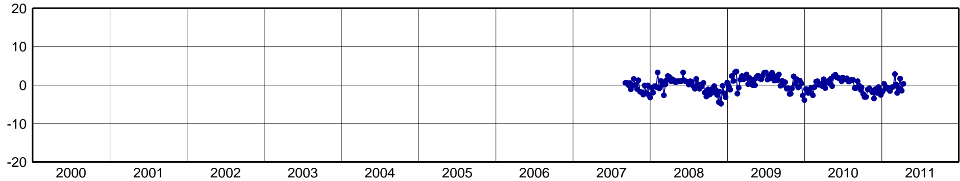
CEFE-North Component [mm]
