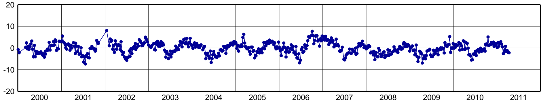
KOUR-North Component [mm]
