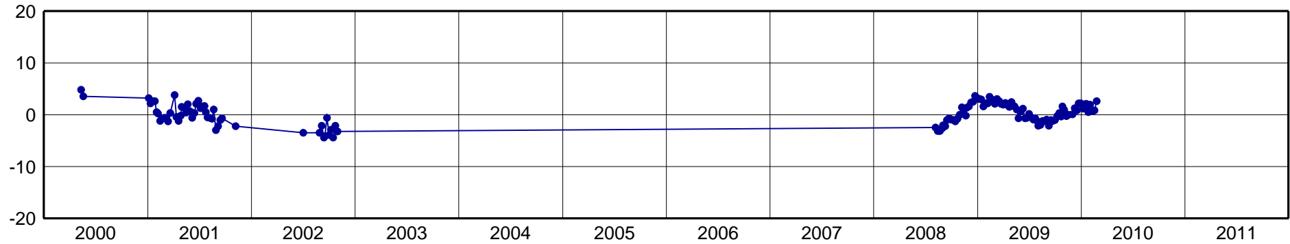
VALP-North Component [mm]
