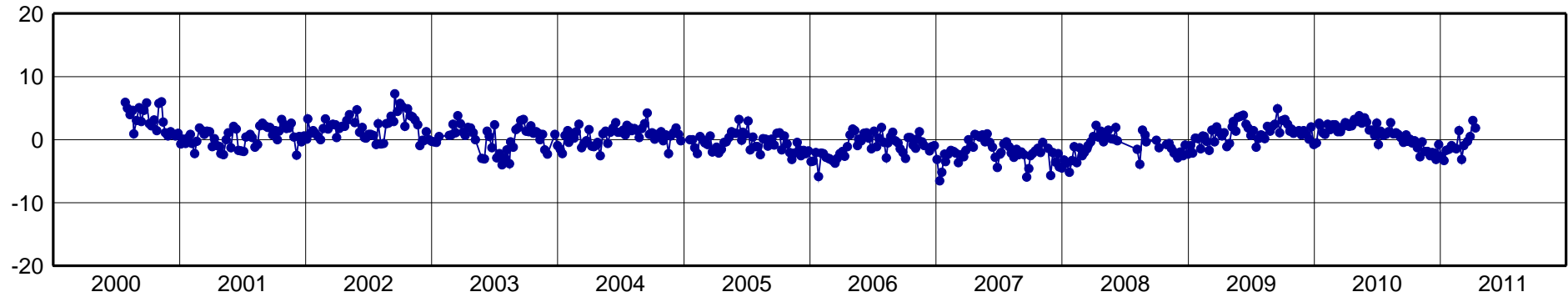
GUAT-North Component [mm]
