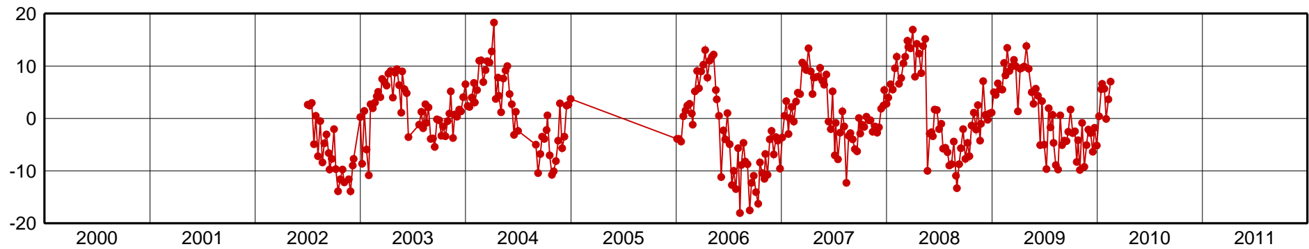
ANTC-Up Component [mm]
