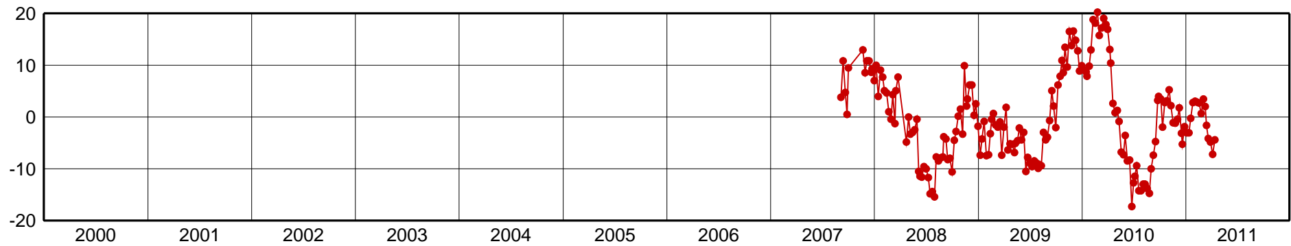
BOAV-Up Component [mm]
