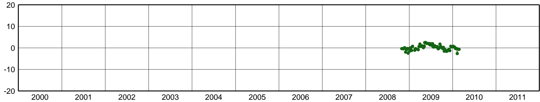
UYTA-East Component [mm]
