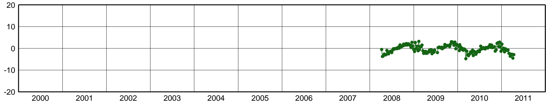
RJCG-East Component [mm]
