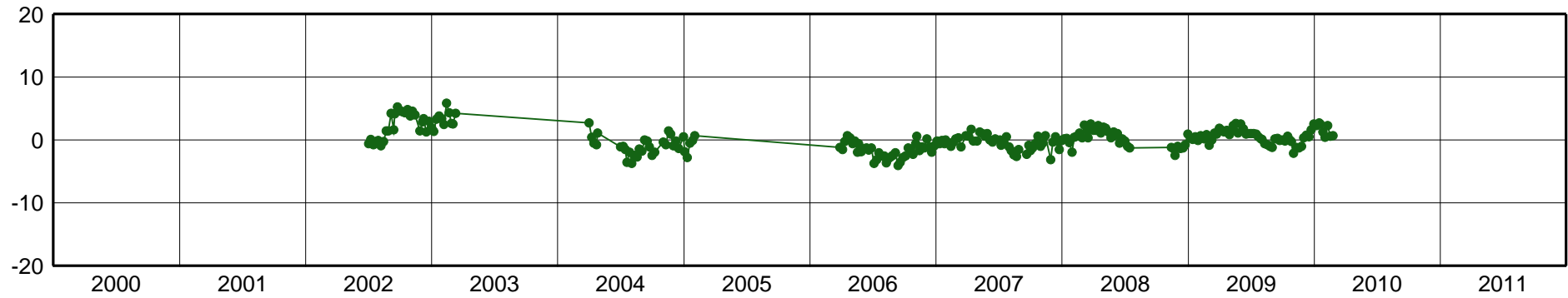
LHCL-East Component [mm]
