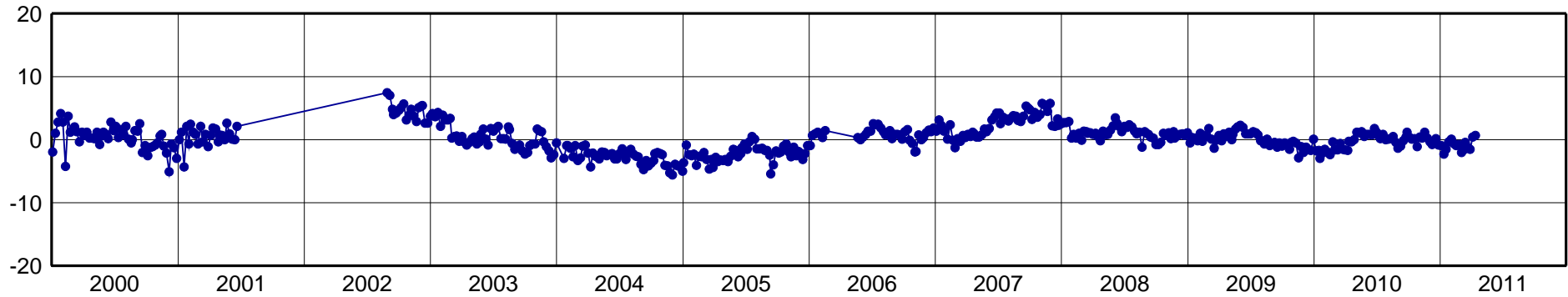
AREQ-North Component [mm]
