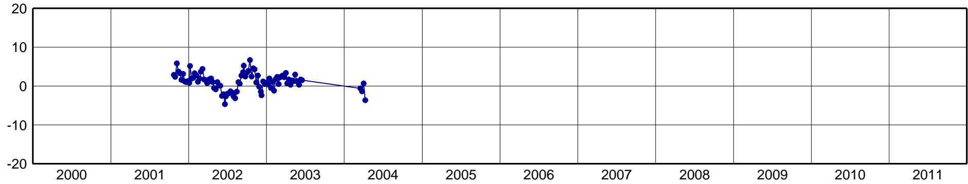
TEG1-North Component [mm]
