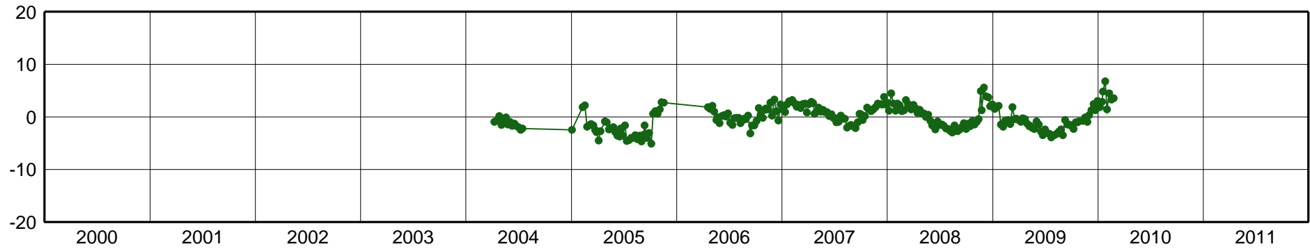
UCOR-East Component [mm]
