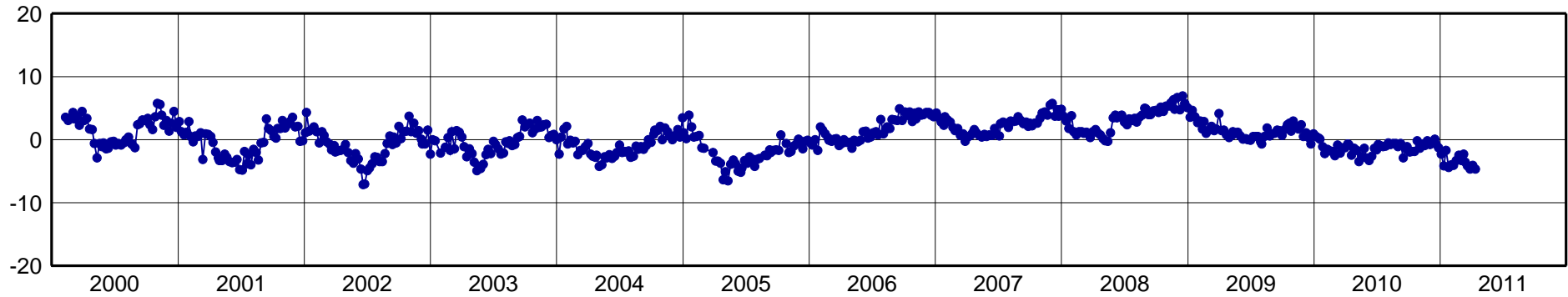
BOGA-North Component [mm]
