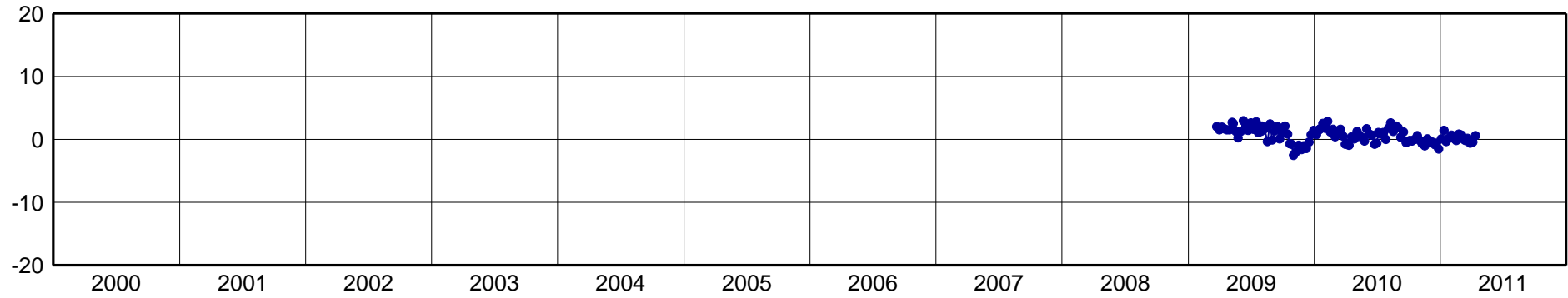
IDGO-North Component [mm]
