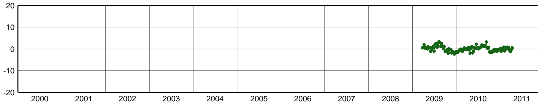
ICAM-East Component [mm]
