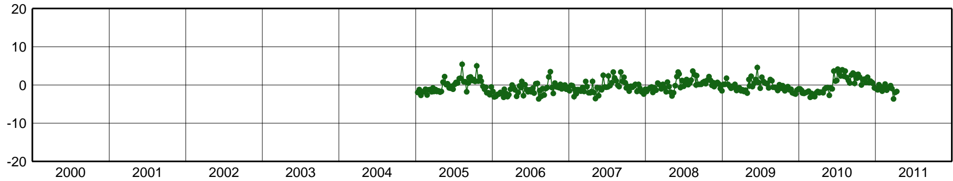
MTY2-East Component [mm]
