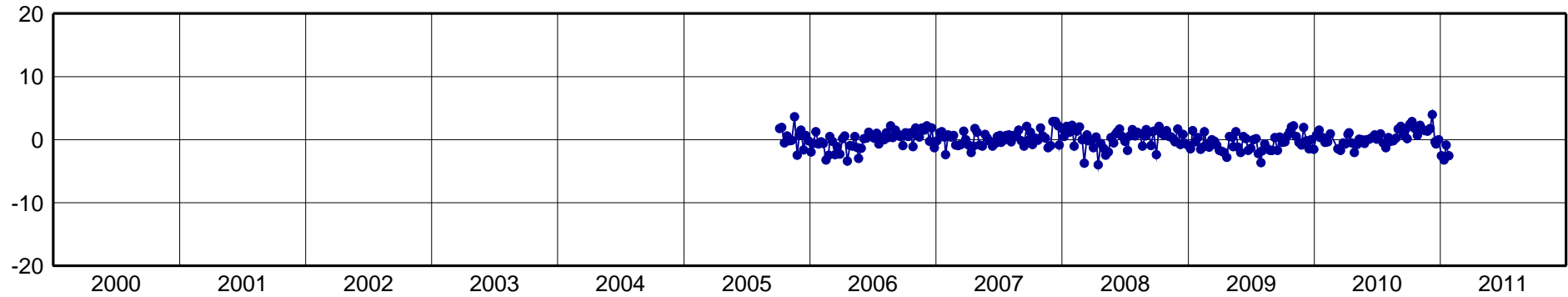
BUEN-North Component [mm]
