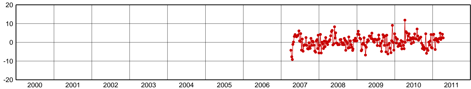
ONRJ-Up Component [mm]
