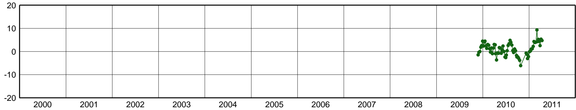
JBAL-East Component [mm]
