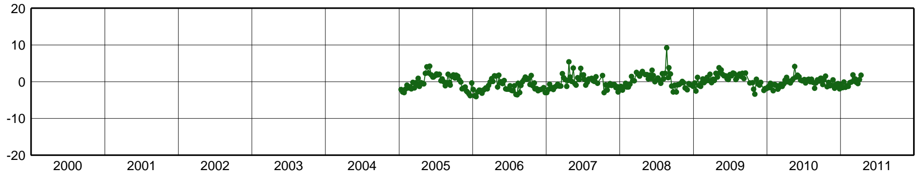
TAMP-East Component [mm]
