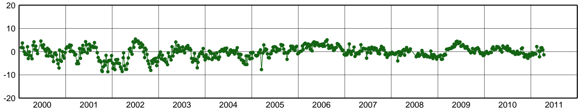
MARA-East Component [mm]
