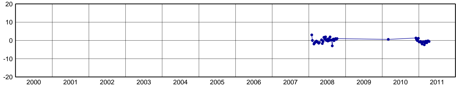
AMHU-North Component [mm]
