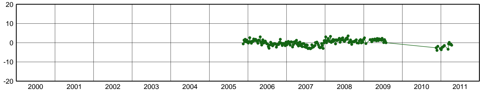
NEVA-East Component [mm]
