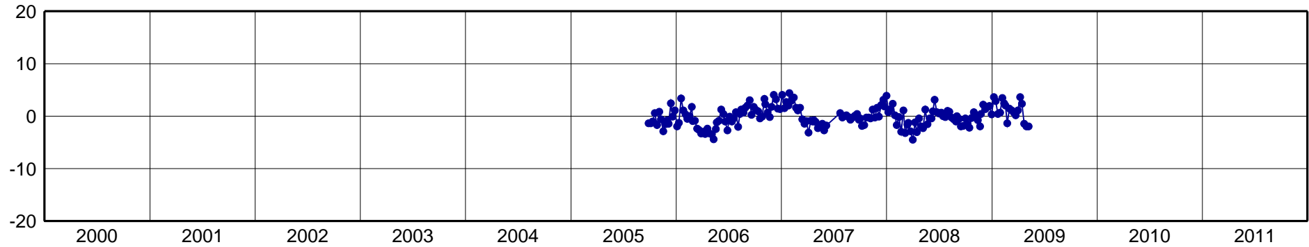
BUCA-North Component [mm]
