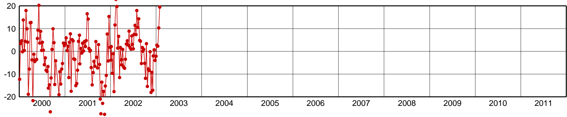
EISL-Up Component [mm]
