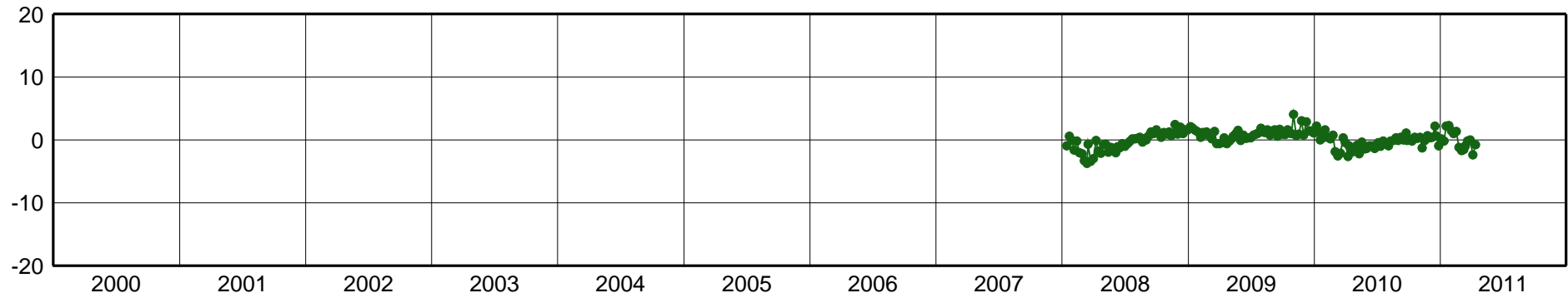
MGUB-East Component [mm]
