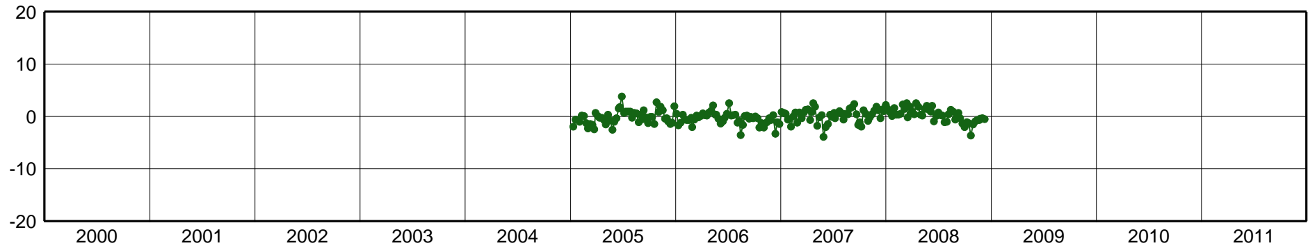
CAM2-East Component [mm]
