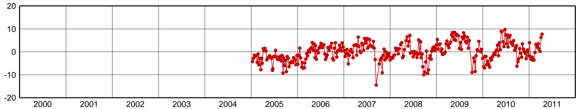
TAMP-Up Component [mm]
