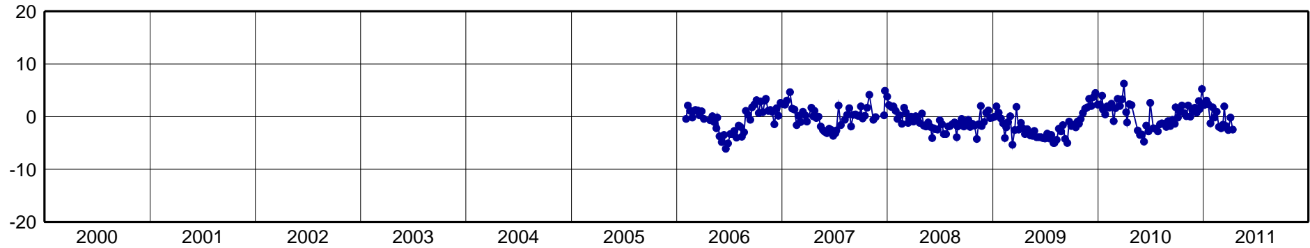
SRZN-North Component [mm]
