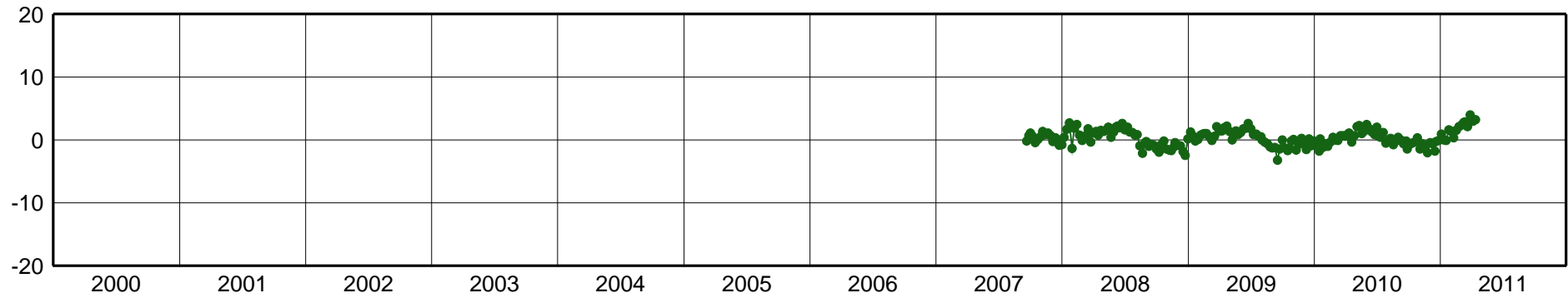
SAGA-East Component [mm]
