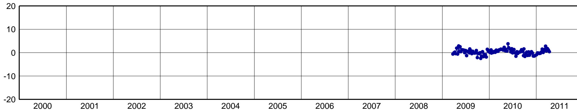
ICAM-North Component [mm]
