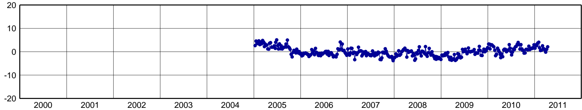
COL2-North Component [mm]
