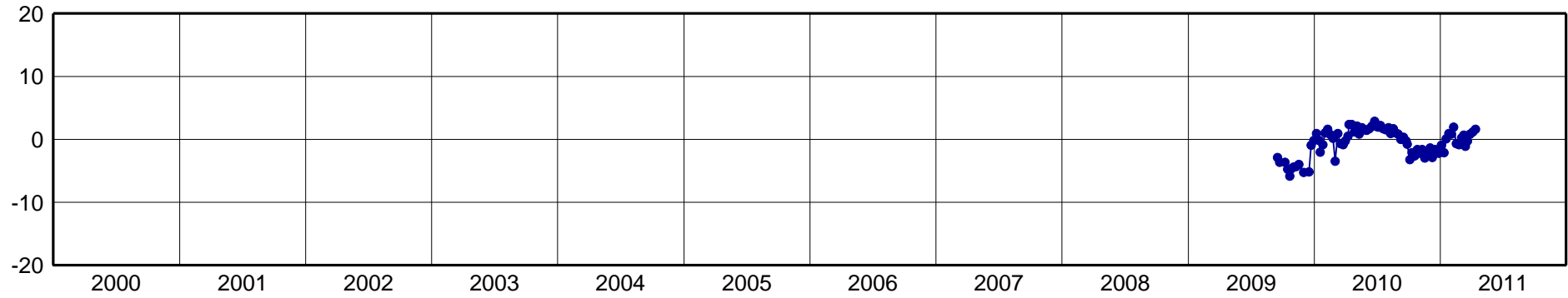
SJRP-North Component [mm]
