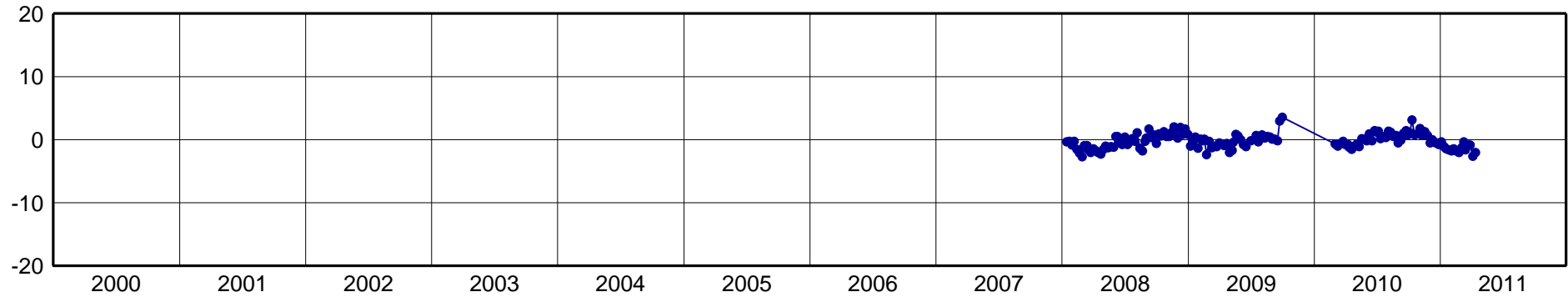
PSTO-North Component [mm]
