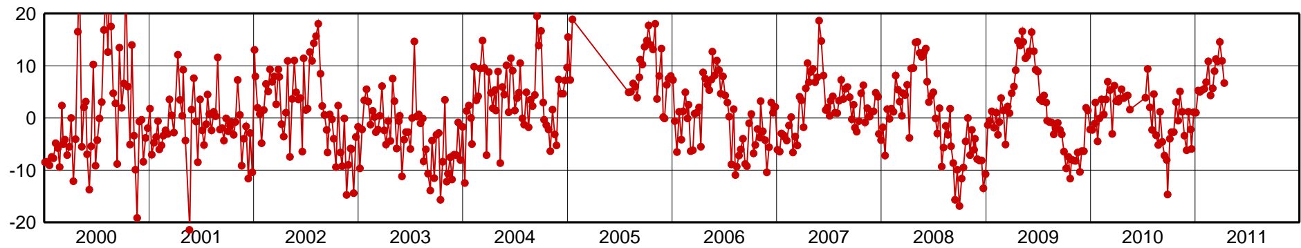
CRO1-Up Component [mm]
