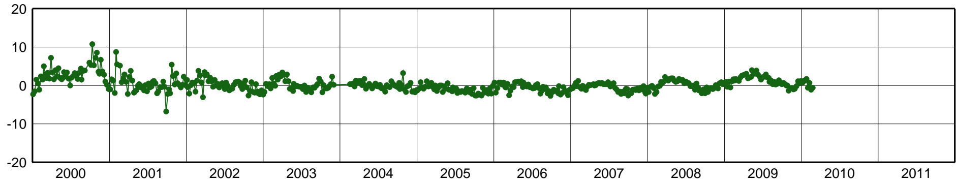
LPGS-East Component [mm]
