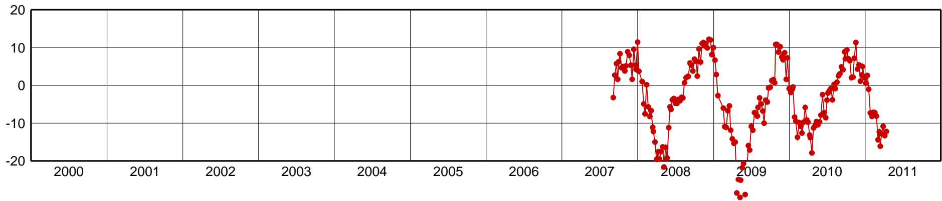
MABA-Up Component [mm]
