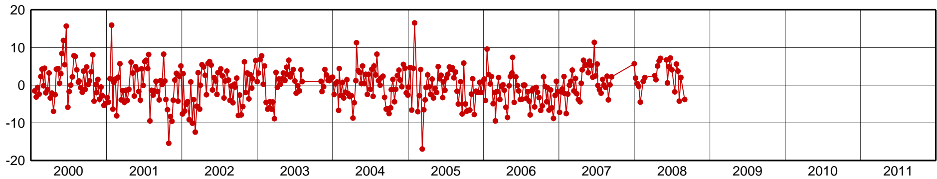
SALV-Up Component [mm]
