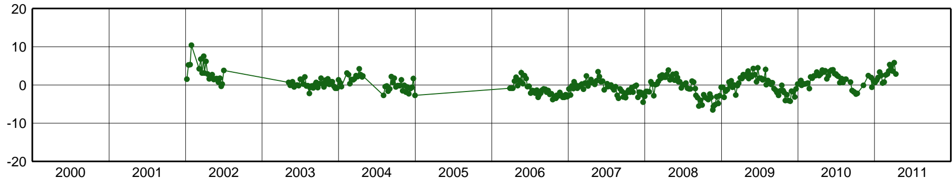
AUTF-East Component [mm]
