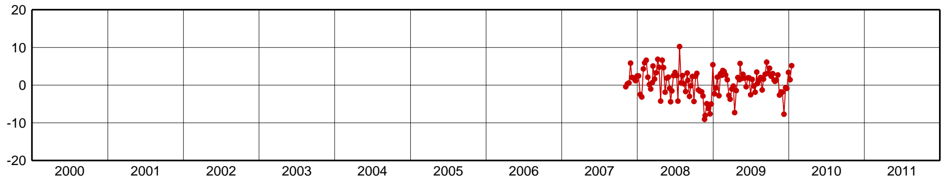
APTO-Up Component [mm]
