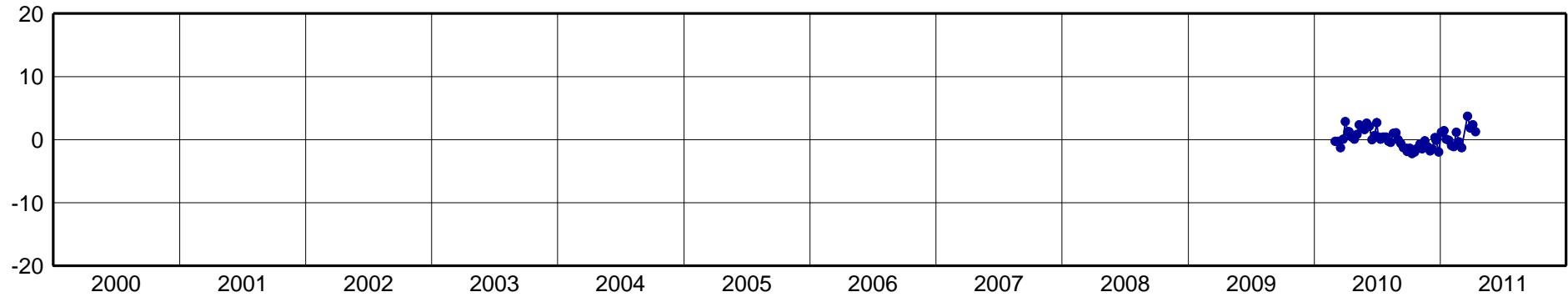
EBYP-North Component [mm]
