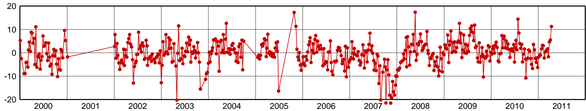
SCUB-Up Component [mm]
