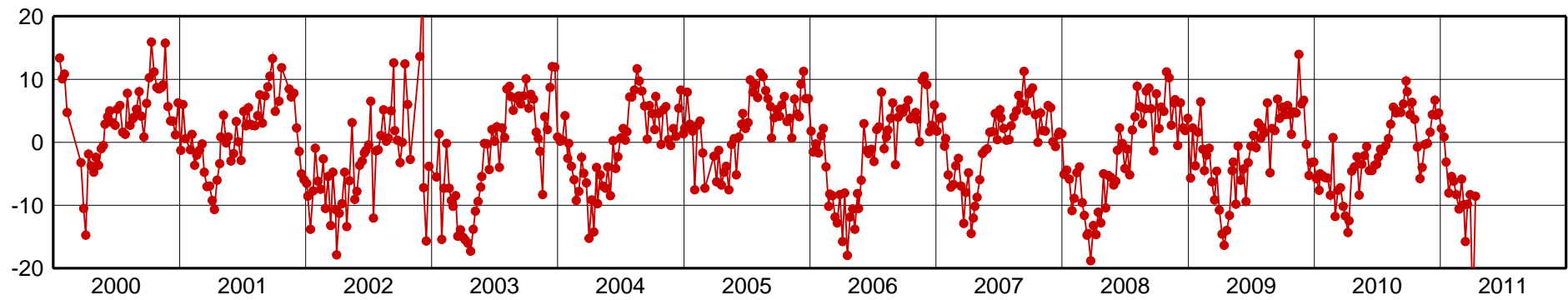
CUIB-Up Component [mm]
