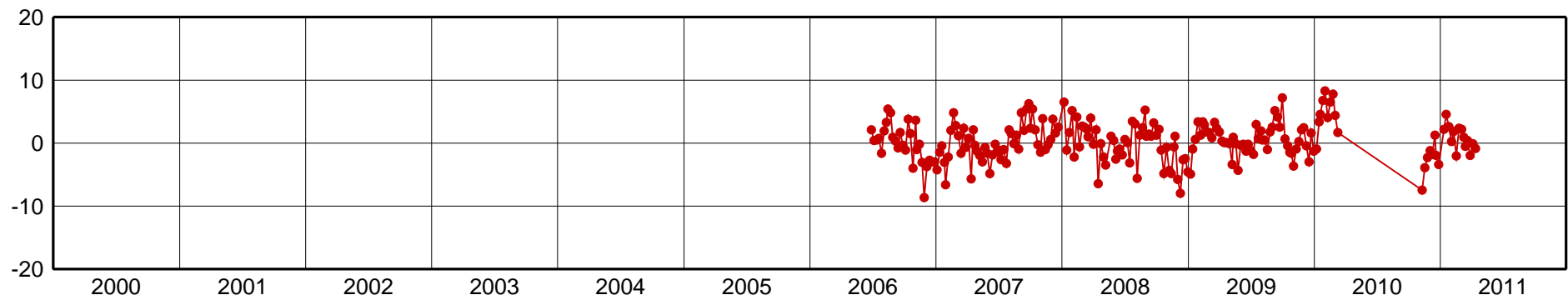
POPA-Up Component [mm]
