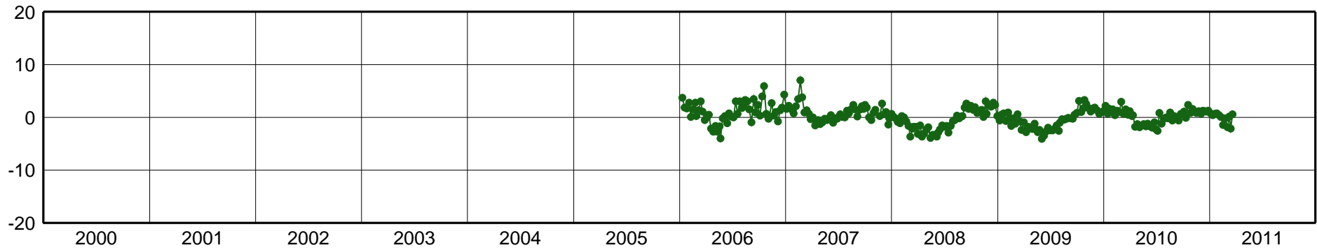
MAPA-East Component [mm]
