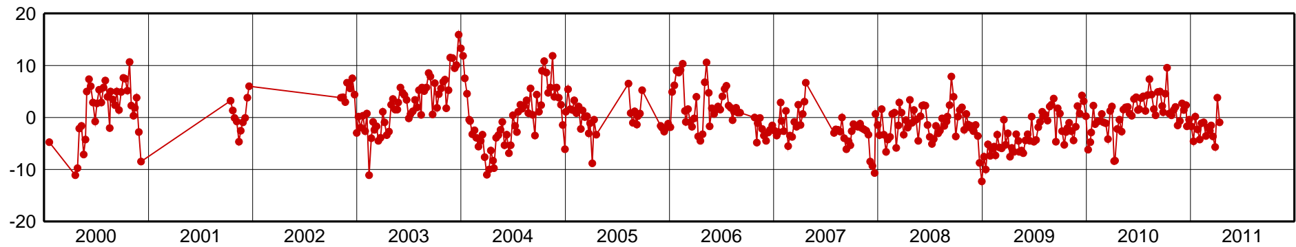
BOMJ-Up Component [mm]
