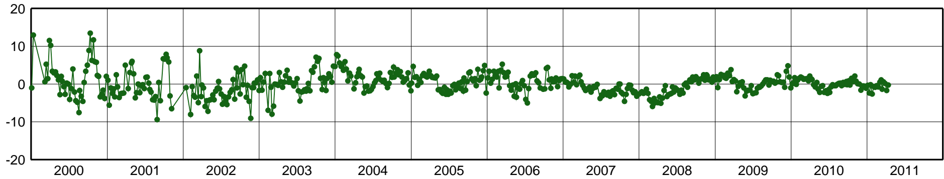
KOUR-East Component [mm]
