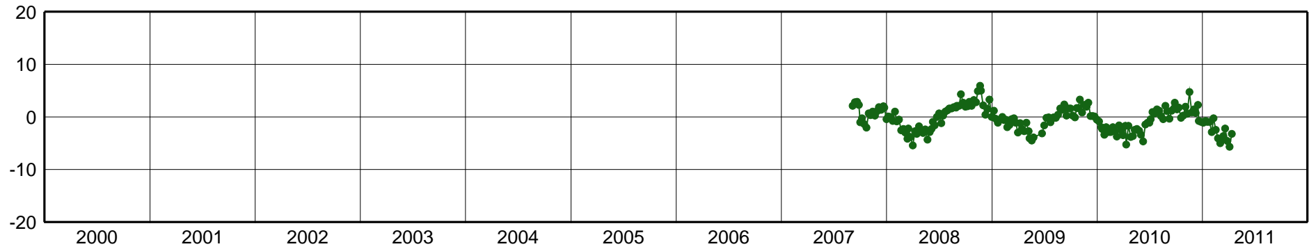
SSA1-East Component [mm]
