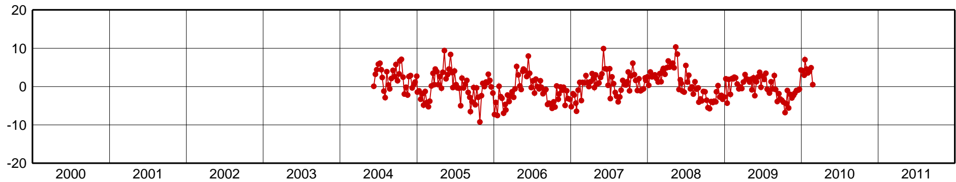
MZAC-Up Component [mm]
