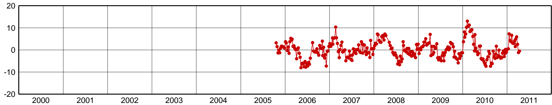
TUNA-Up Component [mm]
