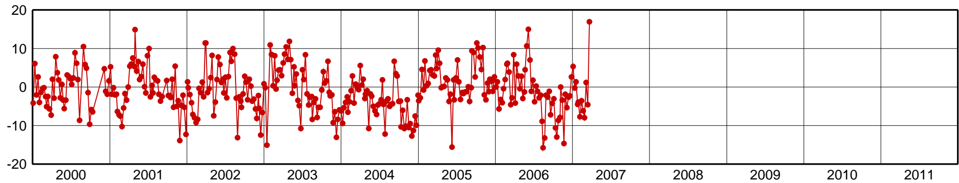
PUR3-Up Component [mm]
