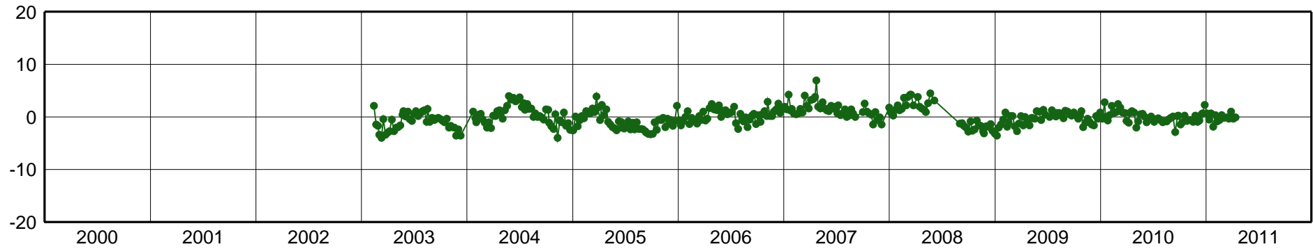
ETCG-East Component [mm]
