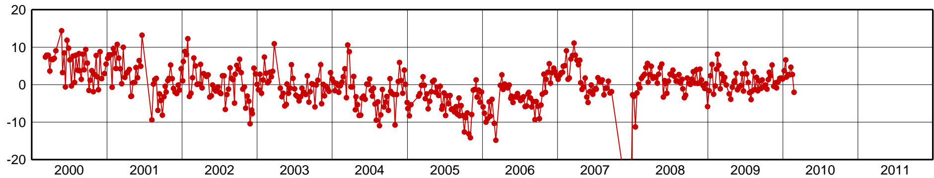
VBCA-Up Component [mm]
