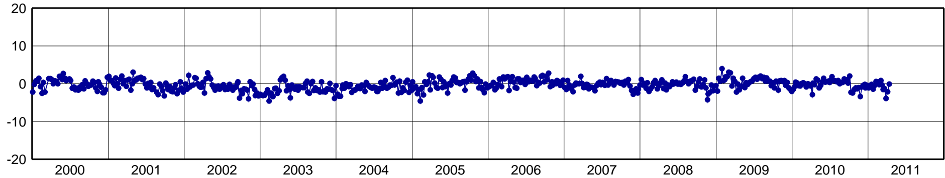
BRAZ-North Component [mm]
