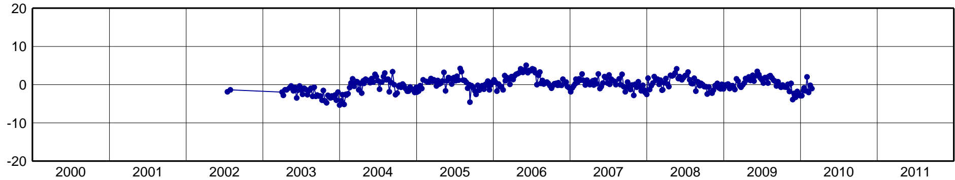
SMAR-North Component [mm]
