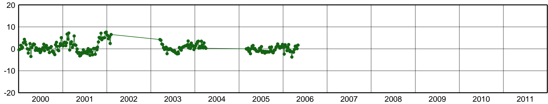
CORD-East Component [mm]
