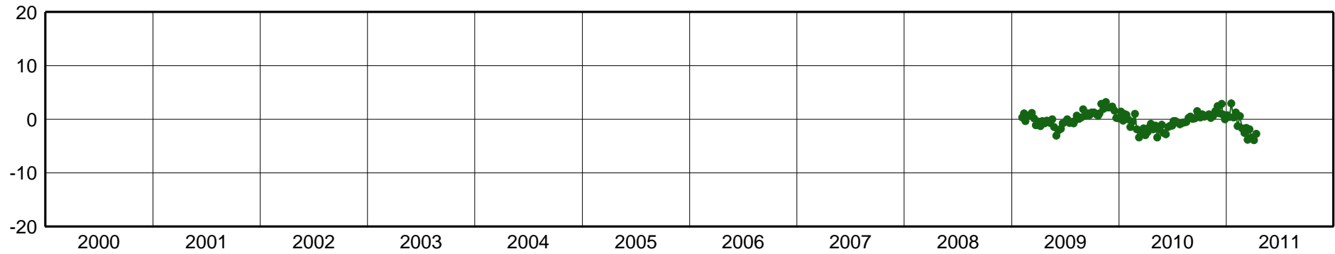
MGBH-East Component [mm]
