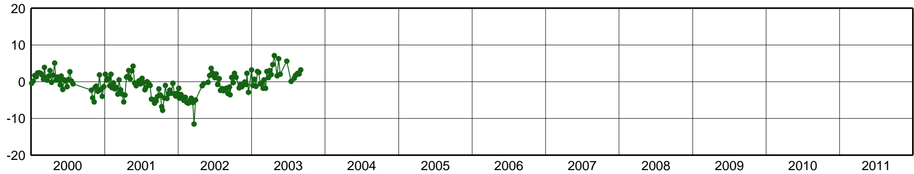
JAMA-East Component [mm]
