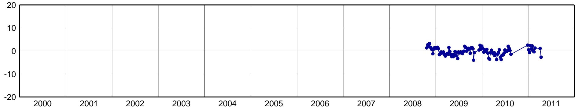
DAVI-North Component [mm]
