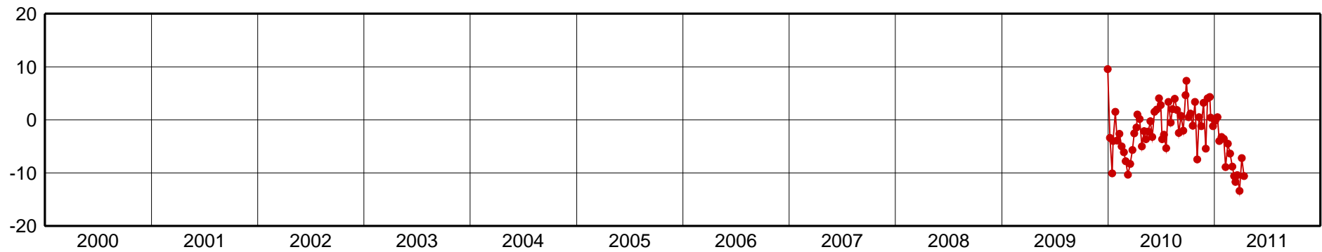
SCRZ-Up Component [mm]
