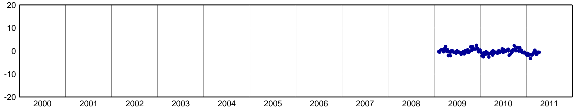
LJEC-North Component [mm]
