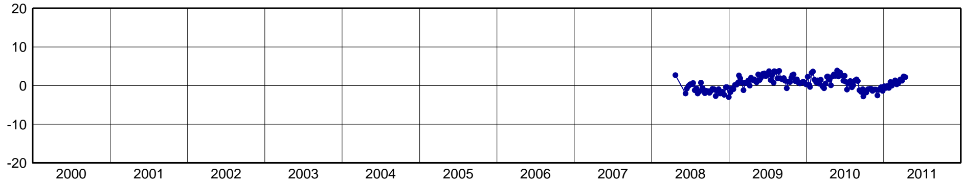
SCCH-North Component [mm]
