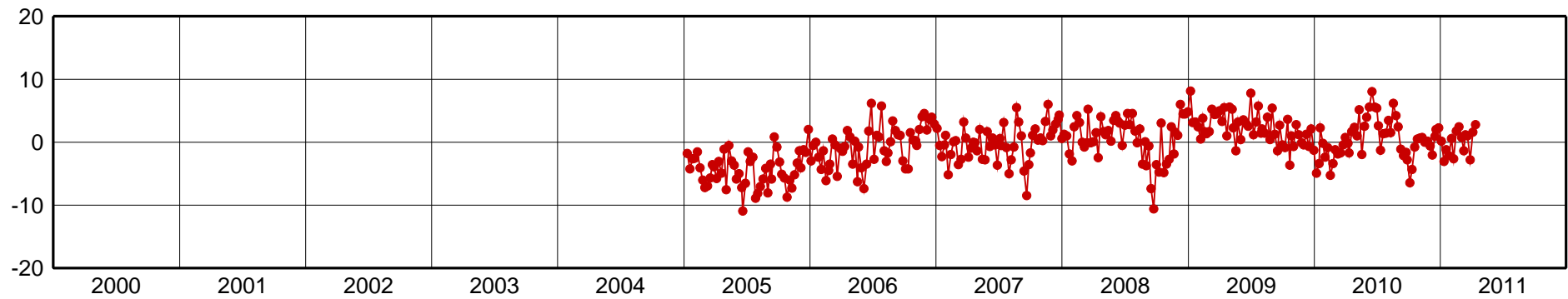
MTY2-Up Component [mm]
