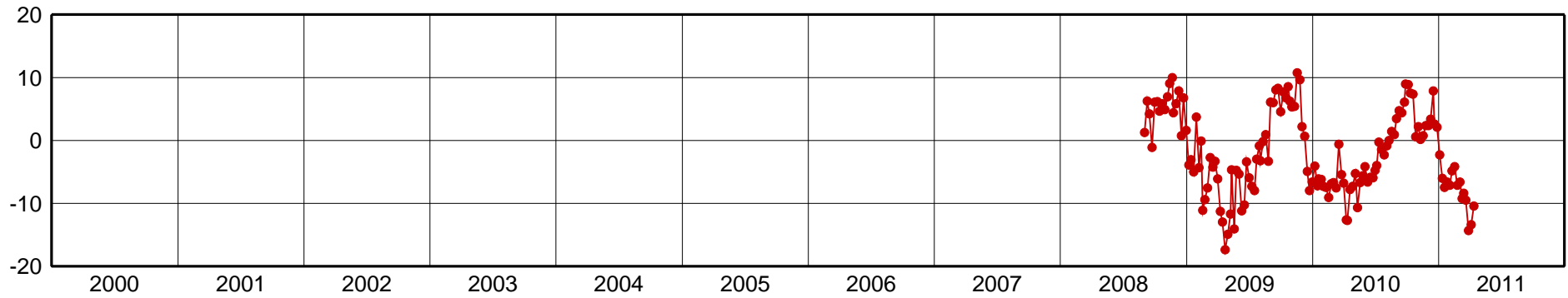
MTBA-Up Component [mm]
