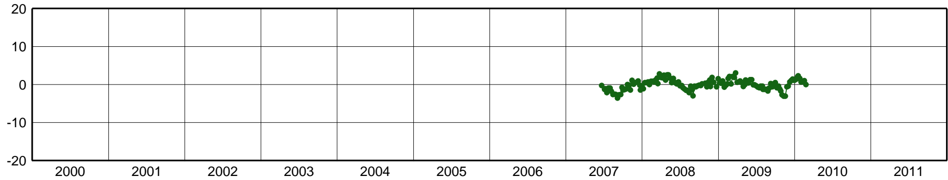
MZAE-East Component [mm]
