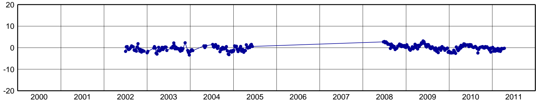
IQQE-North Component [mm]
