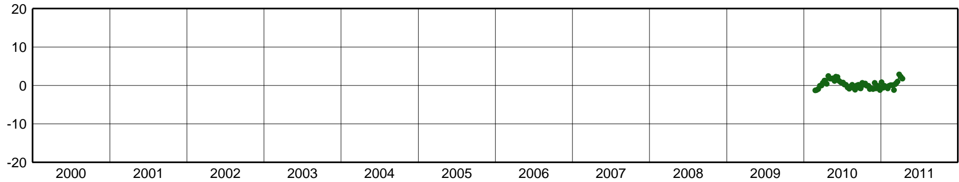
ABPW-East Component [mm]
