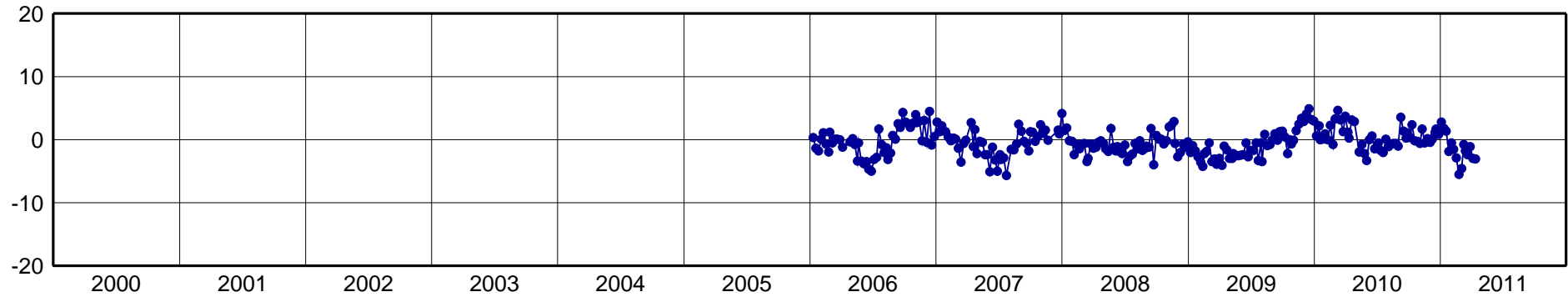
SRNW-North Component [mm]
