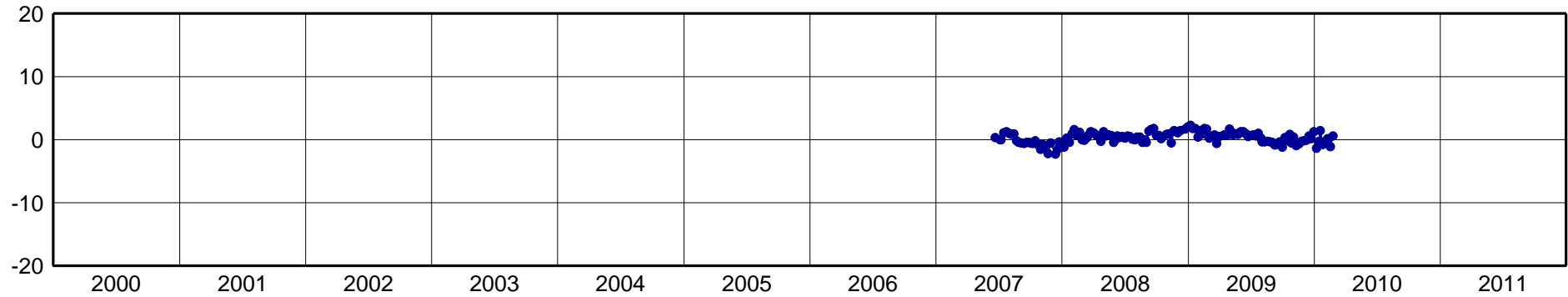
MZAE-North Component [mm]
