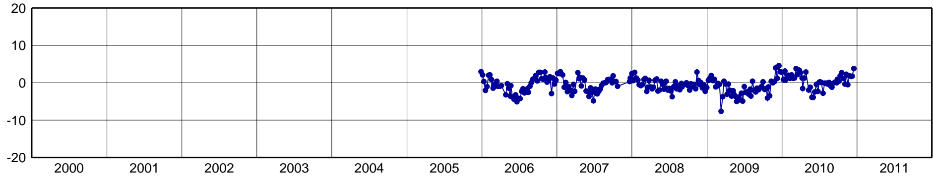
PMB1-North Component [mm]
