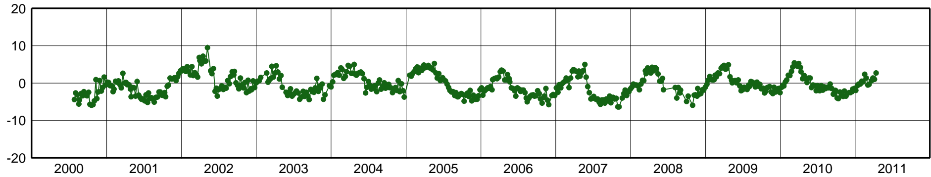
GUAT-East Component [mm]
