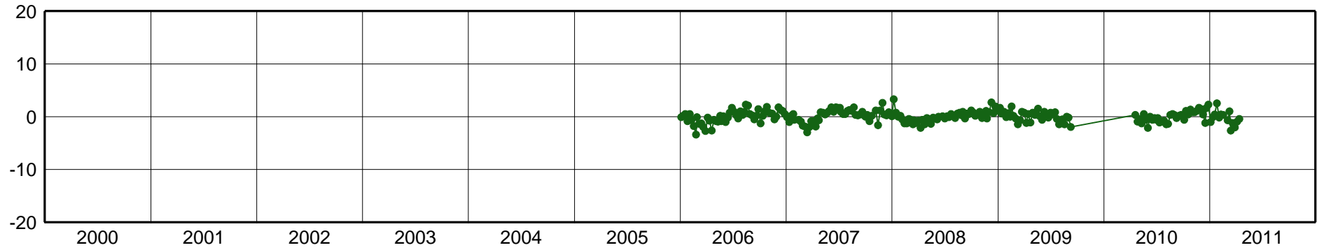
NEIA-East Component [mm]
