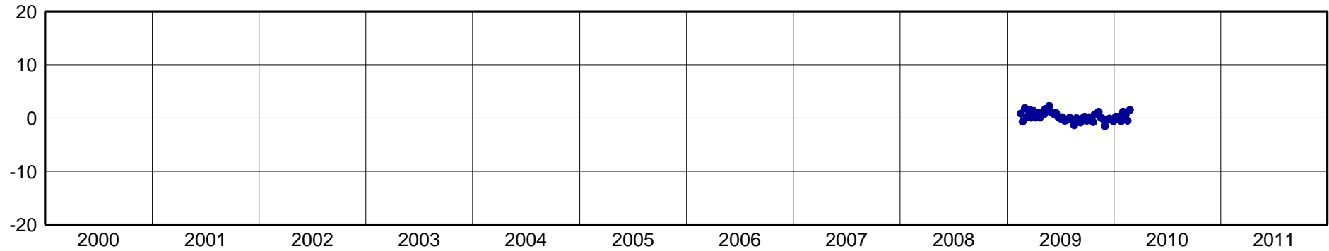
CATA-North Component [mm]
