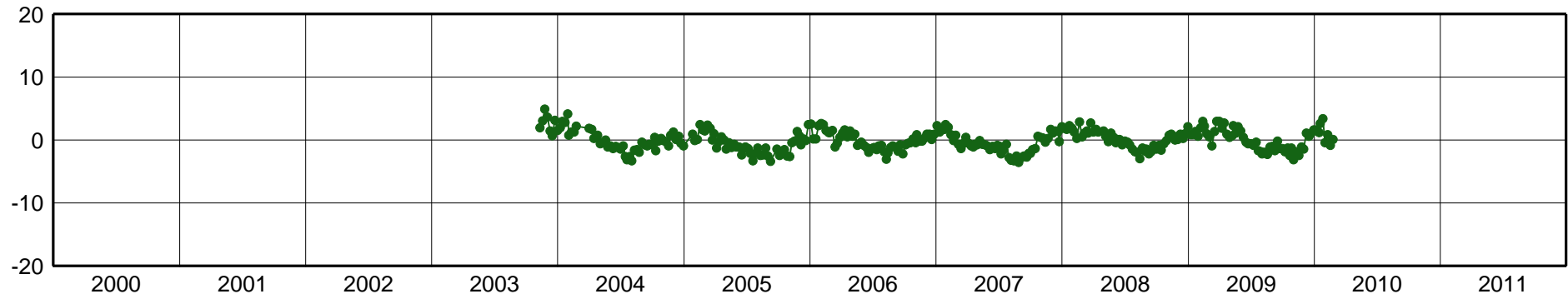
IGM1-East Component [mm]
