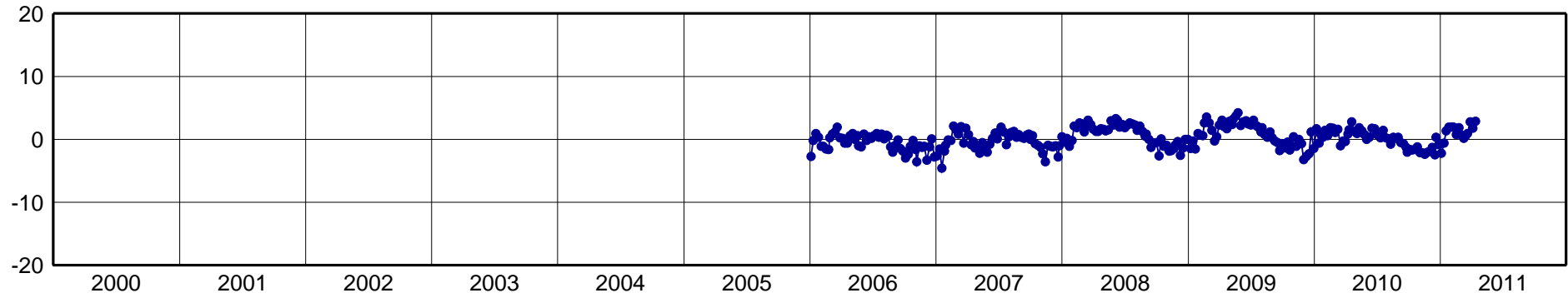
PPTE-North Component [mm]
