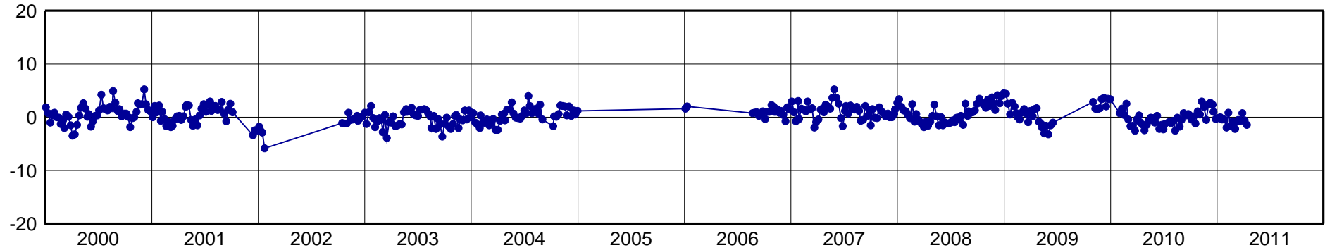
PARC-North Component [mm]
