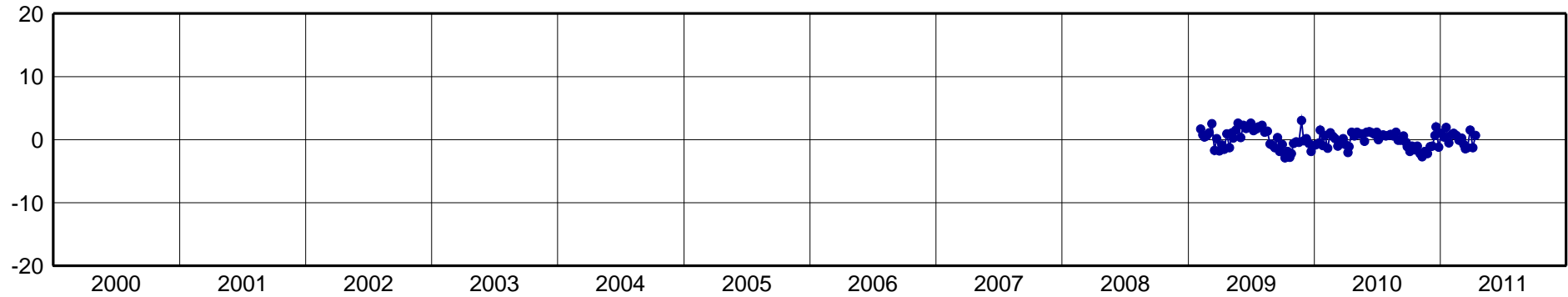
MGBH-North Component [mm]
