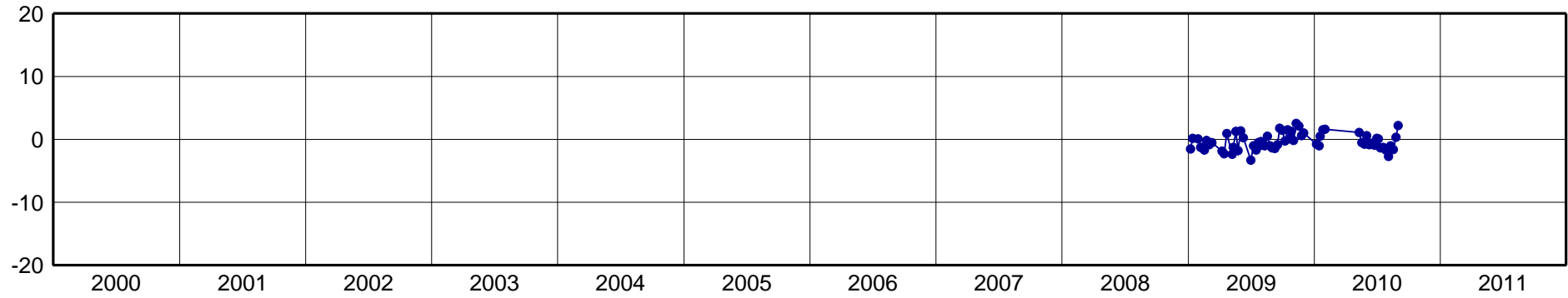
MAGA-North Component [mm]
