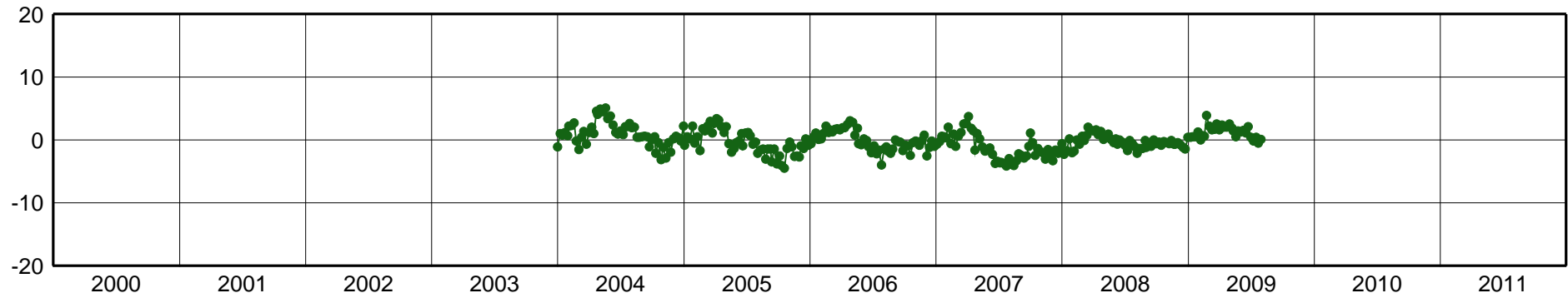
QUI1-East Component [mm]
