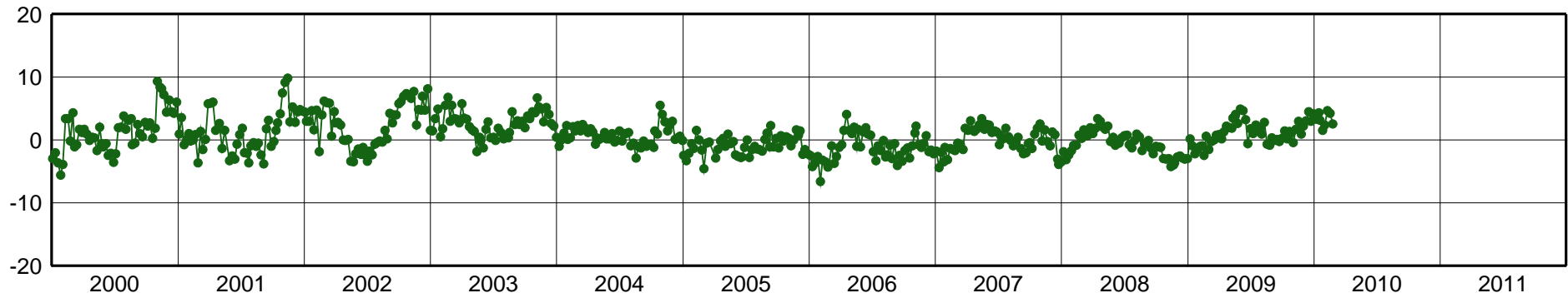
SANT-East Component [mm]
