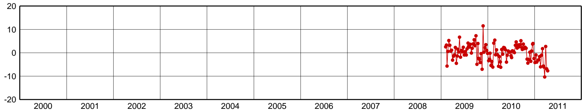
MGBH-Up Component [mm]
