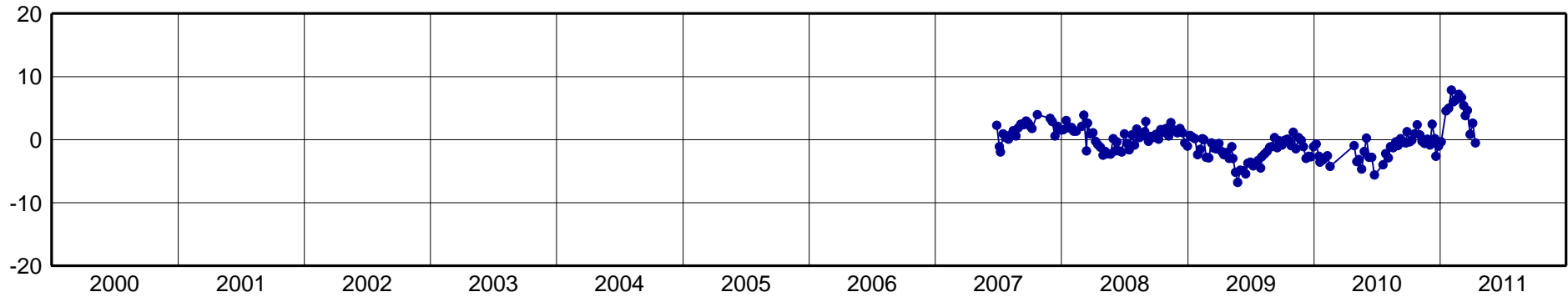
BRFT-North Component [mm]
