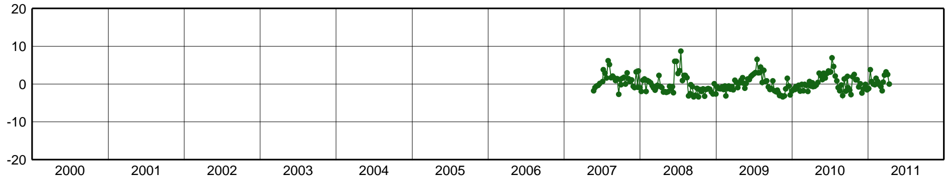
SMRT-East Component [mm]
