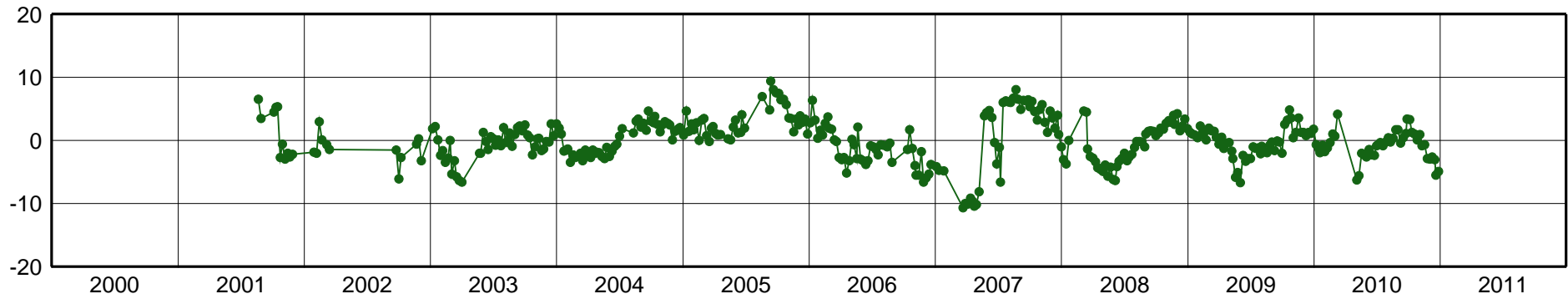
CRAT-East Component [mm]
