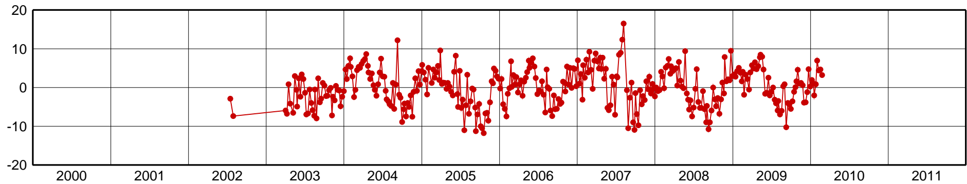
SMAR-Up Component [mm]
