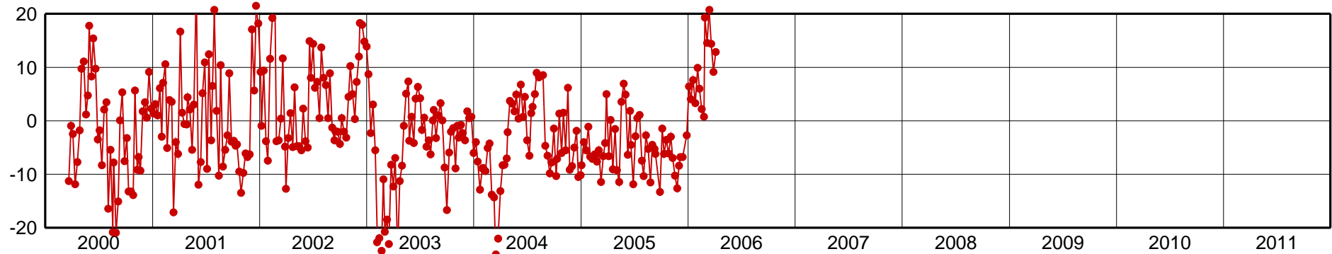
FORT-Up Component [mm]
