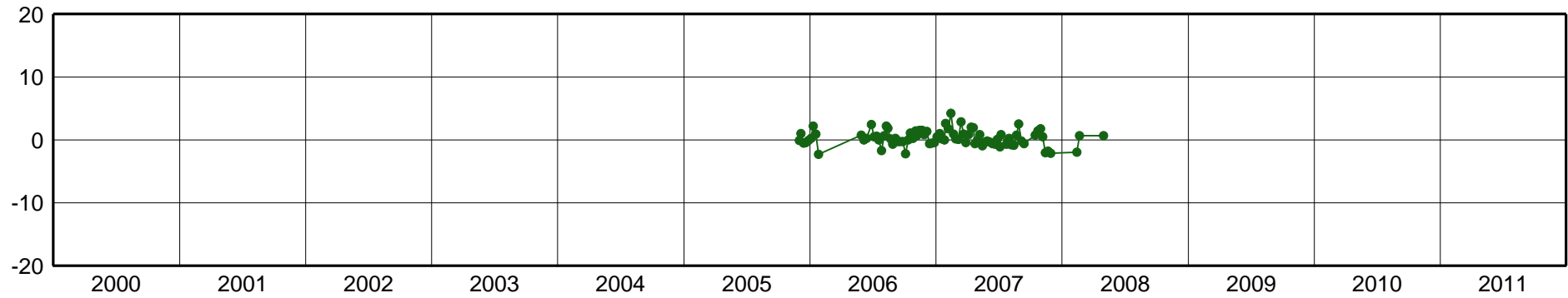
YOPA-East Component [mm]
