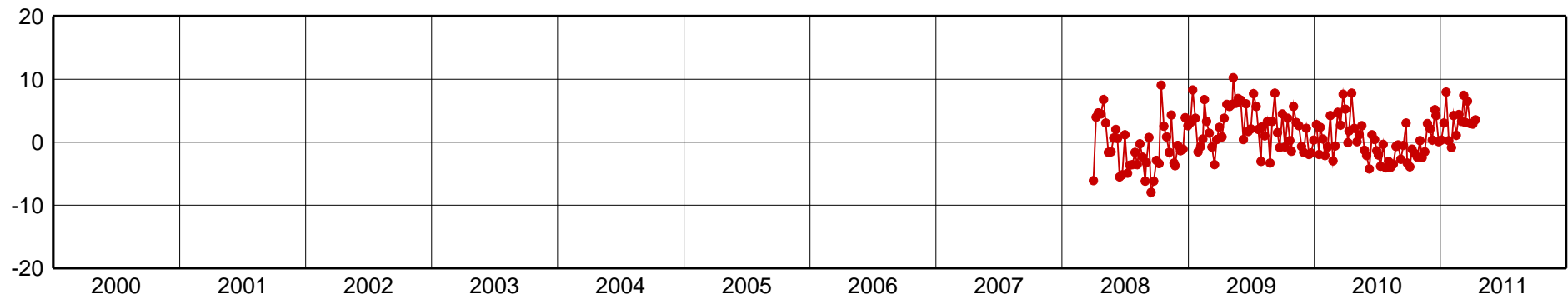
SCLA-Up Component [mm]
