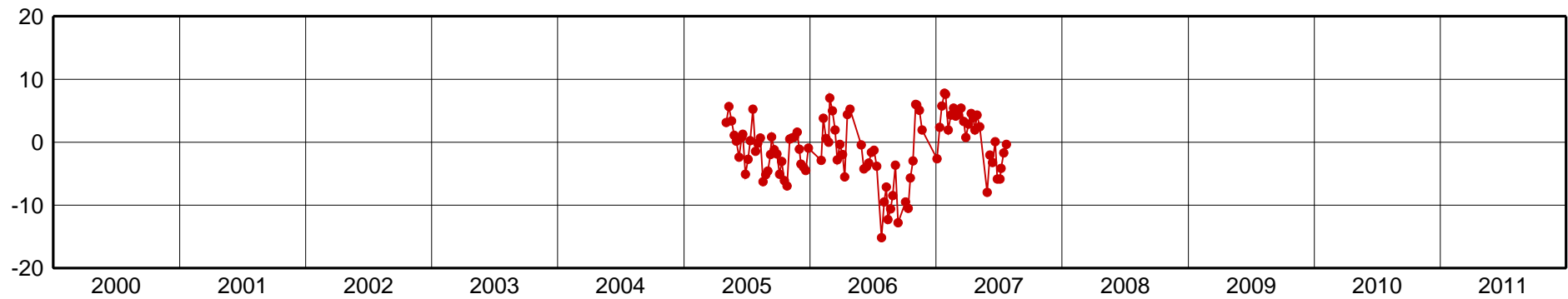
PDES-Up Component [mm]
