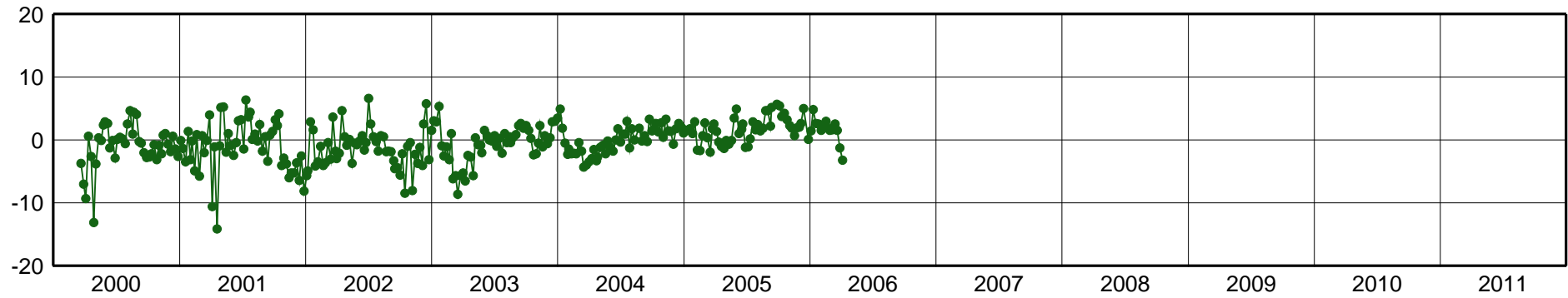
FORT-East Component [mm]
