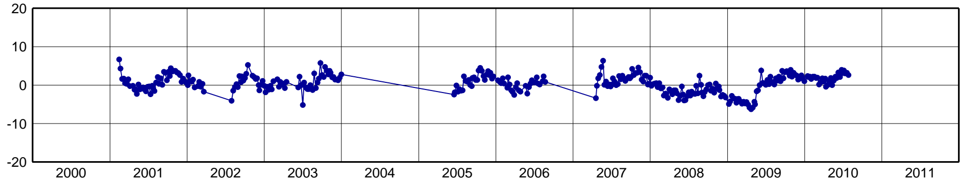
SSIA-North Component [mm]
