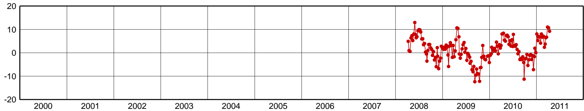
PBCG-Up Component [mm]
