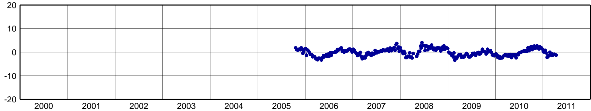
TUNA-North Component [mm]
