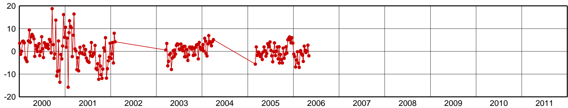
CORD-Up Component [mm]
