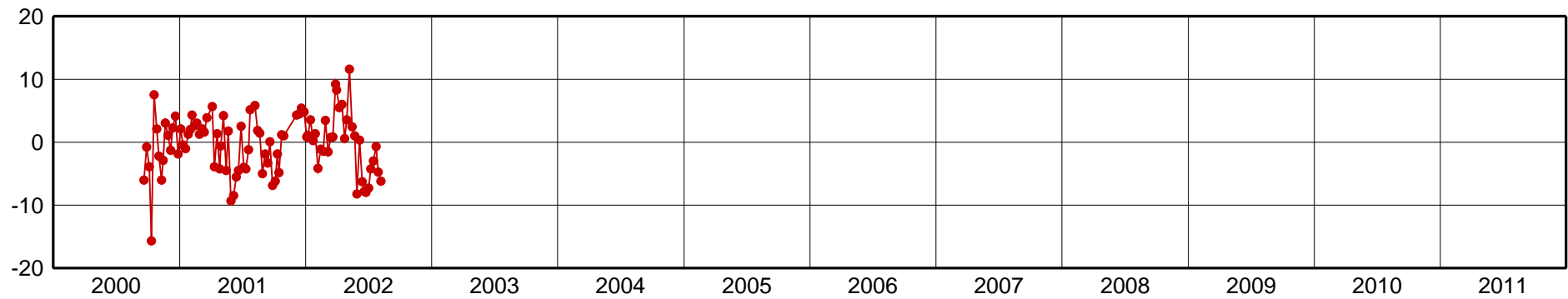
SLOR-Up Component [mm]
