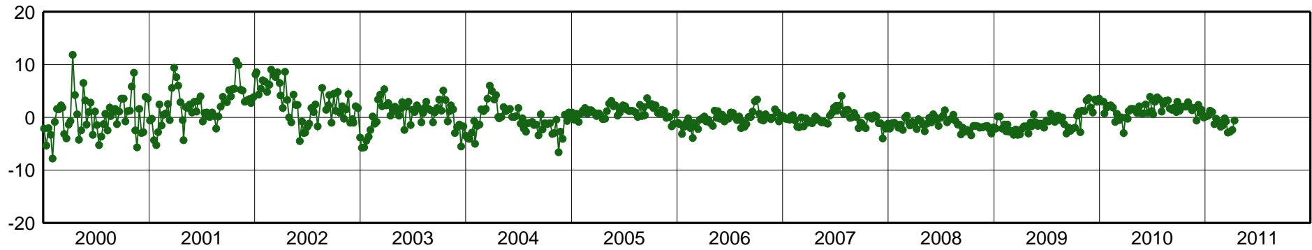
MDO1-East Component [mm]
