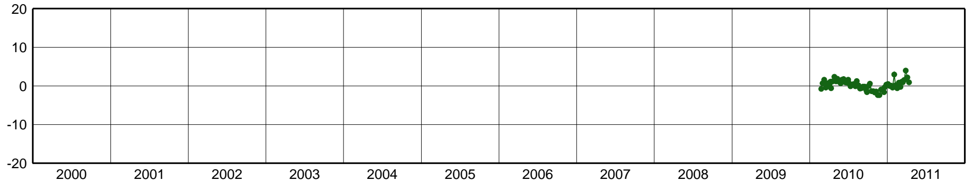
ABPD-East Component [mm]
