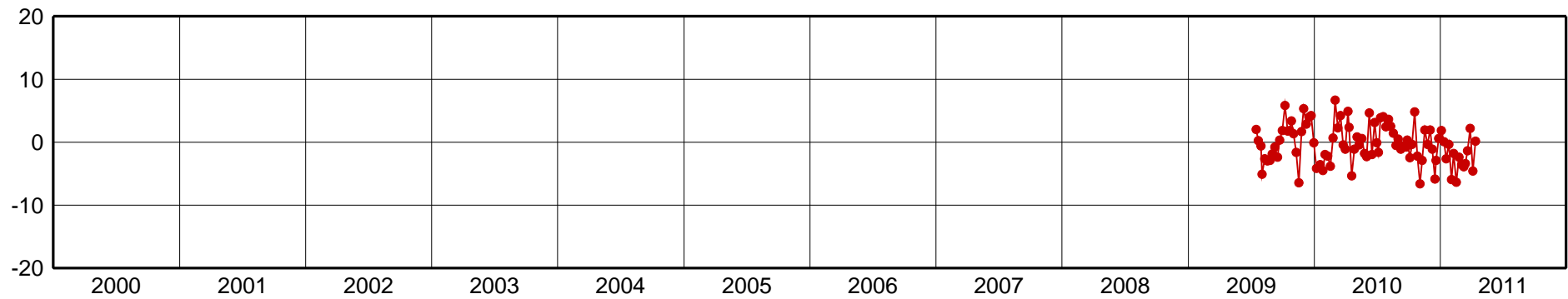
PISR-Up Component [mm]
