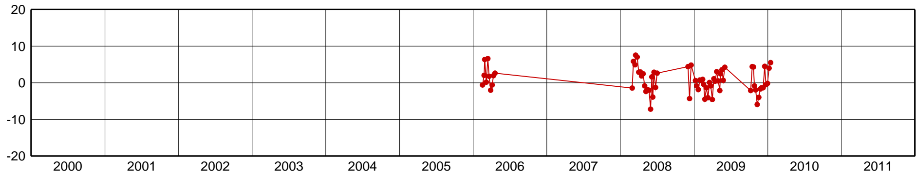
IBAG-Up Component [mm]
