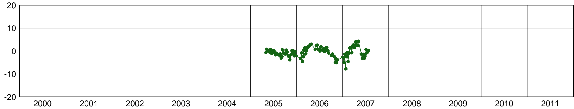
PDES-East Component [mm]
