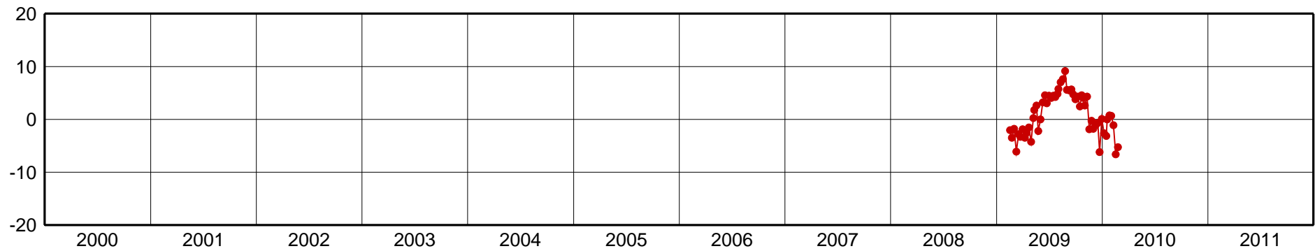
ALUM-Up Component [mm]
