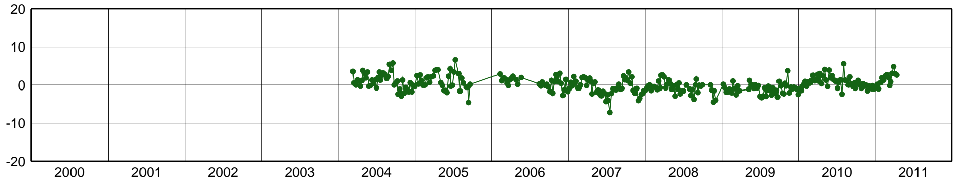
CUCU-East Component [mm]
