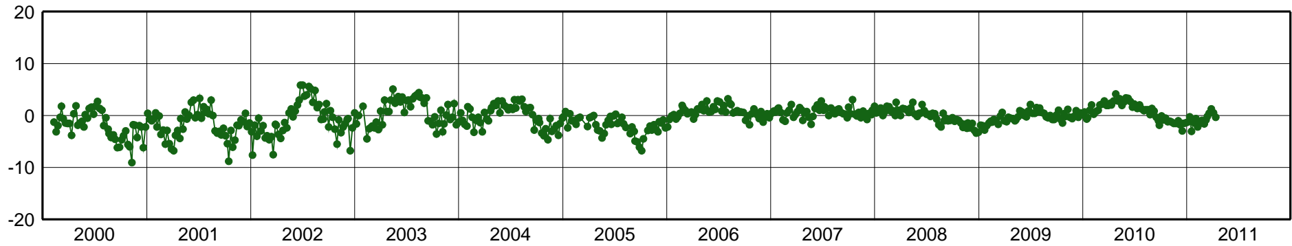
BOGA-East Component [mm]
