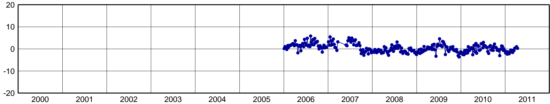
POVE-North Component [mm]
