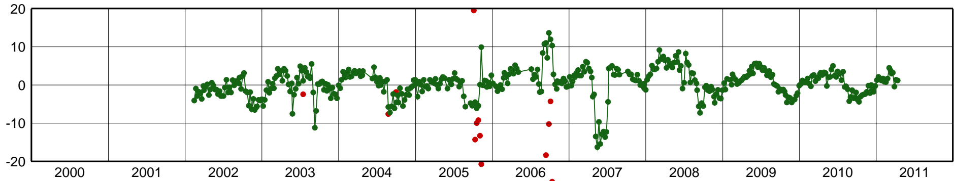
OH2-East Component [mm]
