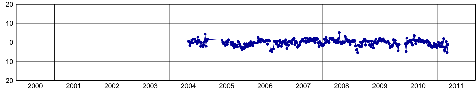
GVAL-North Component [mm]
