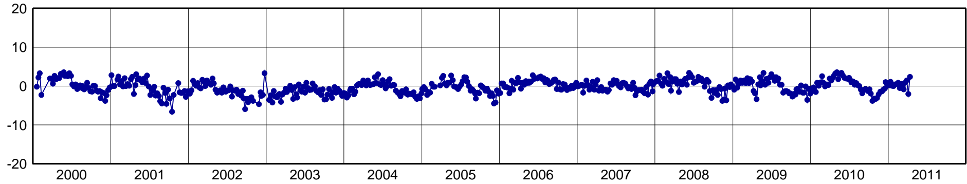
CUIB-North Component [mm]
