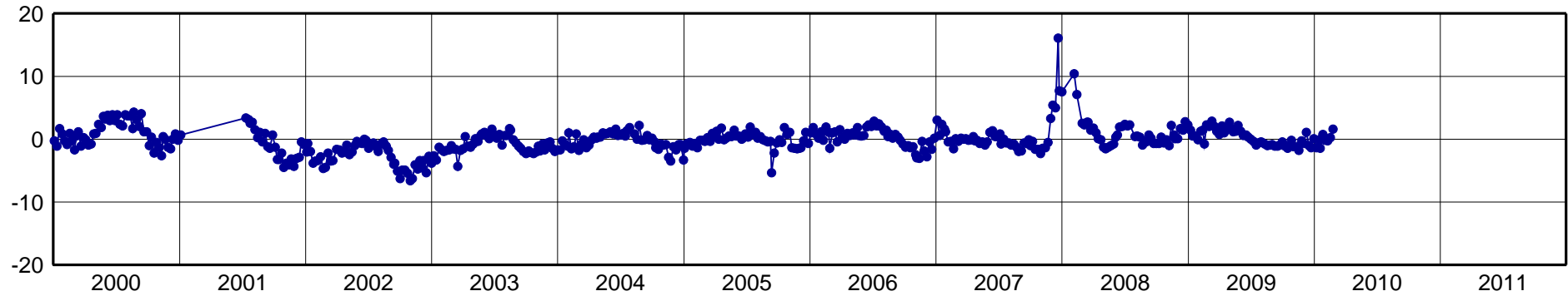
UNSA-North Component [mm]
