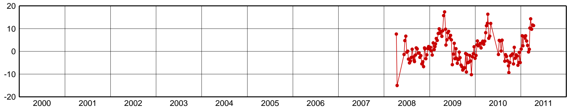
ALAR-Up Component [mm]
