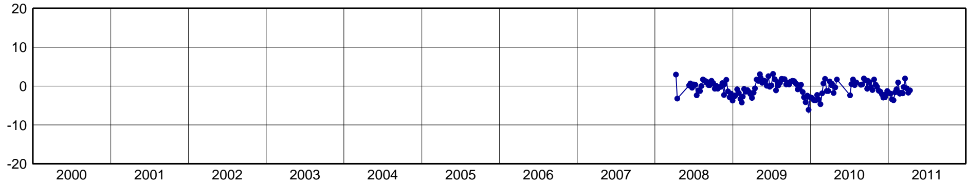
ALAR-North Component [mm]
