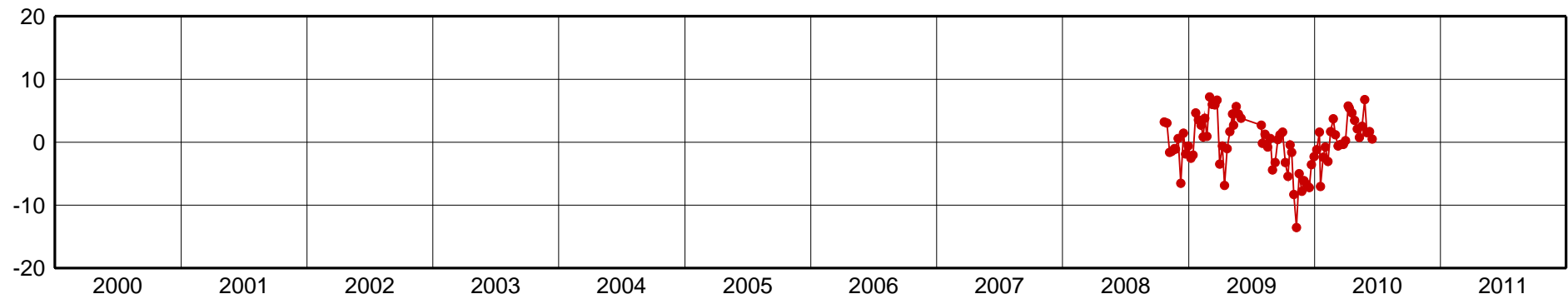
AZUE-Up Component [mm]
