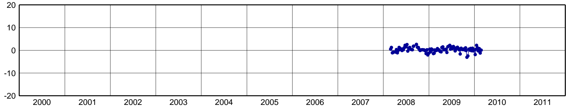
UYRO-North Component [mm]
