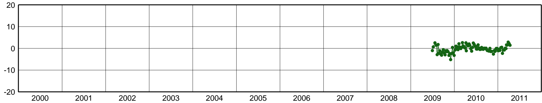
ESMR-East Component [mm]
