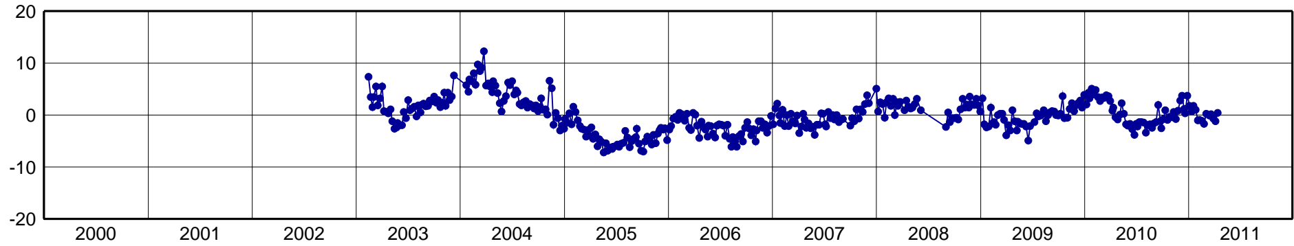
ETCG-North Component [mm]
