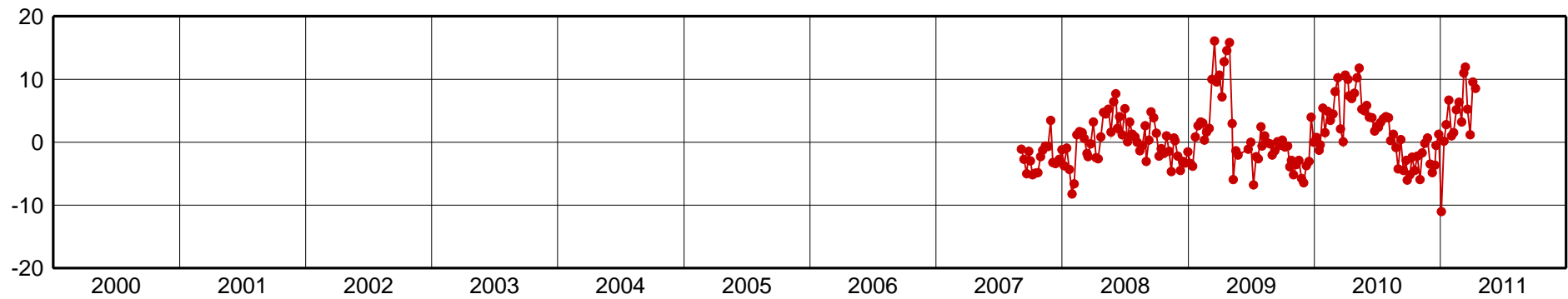
SSA1-Up Component [mm]
