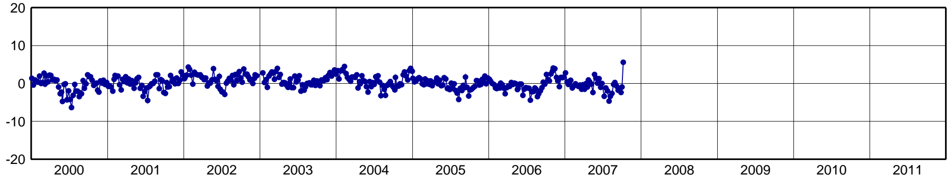
KYW1-North Component [mm]
