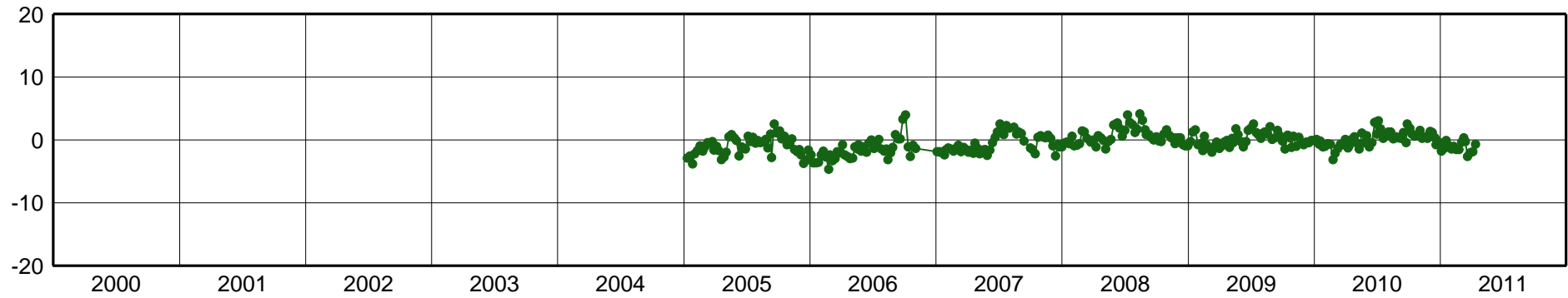
CHIH-East Component [mm]
