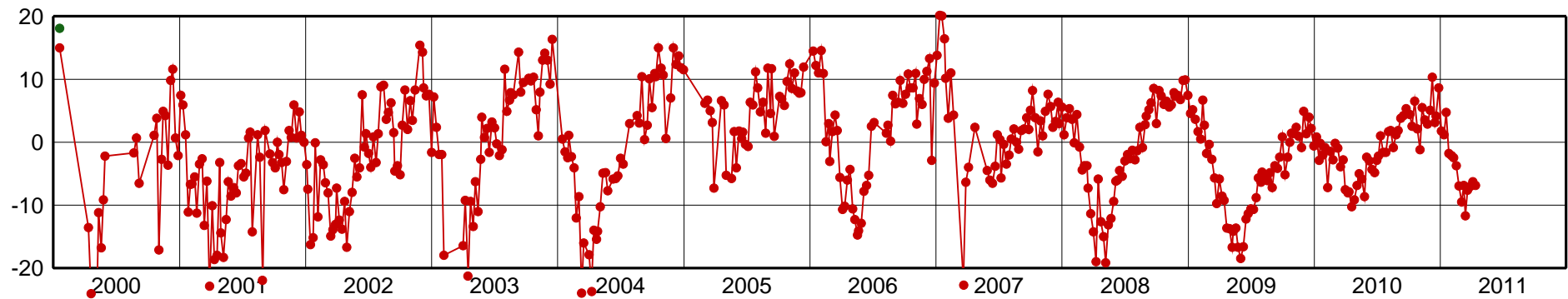
IMPZ-Up Component [mm]
