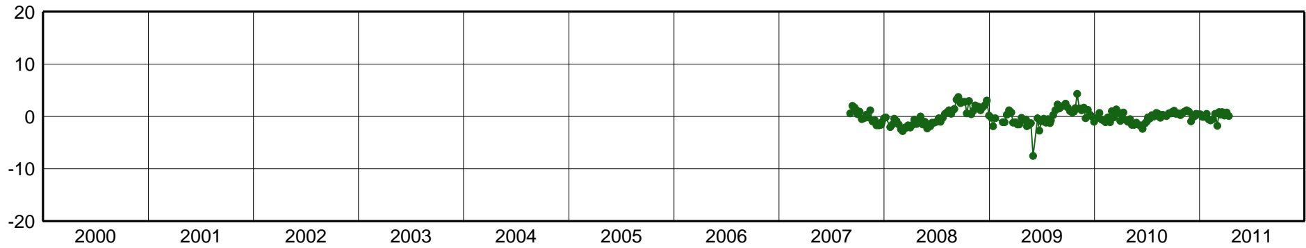
MABA-East Component [mm]
