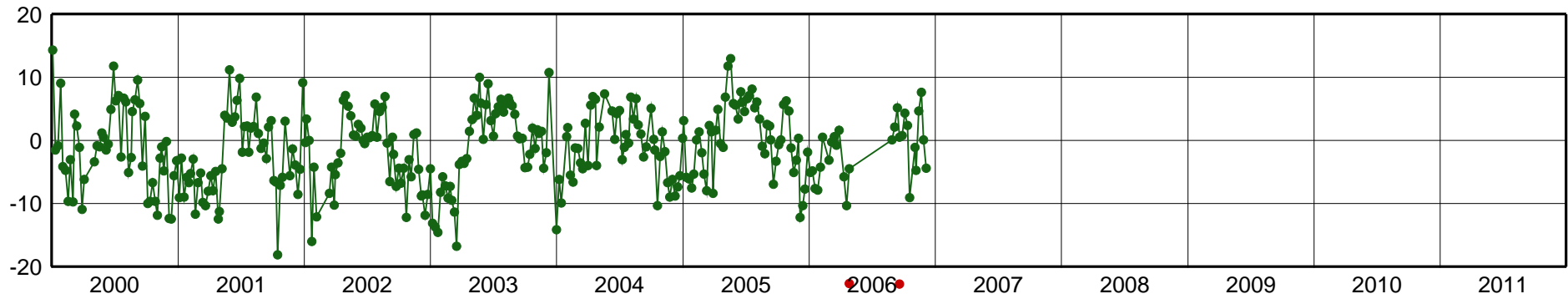
Goug-East Component [mm]
