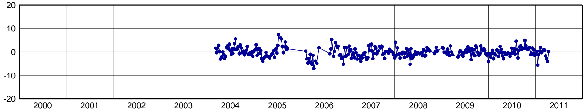
CUCU-North Component [mm]
