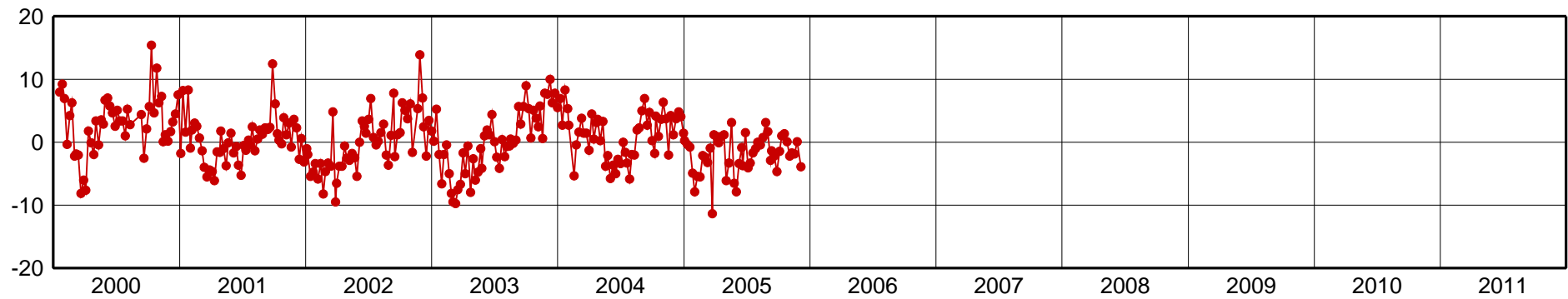
UEPP-Up Component [mm]
