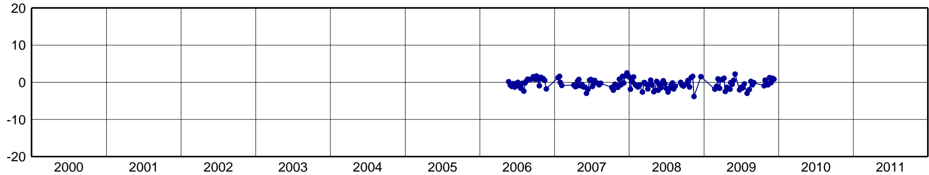
BANS-North Component [mm]
