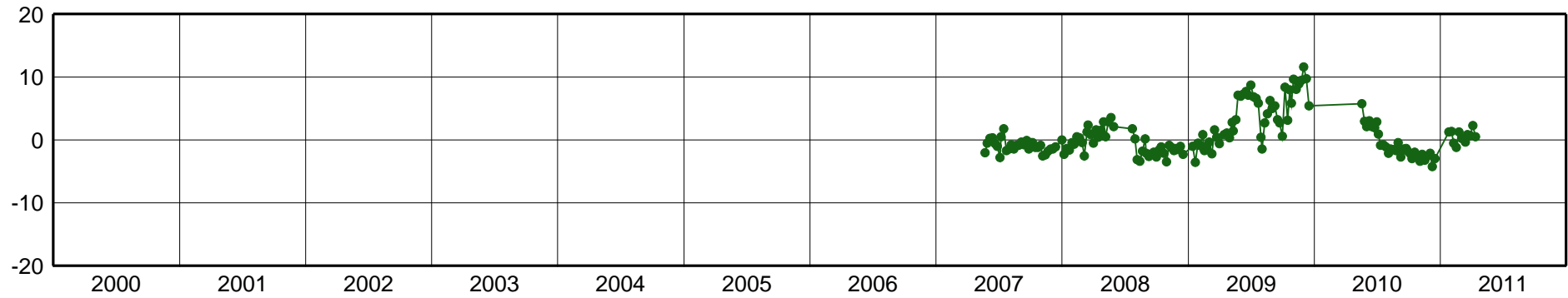
BERR-East Component [mm]
