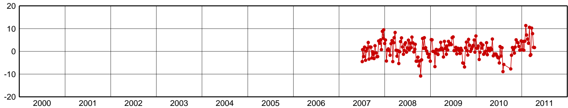
GRE0-Up Component [mm]
