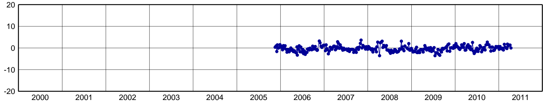
CBSB-North Component [mm]
