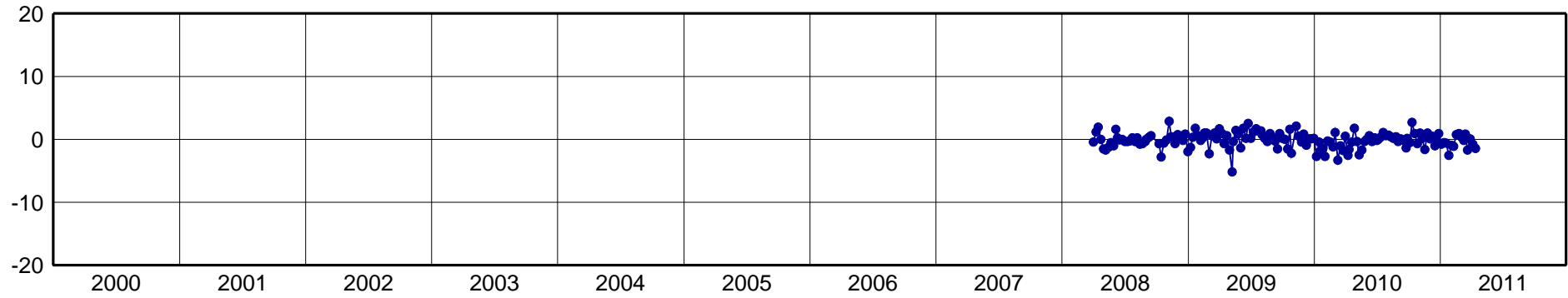
MTSF-North Component [mm]
