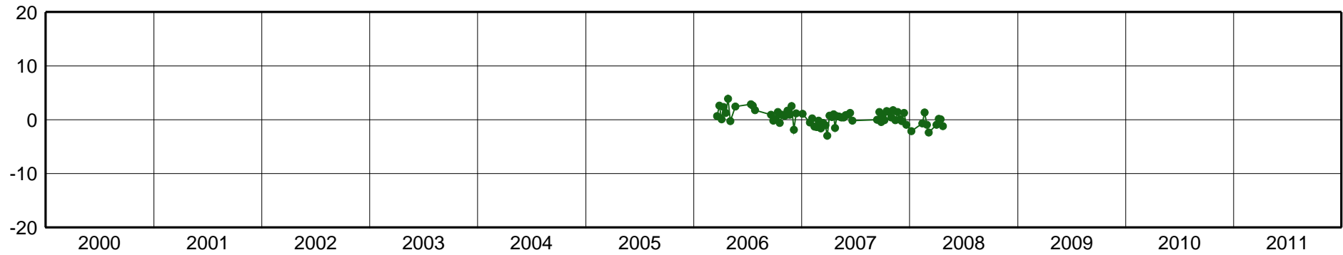
MOTE-East Component [mm]
