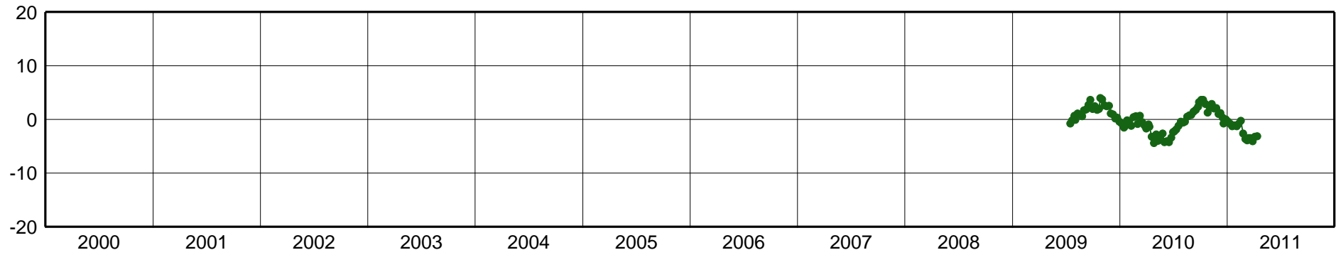
PISR-East Component [mm]
