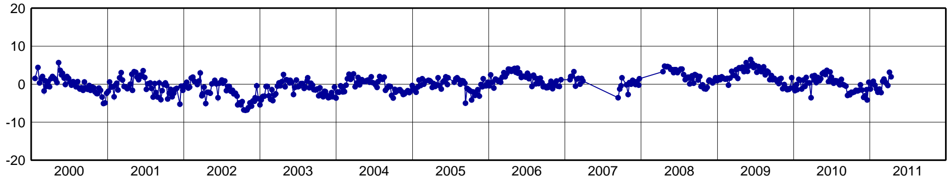
POAL-North Component [mm]
