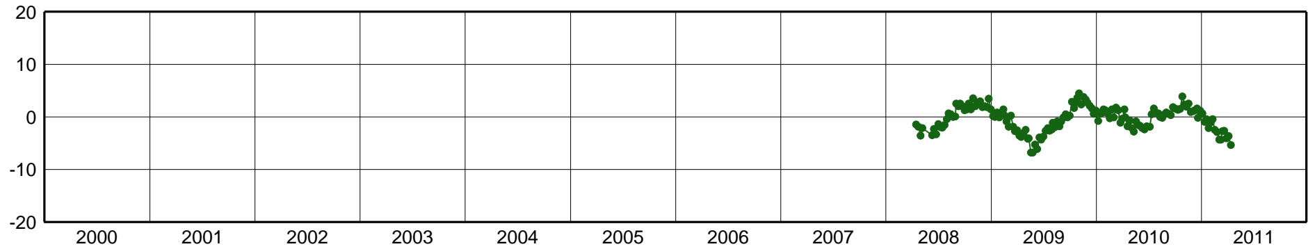
CEEU-East Component [mm]
