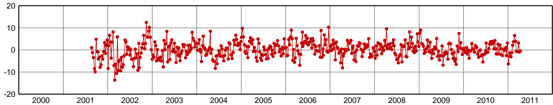
RIOD-Up Component [mm]
