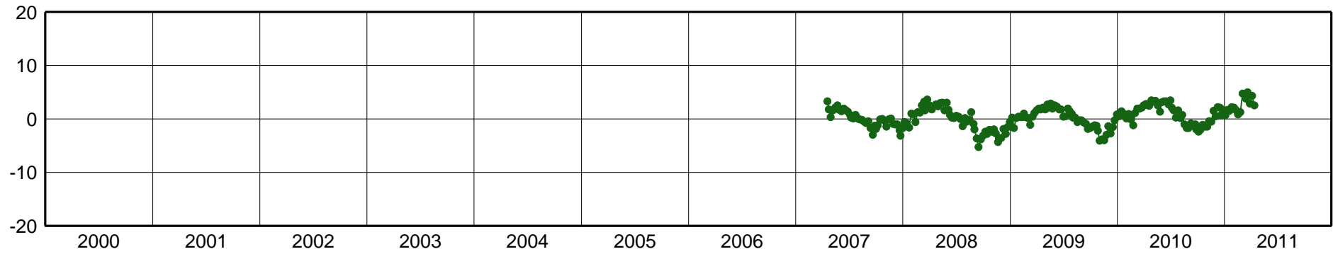
RIO2-East Component [mm]
