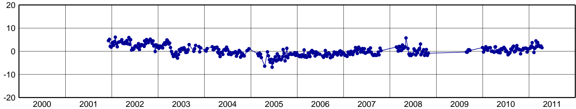
ELEN-North Component [mm]
