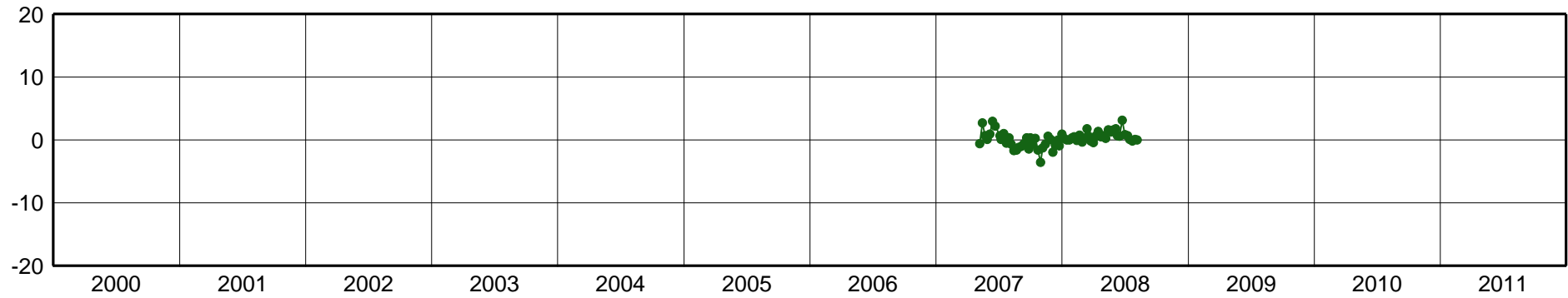
ANDS-East Component [mm]
