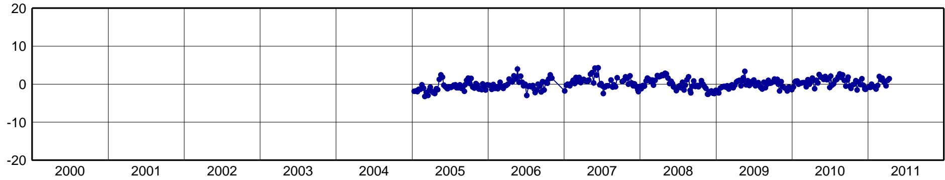
VIL2-North Component [mm]
