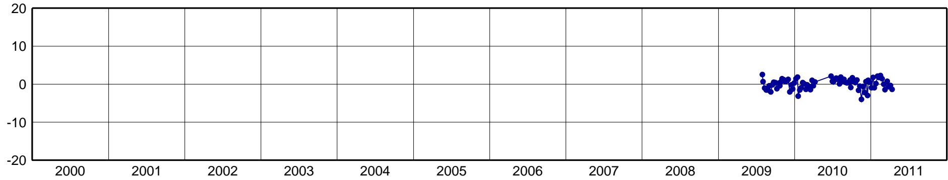
CALL-North Component [mm]
