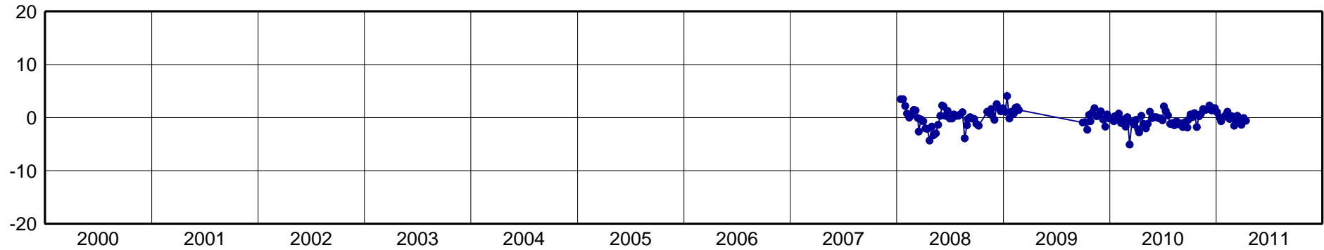
ROGM-North Component [mm]
