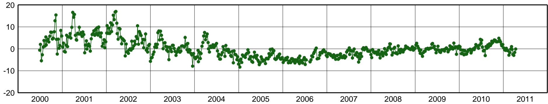
GOLD-East Component [mm]
