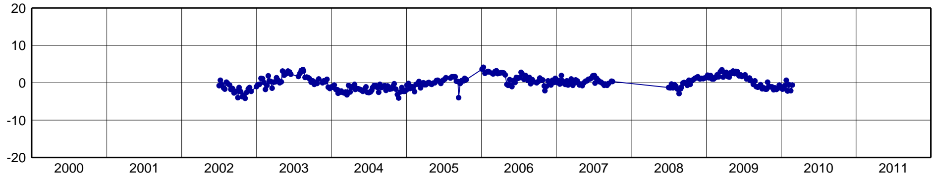
COPO-North Component [mm]
