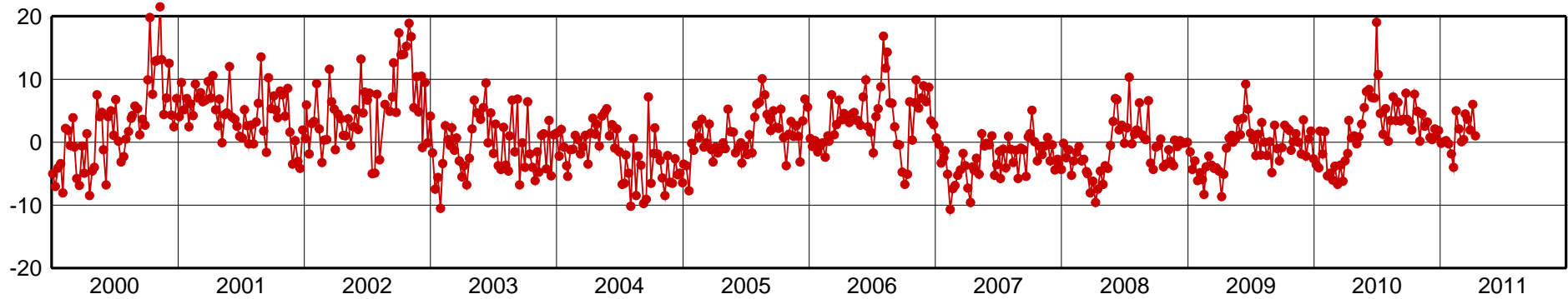
MDO1-Up Component [mm]
