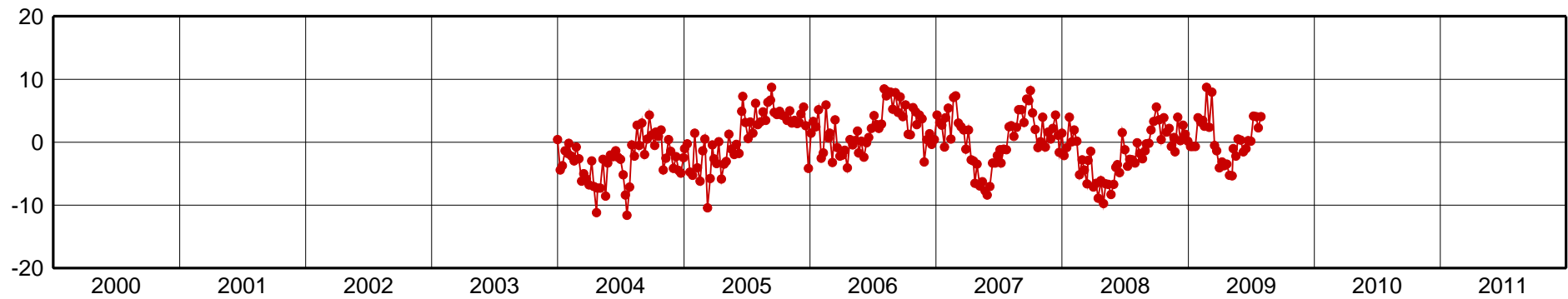
QUI1-Up Component [mm]
