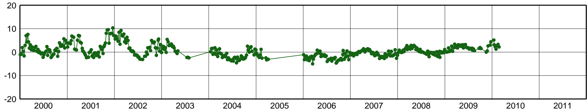
CFAG-East Component [mm]
