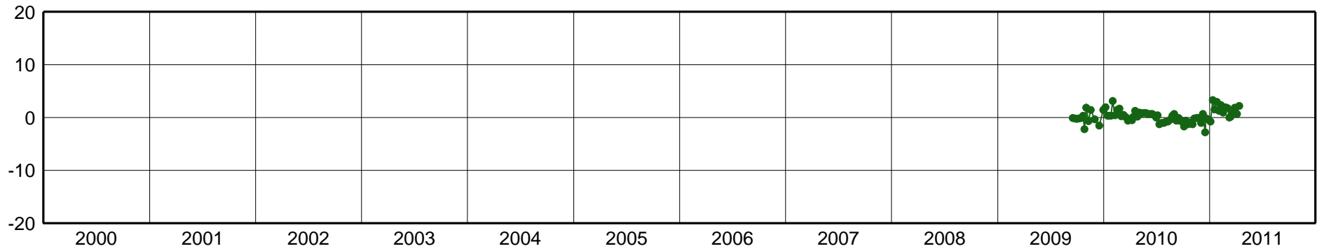
ROSA-East Component [mm]
