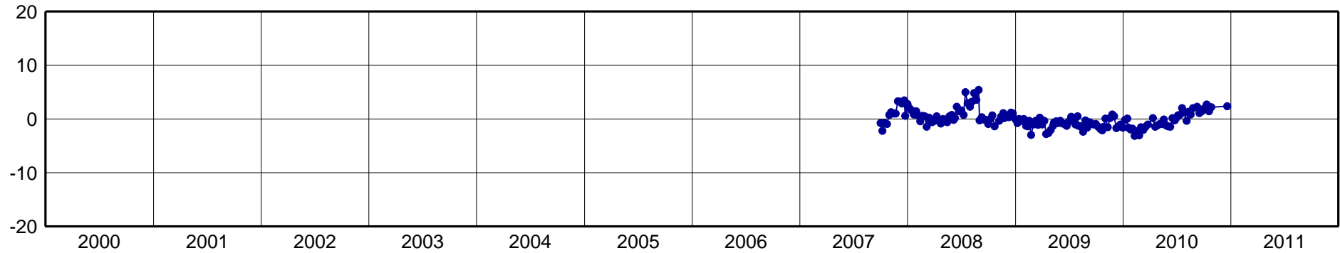
FQNE-North Component [mm]
