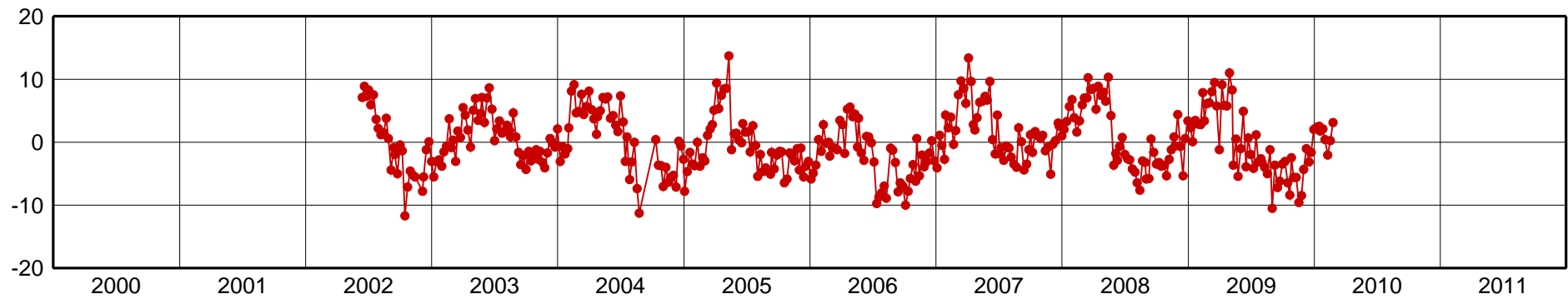
CONZ-Up Component [mm]
