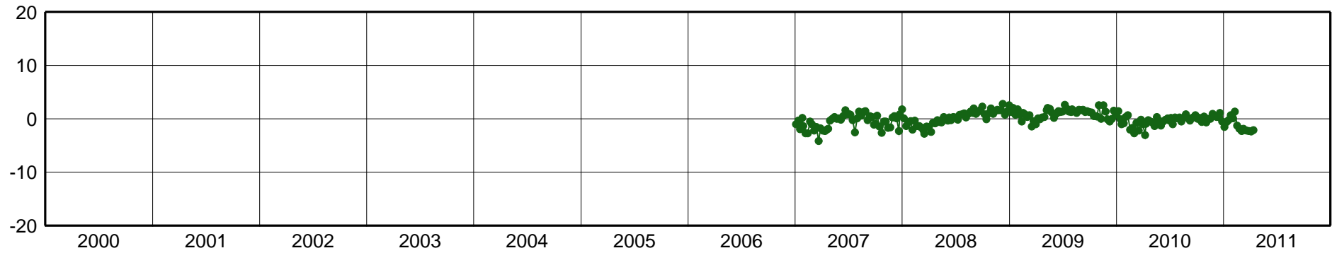
POLI-East Component [mm]
