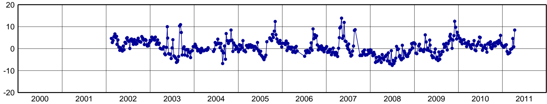
OH2-North Component [mm]
