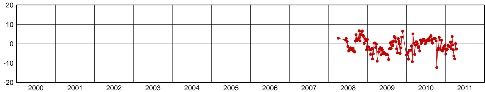
MGMC-Up Component [mm]
