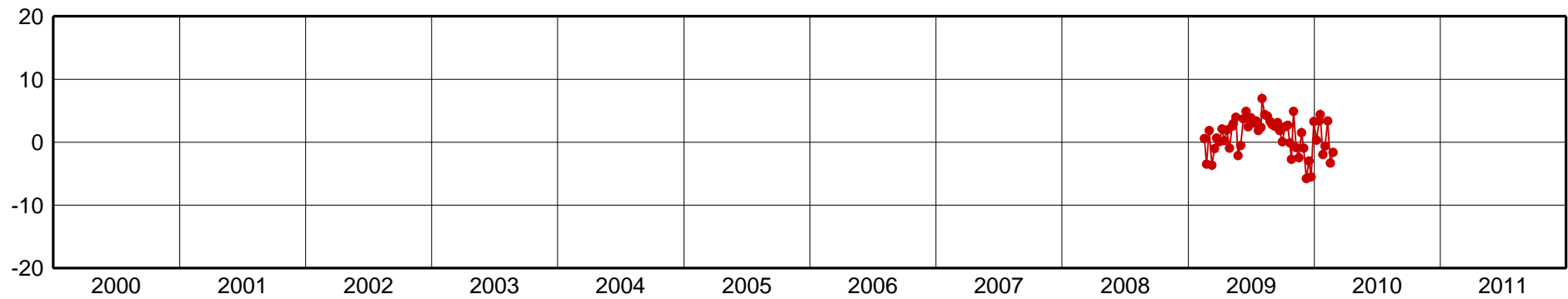
CATA-Up Component [mm]
