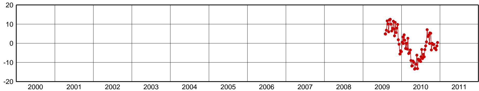
IQUI-Up Component [mm]
