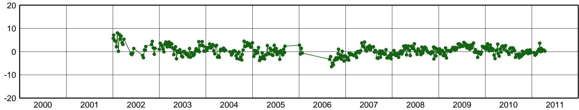
TUCU-East Component [mm]
