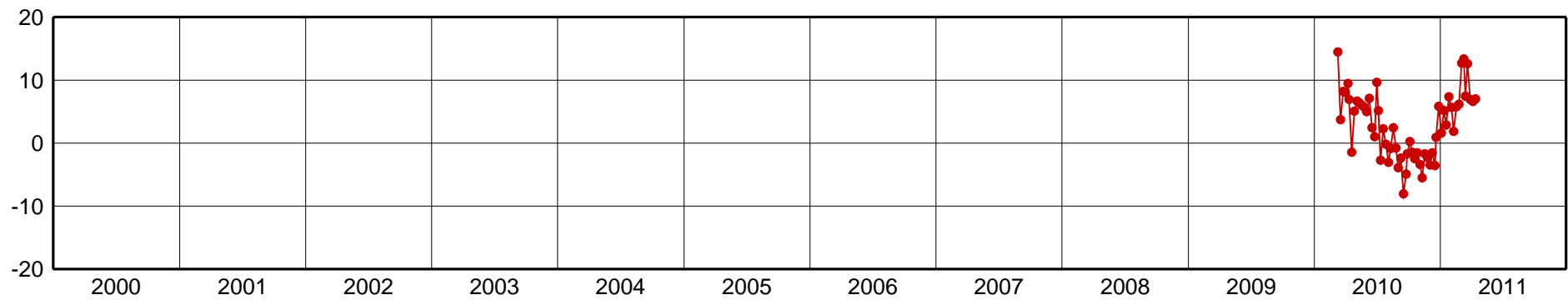
MPL2-Up Component [mm]
