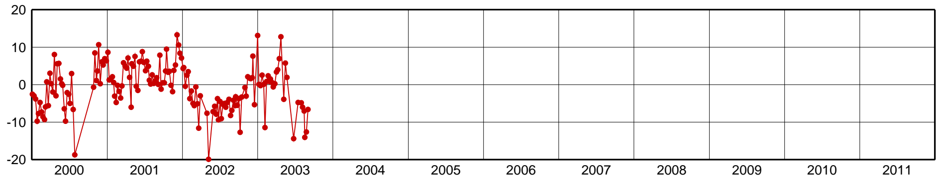
JAMA-Up Component [mm]
