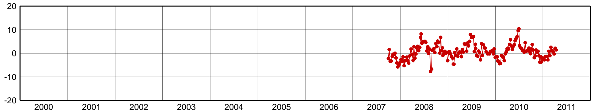
CULC-Up Component [mm]
