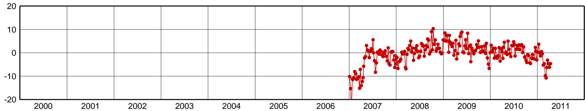
POLI-Up Component [mm]
