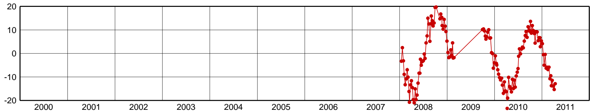
ROGM-Up Component [mm]
