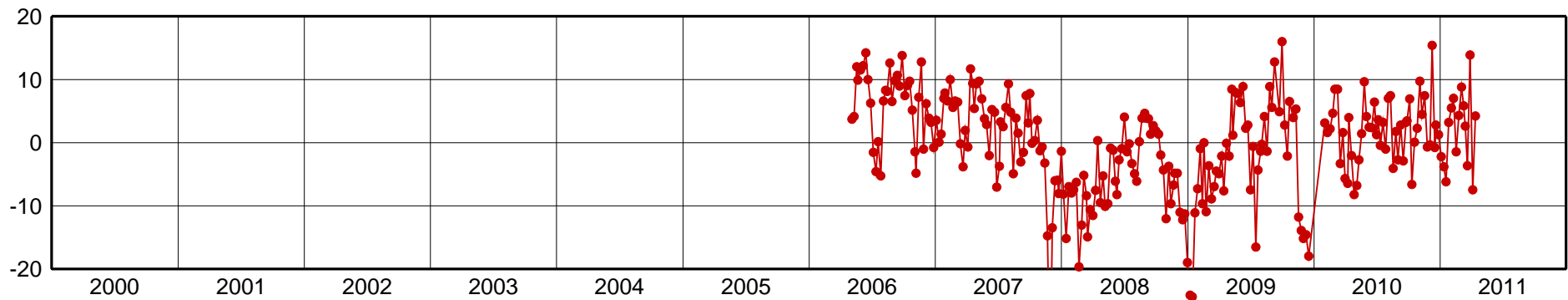
SAMA-Up Component [mm]
