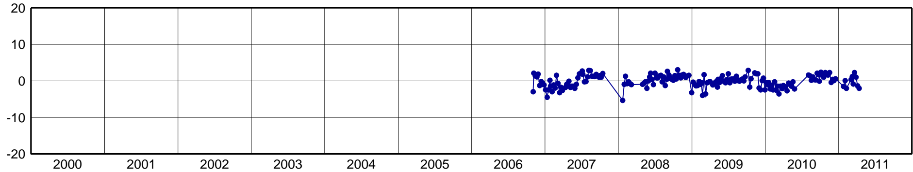
FLOR-North Component [mm]
