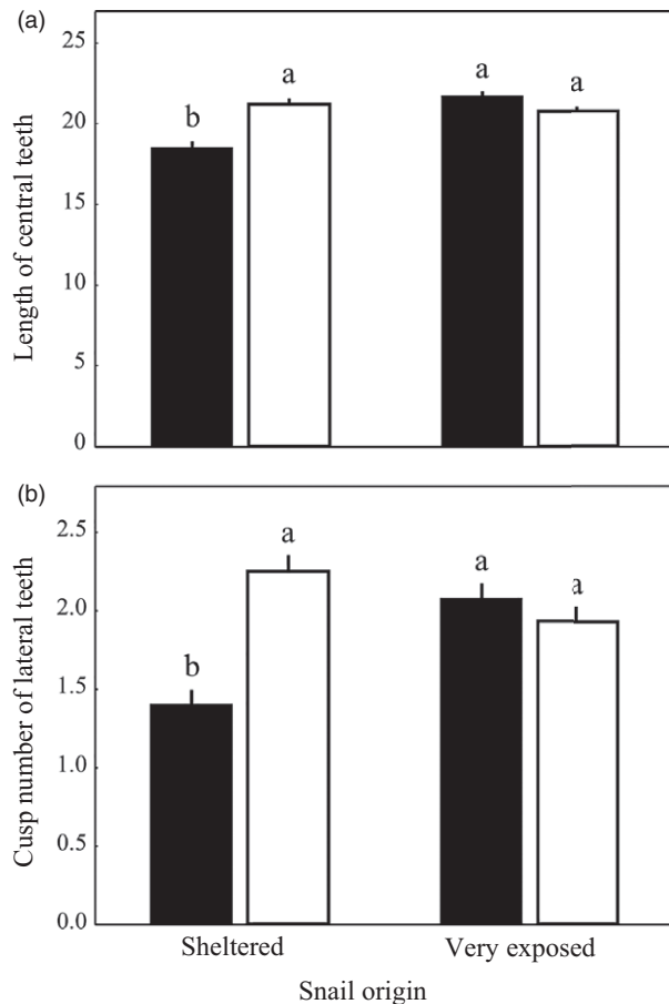
Fig. 4. (a) Length of central teeth (in \mu\text{m} ) and (b) number of cusps in lateral teeth (mean + SE) of radulae in Littorina obtusata fed Fucus vesiculosus from sheltered (black bars) or exposed (white bars) habitats in Nova Scotia. Treatments sharing the same letter did not differ significantly from one another.
