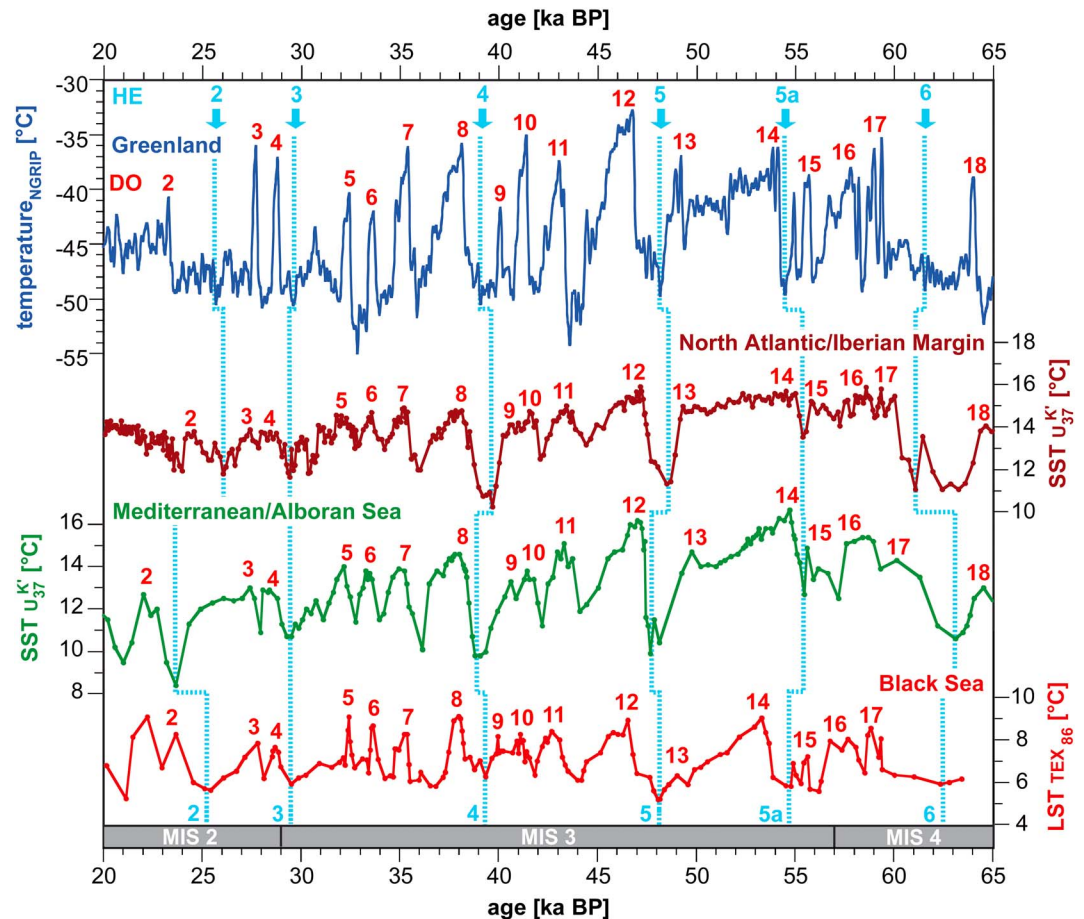
Figure 2. Temperature variability in the North Atlantic and Europe during the last glacial (65–20 ka). Greenland temperature [Kindler et al. , 2014] (NGRIP), alkenone-based sea surface temperature (SST) from the North Atlantic/Iberian Margin [Martrat et al. , 2007] (core MD01-2444) and from the western Mediterranean Sea/Alboran Sea [Martrat et al. , 2004] (Ocean Drilling Program (ODP) Site 977A) are shown together with the TEX 86 -based lake surface temperature (LST) from the southeastern Black Sea (core 25GC-1, this study). Red numbers denote DO interstadials, blue numbers HE.
