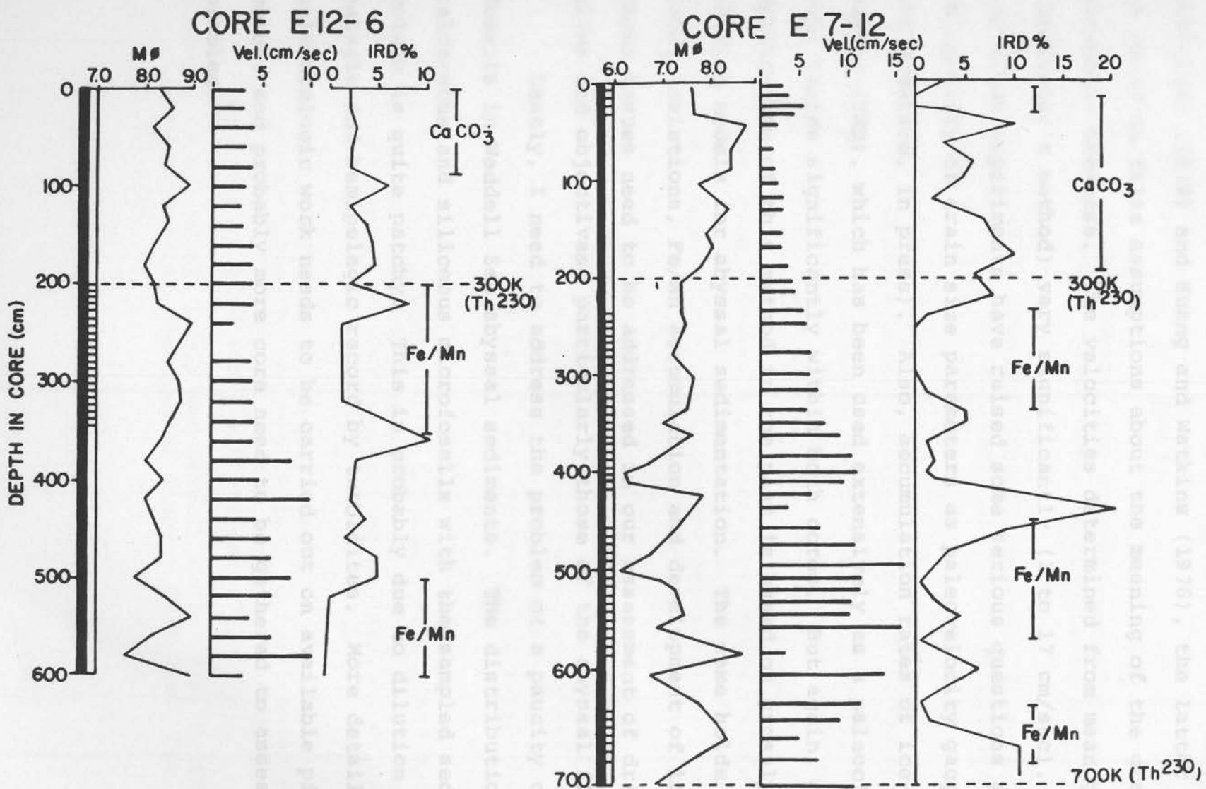
Figure 42. Example of variations in grain size, calcium carbonate content, and Fe/Mn micronodule content in Weddell Sea abyssal cores.
