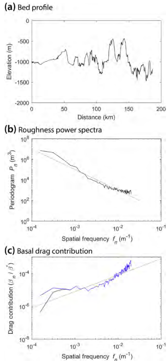
Figure 6. (a) Bed elevation (equal to water depth for sea-floor data) versus distance along flow line. (b) Roughness power spectra P_n versus spatial frequency f_n . (c) Scaled basal drag contributions \beta_n/\beta^* versus f_n for along-flow profile (6) offshore from Pine Island and Thwaites glaciers (for location see Fig. S5a). The red lines in (b) and (c) are based on an assumption of Brown-noise power spectrum that falls off as the inverse square of spatial frequency. At low spatial frequencies, drag contributions depend on the function F (see Sect. 4.2) with the two limiting cases shown: F_1 (blue), F_2 (black).
