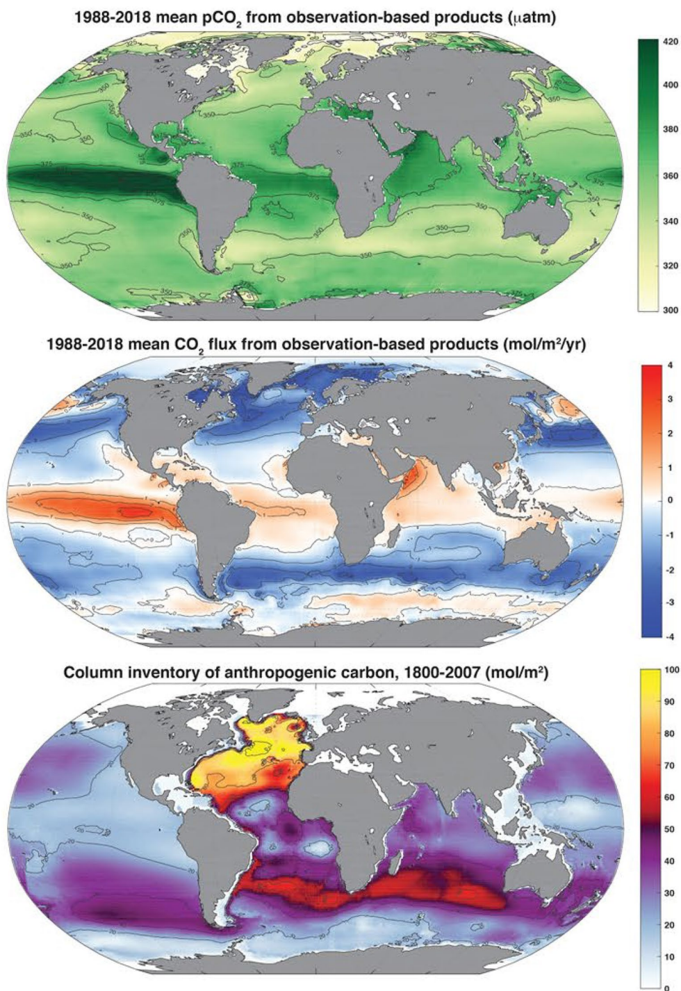
Figure 7. Surface ocean p\text{CO}_2 (top); and air-sea \text{CO}_2 flux ( F_{\text{net}} ), positive flux to the atmosphere (middle), 1988–2018, mean of 6 observation-based products (Fay et al., 2021); column inventory of anthropogenic carbon ( C_{\text{ant}} , bottom), 1800–2007 (Gruber, Clement, et al., 2019; Sabine et al., 2004).
