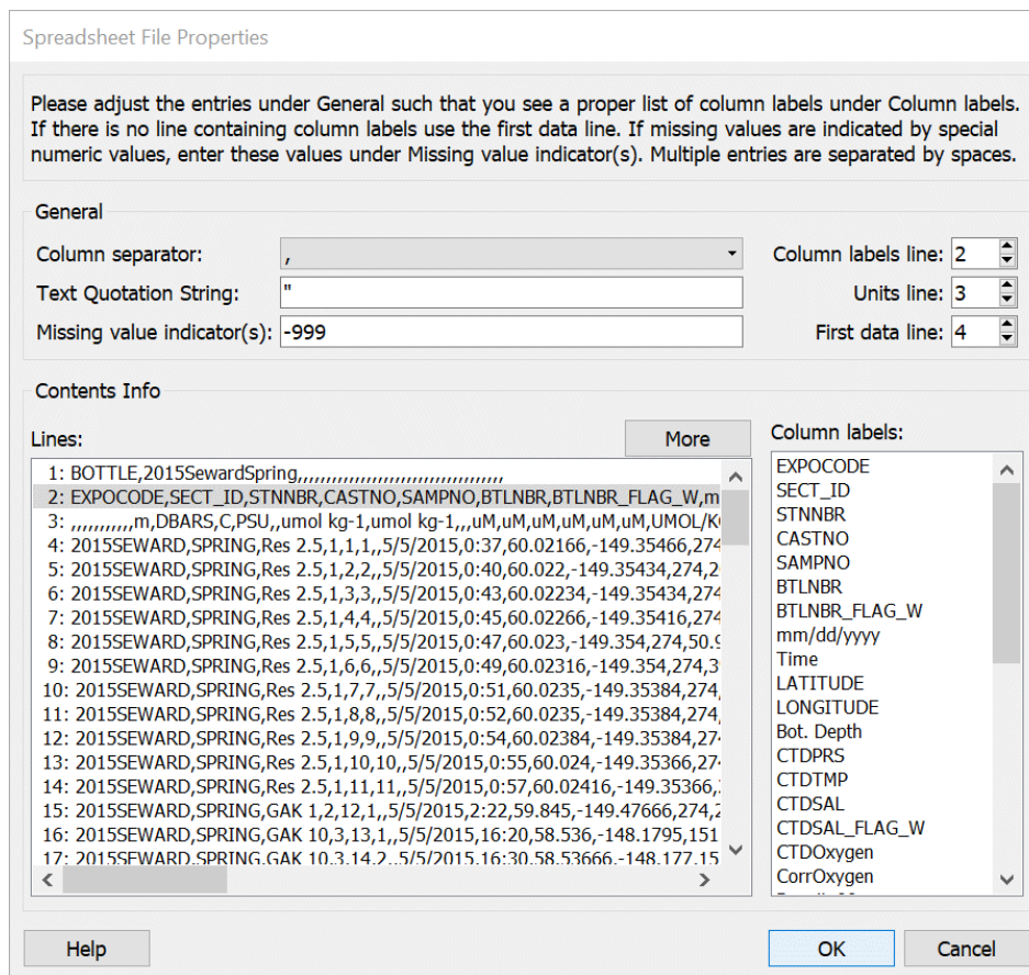
Figure 4-1: The spreadsheet file properties dialog.
