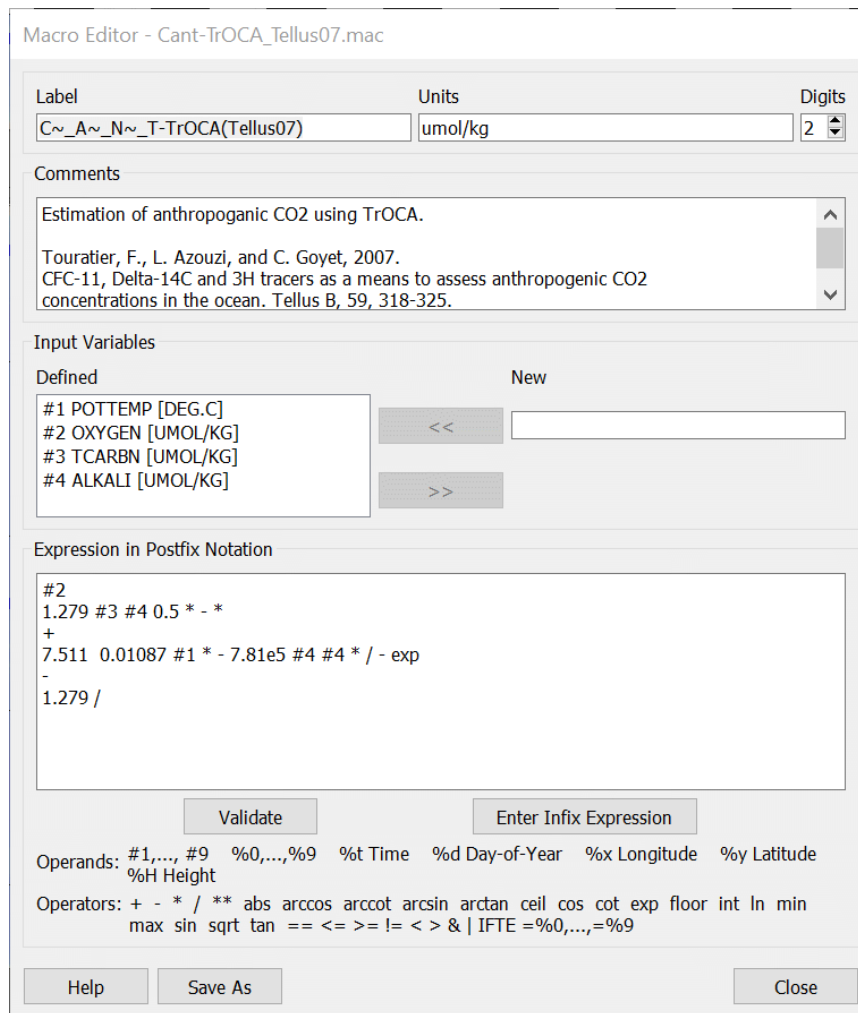
Figure 6-3: The macro editor dialog
