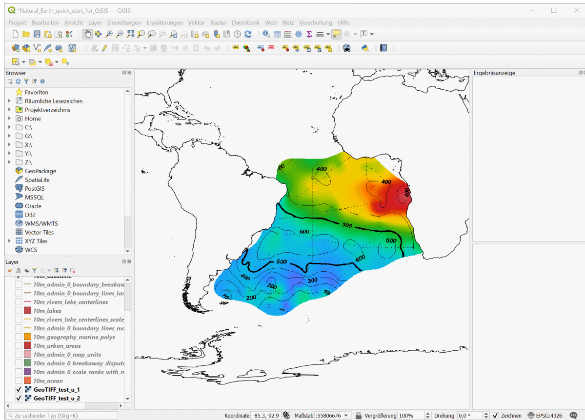
Figure 1-8: GIS example showing depth contours of the \sigma_0=27.0 isopycnal on top of color-coded phosphorus concentrations on the same isopycnal.
