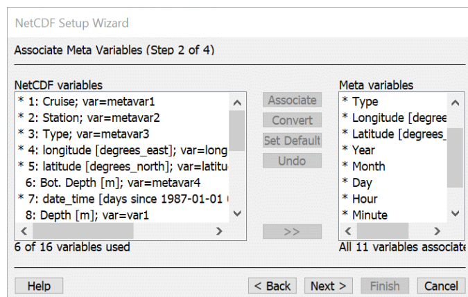
Figure 13-2: The netCDF setup wizard (step 2 of 4)
