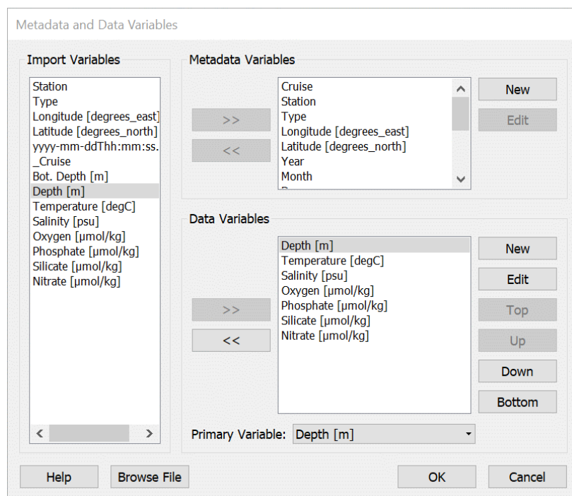
Figure 3-2: The Metadata and Data Variables dialog.
