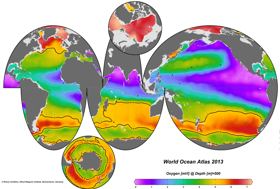
Figure 1-9: Oxygen distribution on the 500 m depth isosurface shown as interrupted map. Interrupted maps are produced via the "Save As Interrupted Map" option of the plot's context menu.
