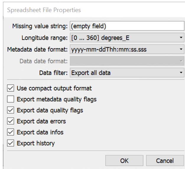
Figure 5-1: Spreadsheet File Properties dialog.
