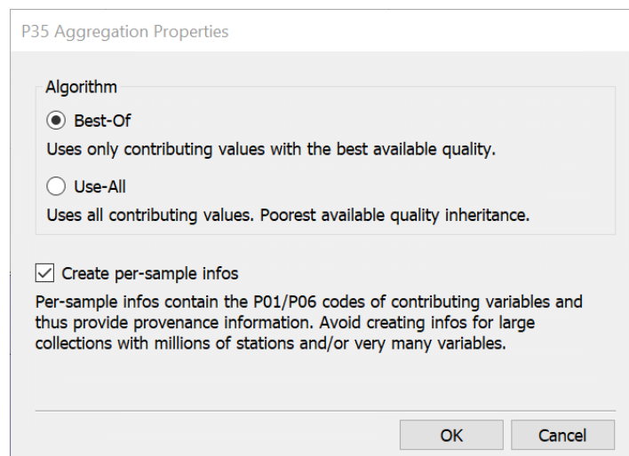
Figure 5-2: The P35 Aggregation Properties dialog.
