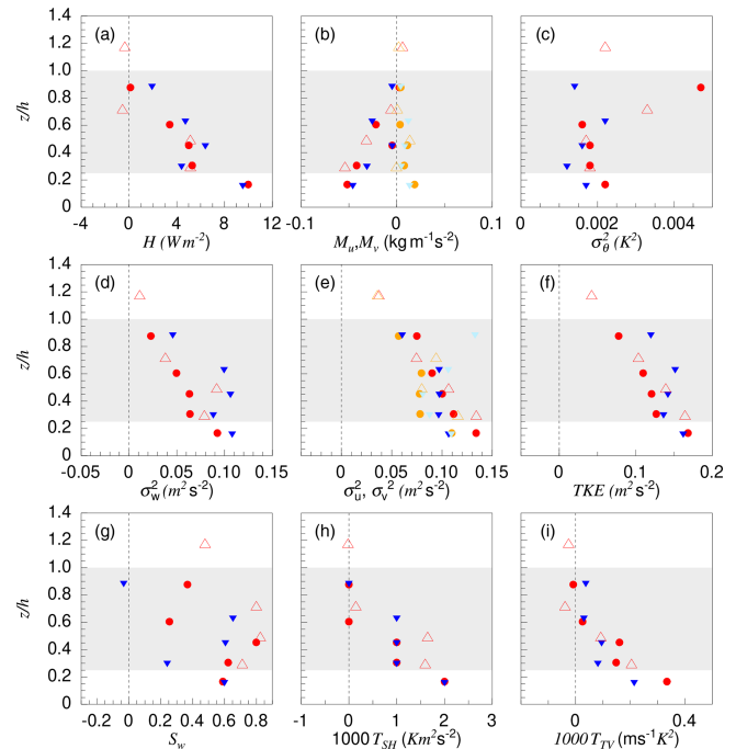
Figure 10. Turbulence statistics based on horizontal flight legs of 14 June 2017 obtained from Polar 5 (closed symbols) and Polar 6 (open symbols). Results of Polar 5 refer to the two northernmost dashed blue legs shown in Fig. 8. The Polar 6 result refers to its northernmost flight leg (red in Fig. 8). Altitude is normalized by the cloud-top height, h = 400 \text{ m} . The bright symbols (light blue and orange) refer to M_v and \sigma_v^2 , while the dark (red and blue) symbols in the corresponding panels refer to M_u and \sigma_u^2 .
