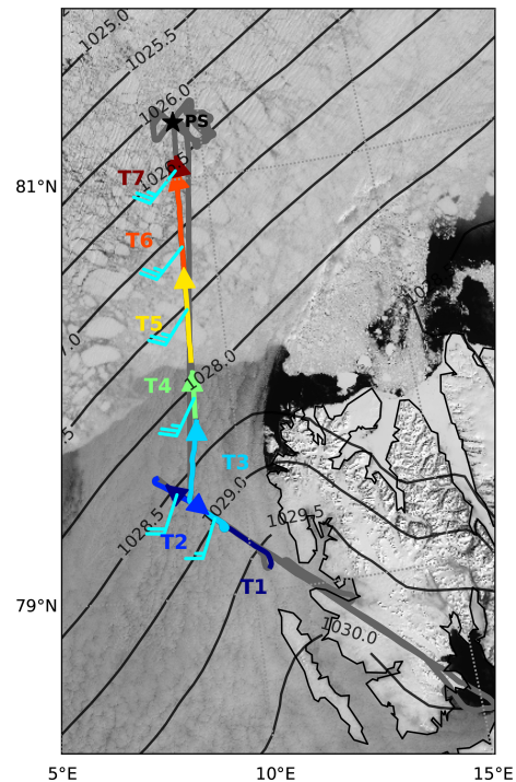
Figure 5. Polar 6 flight track on 2 June 2017 overlaid on the MODIS satellite image. T1–T7 represent descents and ascents of the aircraft. The wind barbs are showing the wind speed and direction averaged over the profile segments within the ABL. Isobars represent the mean sea level pressure field based on the ERA5 re-analysis.
