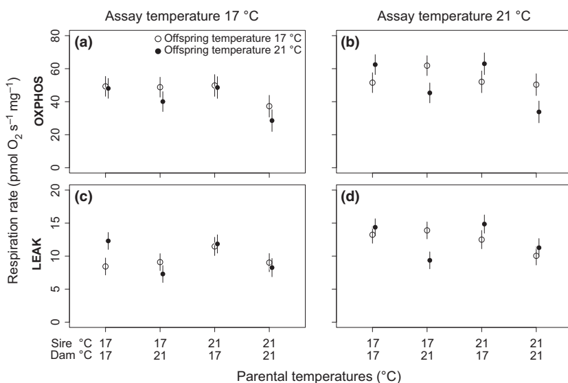
Fig. 3. Offspring respiration rates (pmol O 2 s -1 mg -1 ) measured as OXPPOS assayed at (a) 17 °C and (b) 21 °C, and LEAK assayed at (c) 17 °C and (d) 21 °C for each parental temperature combination. Offspring reared at 17 °C are shown as open circles and offspring reared at 21 °C as closed circles. Parental temperature combinations are shown as male (sire) temperature (upper × axis) and female (dam) temperature (lower × axis). Points depict least square means (±SE) for all families within a temperature combination group.
