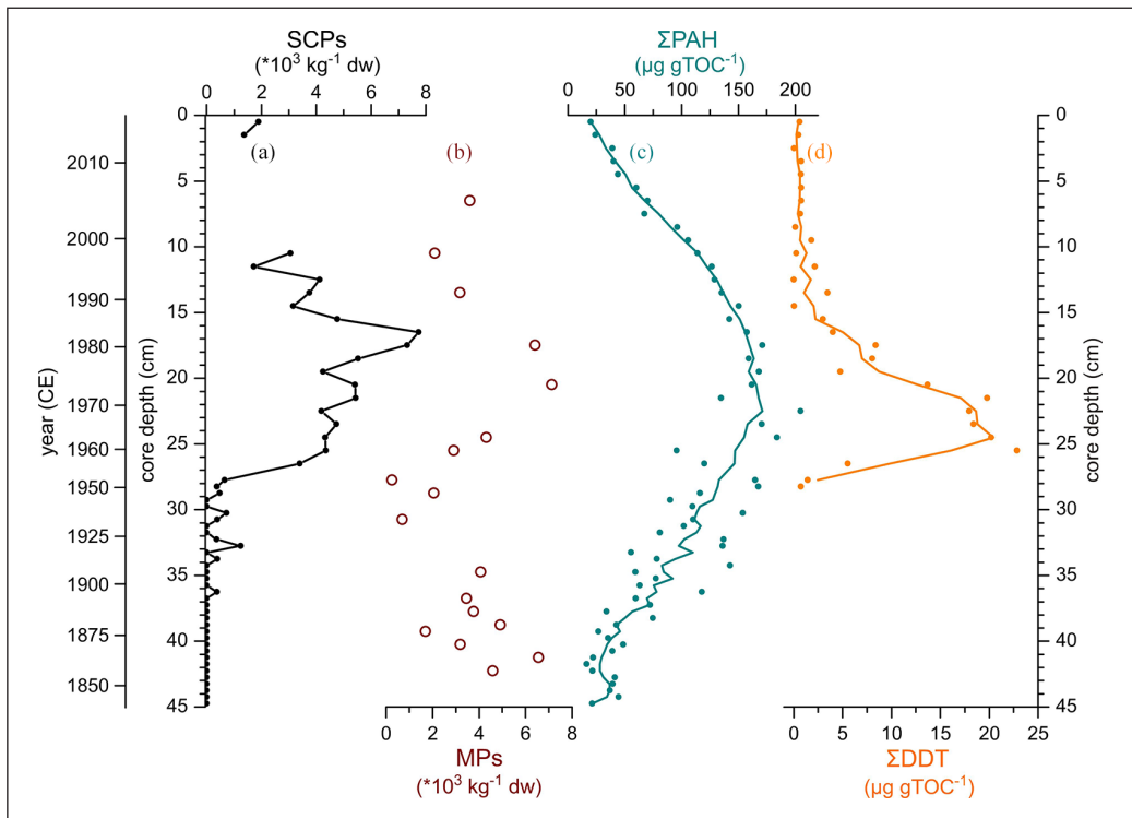
Figure 4. Depth profiles of SCPs (a), microplastics (b), \Sigma PAH (c) and \Sigma DDT (d) contents in core EMB201/7-4. Reproduced in colour in online version.
