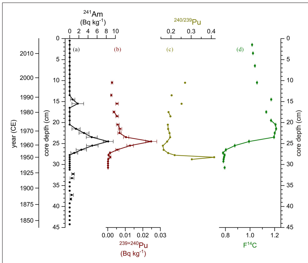
Figure 3. Depth profiles of ^{241}\text{Am} (a) and ^{239+240}\text{Pu} (b) activities, ^{240/239}\text{Pu} (c), and F^{14}\text{C} (d) in core EMB201/7-4. Reproduced in colour in online version.
