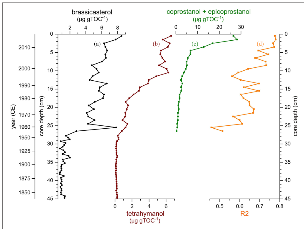
Figure 7. Depth profiles of brassicasterol (a) and tetrahymanol (b) contents, the sum of coprostanol and epicoprostanol contents (c), and the faecal stanol-based R2 ratio (d) in core EMB201/7-4. Reproduced in colour in online version.
