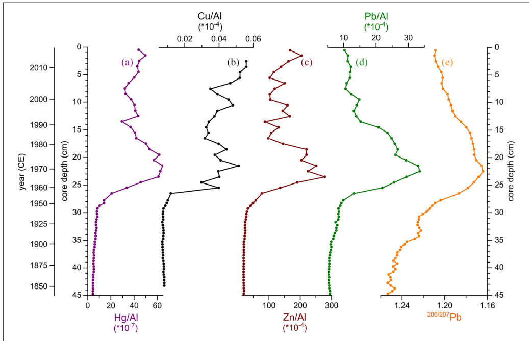
Figure 6. Depth profiles of Hg/Al (a), Cu/Al (b), Zn/Al (c), Pb/Al (d) and ^{206}/^{207}\text{Pb} (e) reversed plotted in core EMB201/7-4. Reproduced in colour in online version.
