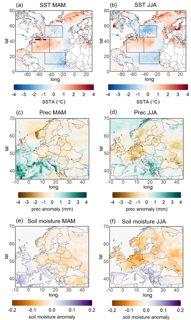
Figure 7. Anomalies of sea surface temperature (SST; a, b ), precipitation ( c, d ), and soil moisture ( e, f ) in the ERA5 reanalysis (compared to the reference period 1981–2010) for spring (March to May, MAM; a, c, e ) and summer (June to August, JJA; b, d, f ) months. Boxes in ( a ) and ( b ) indicate the regions for the tripolar SST pattern.
