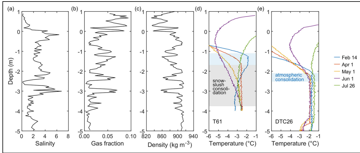
Figure 2. Ice physical parameters and temperatures for Alli's Ridge. (a) Measured sea-ice salinity, (b) estimated relative gas fraction and (c) estimated sea-ice density from in situ measurements of ice salinity from ice coring from July 15 and temperature from ice mass balance buoy DTC26, and measurements of sea-ice density for laboratory temperature of -15^{\circ}\text{C} for the Eastern transect at x = 5.5 m. Vertical ridge temperature profiles from ice mass balance buoys (d) T61 and (e) DTC26 for various dates. Blue-shaded and grey-shaded areas represent atmospheric and snow-slush modes, respectively, of the ridge consolidation.
