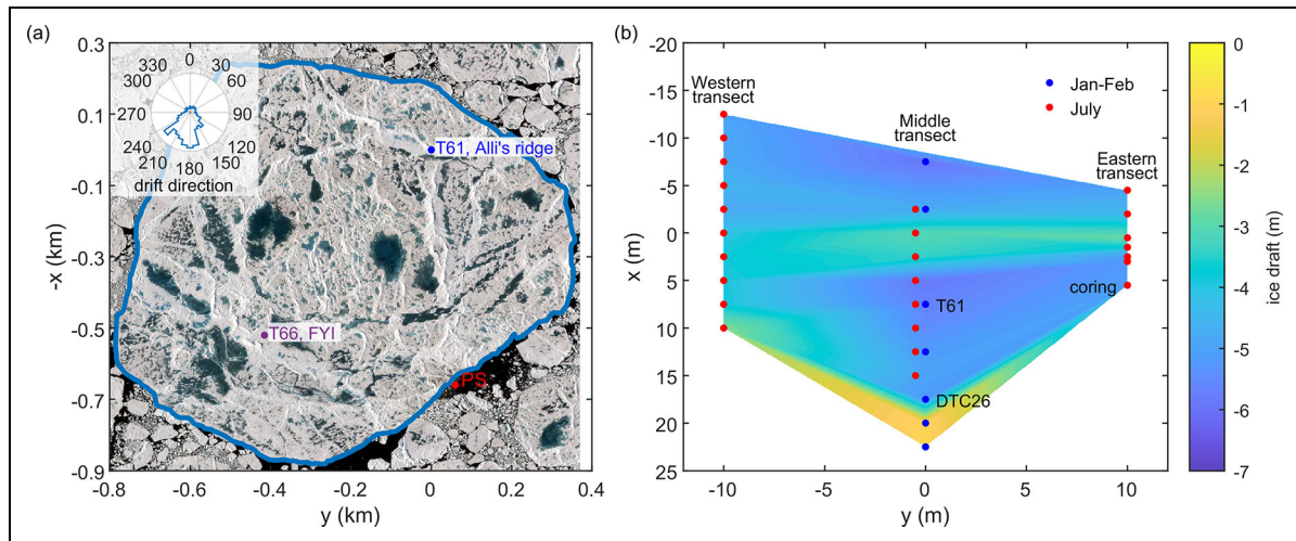
Figure 1. Location of Alli's Ridge, ice mass balance buoys, and drilling transects in MOSAiC Central Observatory. (a) Location of SIMBA ice mass balance buoys 2020T61 (T61, blue dot), 2019T66 (T66, purple dot) and Polarstern (PS, red dot) within the Central Observatory outline (blue line). The background is the satellite image of the ice floe on July 1 from Planet Labs. The polar histogram shows the frequency of ice drift direction in relation to the displayed ice floe orientation, with prevailing drift in the South direction ( 174^\circ ; Schmithüsen, 2021). (b) Location of ice drilling at Alli's Ridge with a contour plot of the keel depth (combined drilling data from winter and summer).
