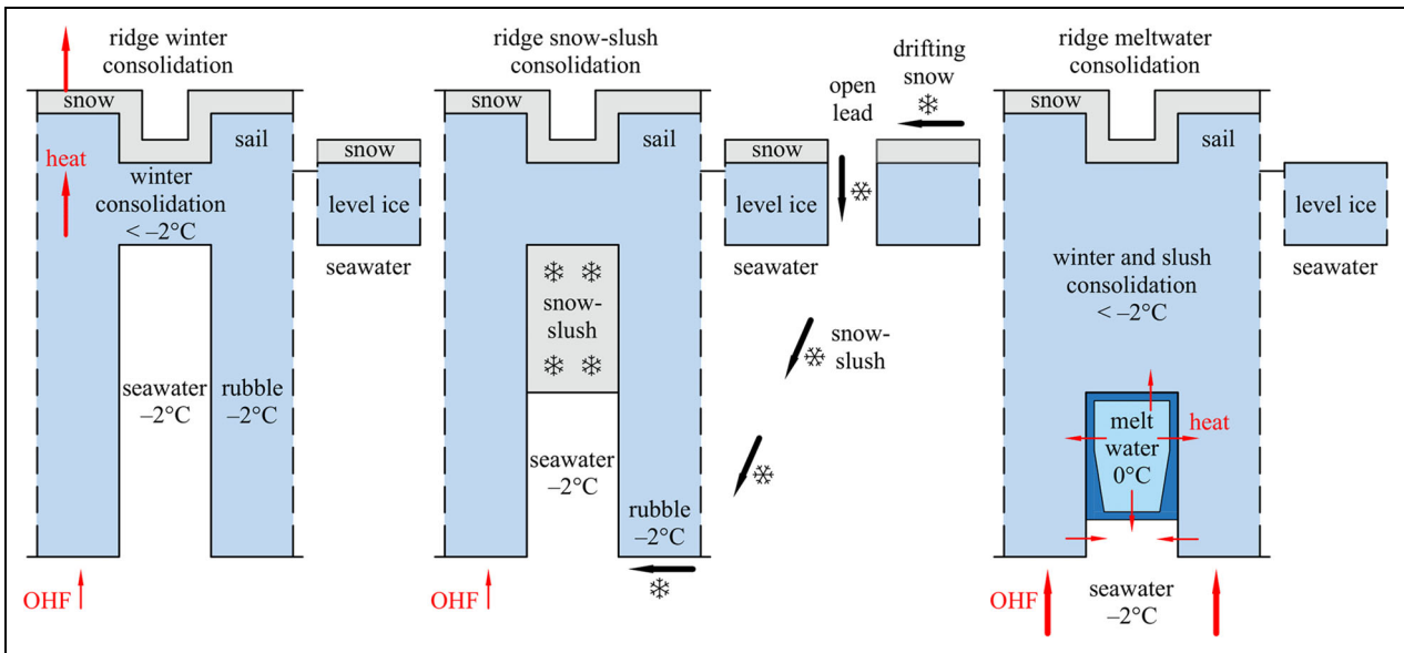
Figure 8. Mechanisms of ridge consolidation. Schematic of different consolidation mechanisms for first-year ridges observed during MOSAiC and associated heat fluxes resulting in consolidation. Each of the three illustrations represents a unit void in a sea-ice ridge, surrounded by two ice blocks. Blue-shaded areas are associated with sea ice grown via atmospheric cooling, grey-shaded areas are associated with snow and snow-slush, and cyan and dark-blue shaded areas are associated with fresher meltwater and refrozen meltwater. The red arrows represent the heat fluxes including the ocean heat flux (OHF), while the black arrows represent snow-slush mass transfer.
