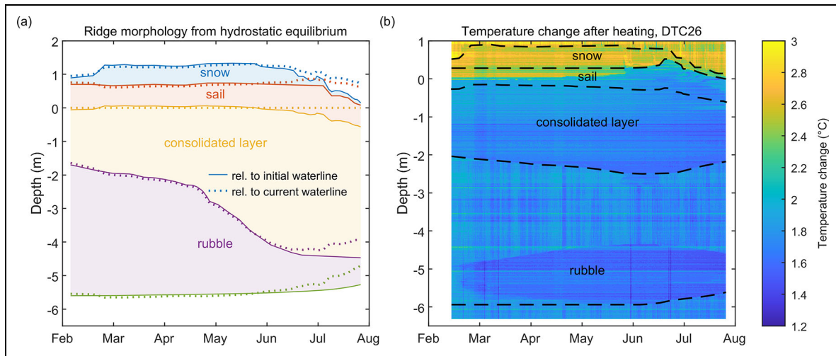
Figure 5. Ridge interface thickness and draft evolution. (a) Evolution of interfaces of snow, sail, consolidated layer, and rubble estimated using hydrostatic equilibrium for the average morphology of Alli's Ridge. The interfaces relative to the initial waterline are shown as solid lines and interface drafts (relative to current waterline) are shown as dotted lines. (b) Contour plot of the temperature change after heating, with estimated interfaces of snow, sail, consolidated layer, and rubble for the ice mass balance buoy DTC26.
