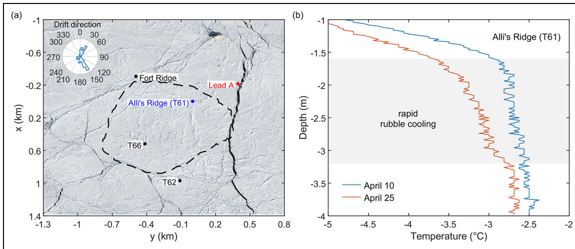
Figure 7. Location of ridges and leads during warming event in April and rubble cooling. (a) Location of Alli's Ridge, Fort Ridge, Lead A, T66 and T62 buoys within the Central Observatory outline on July 1 (black-dashed line) with the background of the aerial image of the ice floe from April 23. The polar histogram shows the frequency of ice drift direction in relation to the displayed ice floe orientation during April 15–23. (b) Vertical ridge temperature profiles from T61 before and after the warming event in April. Grey-shaded area represents the region of rapid cooling of ice rubble.
