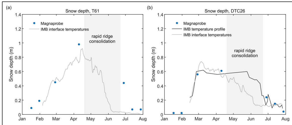
Figure 4. Snow depth estimates from the two ice mass balance buoys T61 and DTC26. (a) Snow depth for T61 was estimated only from interface temperatures (grey line) due to insufficient thermistor string length. (b) Snow depth for DTC26 was estimated from the temperature profile (black line) by locating the depth with the largest temperature gradient change and from air-snow, snow-ice, and ice-water interface temperatures (grey line). Snow depth estimates from interface temperatures were smoothed using a running average filter with 15-day window. Grey-shaded areas represent the period of rapid ridge consolidation.
