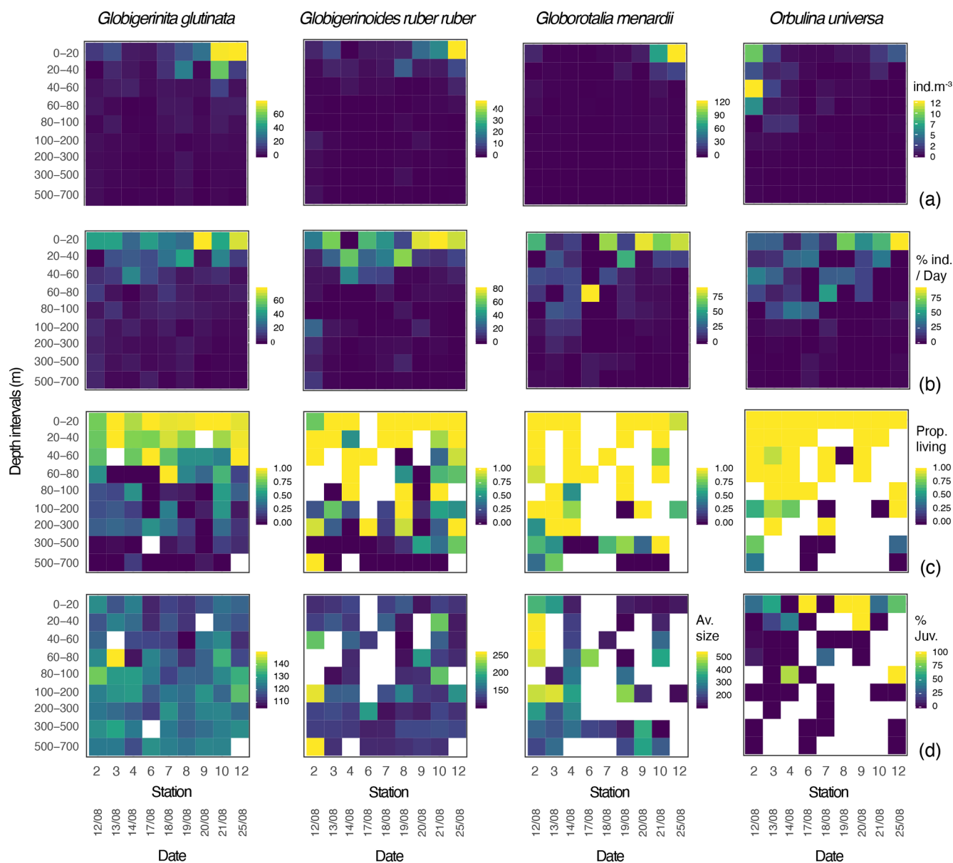
Figure 3. Globigerinita glutinata , Globigerinoides ruber ruber , Globorotalia menardii and Orbulina universa (a) abundances (individuals \text{m}^{-3} ), (b) normalised abundances per day (%), (c) ratio between living and dead specimens, and (d) average size based on the minor axis ( \mu\text{m} ) and excluding all specimens smaller than 100 \mu\text{m} , per depth interval (y axis) and per station and date (x axis). White squares represent the absence of specimens. For O. universa panel (d) displays the percentage of trochospiral specimens, with yellow indicating trochospiral specimens only and dark blue indicating spherical specimens only.
