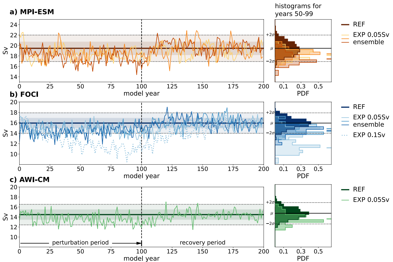
Figure 3. Response in Atlantic Meridional Overturning Circulation (AMOC) strength to the freshwater perturbation in (a) MPI-ESM, (b) FOCI, and (c) AWI-CM. Time series shows annual mean AMOC strength of the perturbation experiments. Long-term mean reference AMOC strength is shown as a bold straight line in the background of each panel along with shading for standard deviation (darker \pm 1\sigma , lighter \pm 2\sigma ) of PI-control interannual variability. Histograms on the right depict the respective distributions of the annual mean AMOC strength from the reference run using the entire time series and for the perturbation experiments using the last 50 years of the perturbation period (years 50–99); bin width is 0.5 Sv and consistent color coding is applied; a short horizontal line on the very right in the histogram plots marks the respective mean of each distribution. AMOC strength is defined as the vertical maximum of the zonal mean meridional stream function in the North Atlantic, here at 26.5^{\circ}\text{N} . Panel (b) also includes the results of the 0.1 Sv freshwater perturbation experiment with FOCI as dashed time series and bright blue histogram.
