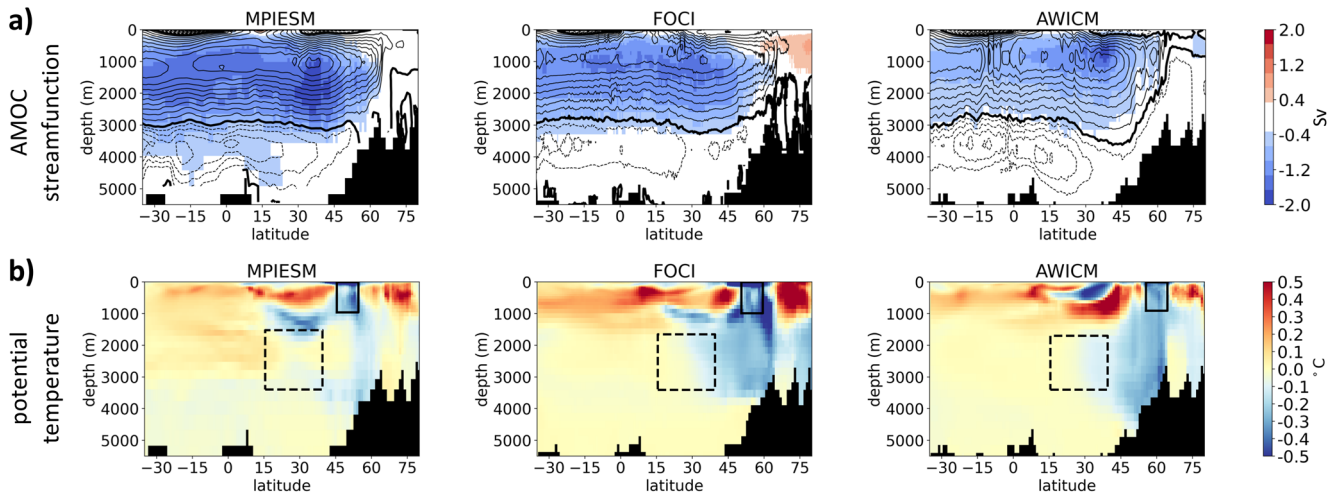
Figure 4. (a) The long-term mean reference state of the meridional overturning circulation in the Atlantic (black contours) and its response to the freshwater perturbation (colors). (b) Change in zonal mean potential temperature for the Atlantic Ocean due to freshwater perturbation. Differences are computed based on an average of years 50–99 of the experiments using ensemble means for MPI-ESM and FOCI.
